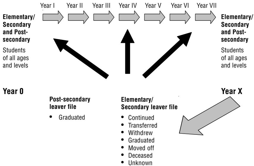
Figure 4: Cohort tracing model
