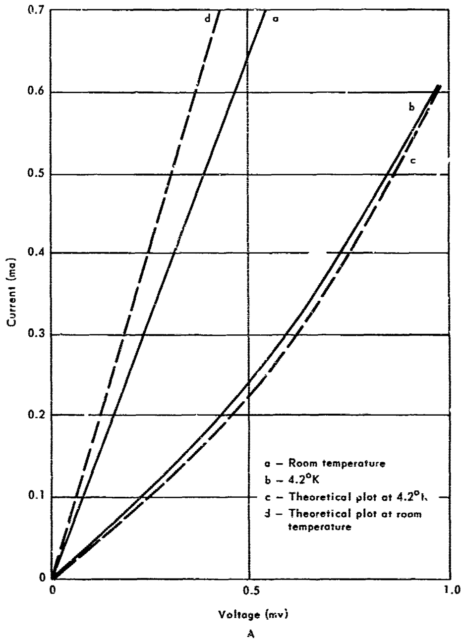
Figure 11. X-Y recorder plot of I-V characteristic of Al/Al 2 O 3 /Pb diodes.
