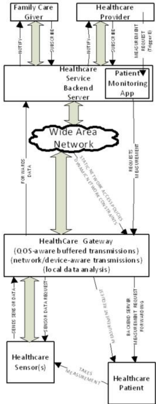
Figure 7-1 Healthcare Measurement Data Processing Flow
