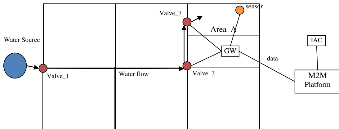
Figure 12-23 Smart Irrigation System
