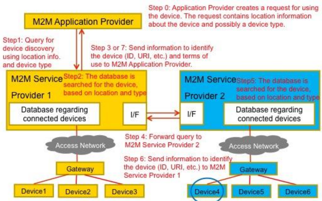
3819 Figure 12-20: High Level Illustration of Semantics discovery across M2M Service Providers
