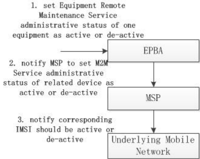
EP suspends or resumes Equipment Remote Maintenance Service
