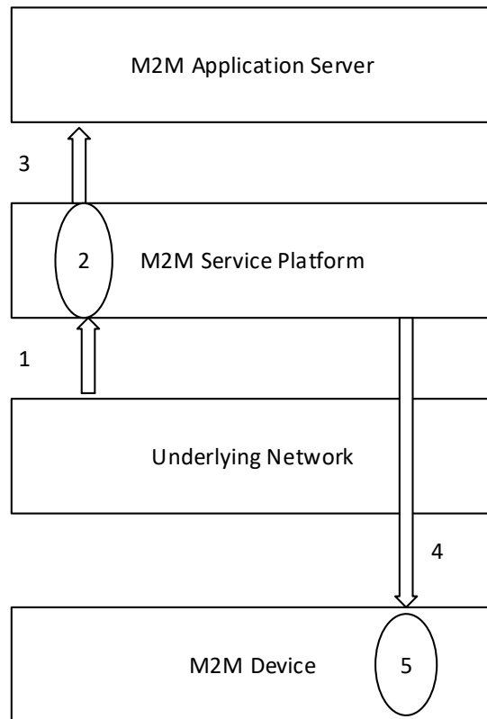
Figure 12-2: Normal Flow 1 of Data Traffic Management by Underlying Network Operator
