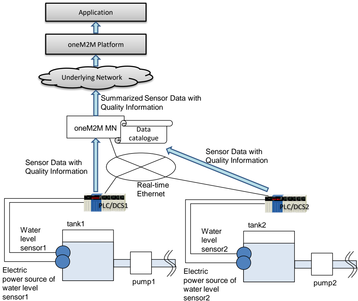
4383 4384 4385 Figure 12-28 Quality of sensor data
