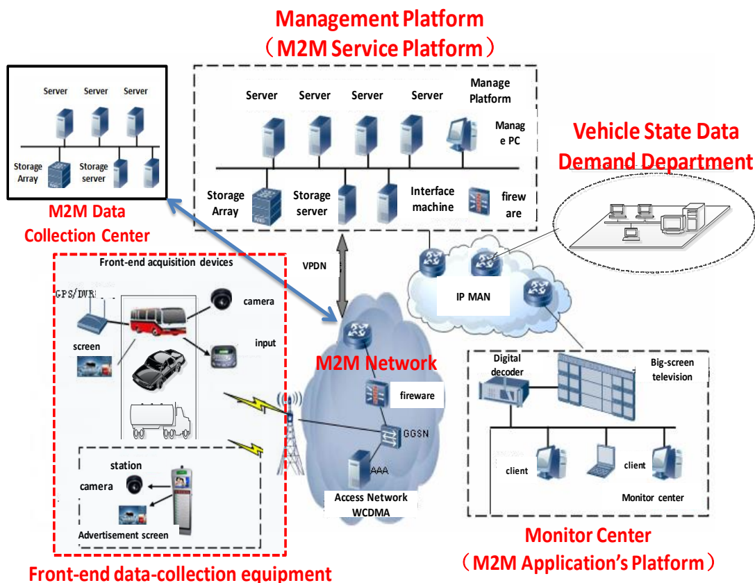
Figure 12-9 Vehicle Operation Management System
