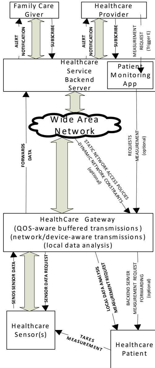
Figure 7-4 Local Gateway Data Analysis Flow
