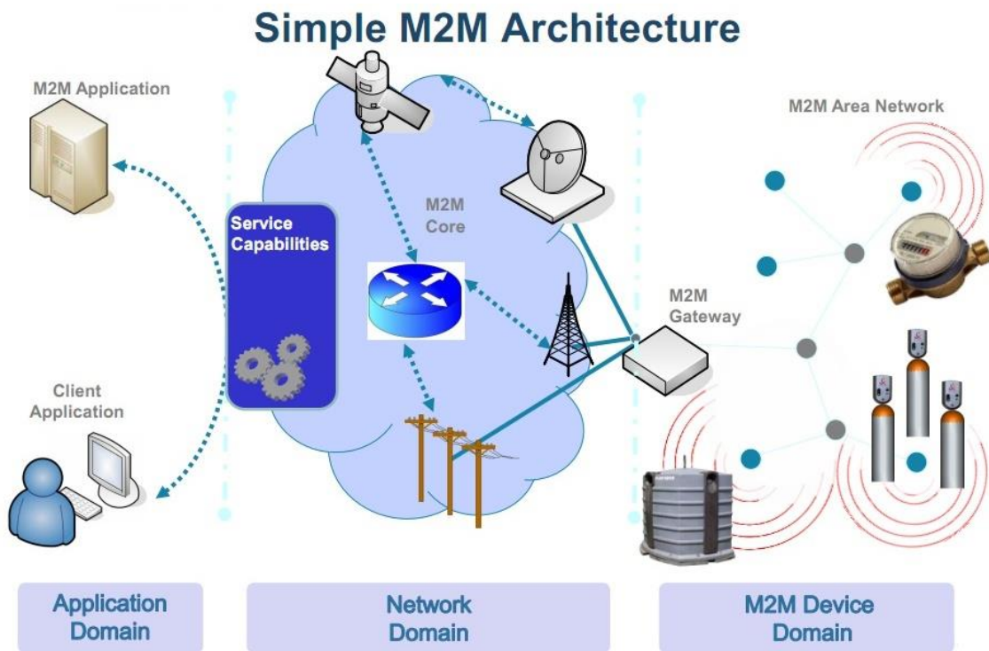
2773 Figure 12-2 Extended Smart Metering Configuration (source: ETSI)
