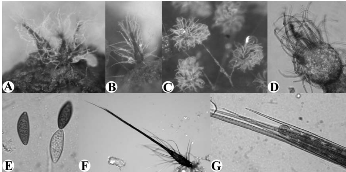
Fig. 1. A-B: Perithecia of Chaetomium ampullare . C-E. Chaetomium fusiforme . C-D: Perithecia. E: Young and mature ascospores. F-G. Chaetomium longicolleum . F: A perithecium. G: Terminal portion of the perithecium. Scale bar: A-B = 250 \mu m, C & F = 100 \mu m, D = 20 \mu m, E = 6 \mu m, G = 12 \mu m.
