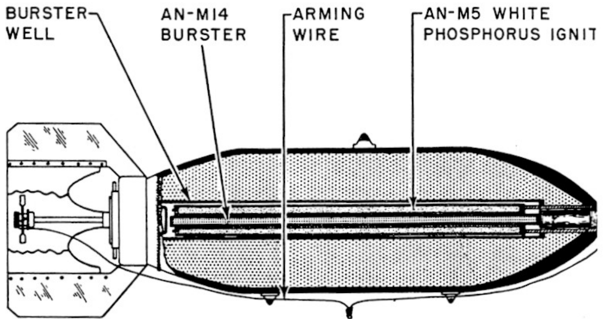
Figure 307. 500-pound Incendiary Bomb AN-M76
