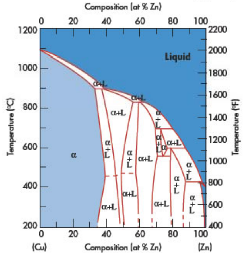
COPPER vs ZINC PHASE DIAGRAM (typical)
