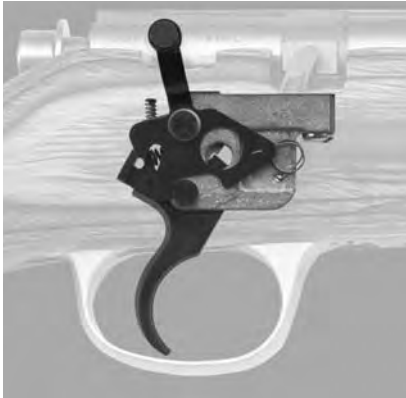
Marlin T-900 fire control system
