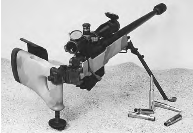
Model 93 folding model
