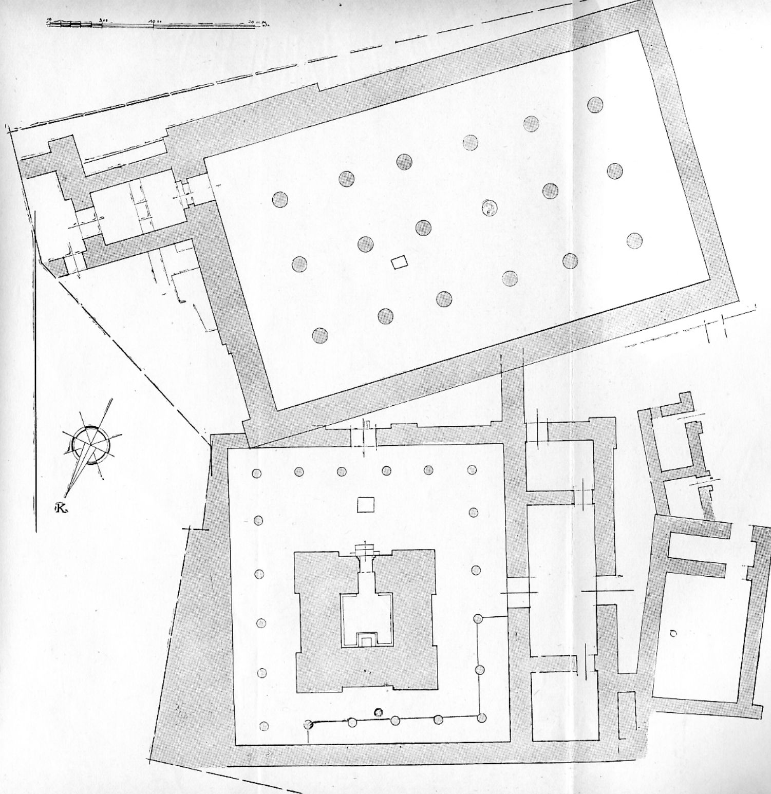
Plan. 2 Altintepe, Plan of the Temple and Audience-Hall
