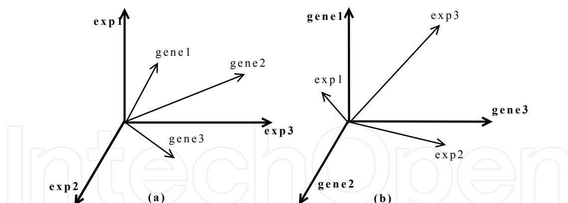
Fig. 1. Gene expression data interpretations: (a) a set of vectors representing expression values for one gene under different experiments and (b) a set of vectors representing expression values for multiple genes under a single experiment
