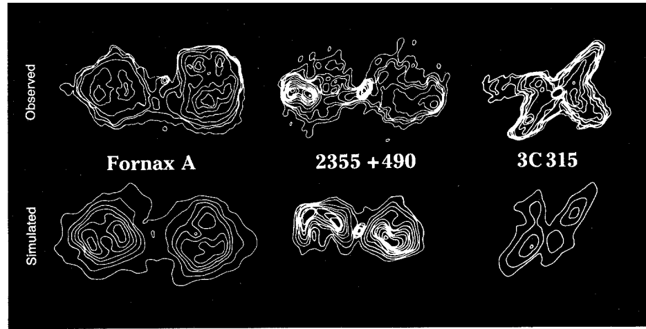
Supercomputer simulations of interactions between a pair of galaxy-size plasma filaments can reproduce the shapes of cosmic radio sources. The brightness maps of actual double radio galaxies in the top row show bewildering variety. Those at bottom are all from different stages of one simulation. The left figure corresponds to some 20 million years after the interaction begins; time increases toward the right plot, which depicts the simulated interaction some 40 million years later. These calculations suggest that apparently unrelated radio galaxies may be part of the same family, but at different stages of development.
