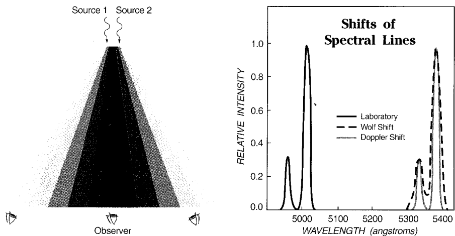
Left: Due to the Wolf effect beamed emission from two separate sources can interact and shift the wavelengths of lines in their spectra. The change can be redward or blueward by different amounts depending on the observer’s point of view, but from “head-on” the shift is to the red. This is a distinctly different process than the more familiar Doppler effect. Right: Here the two mechanisms are compared for the case of oxygen lines with a redshift of 0.07. However, the light sources involved in the Wolf effect are stationary , not fleeing the observer at 84 kilometers per second.
