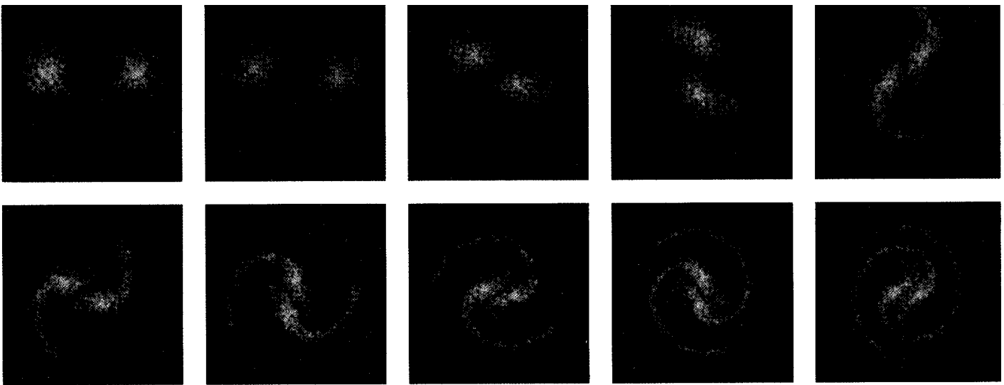
These images from a supercomputer simulation trace the development of spiral structure in two interacting plasma blobs over a span of nearly 1 billion years. At the start of the interaction at upper left the filaments are 260,000 light-years apart; all 10 panels are reproduced at the same scale. Simulations such as this can reproduce the full range of observed spiral-galaxy types using electromagnetic processes rather than gravitational ones. Unless otherwise noted, all illustrations are courtesy the author.
