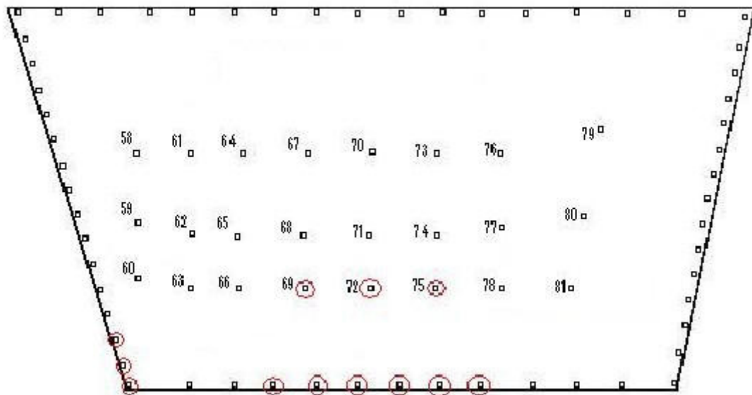
Diagram showing steel-column arrangement in WTC 7, view looking down on the roof. Circled columns were possibly damaged due to debris from WTC 1 collapse, some 350 feet
