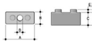
Distance plate
