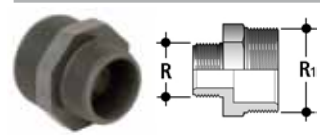
Barrel nipple reduced
