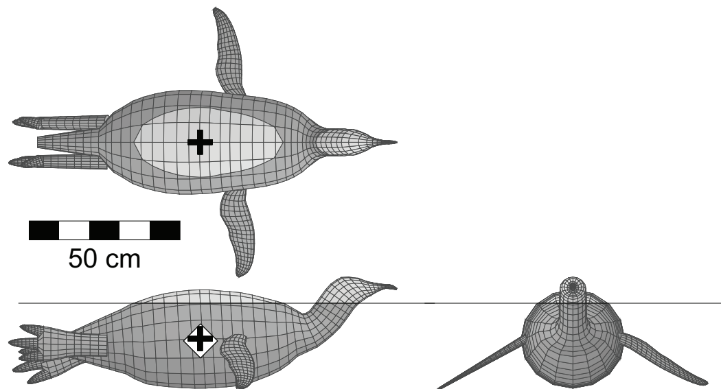
Figure 4 Dorsal, lateral and anterior views of the floating model of the emperor penguin ( Aptenodytes forsteri ). This example of an extant, aquatic, predatory theropod was done as another test of the validity of the methods employed with the extinct theropods. The model is in its final, equilibrium flotation state with a full lung, and replicates the situation seen in living emperor penguins floating at the water surface. Unlike all the other flotation tests, this one is done with seawater of density 1,026 gm/l. Colours and symbols as per Fig. 3. See Table 2 for details of the model and its floating state.
