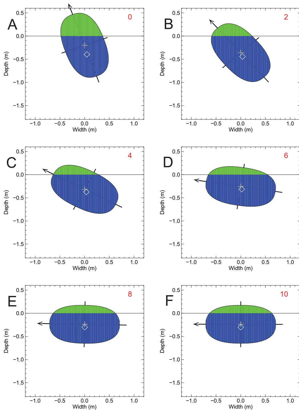
Figure 9 A test of lateral stability of the floating Spinosaurus model using a disk representing the cross-sectional area of the axial body at the position of the CM from the floating model of Fig. 5A. The disk was given a 20 sideways tip, but over the course of 10 simulation cycles it quickly rolled onto its side to a new position of stable equilibrium. Symbols and colors as per Fig. 7.
