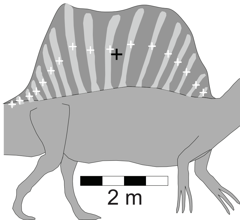
Figure 2 Detailed view of the Spinosaurus 'sail' and its associated neural spines (after Ibrahim et al. (2014) ). These details were used to determine the relative fractions of the bony and soft tissue components of the sail which were then used to compute the mass and center of mass of the sail. These latter two values were components in the final calculations of the mass, center of mass, and buoyant characteristics of the complete Spinosaurus model. Small white '+'s are the centroids of the individual spines. Large black '+' is the centroid of the entire sail. See 'Methods' for details of the calculations.
