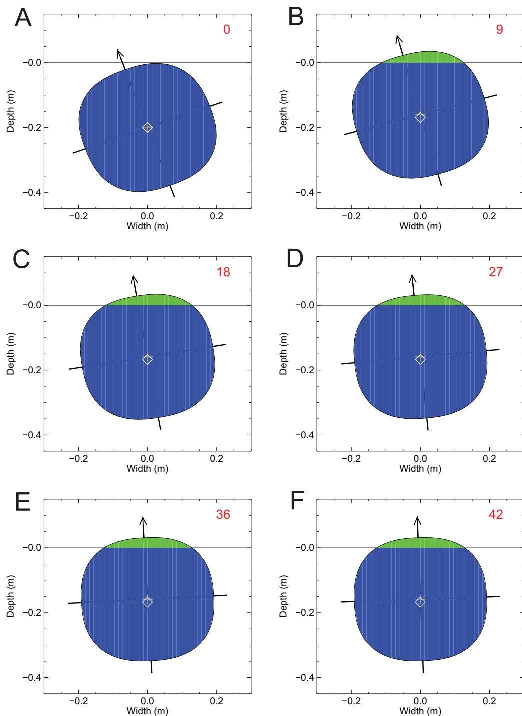
Figure 8 A test of the lateral stability of the floating Alligator model using a disk representing the transverse section of the immersed axial body at the position of the CM from the floating model of Fig. 3B. The disk was given a 20 sideways tip, but over the course of 42 simulation cycles it slowly returned to an upright orientation by passive self-righting. Symbols and colors as per Fig. 7.
