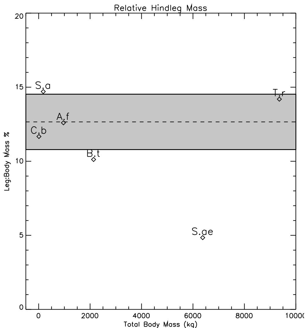
Figure 12 Relative mass fractions of the hindlimbs of the theropods in the present study highlighting the small size of the restored Spinosaurus hindlimbs. Dashed line represents the mean value of 12.6%. Grey band spans plus and minus one standard deviation about the mean. The Spinosaurus limb mass was not used in the calculation of the mean and standard deviation. A.f, Allosaurus fragilis ; B.t, Baryonyx (Suchomimus) tenerensis ; C.b, Coelophysis bauri ; S.a, Struthiomimus altus ; S.ae, Spinosaurus aegyptiacus ; T.r, Tyrannosaurus rex .
