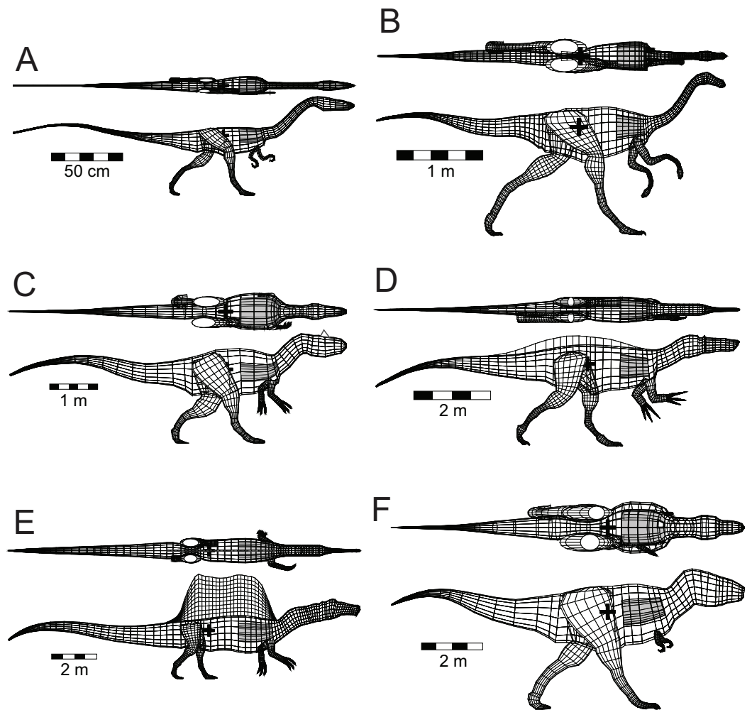
Figure 1 Dorsal and lateral views of the theropod models used for flotation tests. (A) Coelophysis bauri ; (B) Struthiomimus altus ; (C) Allosaurus fragilis ; (D) Baryonyx (Suchomimus) tenerensis ; (E) Spinosaurus aegyptiacus ; (F) Tyrannosaurus rex . Animals in order of increasing mass. Lung volumes and positions are represented by the dark grey cylinders in the chest regions. Black '+' denotes the computed center of mass. See Tables 1 and 2 for model image sources and model details, respectively.
