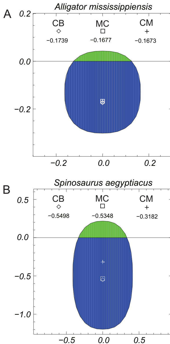
Figure 7 Graphical views of the metacentric heights (MC '□'), centers of buoyancy (CB '◇'), and centers of mass (CM '+') computed from the three-dimensional models. (A) Alligator mississippiensis ; (B) Spinosaurus aegyptiacus . A center of mass above the metacentric height indicates an unstable situation, which is clearly the case for the Spinosaurus . Stated measurements are relative to the water line and are in meters. See 'Methods and Results' sections for more details. Green indicates the 'dry' area above the waterline, while the blue is the 'wet,' immersed portion.
