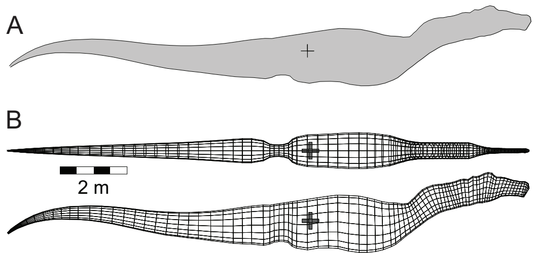
Figure 11 Centres of mass determinations for the axial body of Spinosaurus using two different methods. (A) Two-dimensional silhouette with constant areal density; (B) three-dimensional mesh without lung cavity or air sacs. In neither case does the CM reside at the midpoint of the trunk region as claimed by Ibrahim et al. (2014) . See ‘Discussion’ section. Full-size DOI: 10.7717/peerj.5409/fig-11
