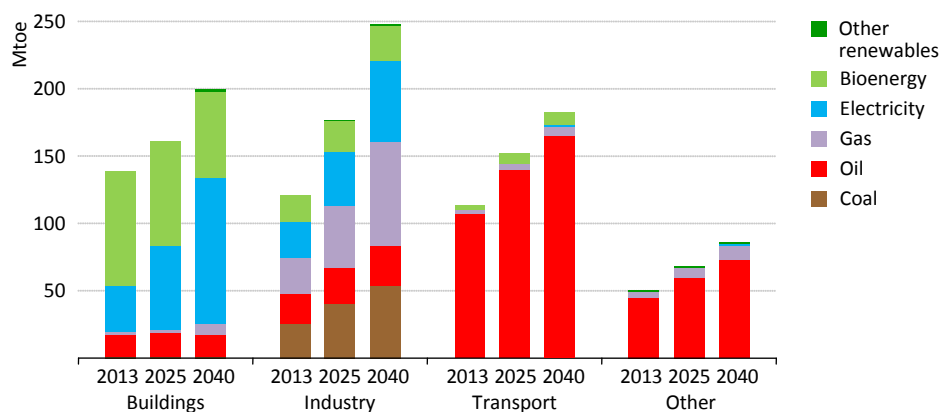
Figure 2.6 ▶ Final energy consumption by fuel and sector in Southeast Asia
