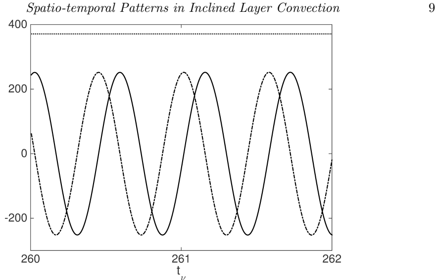
Figure 6: The coefficients A (horizontal upper dotted line), B(t) (dash-dotted) and C(t) (solid line) in (4.1) as function of time in units of T_s ; B(t), C(t) are multiplied by a factor of four for better visualisation.
