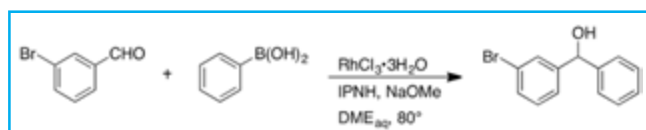
Figure 2c. Boronic acid approach to aryl portion of Gliflozins.
