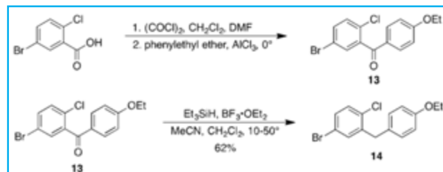
Figure 2d. Friedel-Crafts approach to aryl portion of Gliflozins.
