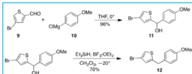
Figure 2a. Grignard approach to aryl portion of a Gliflozins.
