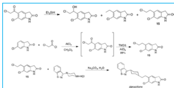
Figure 3a. Reduction of the benzoyl carbonyl in the synthesis of Ziprasidone.
