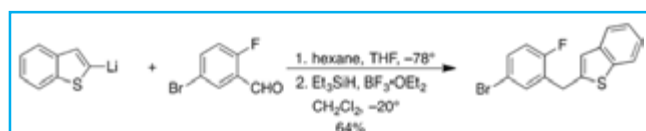
Figure 2b. Lithium reagent approach to aryl portion of a Gliflozins.
