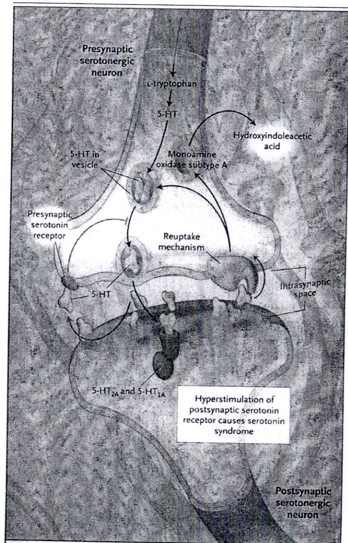
Figure 3. Serotonin Biosynthesis and Metabolism.
