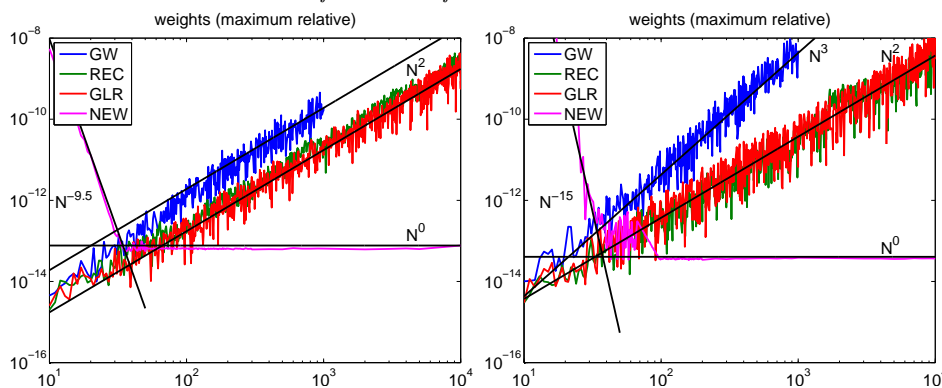
FIG. 4.5. Observed maximum relative errors in the weights in Gauss–Jacobi for \alpha = 0.1 , \beta = -0.3 (left) and \alpha = 2 , \beta = -0.75 (right). As with the analogous plot for the Gauss–Legendre weights, we see the error in the new algorithm is independent of n .
