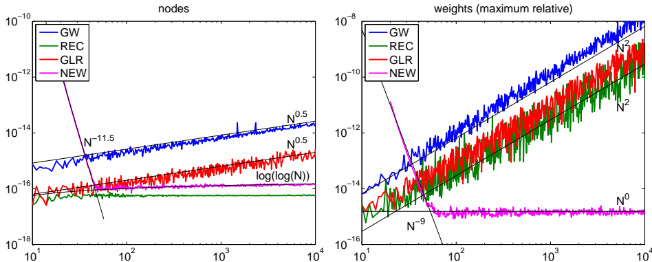
FIG. 2.1. Observed error in computing Gauss–Legendre nodes and weights. GW uses the dgau routine from the ORTHOPOL library [16], REC is glfixed from the GSL library [12], GLR is a Fortran implementation supplied by the authors of [21], and NEW is a MATLAB implementation of the algorithm presented in this paper. The C and Fortran codes are interfaced with MATLAB via MEX files. See Figure 4.3 for analogous plots of quadrature error and computational time.
