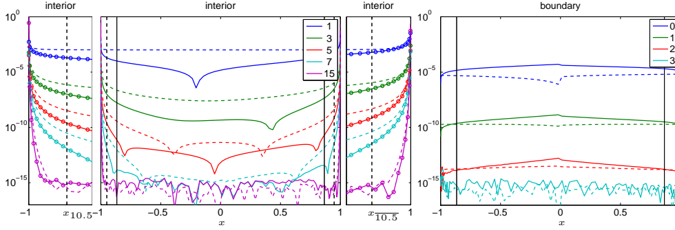
FIG. 3.7. Error in evaluating the Jacobi polynomial P_{100}^{(0.1, -0.3)} and its derivative using the asymptotic formulae (3.24) and (3.27). Clearly the interior formula (3.24) can in practice be used much closer to the boundary than the convergence region of \cos(5\pi/6) < x < \cos(\pi/6) suggests (vertical solid line). The first and third panels show that, as with the Legendre polynomial, the boundary formula is only needed for the ten nodes nearest the boundary (vertical dashed lines).
