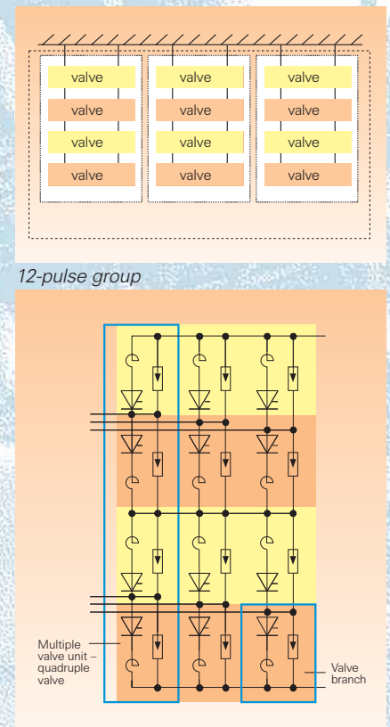
Fig. 5.1-1: Principle circuit diagram of a 12-pulse group consisting of three quadruple valves
