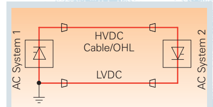
Fig. 2-5: Monopole with metallic return path
