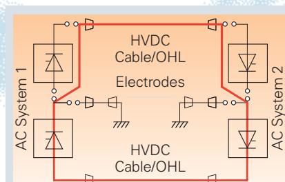
Fig. 2-8: in monopolar metallic return operation (converter pole outage)
