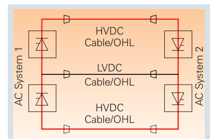
Fig. 2-9: in bipolar balanced operation (normal)
