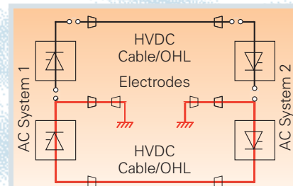
Fig. 2-7: in monopolar ground return operation (converter pole or OHL outage)
