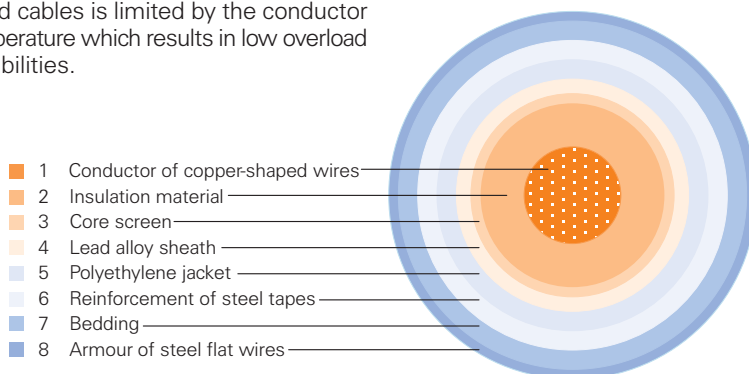
Fig. 5.6.2.2-1: Mass-impregnated cable
