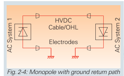
Fig. 2-4: Monopole with ground return path
