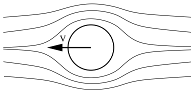
FIG. 10: A body moving in viscous fluid.
