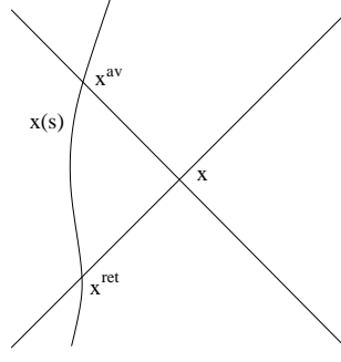
FIG. 8: The observer at x receives the signal emitted from the point x^{\text{ret}} or x^{\text{av}} for the retarded or the advanced propagation, respectively.
