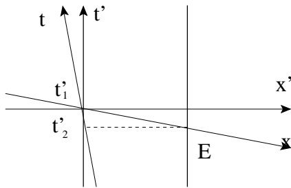
FIG. 5: Lorentz contraction.
