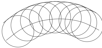
FIG. 7: Huygens principle for a wave front.
