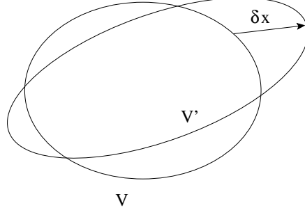
FIG. 6: Deformation of a space-time region.
