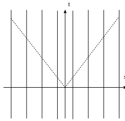
FIG. 1: Synchronization of clocks to the one placed at the origin.
