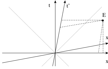
FIG. 4: Lorentz transformations.
