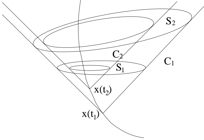
FIG. 9: Energy momentum emitted by an accelerating charge
