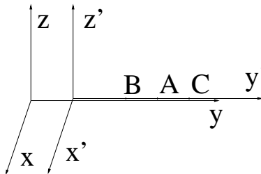
FIG. 1: Synchronization of clocks to the one placed at the origin.
