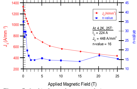
Figure 7: In this figure the current density versus magnetic field at a temperature of 4.2 K (LHe) is plotted. At 25 T a current density of 448 A/mm 2 can be supported, a value that comes close to the 600 A/mm 2 needed for field propulsion.
