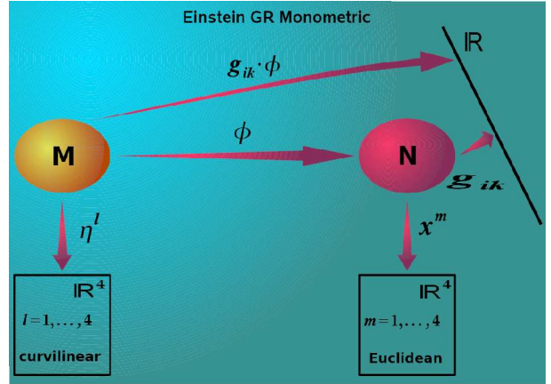
Figure 1: In GR the metric tensor is computed using a mapping from manifold M (curvilinear coordinates \eta^I ) in spacetime \mathbb{R}^4 to manifold N in spacetime \mathbb{R}^4 (Euclidean coordinates x^m ). Calculating the components of the metric tensor as well as lengths, areas, and volumes from the metric tensor a mapping to the set of real numbers is needed [17]. This kind of mapping delivers one type of metric tensor that is responsible for gravity, appearing on the LHS of the Einstein field equations.
