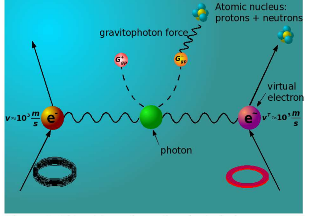
Figure 6: This picture shows the physical phenomenon of gravitophoton pair production from the vacuum, using some kind of Feynman diagram. Gravitophoton production from photons is the cause of the Heim-Lorentz force. The brown sphere on the LHS corresponds to the electrons moving in the current loop, Fig. 5. The sphere on the RHS corresponds to the rotating ring above the current loop, having a circumferential speed of some 10^3 m/s. In the rotating torus virtual electrons are produced by the vacuum, partially shielding the proton charge of the nuclei. At a distance smaller than the Compton wavelength of the electron away from the nucleus, the proton charge increases, since it is less shielded. According to Eq. (6) a value of A larger than 0 is needed for gravitophoton production. As was shown in [12], however, a smaller value of A is needed to start converting photons into gravitophotons to make the photon metric vanish, termed \tilde{A} = v_k v_k^T / c^2 \approx 10^{-11} where v is the velocity of the electrons in the current loop and v^T is the circumferential speed of the torus. From the vanishing photon metric, the metric of the gravitophoton pairs is generated, replacing the value of A by the LHS of Eq. (6) and inserting it into the equation for the gravitophoton metric. This value is then increased to the value of A in Eq.(6). Experimentally this is achieved by the current loop (magnetic coil) that generates the magnetic vector and the tensor potential at the location of the virtual electron in the rotating torus, producing a high enough product v v^T , see Eq. 32 in [13]. The coupling constants of the two gravitophoton particles are different, and only the negative (attractive) gravitophotons are absorbed by protons and neutrons, while absorption by electrons can be neglected. This is plausible since the negative (attractive) gravitophoton contains the metric of the graviton, while the positive repulsive gravitophoton contains the metric of the quintessence particle that does only interact extremely weakly with matter. Through the interaction of the attractive gravitophoton with matter it becomes a real particle and thus a measurable force is generated (see upper part of the picture).
