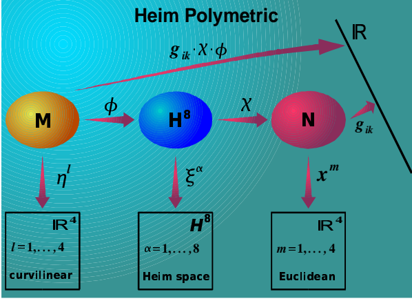
Figure 2: Einstein's goal was the unification of all physical interactions based on his principle of geometrization, i.e., having a metric that is responsible for the interaction. This principle is termed Einstein's geometrization principle of physics (EGP). To this end, Heim and Dröschler introduced the concept of an internal space, denoted as Heim space H^8 , having 8 dimensions. Although H^8 is not a physical space, the signature of the additional coordinates being timelike (negative), these invisible internal coordinates govern events in spacetime. Therefore, a mapping from manifold M (curvilinear coordinates \eta^l ) in spacetime \mathbb{R}^4 to internal space H^8 and back to manifold N in spacetime \mathbb{R}^4 (Euclidean coordinates x^m ) must be used to properly describe the physics. This is a major deviation from GR and leads to a poly-metric. For the construction of the poly-metric see Eqs. (2) and (4).
