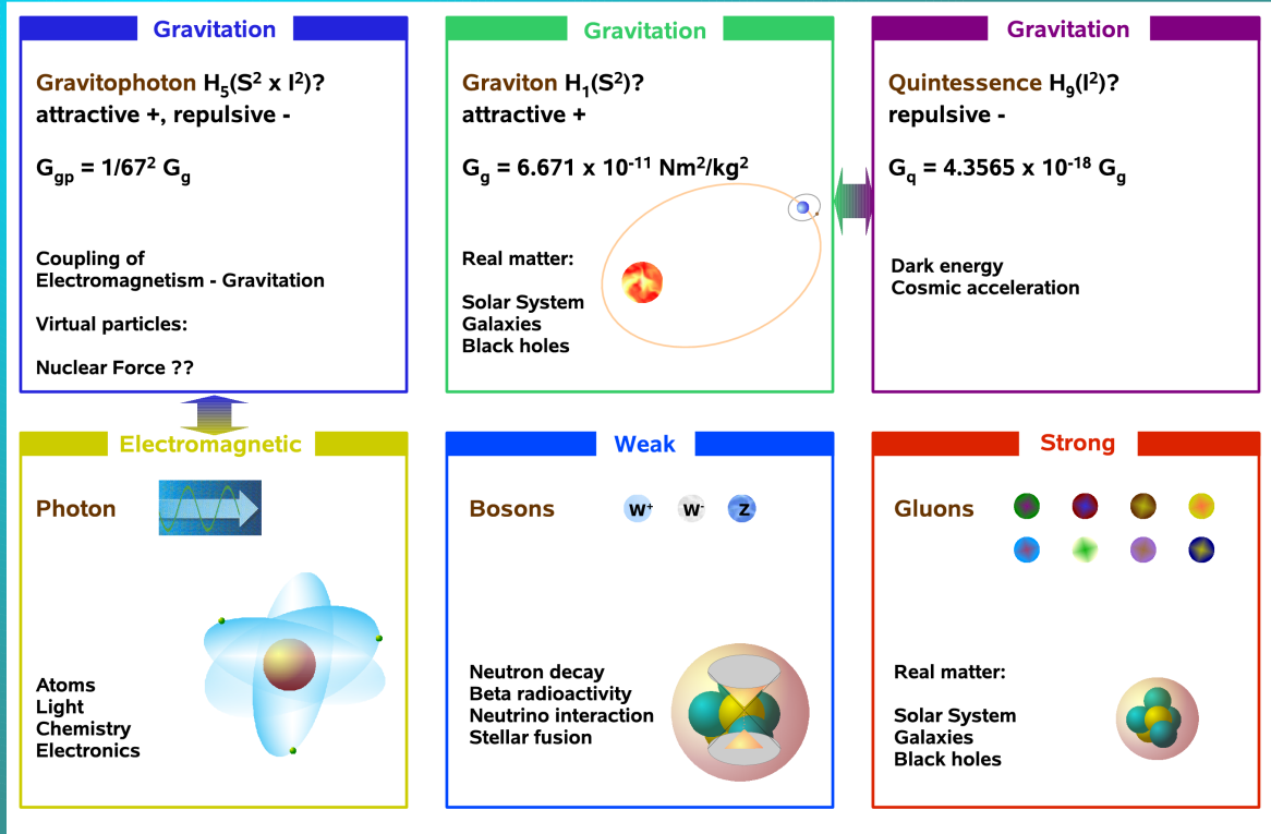
Figure 2. EHT predicts, as one of its most important consequences, two additional, gravitational like interactions and the existence of two messenger particles, termed gravitophoton and quintessence. That is, there is a total of six fundamental physical interactions. The name gravitophoton has been chosen because of the type of interaction, namely the transformation of the electromagnetic field (photon) into the gravitational field (gravitophoton). The arrow between the gravitophoton and electromagnetic boxes indicates the interaction between these messenger particles that is, photons can be transformed into gravitophotons. In the same way the quintessence interaction can be generated from gravitons and positive gravitophotons (repulsive force). It is assumed that first a neutral gravitophoton is generated that decays into a pair of negative (same sign as gravitational potential) and positive gravitophotons.
