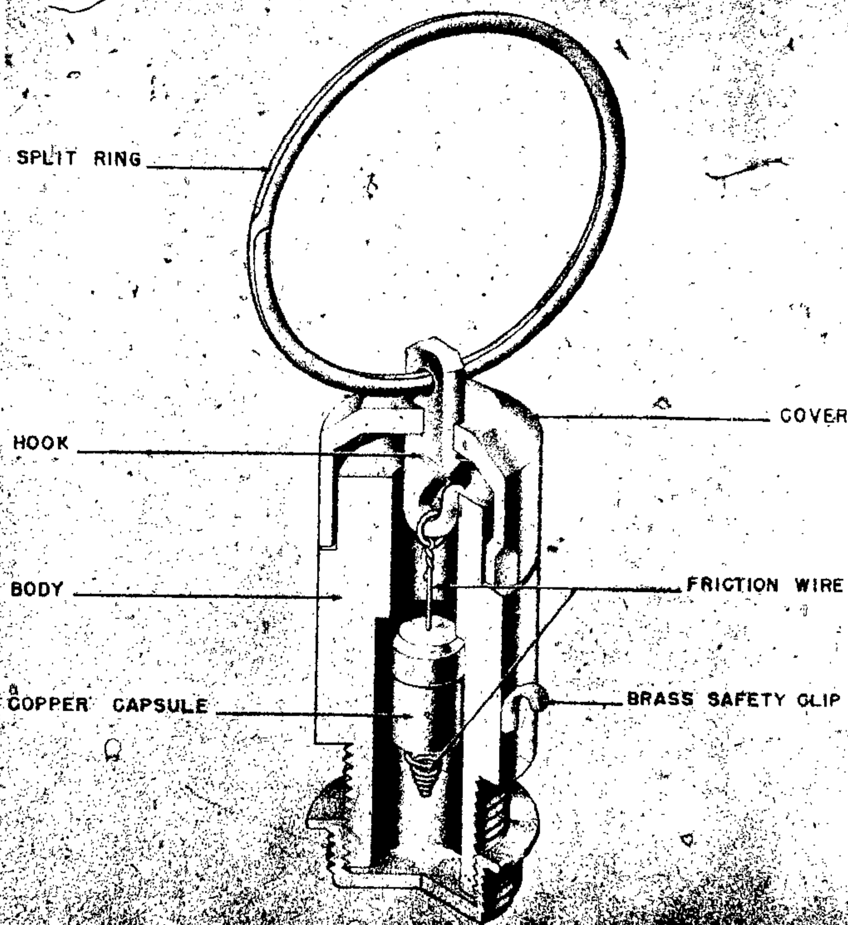
Figure 253—ANZ-29 Friction Igniter Pull Type
