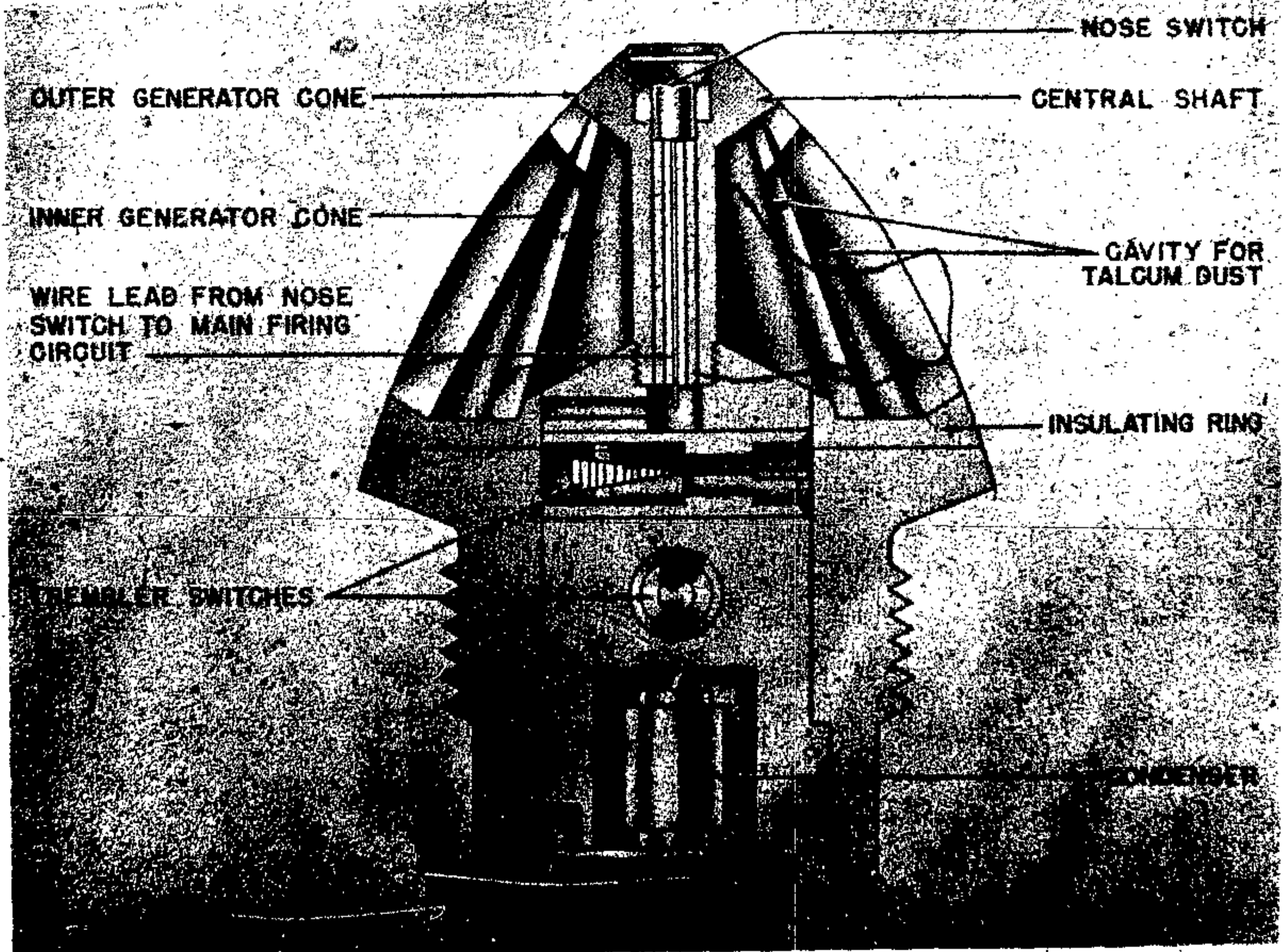
Figure 191A—Dust Fuze for SD-10 Bomb
