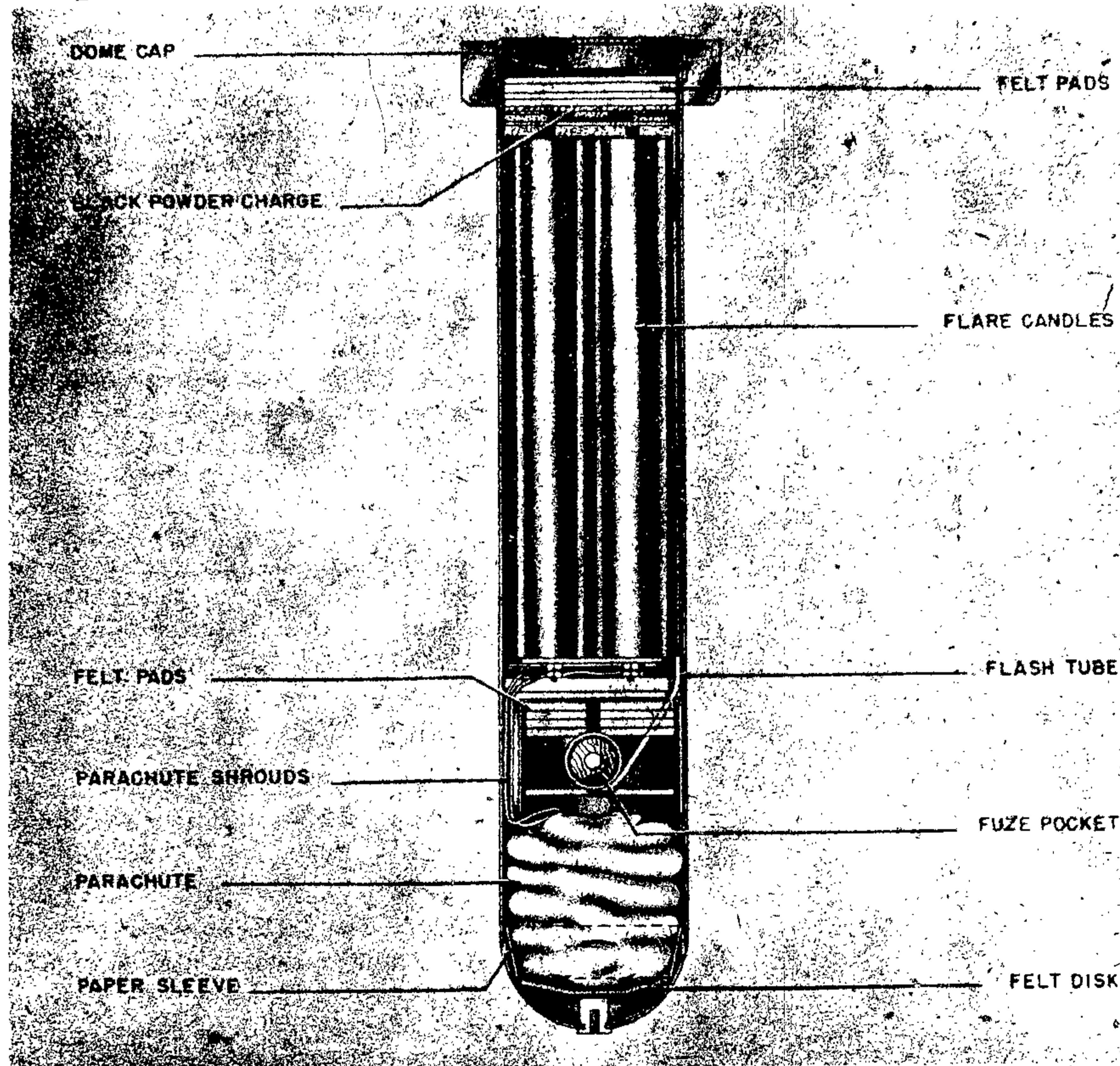
Figure 72—LC 50 F Ausf. C Parachute Flare
