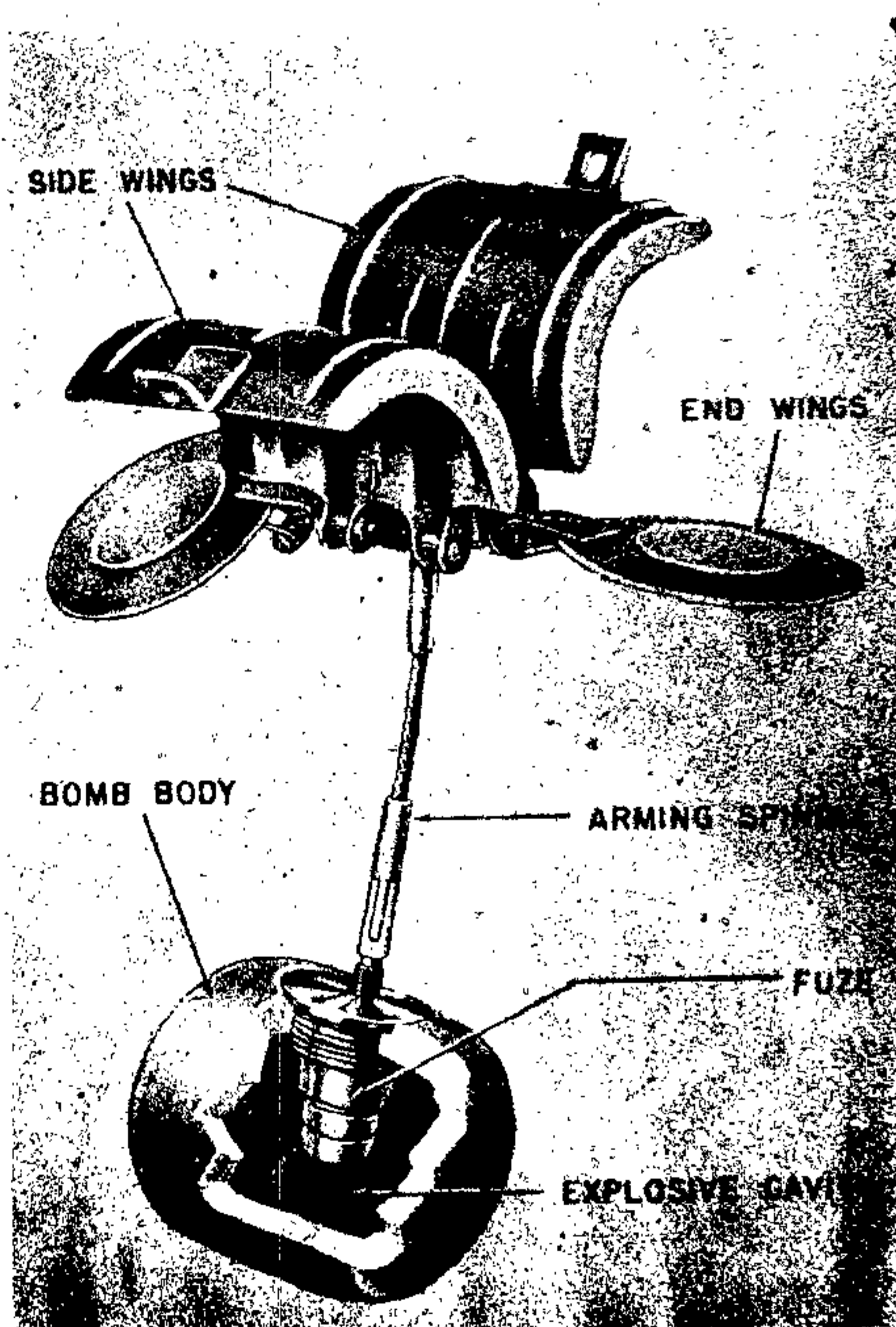
Figure 39B—SD 2-Kg "Butterfly" Bomb
