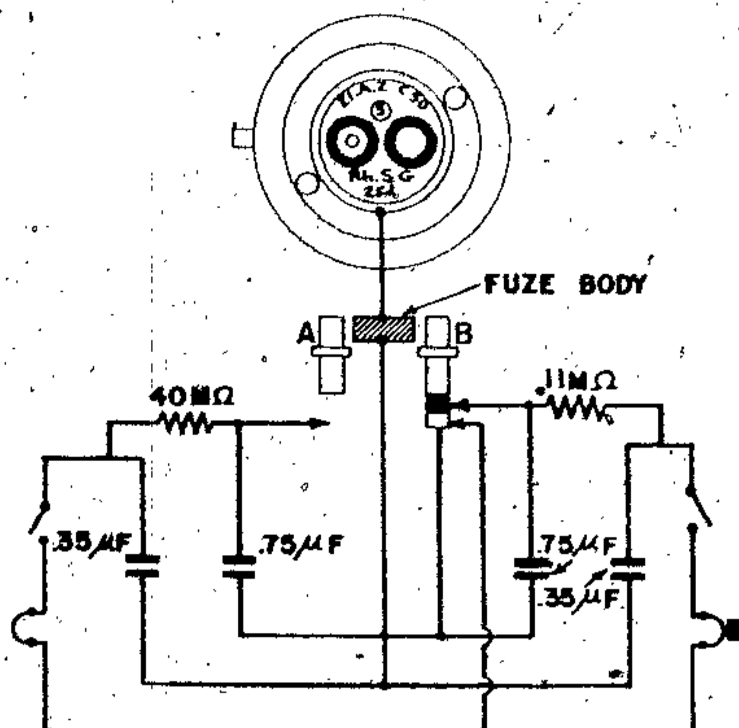
Figure 138—(5) Electrical Impact Fuze
