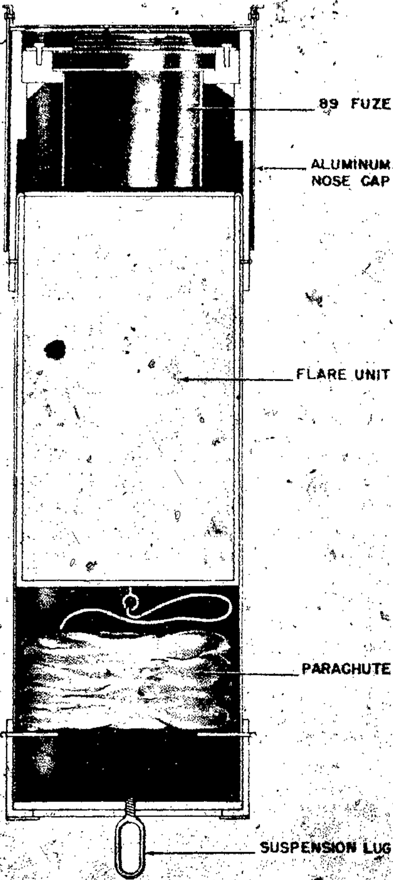
Figure 70—LC 10 Single Candle Parachute Flare
