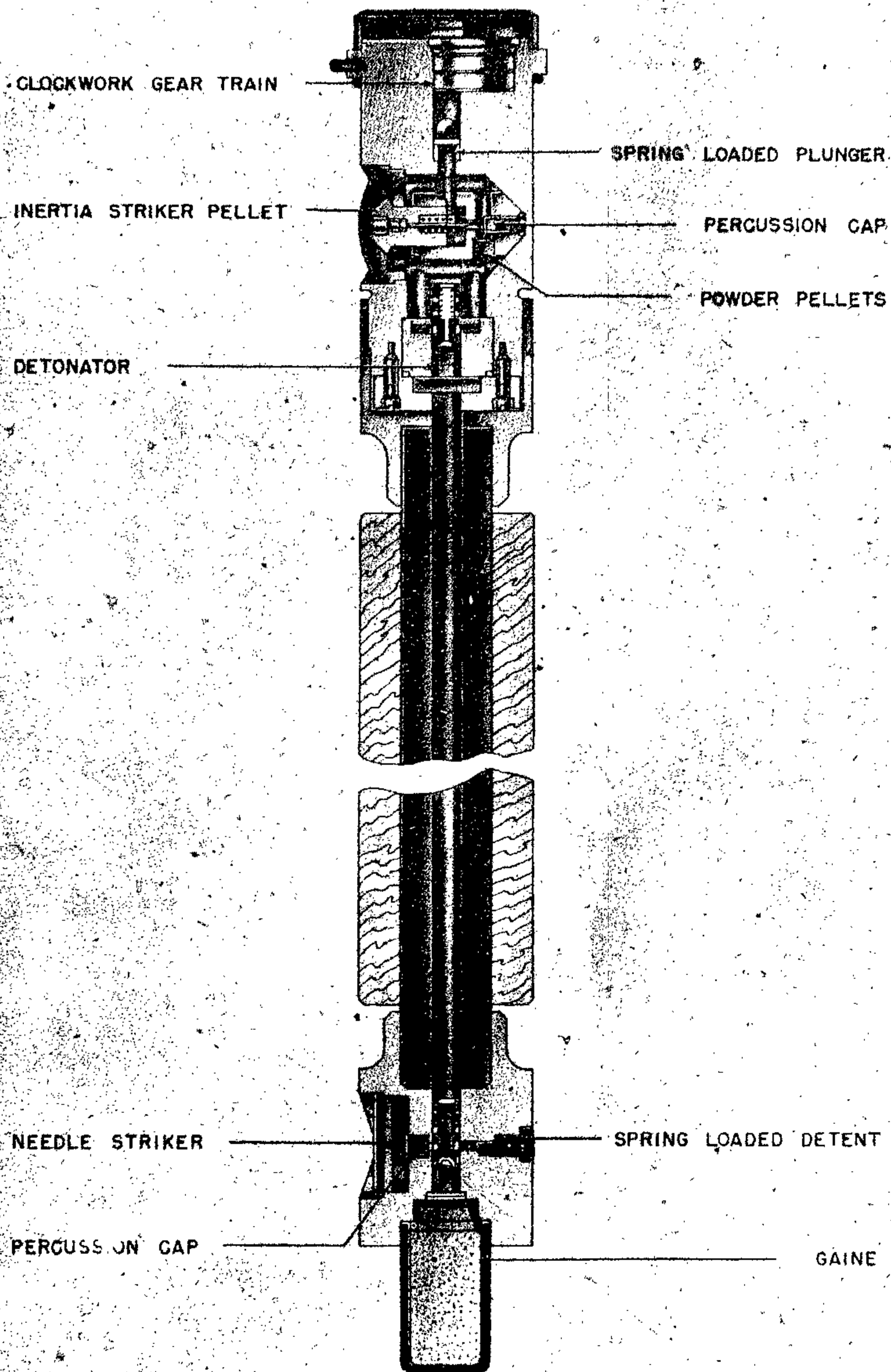
Figure 136—(24)A Mechanical Impact Fuze with Antibreak-up Switch
