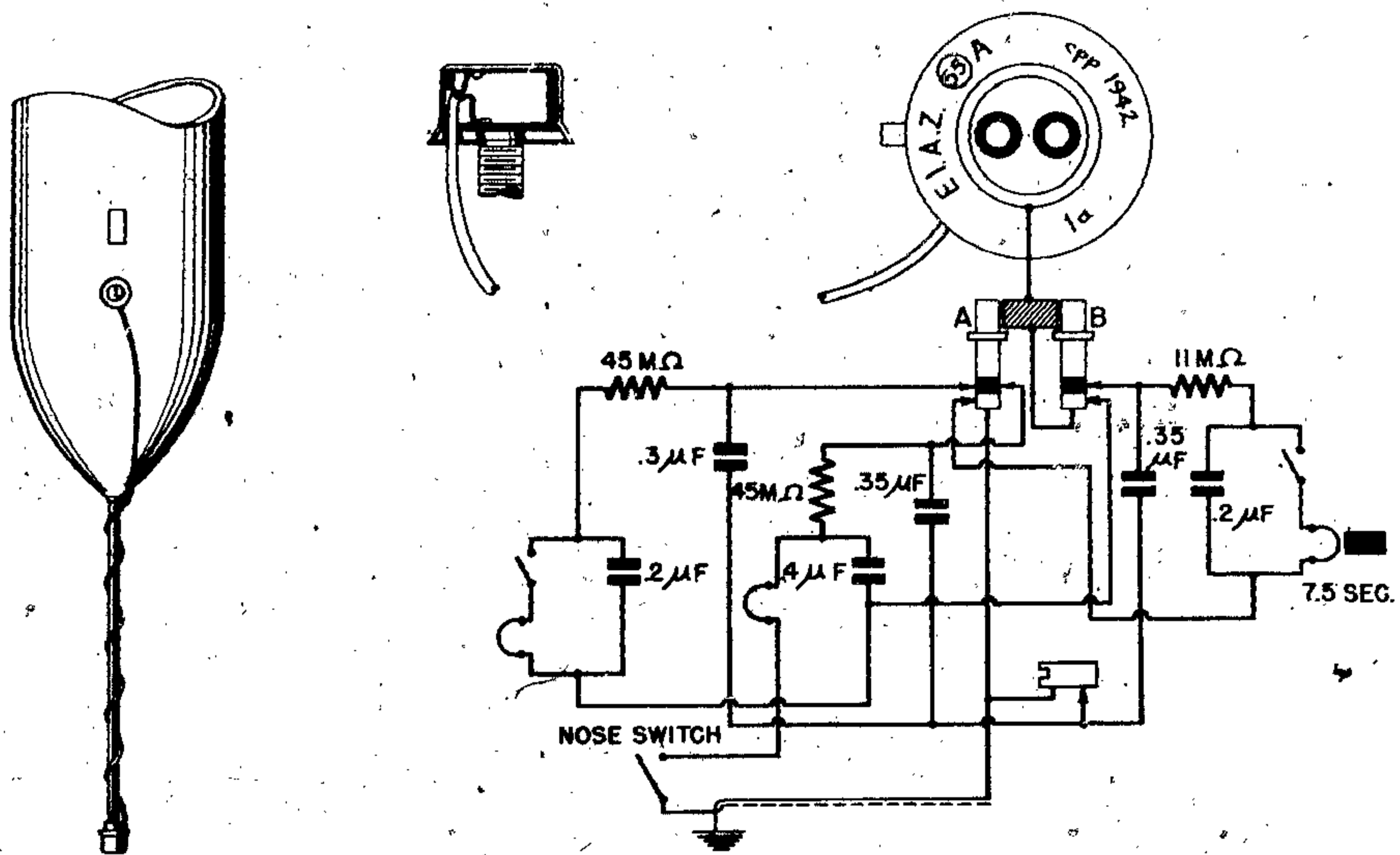
Figure 146—(55)A Electrical Impact Fuze
