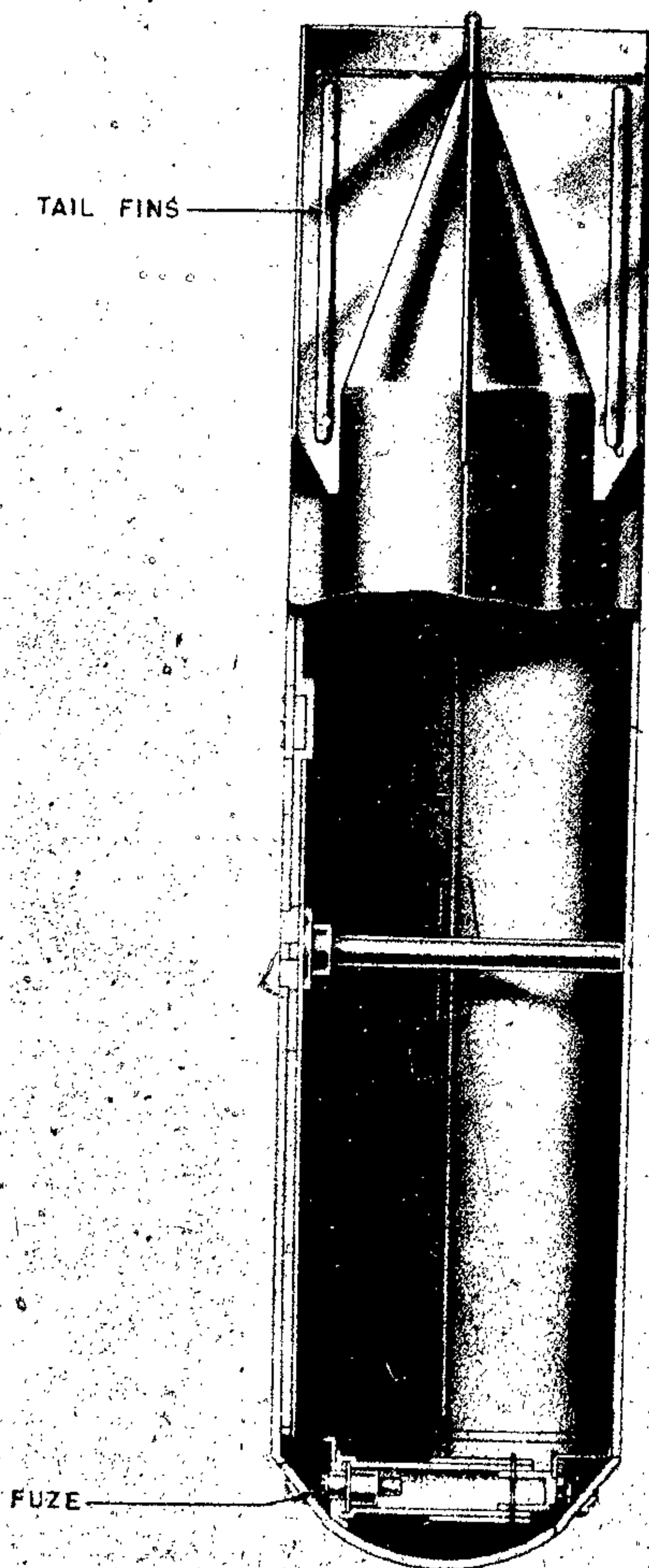
Figure 106—AB 250-2 Container
