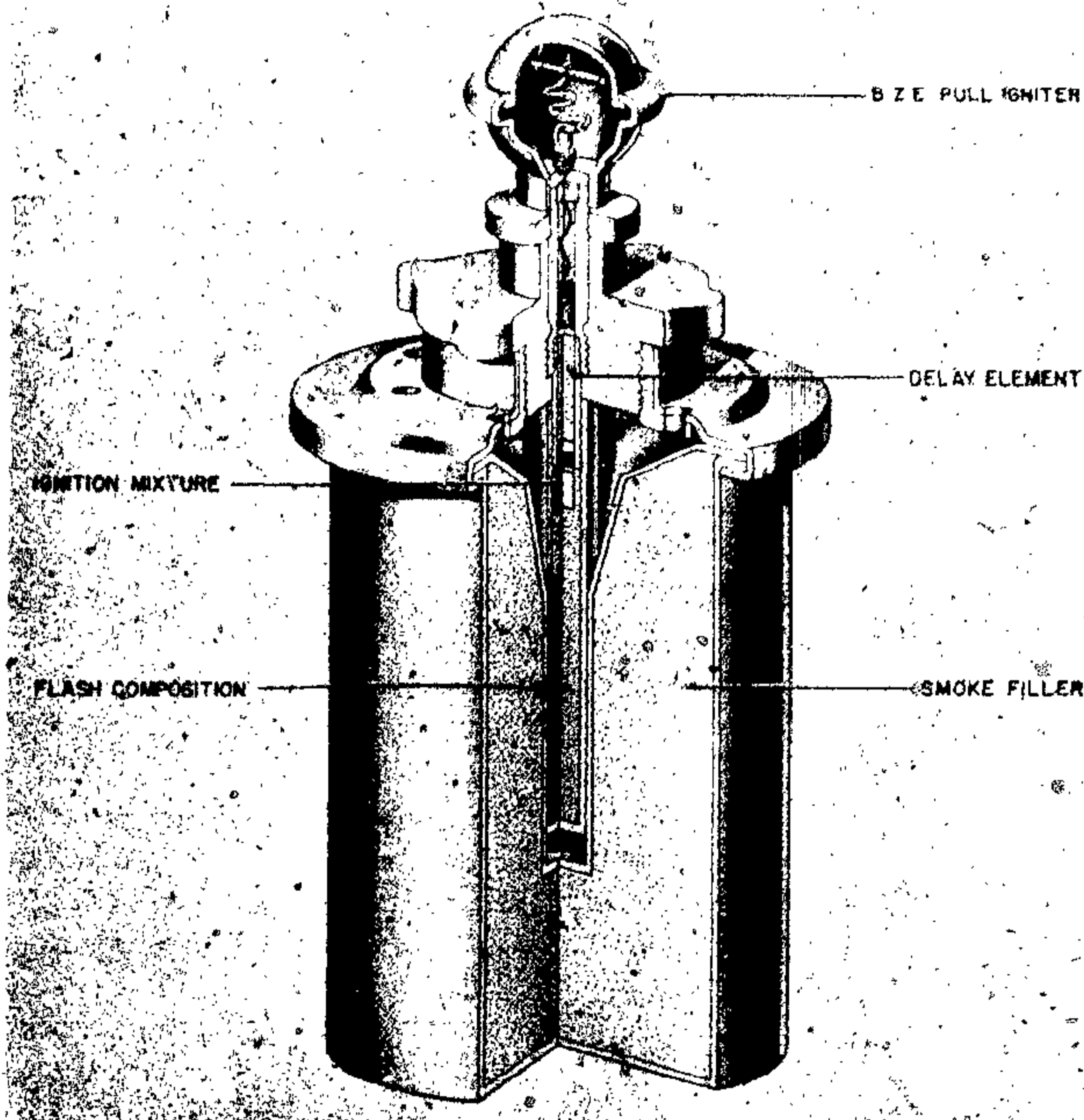
Figure 291—Type 41 Smoke Hand Grenade
