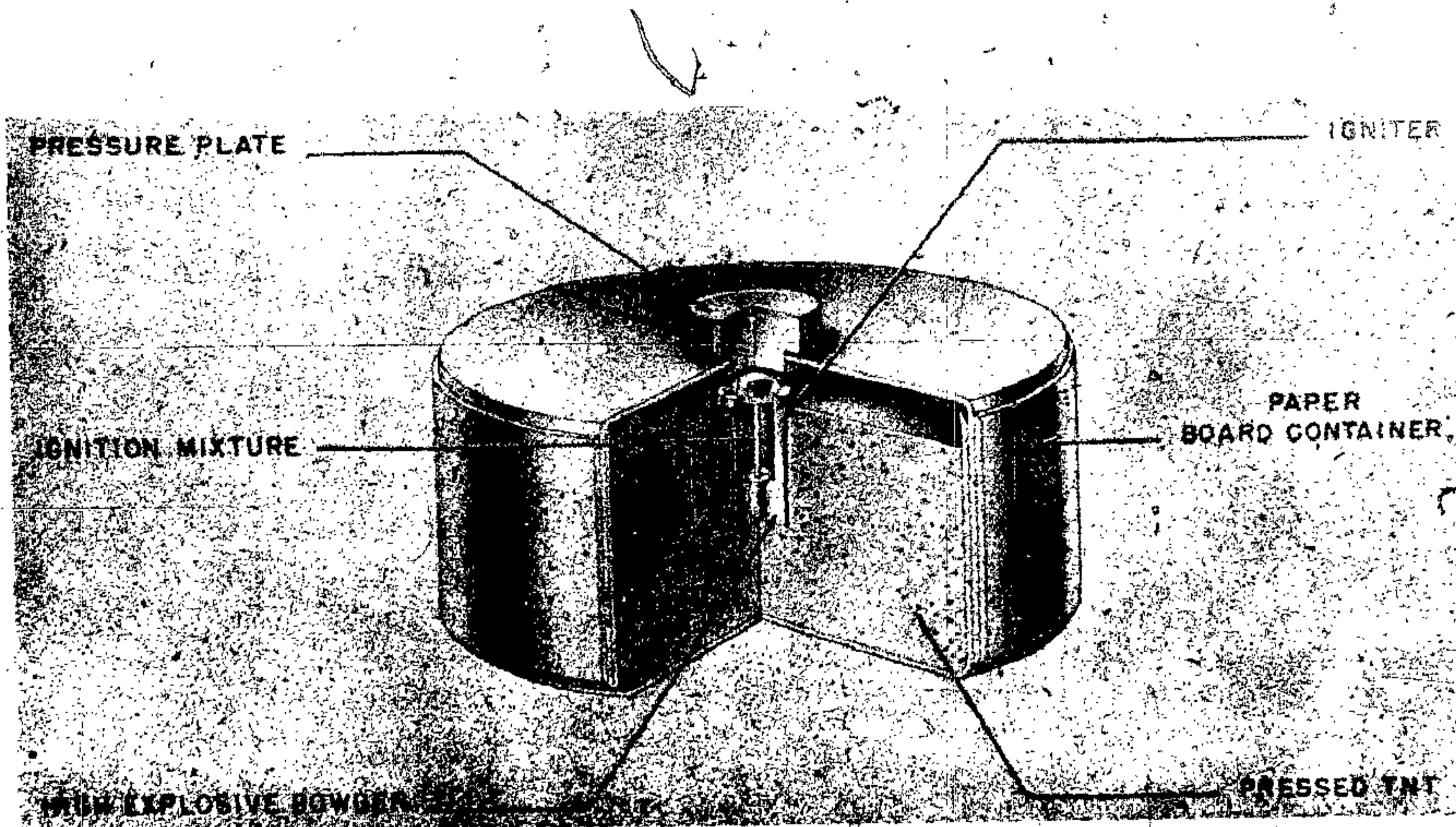
Figure 224—Pappmine Antitank Mine
