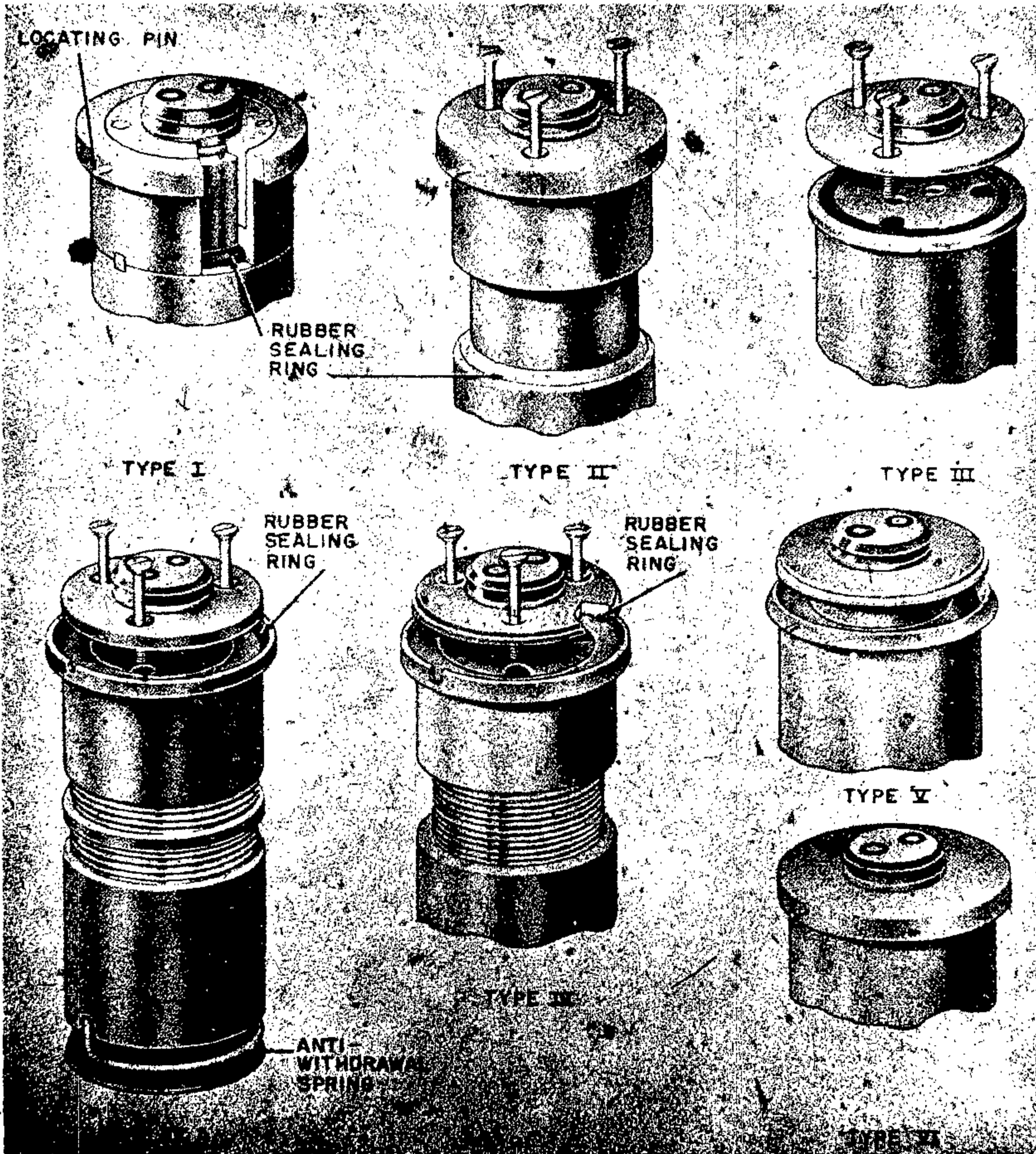
Figure 119—Types of Fuze Construction
