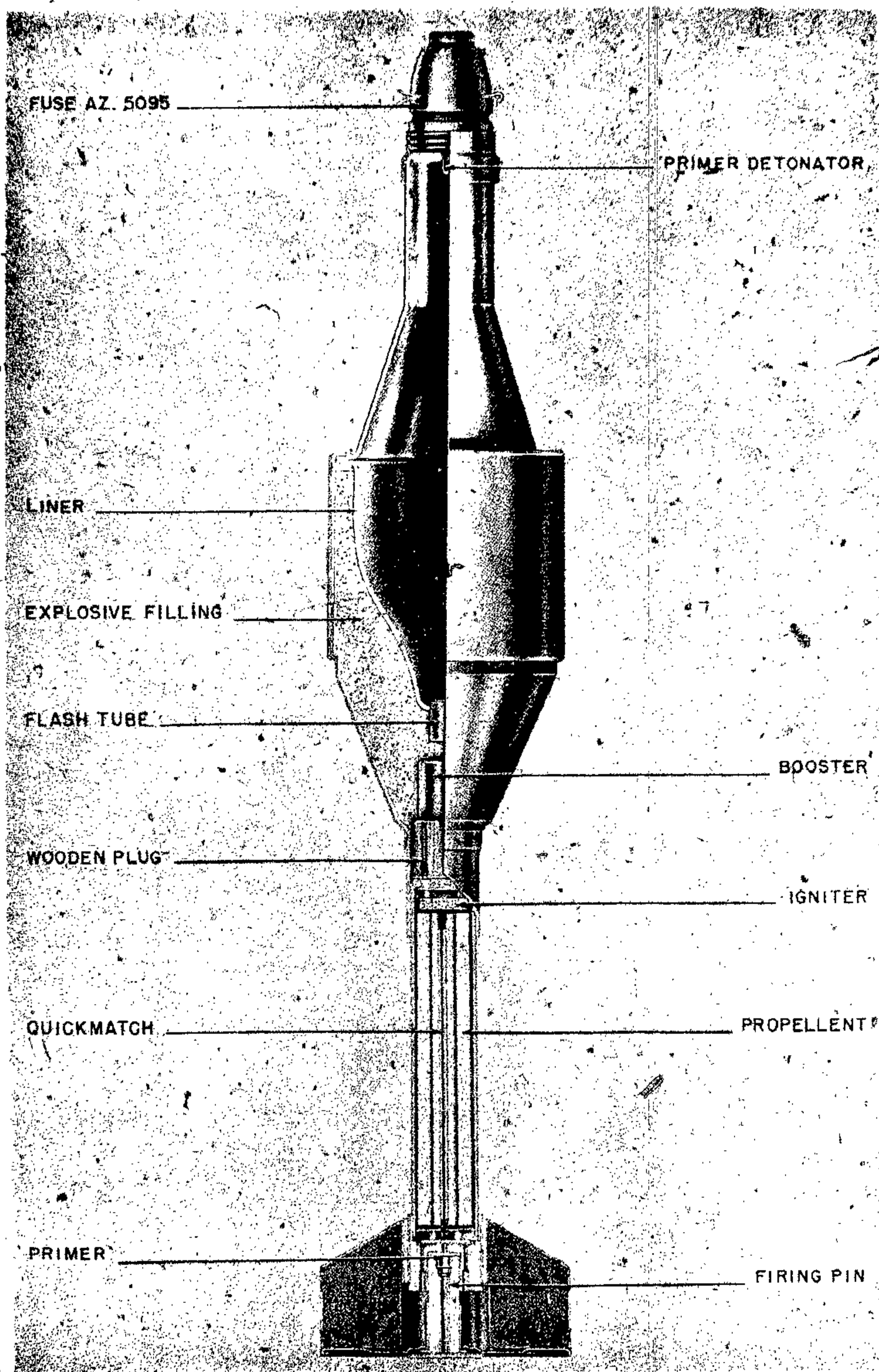
Figure 210—8.8-cm Hollow Charge Antitank Rocket
