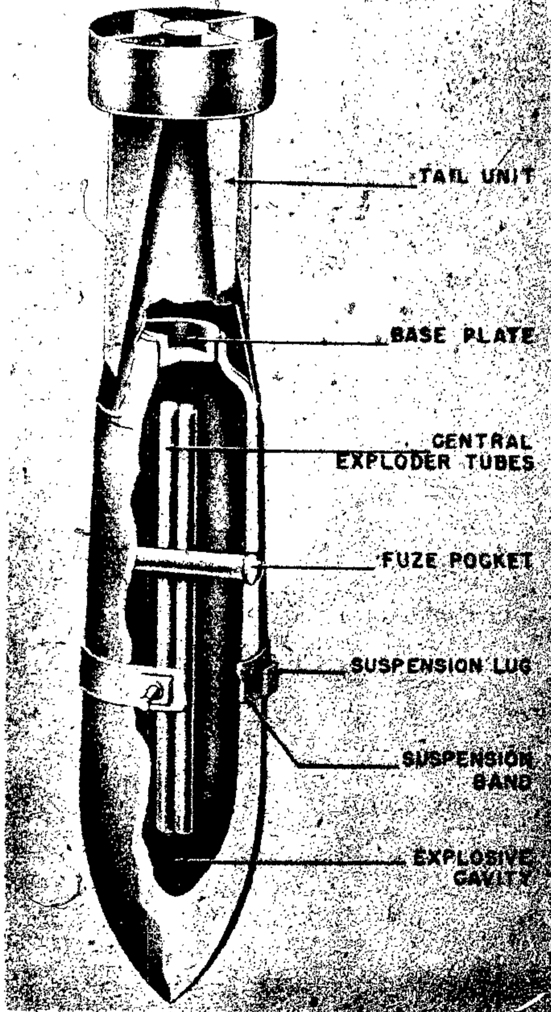
Figure 31—PC 1400-Kg Bomb
