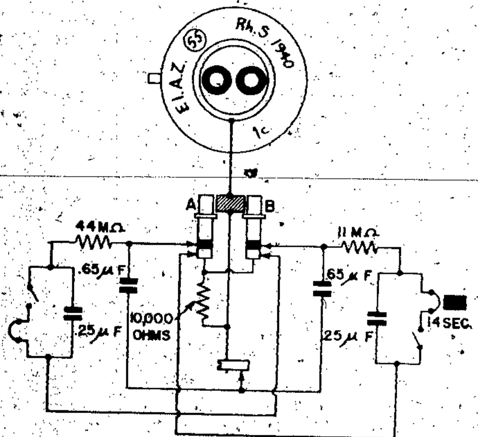
Figure 145—(55) Electrical Impact Fuze
