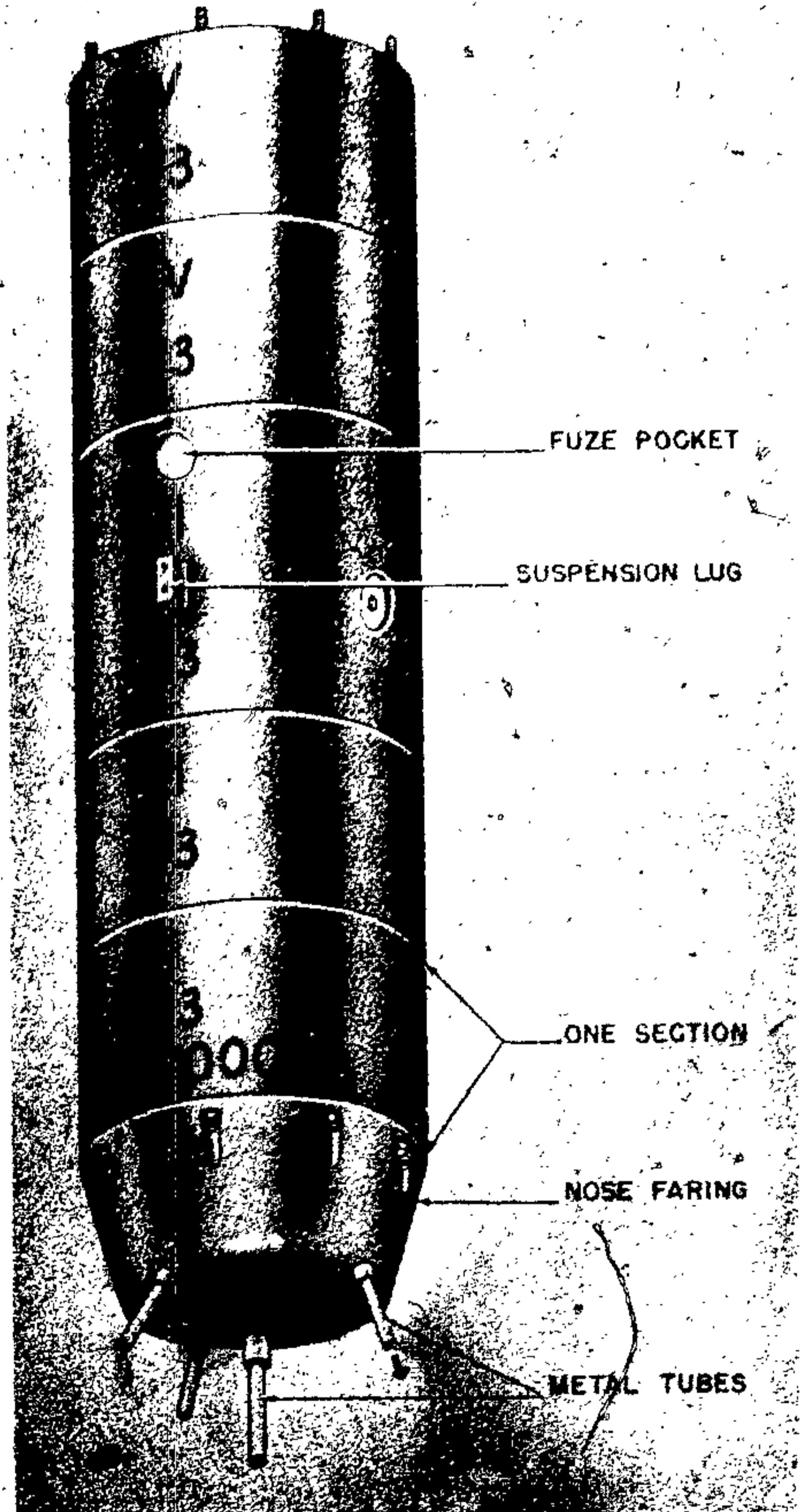
Figure 48—SA 4000-Kg Bomb
