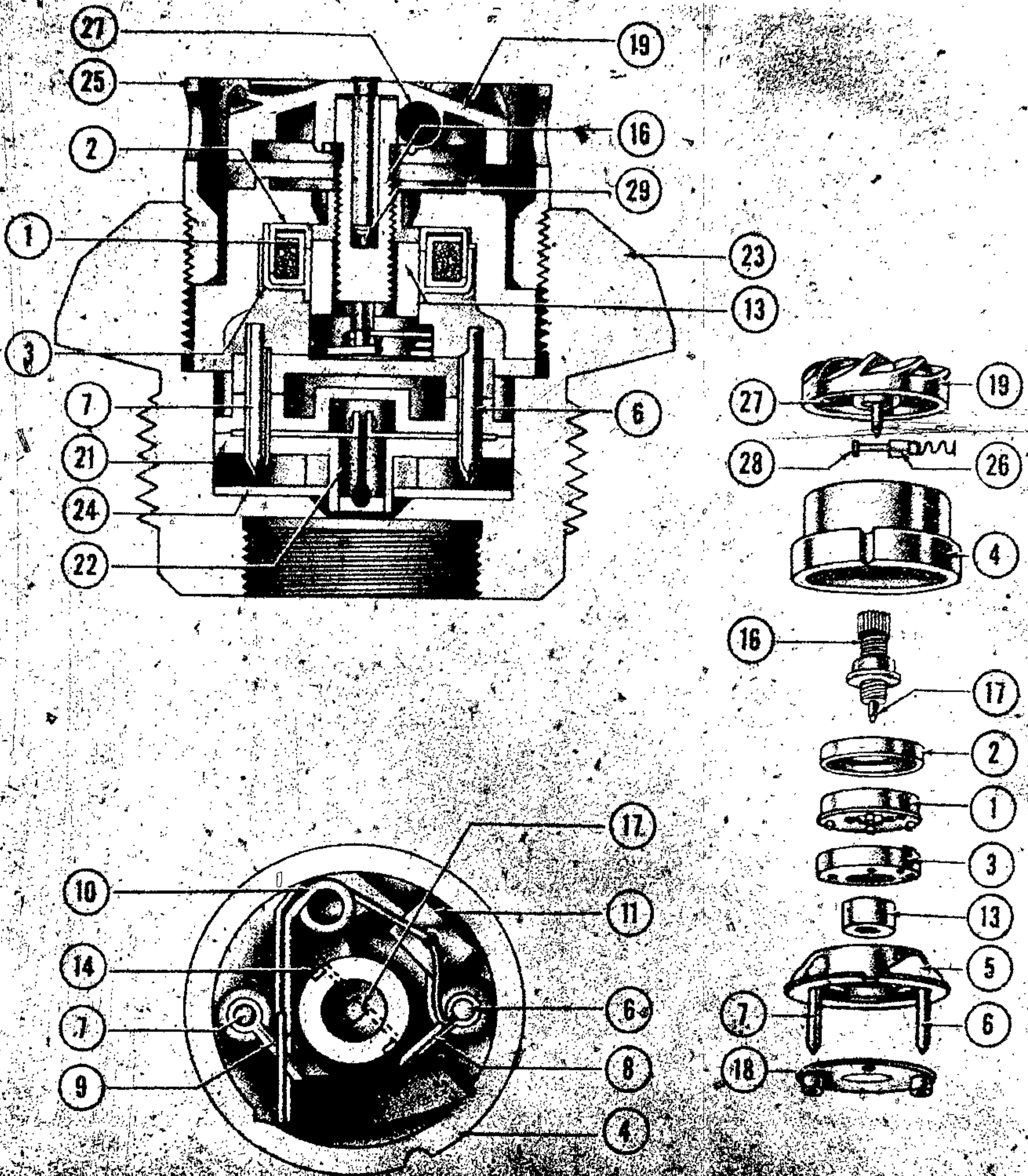
Figure 149—(66) Special Impact Fuze
