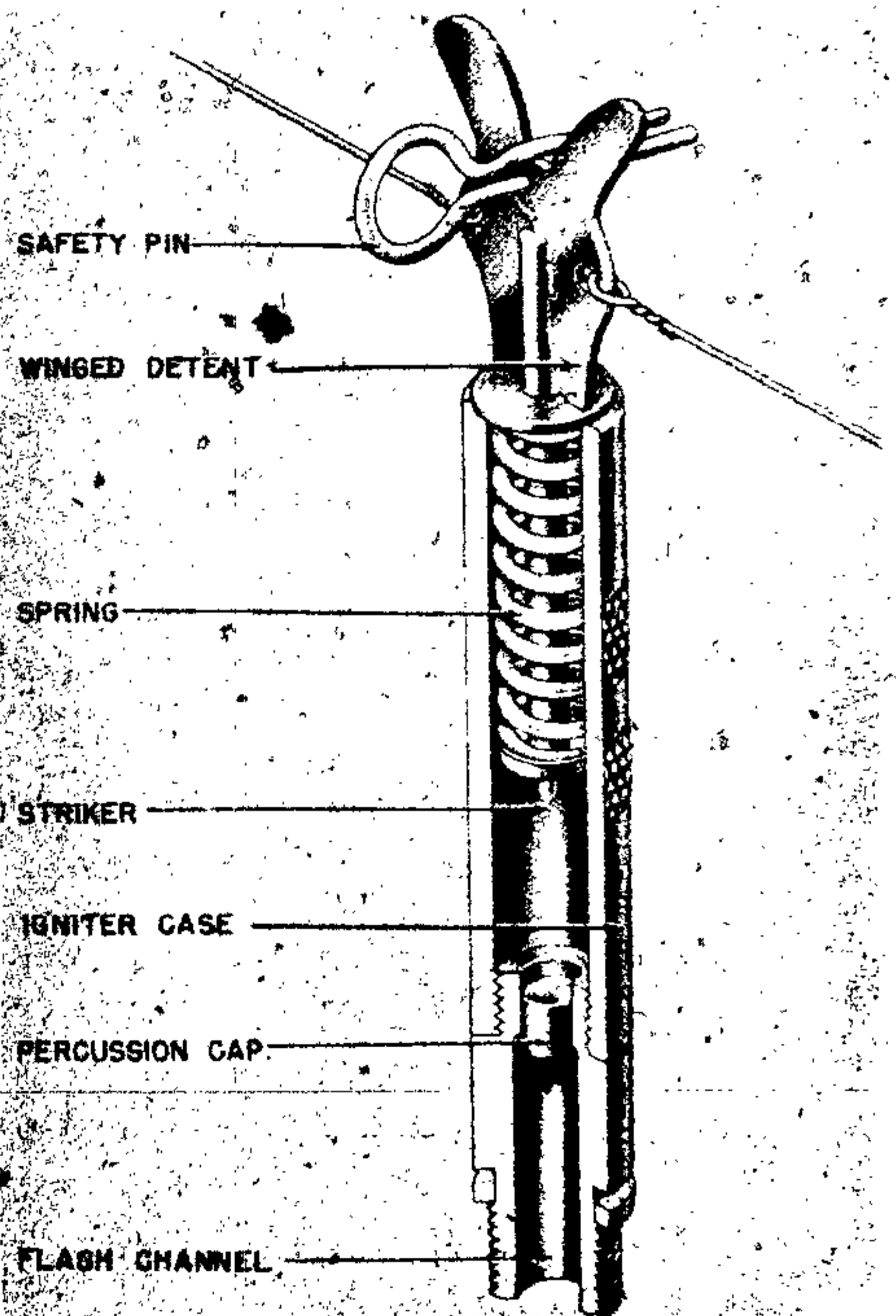
Figure 261—S. Mi. Z. 44 Igniter—Pressure and Pull
