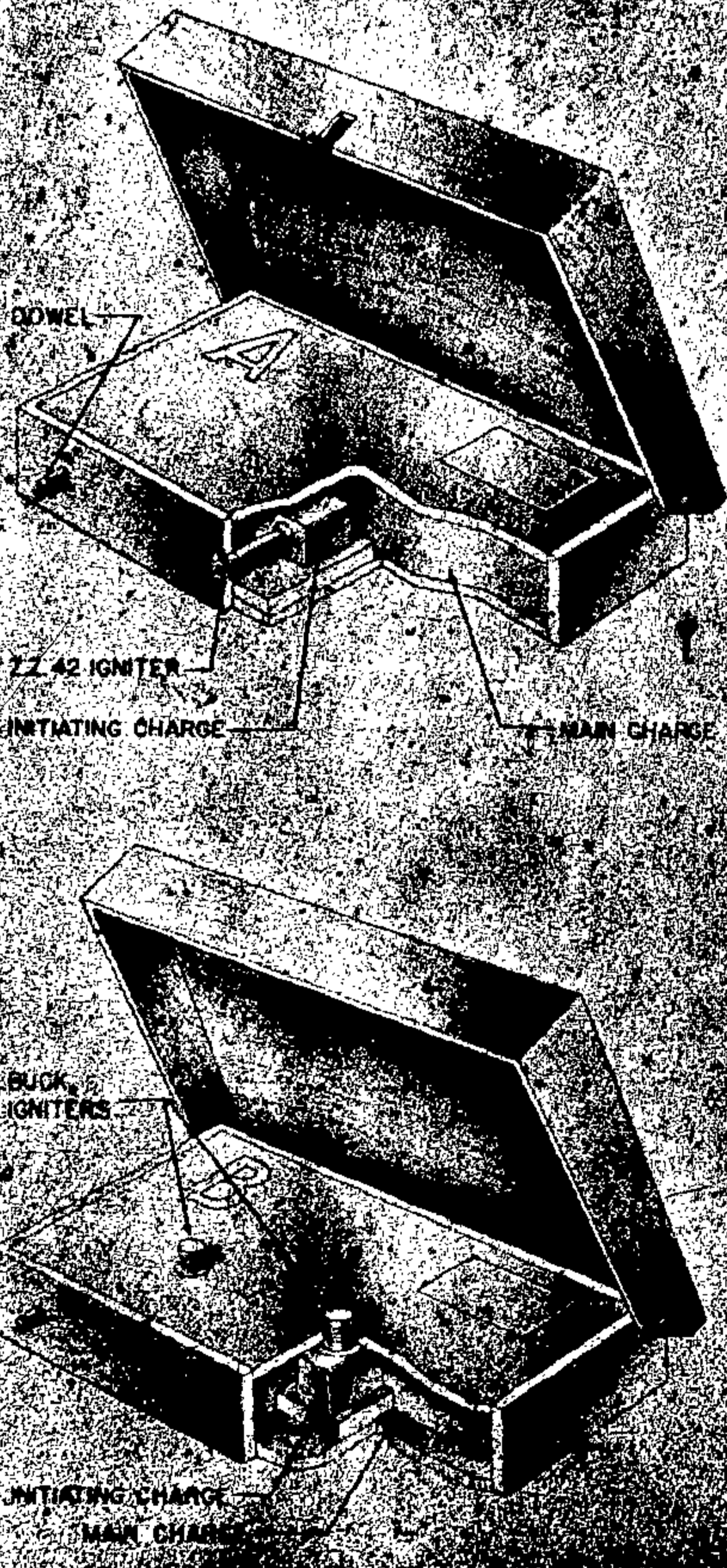
Figure 225—Panzerschnell Antitank Mine
