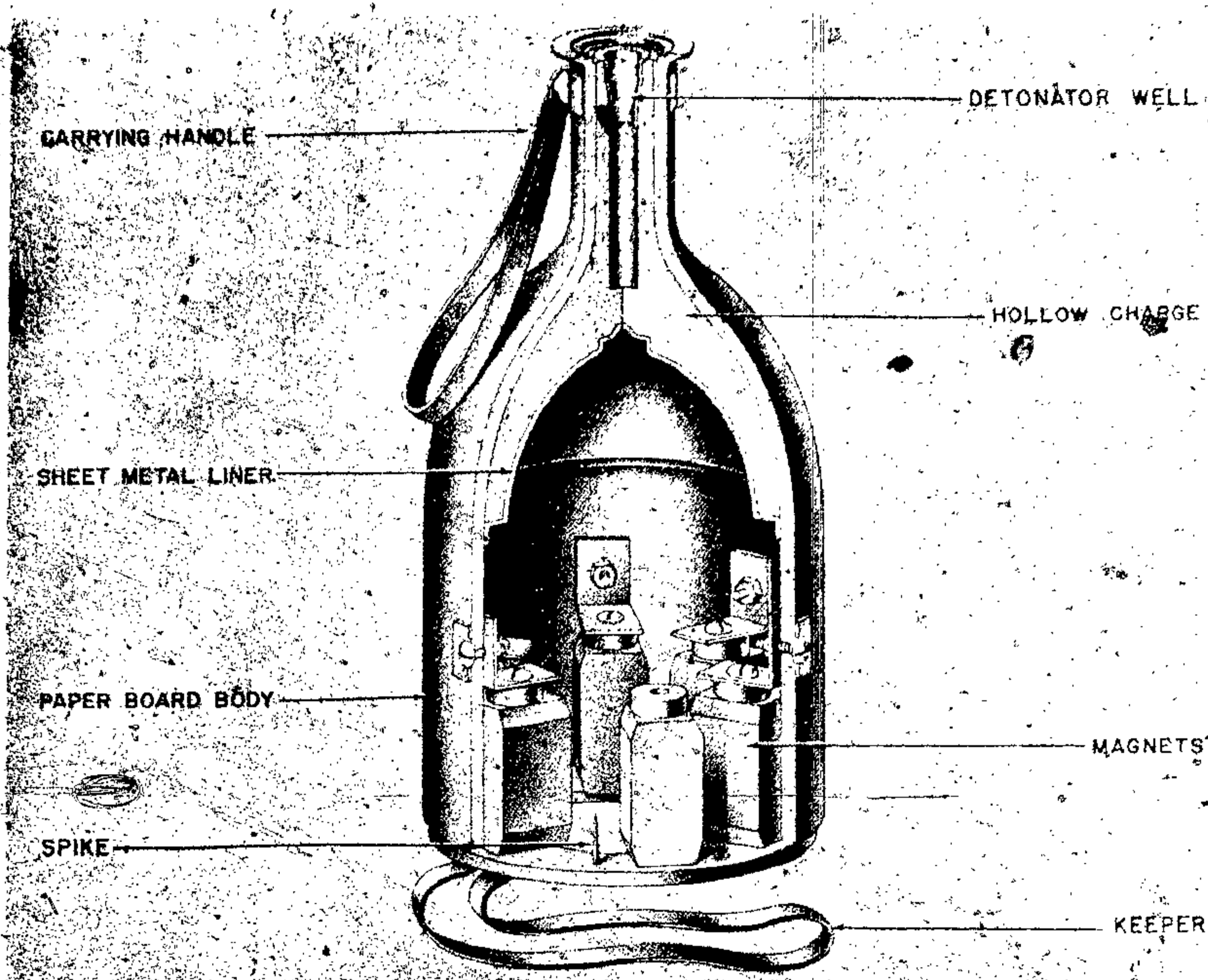
Figure 226—Panzerhandmine 3 Antitank Magnetic Charge Mine
