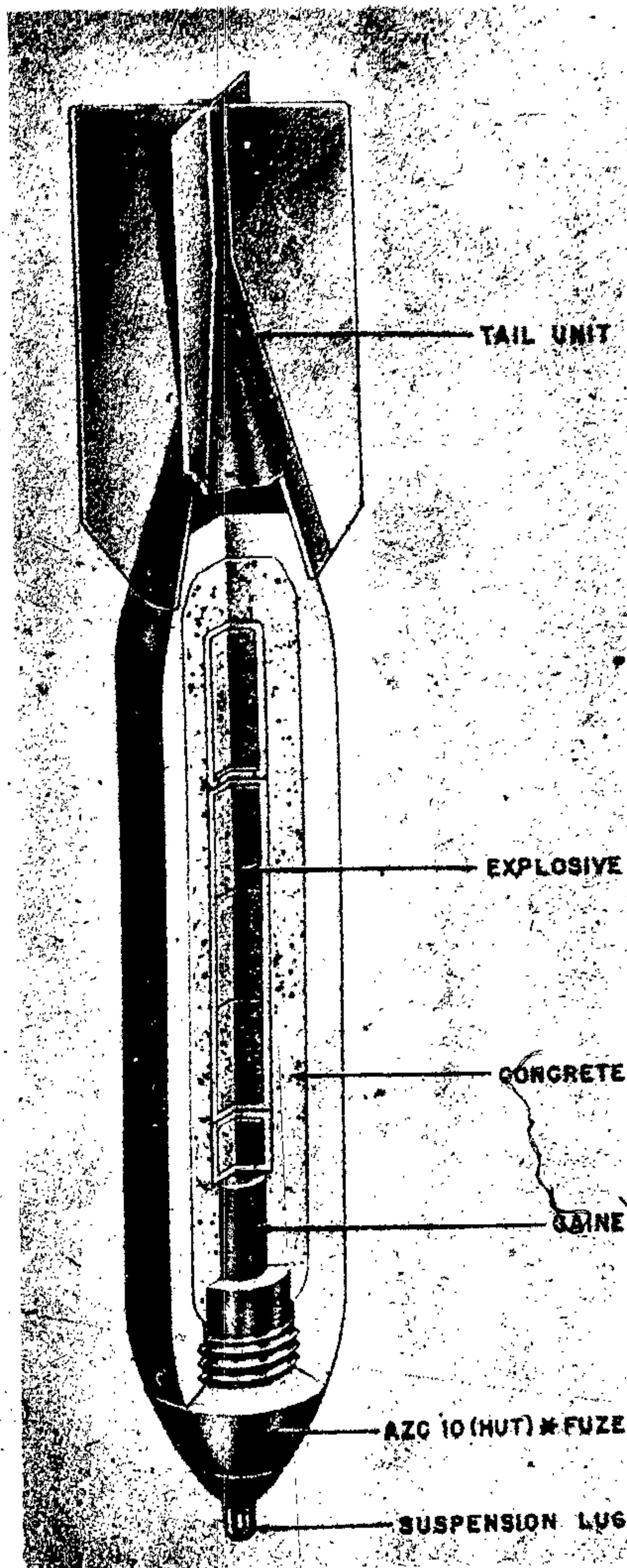
Figure 44—12-Kg SC 10 Concrete Bomb
