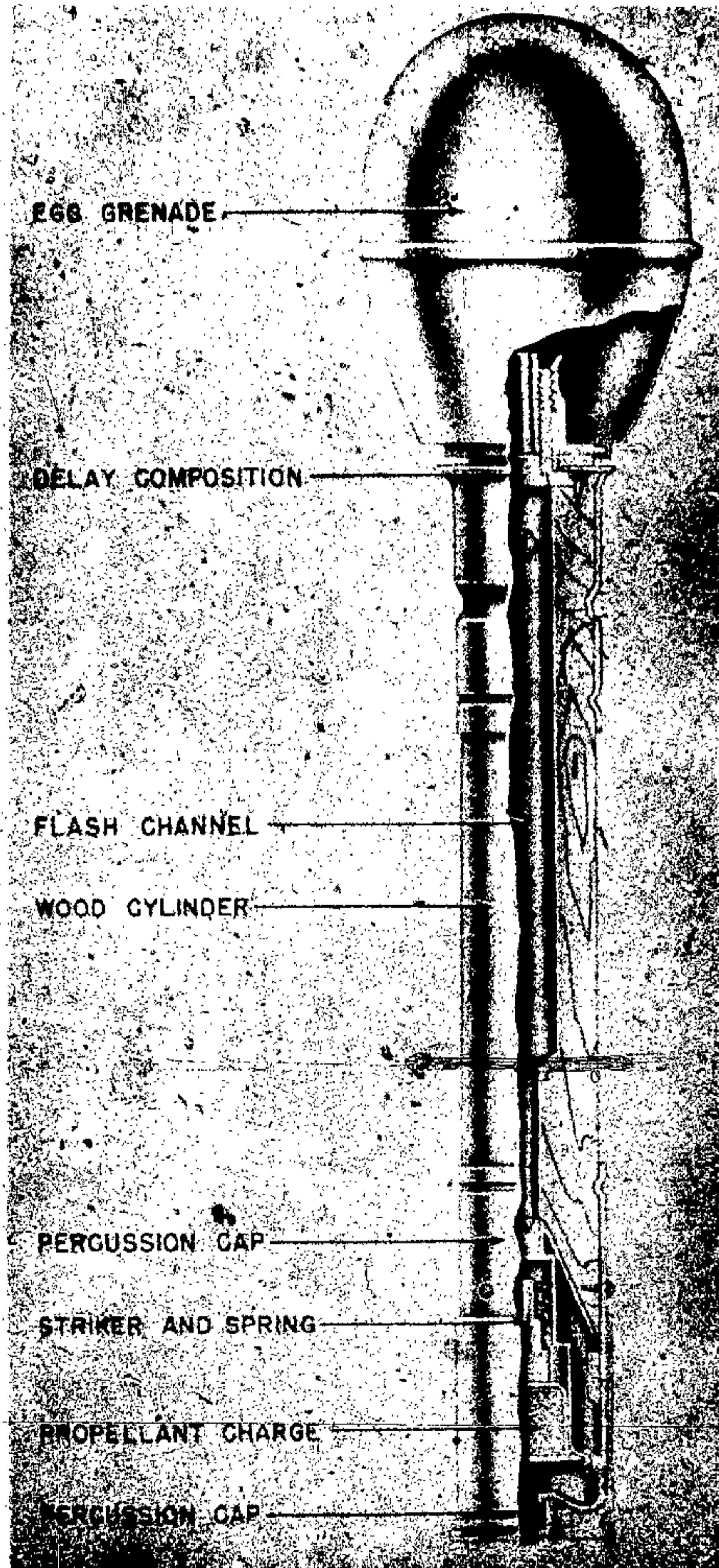
Figure 310—27-mm Egg Type Pistol Grenade
