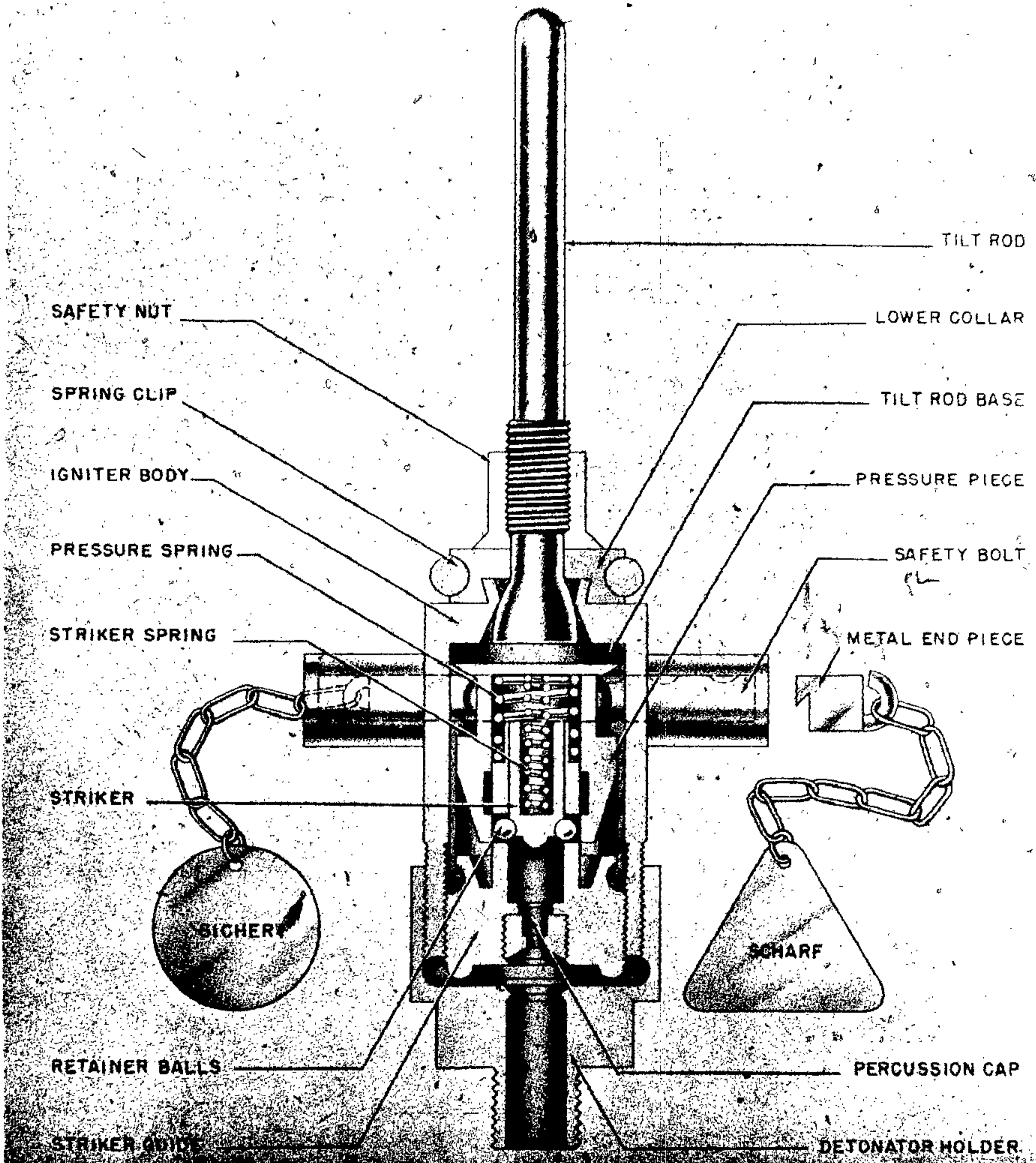
Figure 280—Kippzunder 43, Tilt Type
