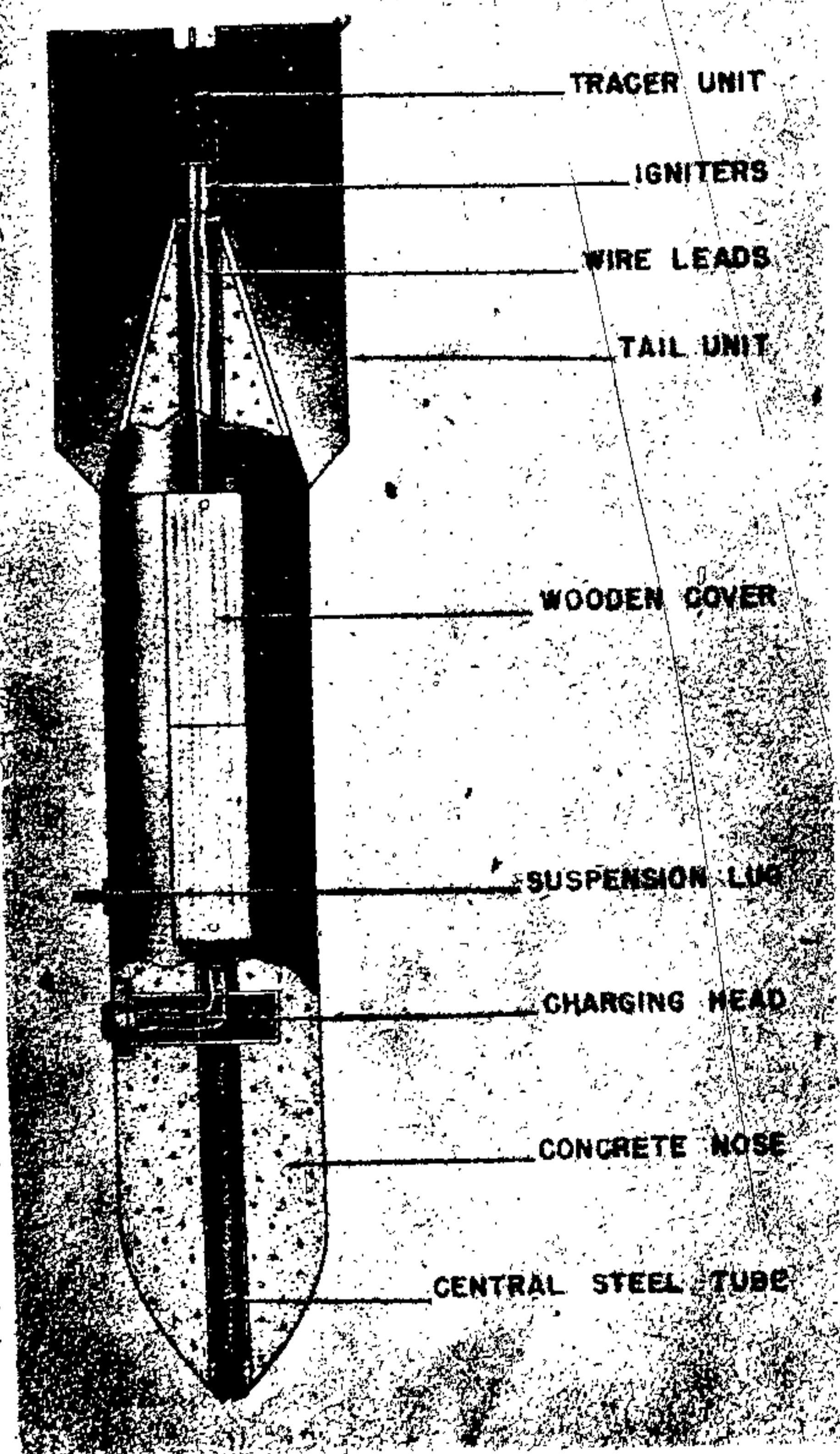
Figure 67—ZC 50-Kg Concrete Practice Bomb, Types I and II
