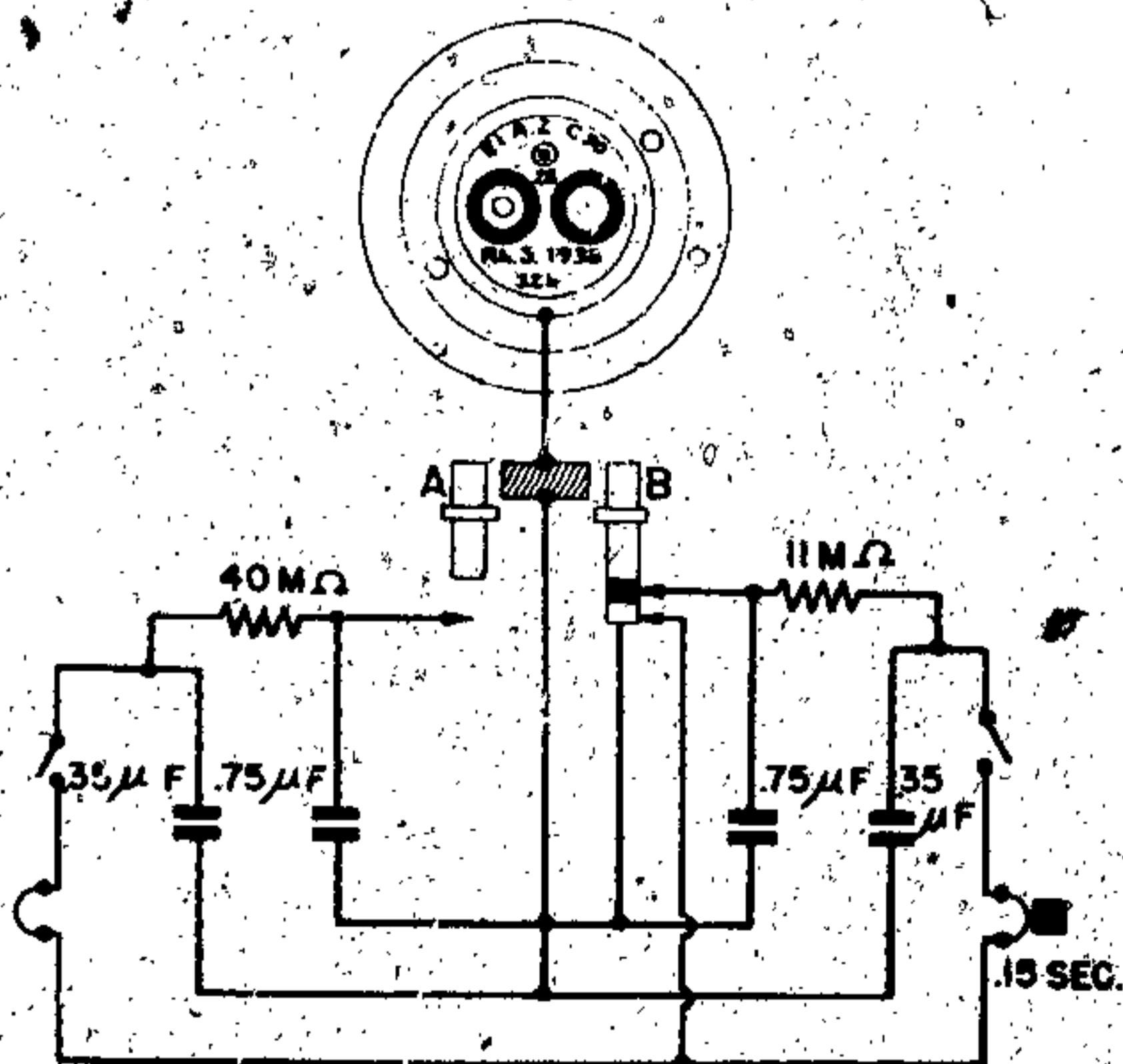
Figure 159—(28)* Electrical Impact Fuze
