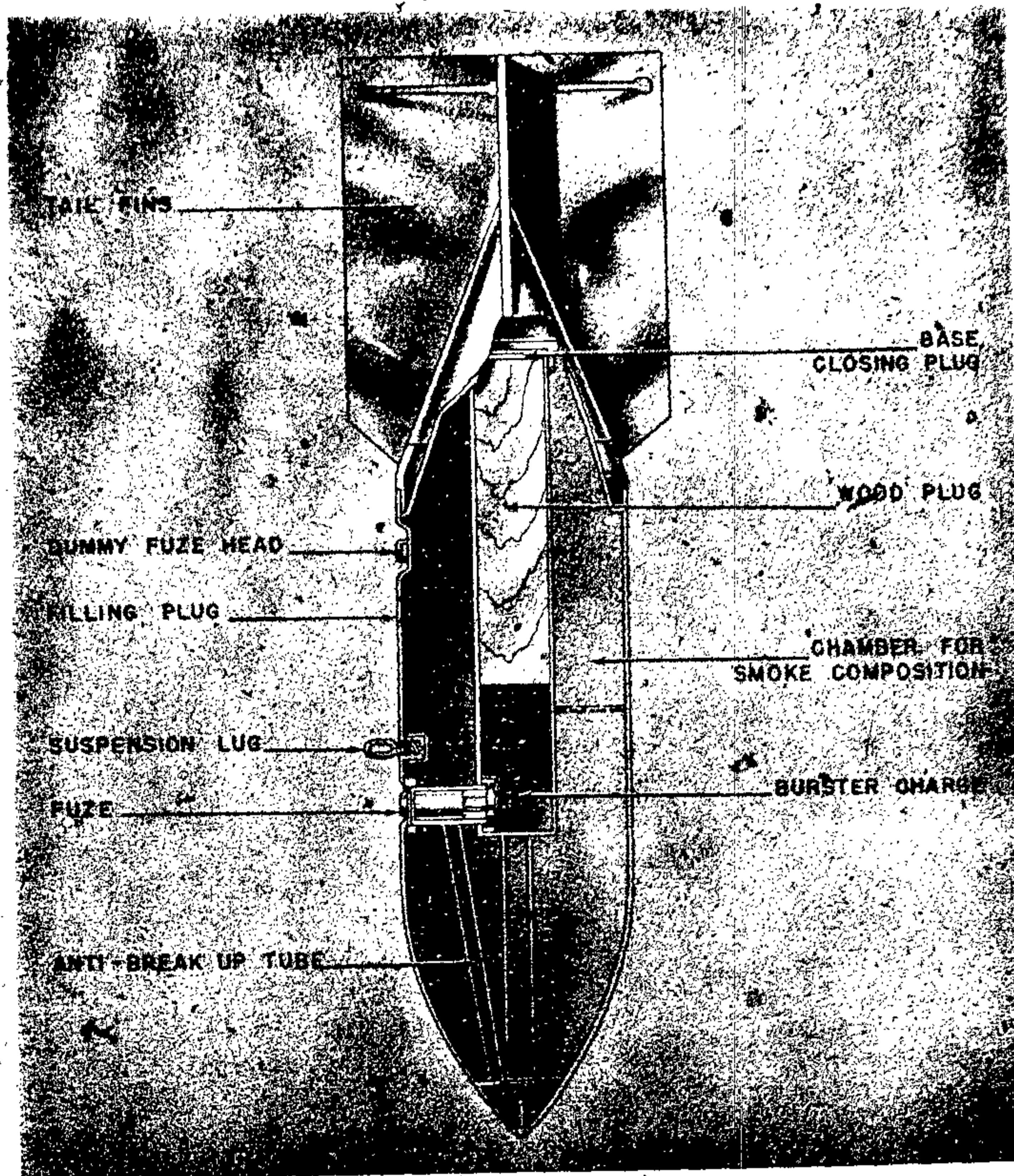
Figure 63—NC 250 S Smoke Bomb
