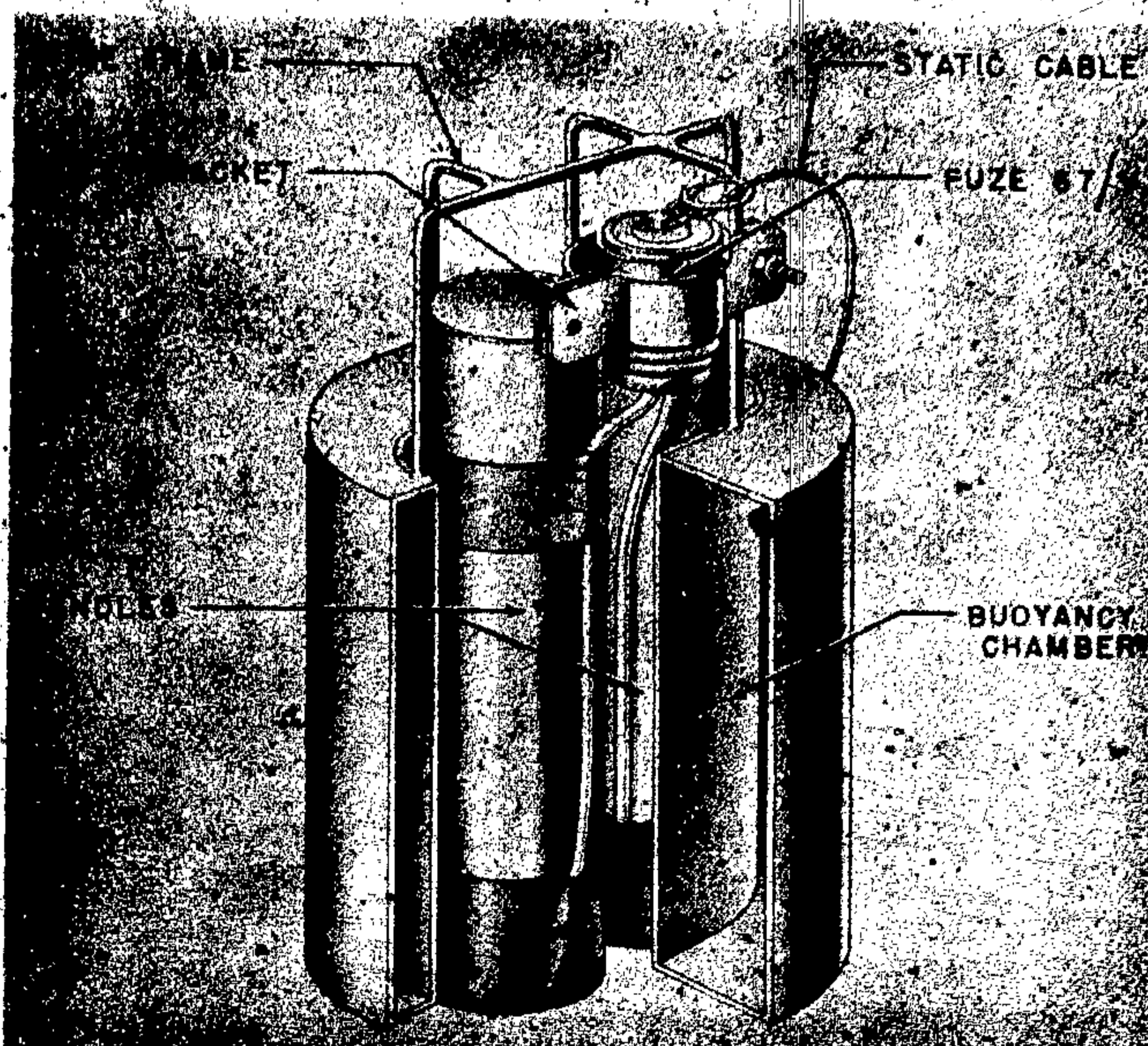
Figure 80—Mark S Flare, Types 1 and 2
