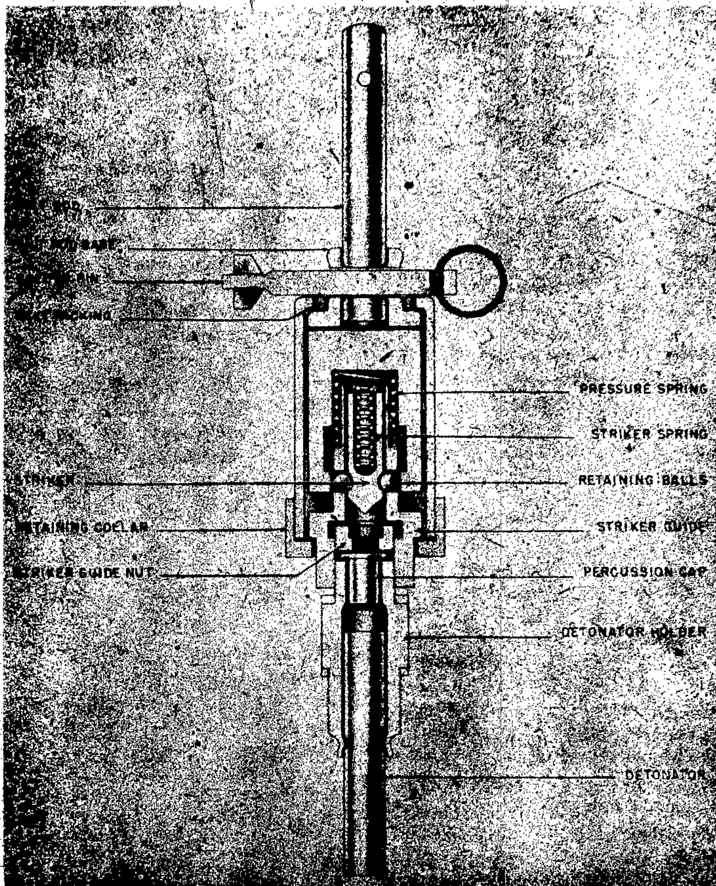
Figure 281—New Type Tilt Igniter (Pressure Tilt Type)
