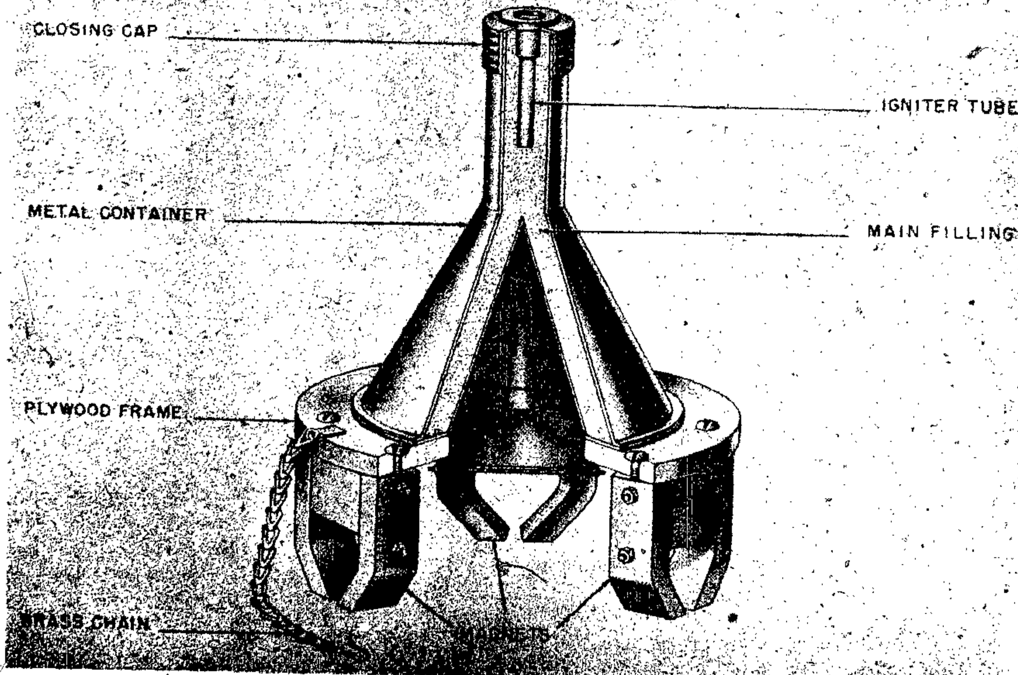
Figure 288—Magnetic Antitank Hand Grenade
