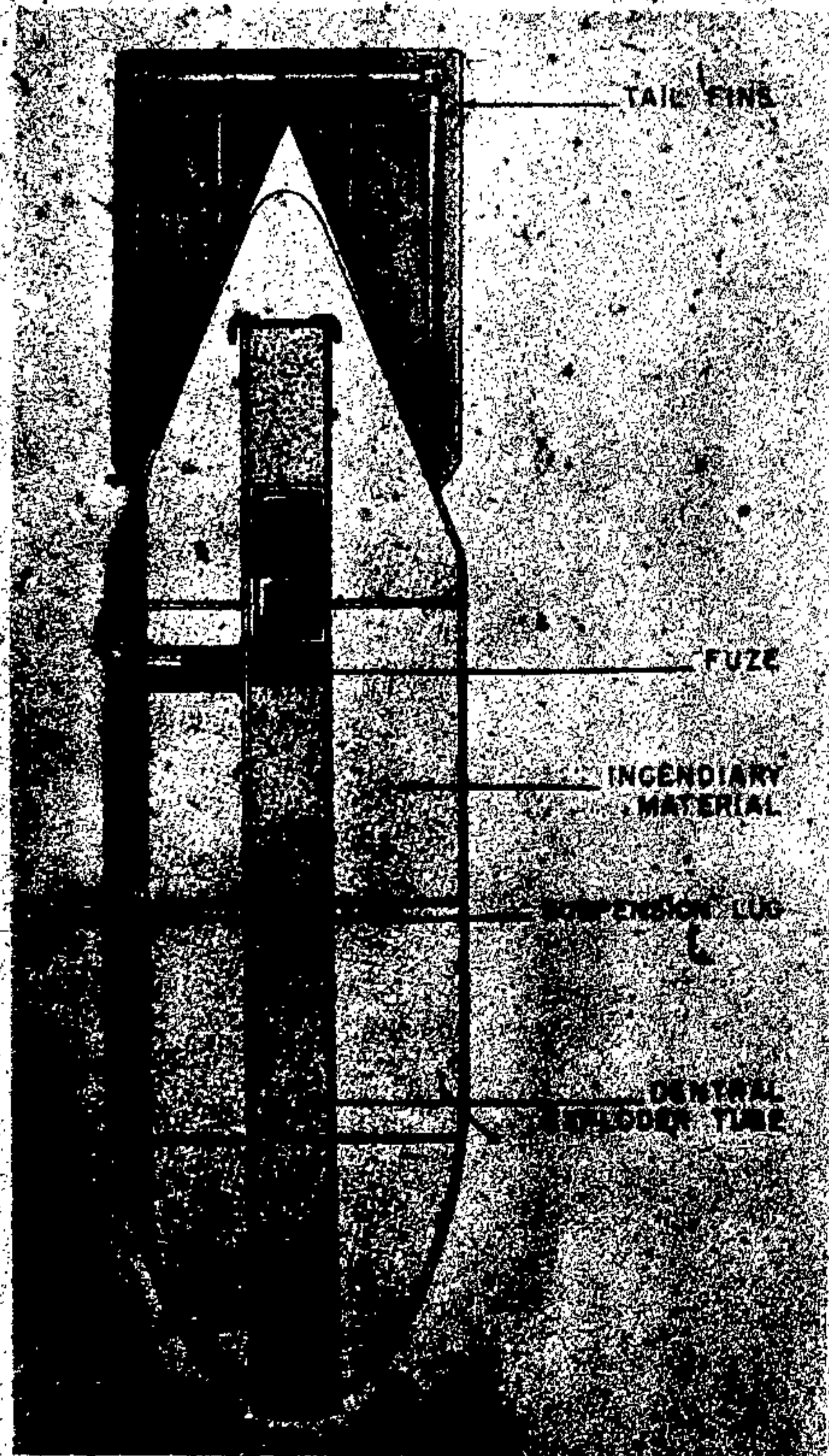
Figure 57—Flam C 500 Bomb
