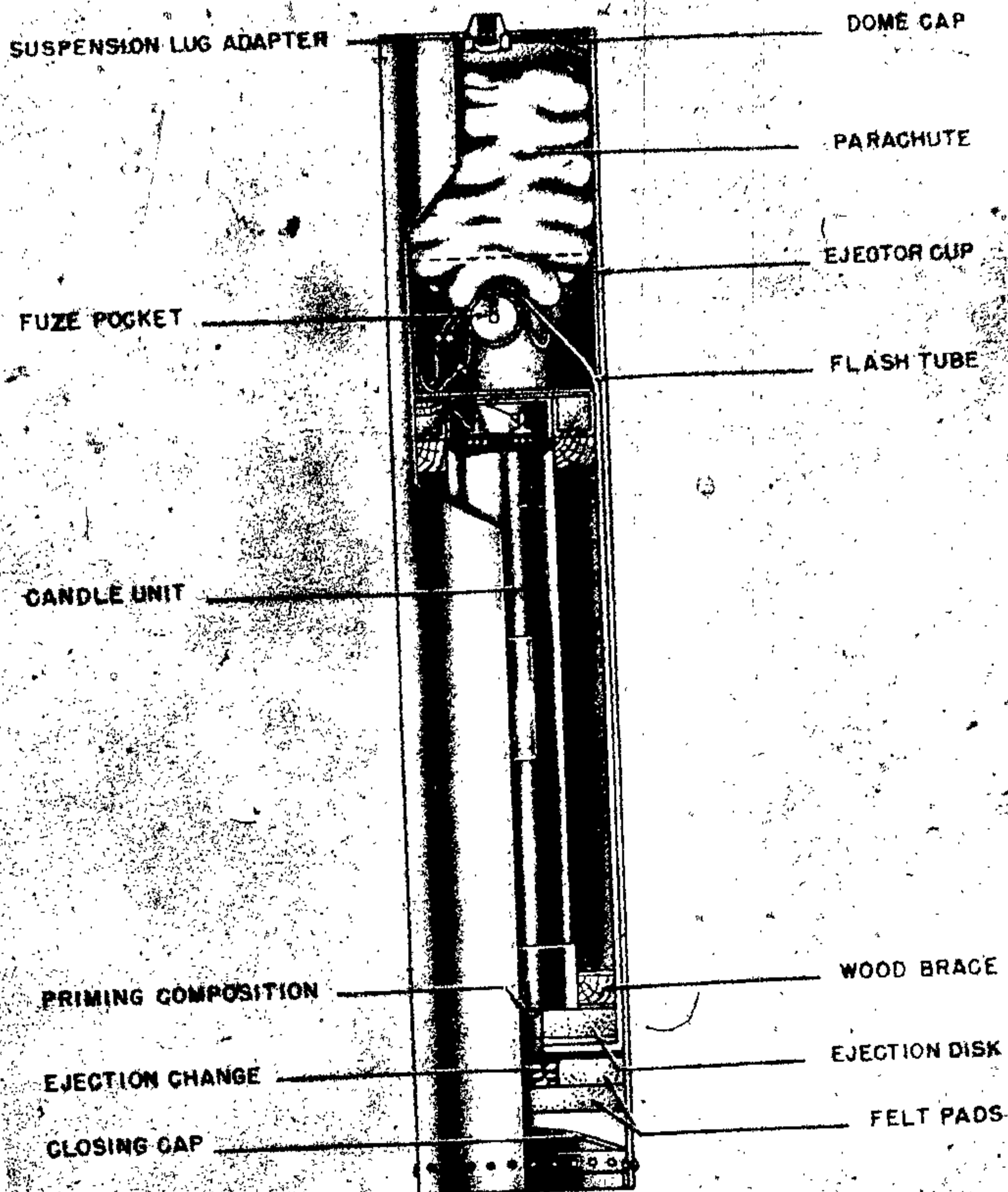
Figure 75—Mark C 50 FA Parachute Flare
