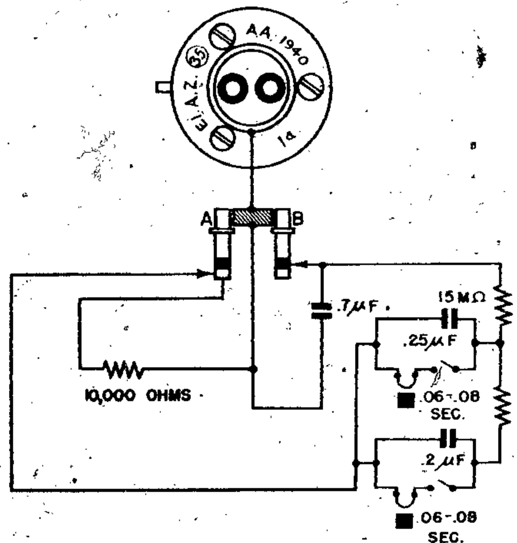
Figure 143—(35) Electrical Impact Fuze
