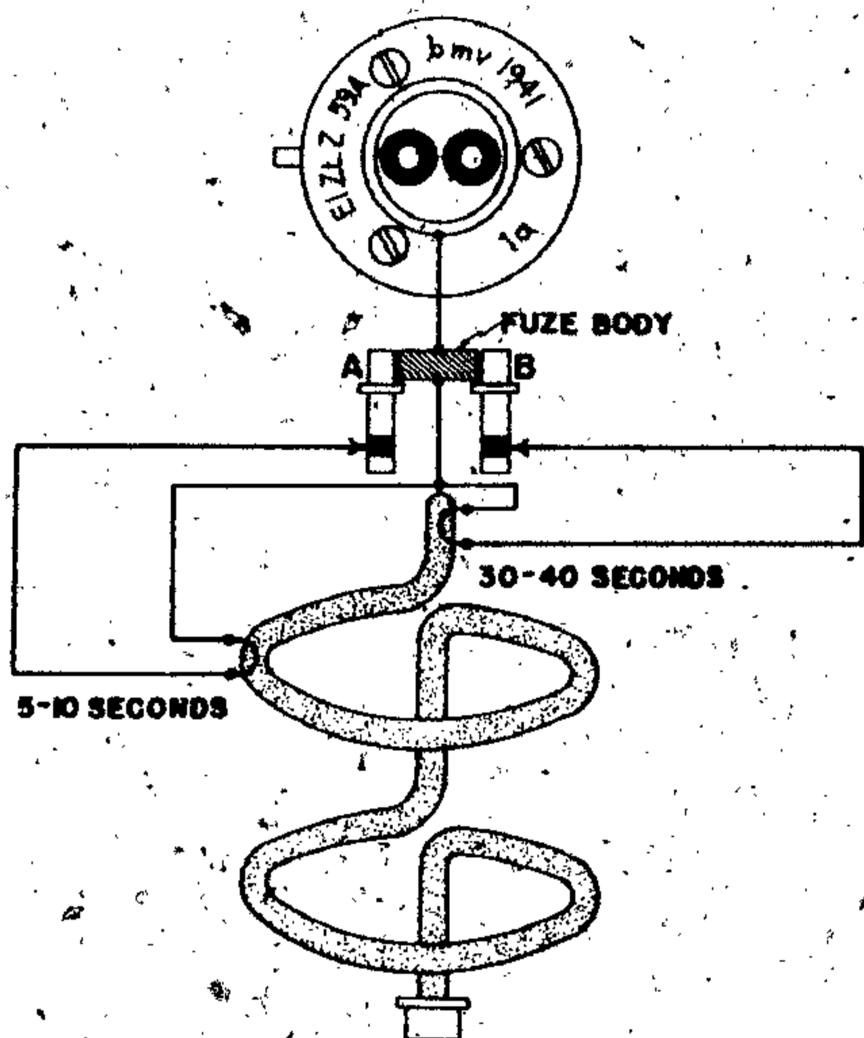
Figure 174—(59)A Electrical Aerial Burst Fuze
