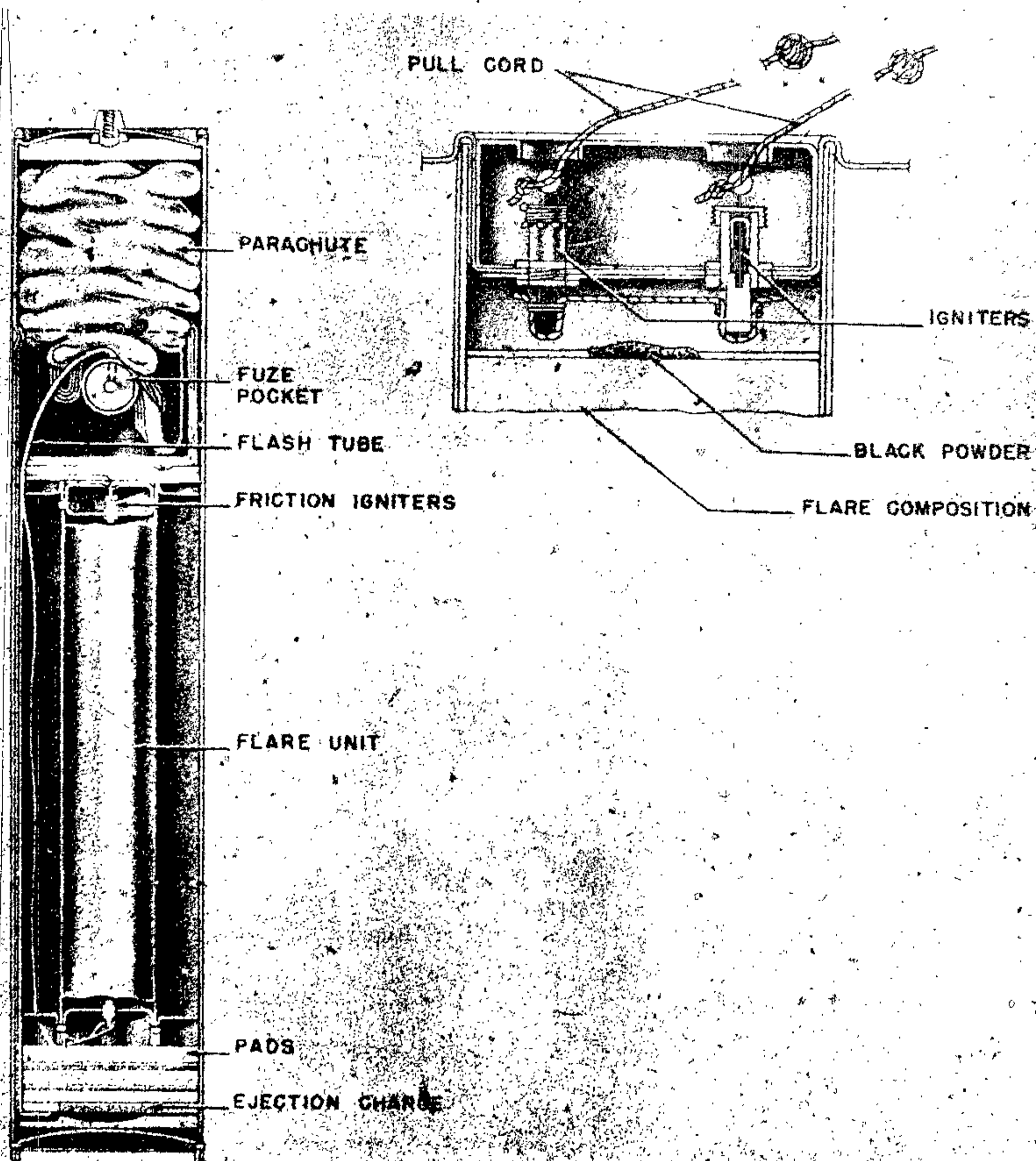
Figure 77—Parachute Flare with Pull Igniter
