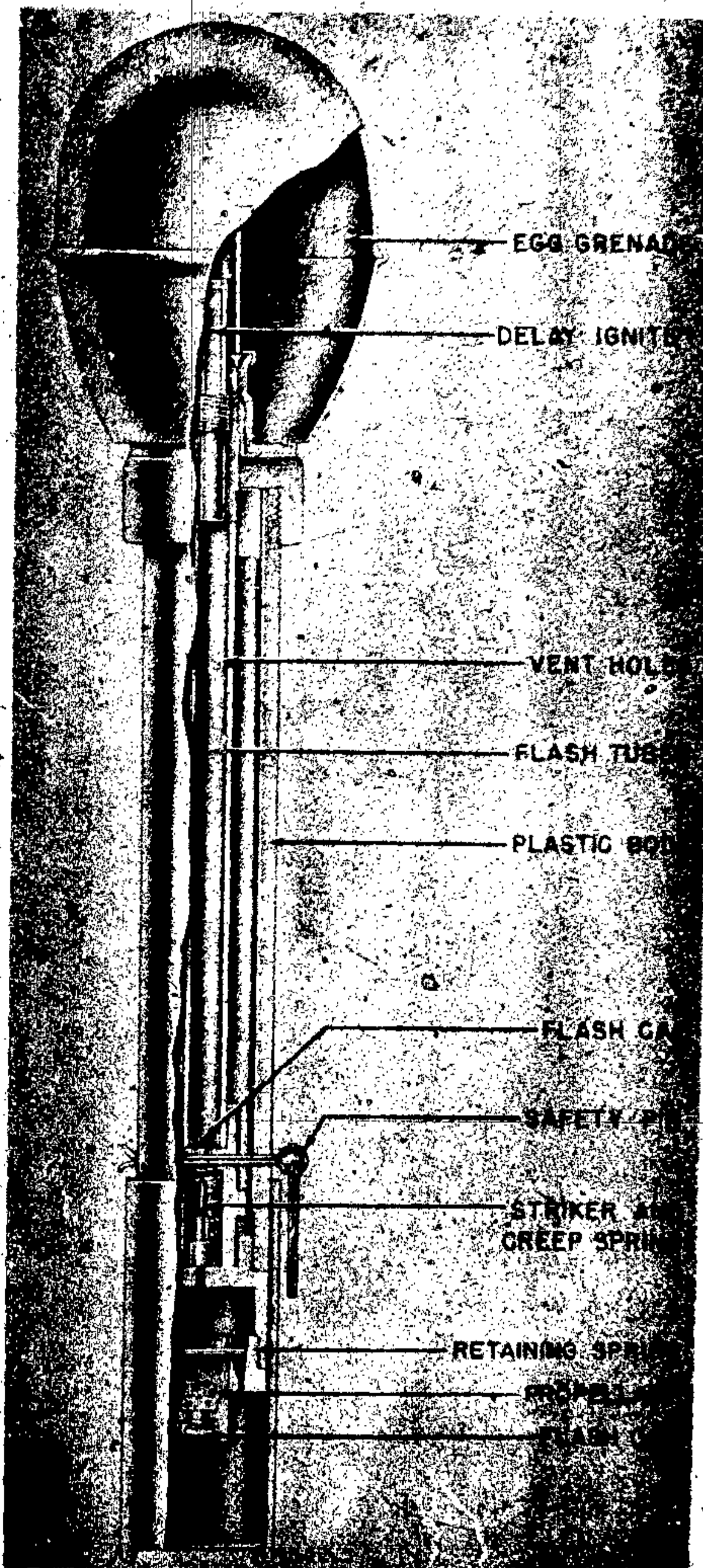
Figure 309—27-mm Pistol Grenade.
