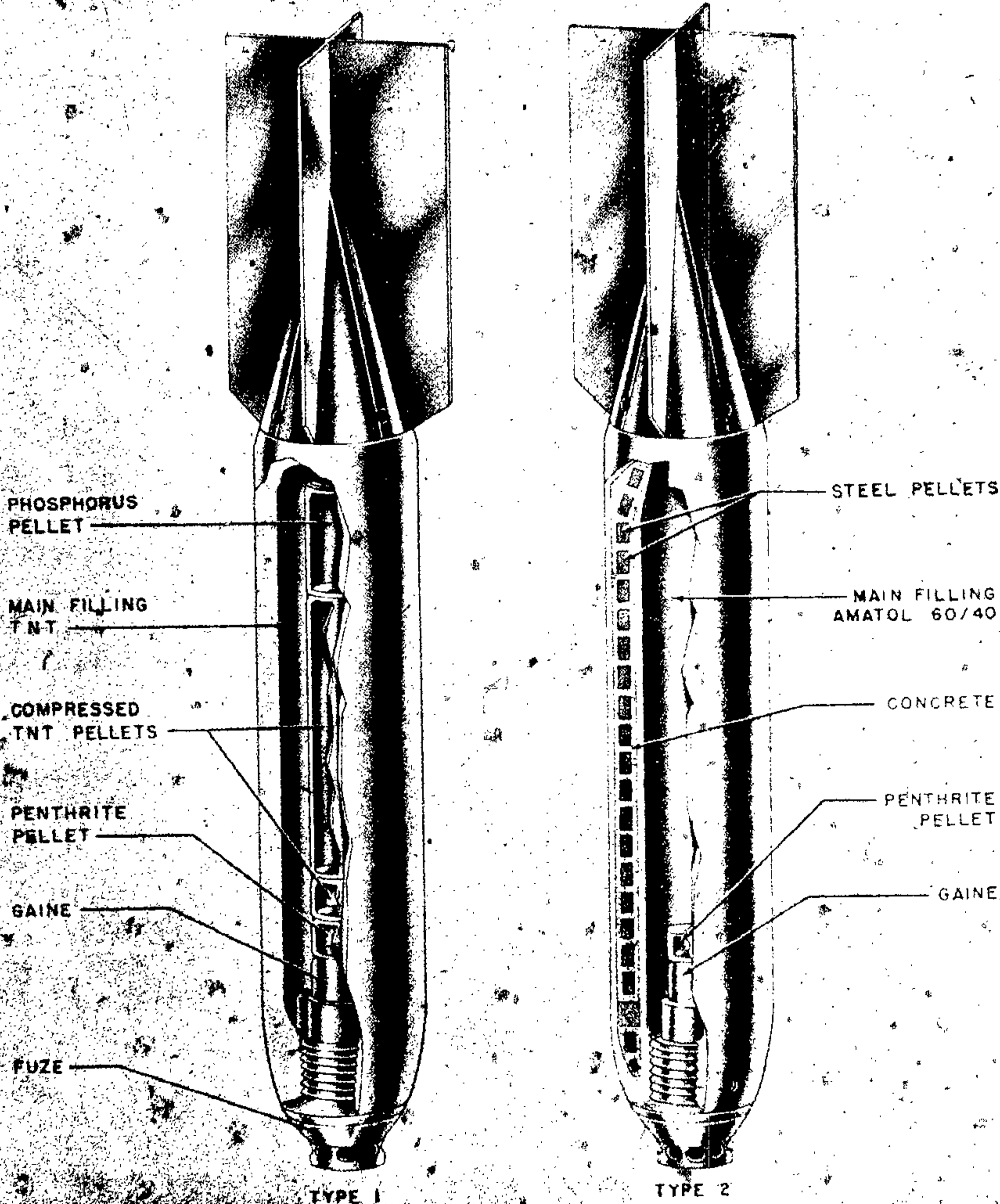
Figure 42—SD 10A Antipersonnel Bomb
