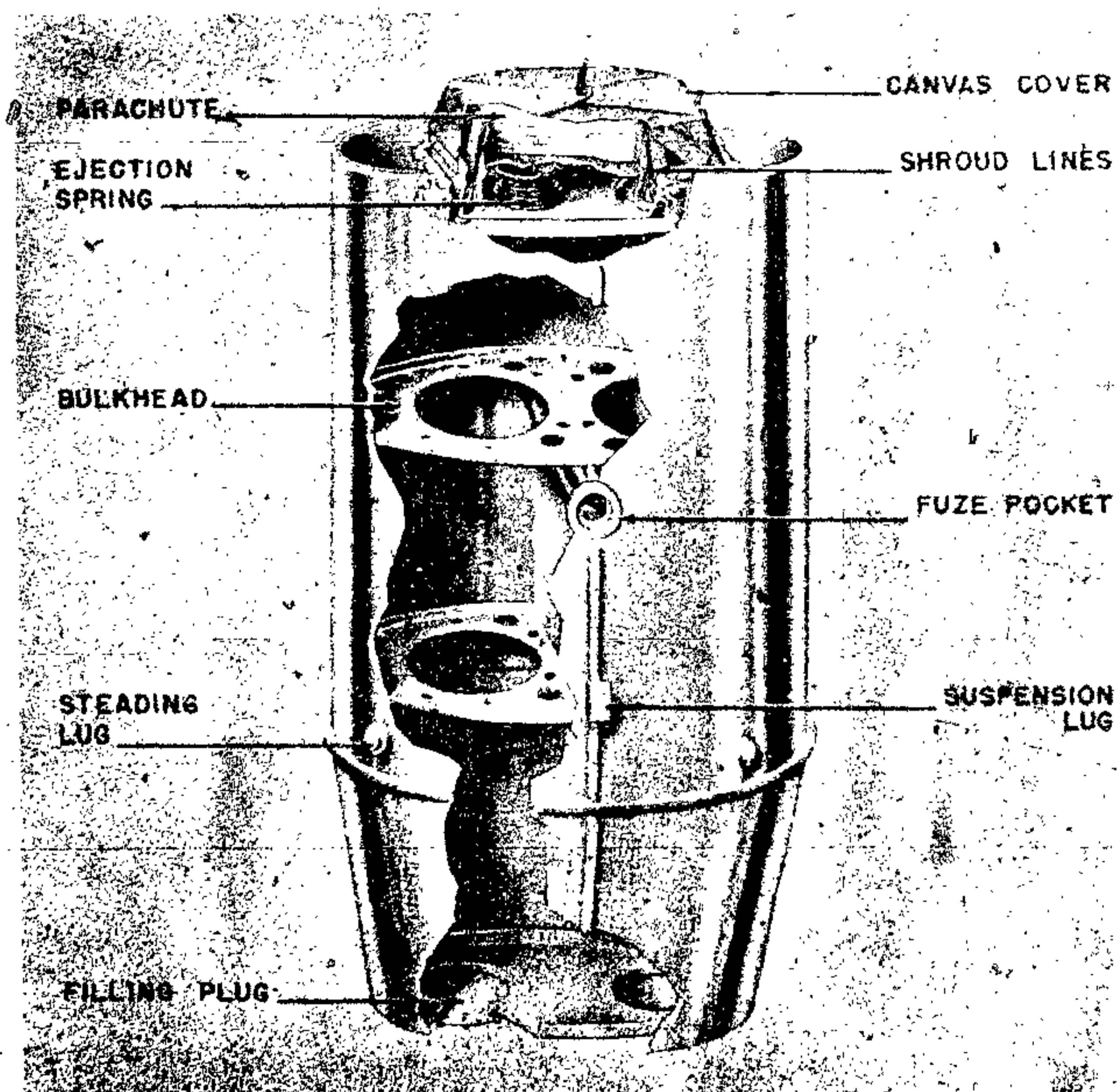
Figure 21—SB 1000-Kg Parachute Bomb
