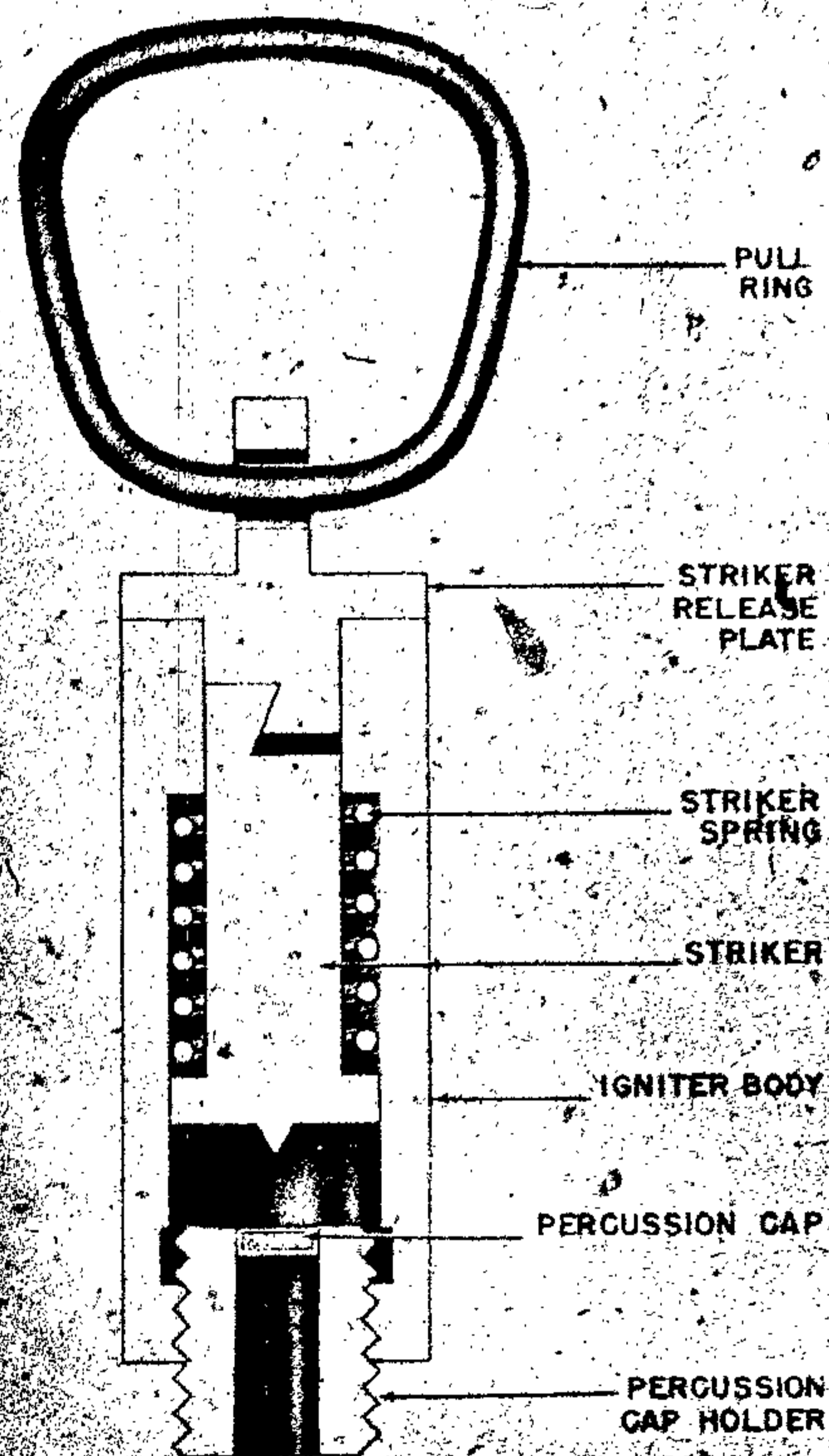
Figure 254—Safety Fuse Igniter, Percussion Type
