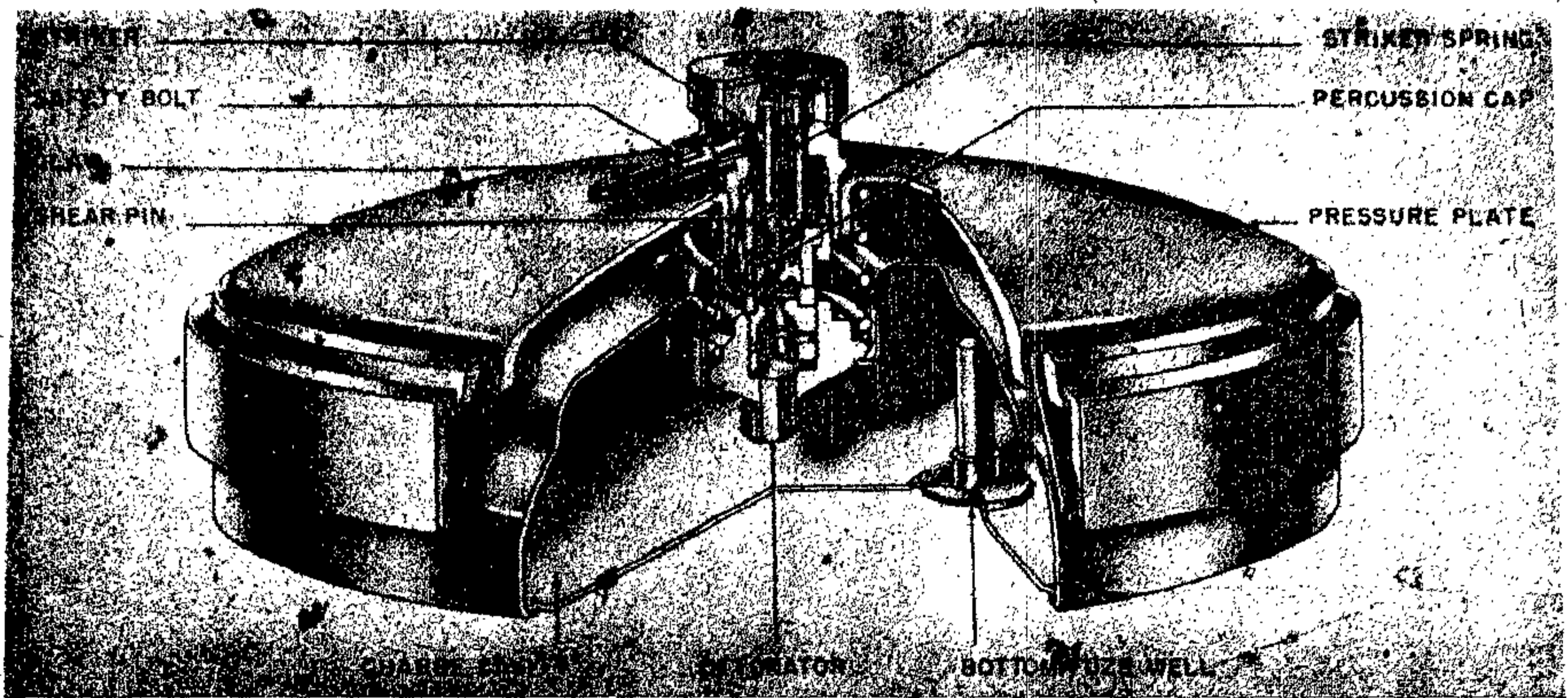
Figure 230—Tellermine 35—Antitank
