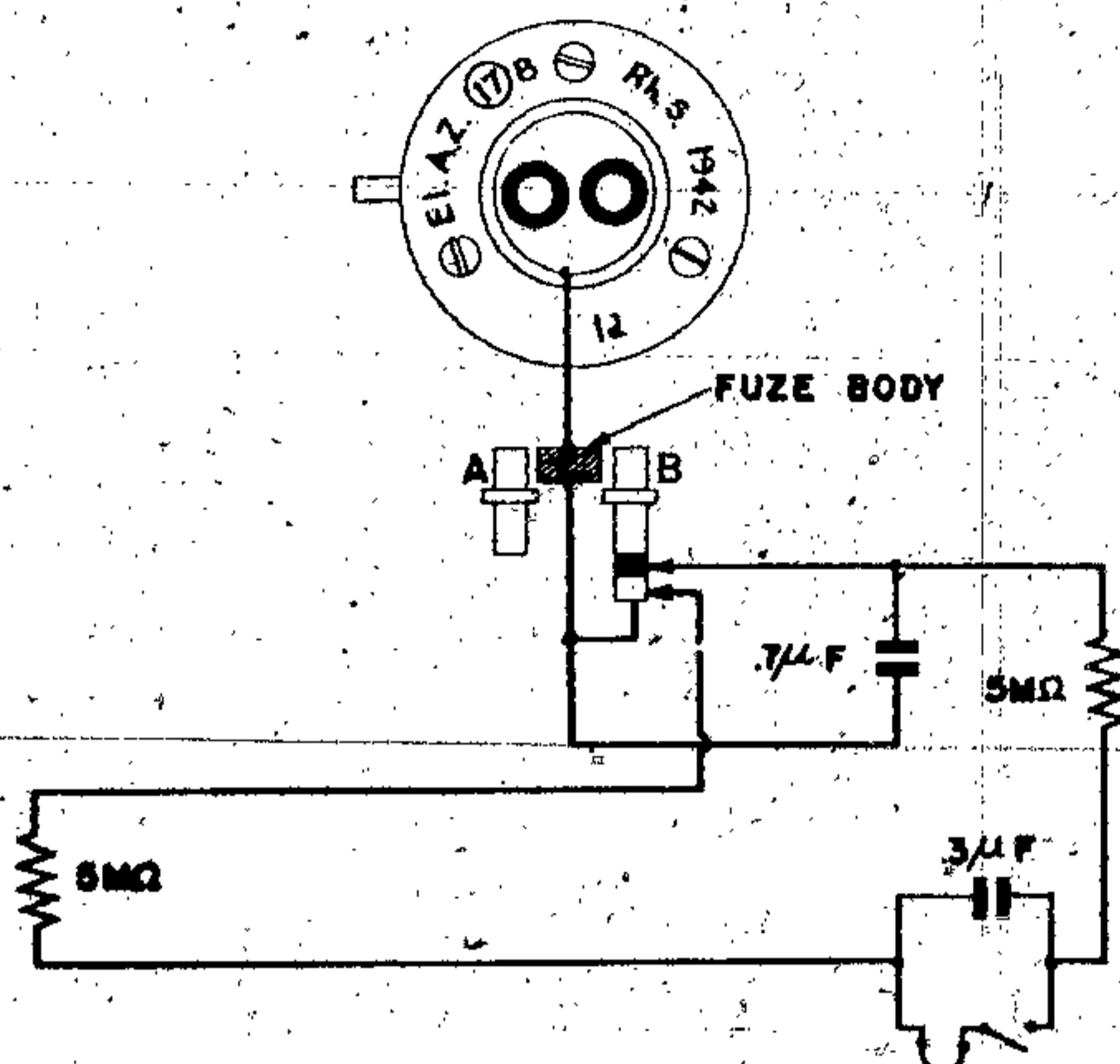
Figure 154—(17)B Electrical Clockwork Time Fuze
