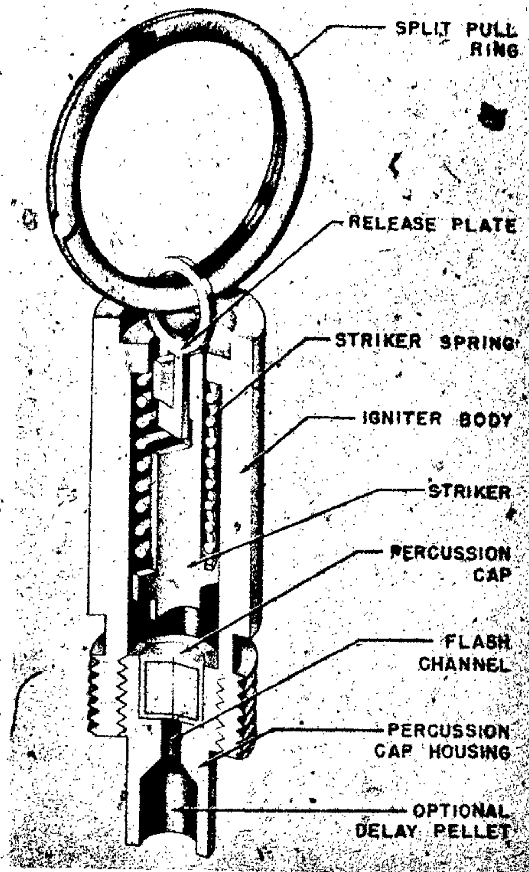
Figure 255—Type 2 Pull Percussion Igniter
