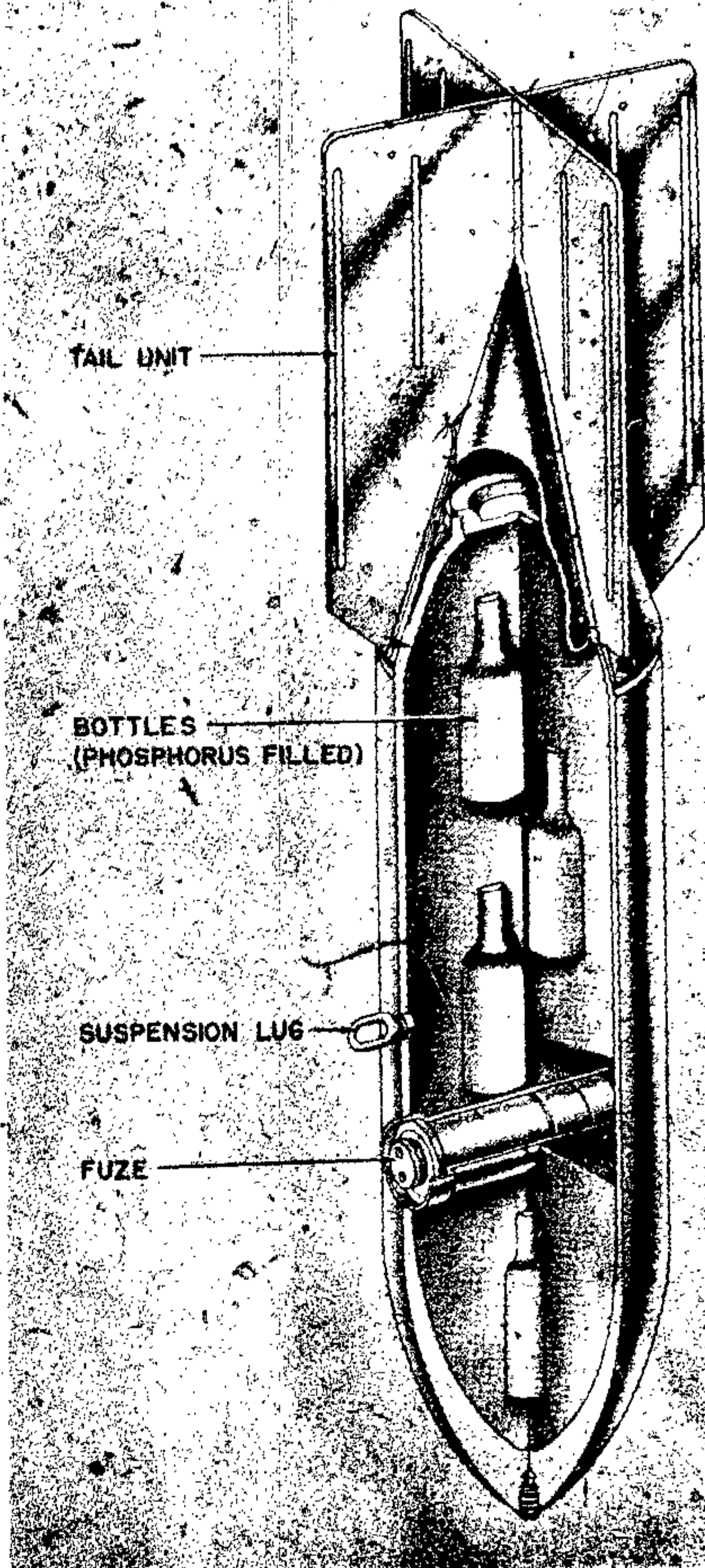
Figure 58—Brand C 50 A Bomb
