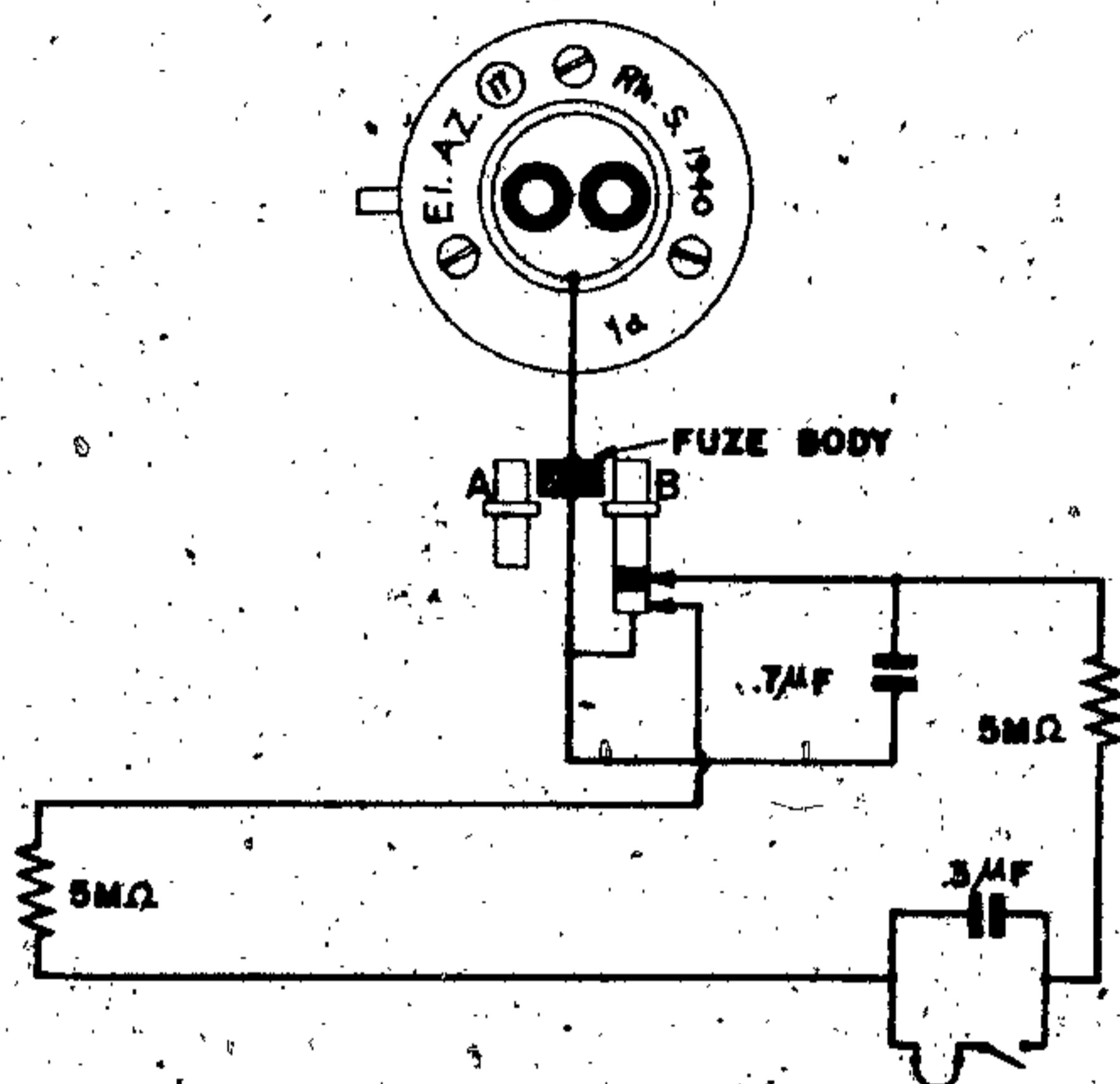
Figure 152—(17) Electrical Clockwork Time Fuze
