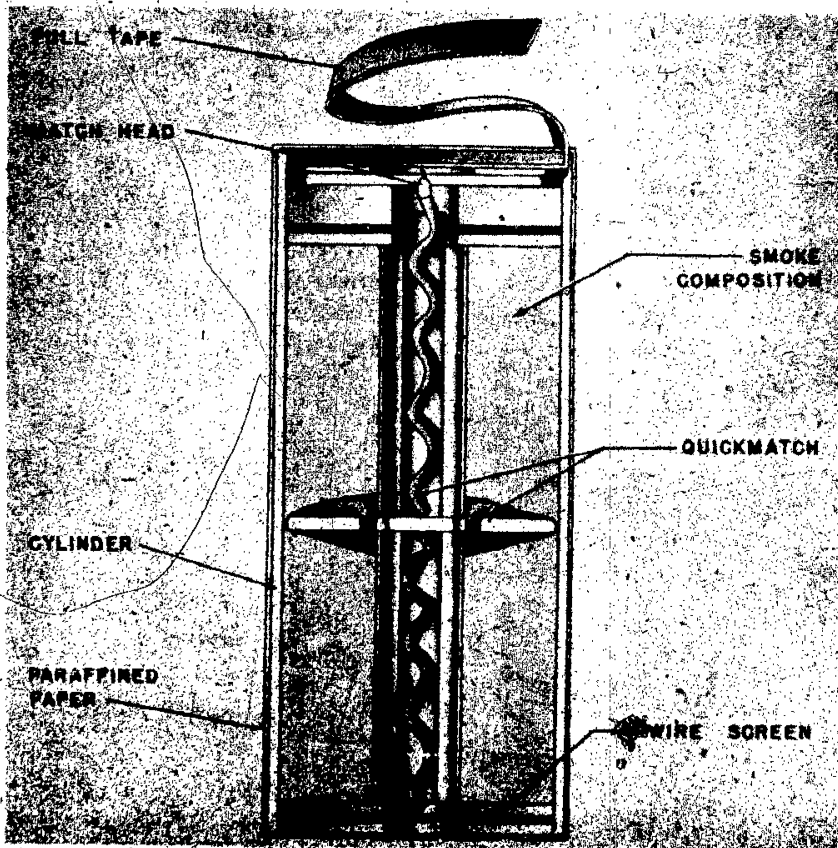
Figure 296—Red Smoke Signal Hand Grenade
