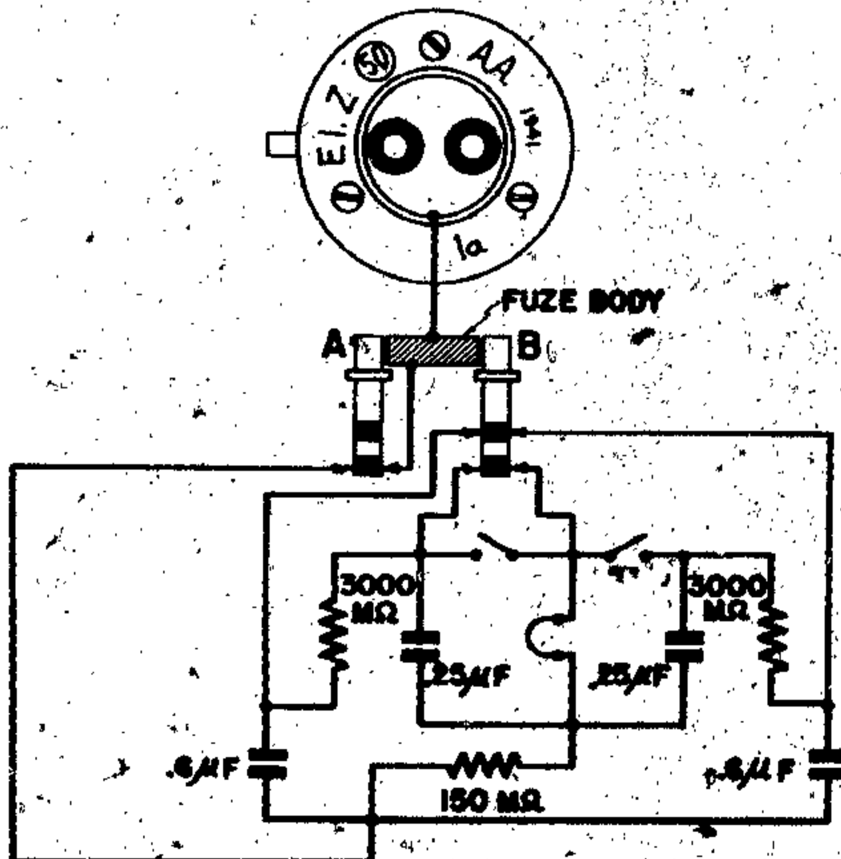
Figure 184—(50) Electrical Antidisturbance Fuze
