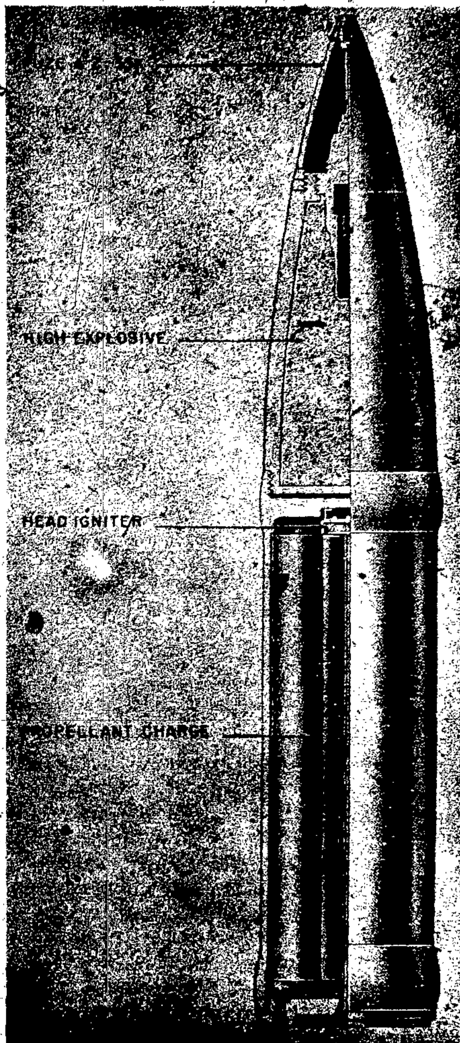
Figure 215—21-cm Aircraft Rocket
