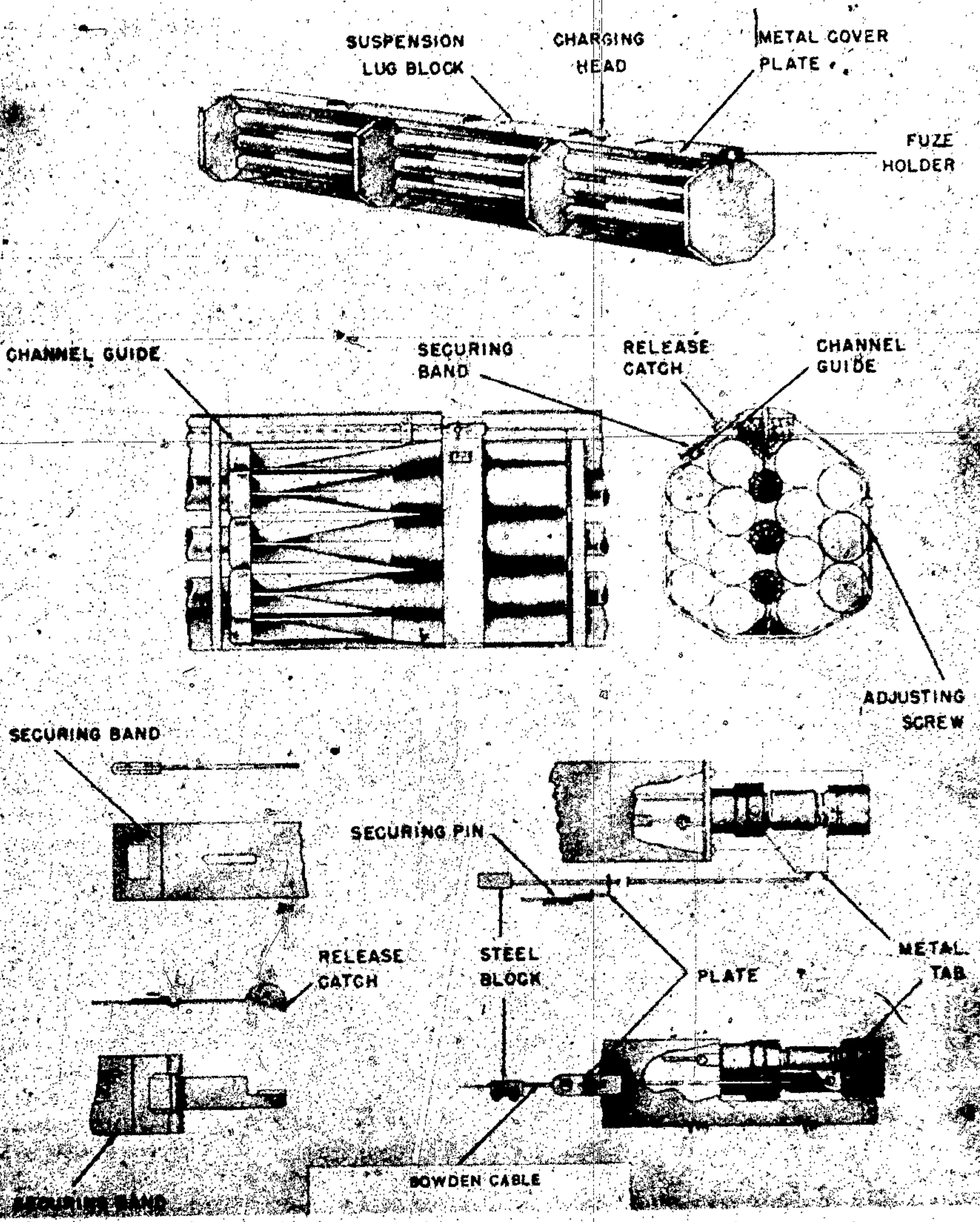
Figure 101—AB 42 Container
