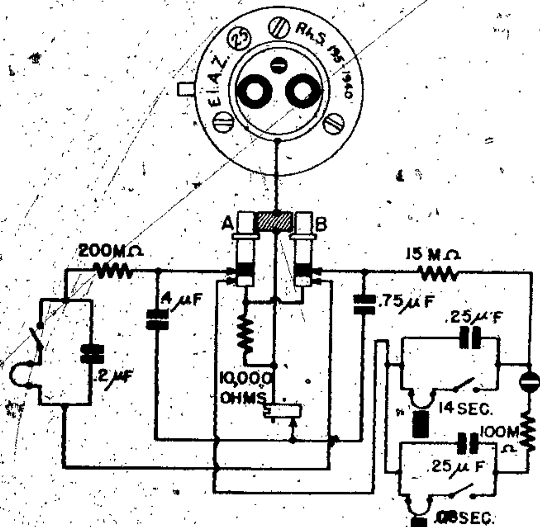
Figure 140—(25) Electrical Impact Fuze
