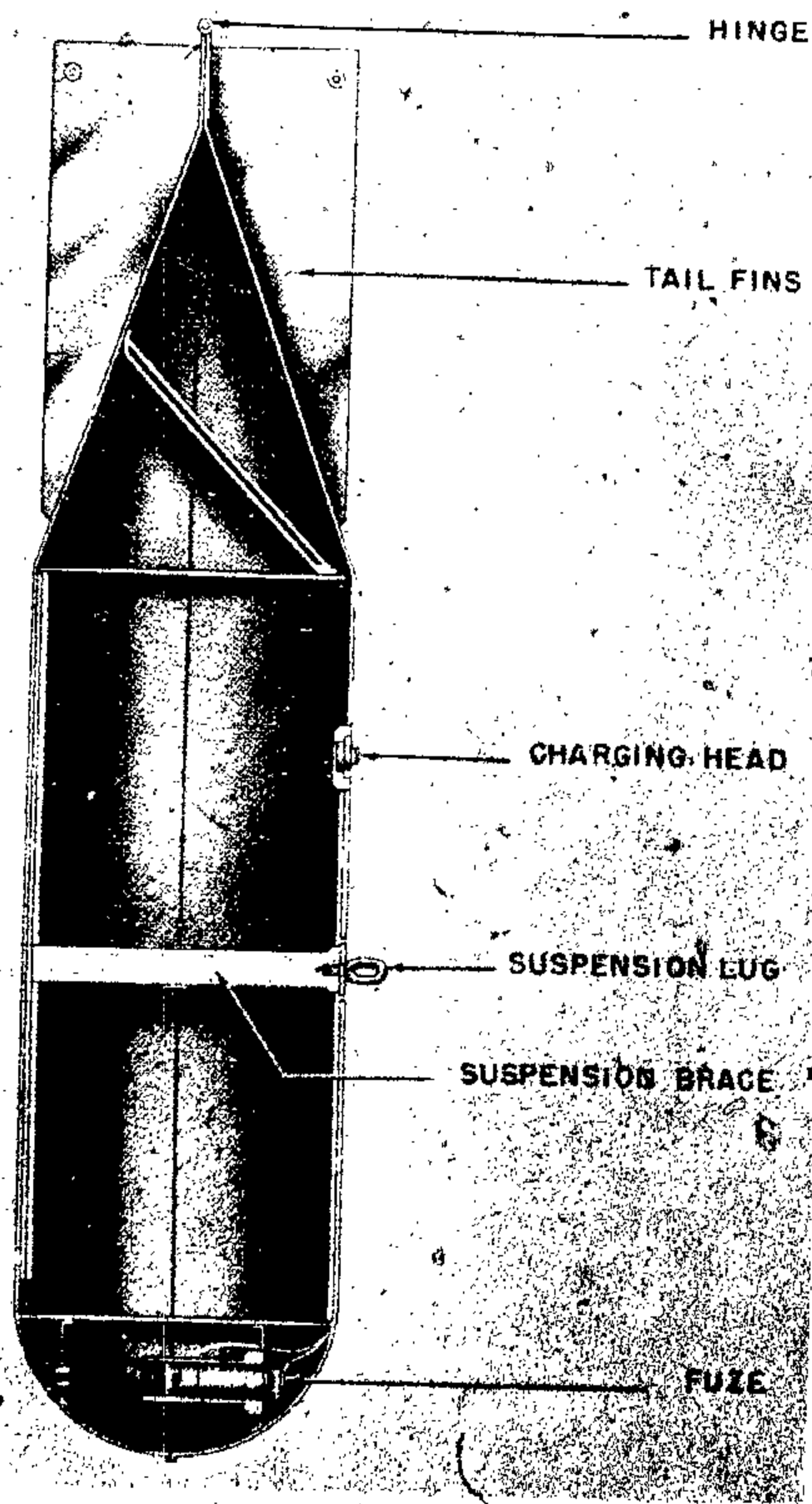
Figure 113—AB 500-1B Container
