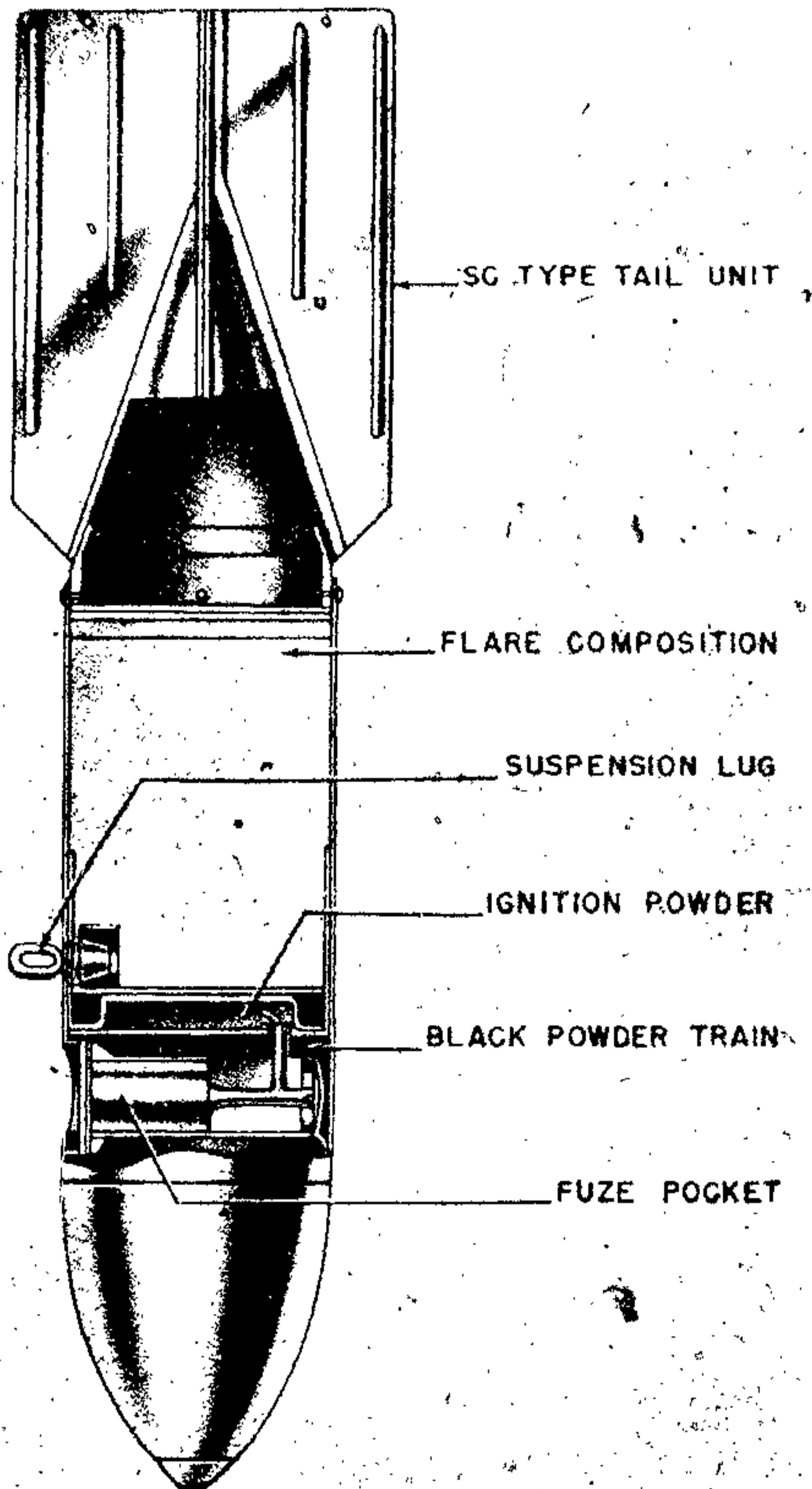
Figure 86—BLC 50 (30-Kg) Photoflash Bomb
