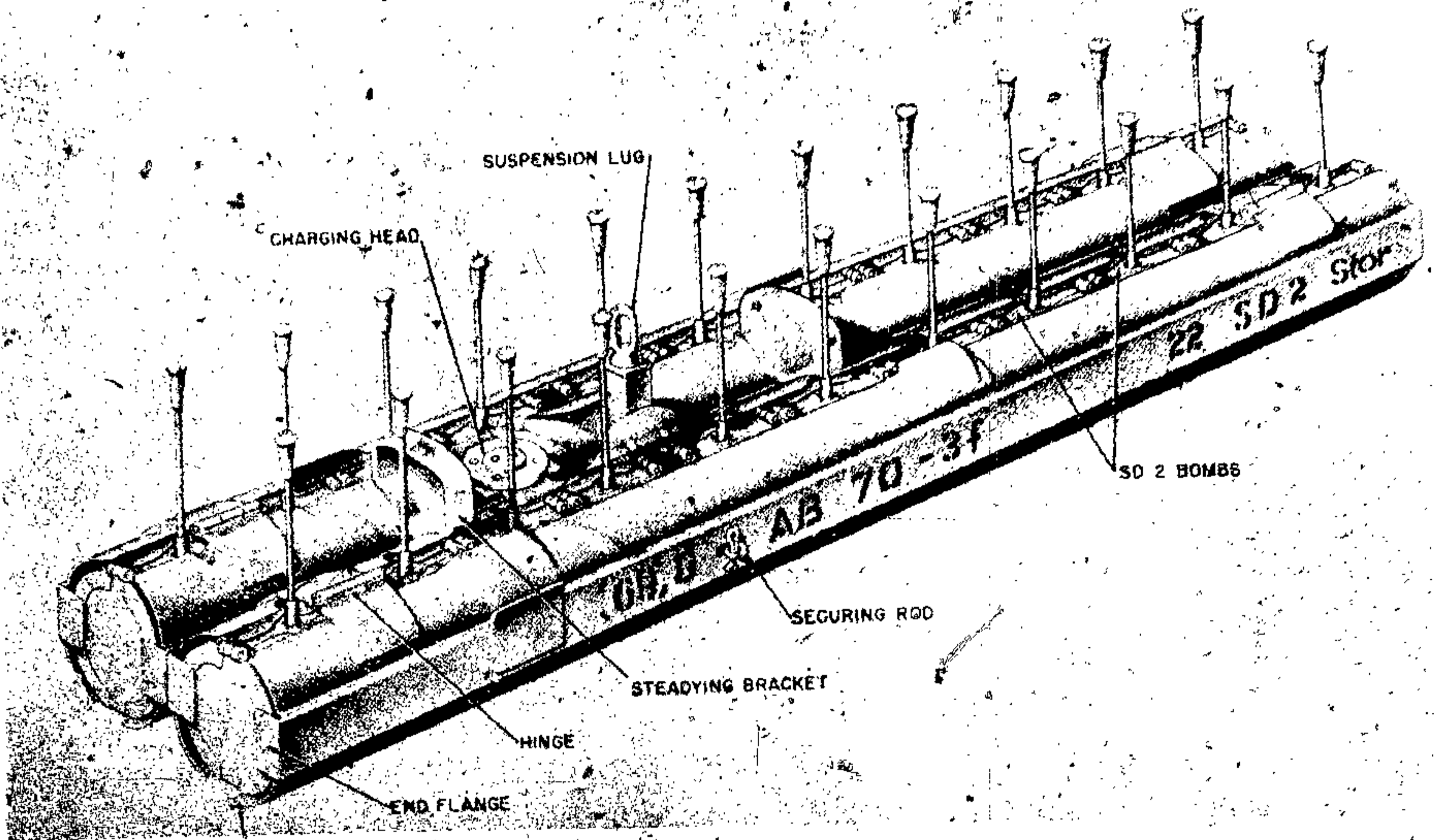
Figure 103A—AB 70-3 Container
