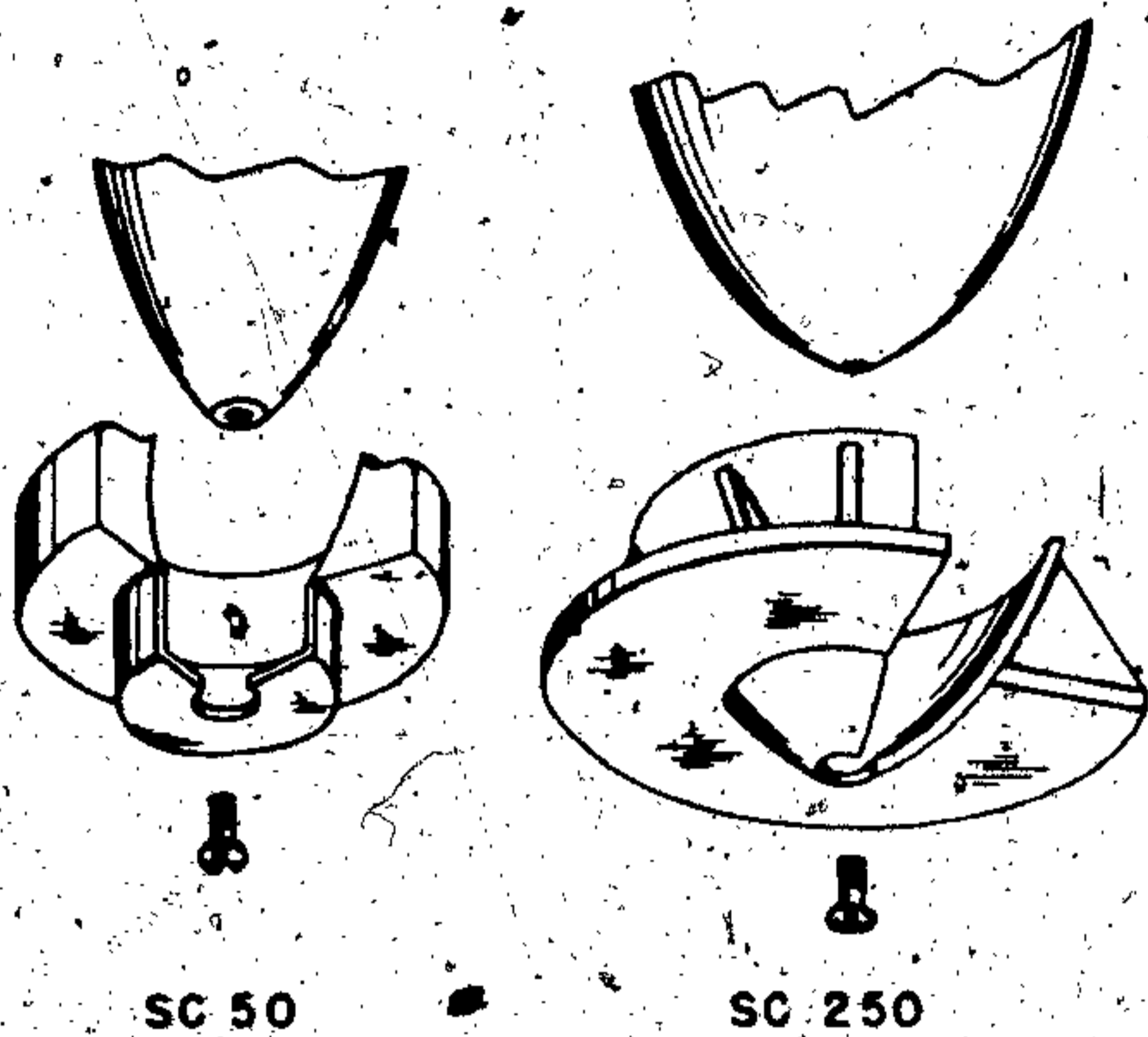
Figure 6—Antiricochet Plates
