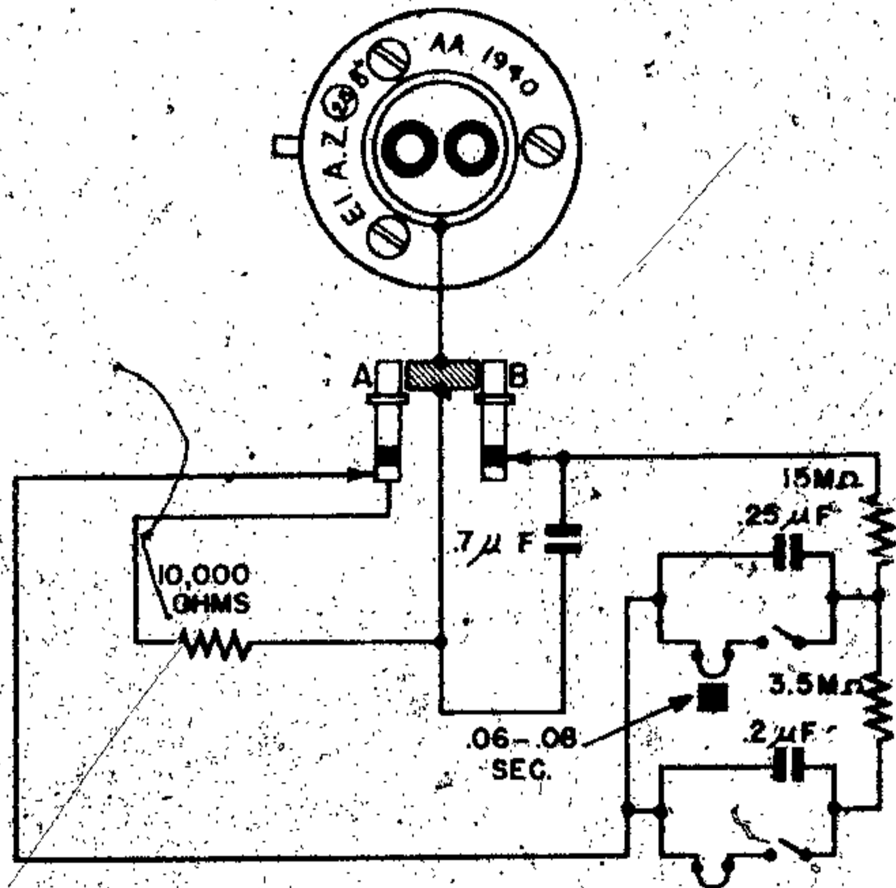
Figure 162—(28)B 07 Electrical Impact Fuze
