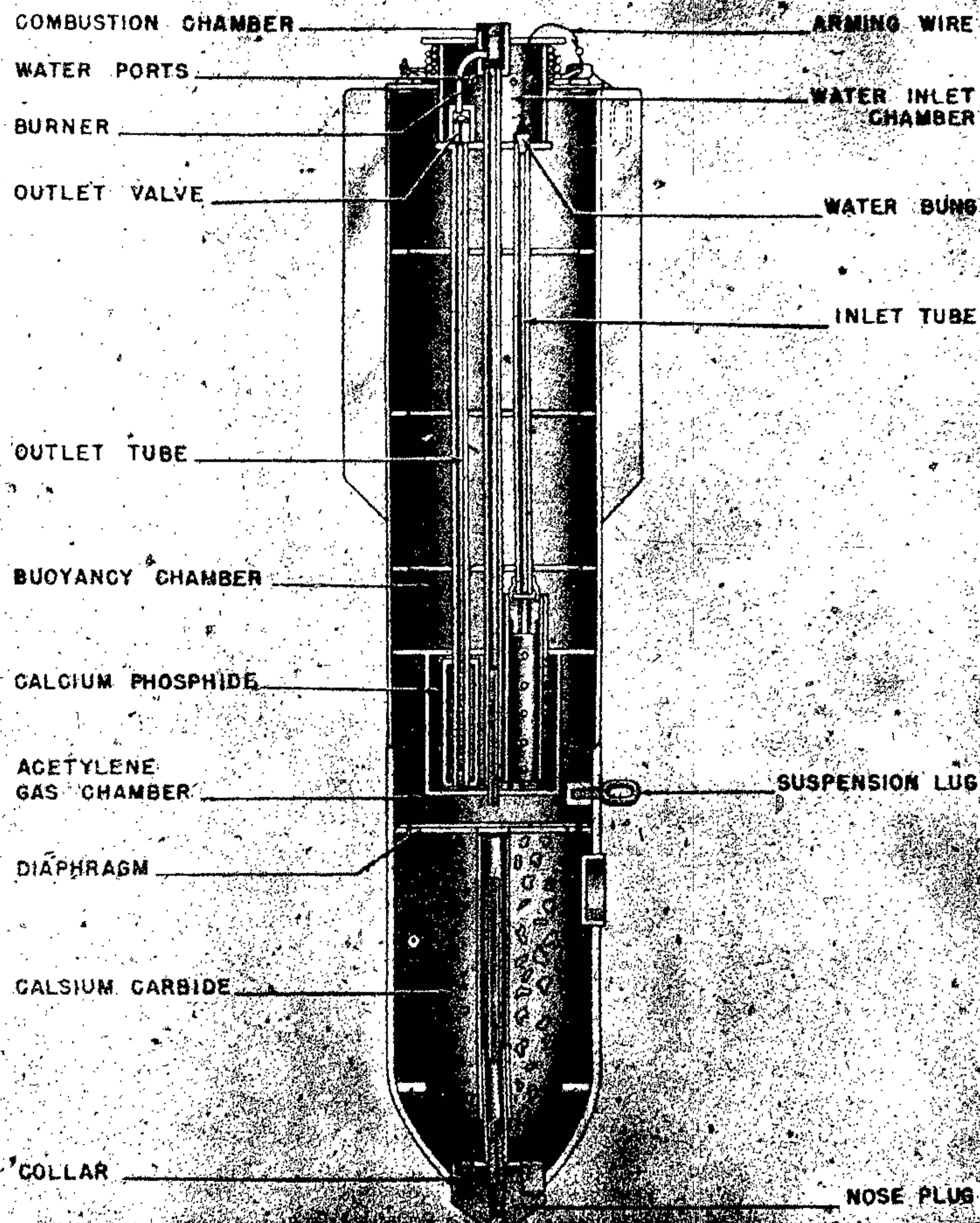
Figure 93—Lux N Flame Float
