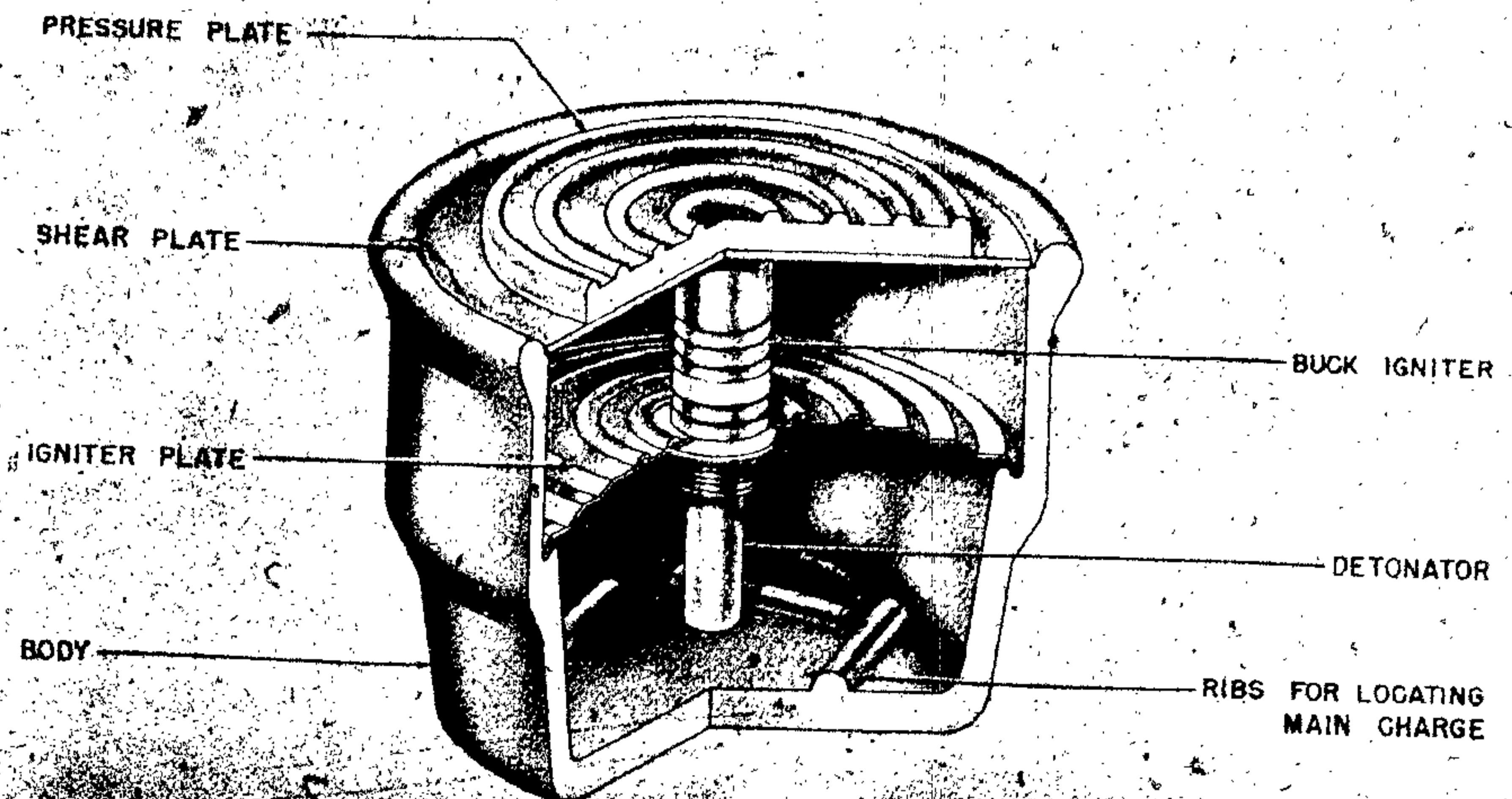
Figure 239—Glassmine 43 (f)—Antipersonnel
