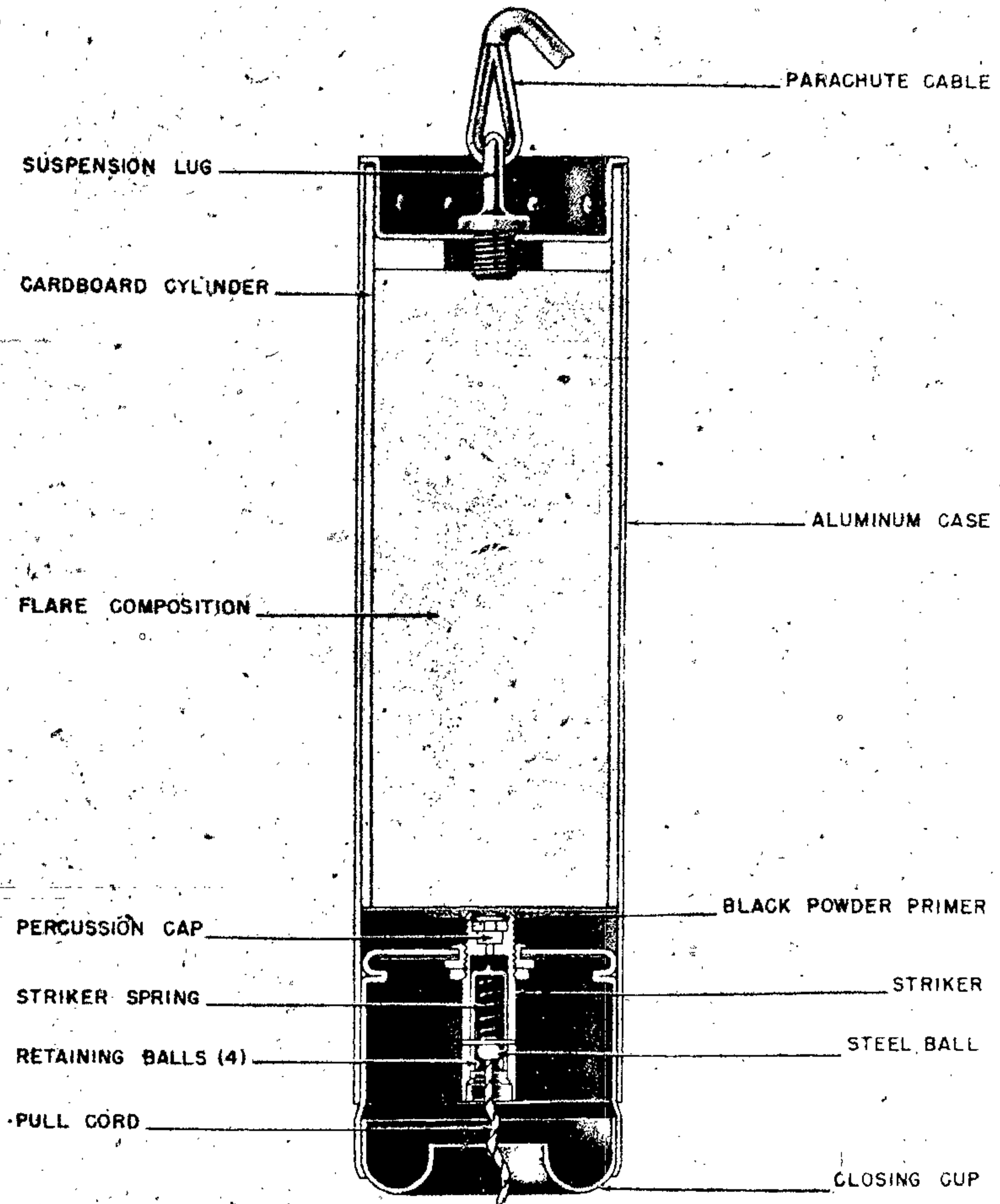
Figure 78—Parachute Flare (White)—Single Unit
