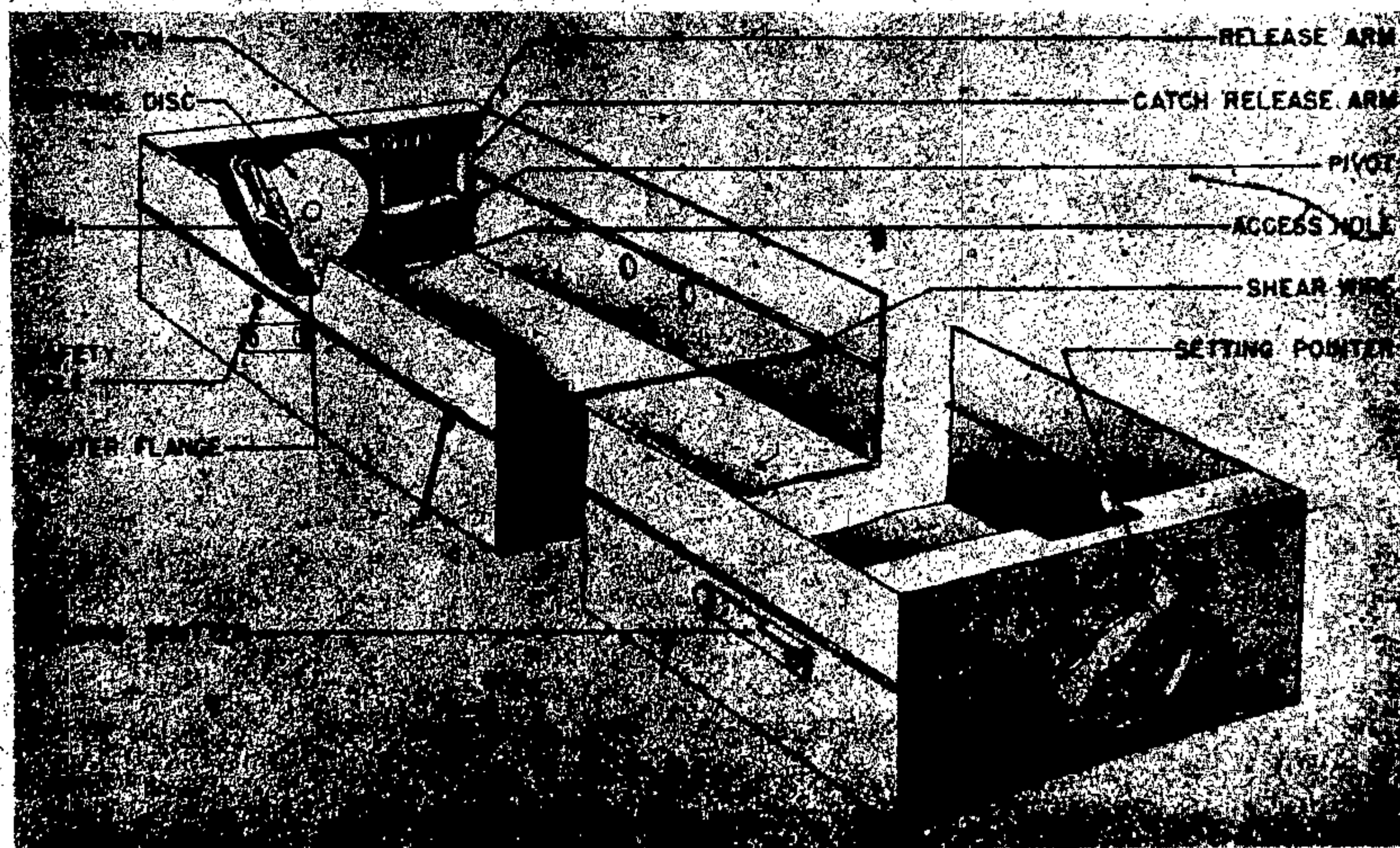
Figure 228—Spreng Riegel 8-Kg Antitank Mine
