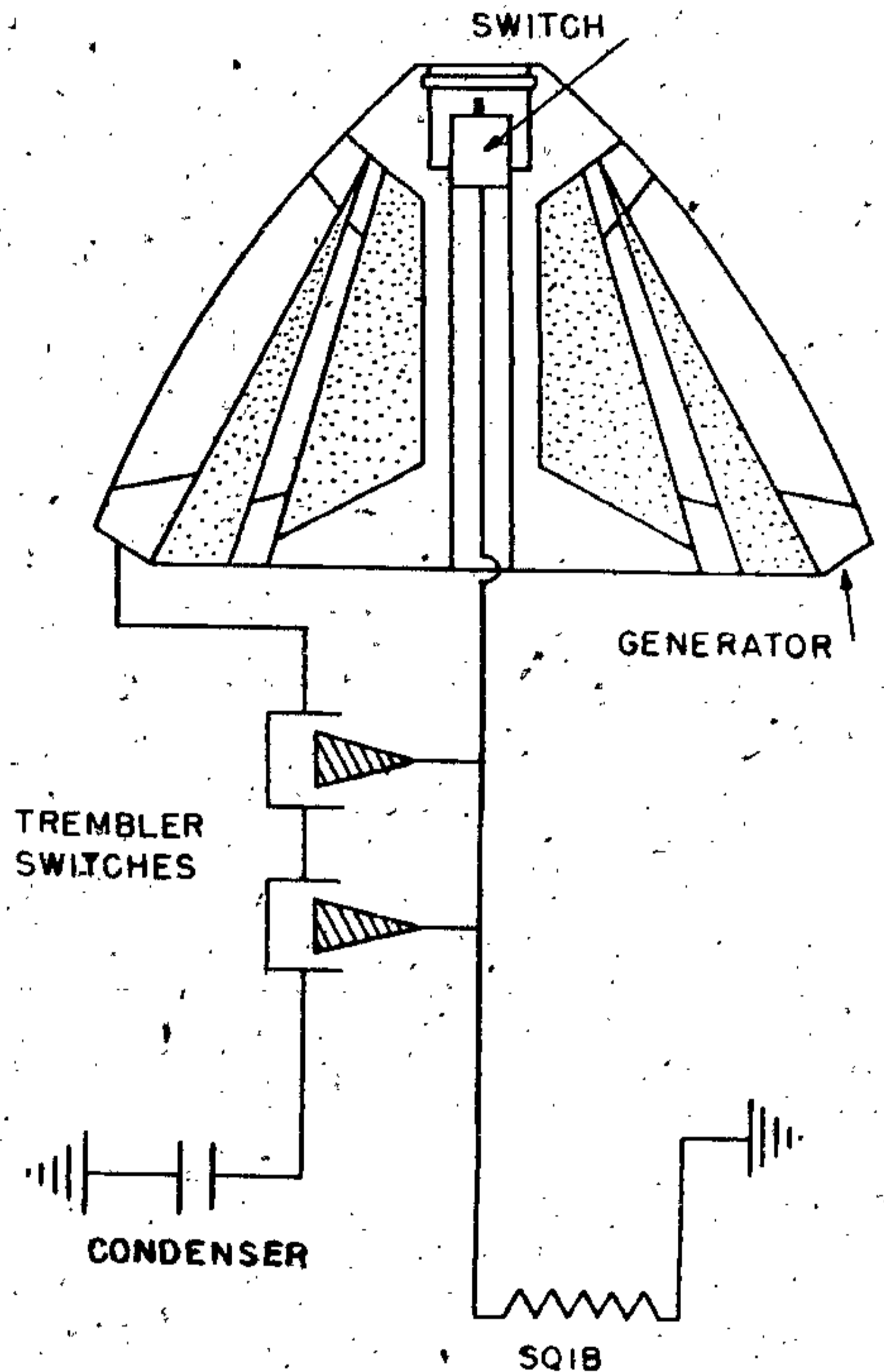
Figure 191B—Dust Fuze for SD 10 Bomb Wiring Diagram
