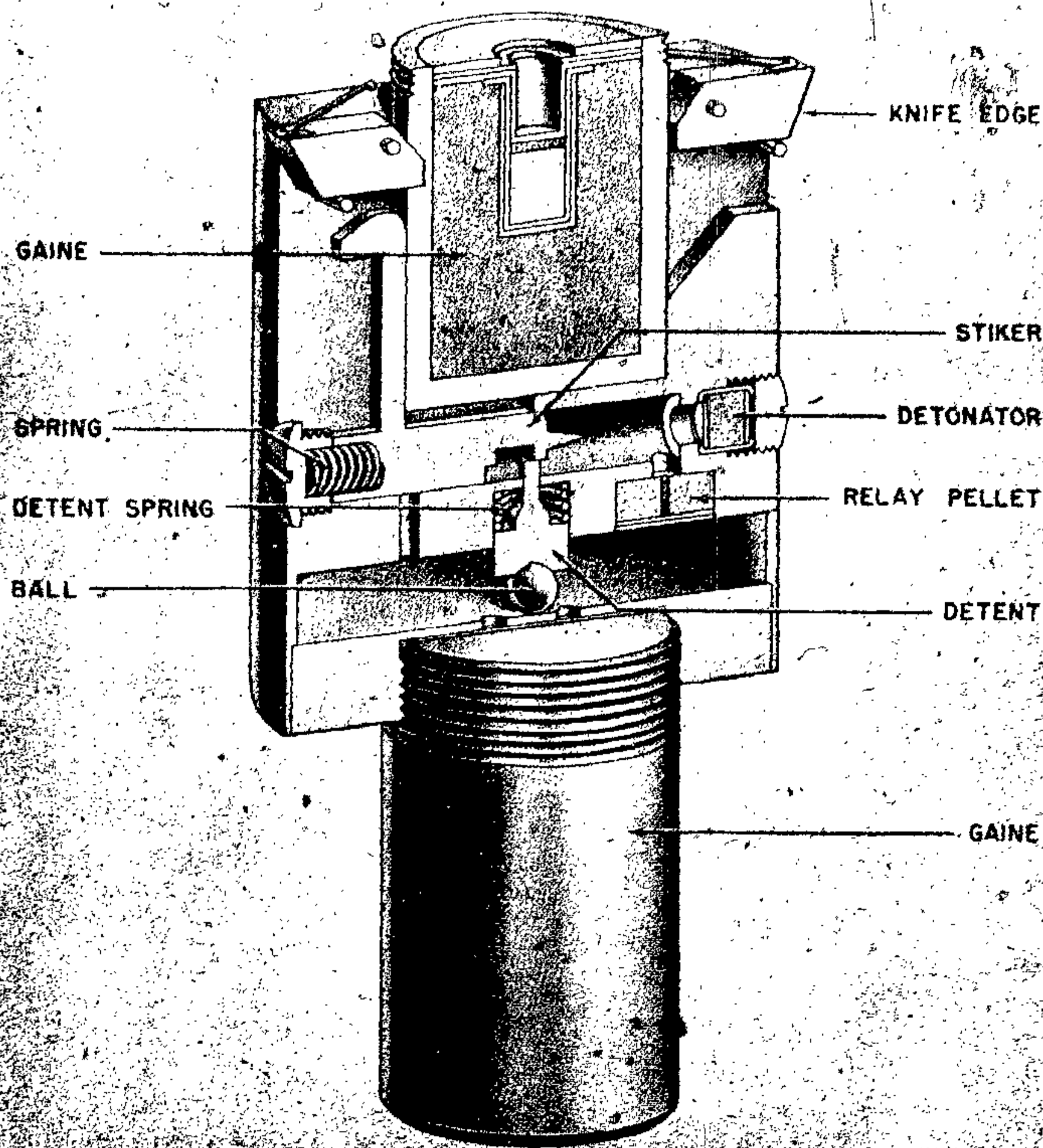
Figure 181—ZUS 40 (Type I) Mechanical Antiwithdrawal
