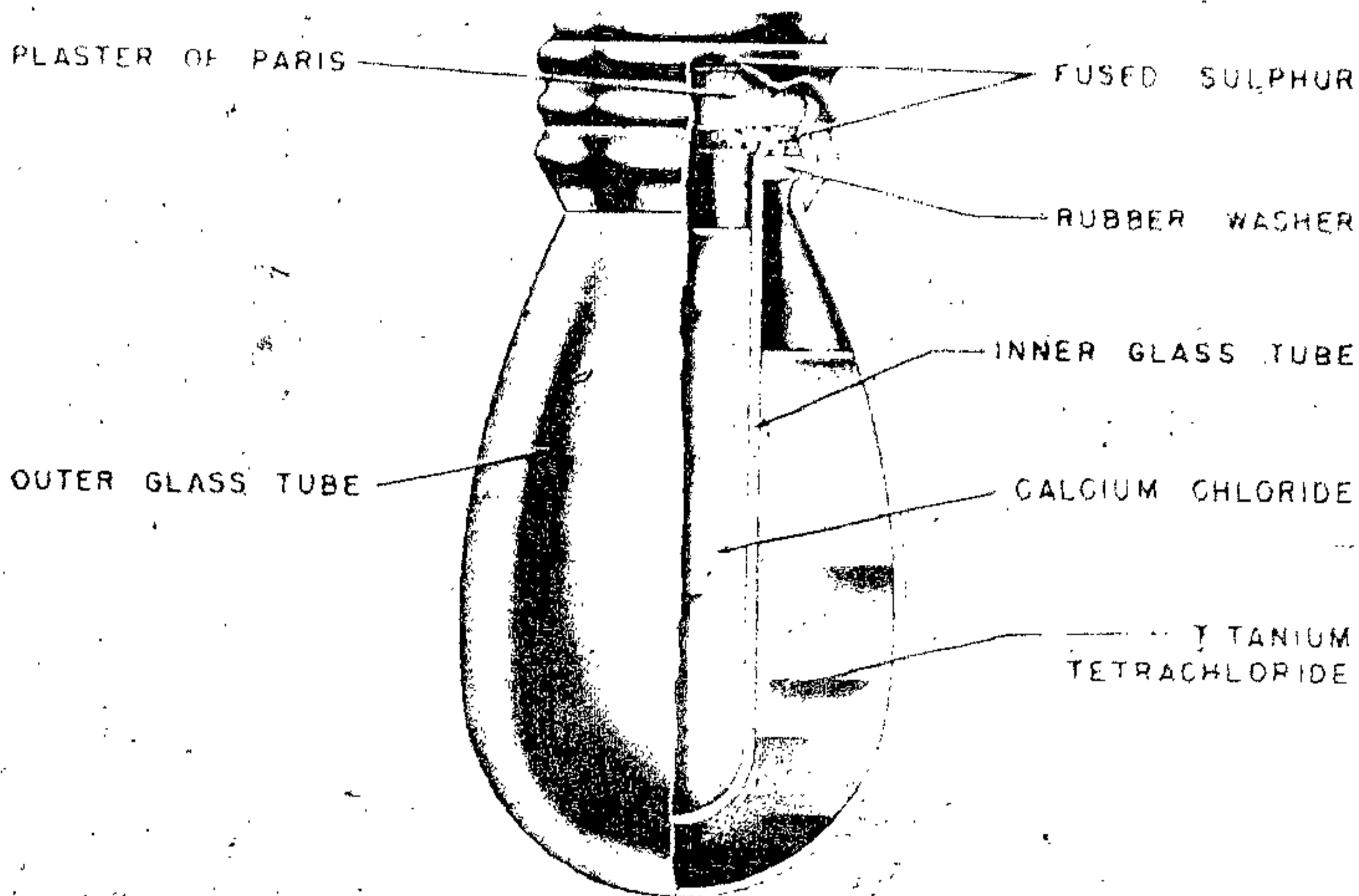
Figure 294—Blendkorper 24 Smoke Hand Grenade
