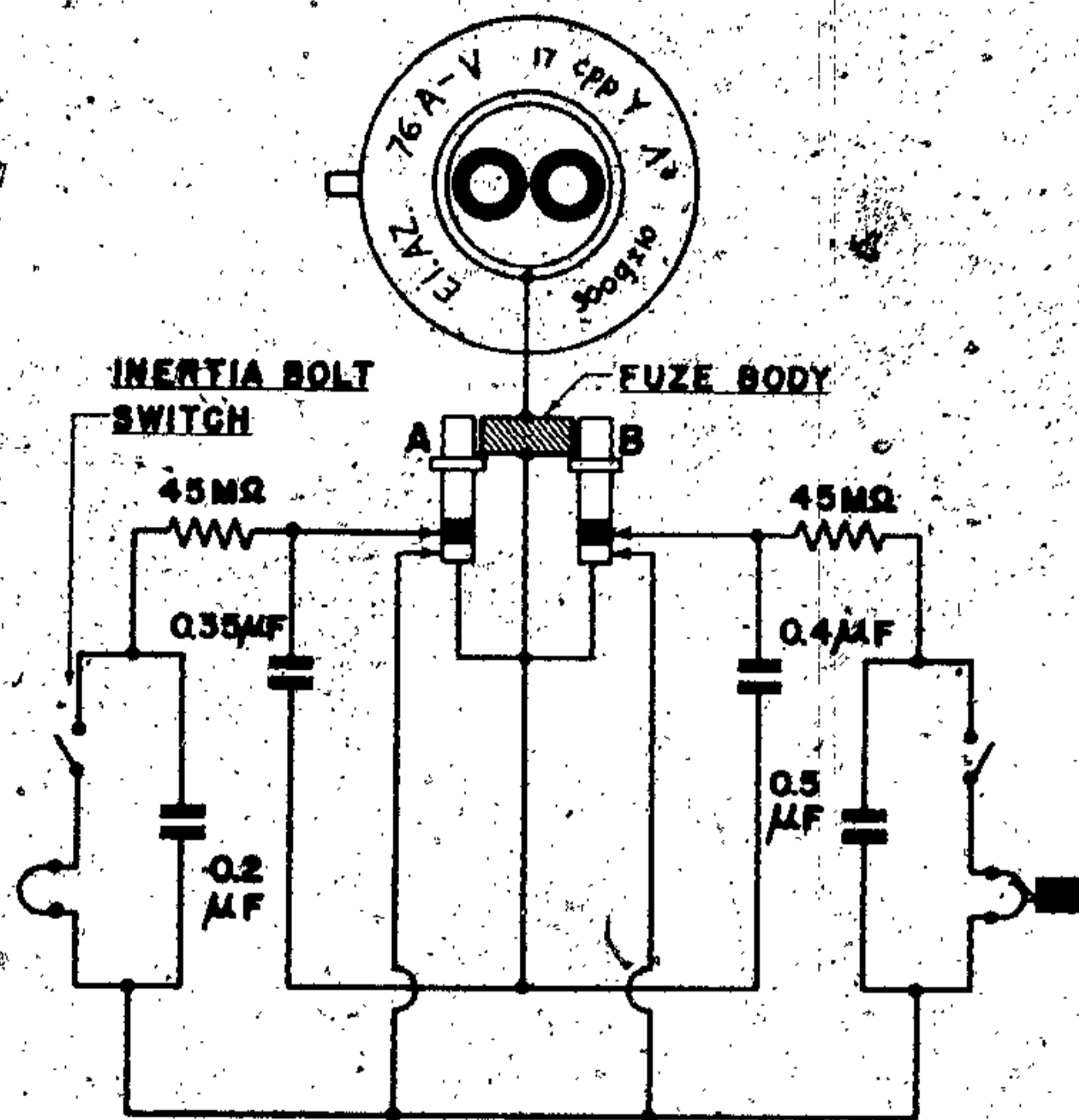
Figure 150—(76)A Electrical Impact Fuze
