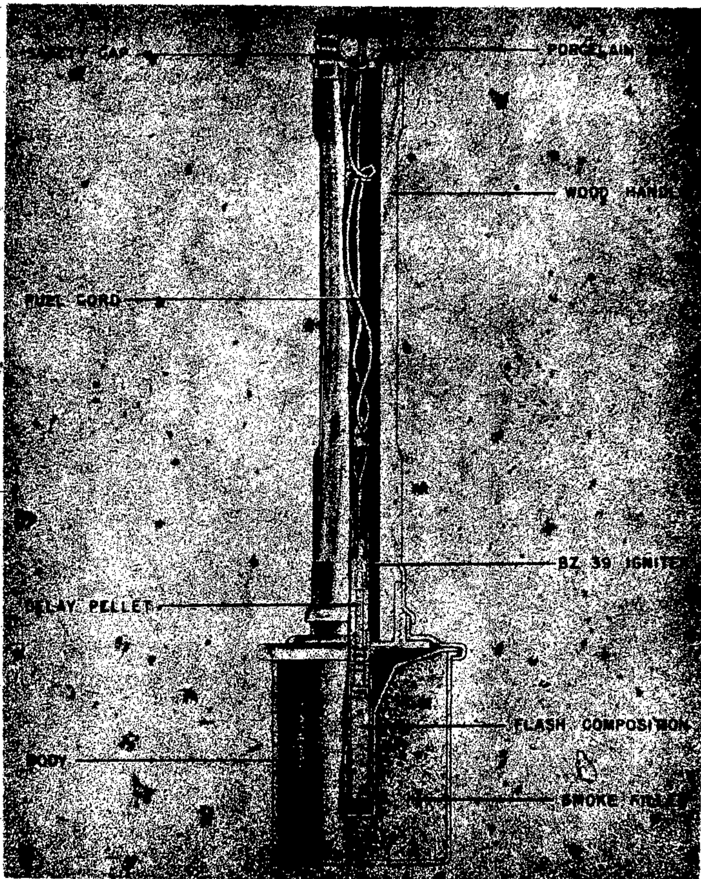
Figure 292—Type 39 Smoke Hand Grenade
