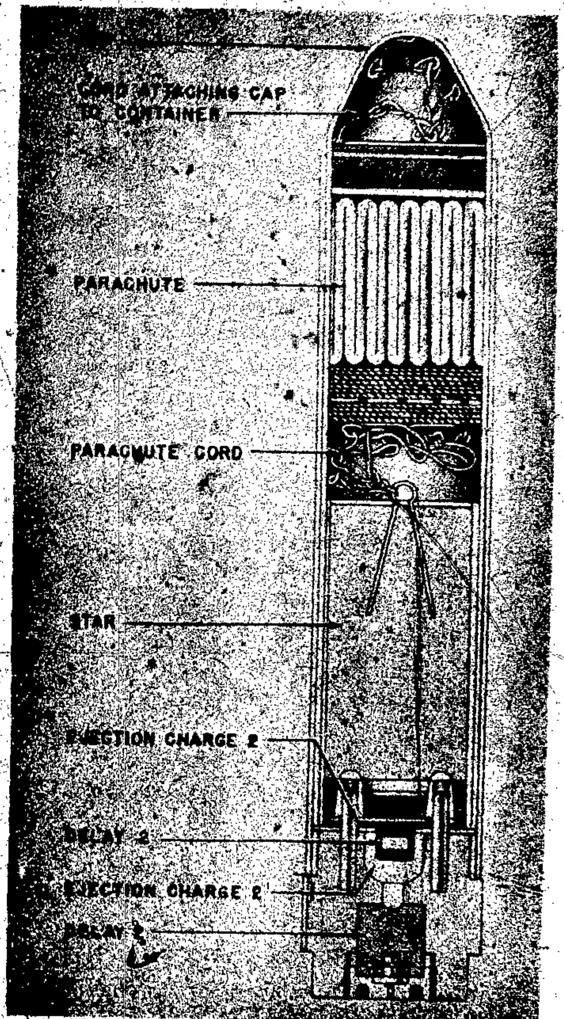
Figure 307—Illuminating Rifle Grenade
