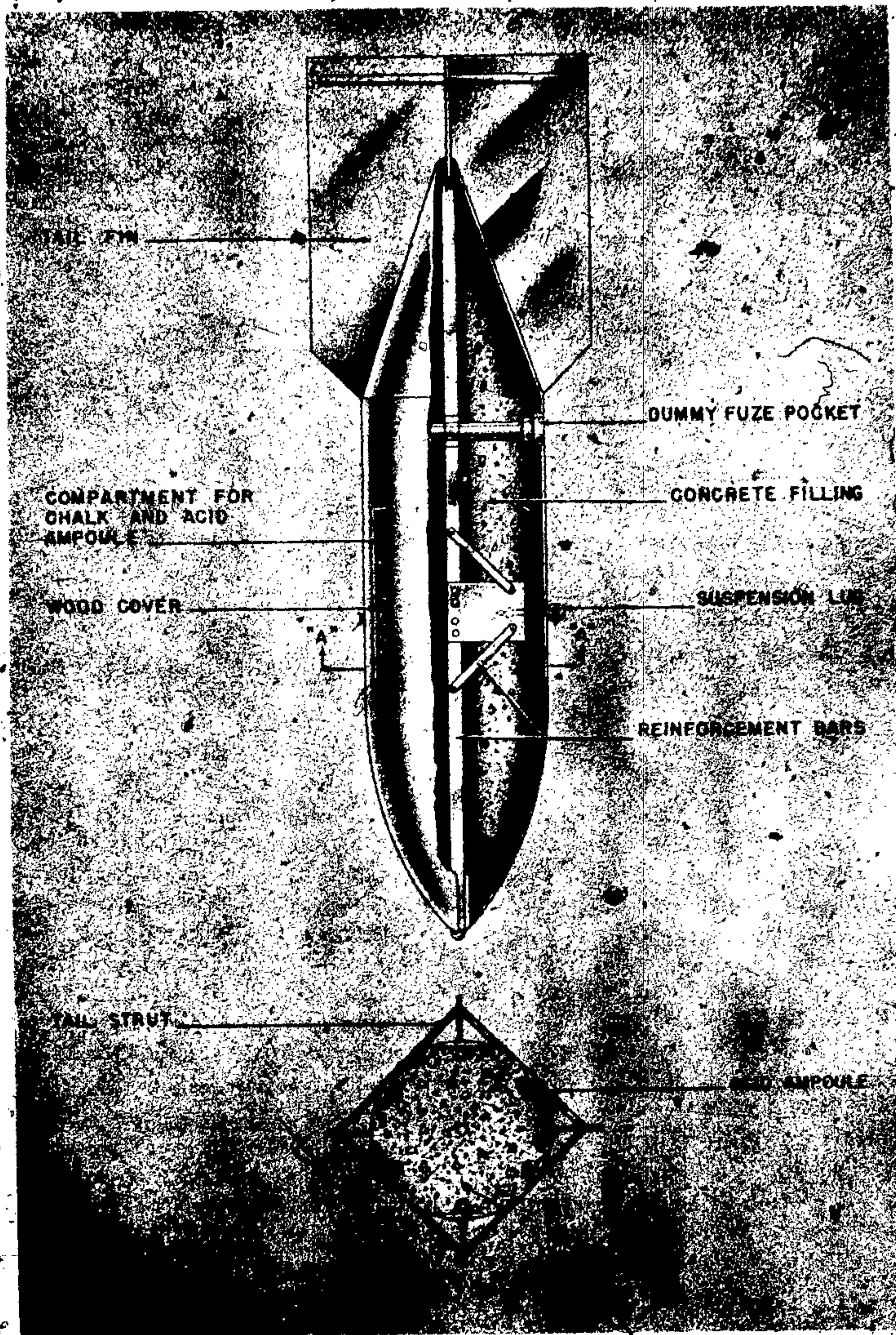
Figure 69—ZC 250-Kg Concrete Practice Bomb (Smoke)
