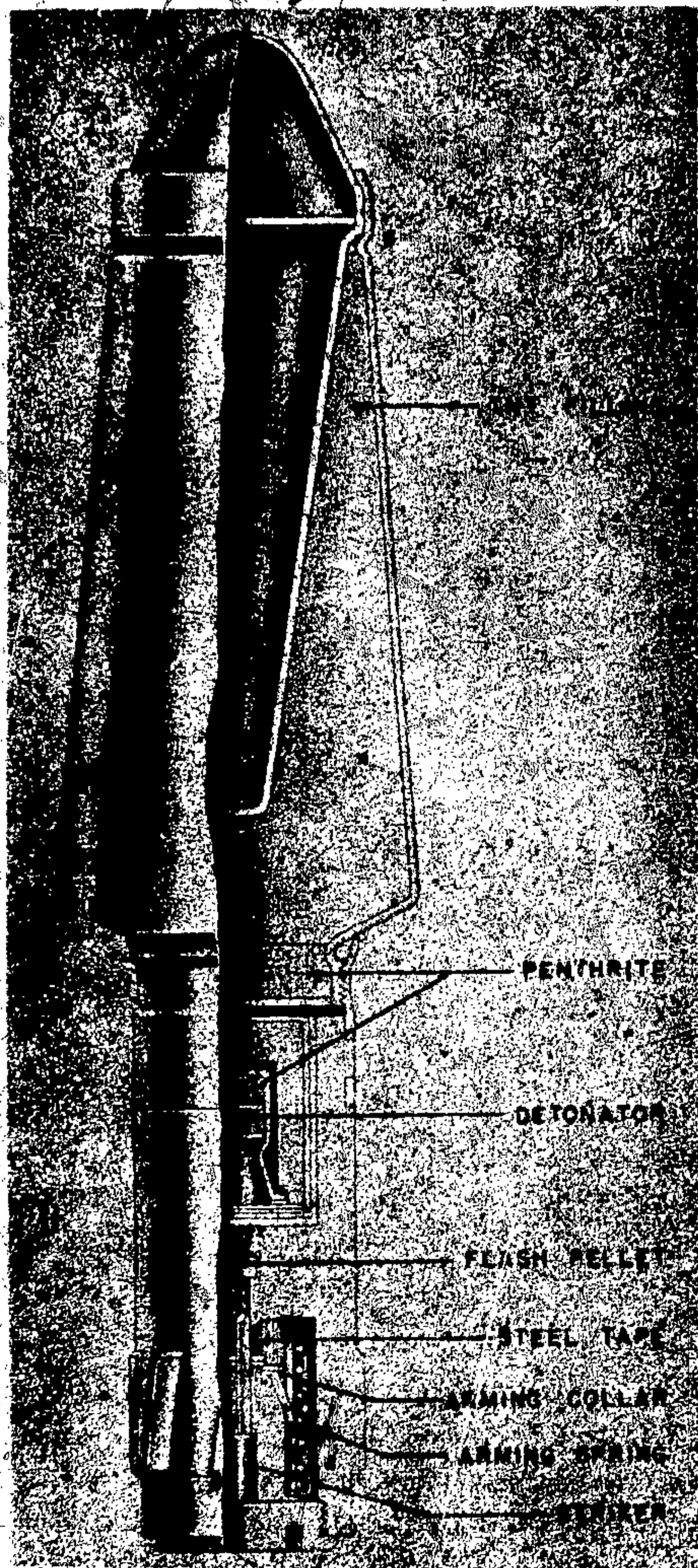
Figure 304—Large Hollow Charge Rifle Grenade
