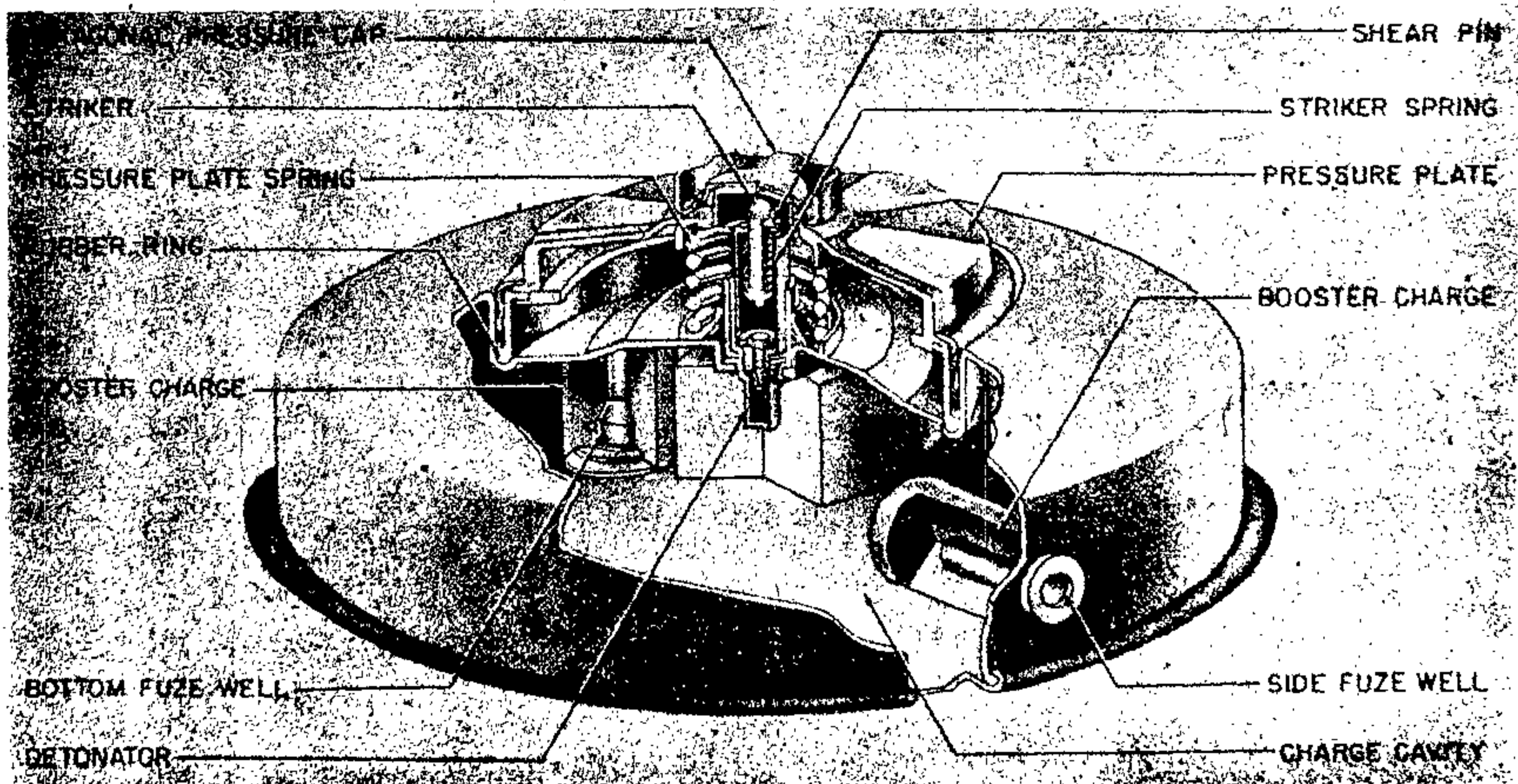
Figure 232—Tellermine 42—Antitank
