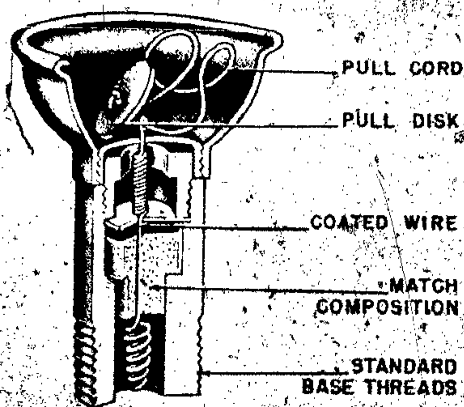
Figure 252—ZDSCHN-ANZ-39 Friction Igniter Pull Type
