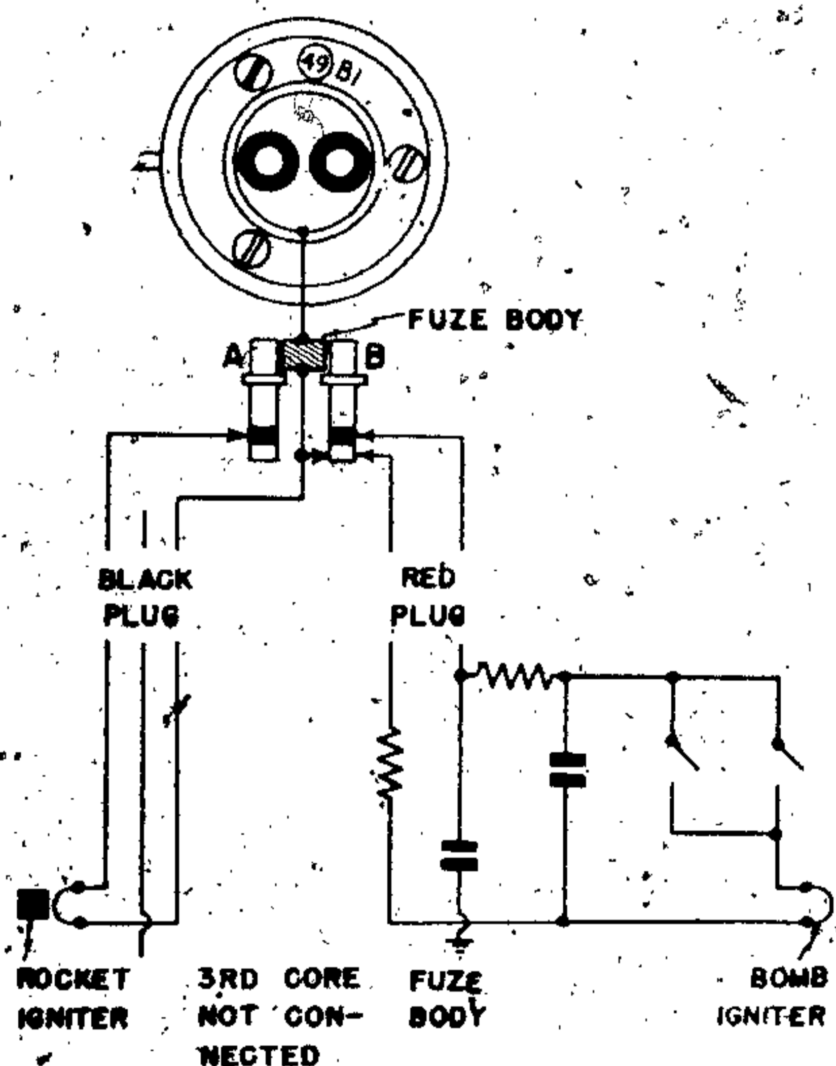
Figure 171—(49)B Rocket Bomb Fuze Assembly
