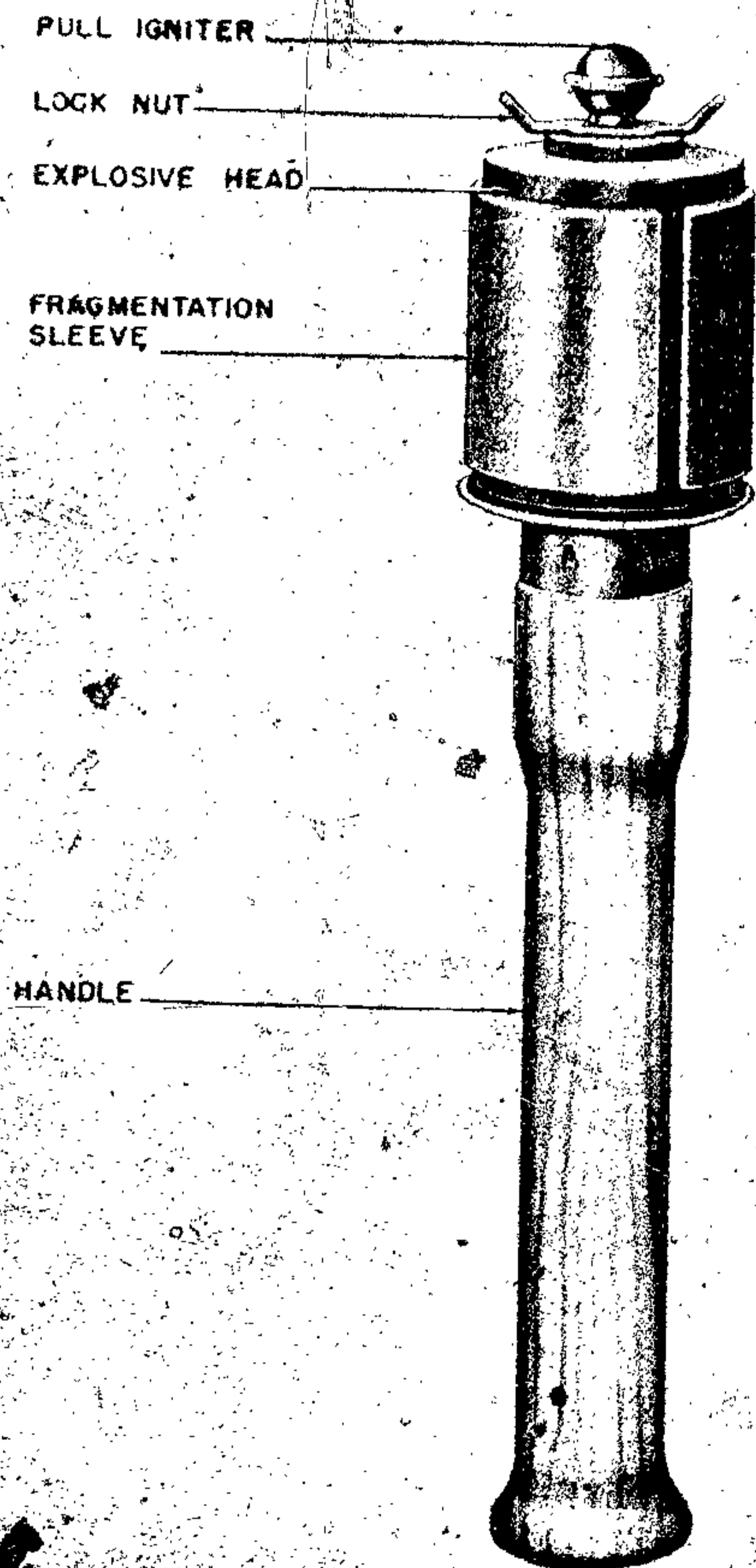
Figure 285—Model 43 Stick Hand Grenade
