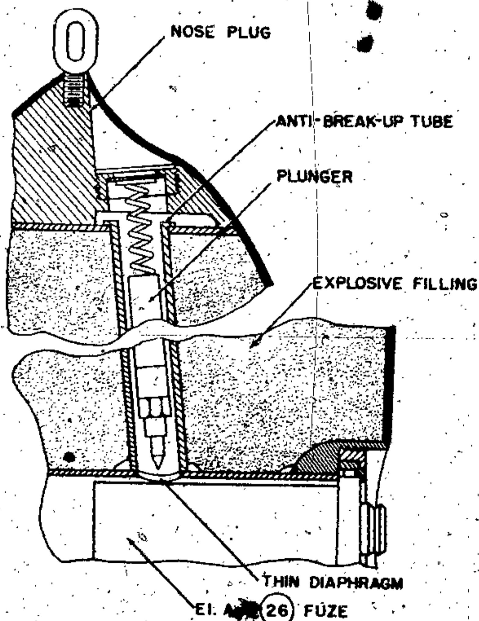
Figure 147A—(26) Electrical Impact (Special)
