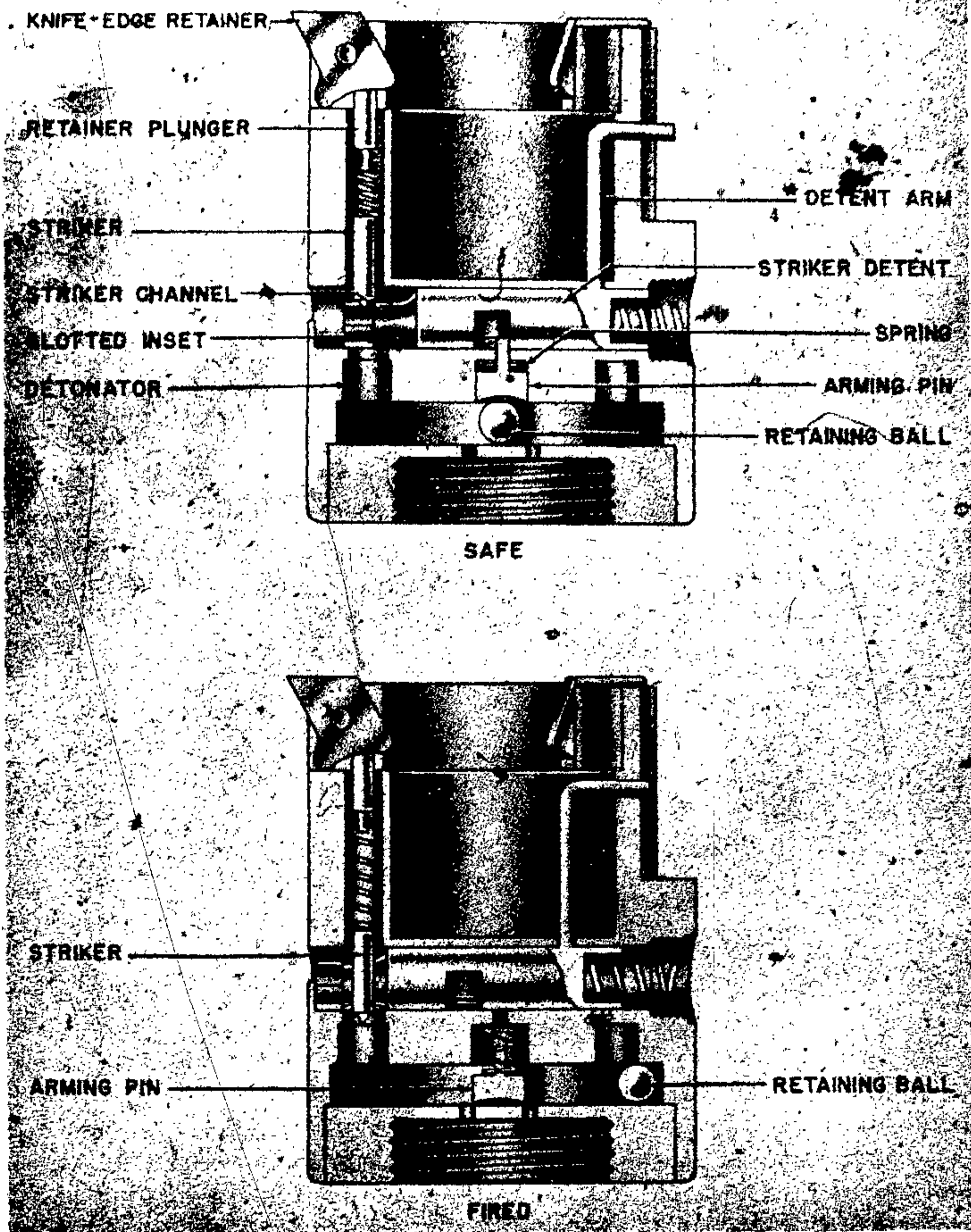
Figure 182—ZUS 40 (Type III) Mechanical Antiwithdrawal
