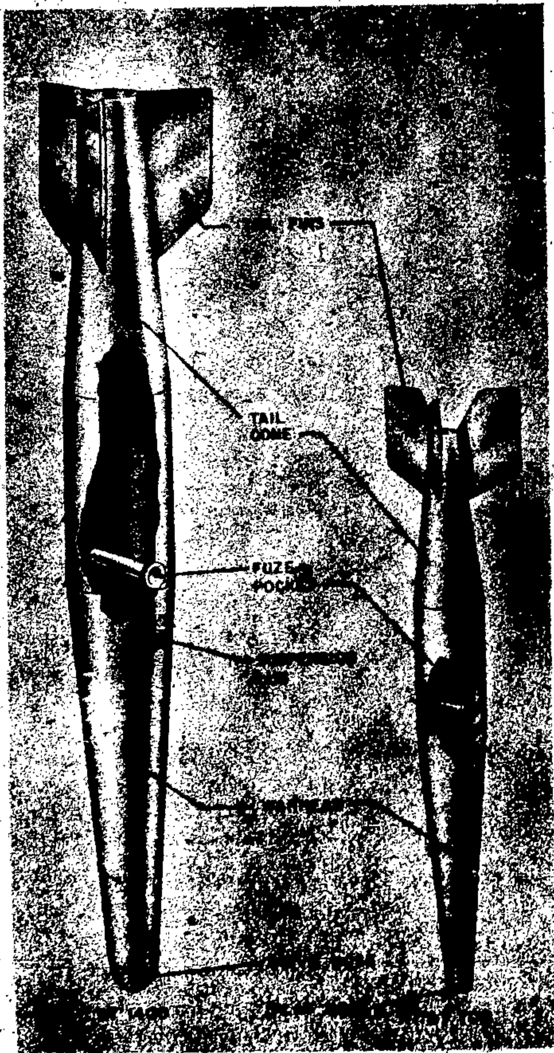
Figure 49—1400-Kg Bomber Torpedo
