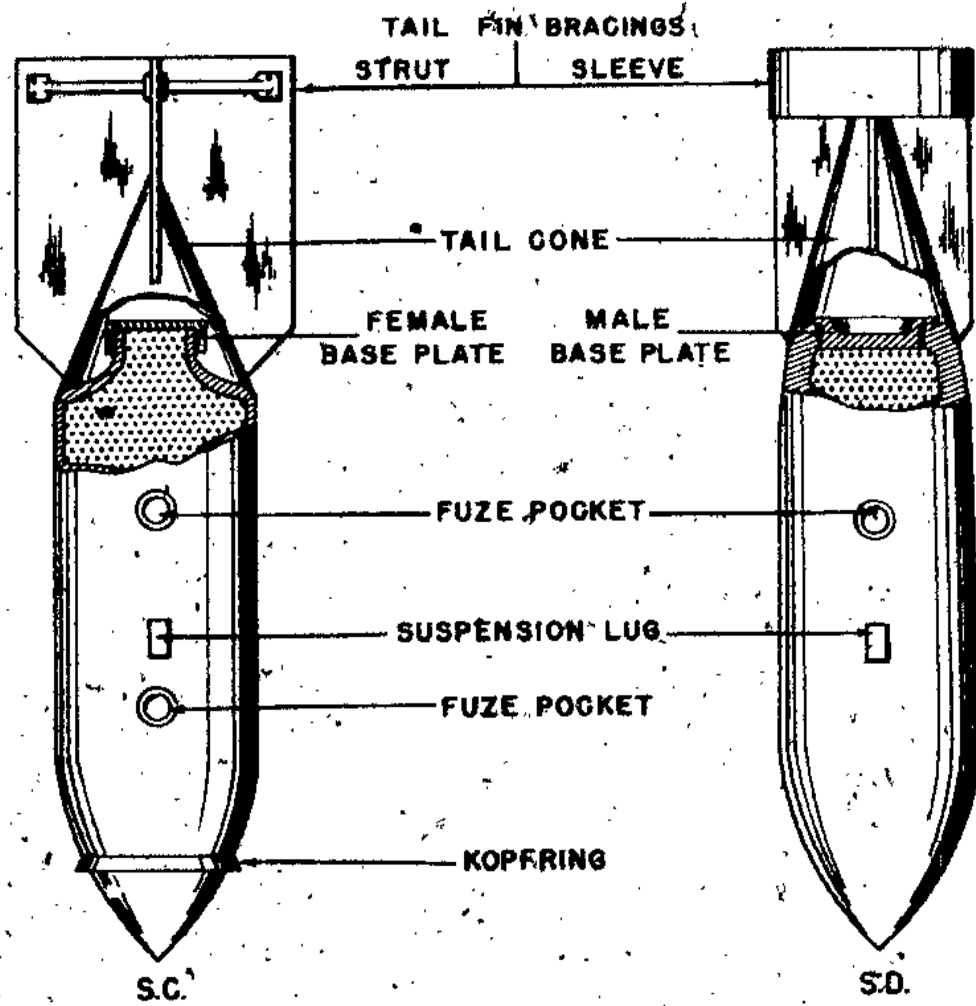
Figure 1—Bomb Component Positions
