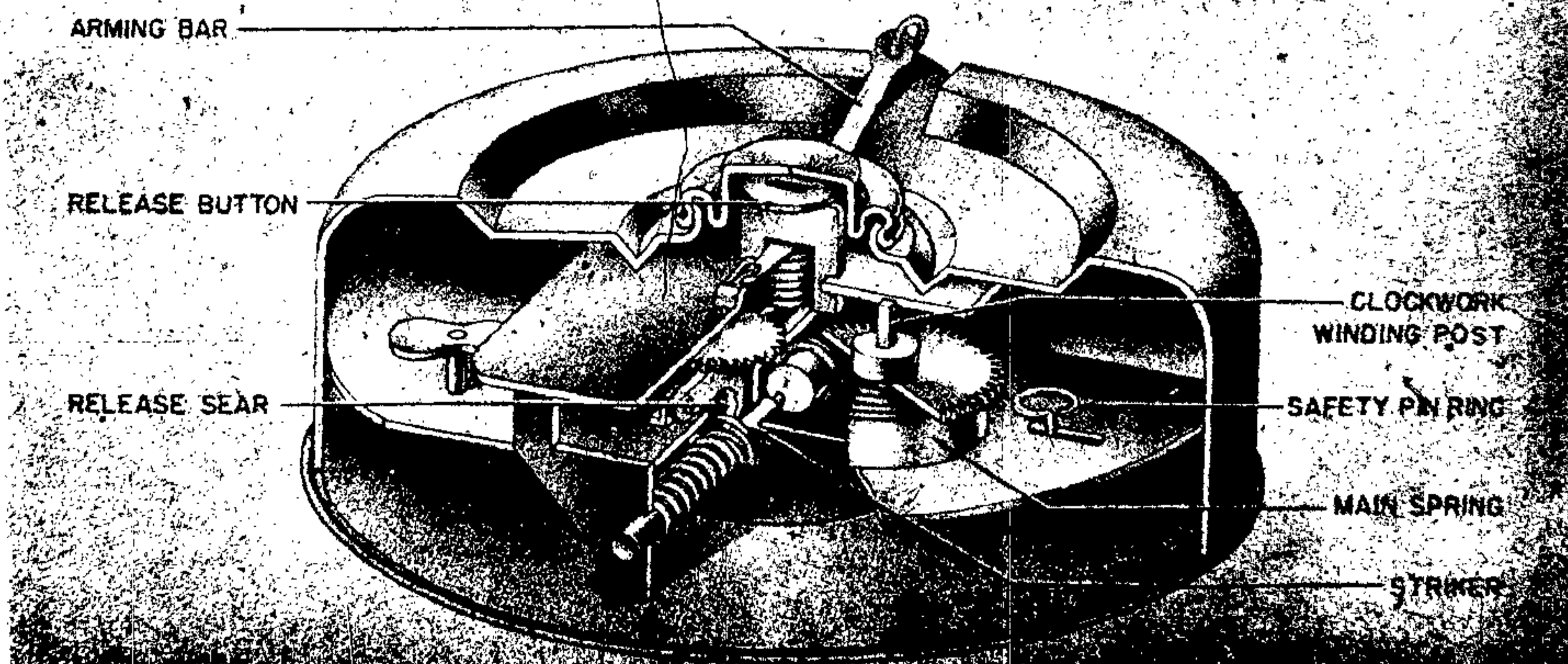
Figure 283—E. Z. 44 Antilifting Device
