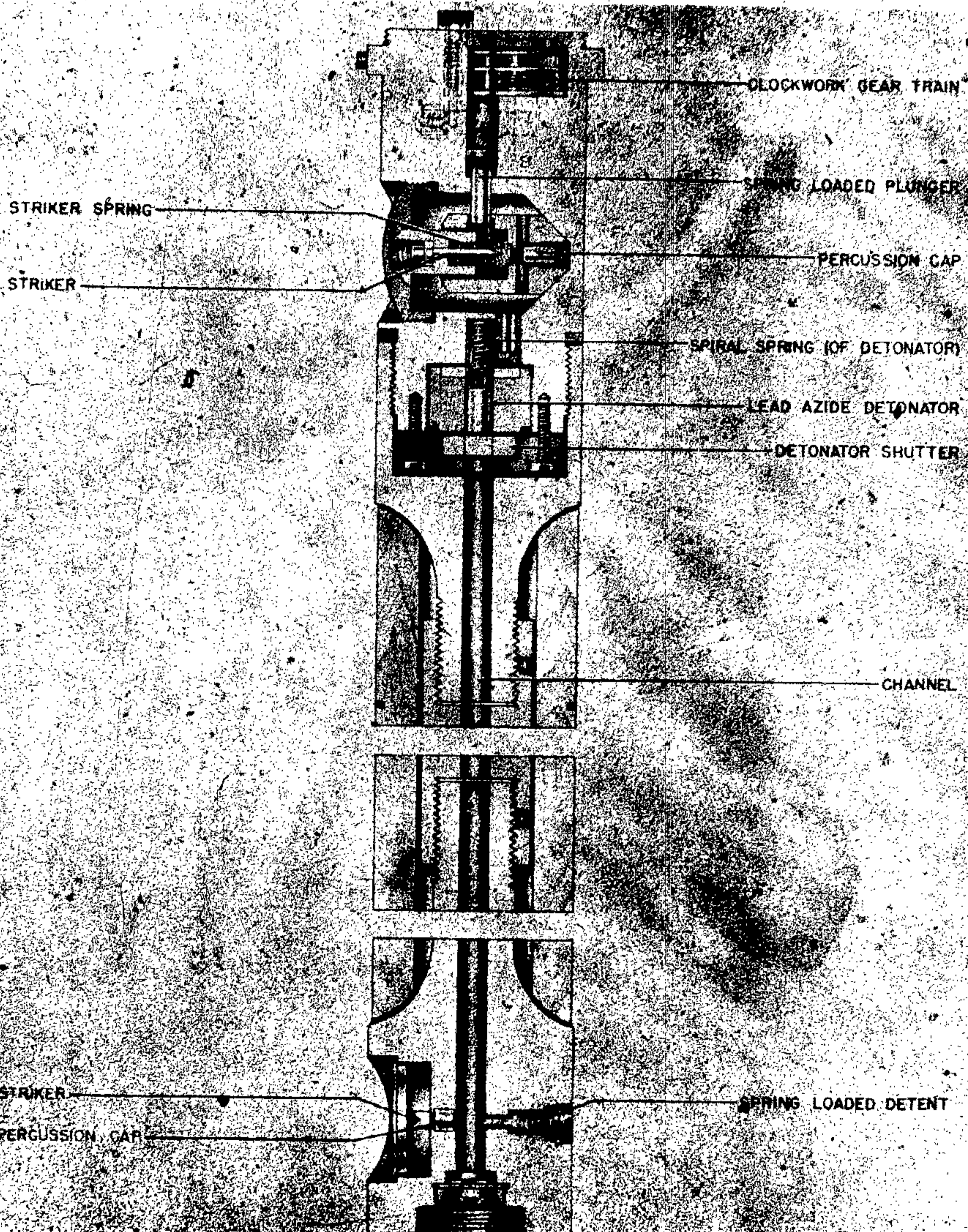
Figure 135—(24) Mechanical Antibreak-up Fuze
