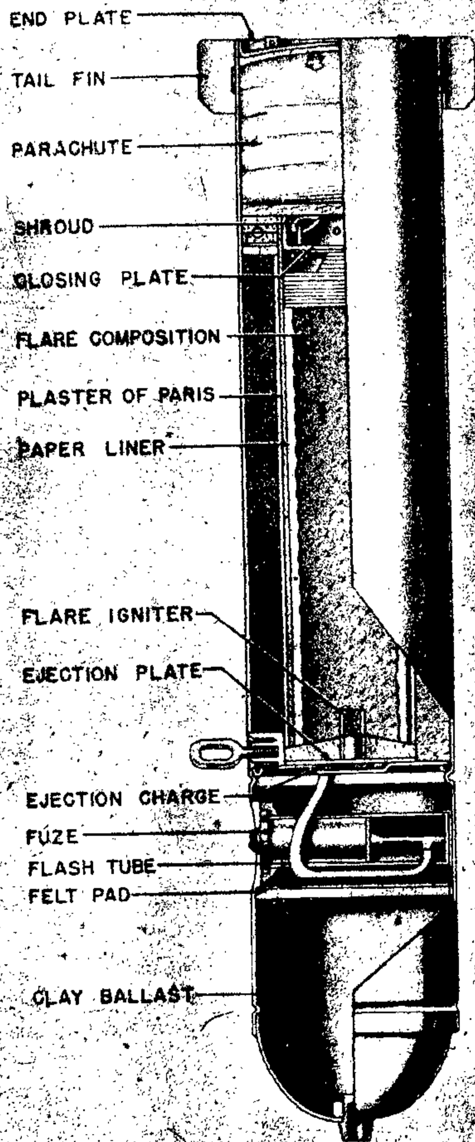
Figure 73—LC 50 F Ausf. E Parachute Flare
