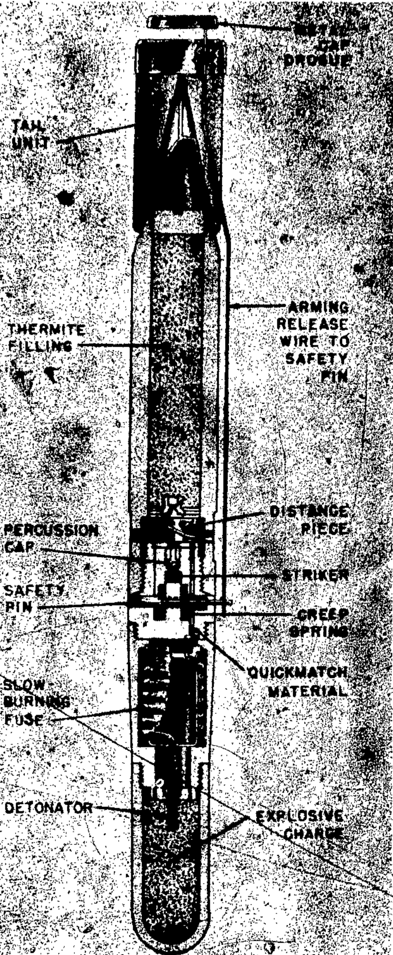
Figure 53—2.2-Kg B2.2EZ Incendiary Bomb
