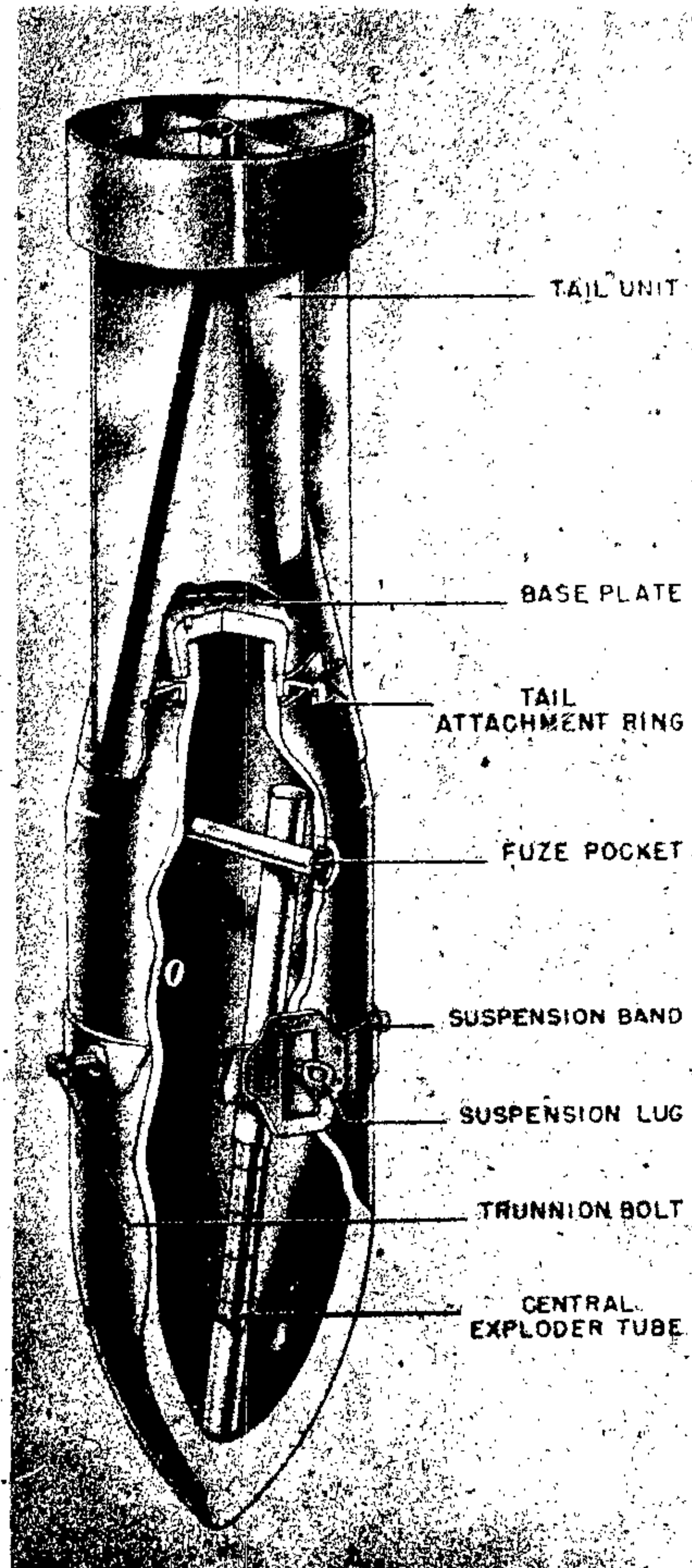
Figure 27—SD 500-Kg Bomb
