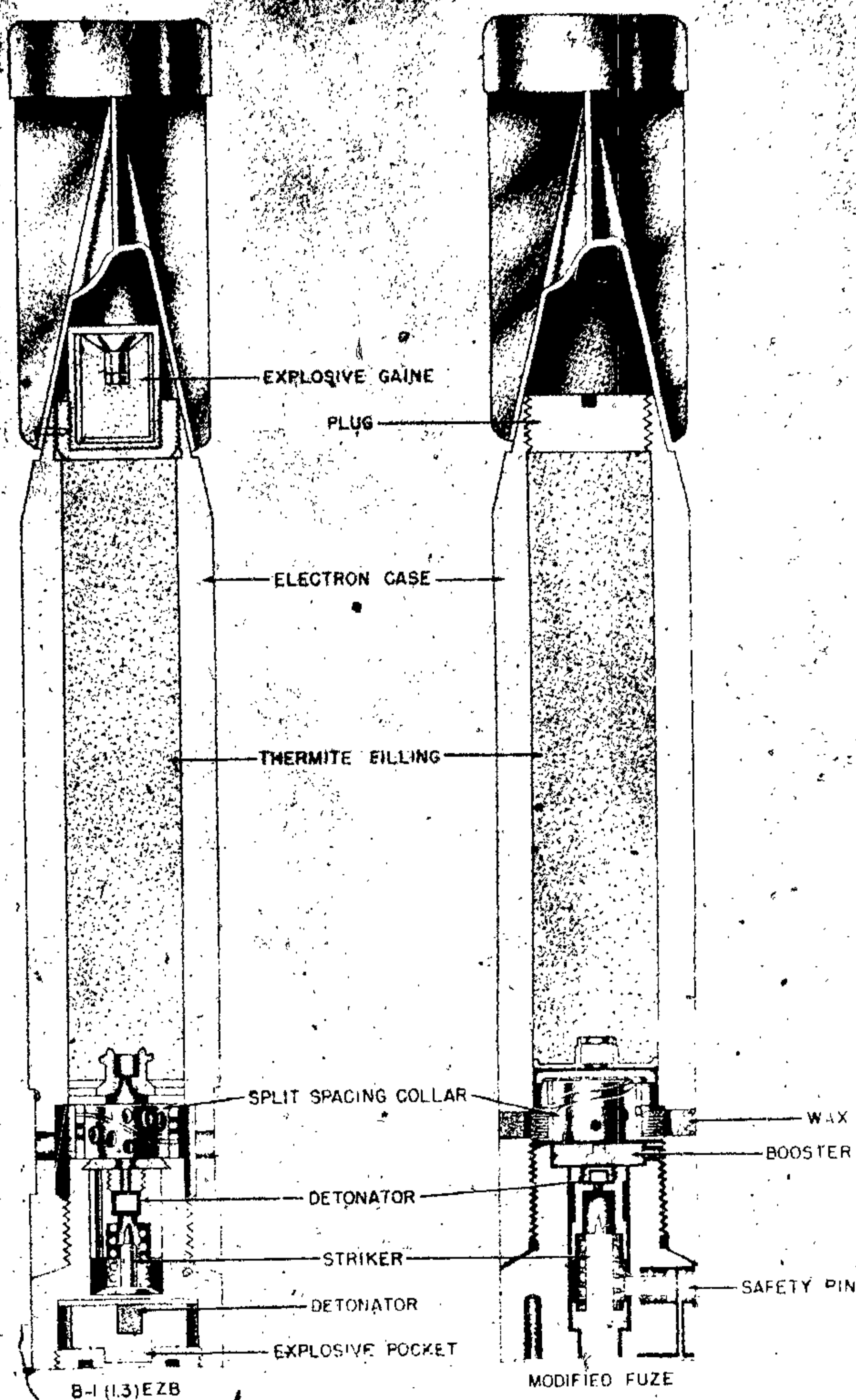
Figure 51—1-Kg B1E, B1EZE, B1EZB Incendiary Bomb
