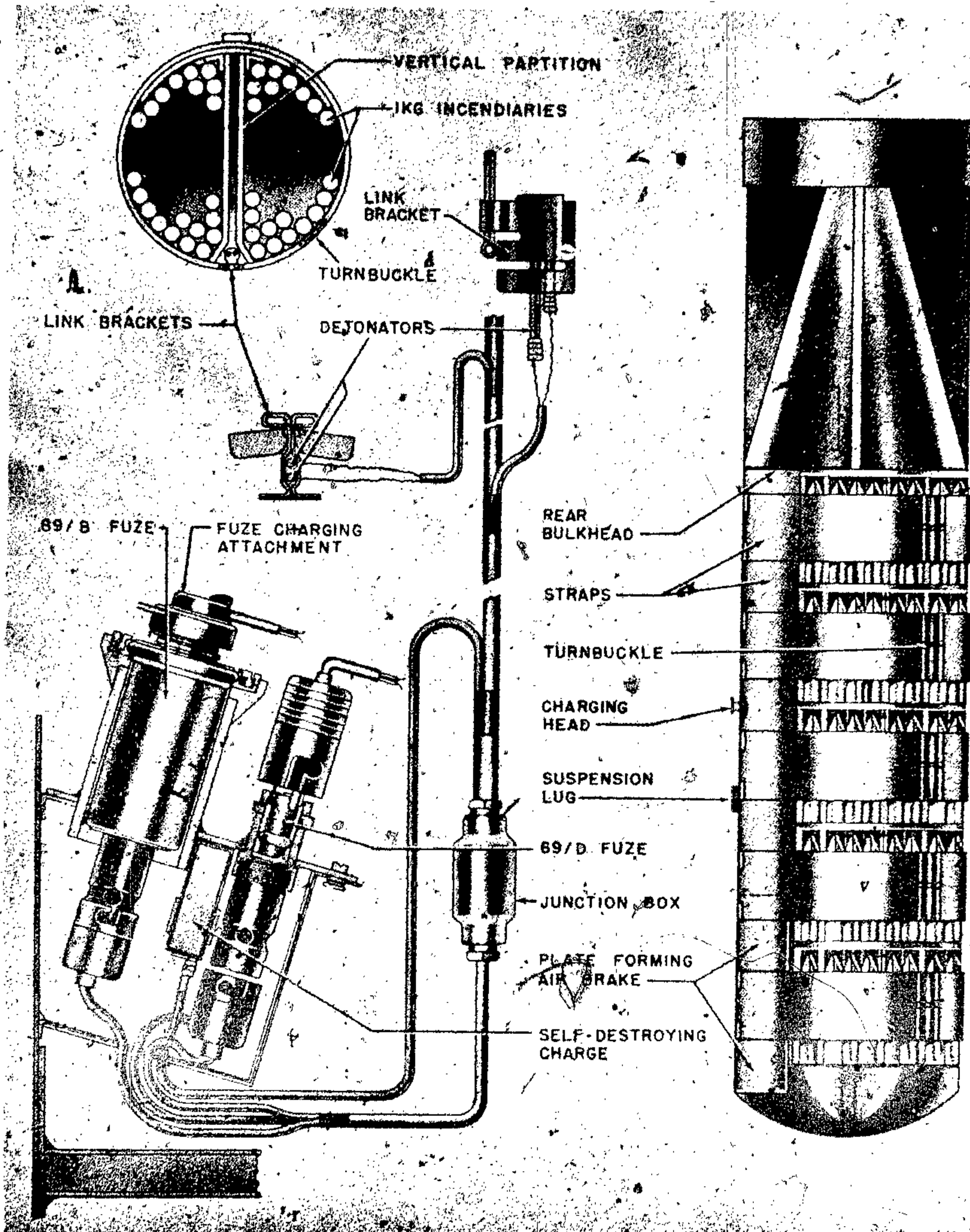
Figure 116—AB 1000-2 Container
