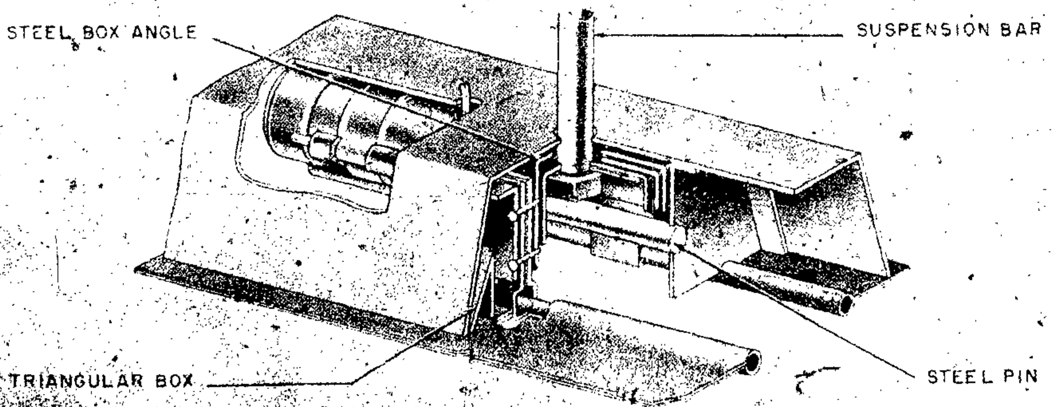
Figure 112—AB 500-3A Cluster Adapter
