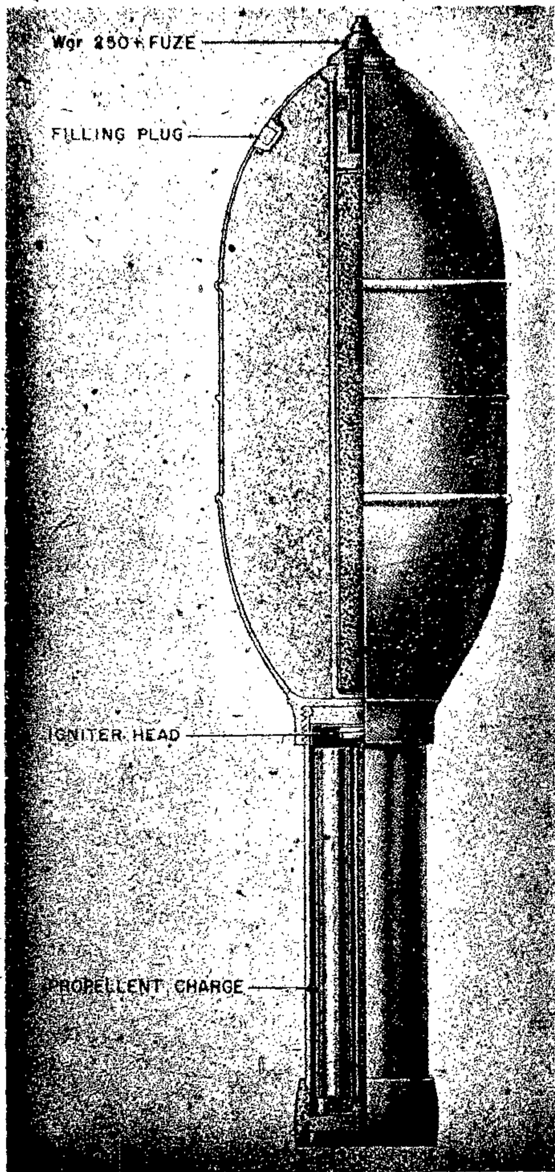
Figure 218—32-cm Incendiary Rocket
