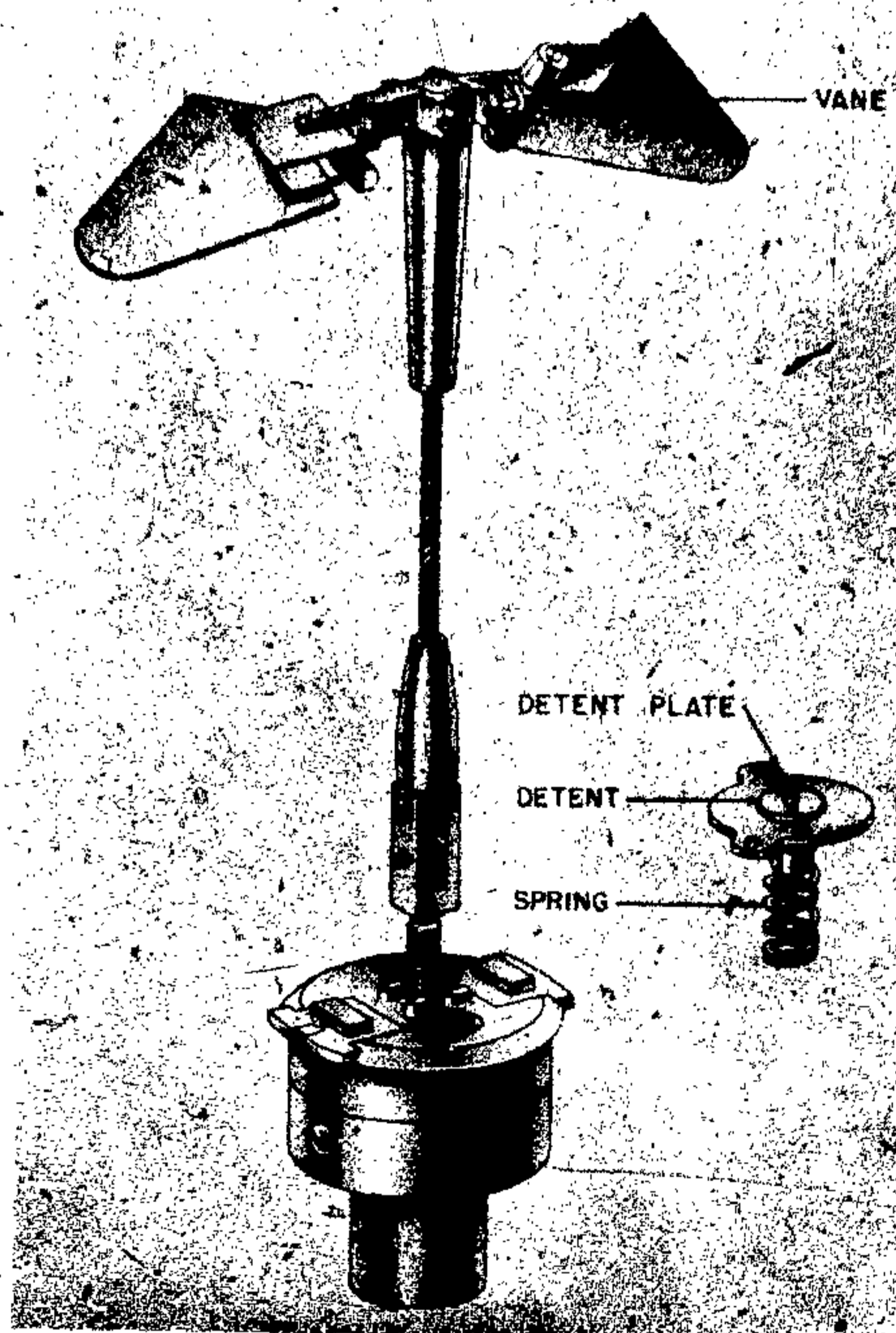
Figure 132—(41)A Mechanical Clockwork Fuze
