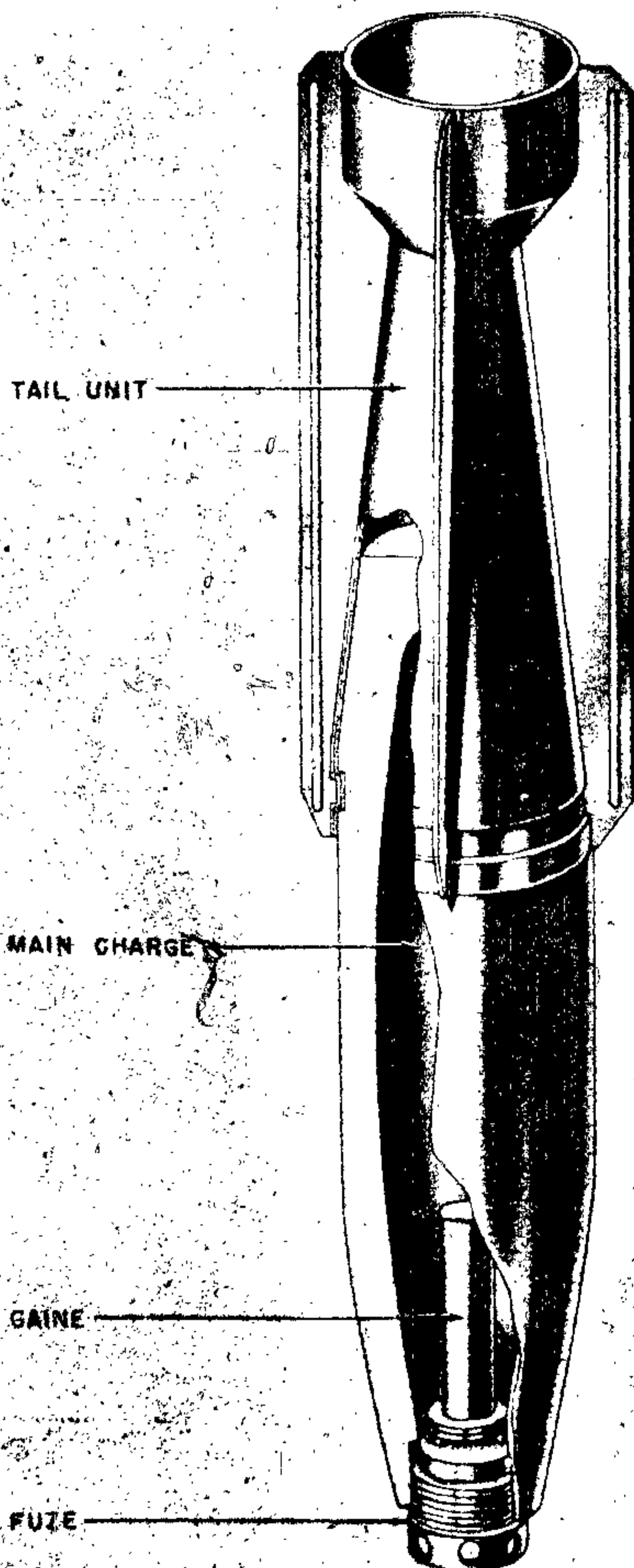
Figure 45—SD 15-Kg Converted German Shell Bomb
