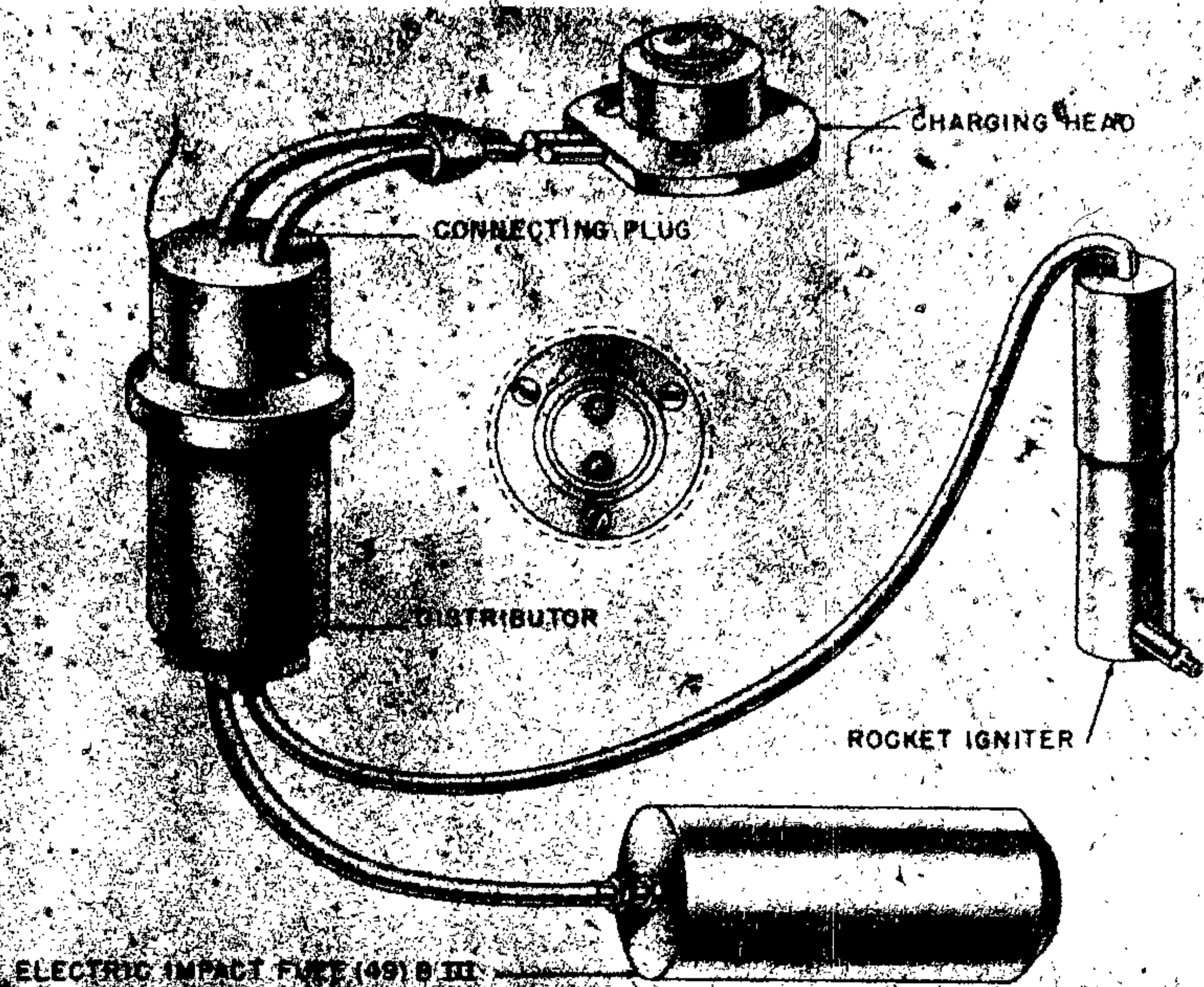
Figure 172—(49)C Rocket Bomb Fuze Assembly
