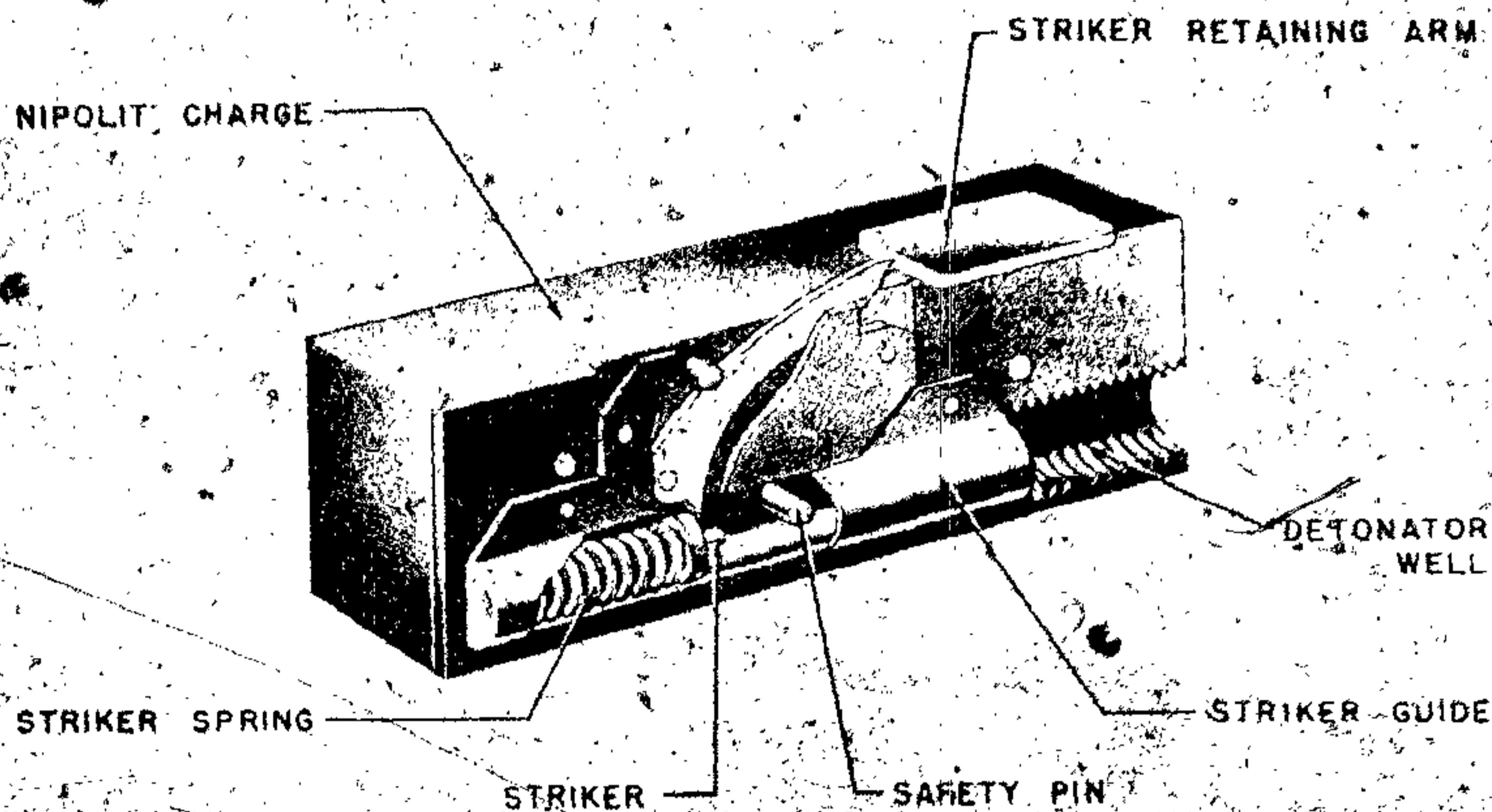
Figure 275—All-Explosive Pressure Release Device
