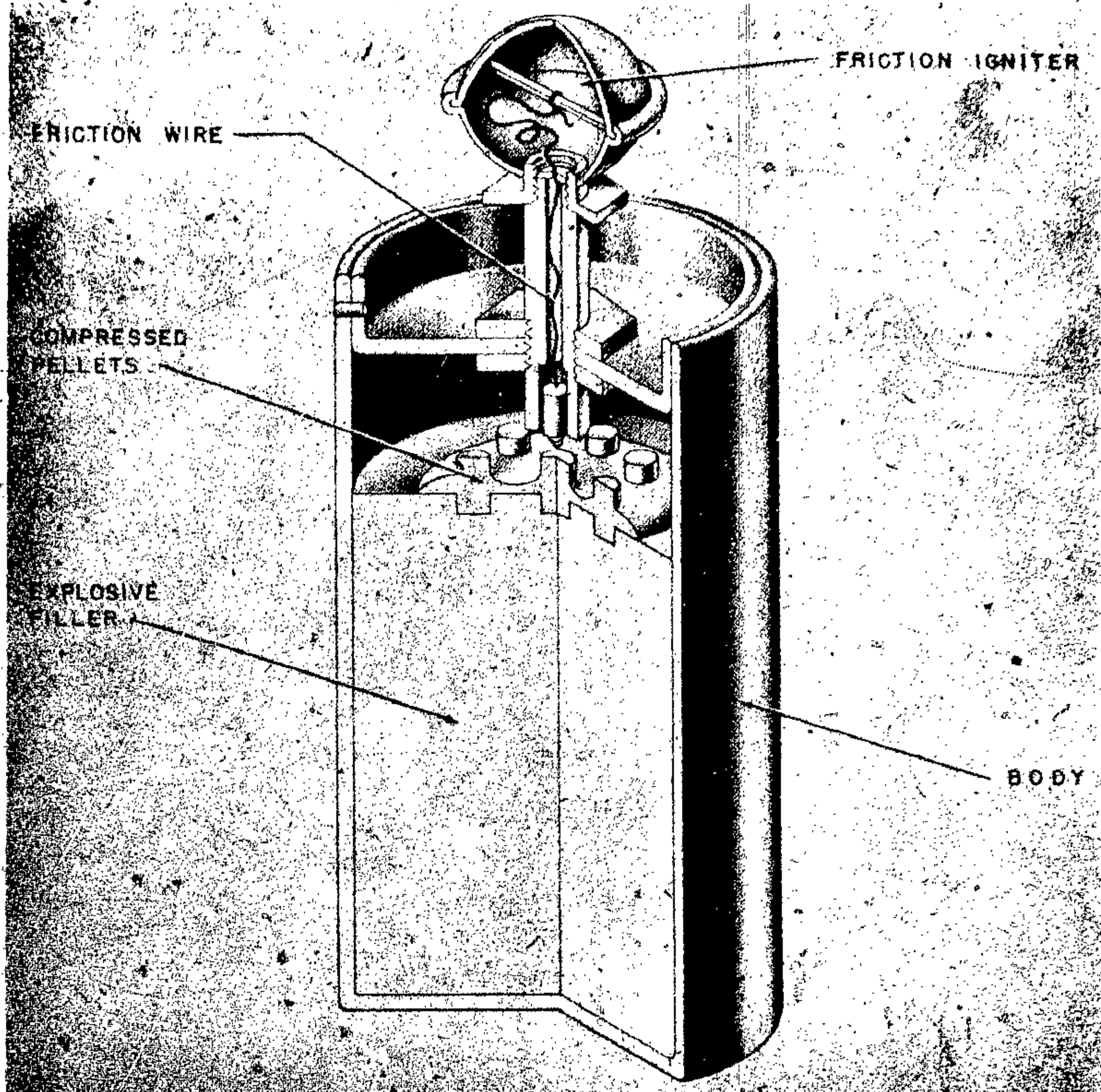
Figure 287—Shaving Stick Hand Grenade
