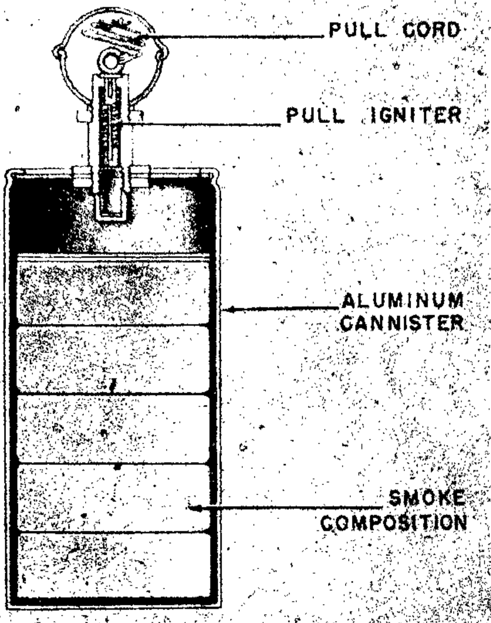
Figure 83—Smoke Signal Flare
