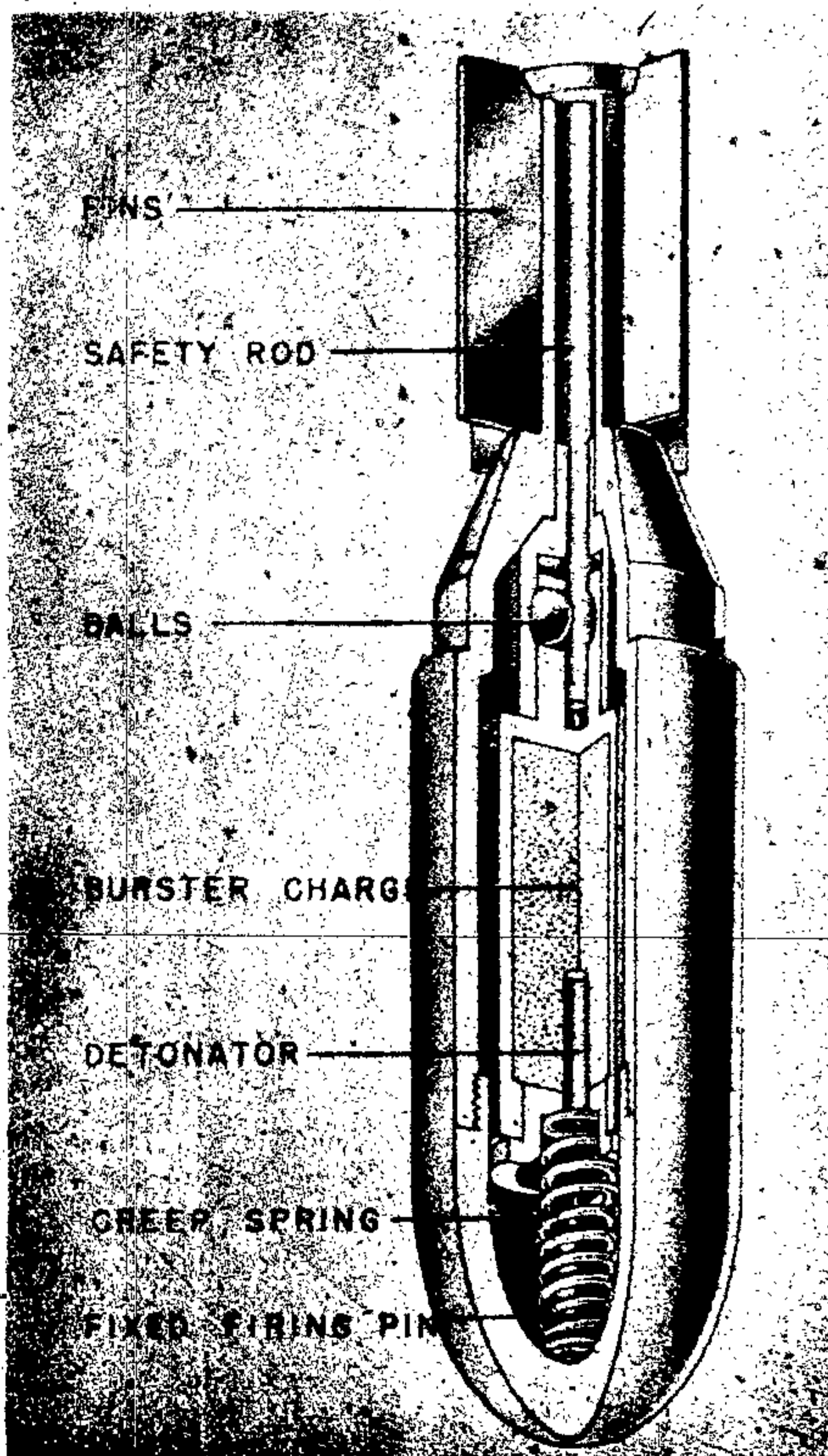
Figure 311—26-mm Pistol Grenade
