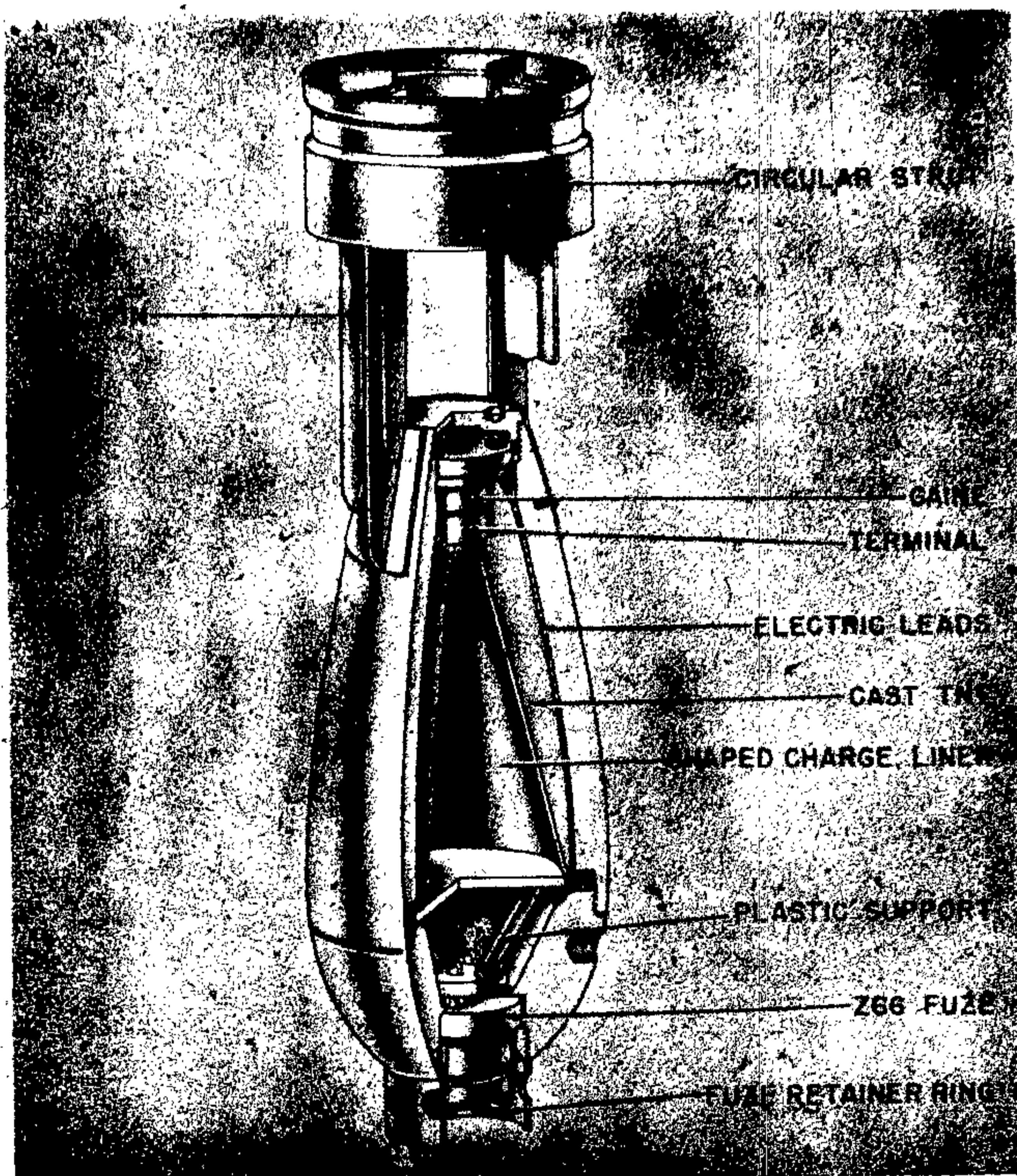
Figure 41—SD 4-Kg HL Hollow Charge Bomb
