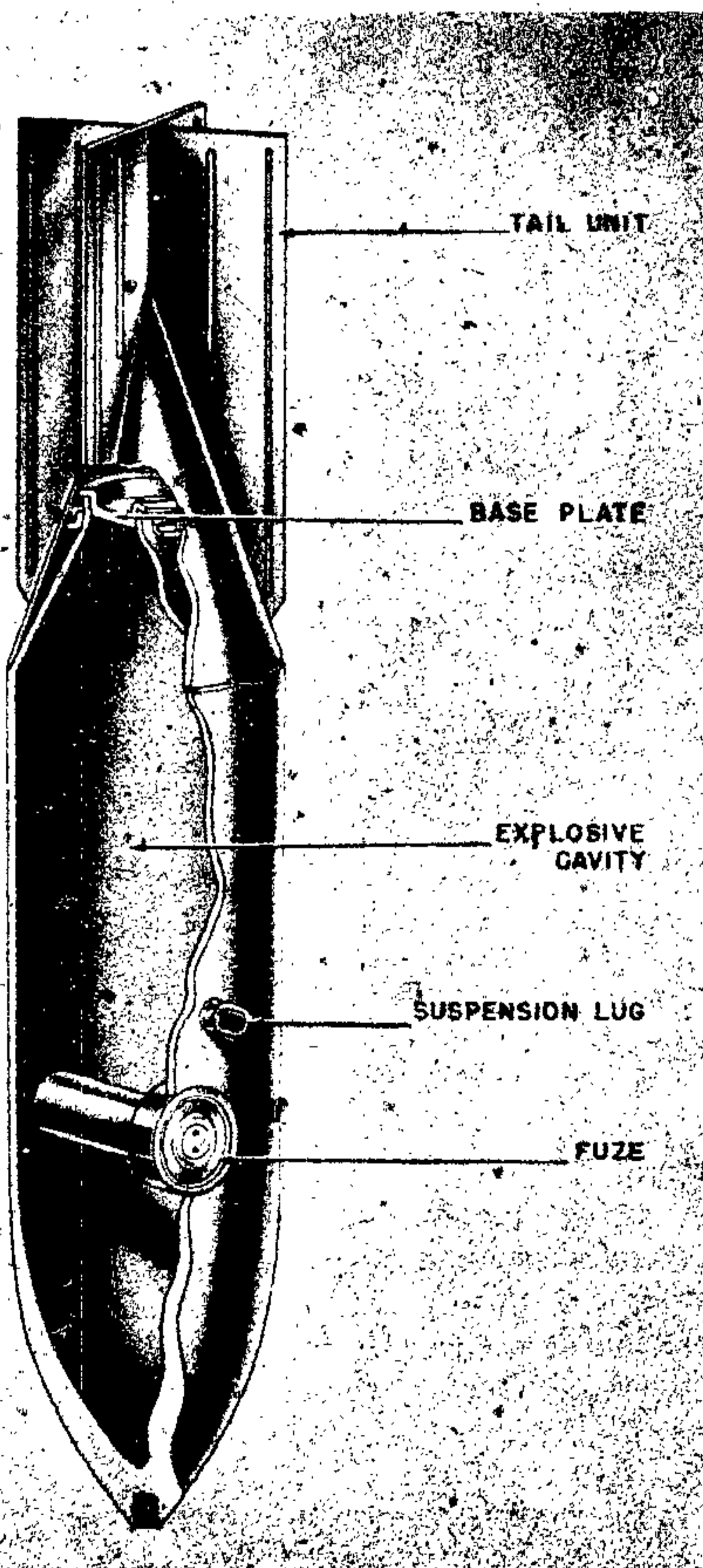
Figure 24—SD 70-Kg Bomb
