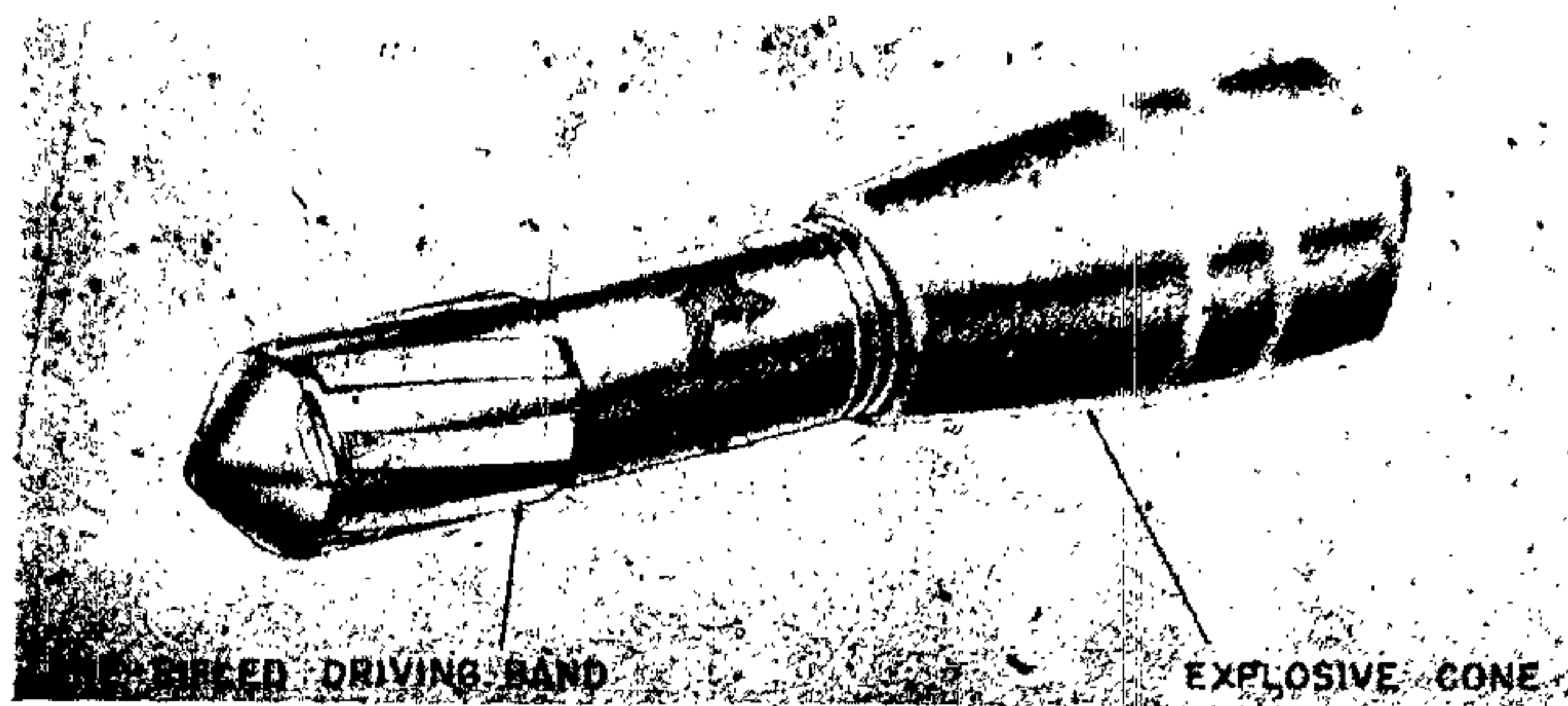
Figure 298—46-mm Hollow Charge Rifle Grenade
