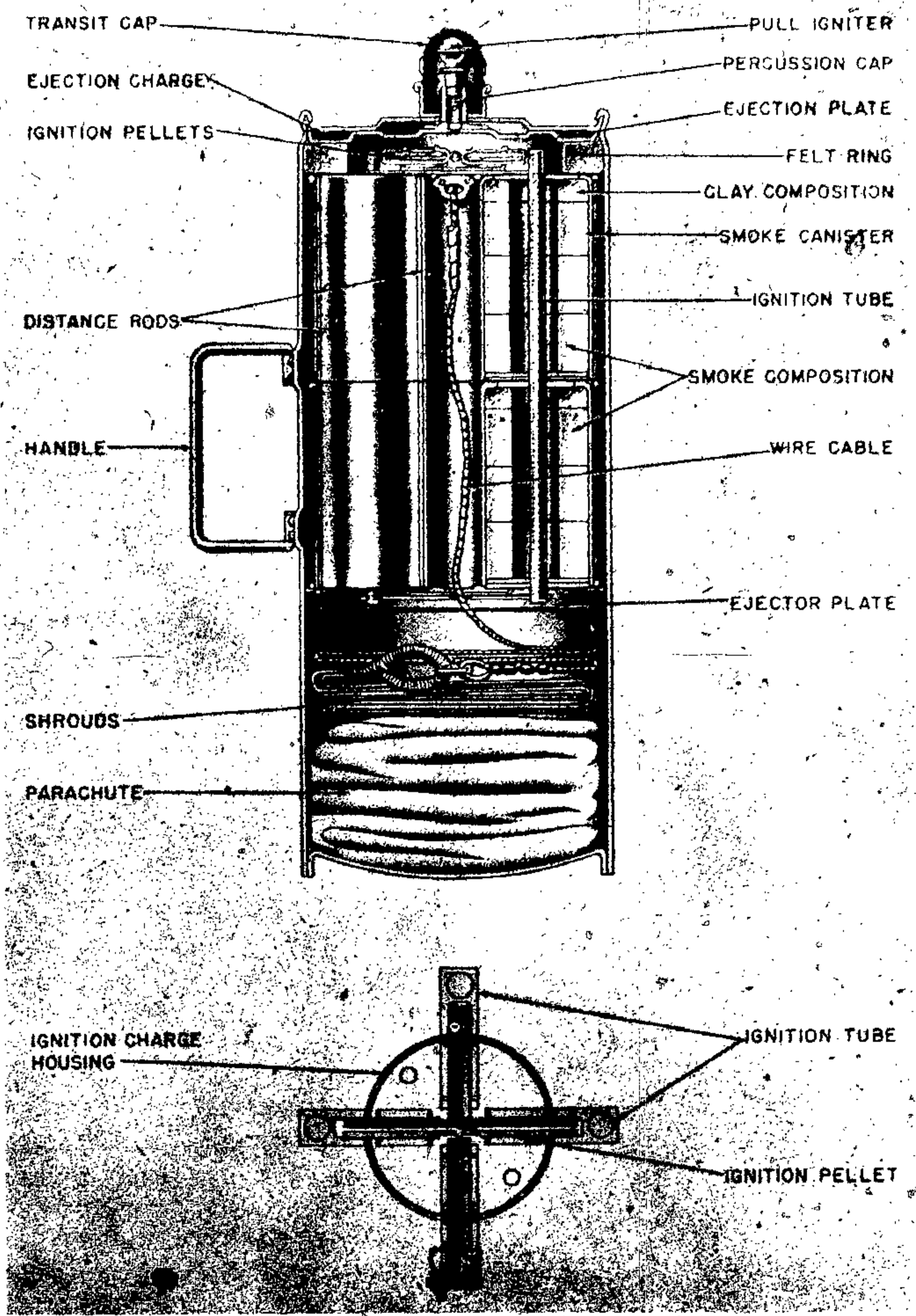
Figure 92—Parachute Recognition Smoke Generator
