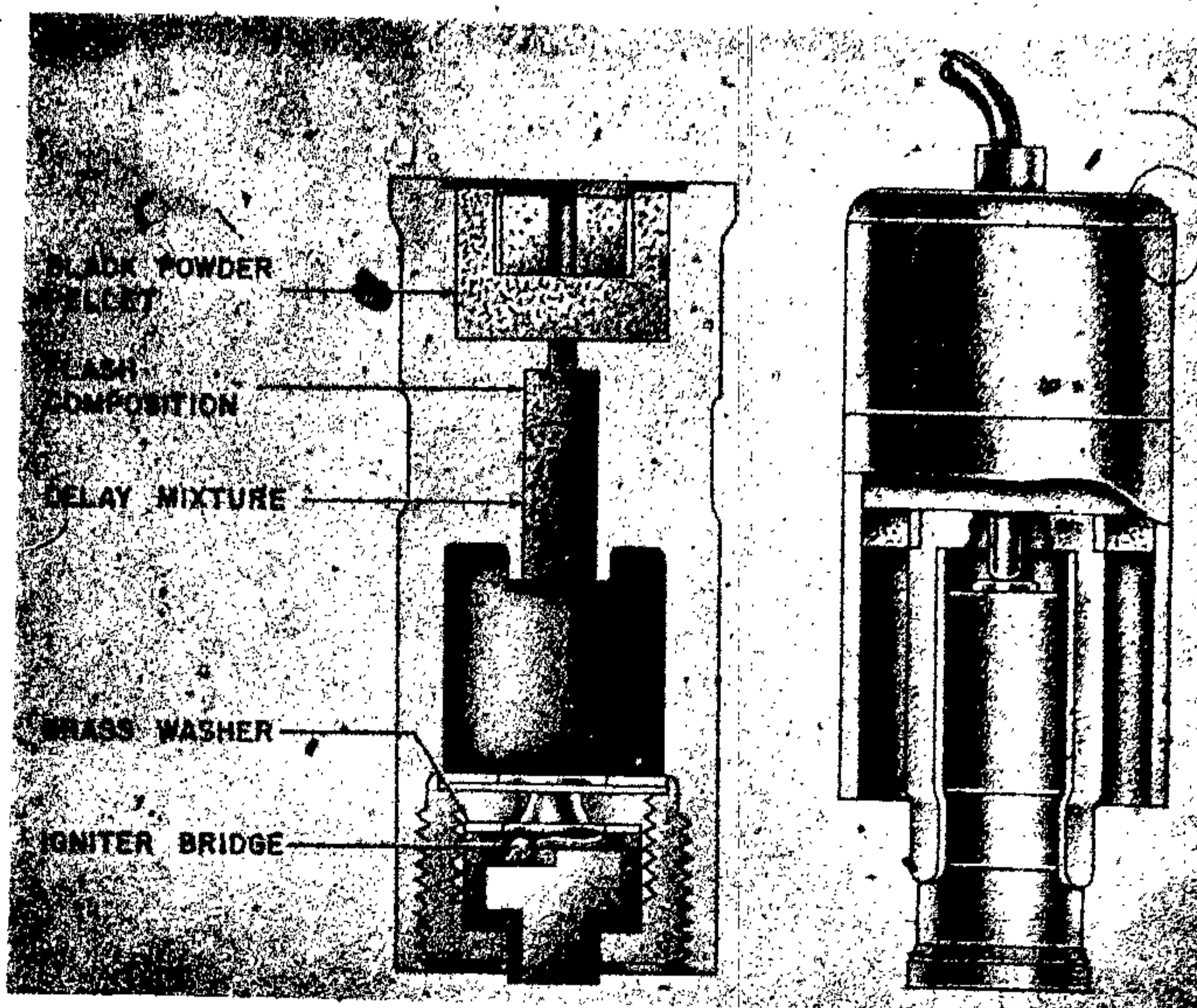
Figure 176—69CII Electrical Aerial Burst Fuze
