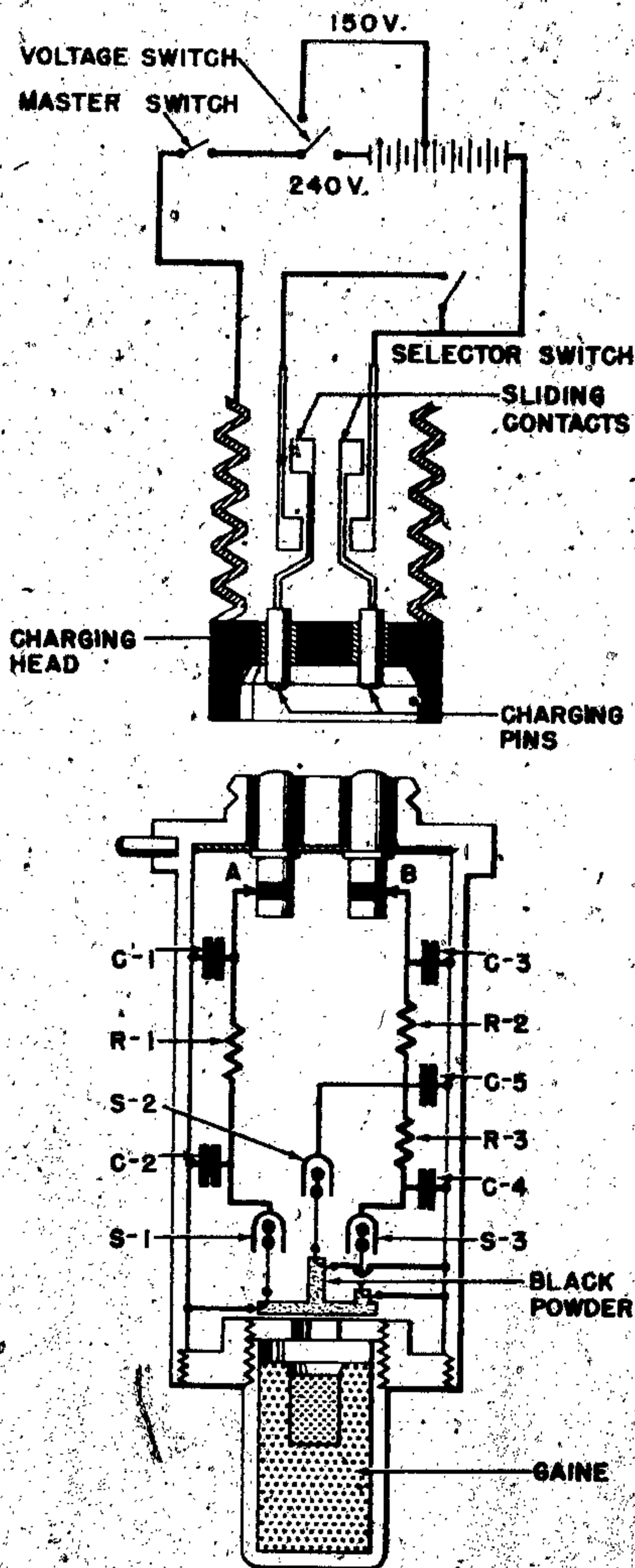
Figure 123—Wiring Diagram of Three Circuit Electrical Fuze
