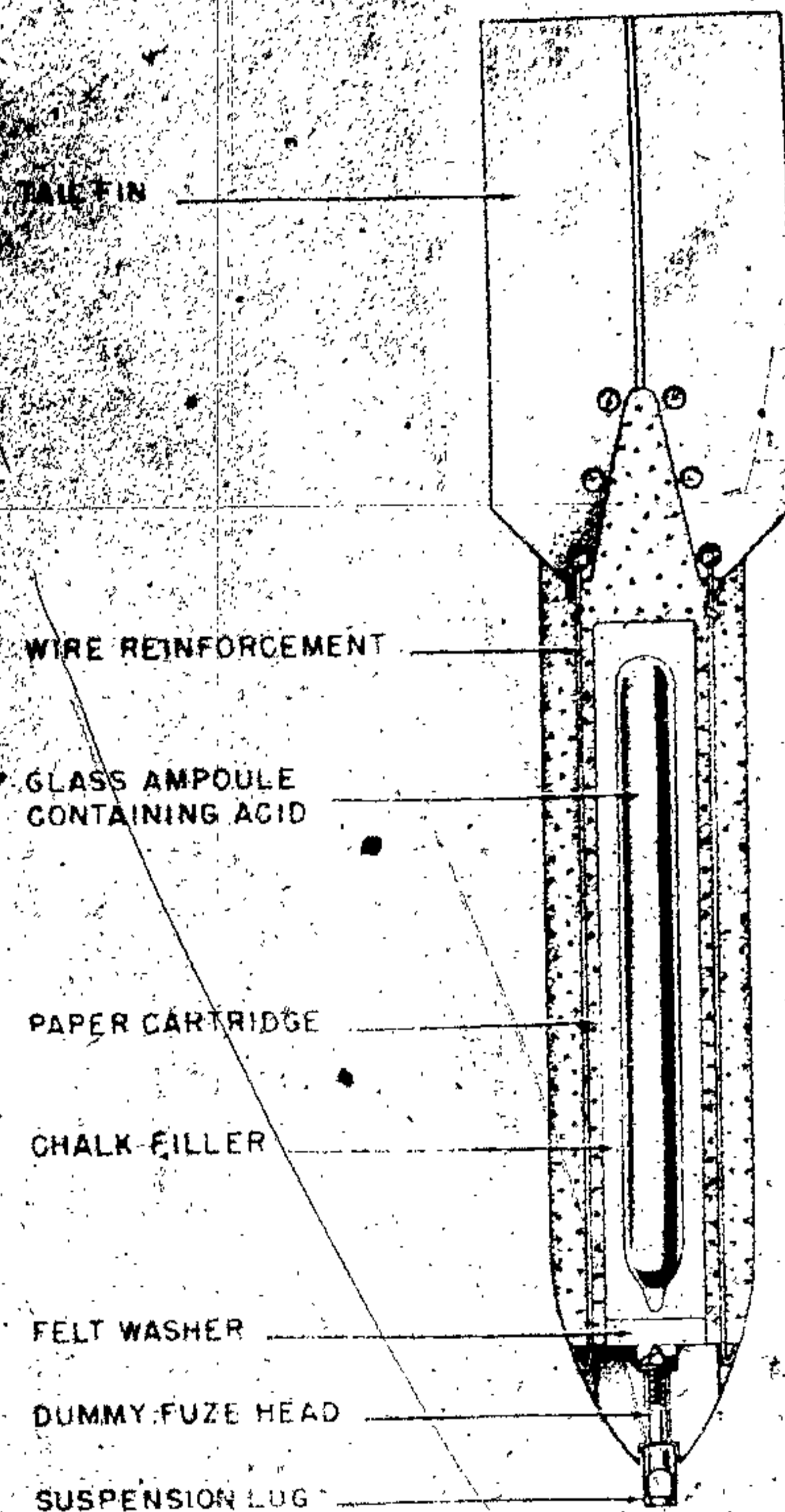
Figure 66—ZC 10-Kg Concrete Practice Bomb
