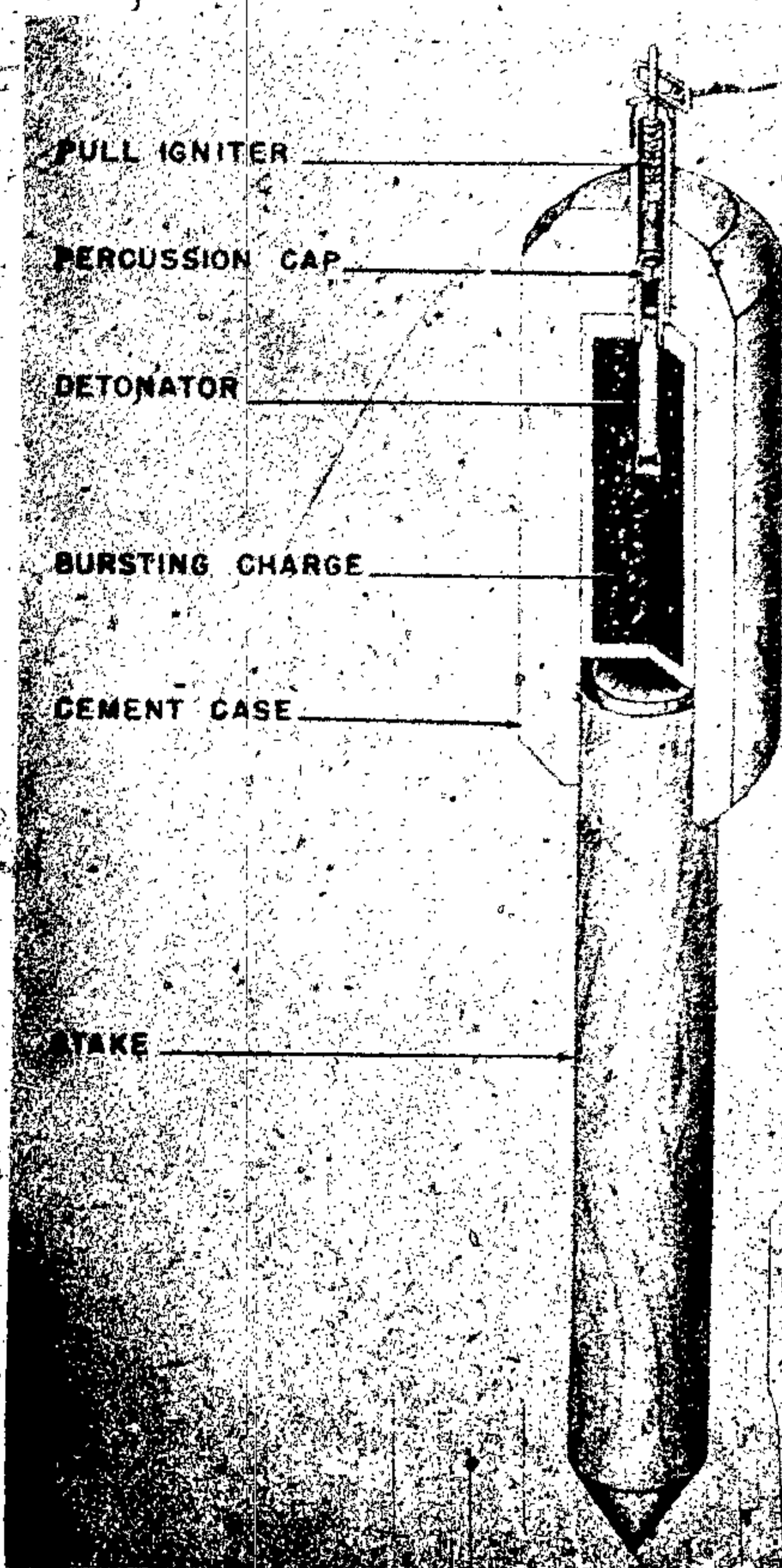
Figure 241—Stockmine—Antipersonnel
