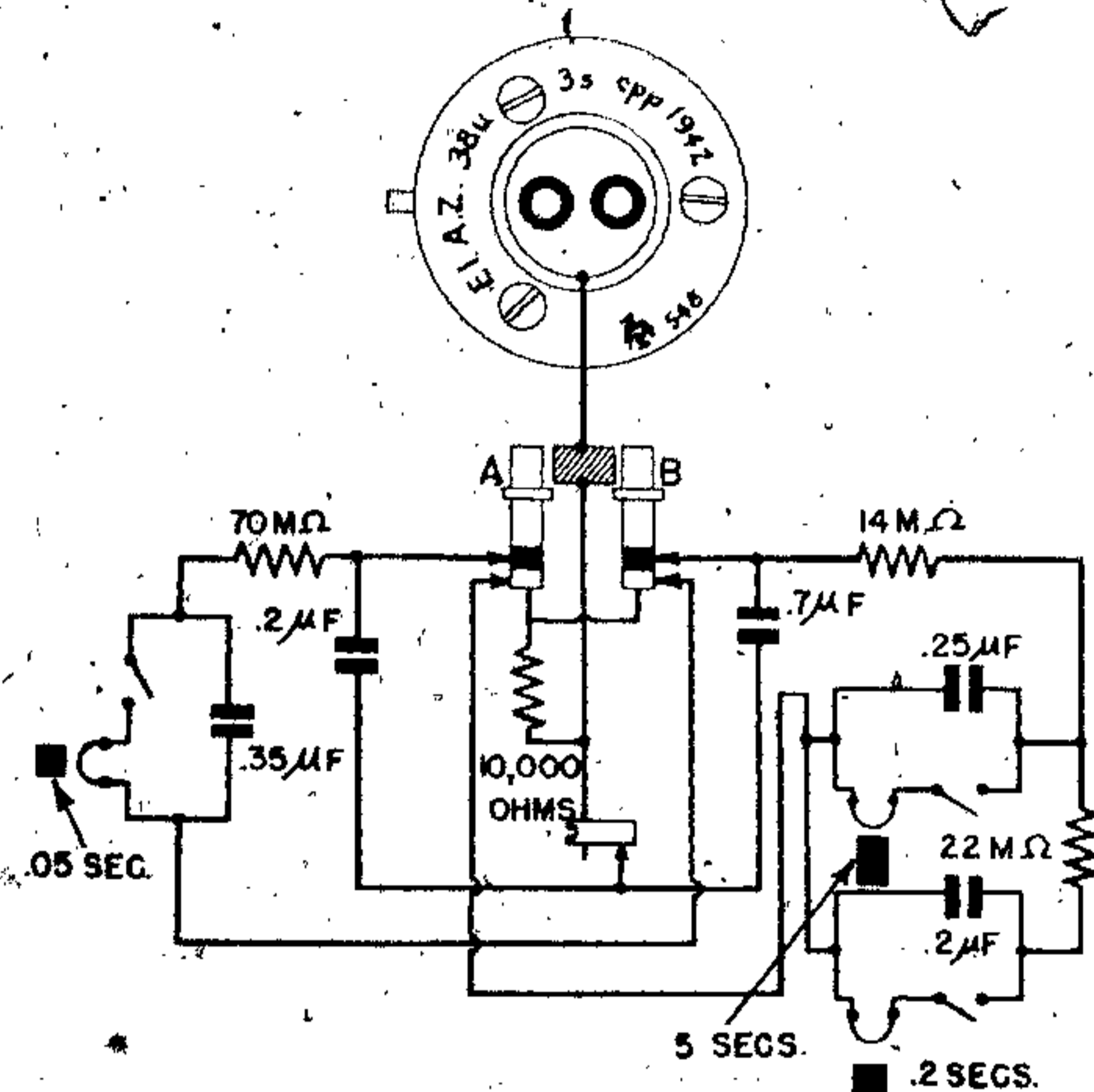
Figure 167—(38 u) Electrical Impact Fuze
