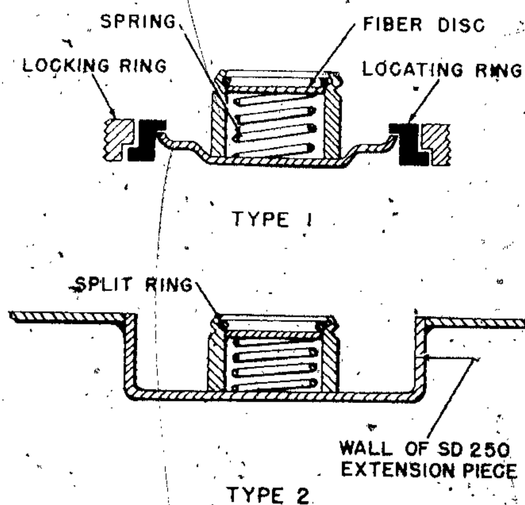
Figure 127—Dummy Fuze Heads
