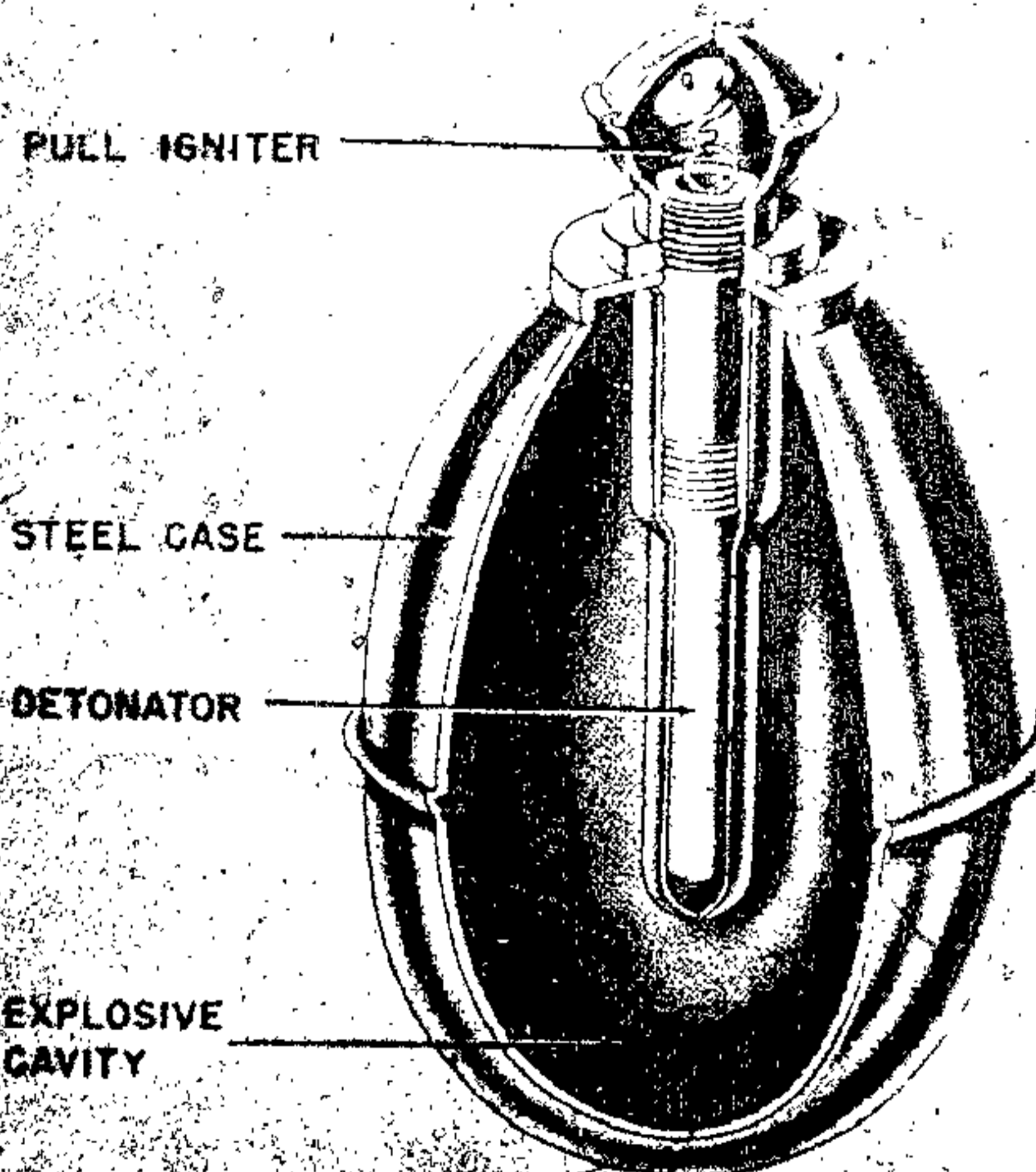
Figure 286—Egg Type 39 Hand Grenade
