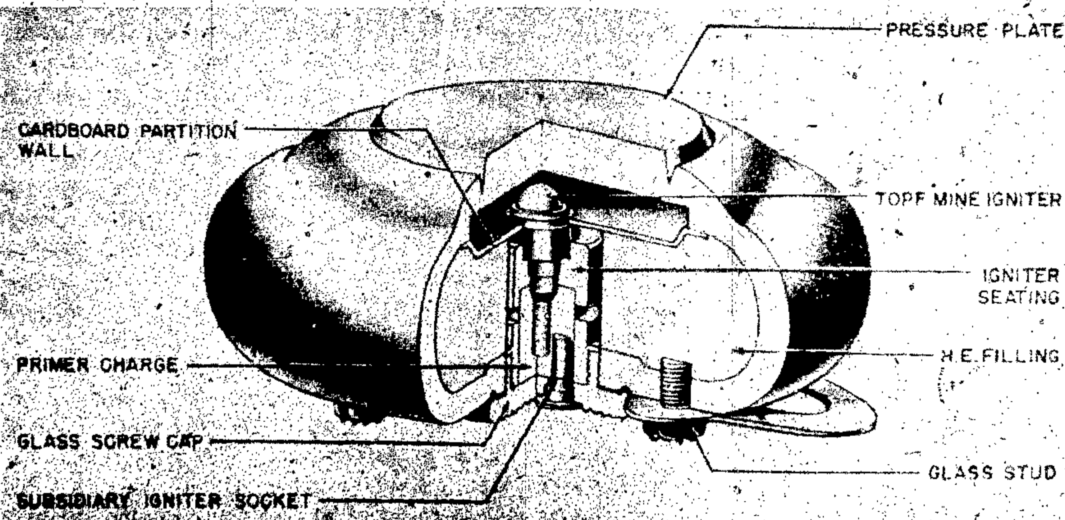
Figure 235—Topf Mine A—Antitank
