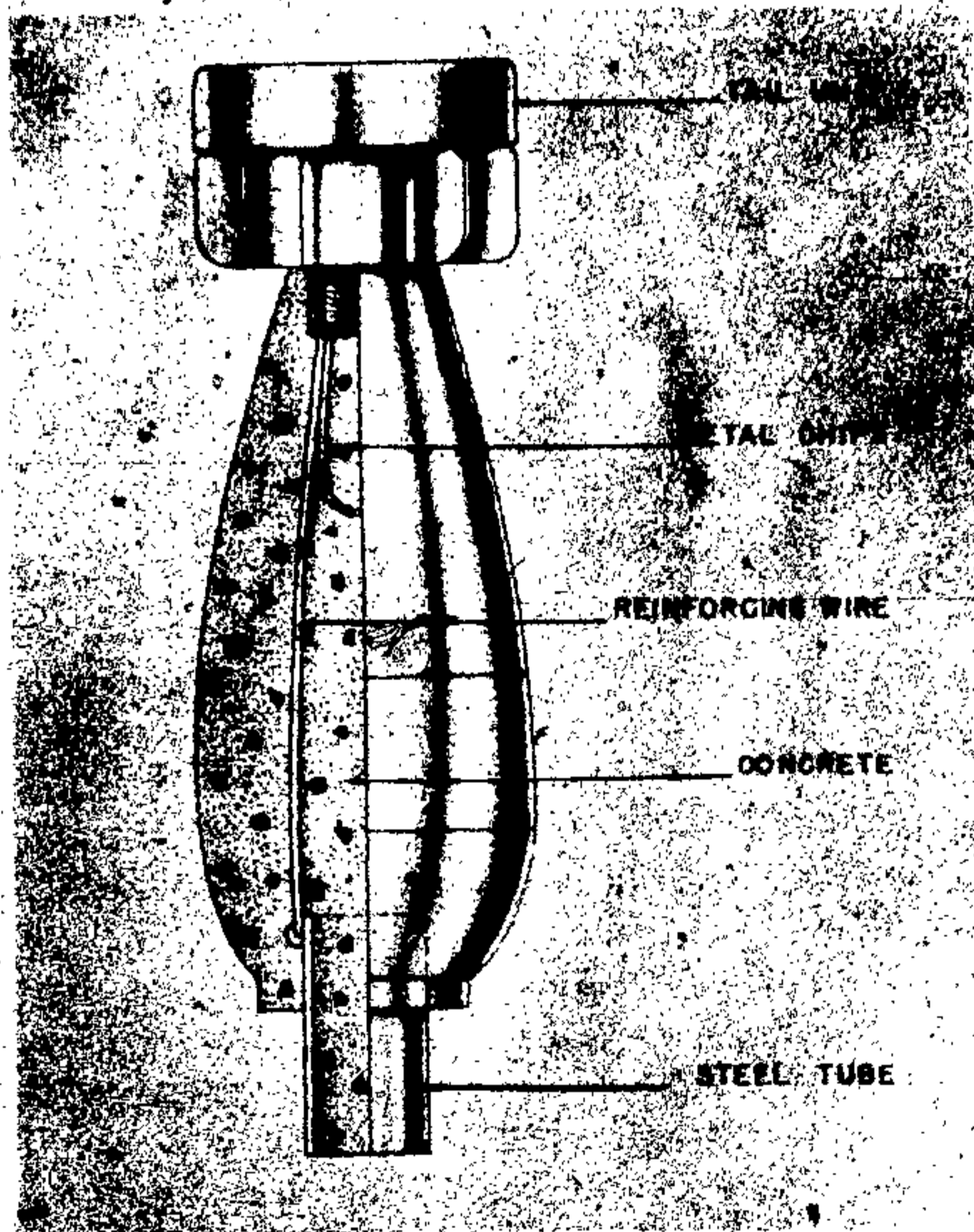
Figure 64—SD 1 Type Practice Bomb
