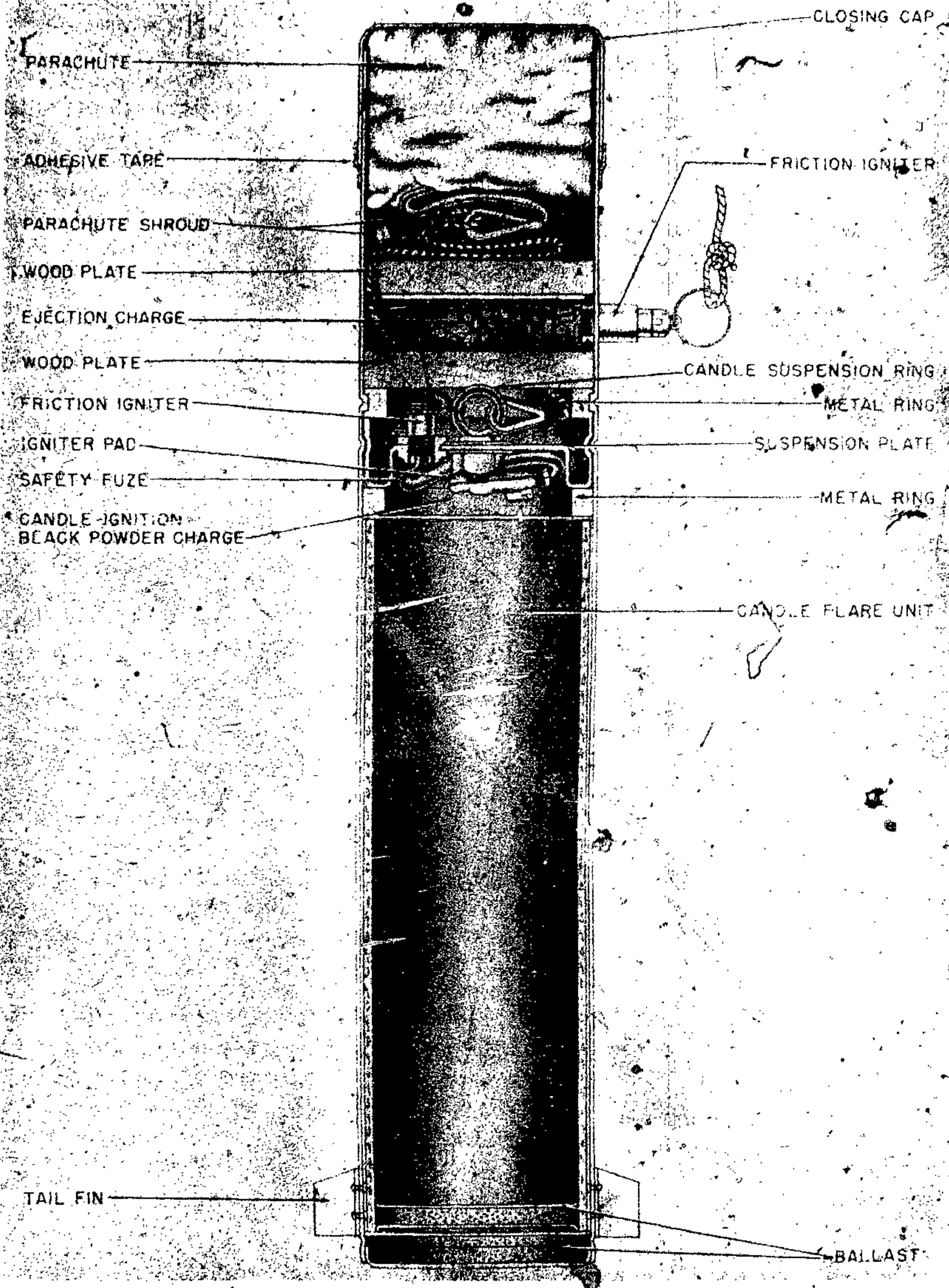
Figure 79—Parachute Flare (Red)—Single Unit
