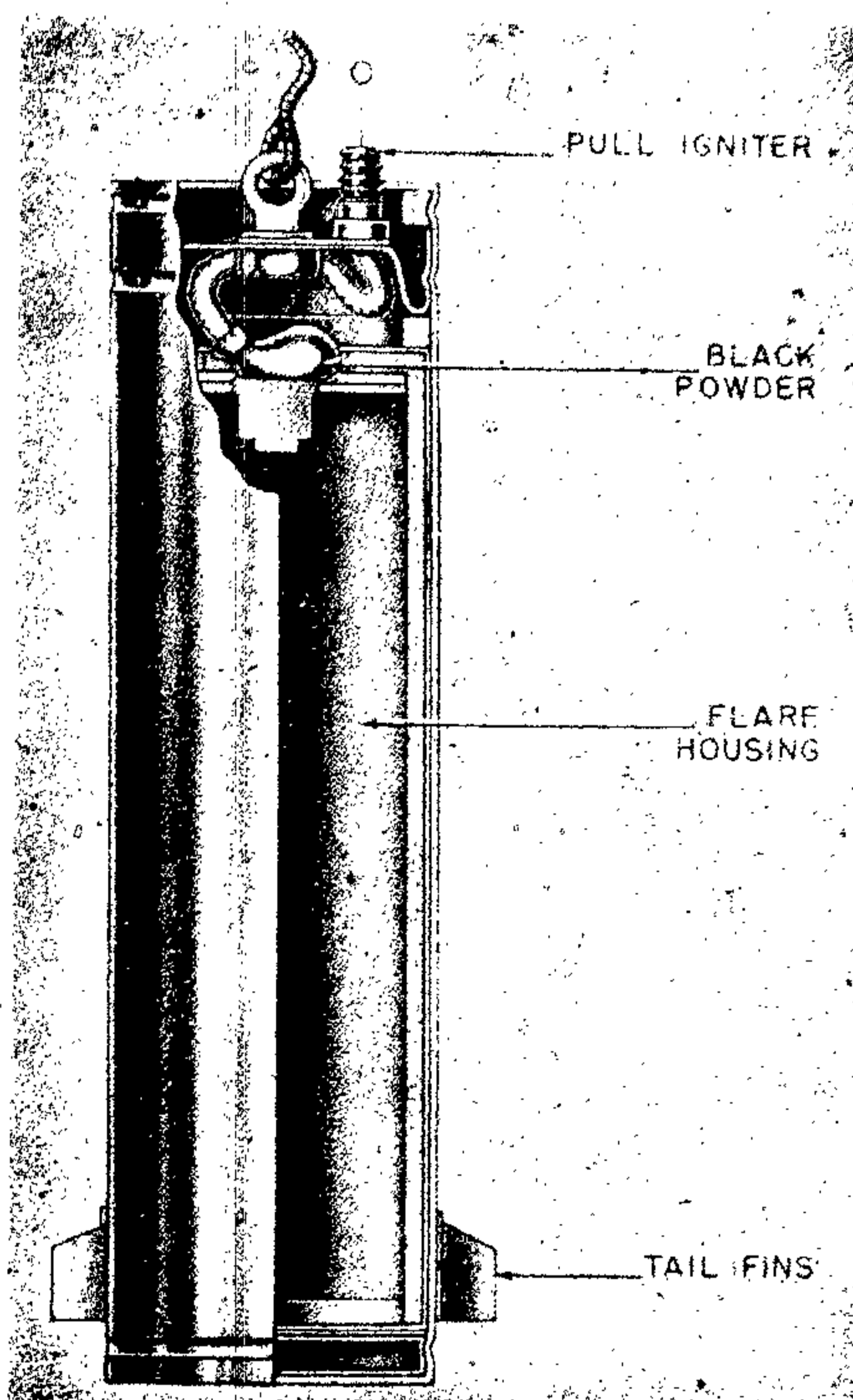
Figure 88—Target Indicator (Red)
