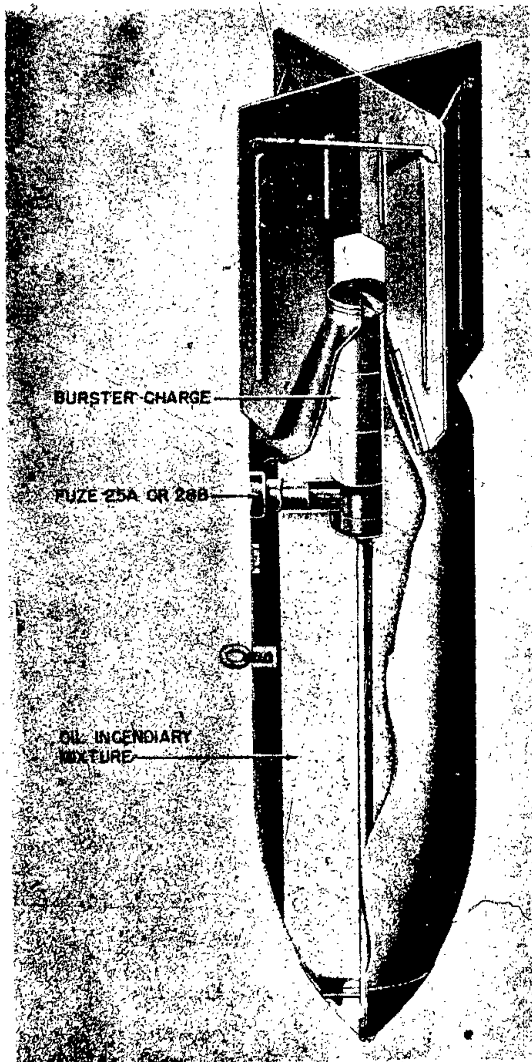
Figure 55—Flam C 250 A Bomb
