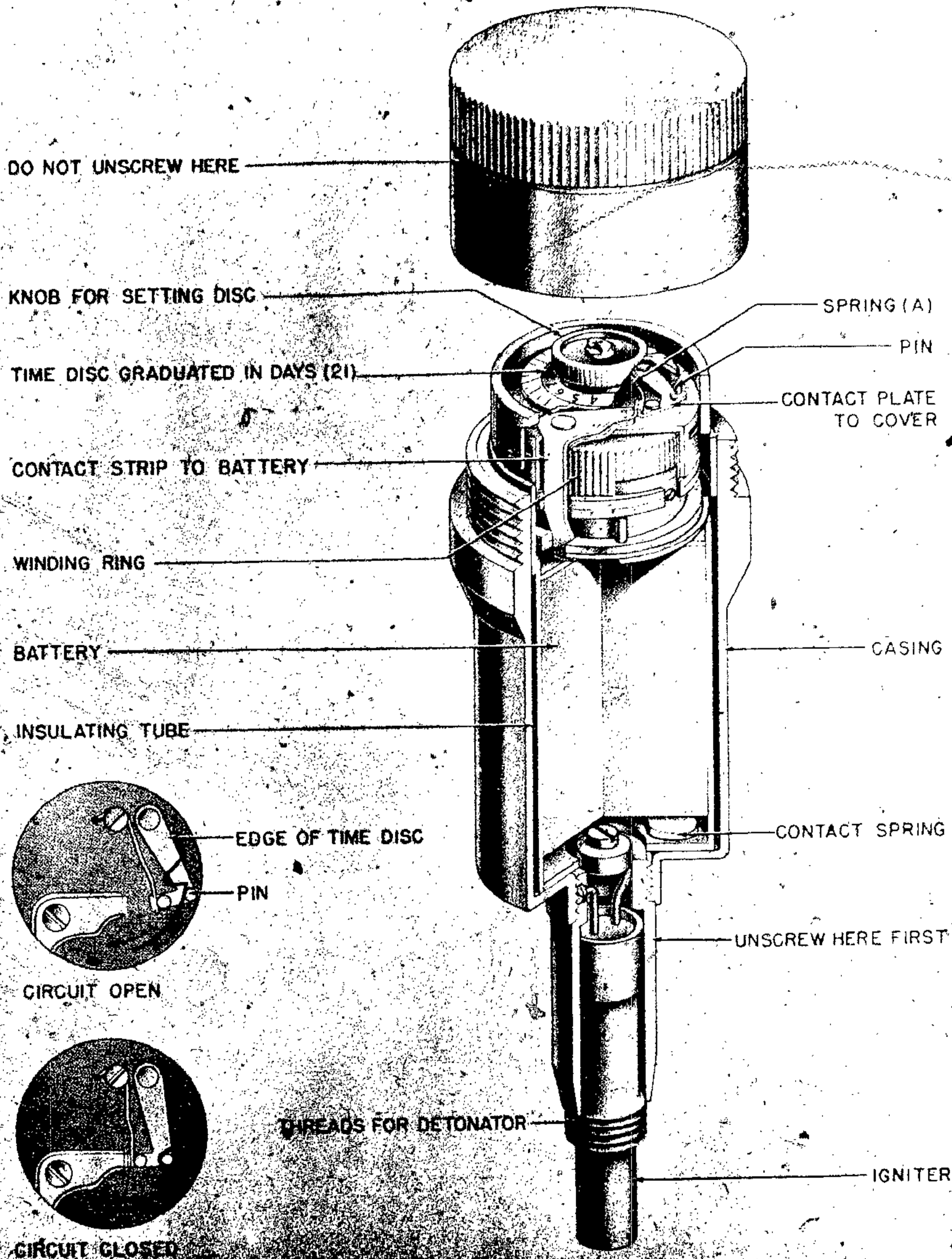
Figure 277—Long-Delay (21-day) Clockwork
