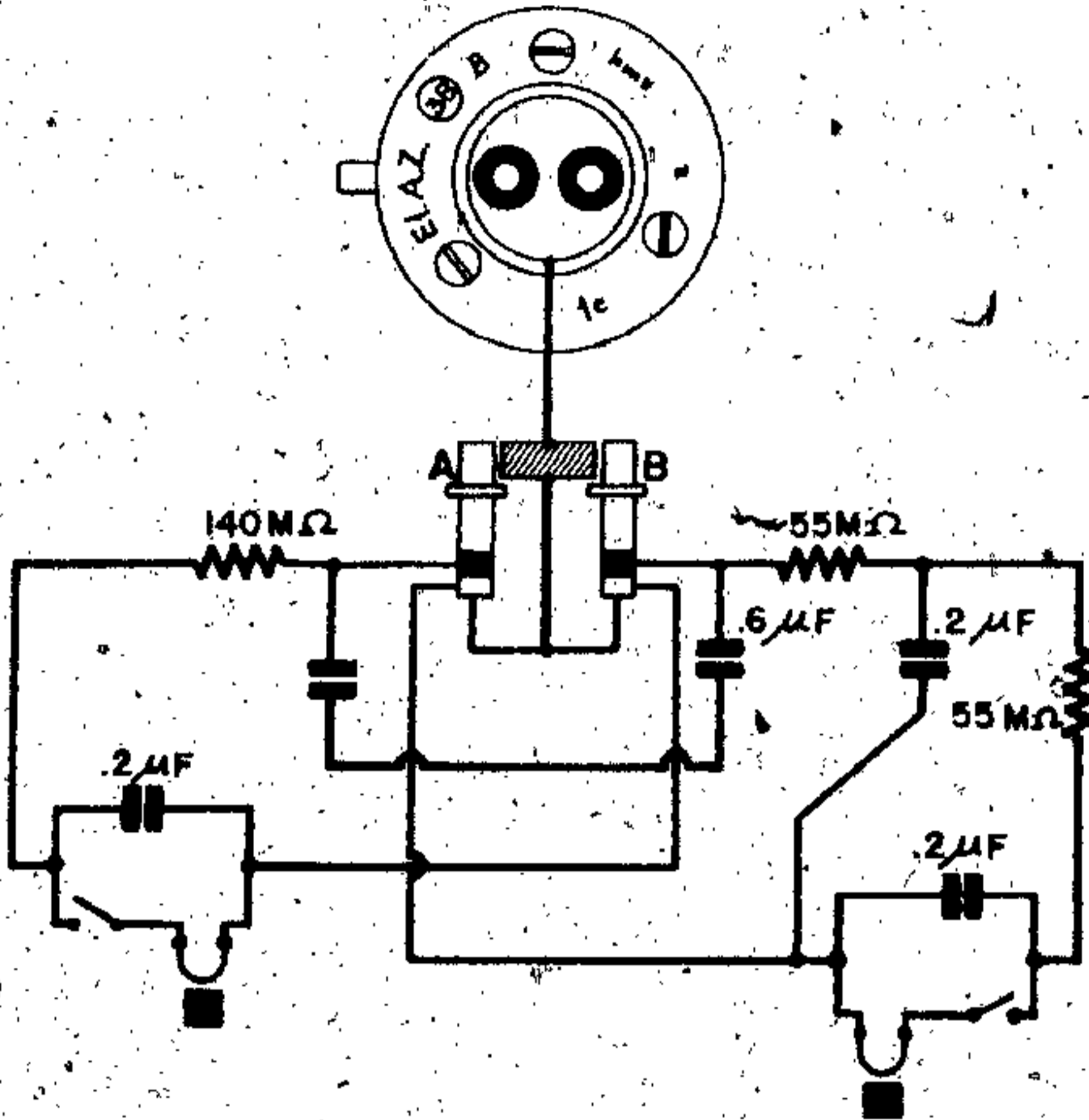
Figure 168—(38)B Electrical Impact Fuze
