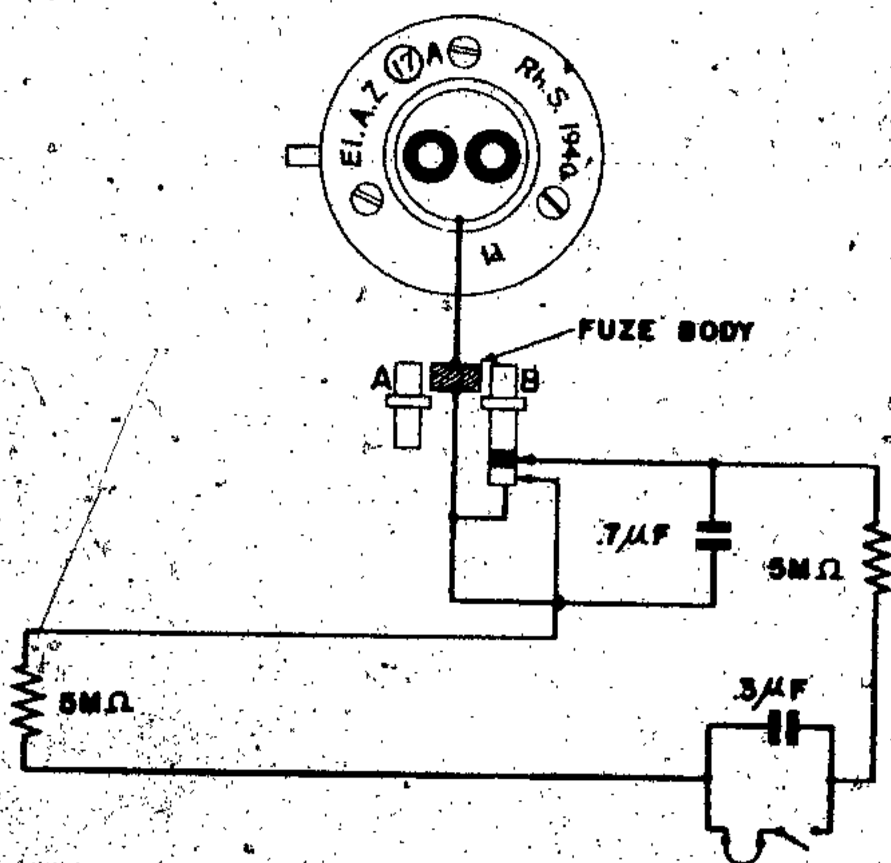
Figure 153B—(17)A Electrical Clockwork Time Fuze Wiring Diagram
