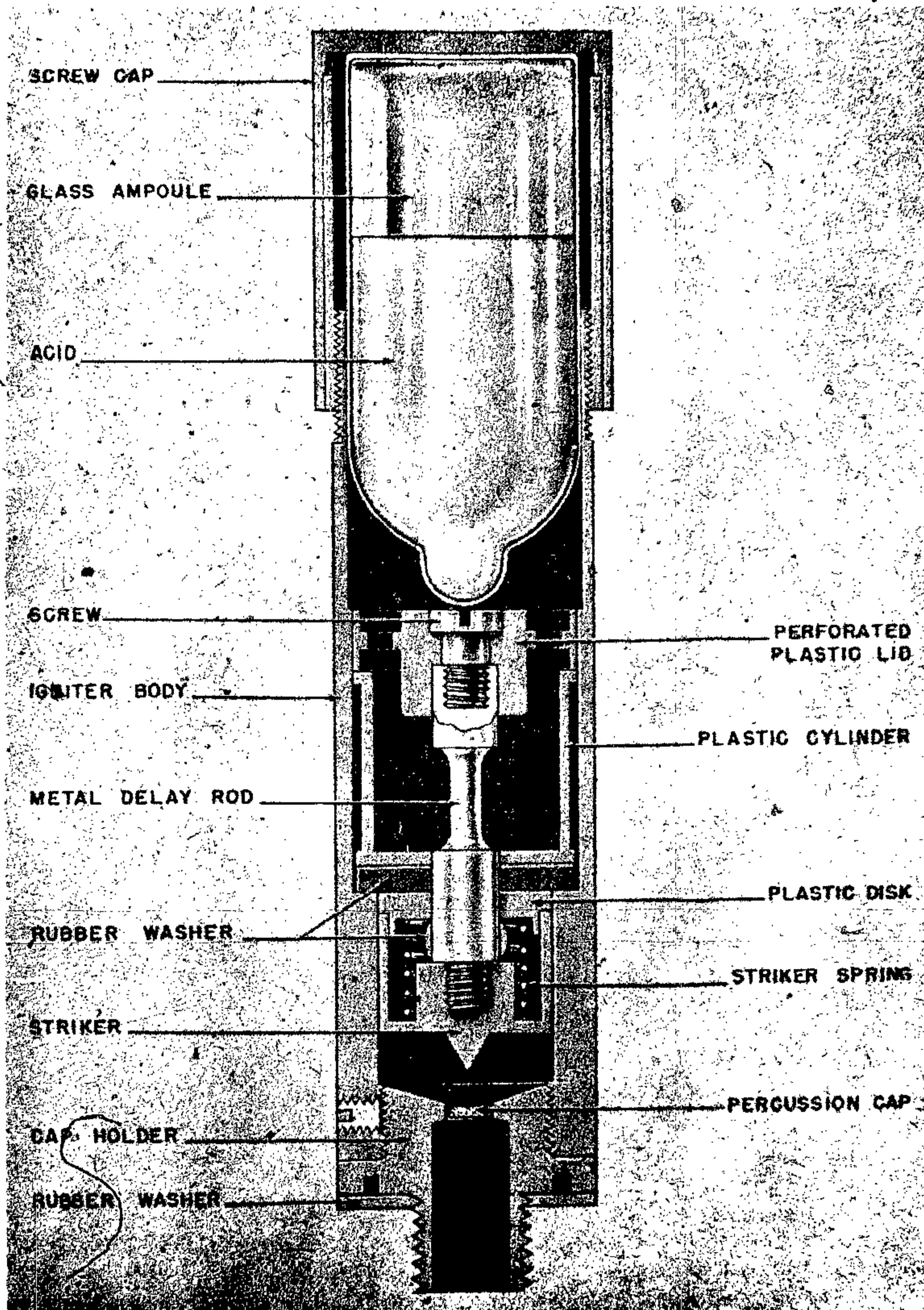
Figure 279—C. M. Z. 41W Chemical Delay Igniter
