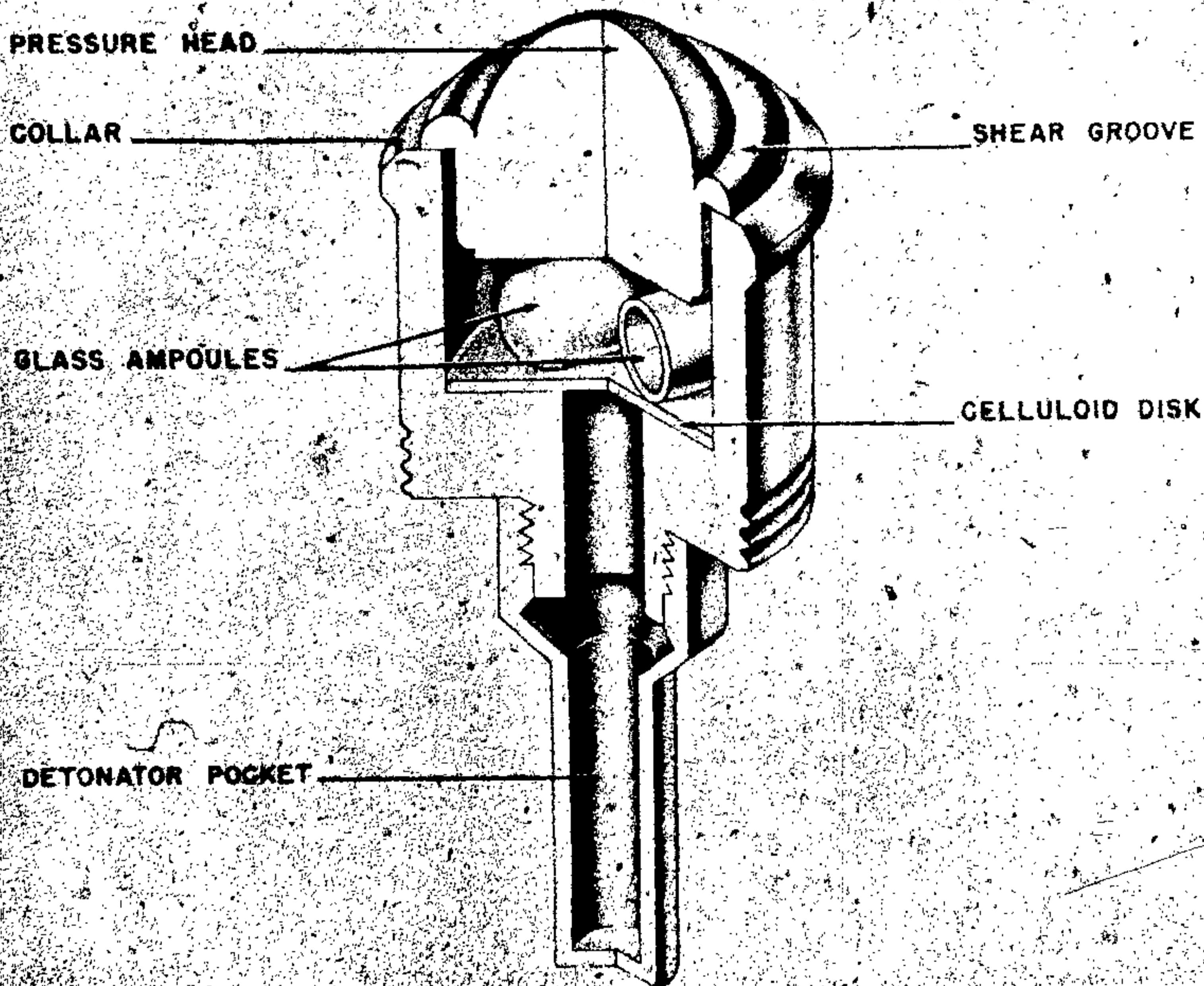
Figure 273—Topf Pressure Igniter
