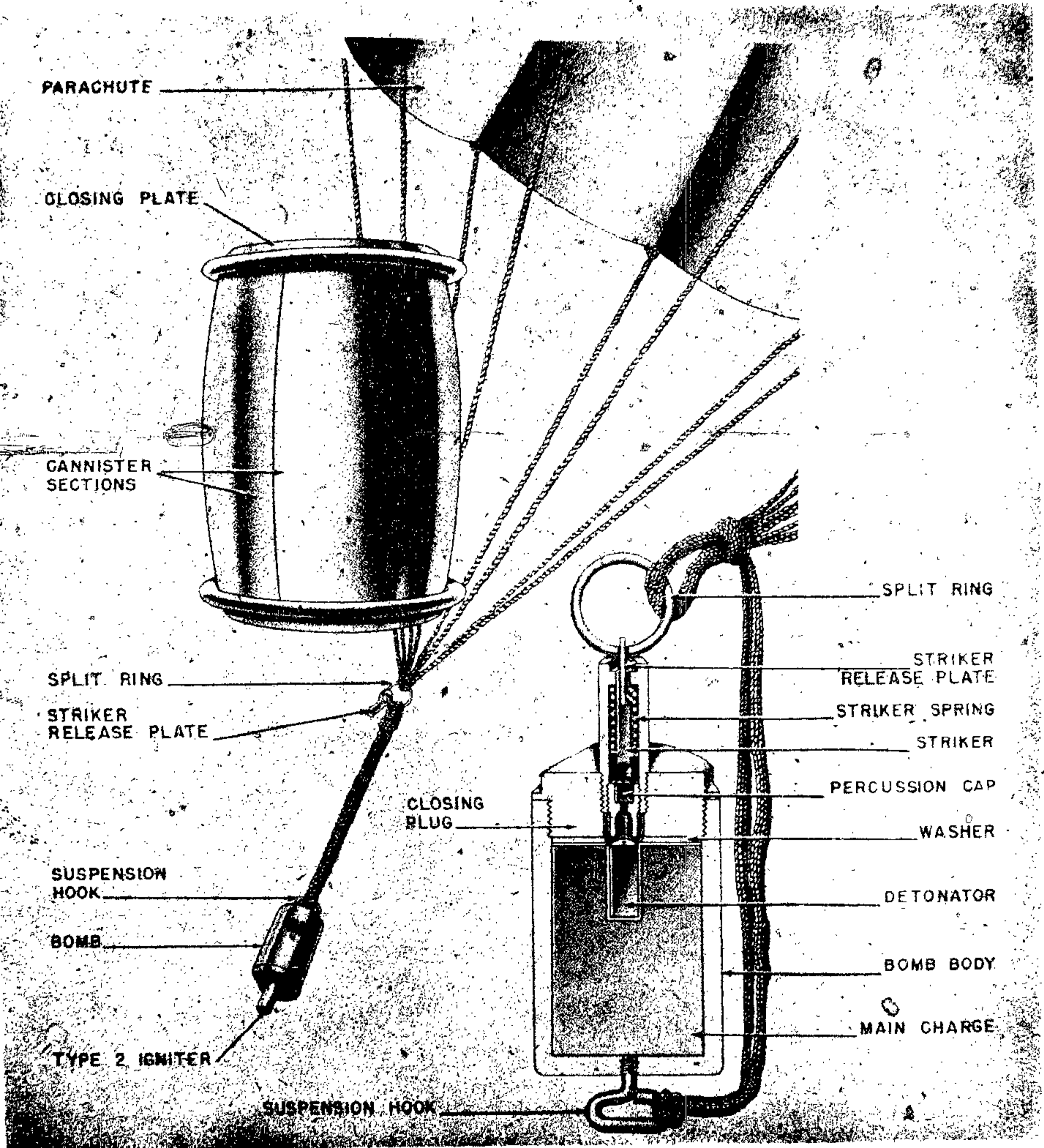
Figure 37—1/2 Kg Antipersonnel Parachute Bomb
