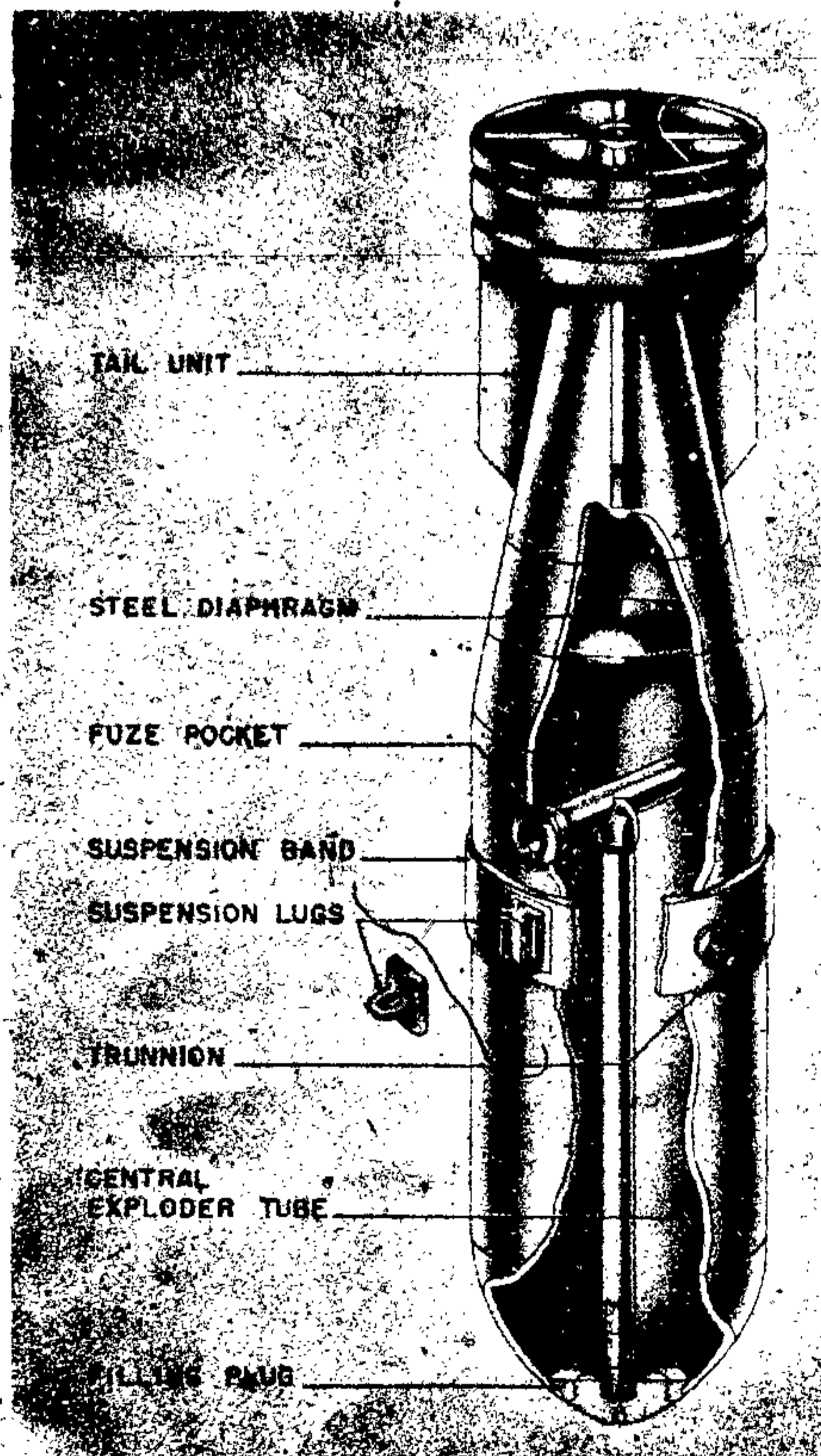
Figure 20—SB 1000-Kg Bomb
