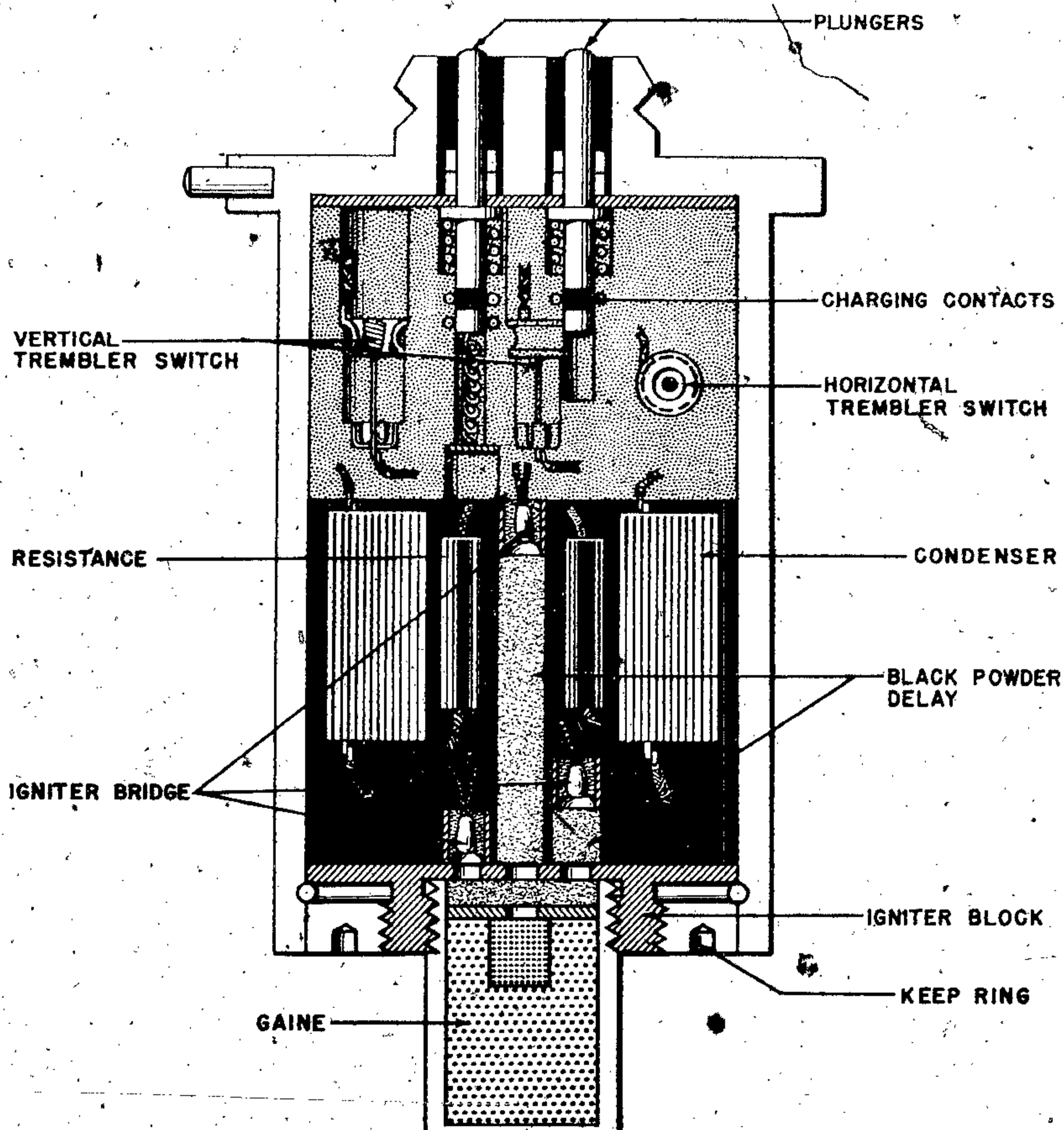
Figure 121—Internal Construction of Electrical Bomb Fuze
