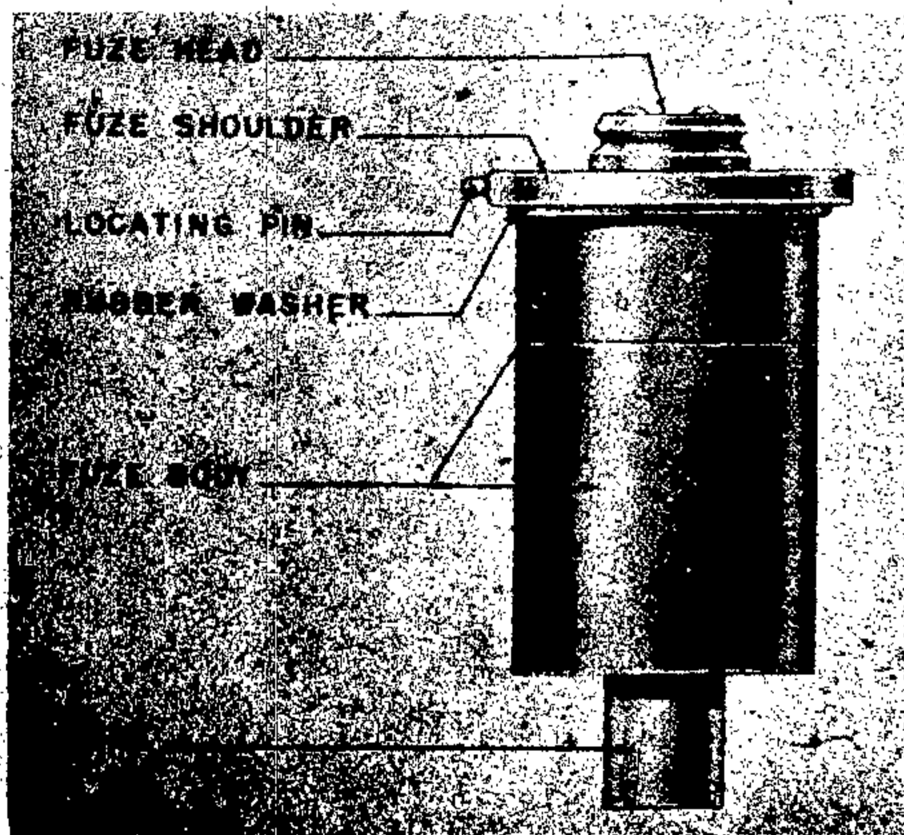
Figure 120—Typical Electrical Bomb Fuze
