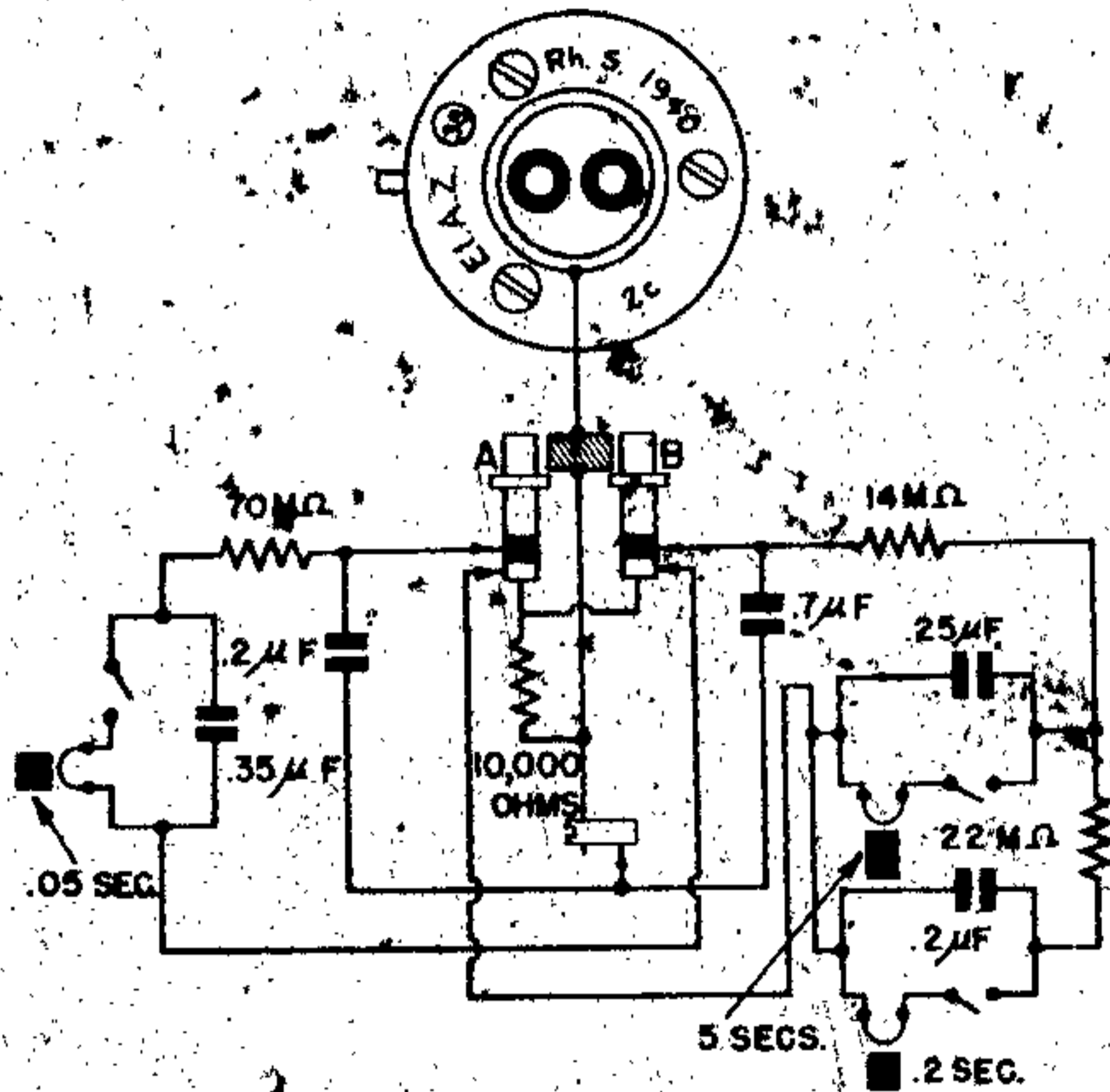
Figure 164—(38) Electrical Impact Fuze
