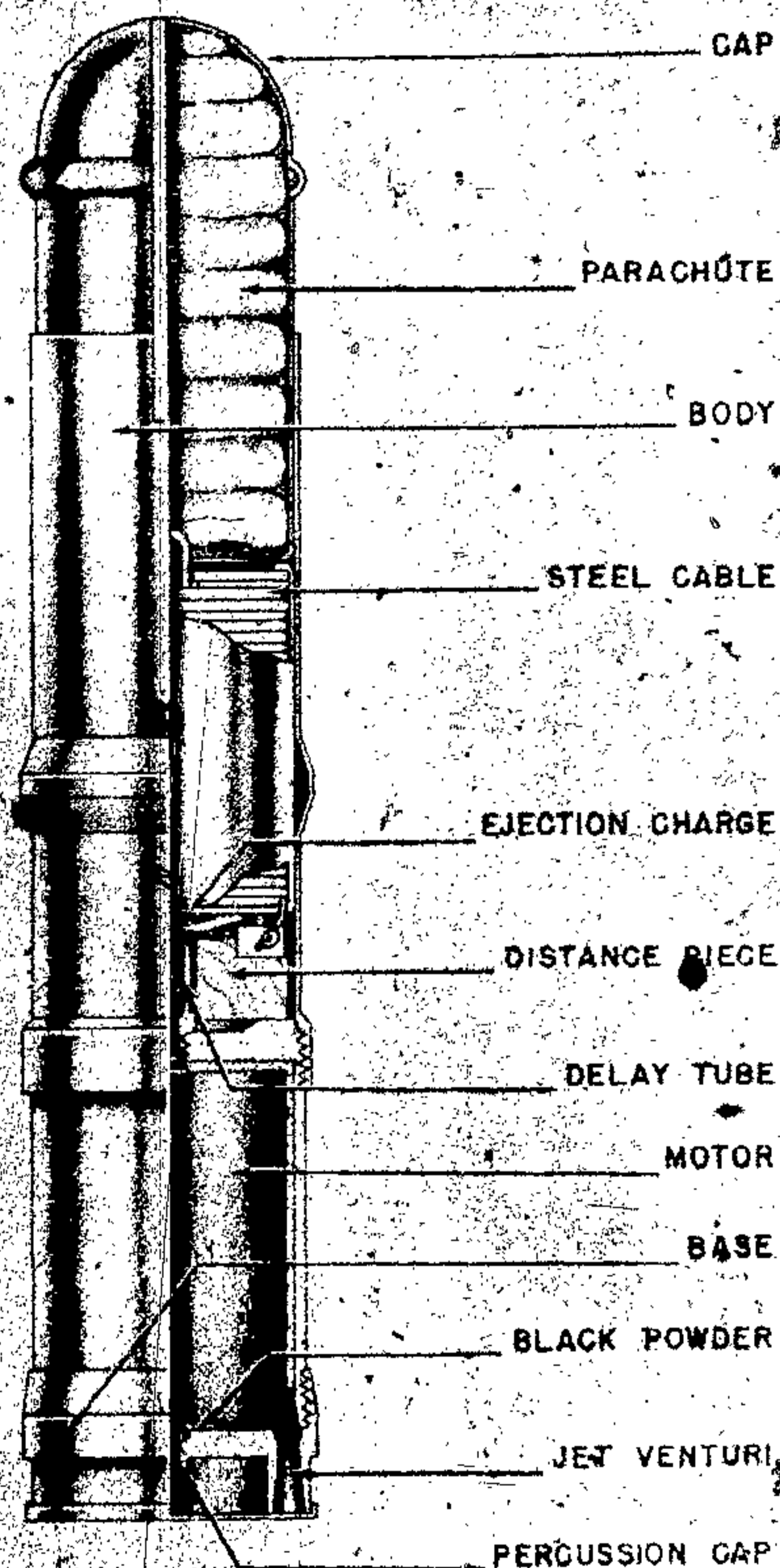
Figure 209—8.6-cm Antiaircraft Rocket (Naval)
