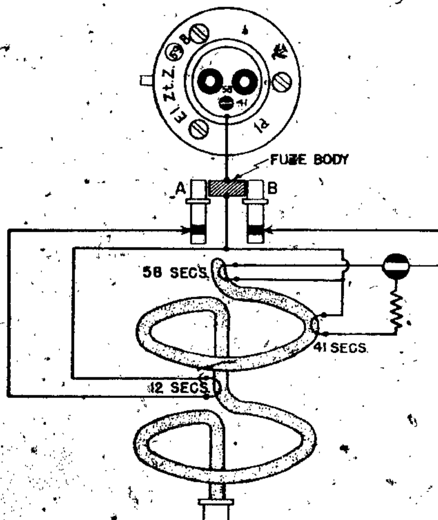
Figure 175—(59)B Electrical Aerial Burst Fuze
