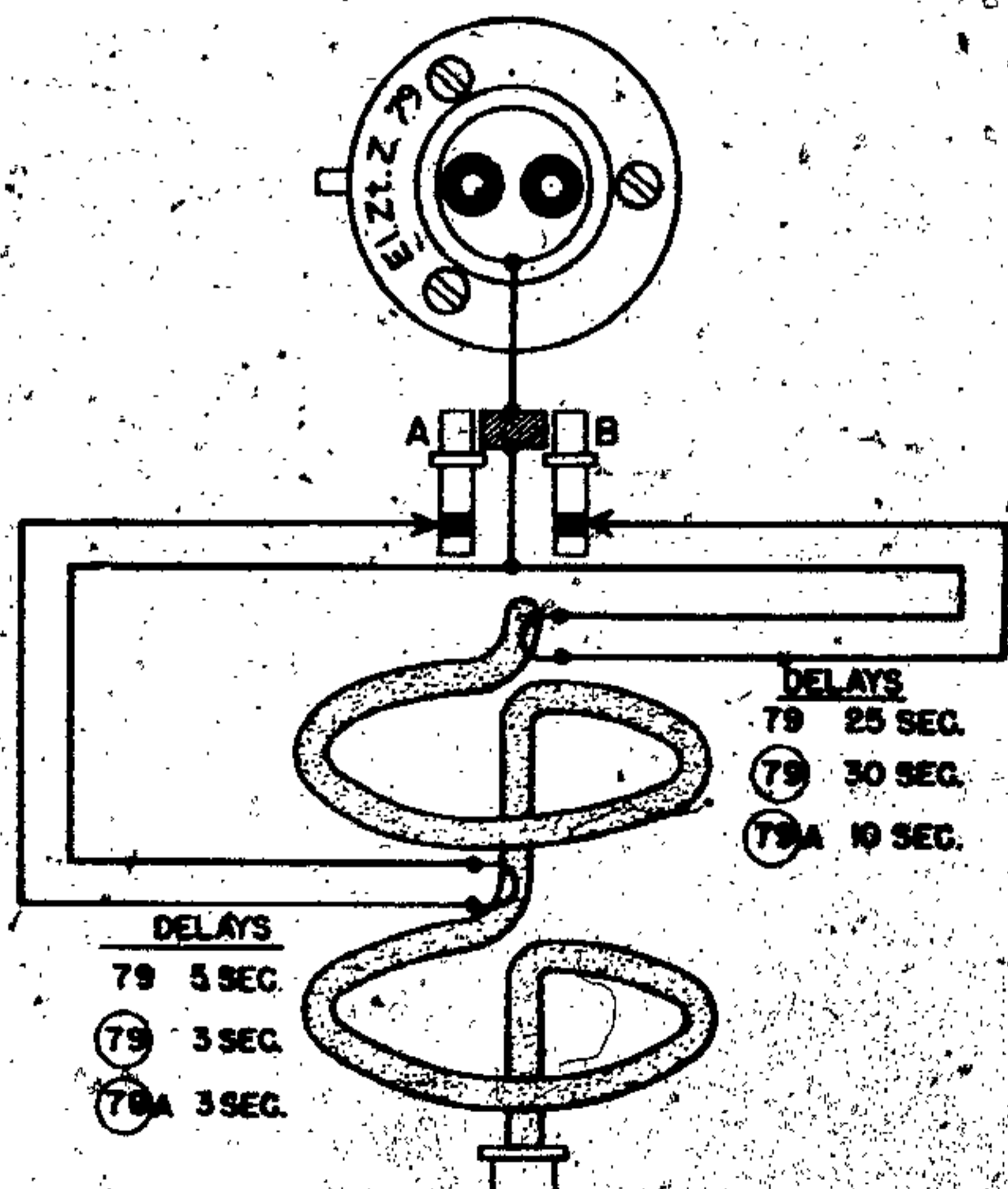
Figure 177—79 Electrical Aerial Burst Fuze
