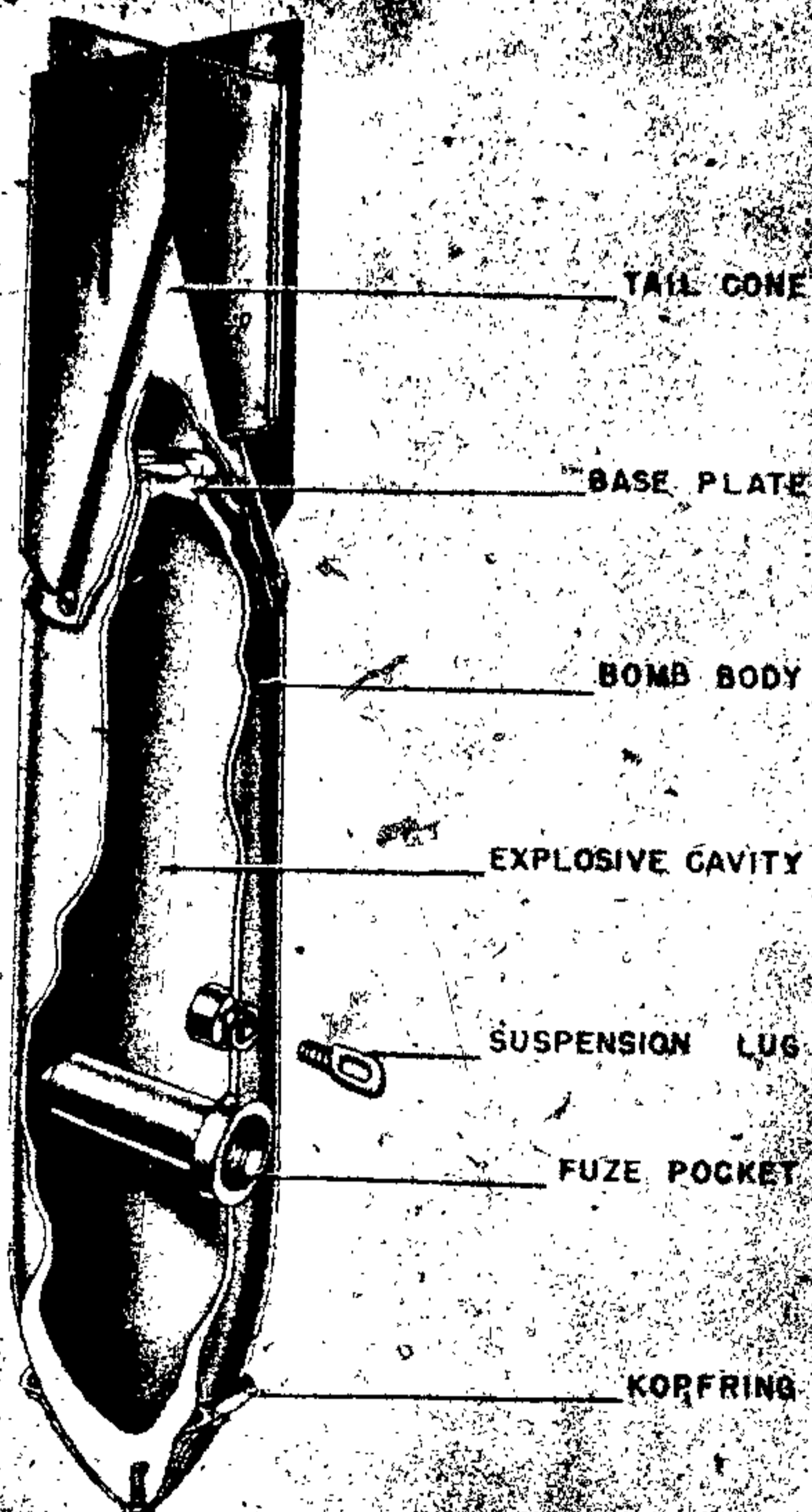
Figure 10—SC 50 Grade I Bomb
