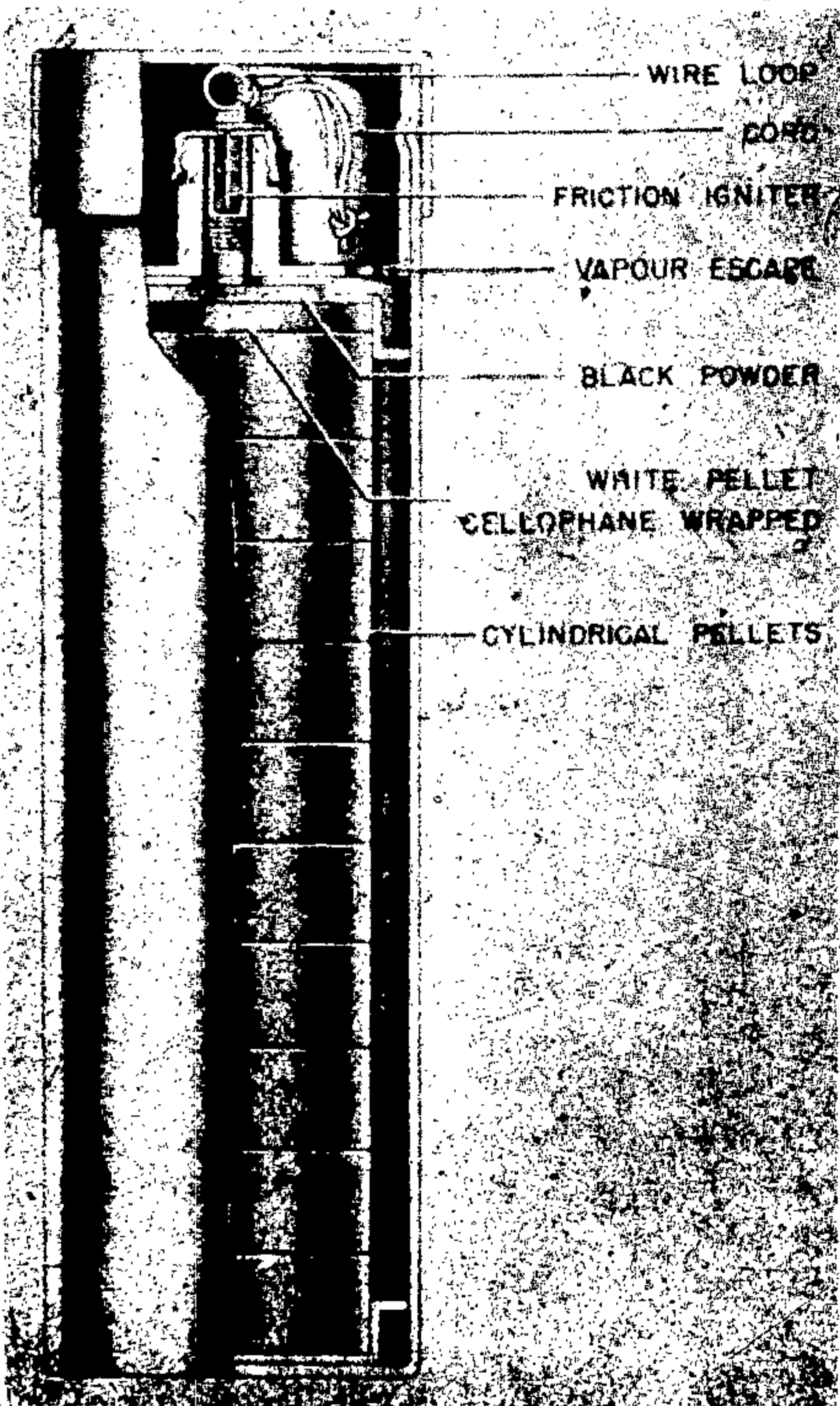
Figure 297—Lachrymatory Hand Grenade
