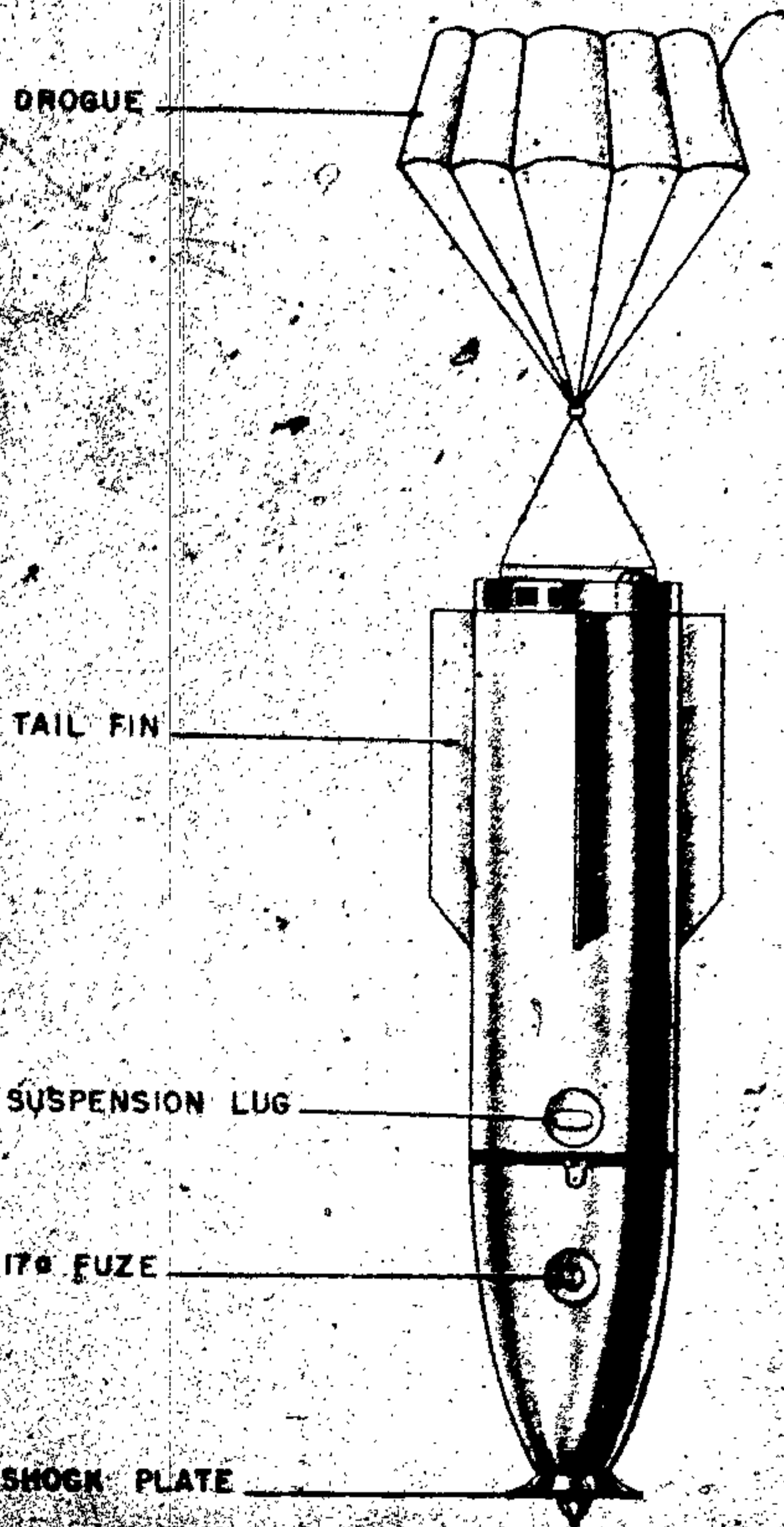
Figure 90—Lux EZ 50 SC Sea Marker
