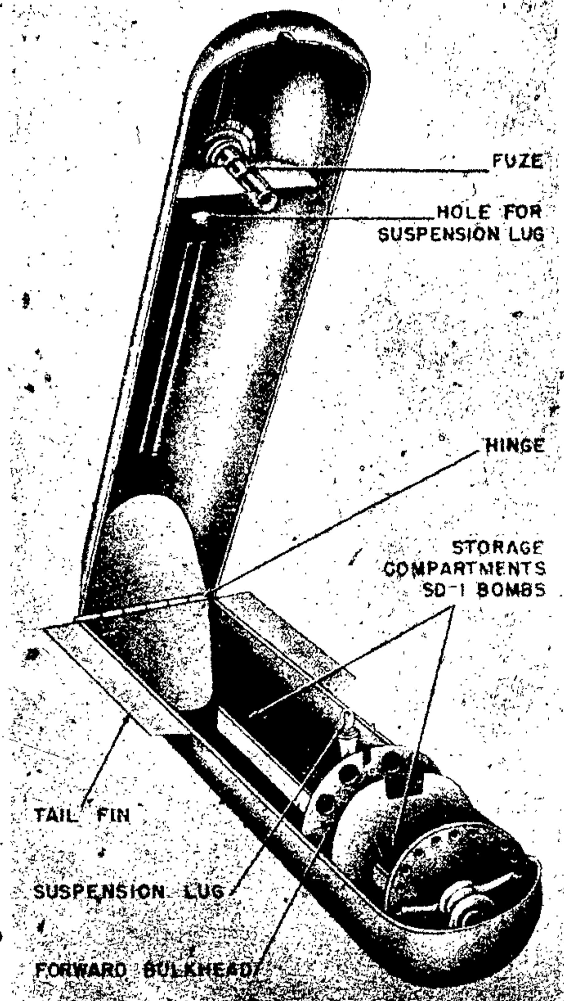
Figure 104—AB 70D1 Container
