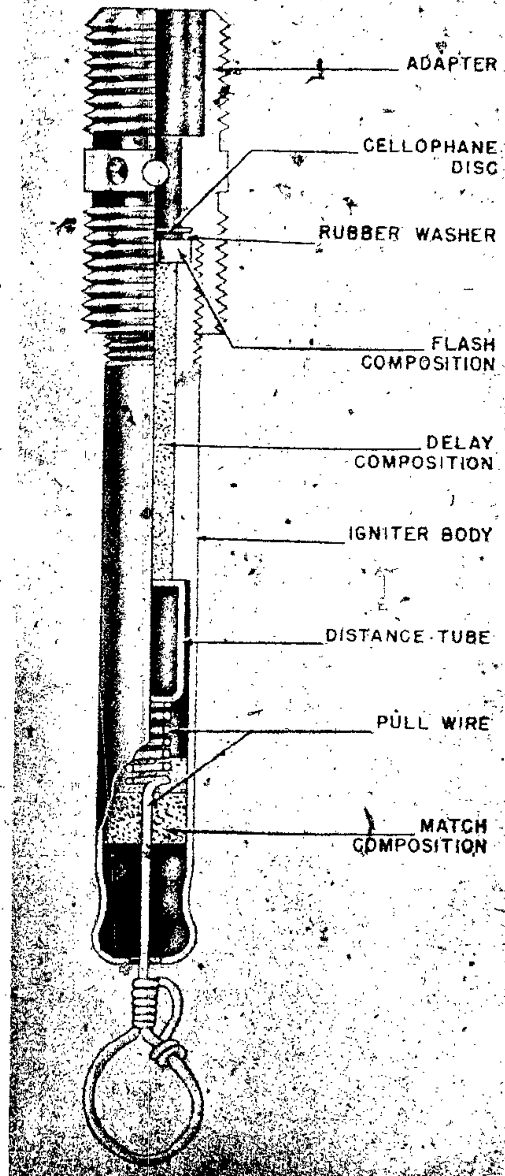
Figure 251—BZ-39 Friction Igniter Pull Type
