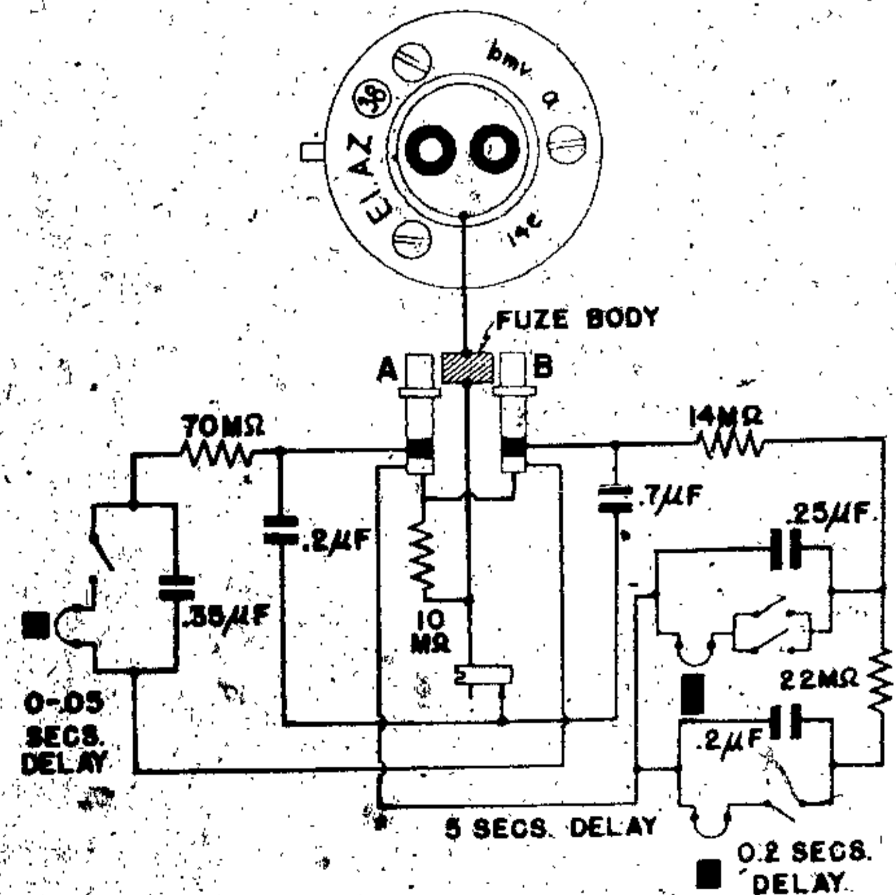
Figure 165—(38) Modified Electrical Impact Fuze
