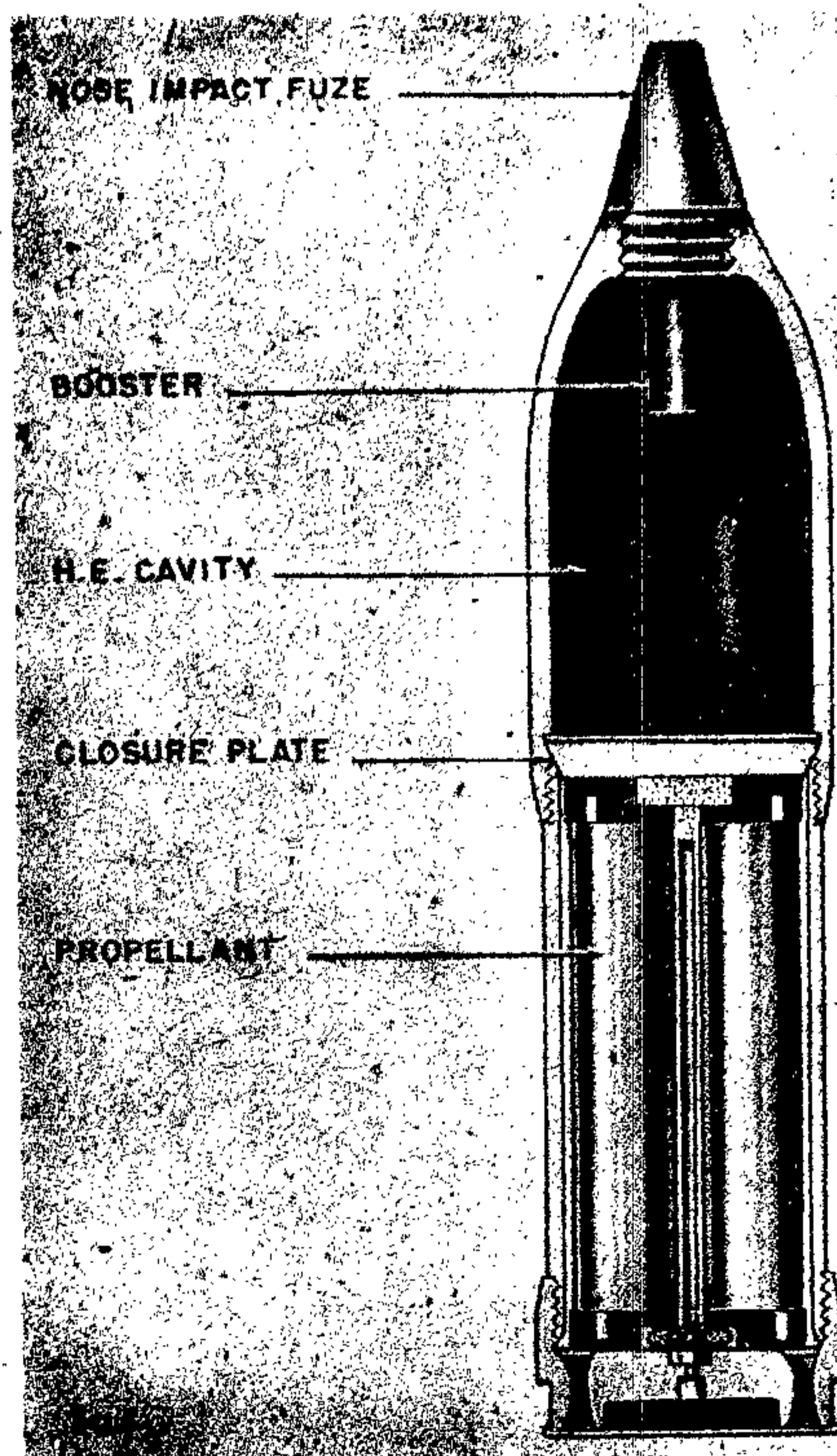
Figure 222—8.6-cm R. Spgr L/4.5 Rocket
