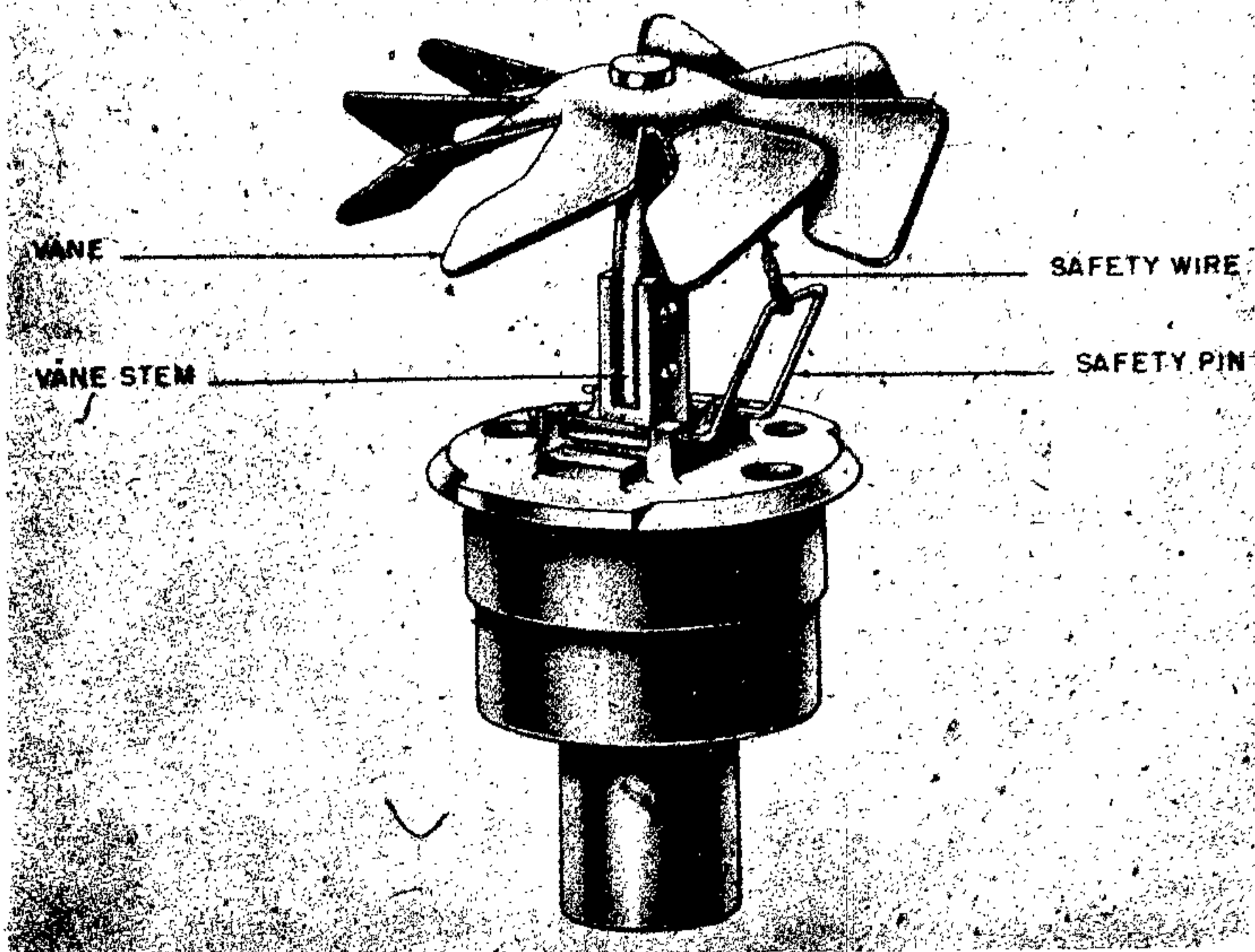
Figure 189—(70) B Modified Antidisturbance Fuze
