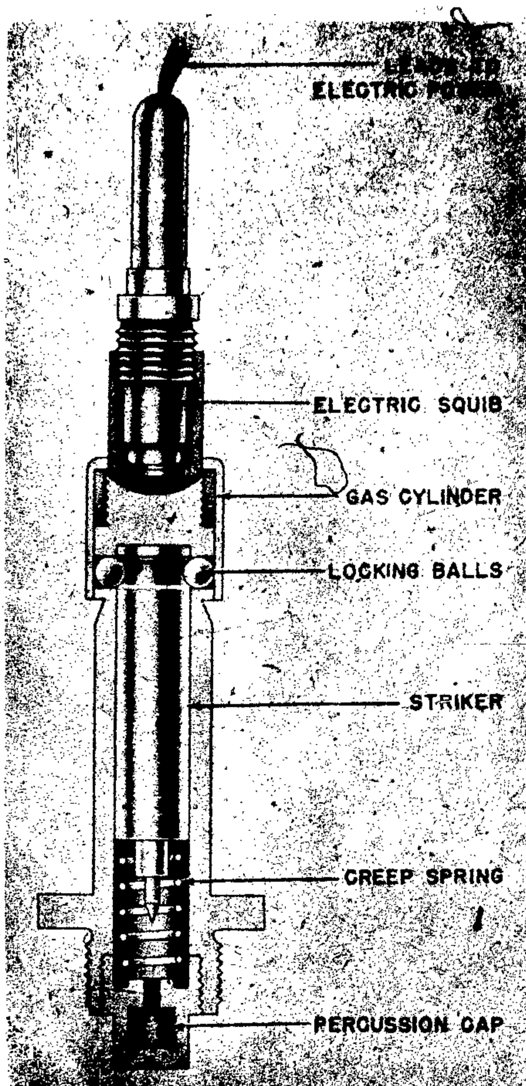
Figure 148—(46) Electrical Impact Tail Fuze
