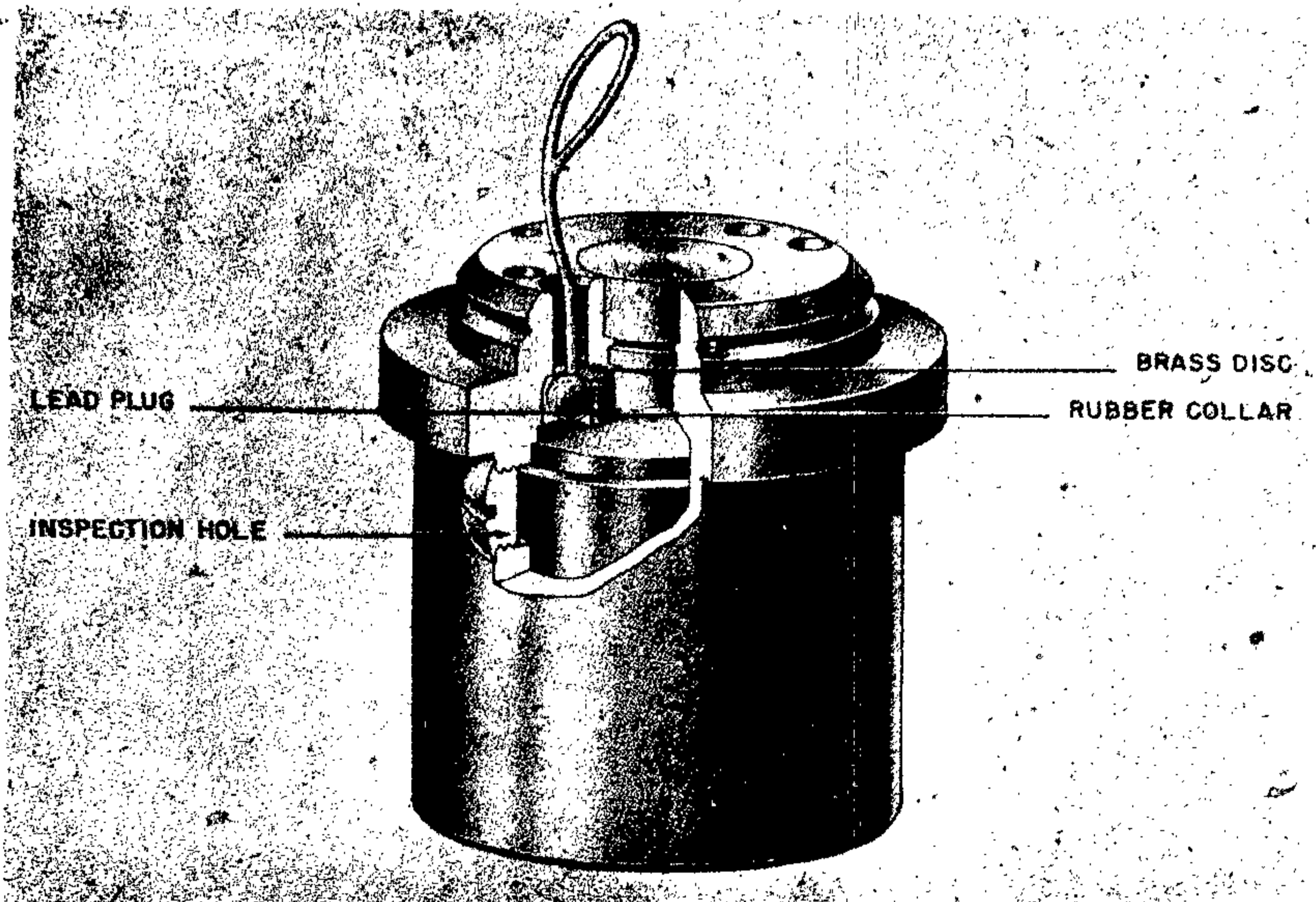
Figure 178—(89) Clockwork Aerial Burst Fuze
