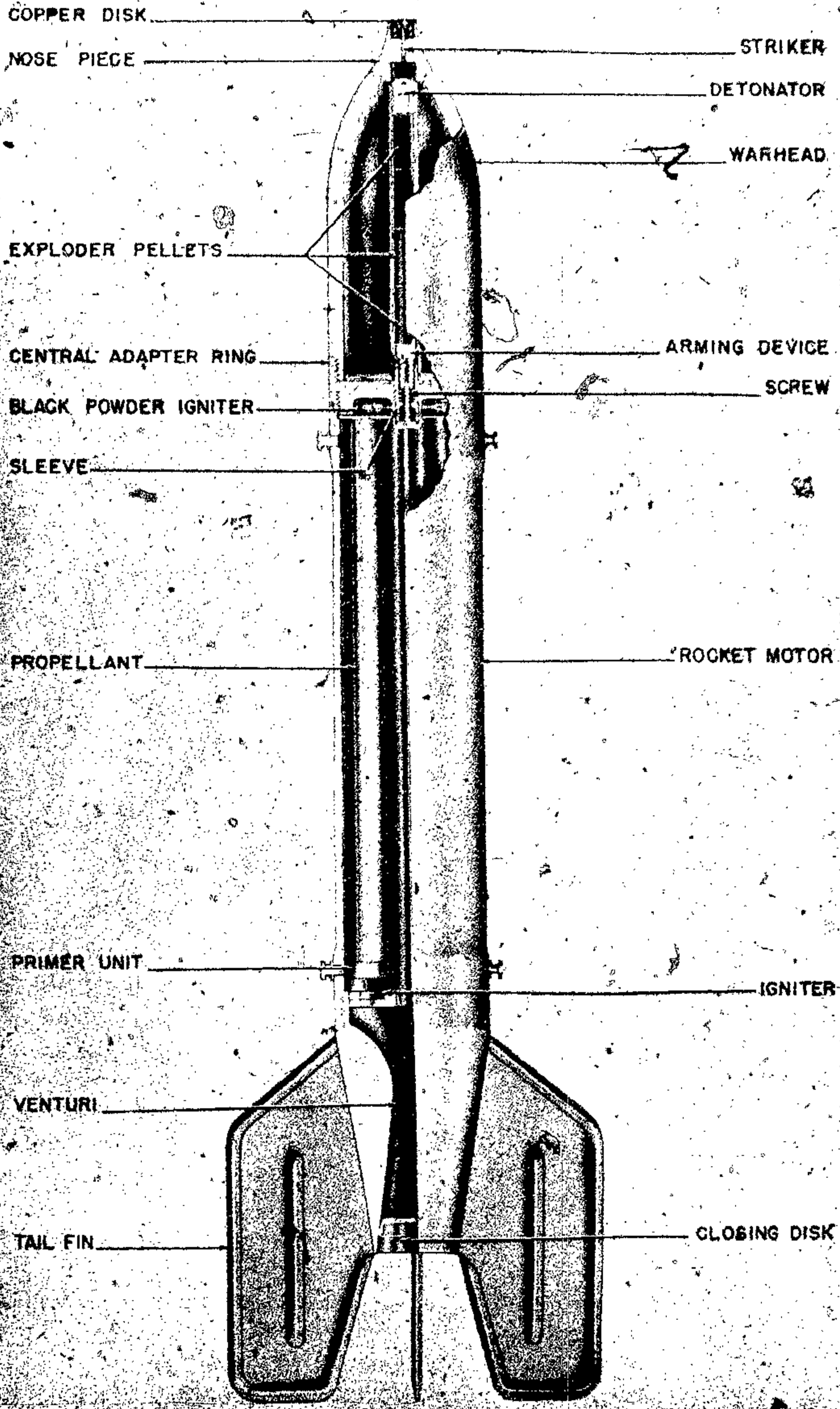
Figure 206—8-cm Aircraft Rocket
