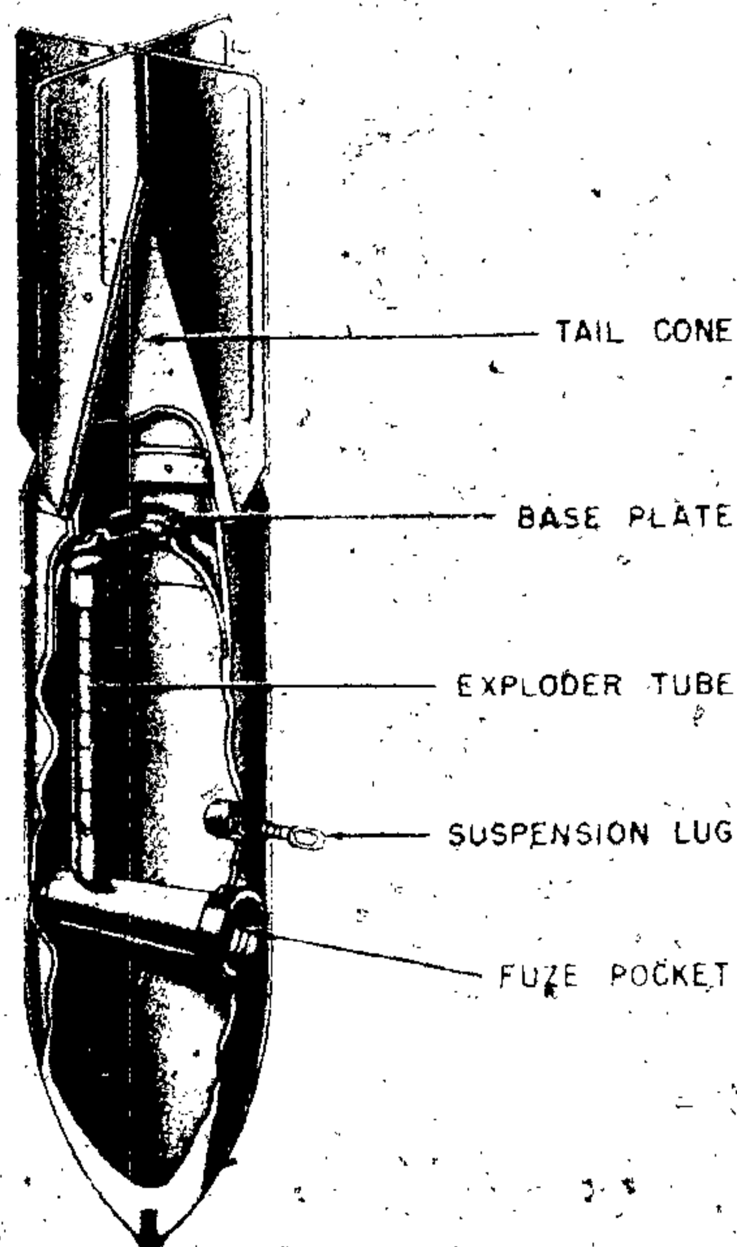
Figure 11—SC 50 Grade II Bomb
