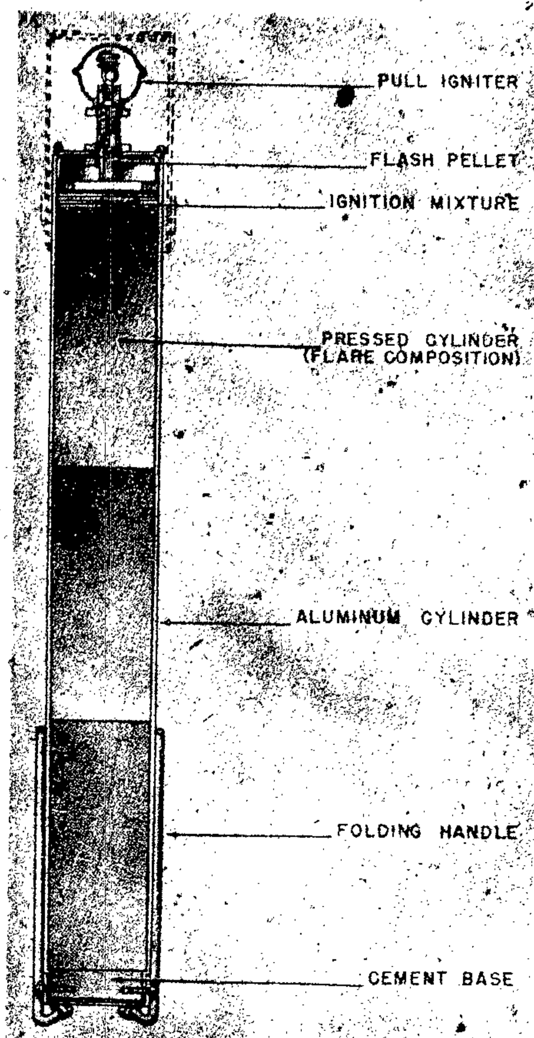
Figure 85—Distress Signal Torch
