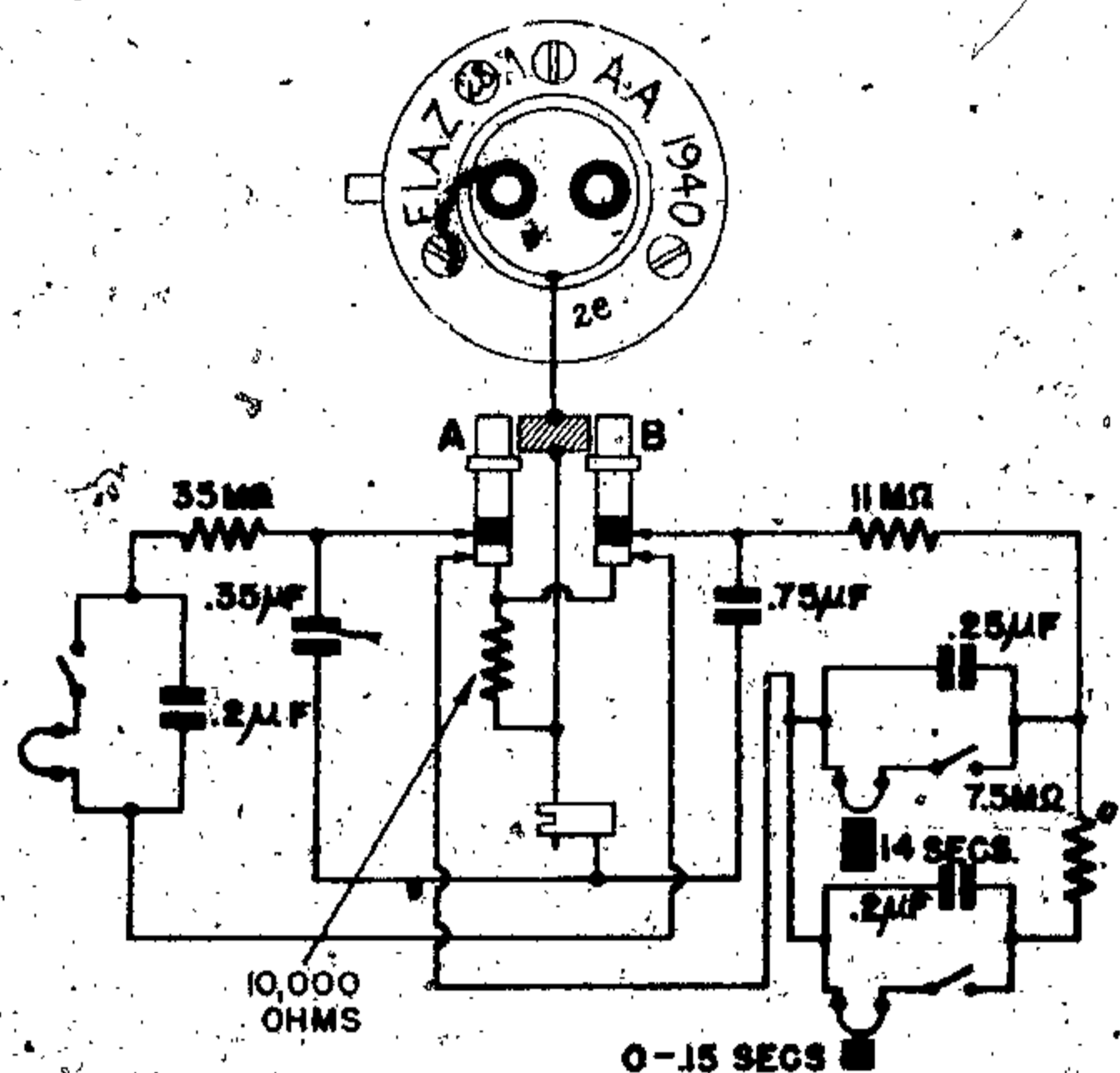
Figure 160—(28)A Electrical Impact Fuze
