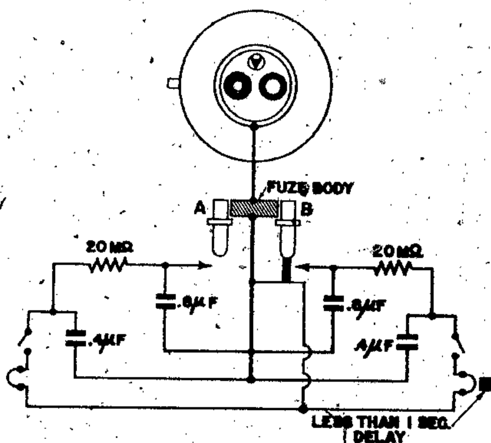
Figure 137—(A) Electrical Impact Fuze
