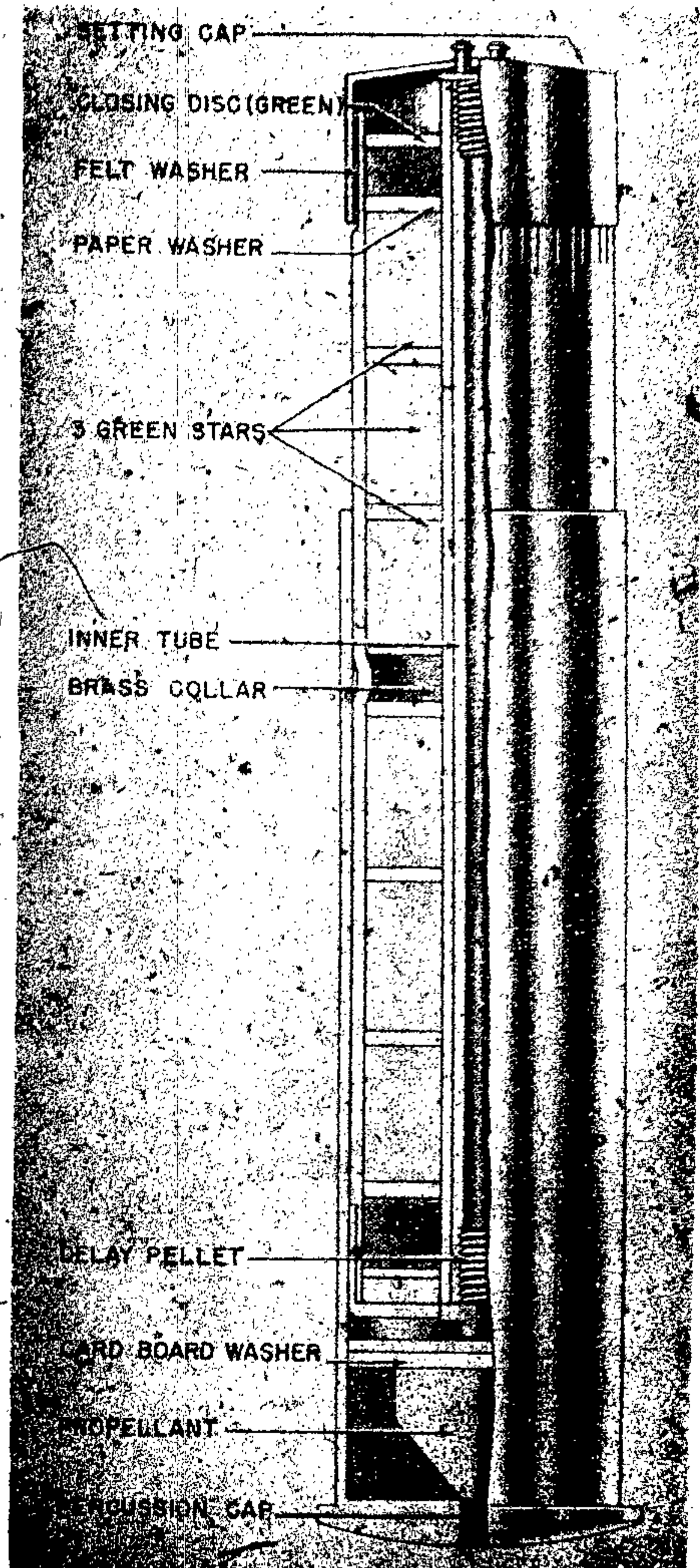
Figure 315—27-mm Multistar Pistol Cartridge
