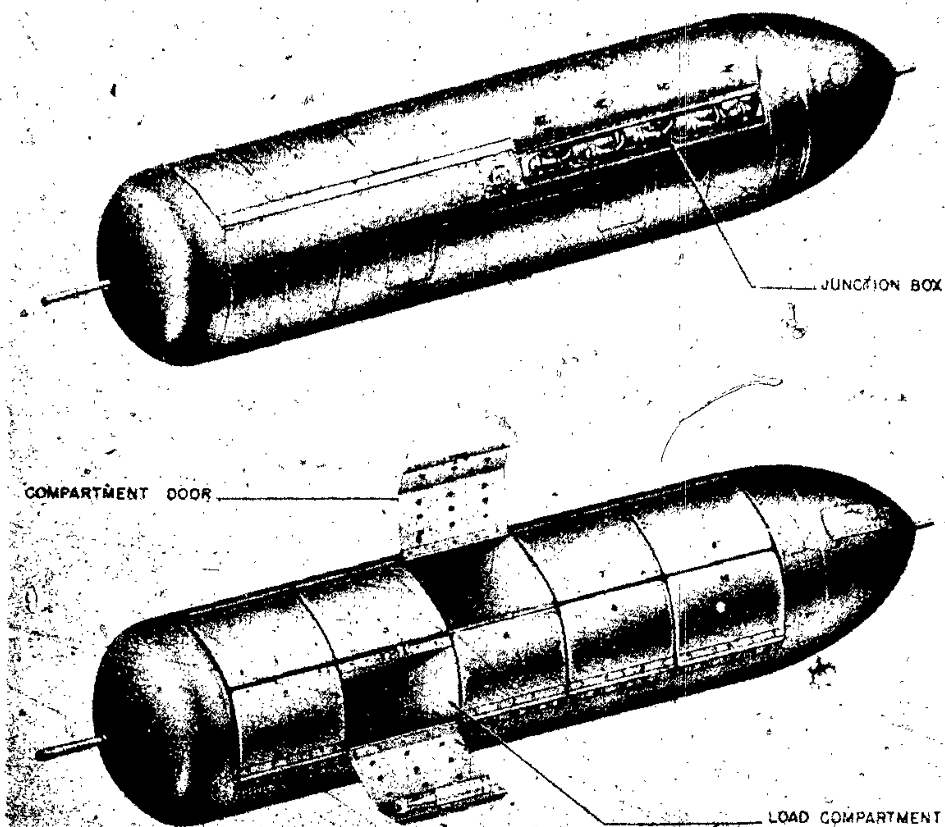
Figure 110—BSB 1000 Container
