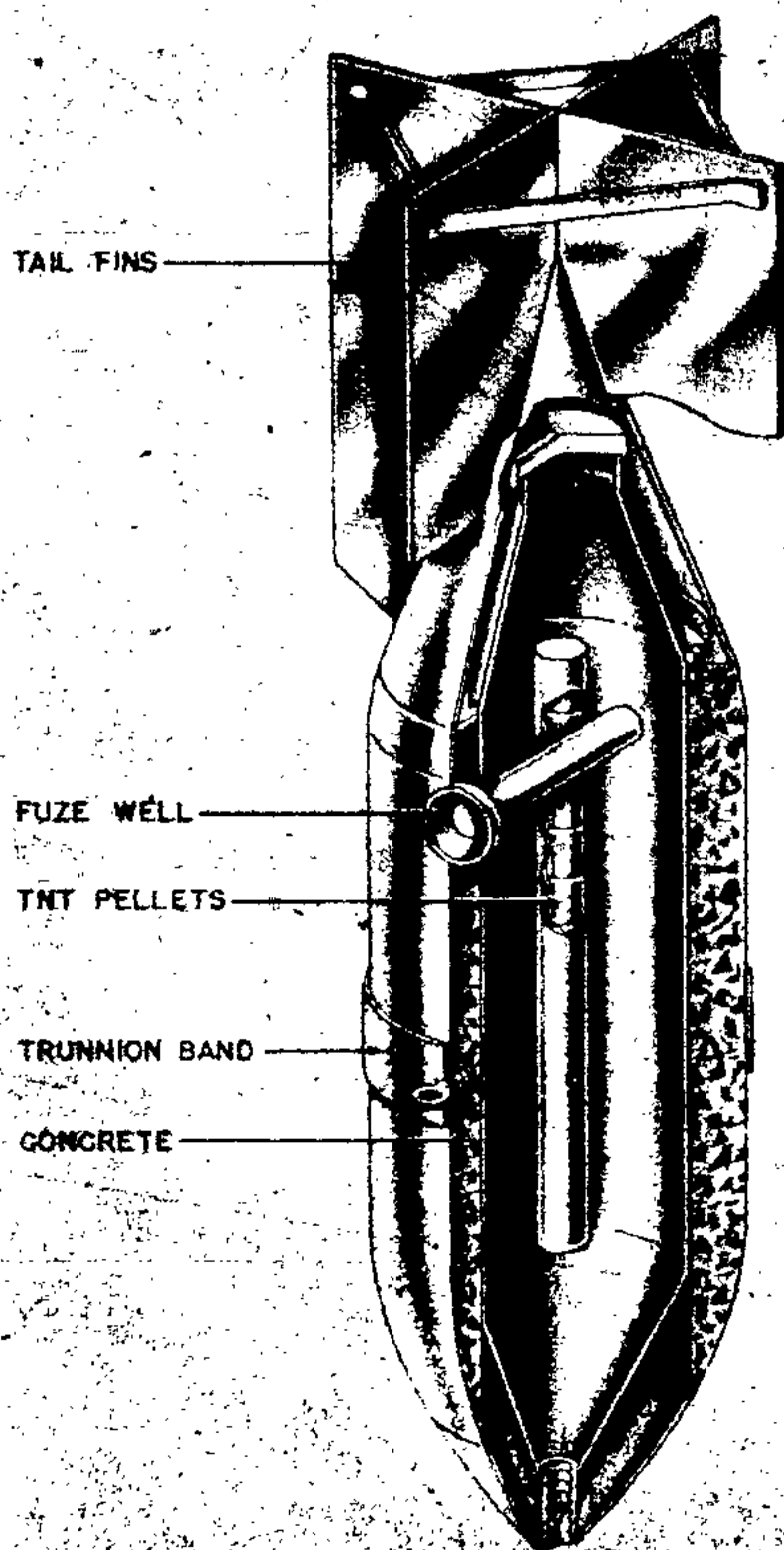
Figure 47—SBe 250-Kg Concrete Bomb
