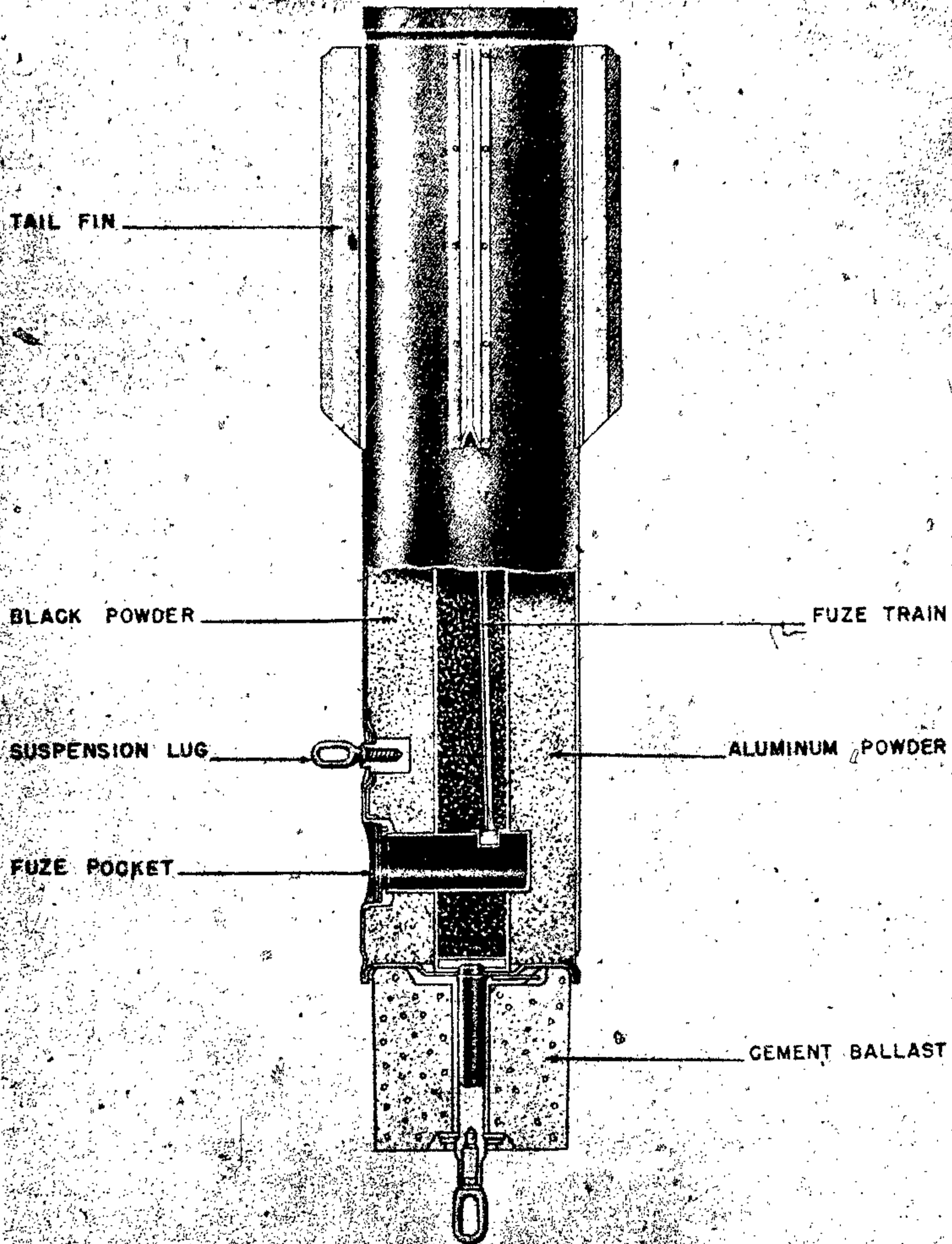
Figure 87—BLC 50/A Photoflash Bomb
