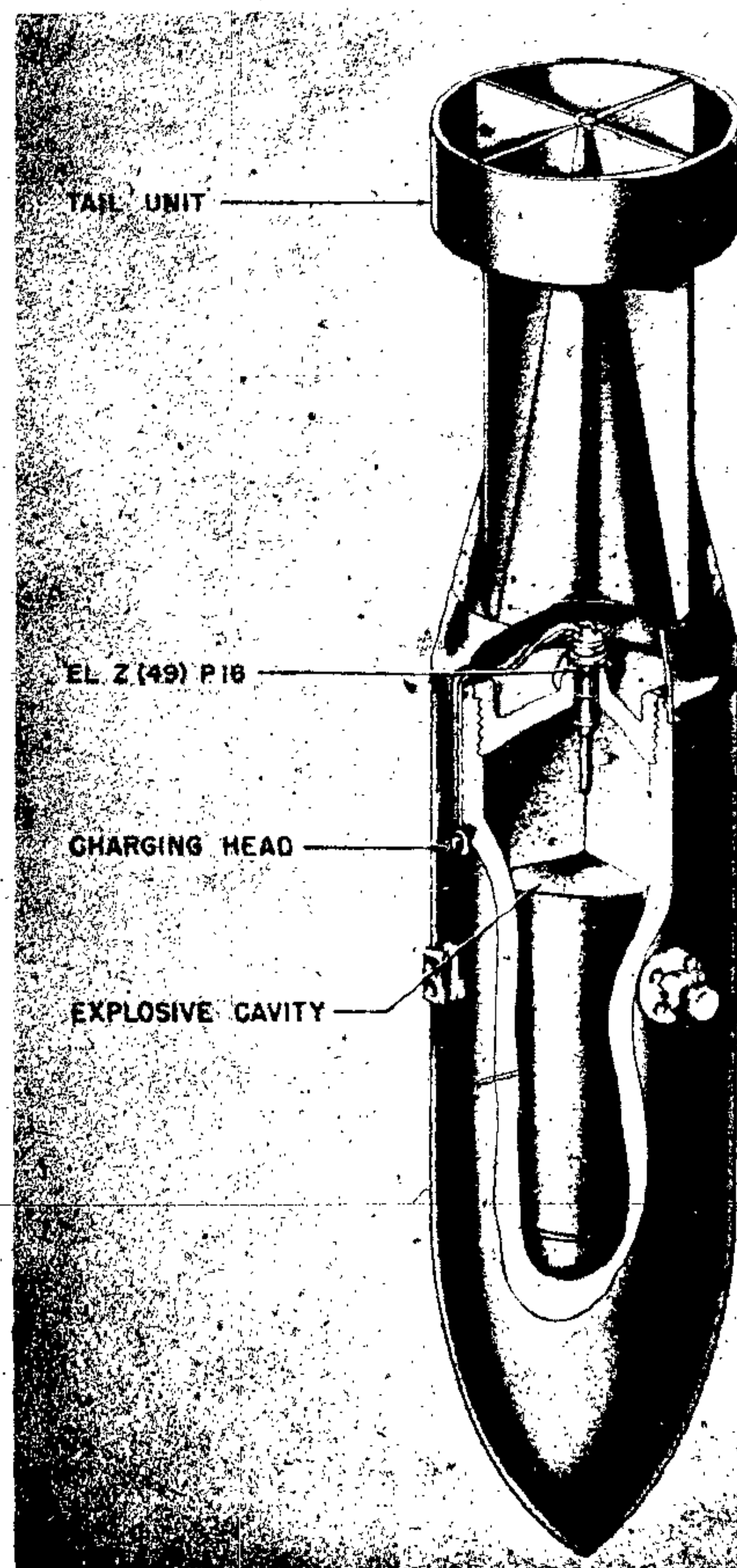
Figure 32—PC 1600-Kg Bomb
