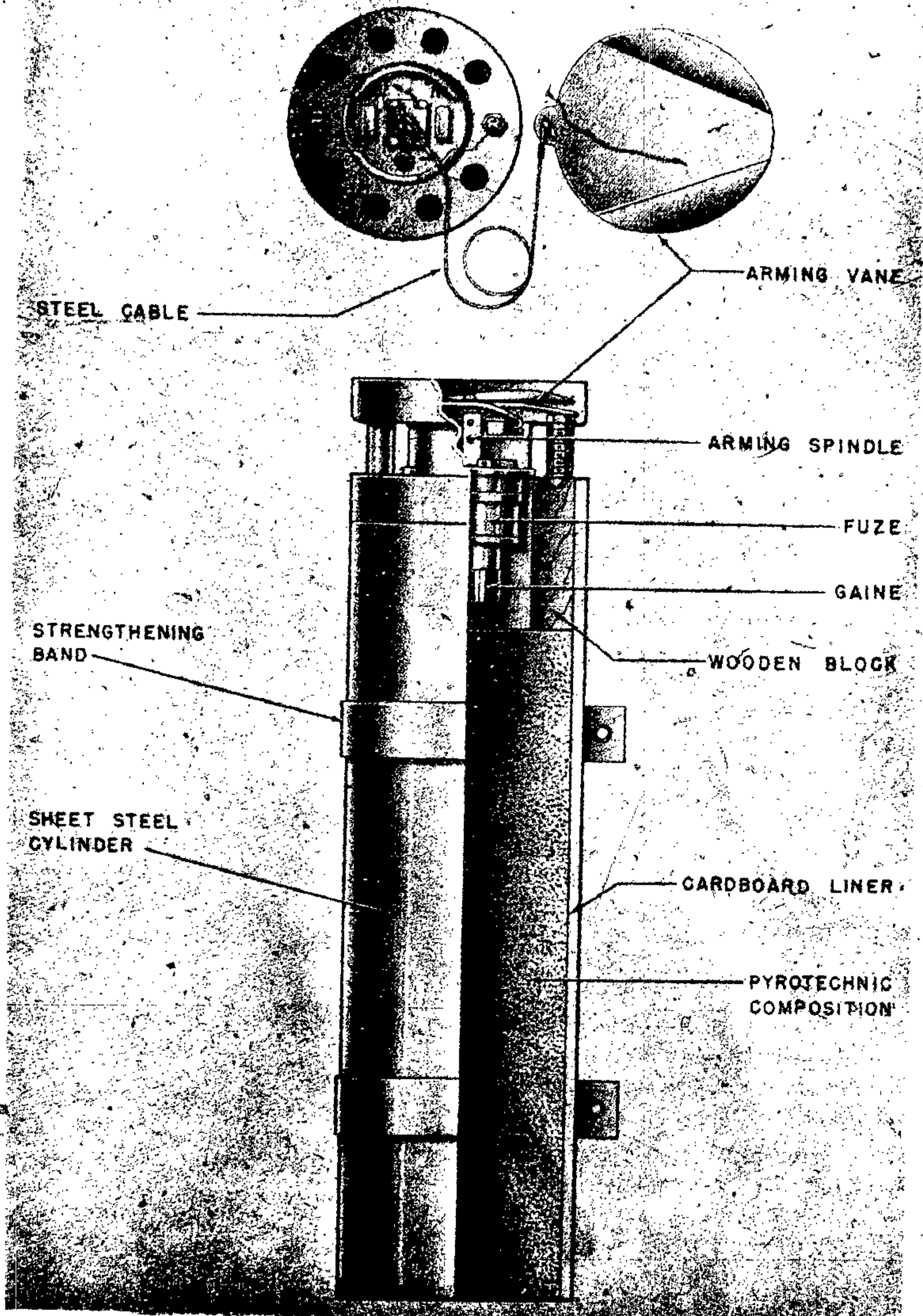
Figure 91—Mark 3 Single Unit Ground Marker (Green)
