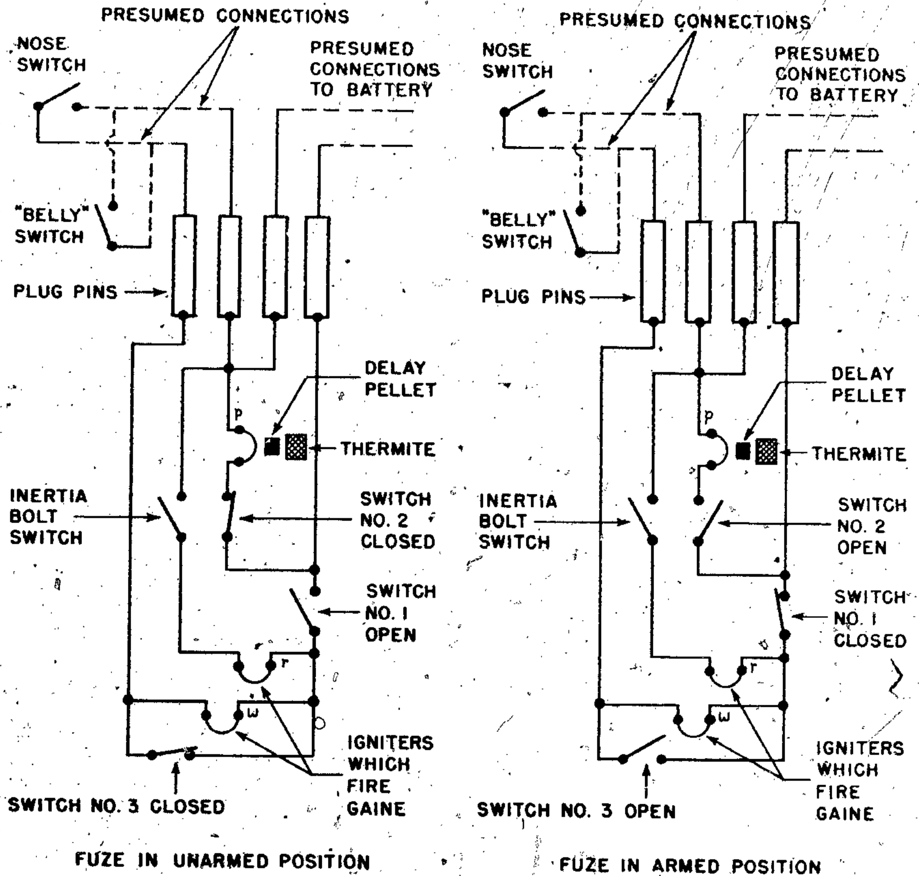
Figure 151B—(106)* Electrical Impact Fuze Wiring Diagram
