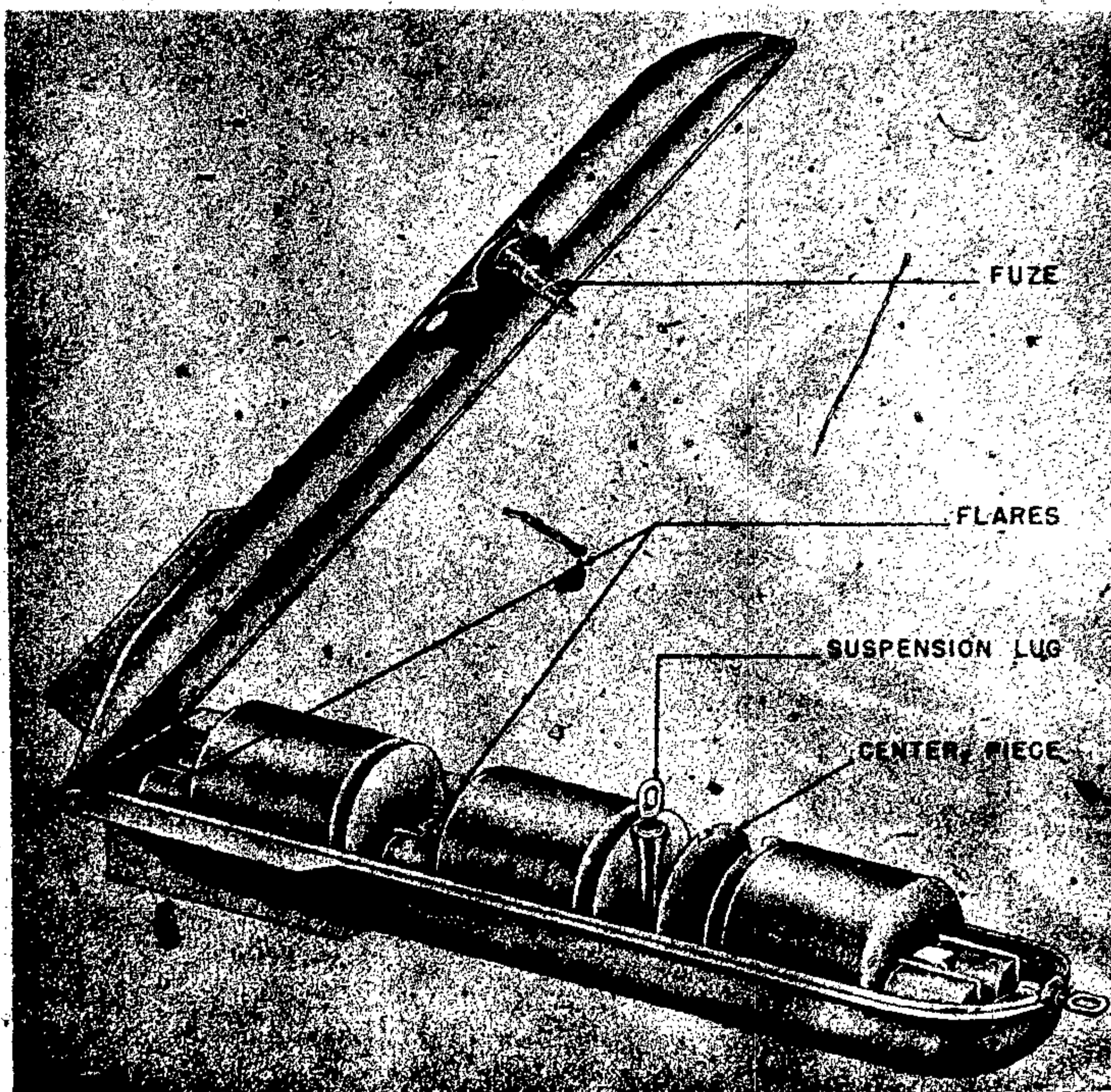
Figure 102—AB 70-3 Container
