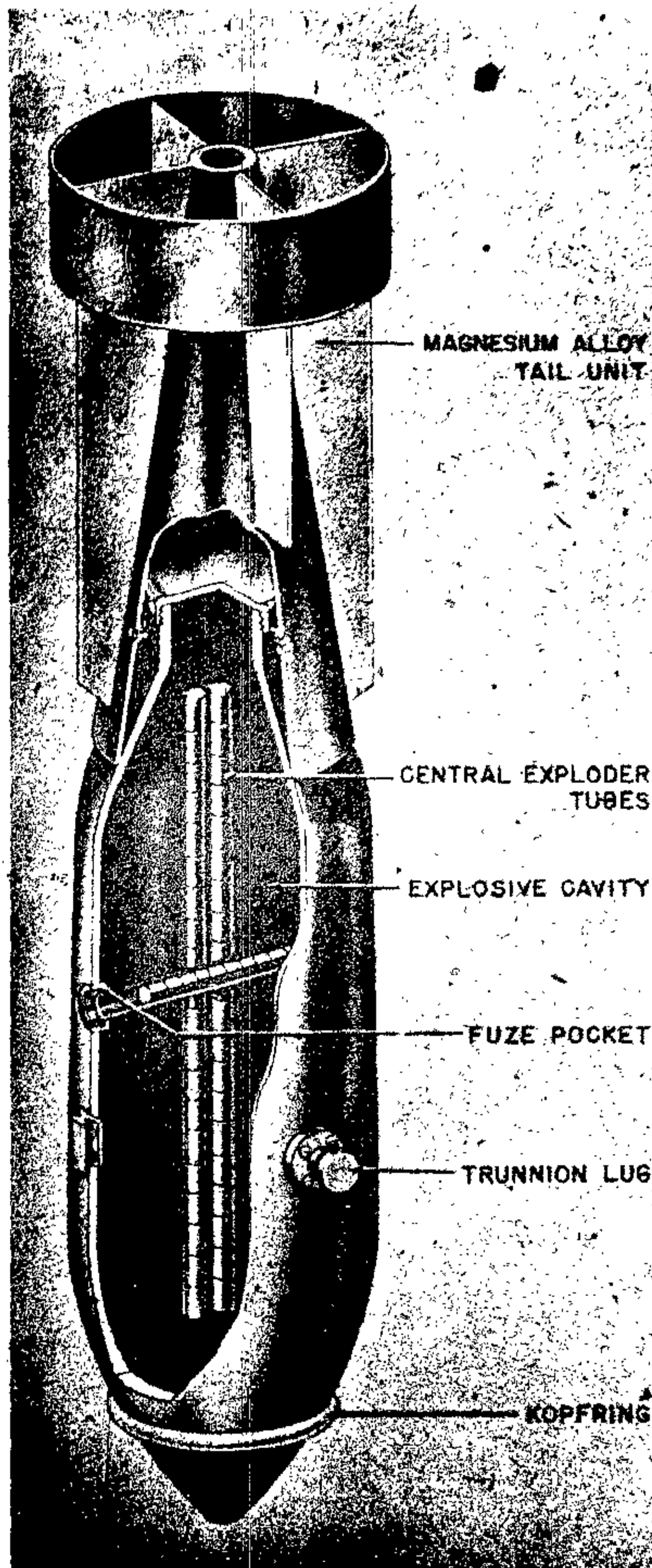
Figure 28—SD 1700-Kg Bomb
