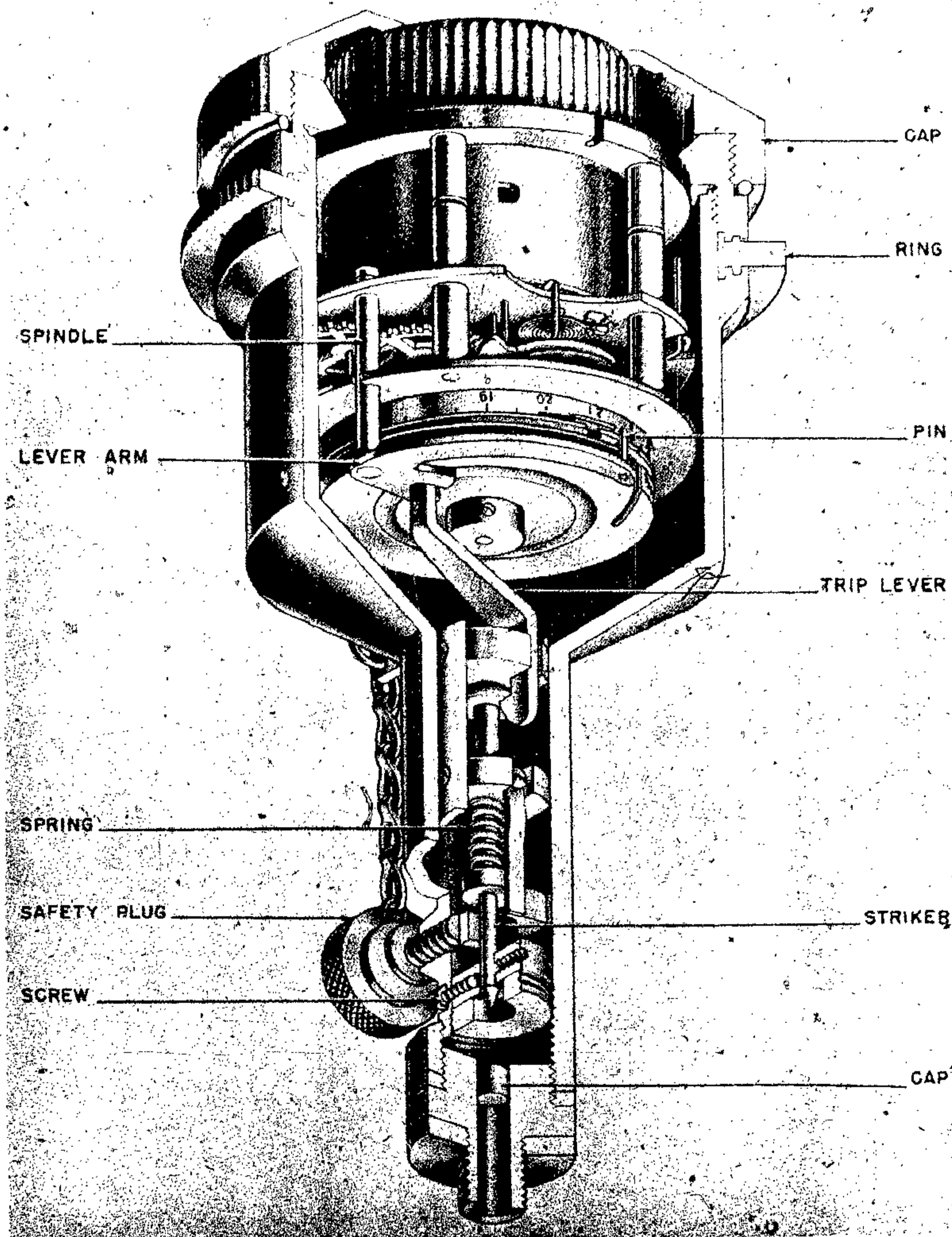
Figure 278—J-Feder 504 Clockwork
