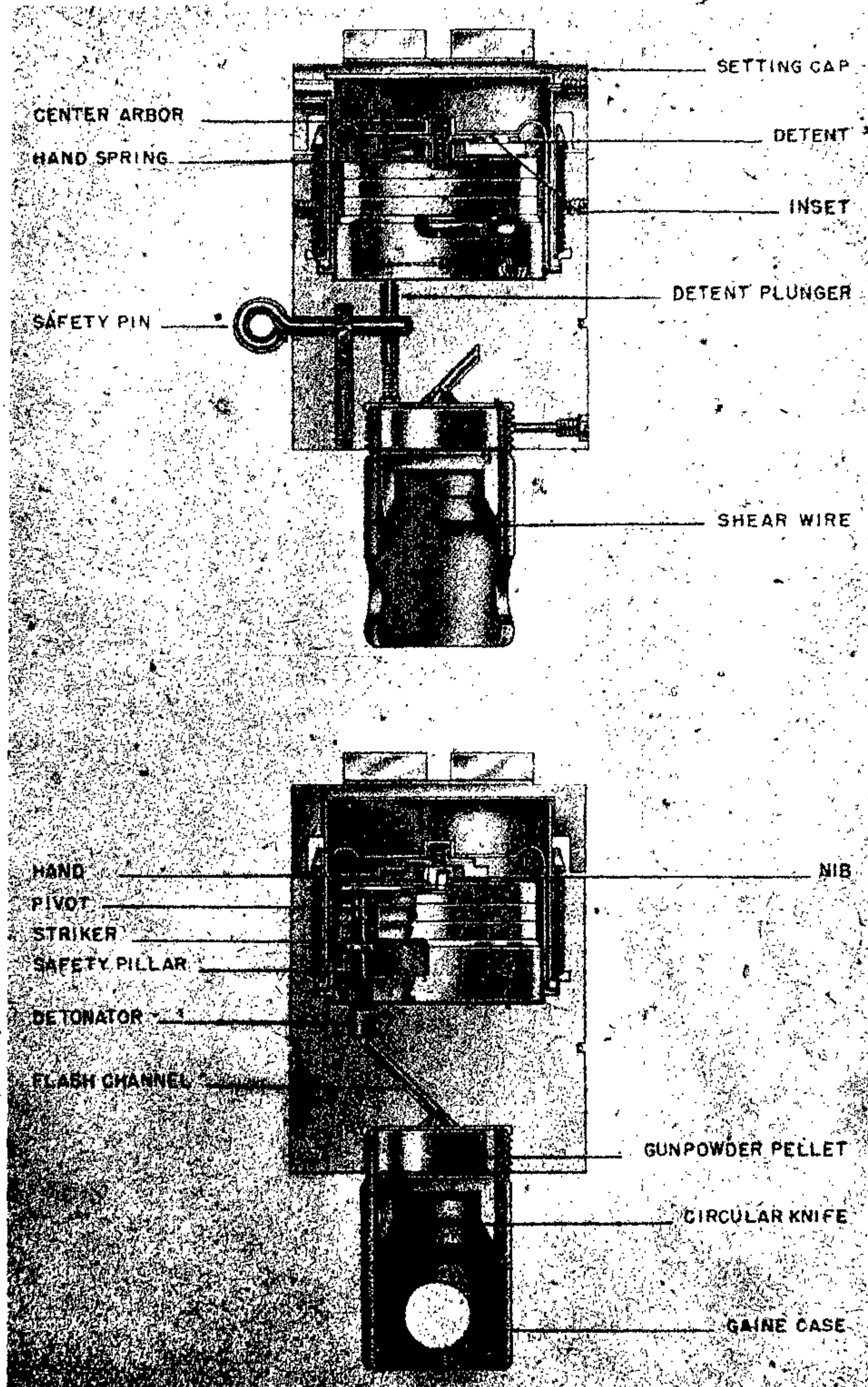
Figure 187—FZ 60 Clockwork Aerial Burst Fuze
