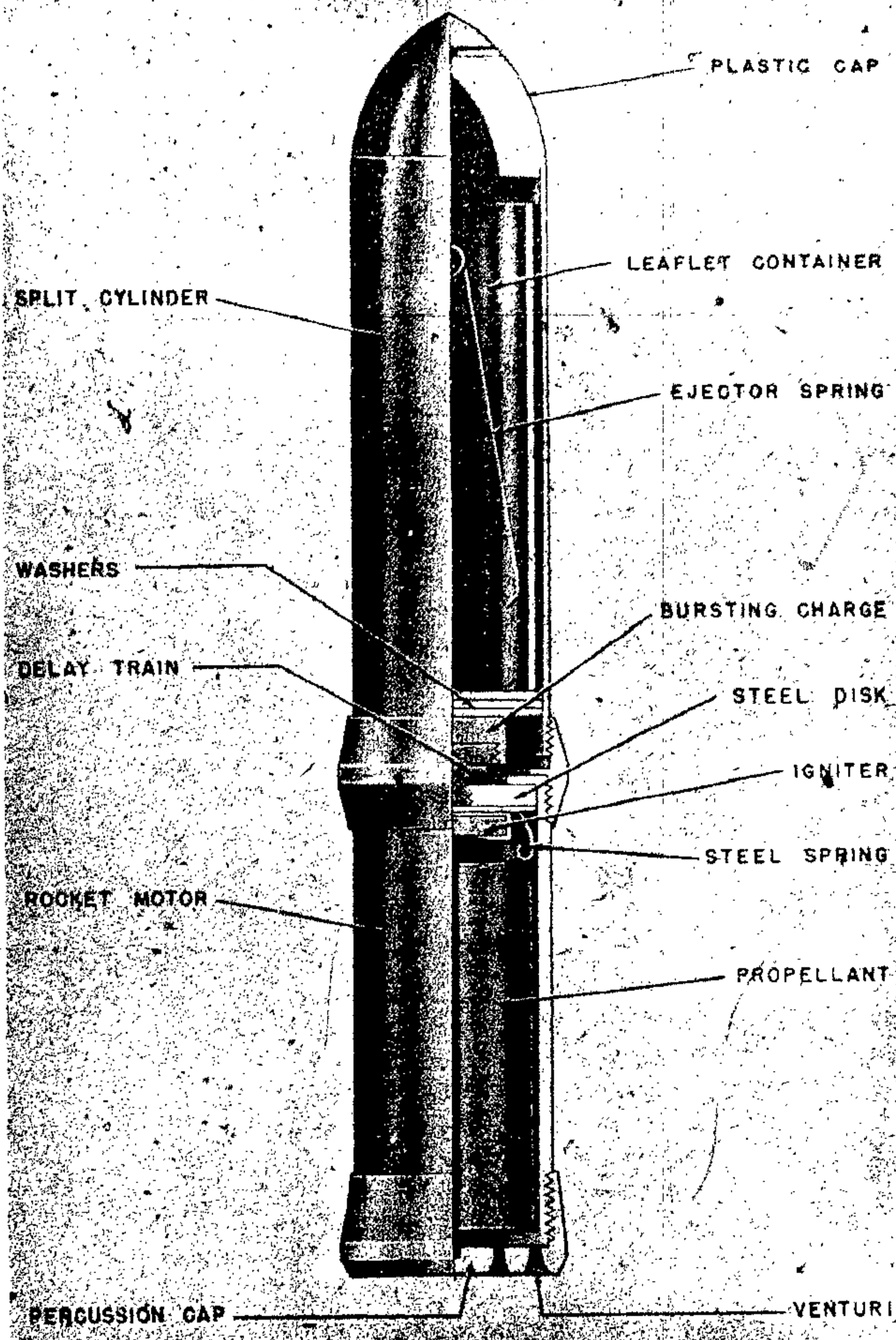
Figure 204—7.3-cm Propaganda Rocket
