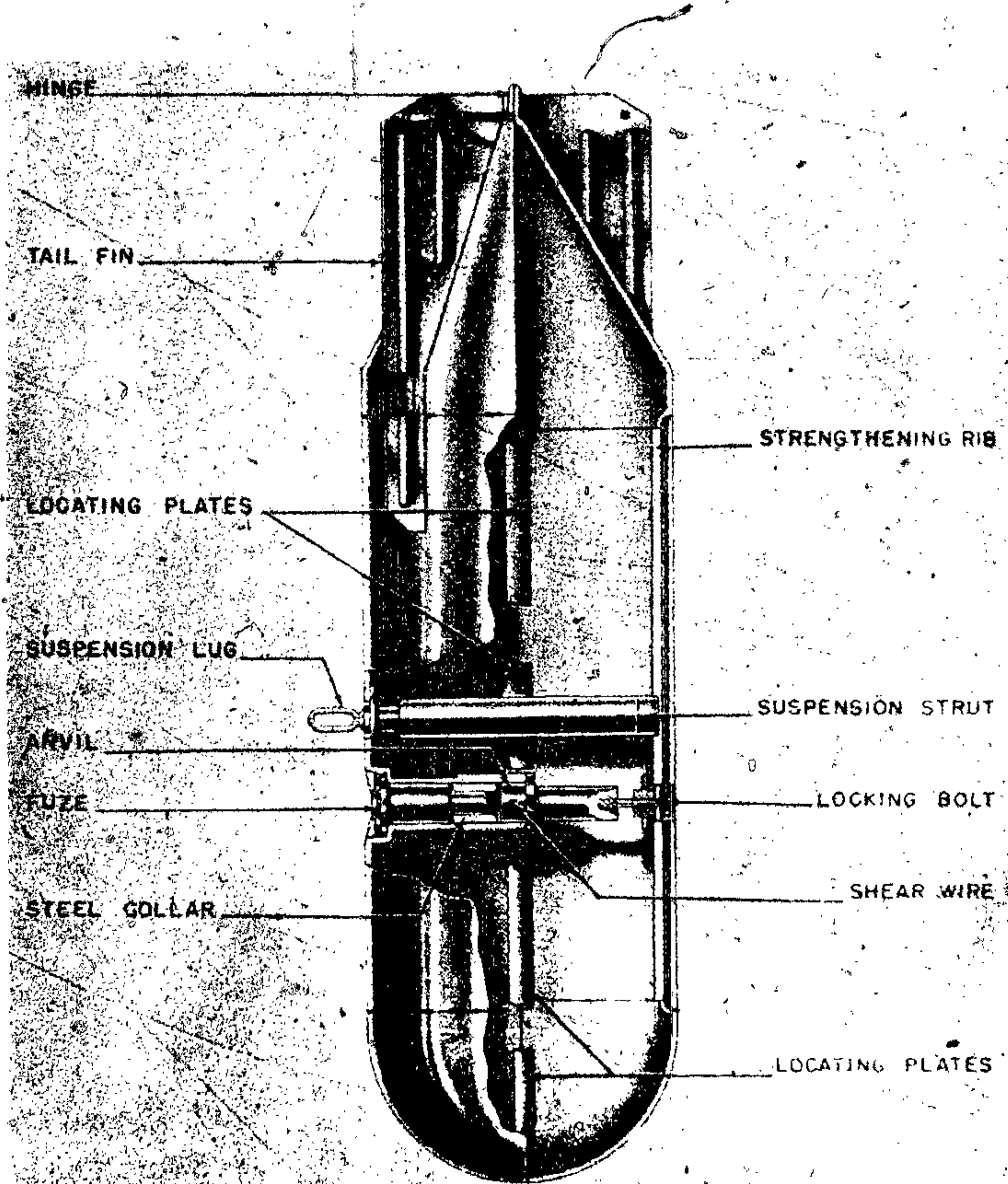
Figure 109—Mark 250 LK Container
