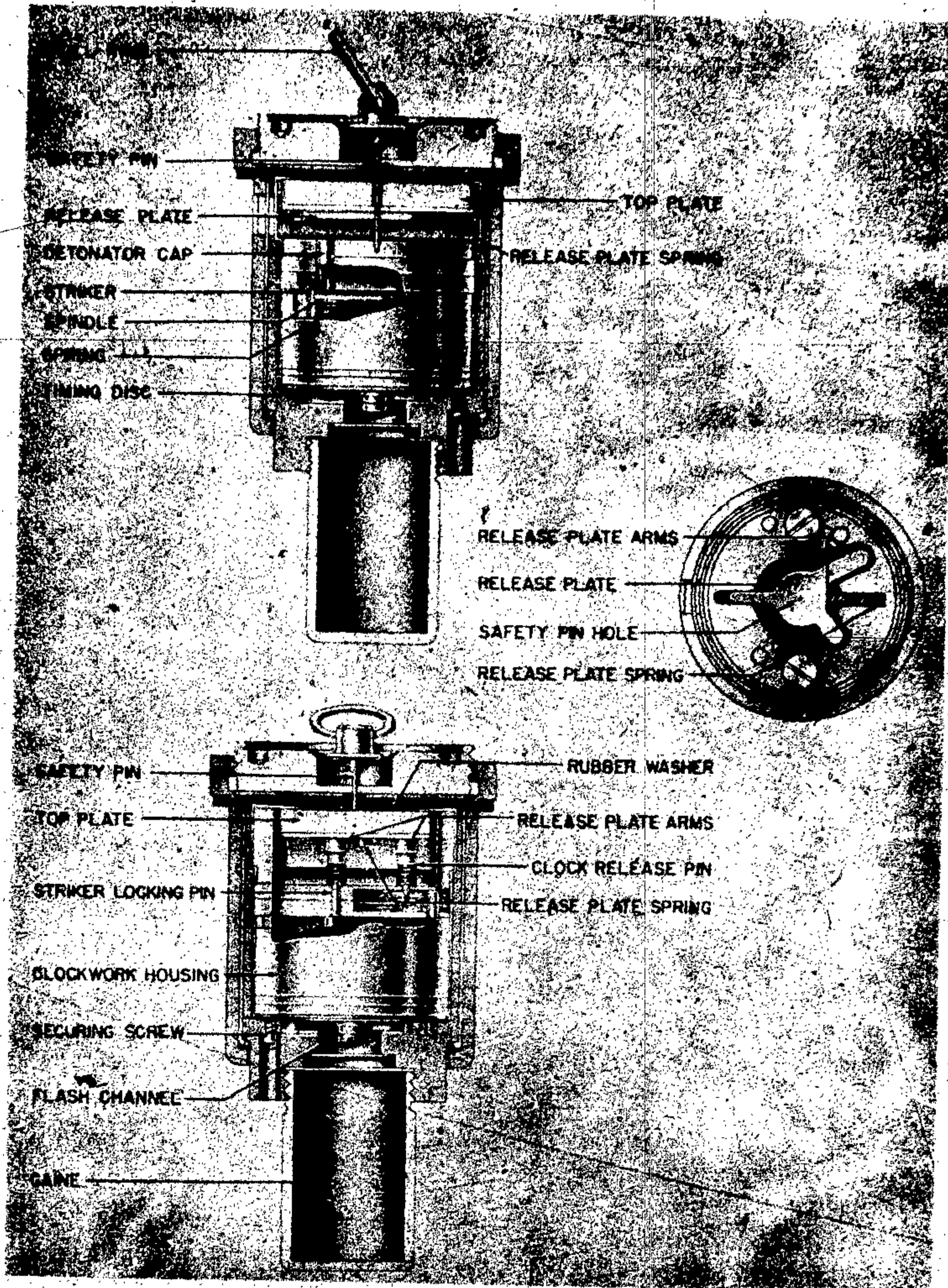
Figure 155—Z 17 Bm. Mechanical Clockwork Fuze
