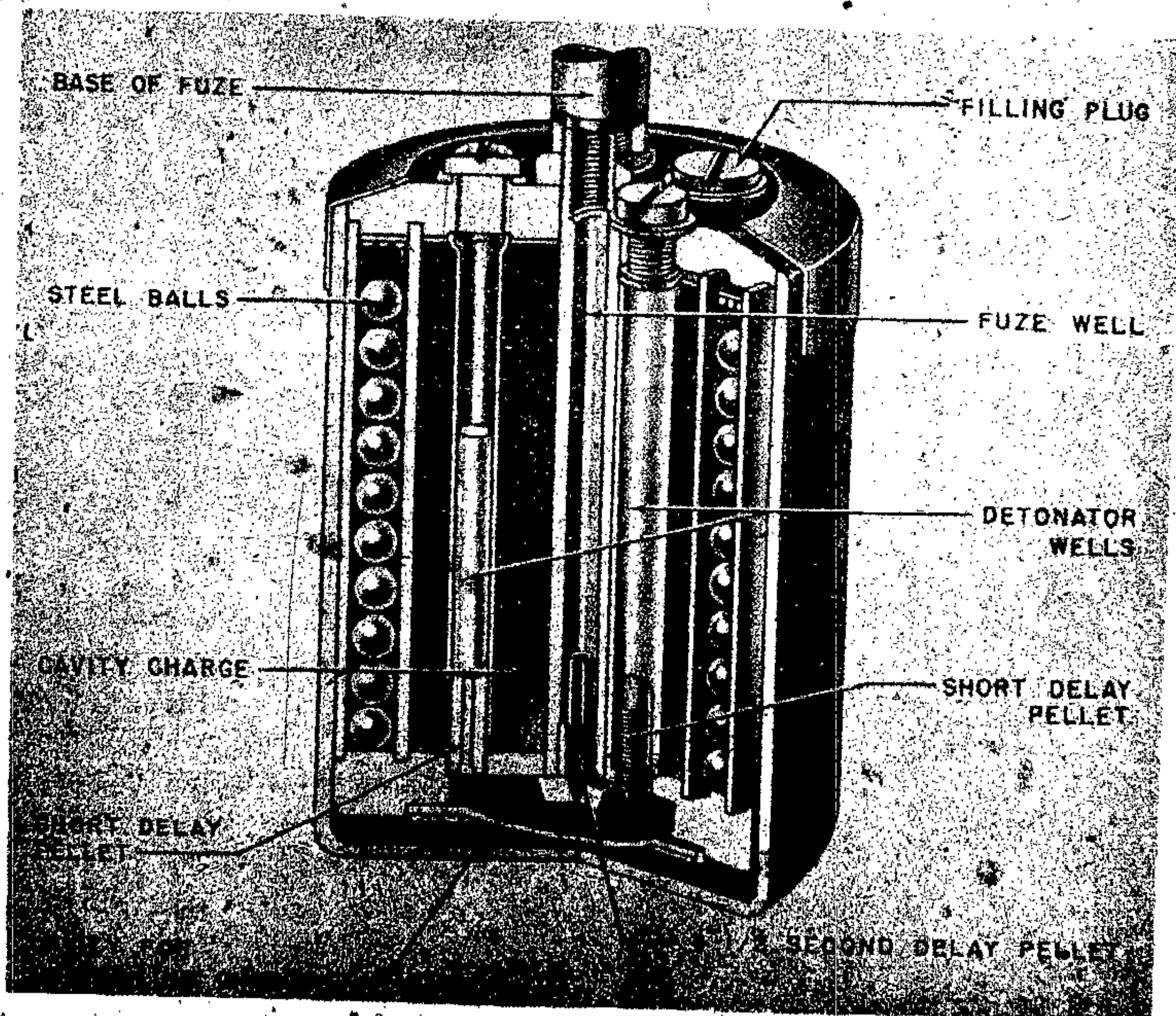
Figure 246—S-Mine 35—Antipersonnel
