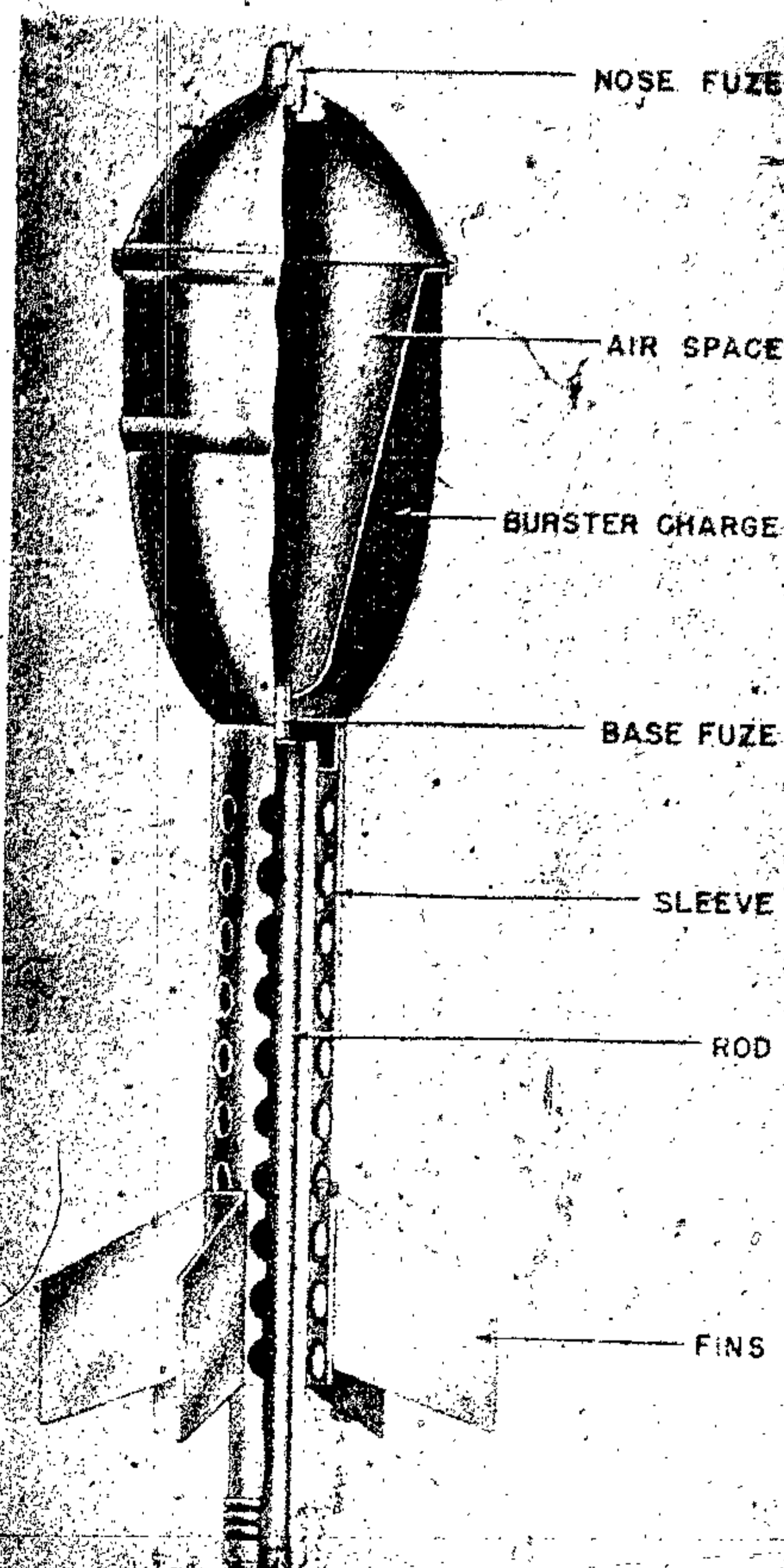
Figure 303—37-mm Hollow Charge Rifle Grenade
