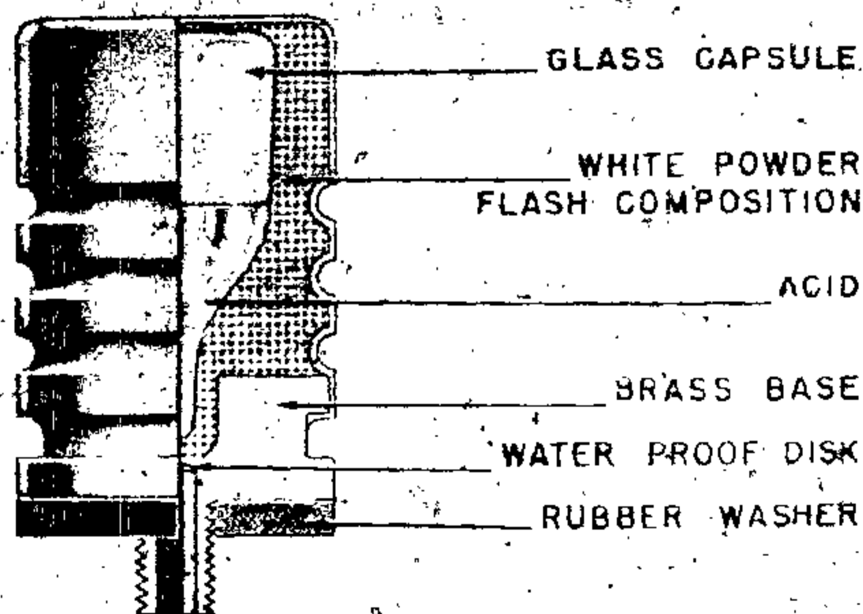
Figure 276—Buck Igniter—Chemical Pressure
