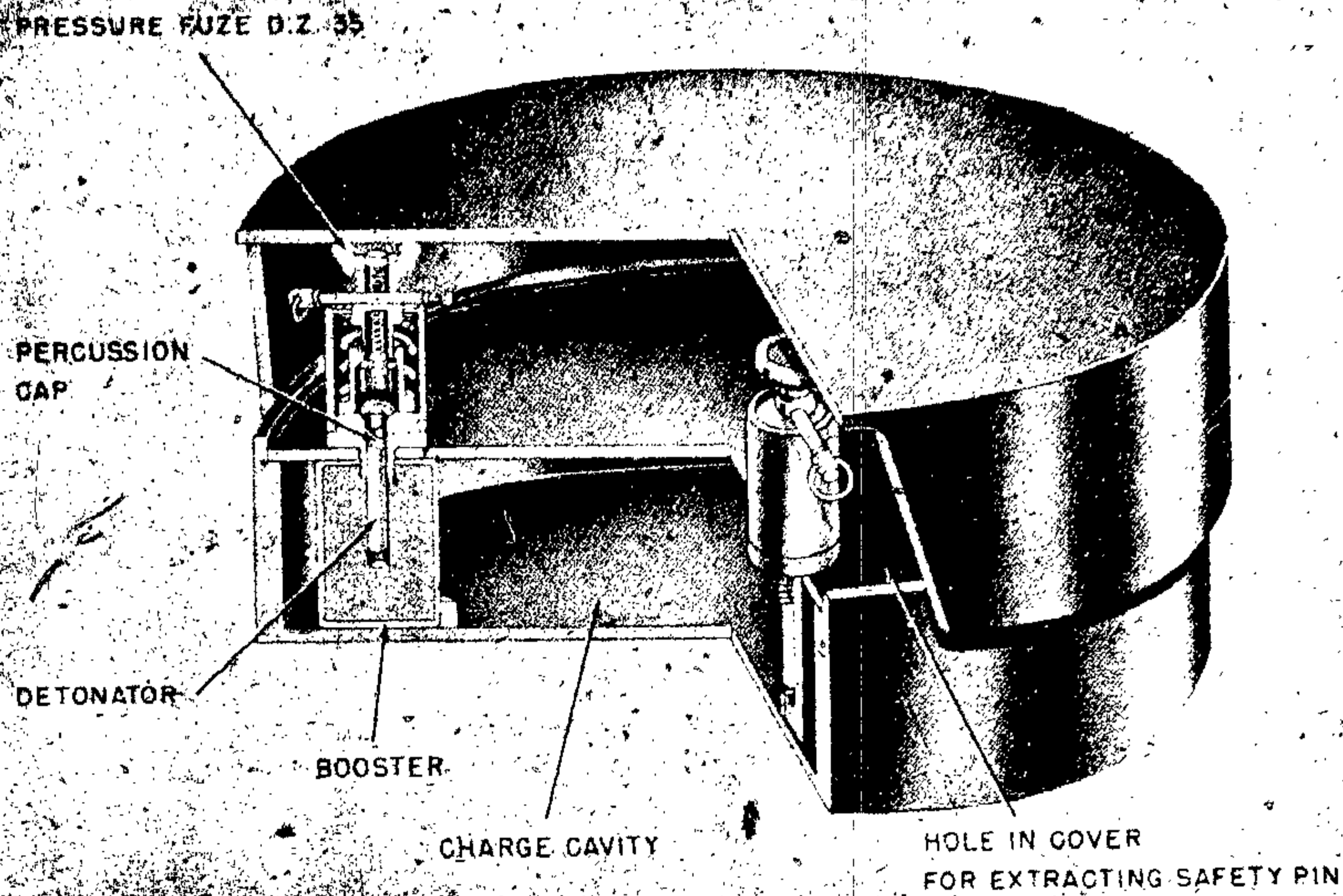
Figure 237—Aluminum Antitank or Antipersonnel Mine
