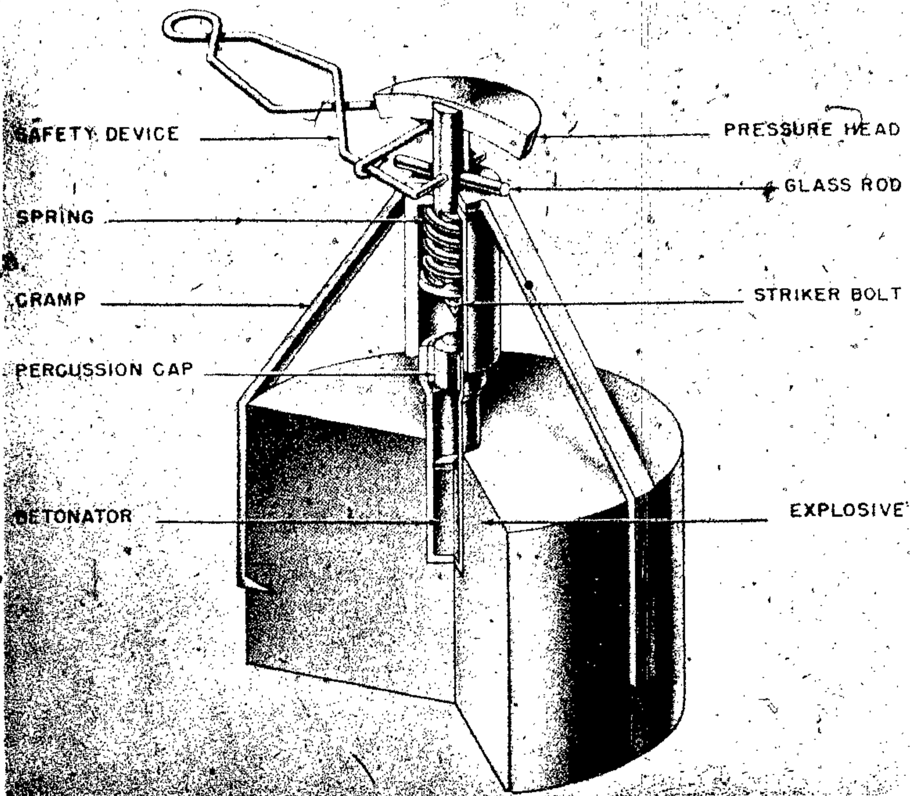
Figure 266—Weissman Pressure Igniter
