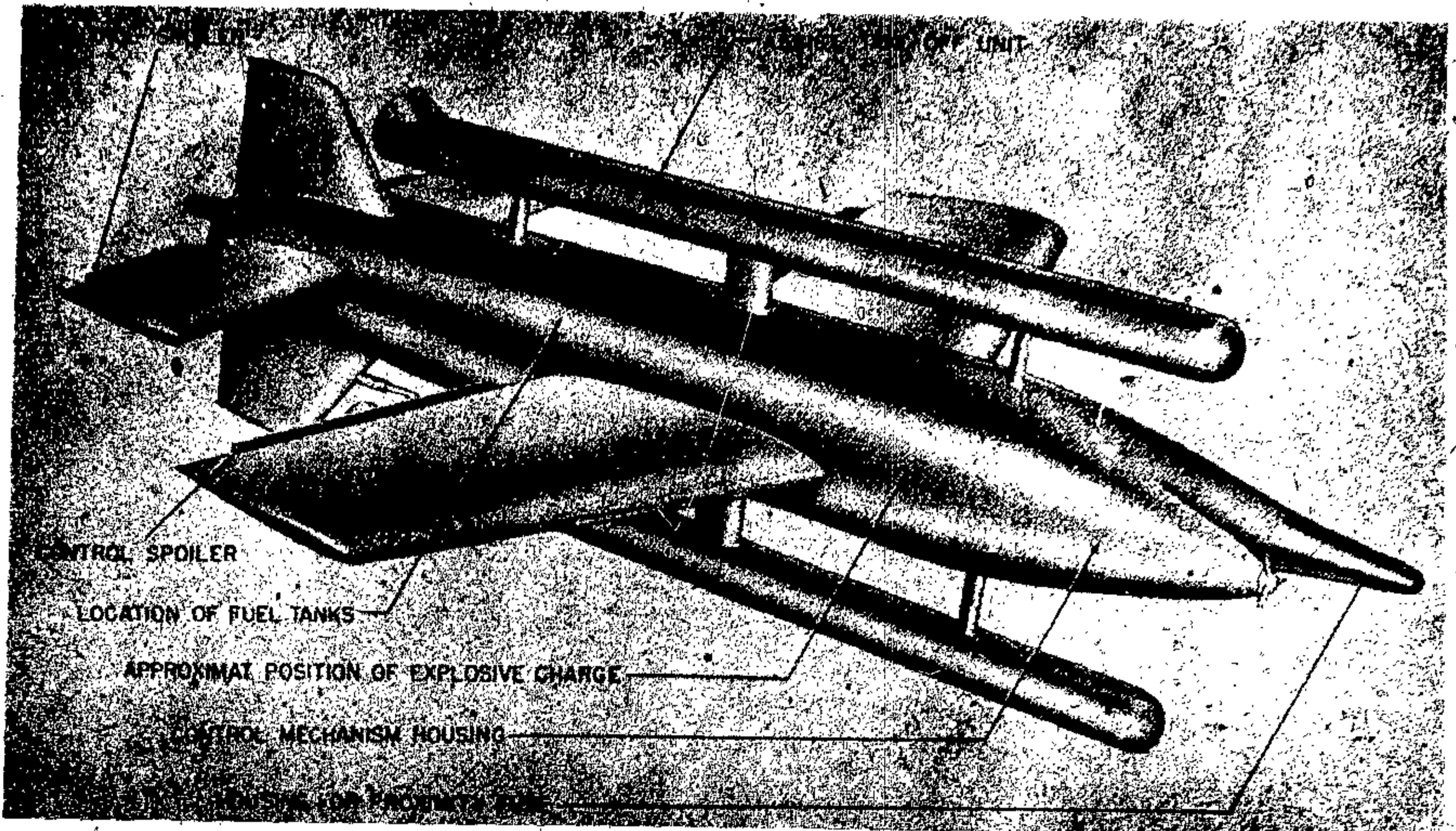
Figure 193—Hs 117 (Hs 297) "Schmetterling"
