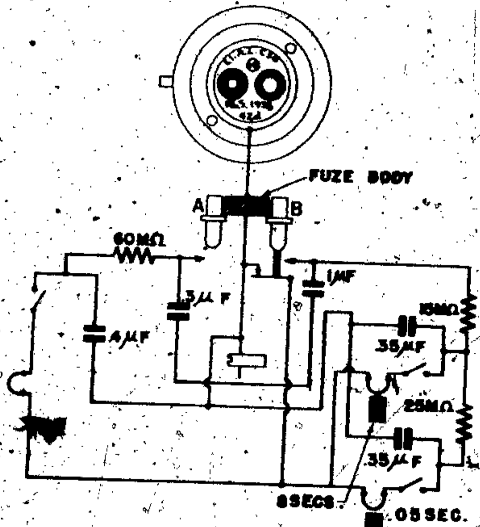
Figure 139—(15) Electrical Impact Fuze
