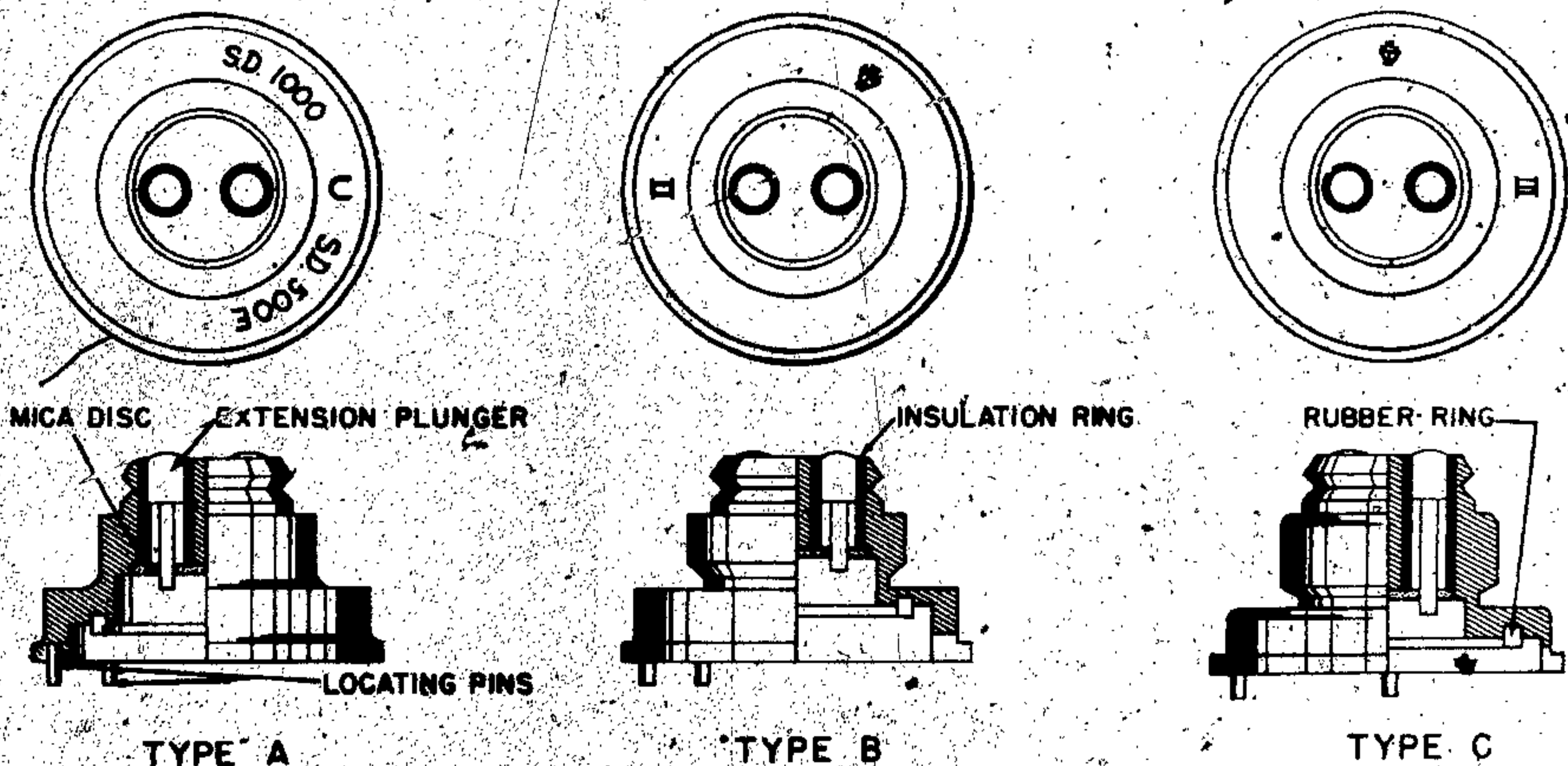
Figure 126—Extension Caps
