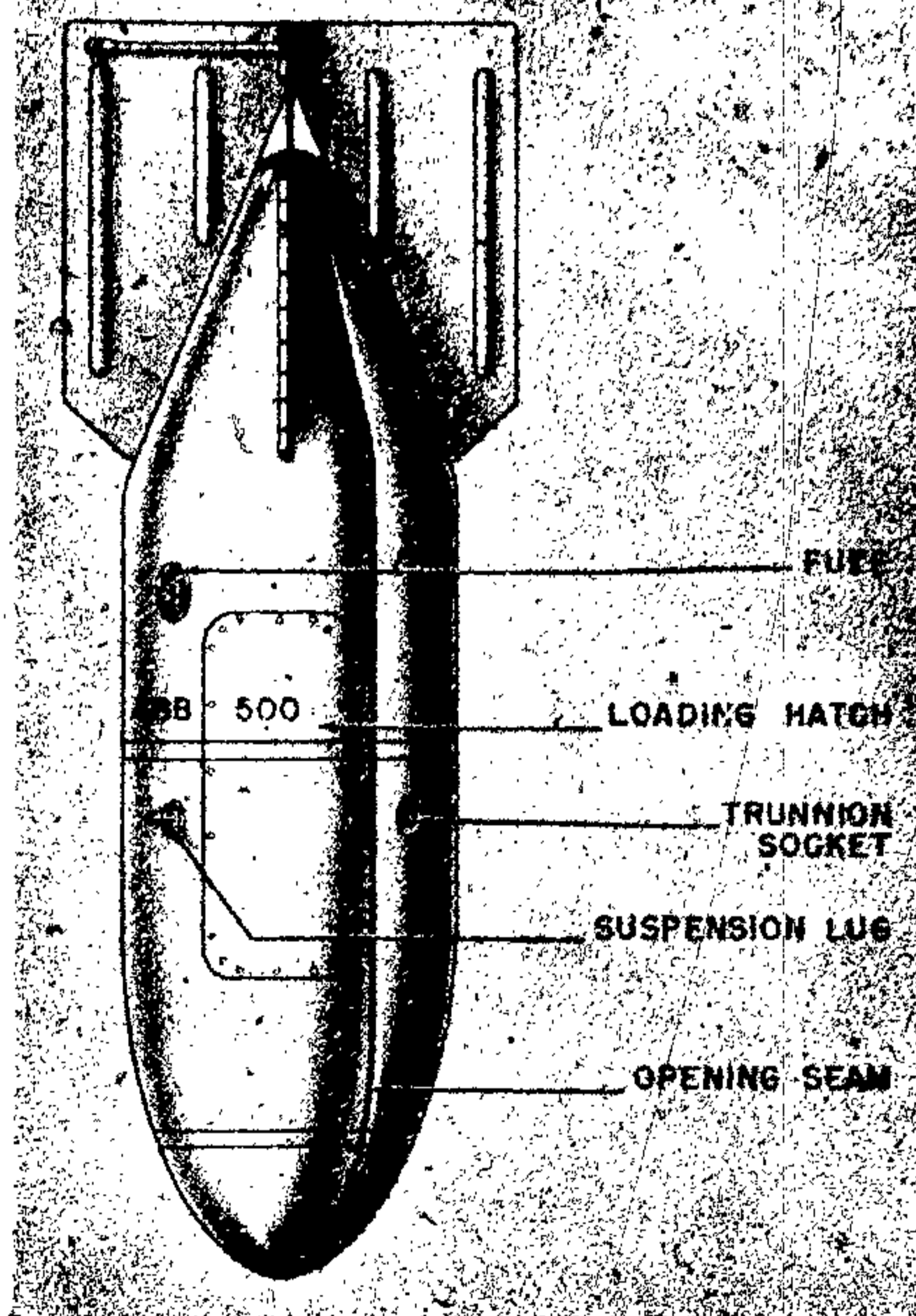
Figure 114—ABB 500 Container.
