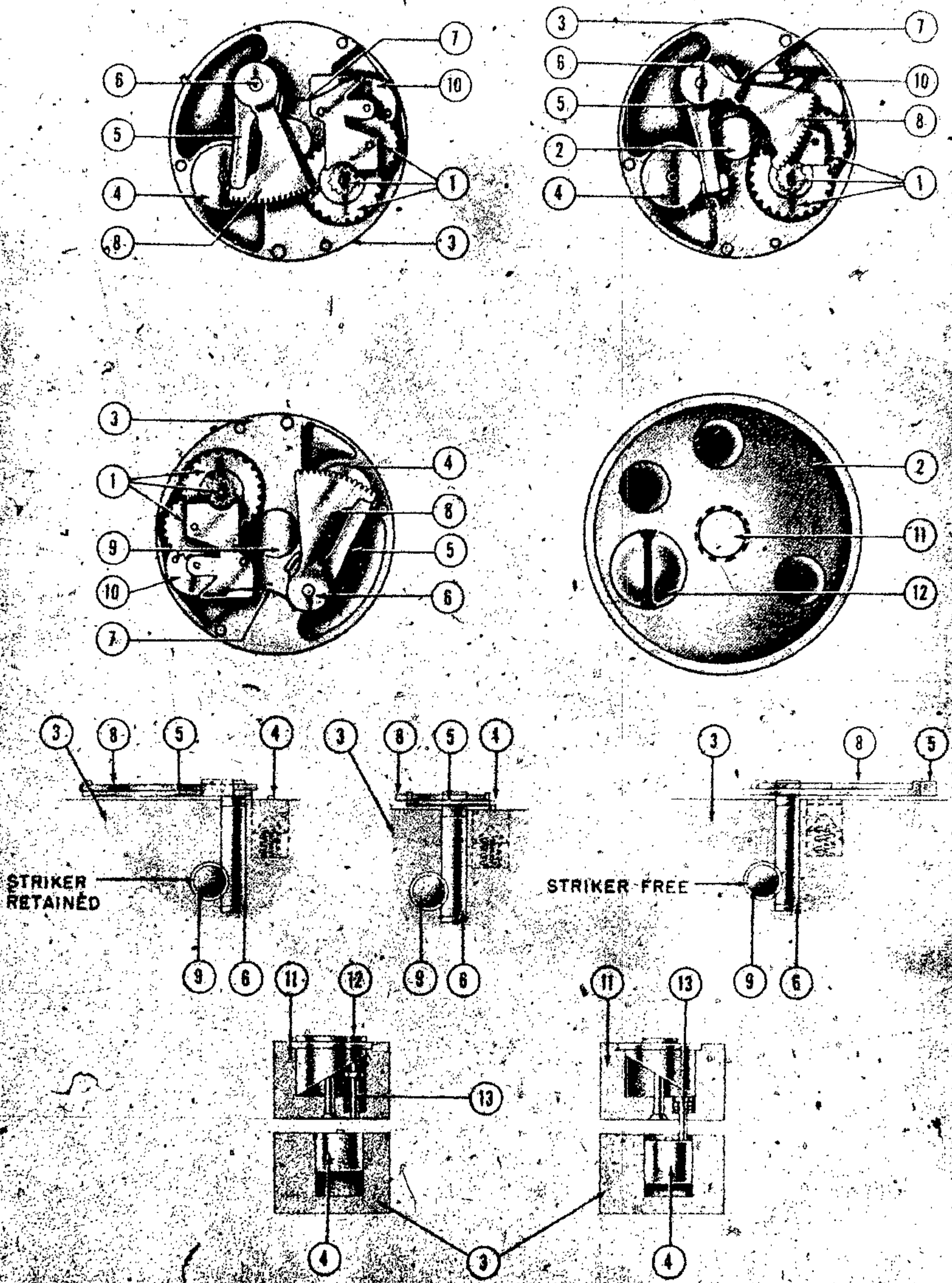
Figure 131—(41) Mechanical Clockwork Fuze
