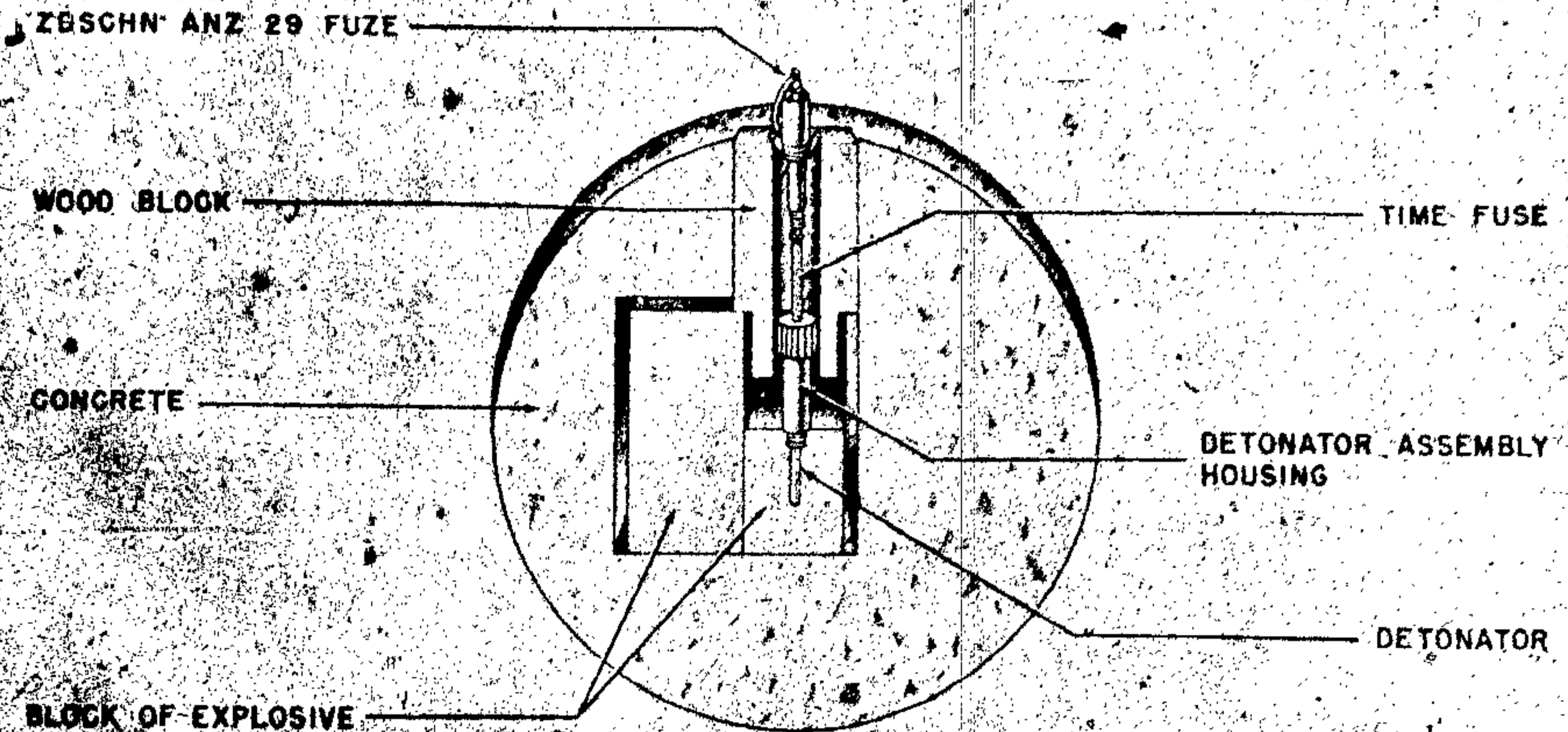
Figure 242—Concrete Ball Mine—Antipersonnel
