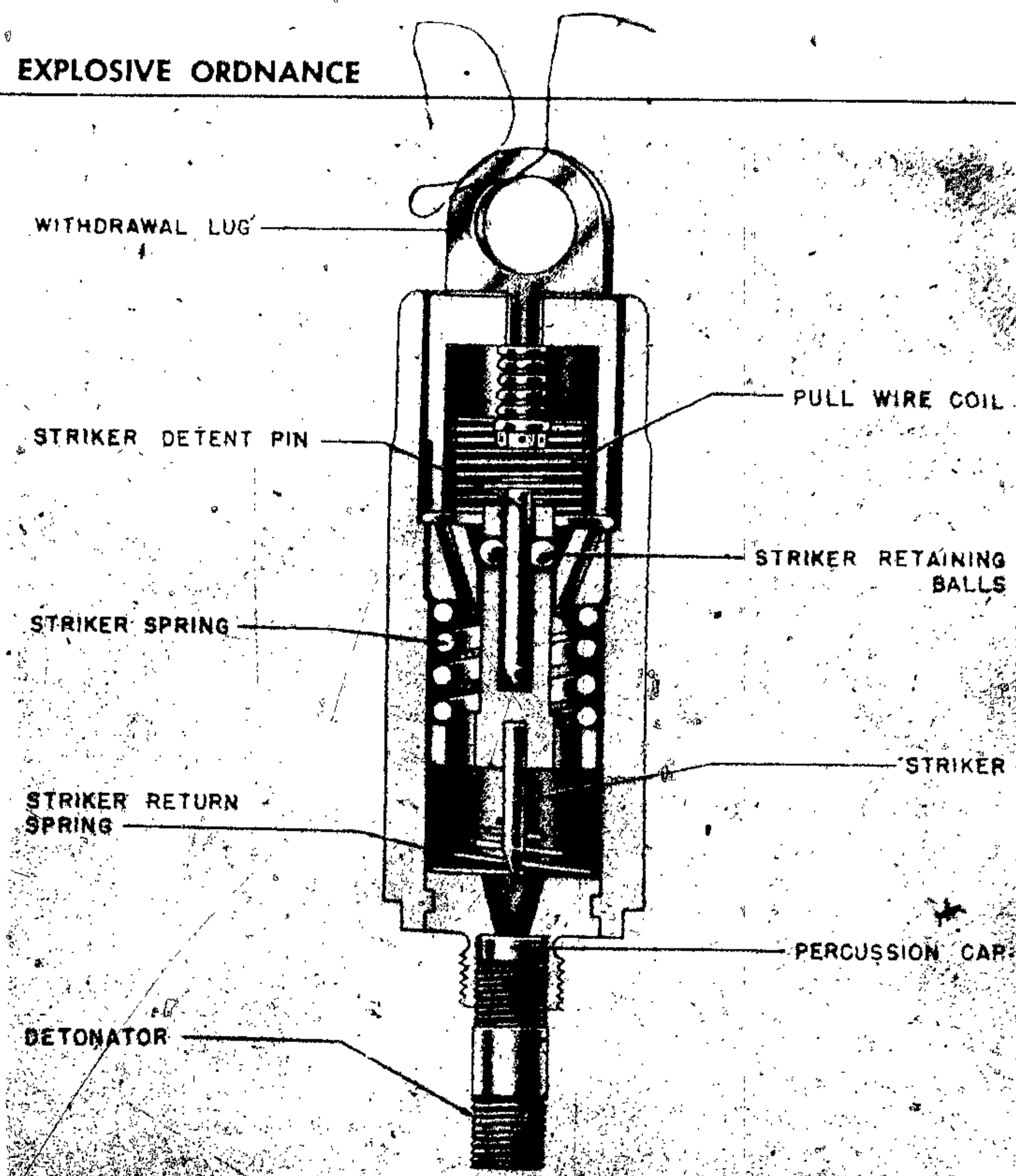
Figure 170—(29) Mechanical Aerial Burst Fuze
