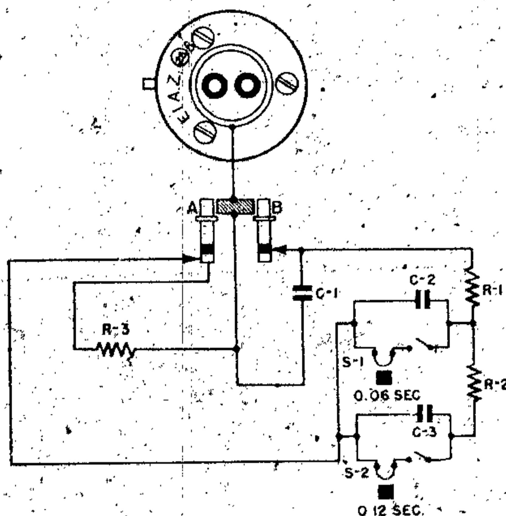
Figure 161—(28)B Electrical Impact Fuze
