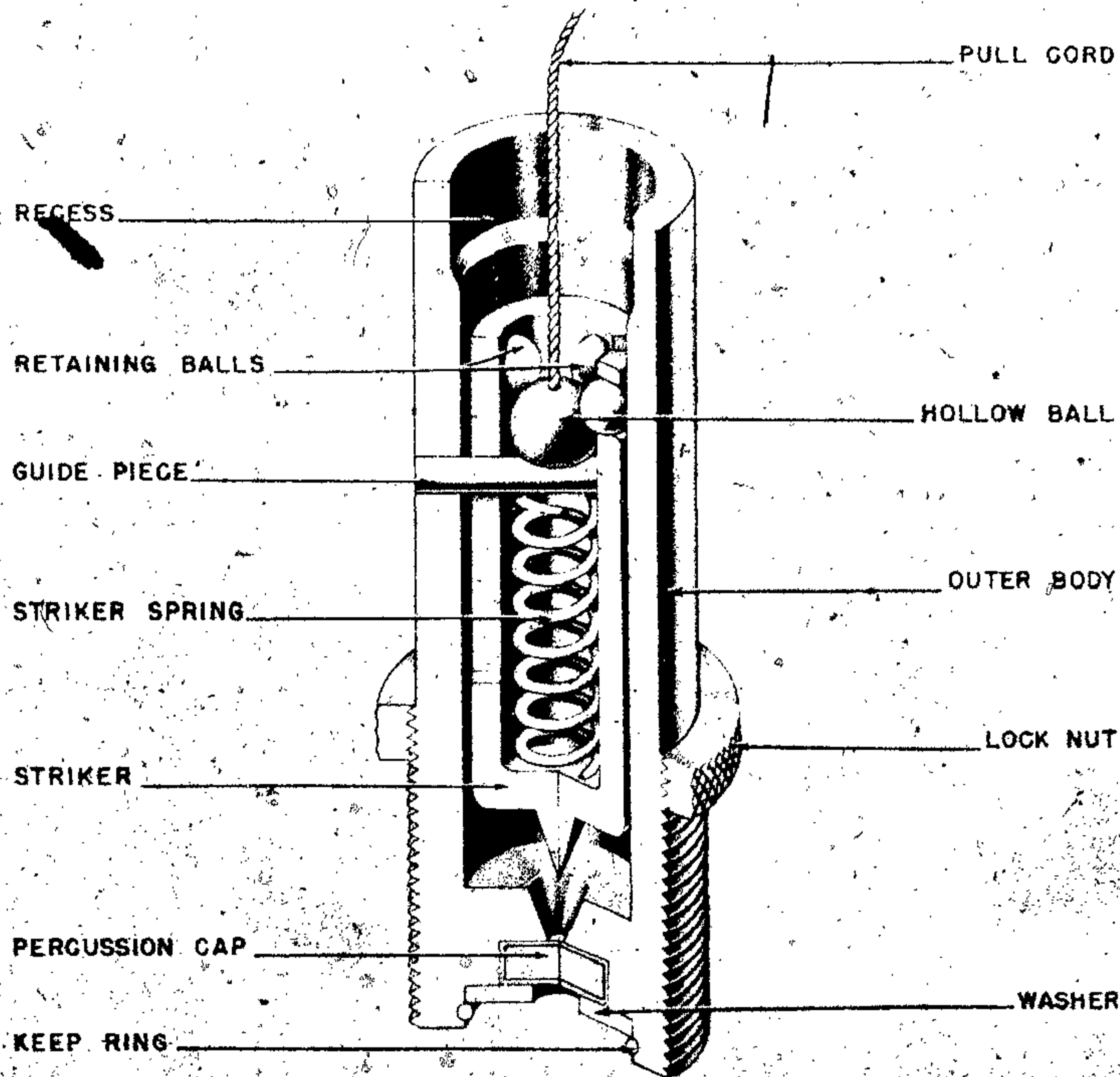
Figure 257—Type 31 Pull Igniter
