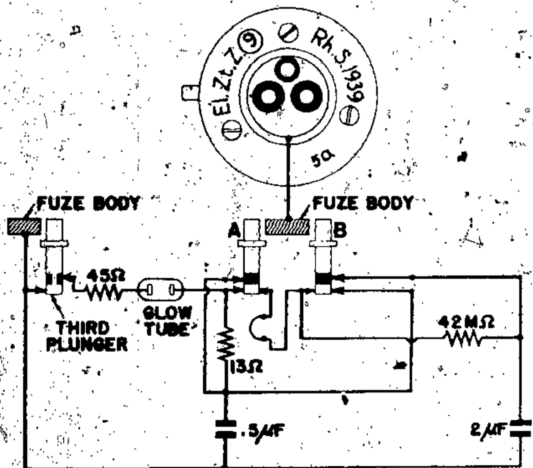
Figure 169—(9) Electrical Aerial Burst Fuze
