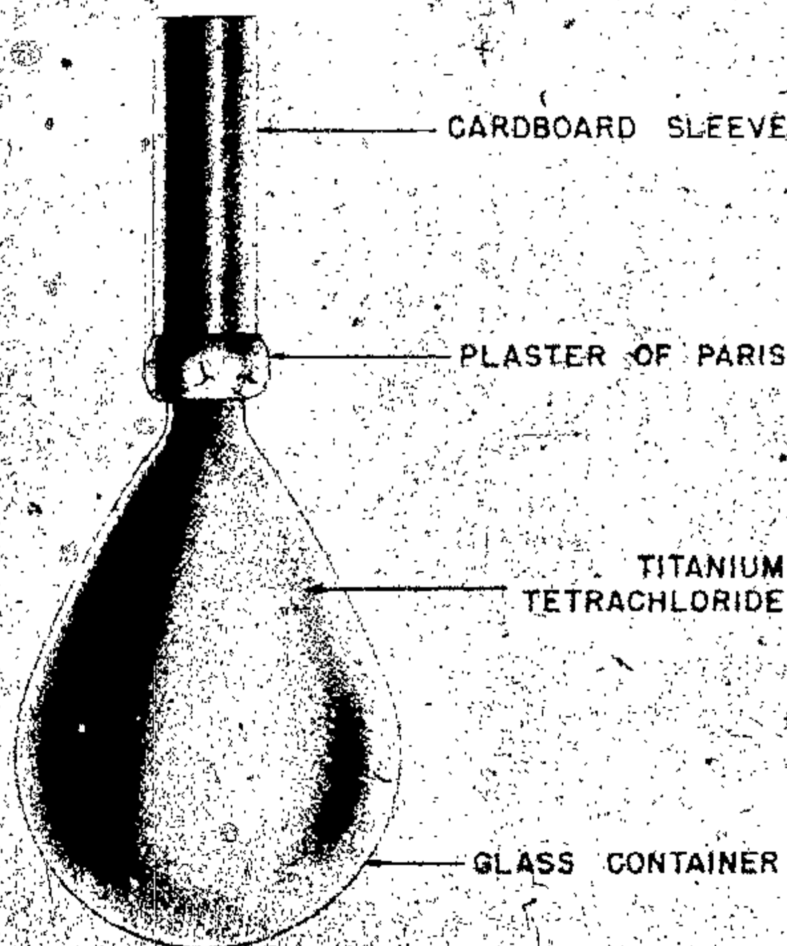
Figure 293—Blendkorpor 14 Smoke Hand Grenade
