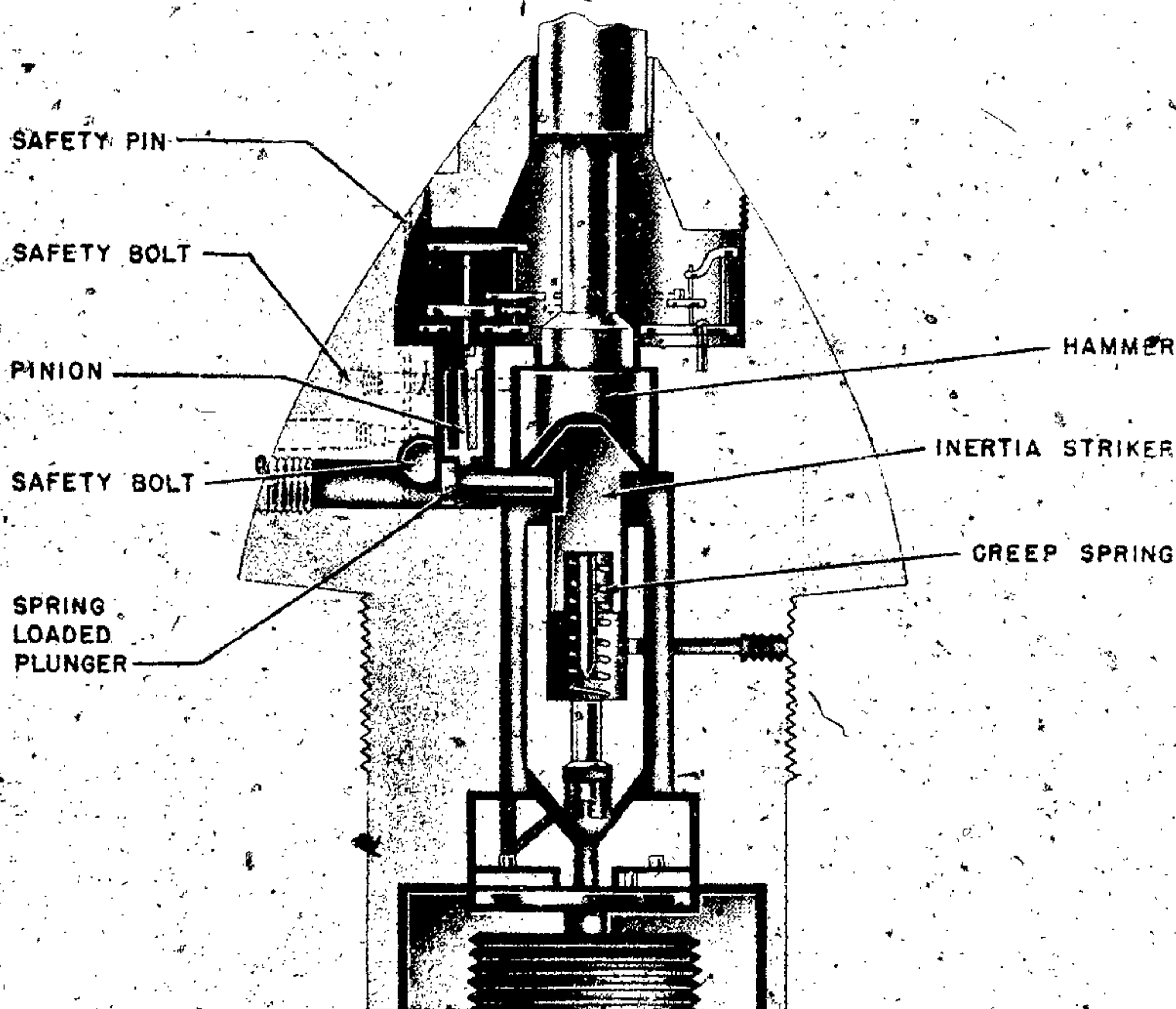
Figure 133—(3) Mechanical Nose Impact Fuze
