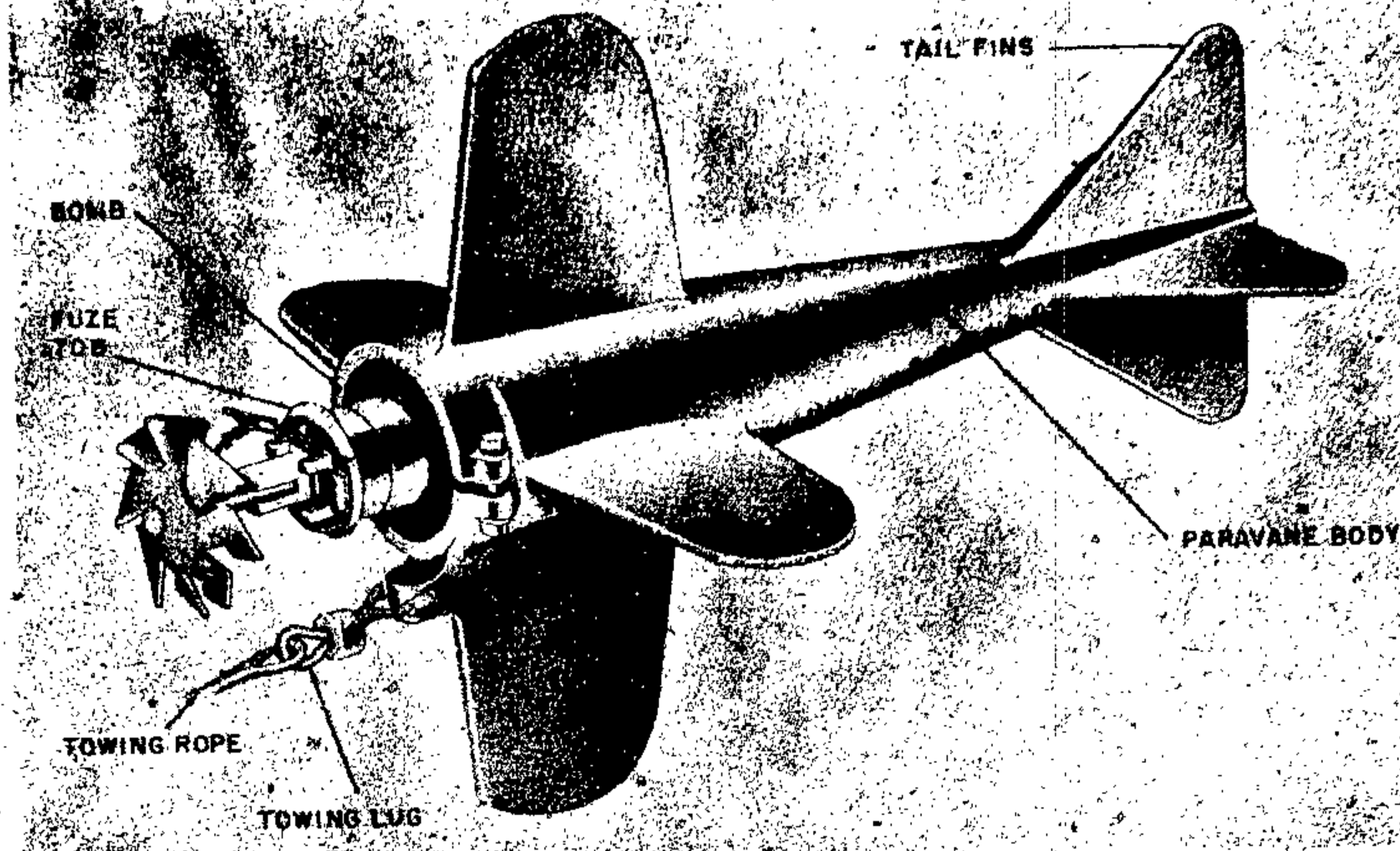
Figure 50—2-Kg Airplane Towed Paravane Bomb
