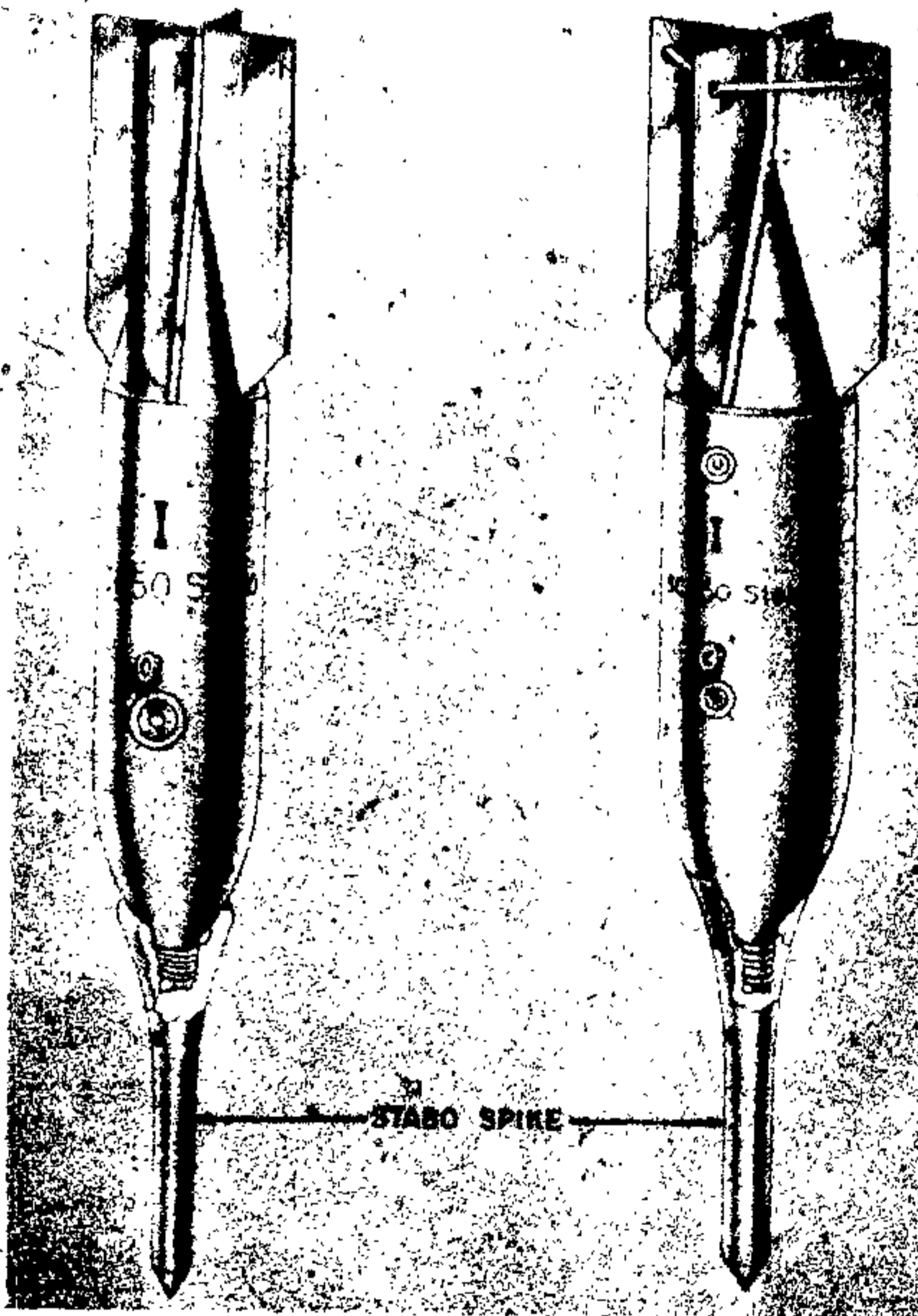
Figure 26—Nose Spikes for Stabo Bombs
