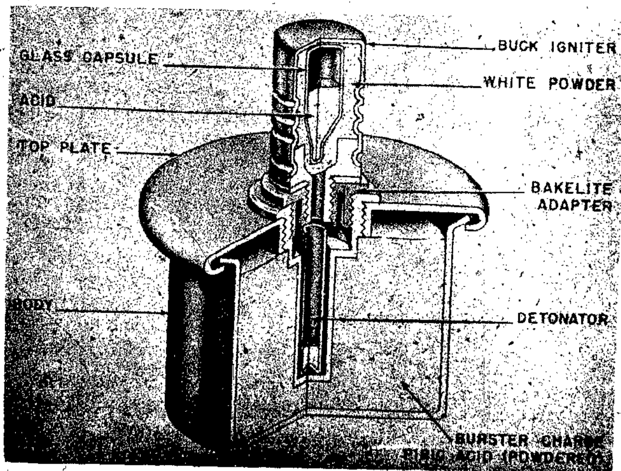
Figure 248—Mustard Pot Mine—Antipersonnel
