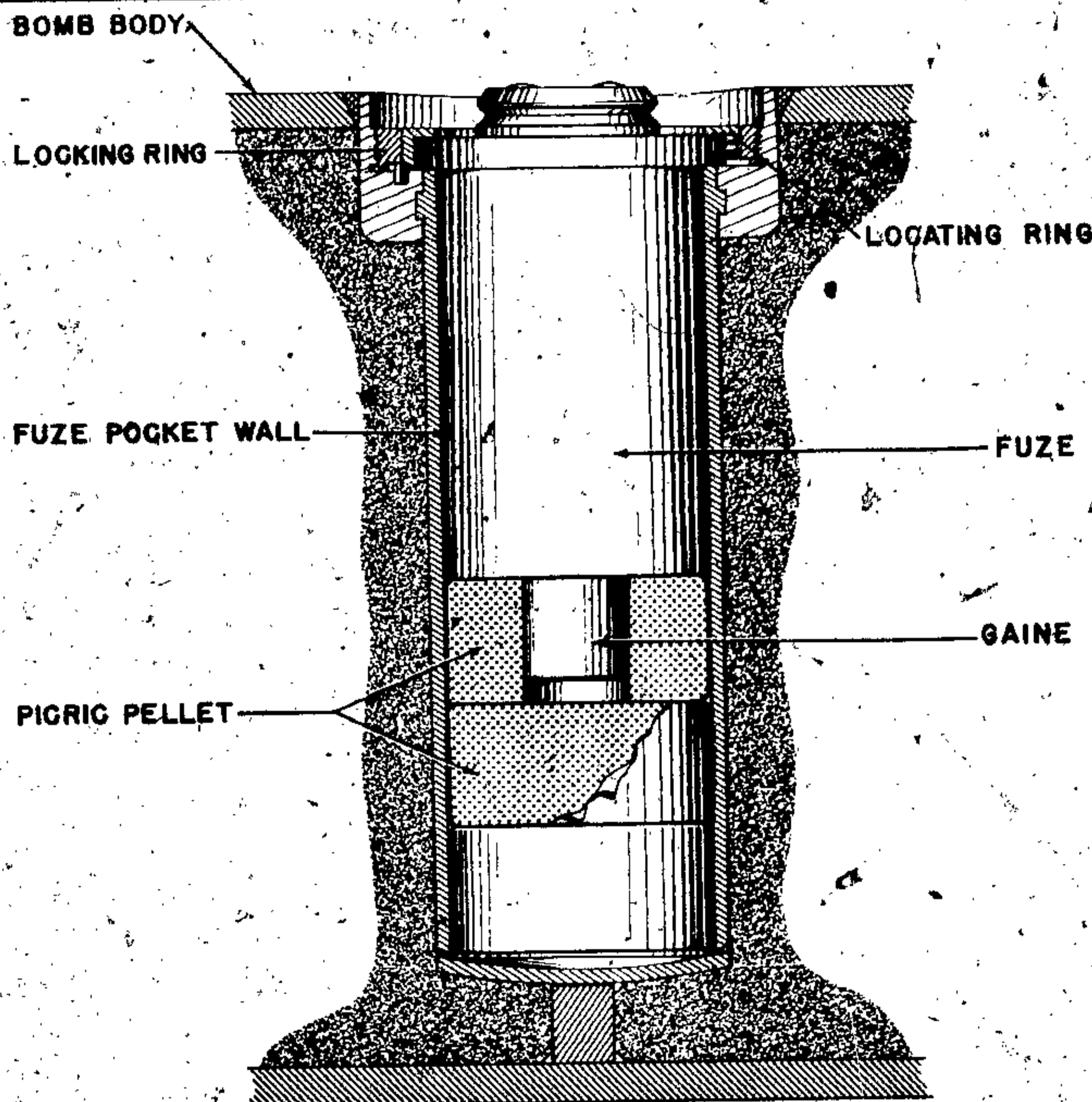
Figure 3—Fuze Pocket In Bomb
