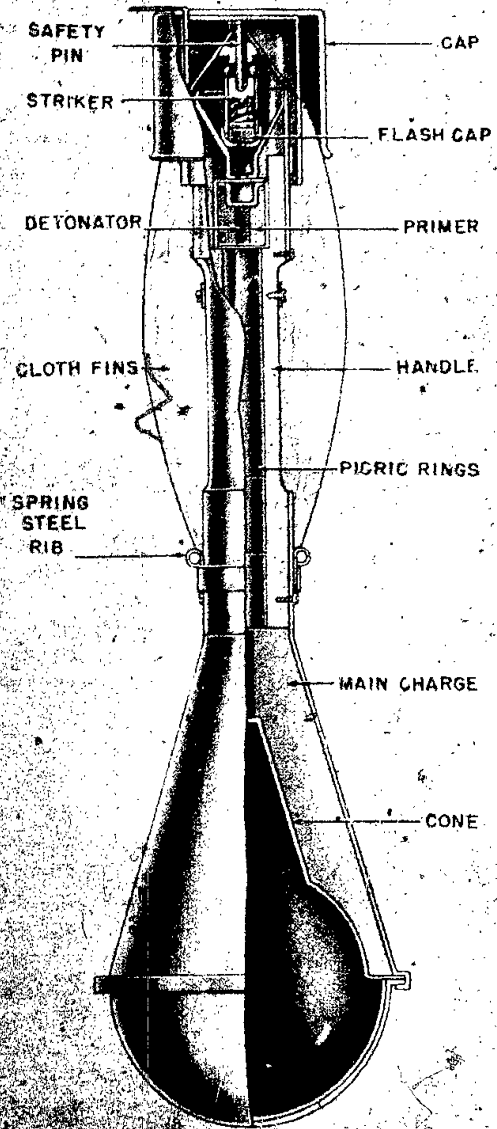
Figure 290—Panzerwurfmine Hollow Charge Hand Grenade
