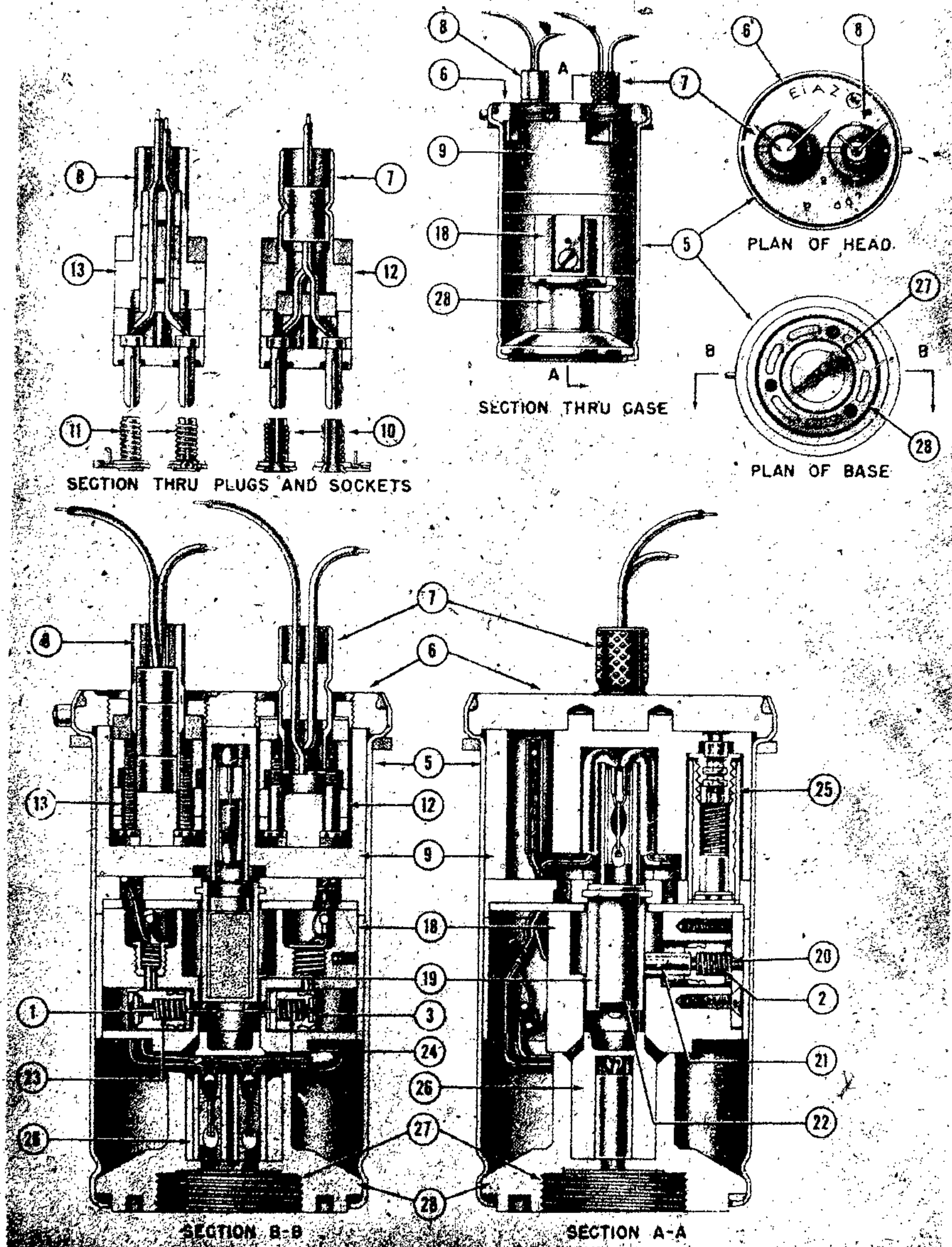
Figure 151A—(106)* Electrical Impact Fuze
