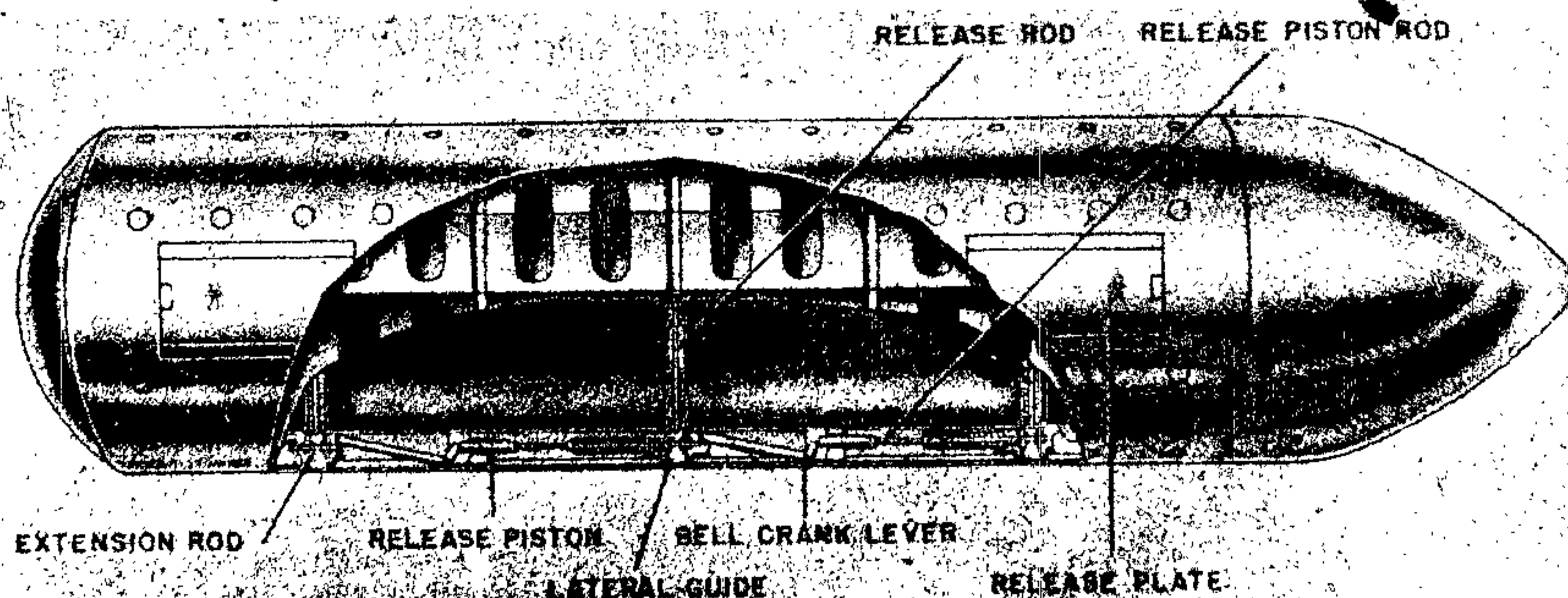
Figure 105—AB 250-1 Container
