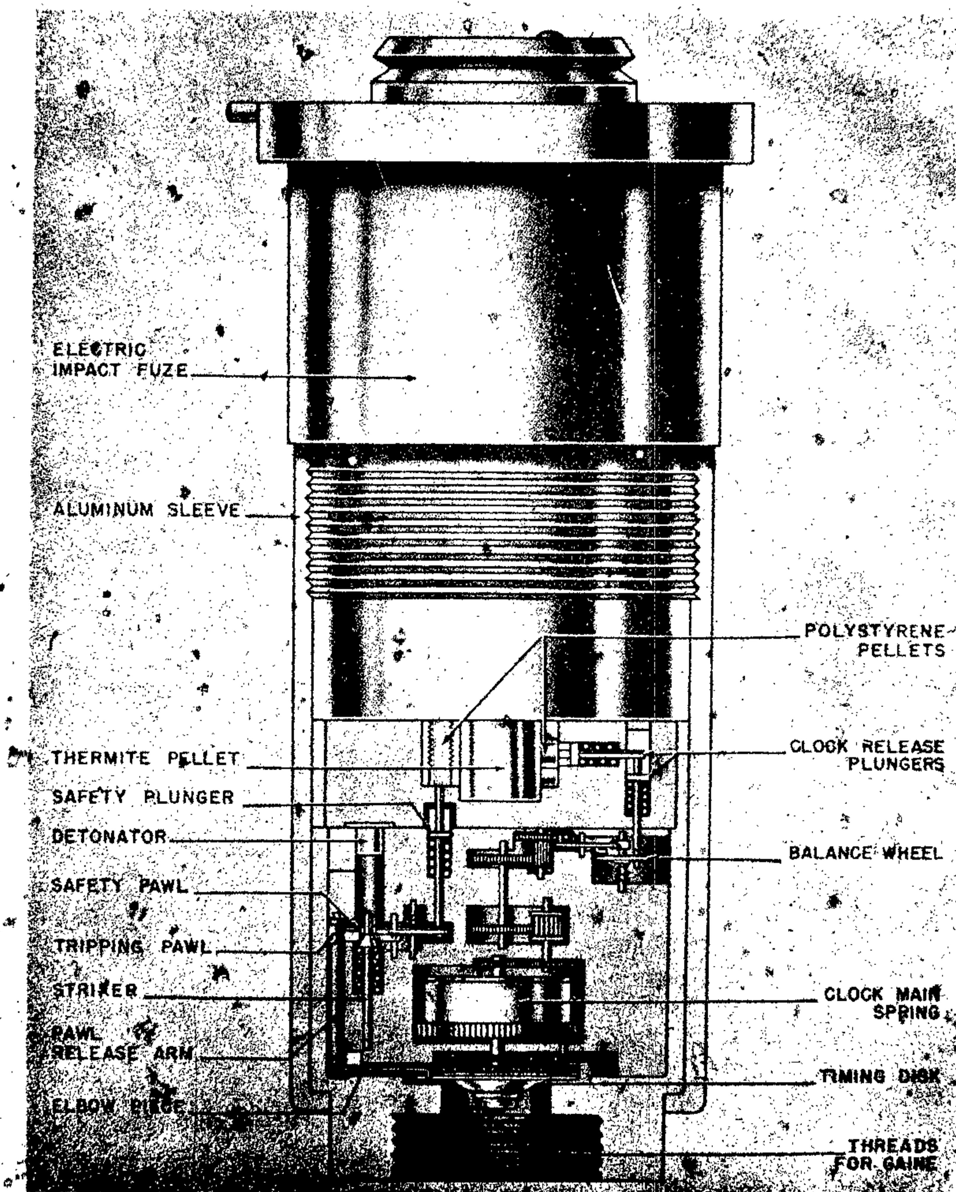
Figure 153A—(17)A Electrical Clockwork Time Fuze
