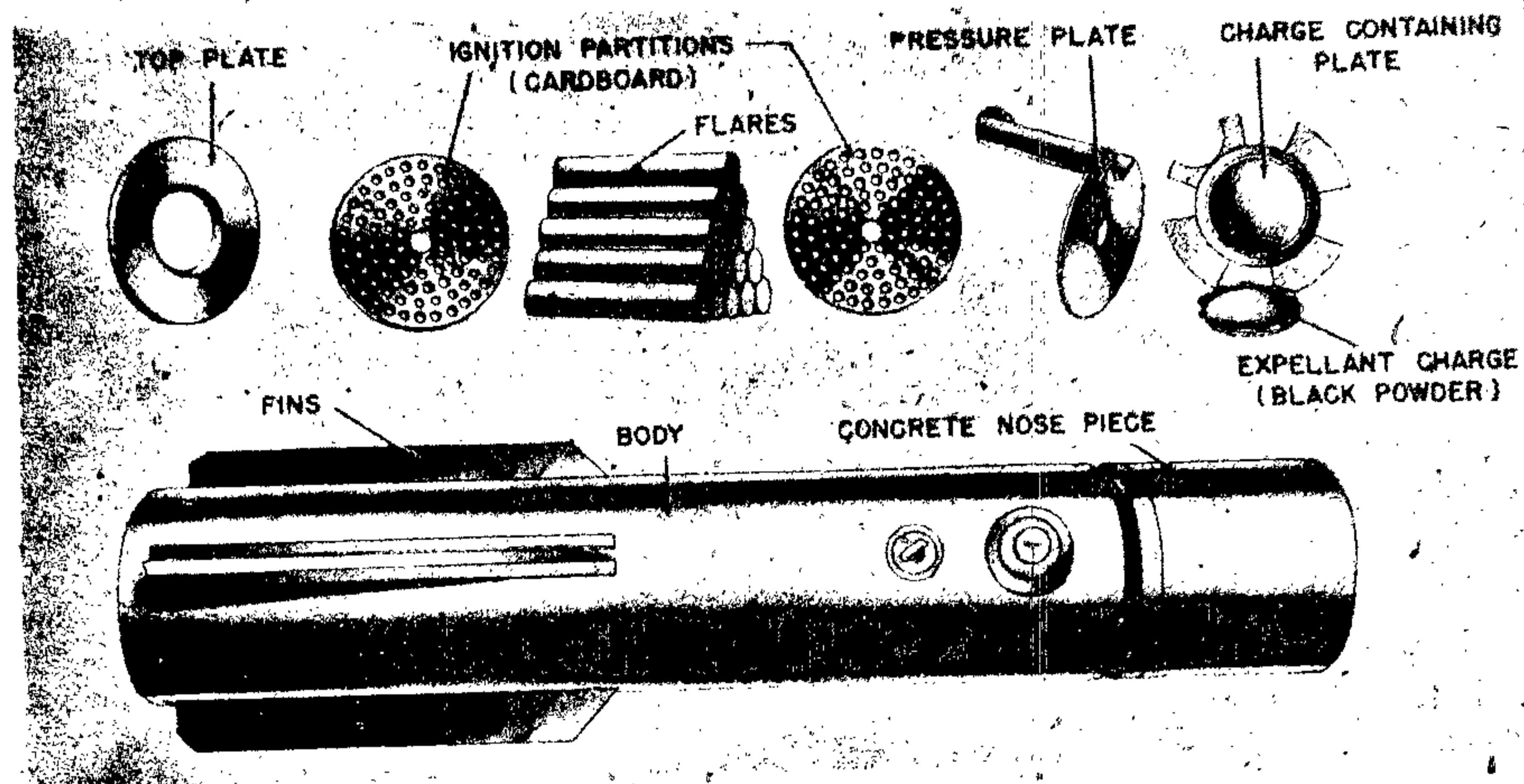
Figure 76—Mark 50 Kask Target Identification Flare
