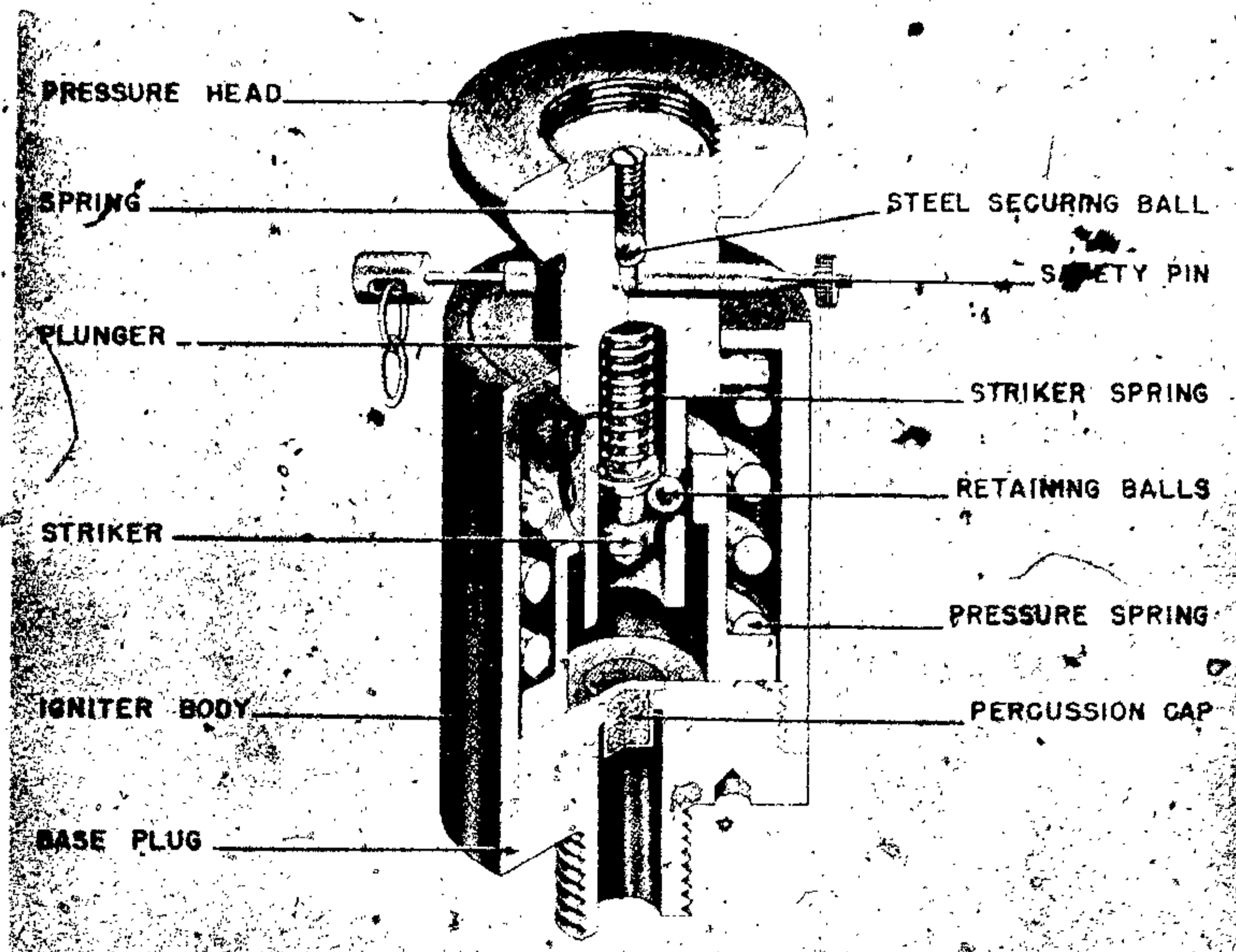
Figure 262—D. Z. 35 (A) Pressure Igniter
