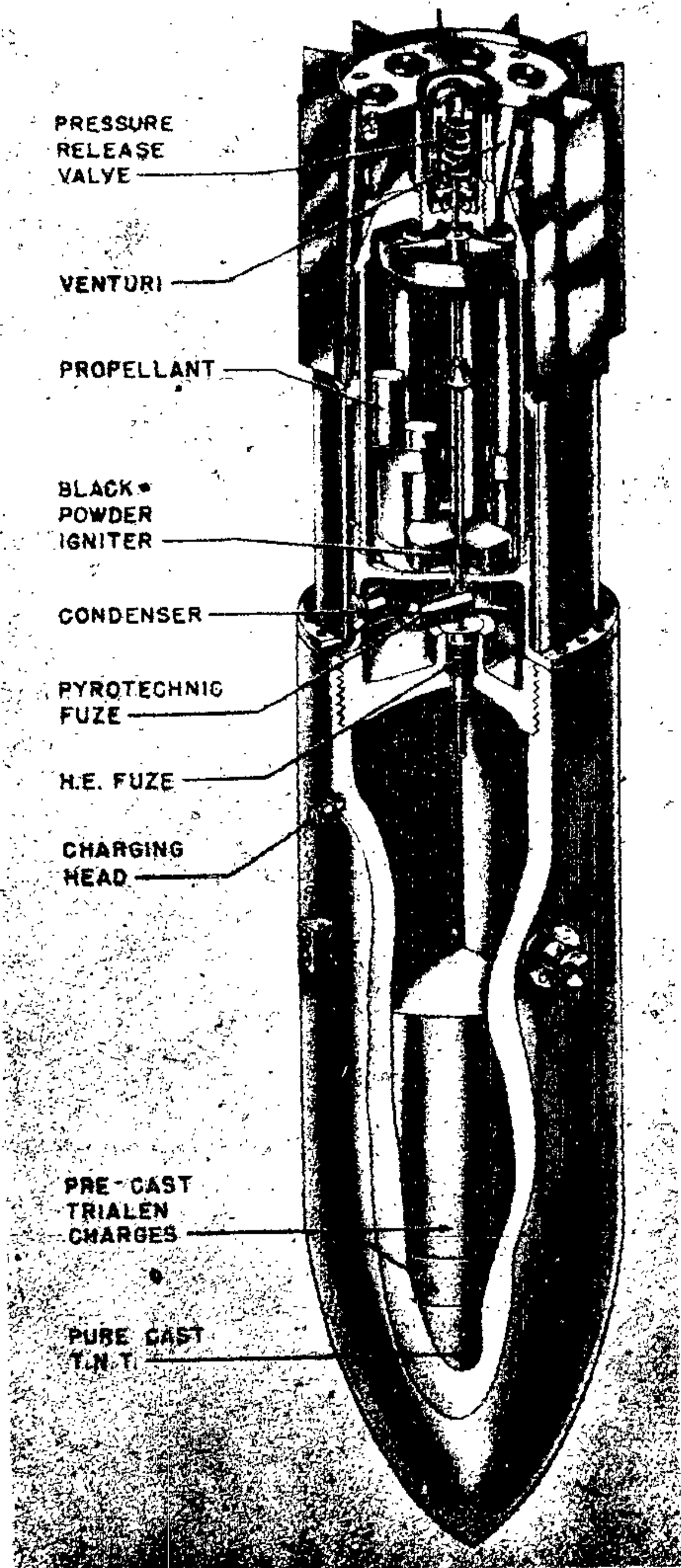
Figure 35—PC 1800 RS Bomb
