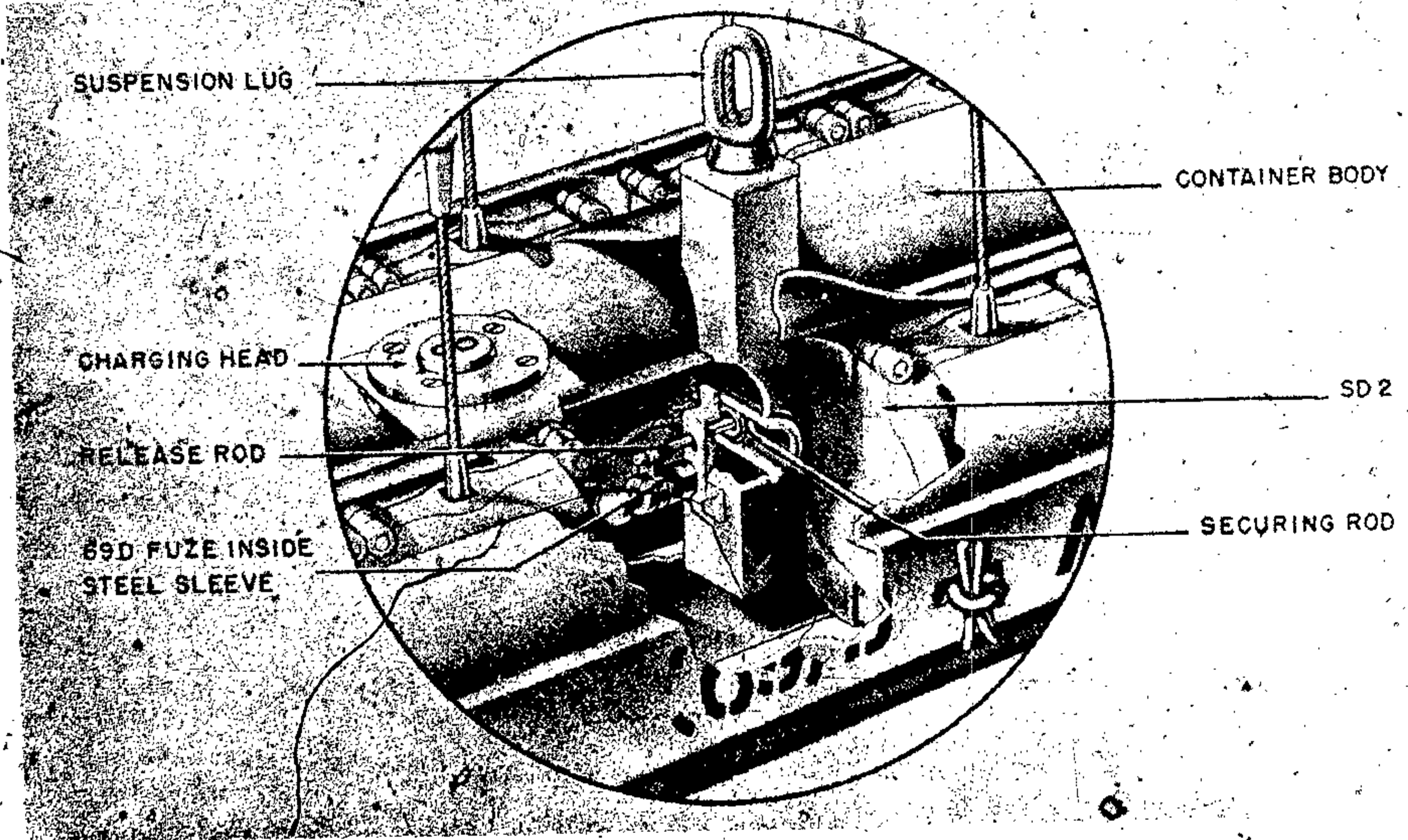
Figure 103B—AB 70-3 Container
