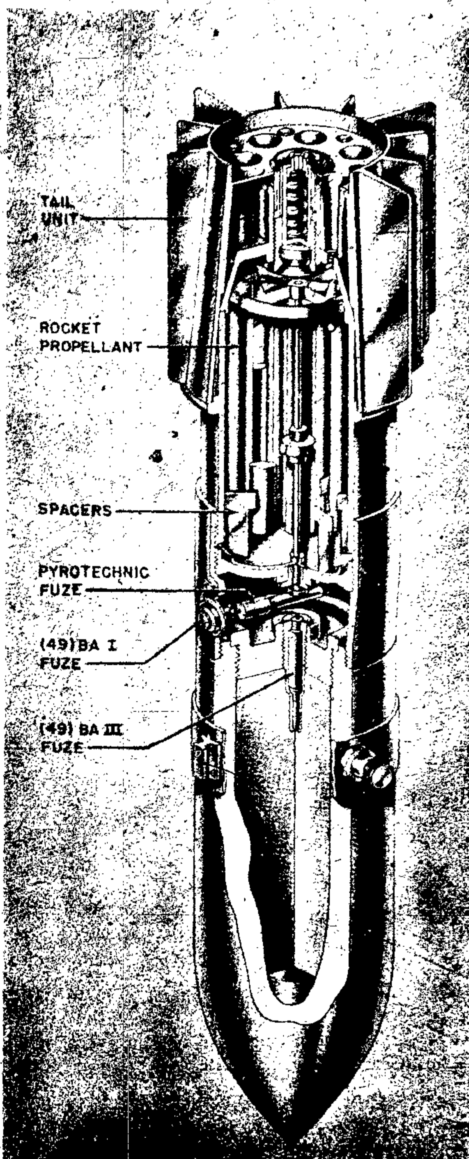
Figure 34—PC 1000 RS Bomb
