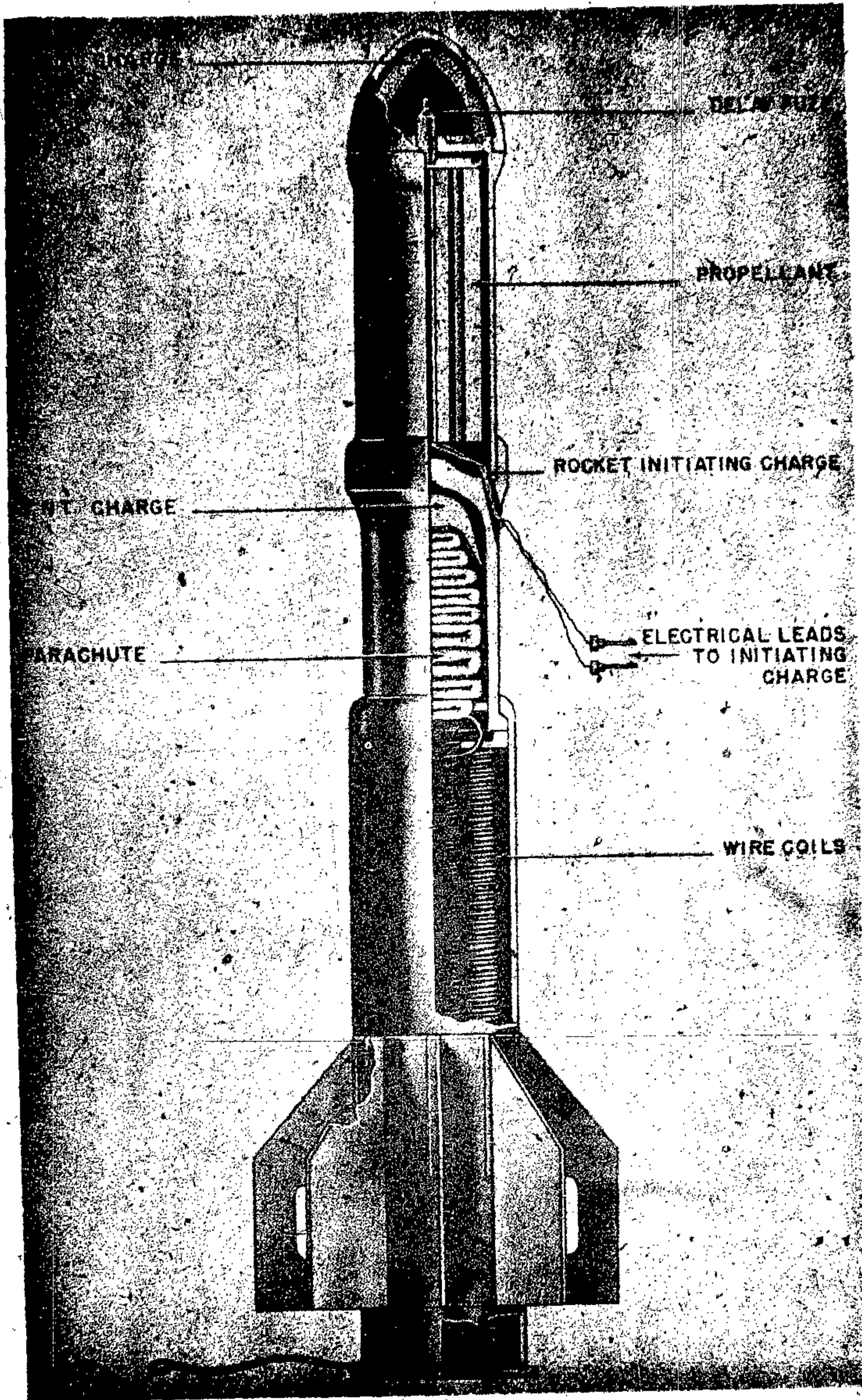
Figure 213—15.2-cm Antiaircraft Rocket
