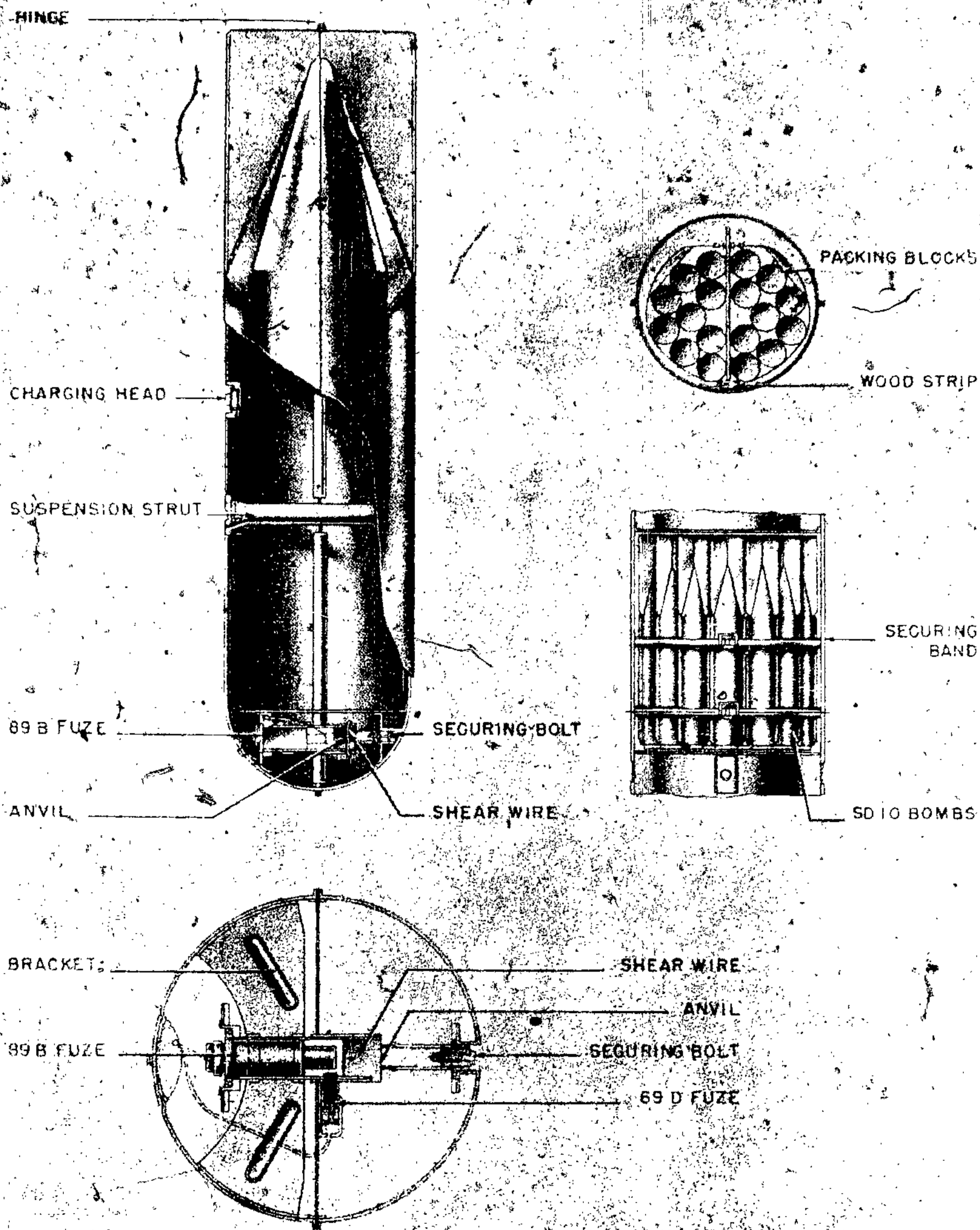
Figure 111—AB 500-1 Container
