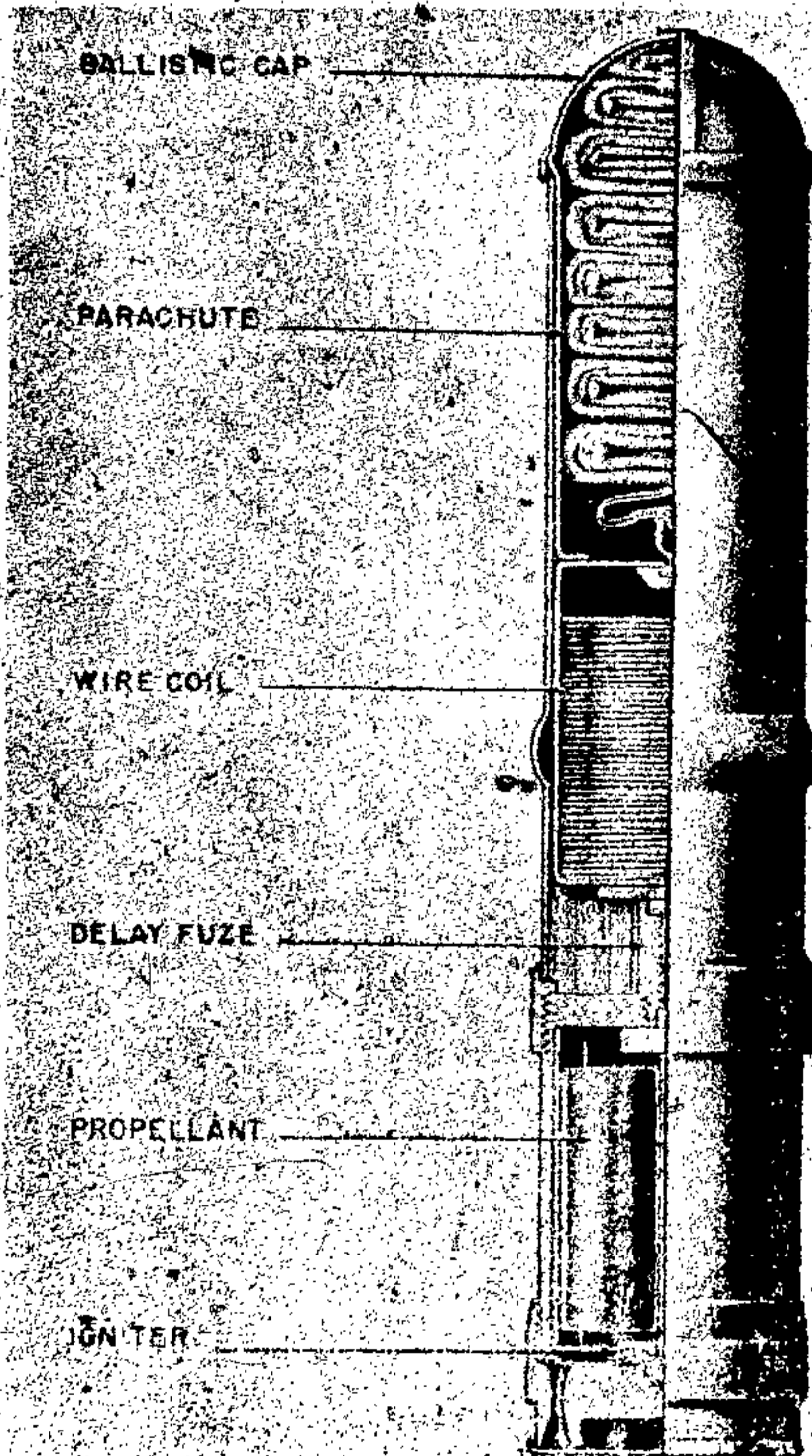
Figure 208—8.6-cm Illuminating Rocket (Naval)
