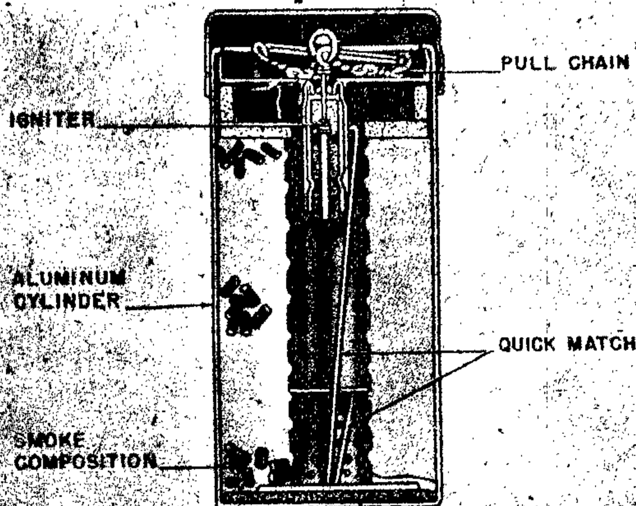
Figure 82—Smoke Flare, Orange, 80
