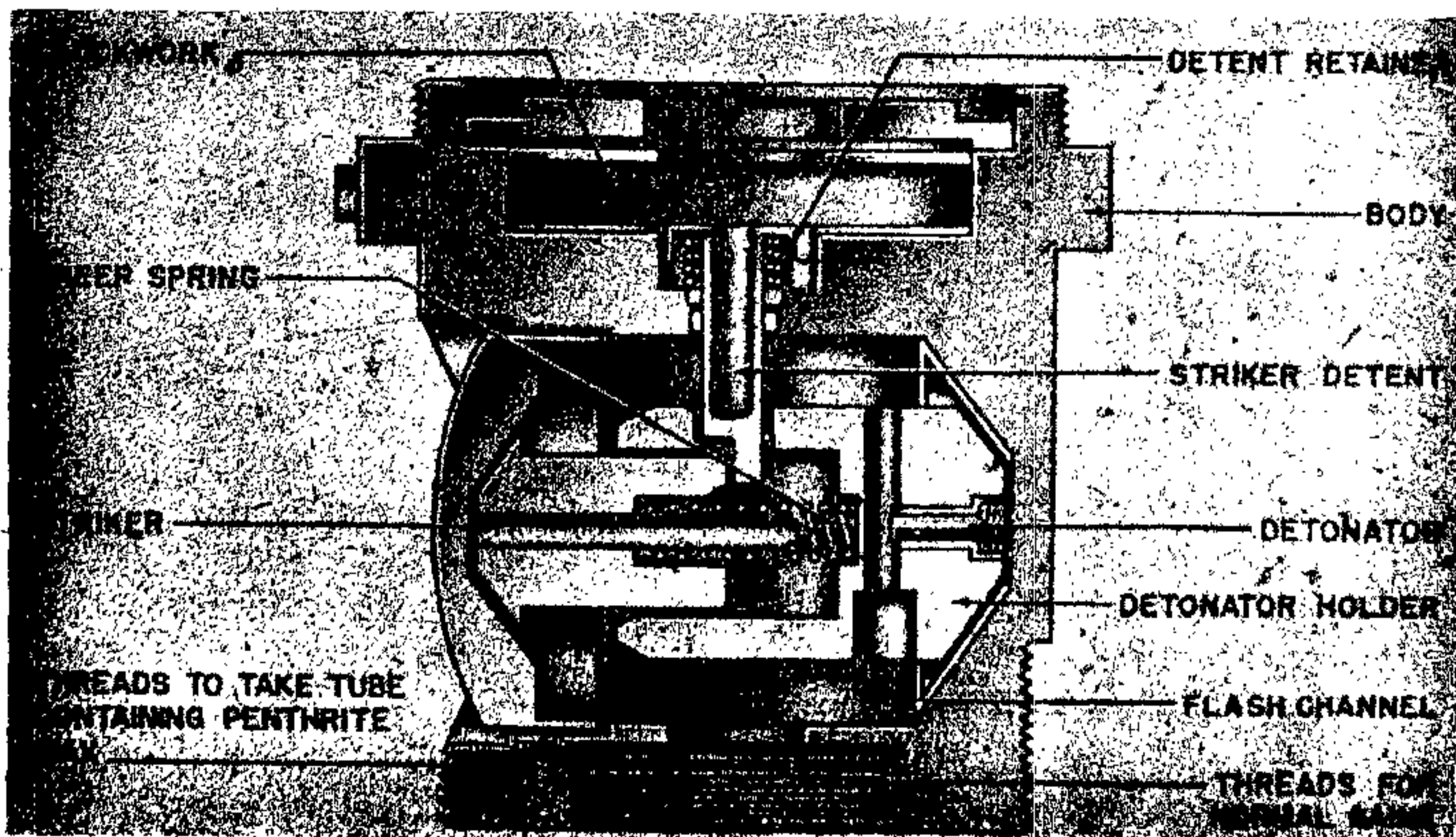
Figure 190—VZ (80) Mechanical All-Ways Action Fuze
