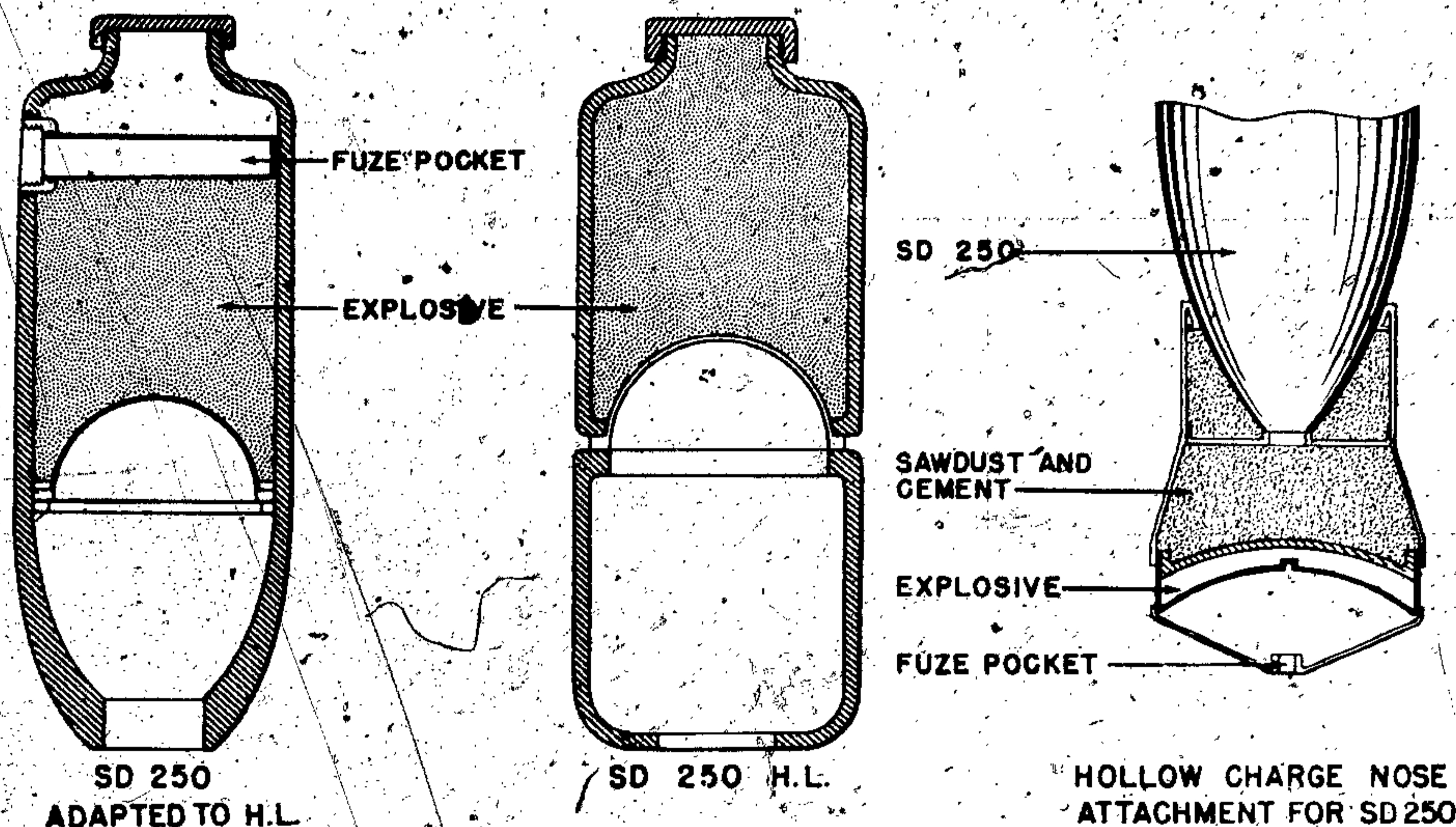
Figure 8—SD and H.L. Hollow Charge Bombs
