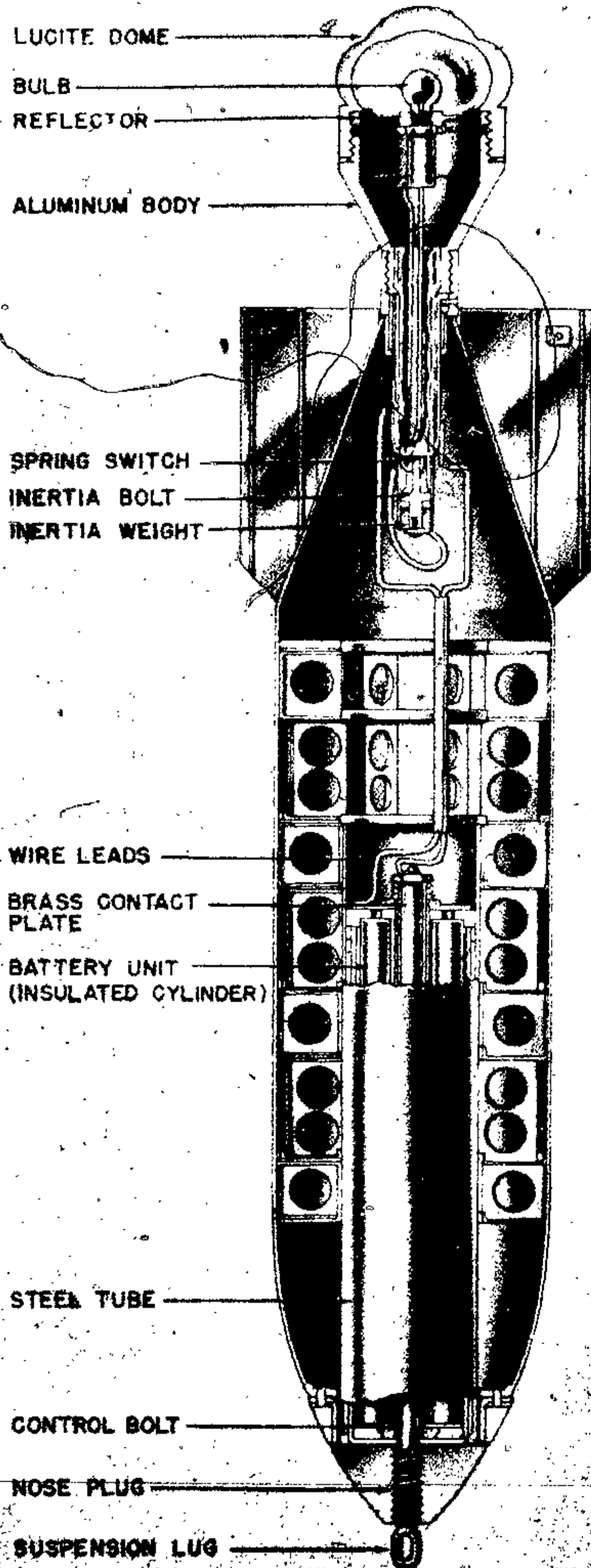
Figure 89—Sea Marker Bomb
