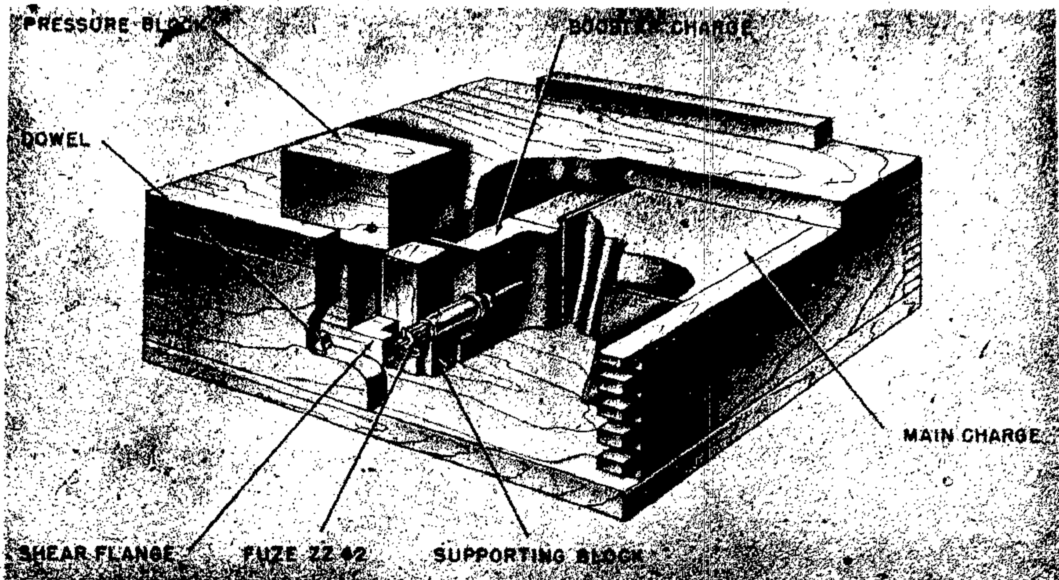
Figure 227—Holzmine 42 Antitank Mine
