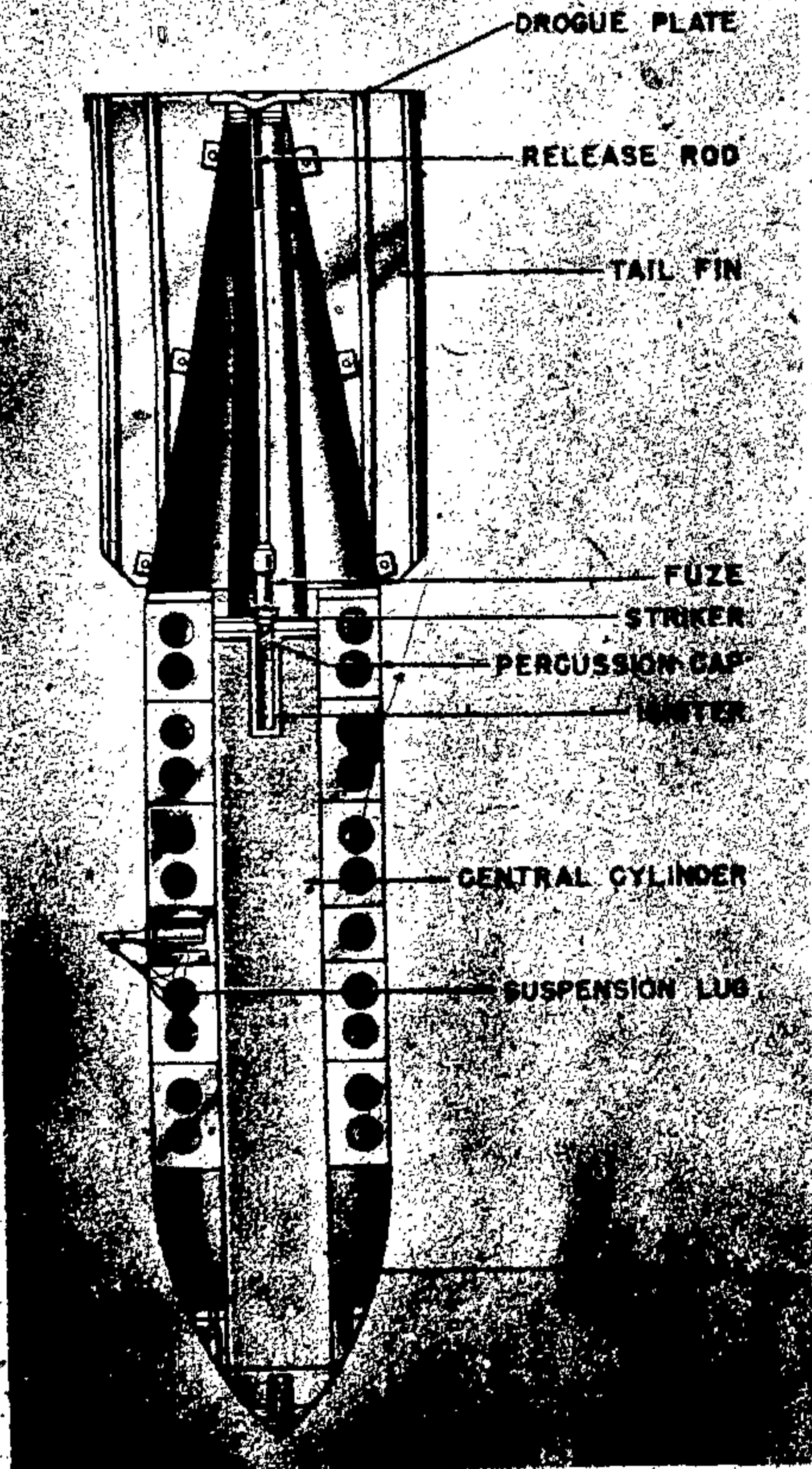
Figure 62—NC 50 W. C. Smoke Bomb
