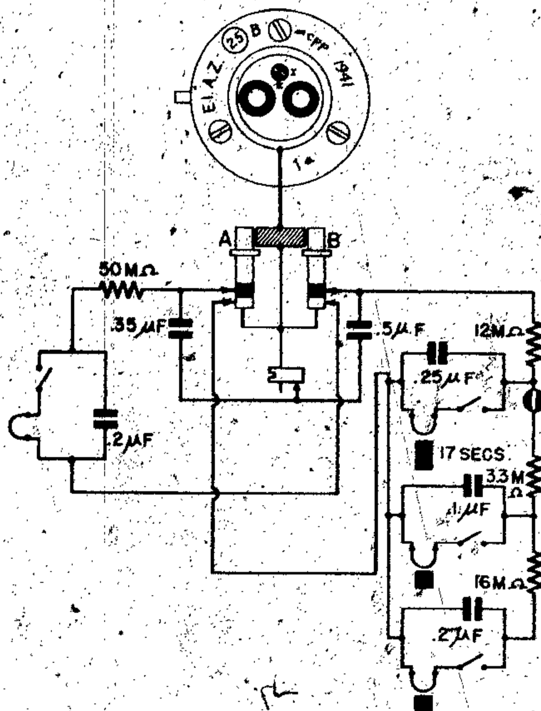
Figure 141—(25)B Electrical Impact Fuze
