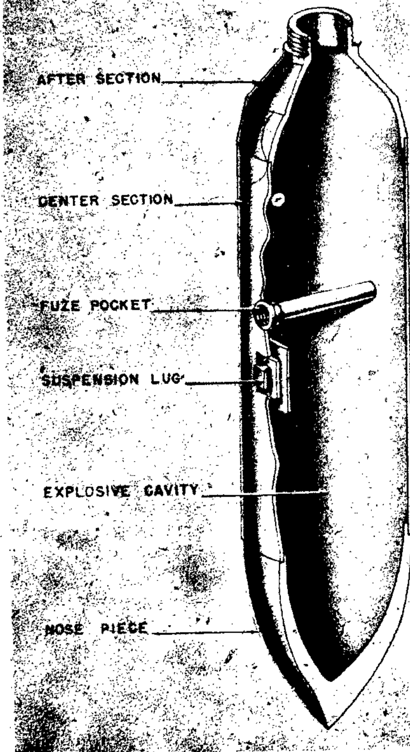
Figure 16—SC 1800-Kg Bomb
