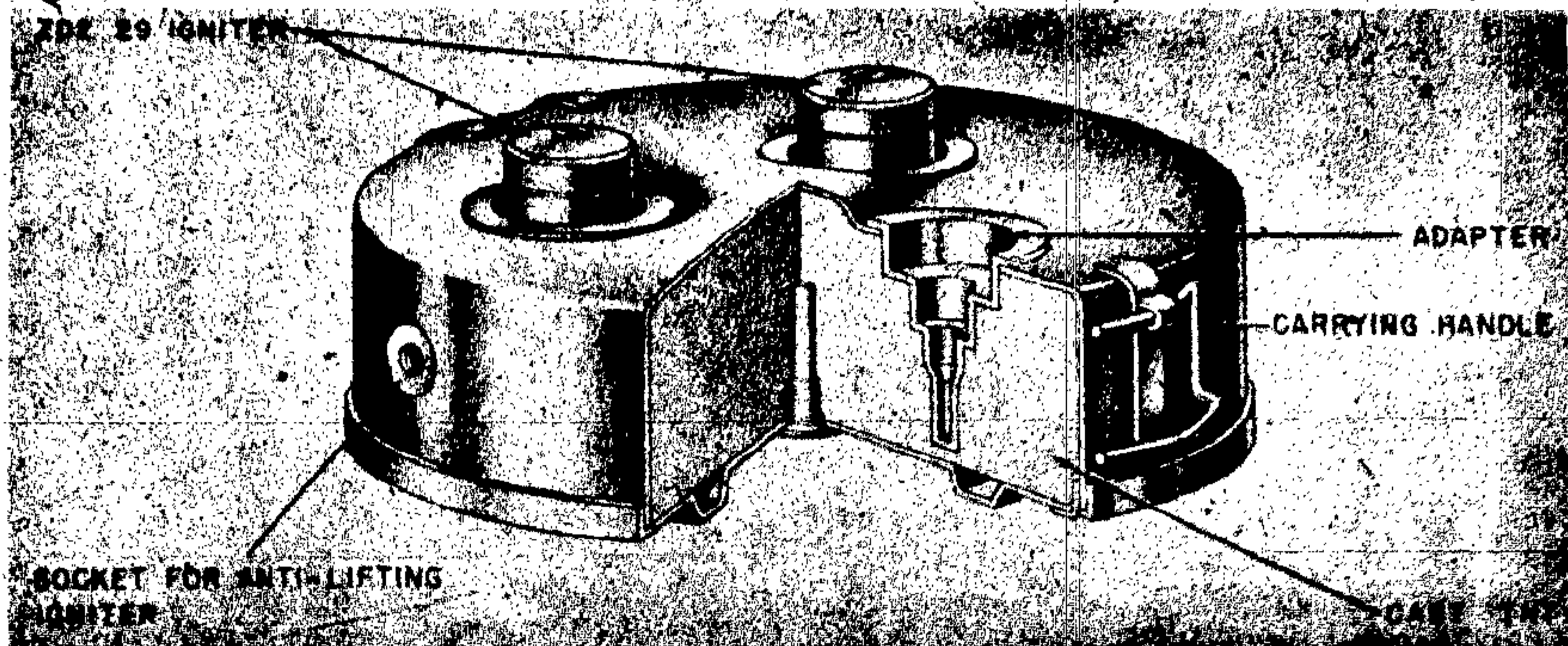
Figure 234—T. Mi. 29 (T-5) Mine—Antitank
