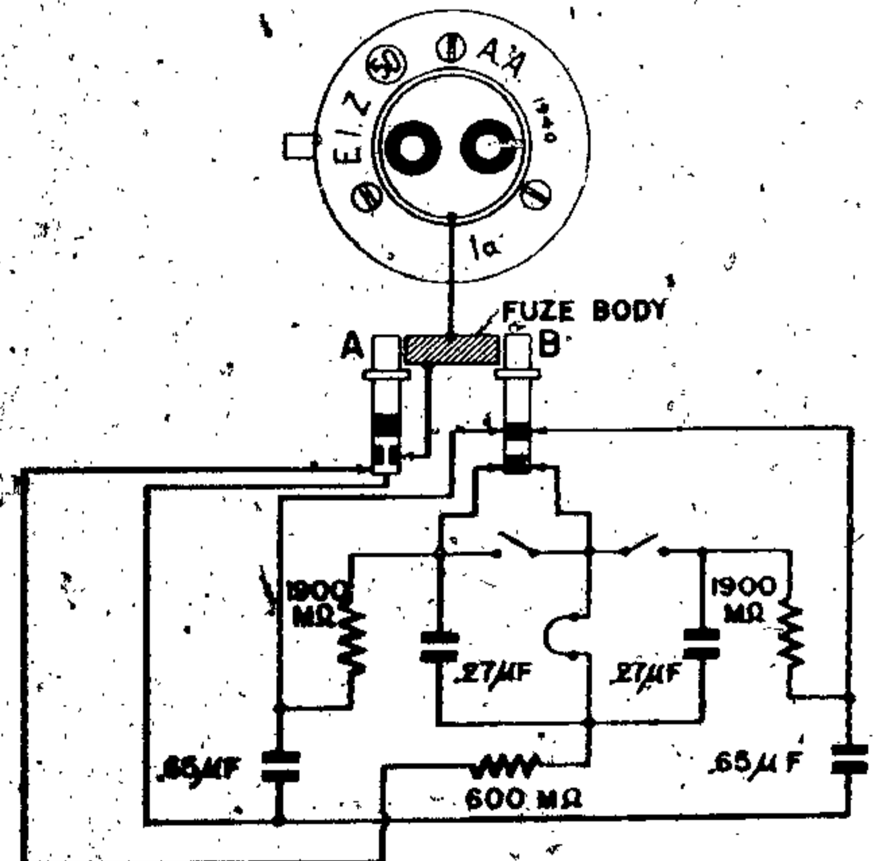
Figure 185—(50) Yellow Top Electrical Antidisturbance Fuze
