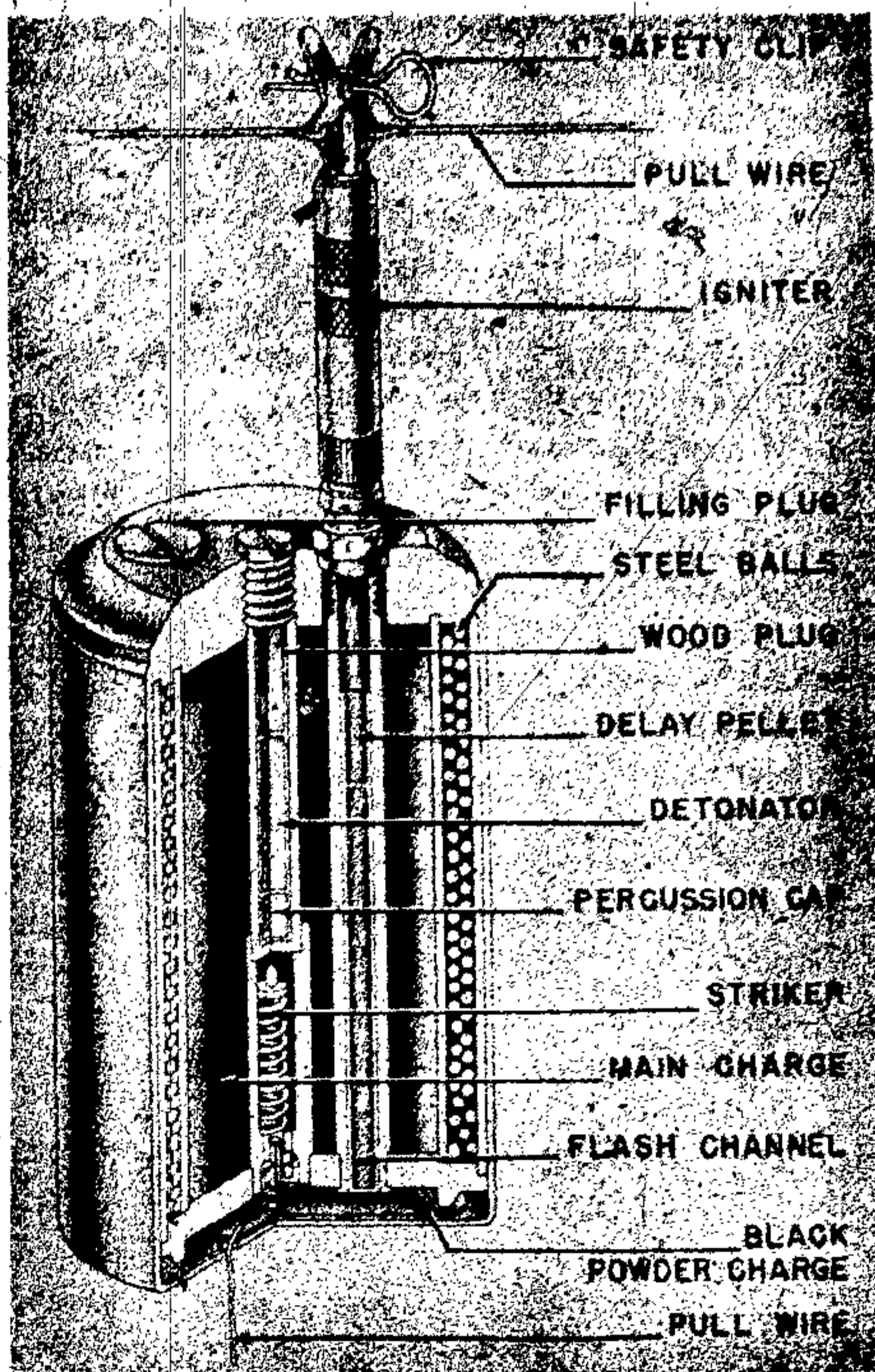
Figure 245—S-Mine 44—Antipersonnel
