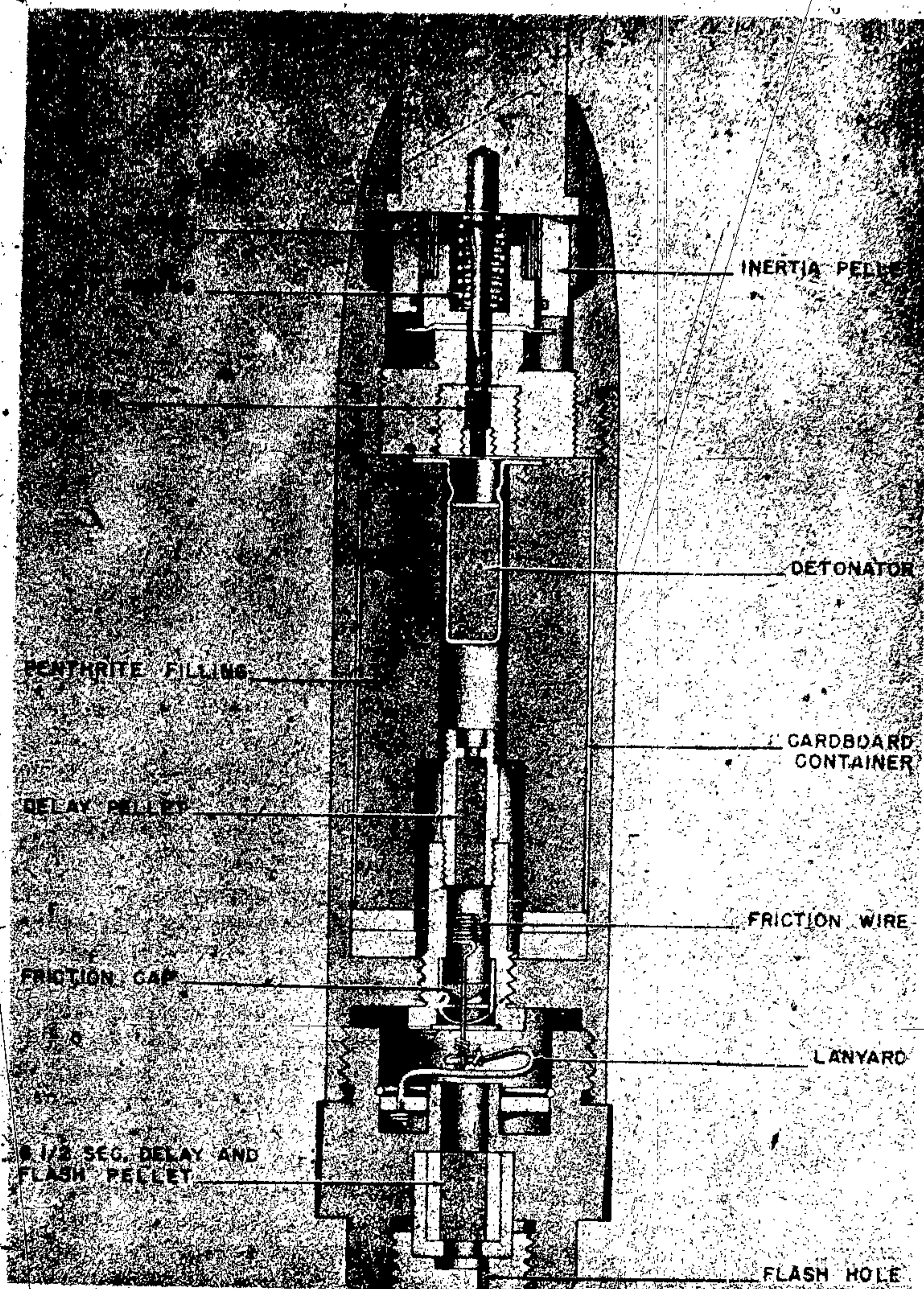
Figure 301—Hand or Rifle Grenade
