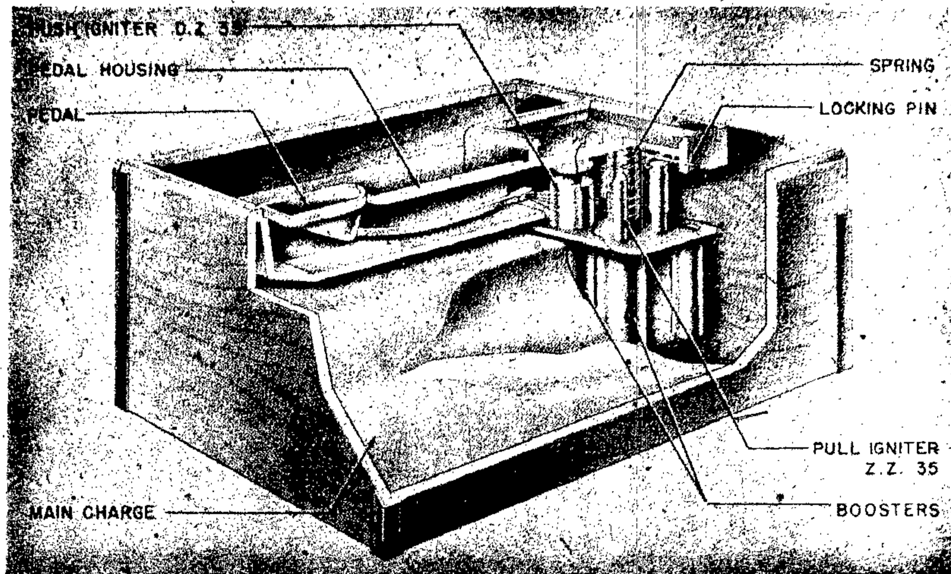
Figure 229—Heavy Antitank Mine
