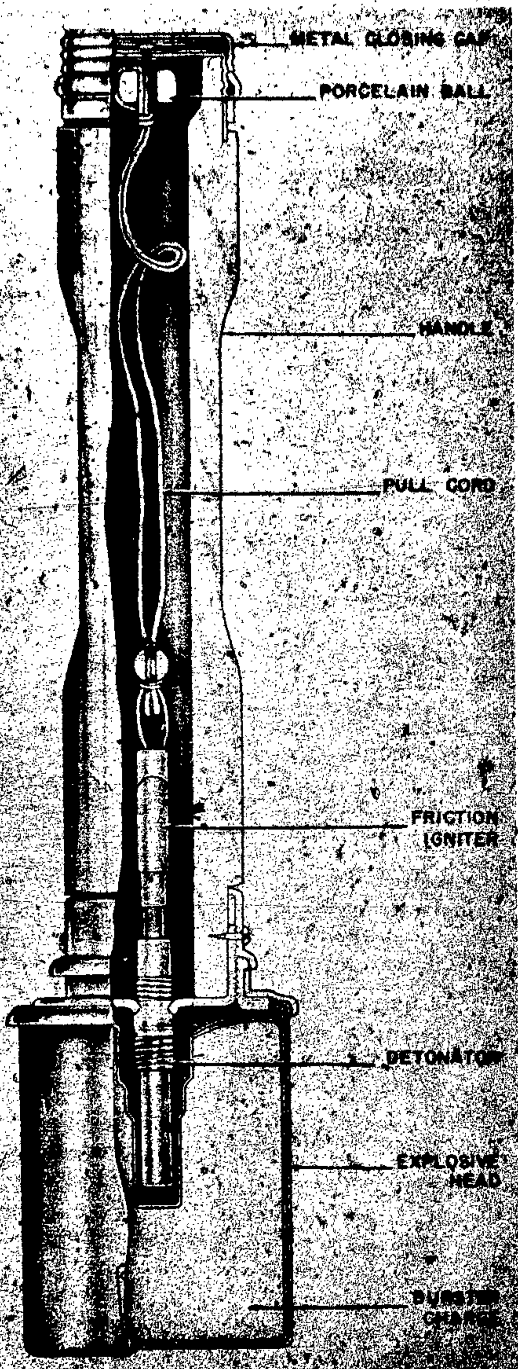
Figure 284—Model 24 Stick Hand Grenade; Model 29 Stick Hand Grenade
