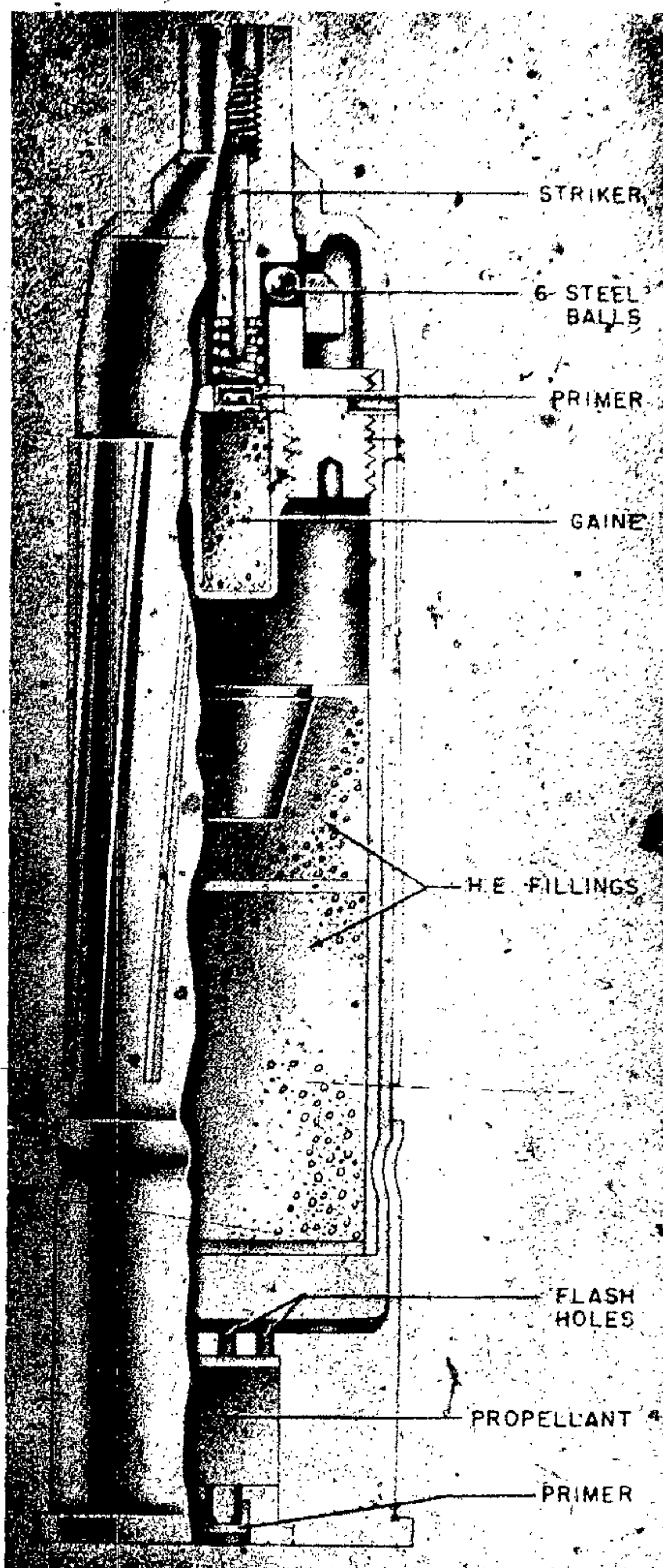
Figure 312—H. E. Cartridge for 27-mm Grenade Pistol
