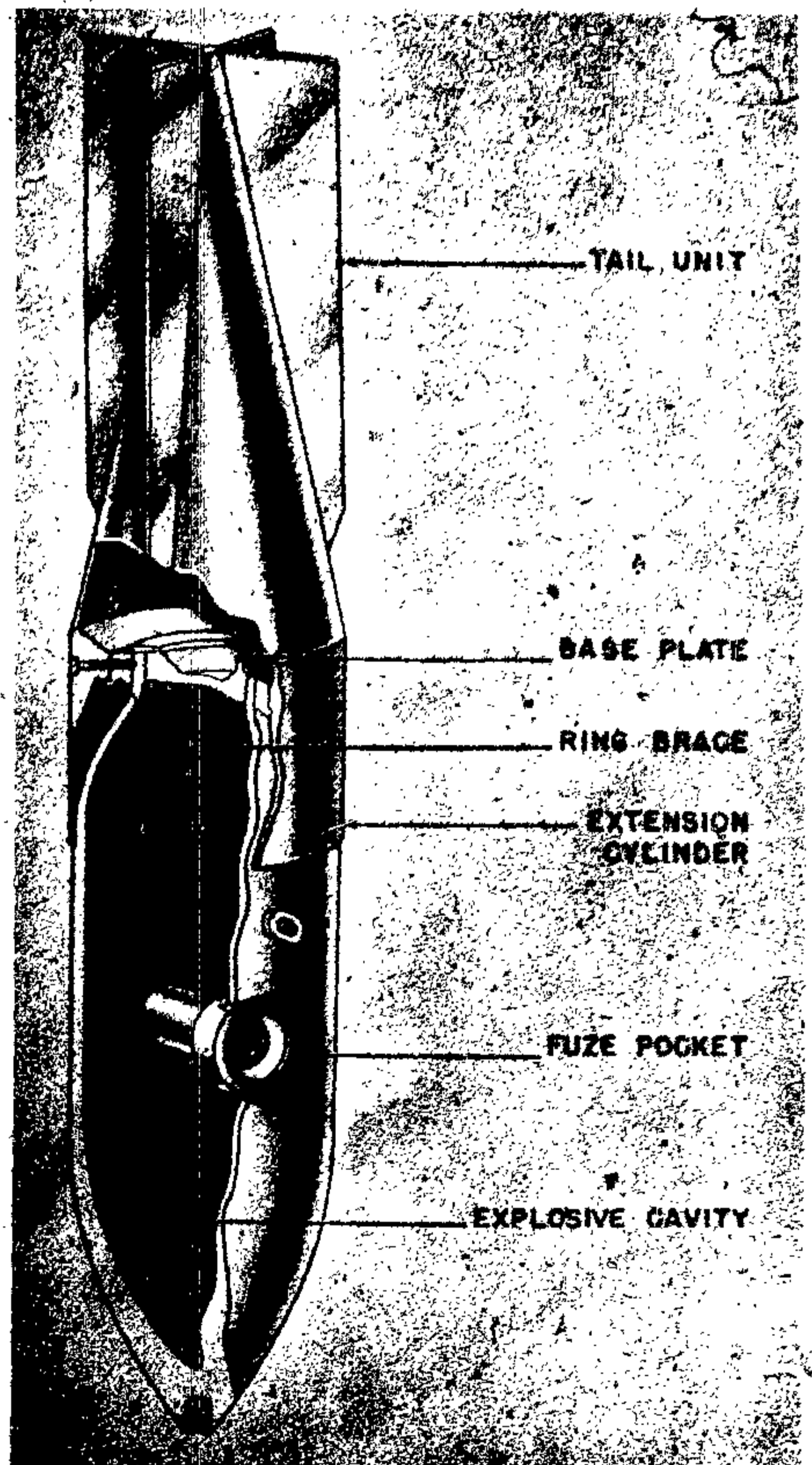
Figure 23—SD 50-Kg Bomb
