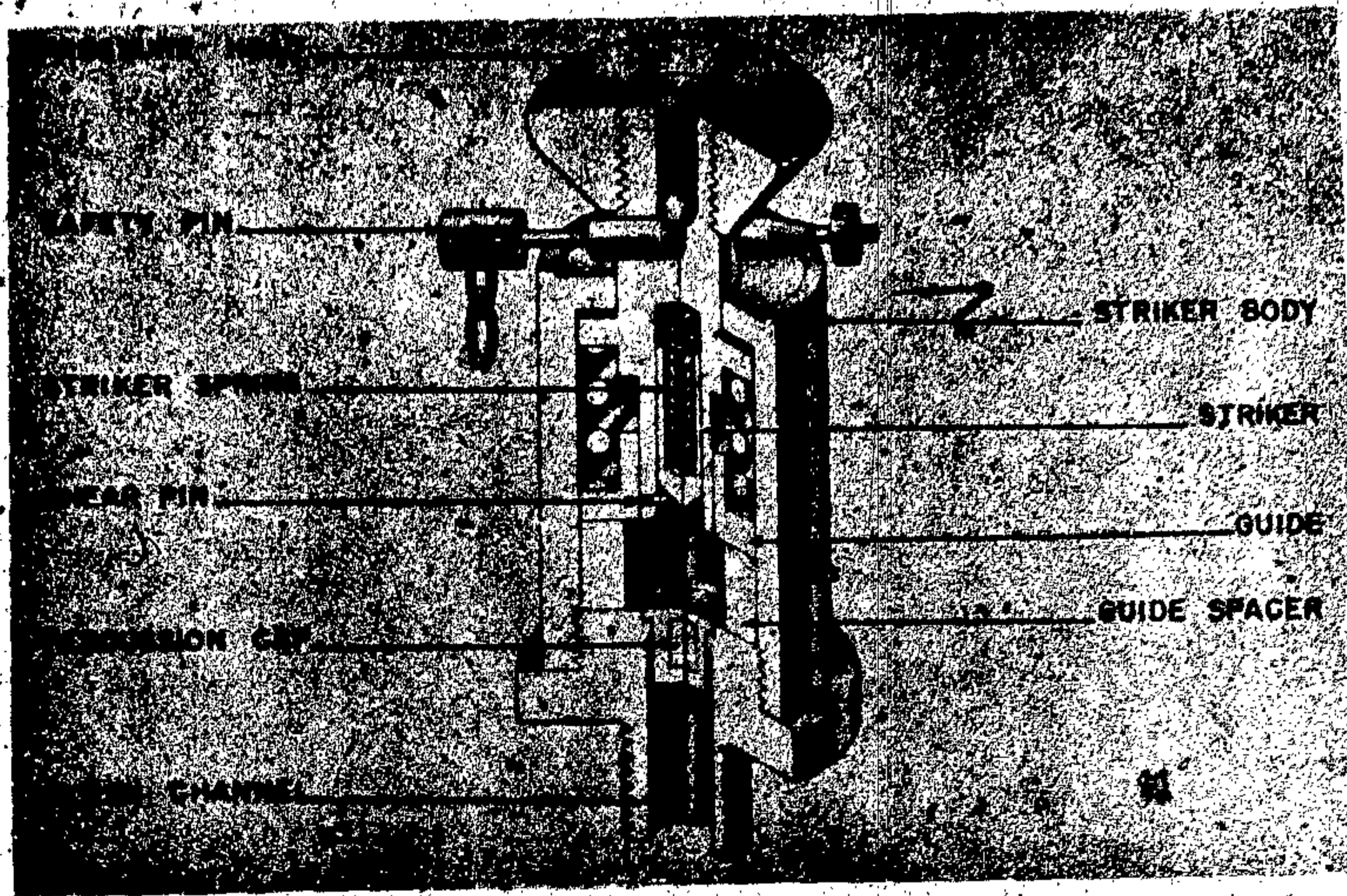
Figure 263—D. Z. 35 (B) Pressure Igniter
