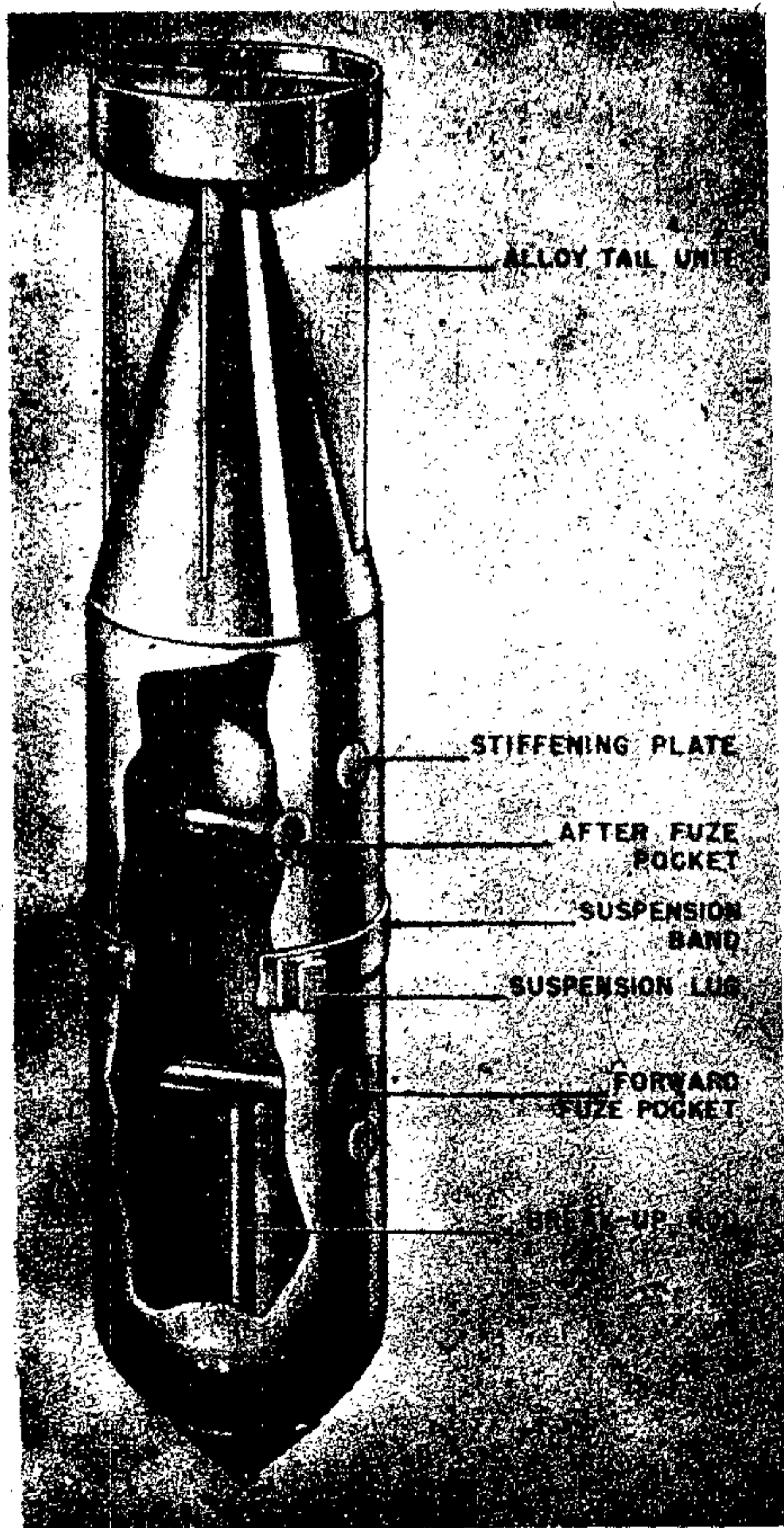
Figure 18—SC 2500-Kg Bomb
