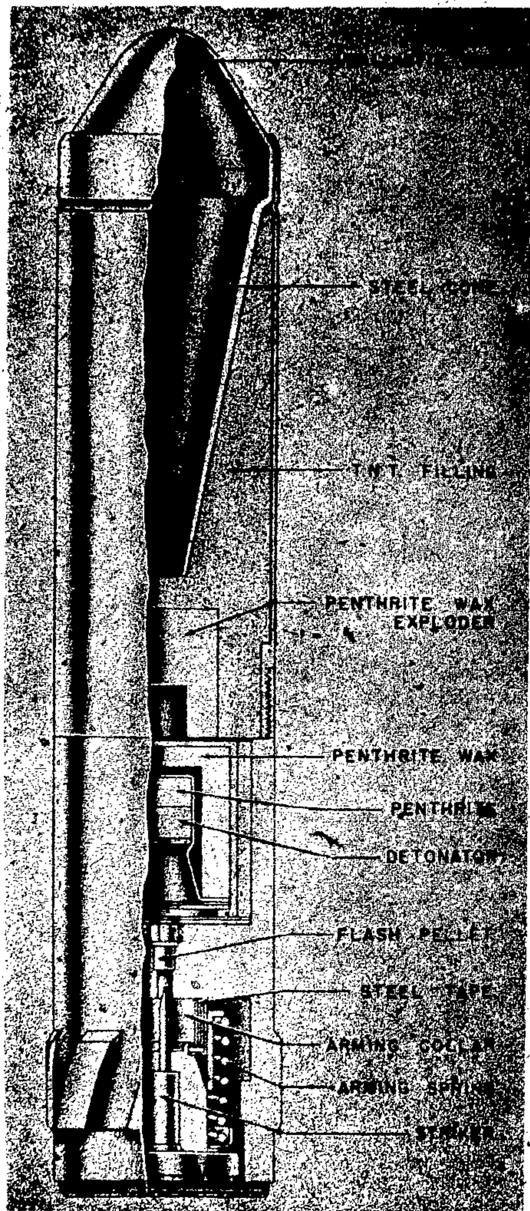
Figure 302—Antitank Hollow Charge Rifle Grenade
