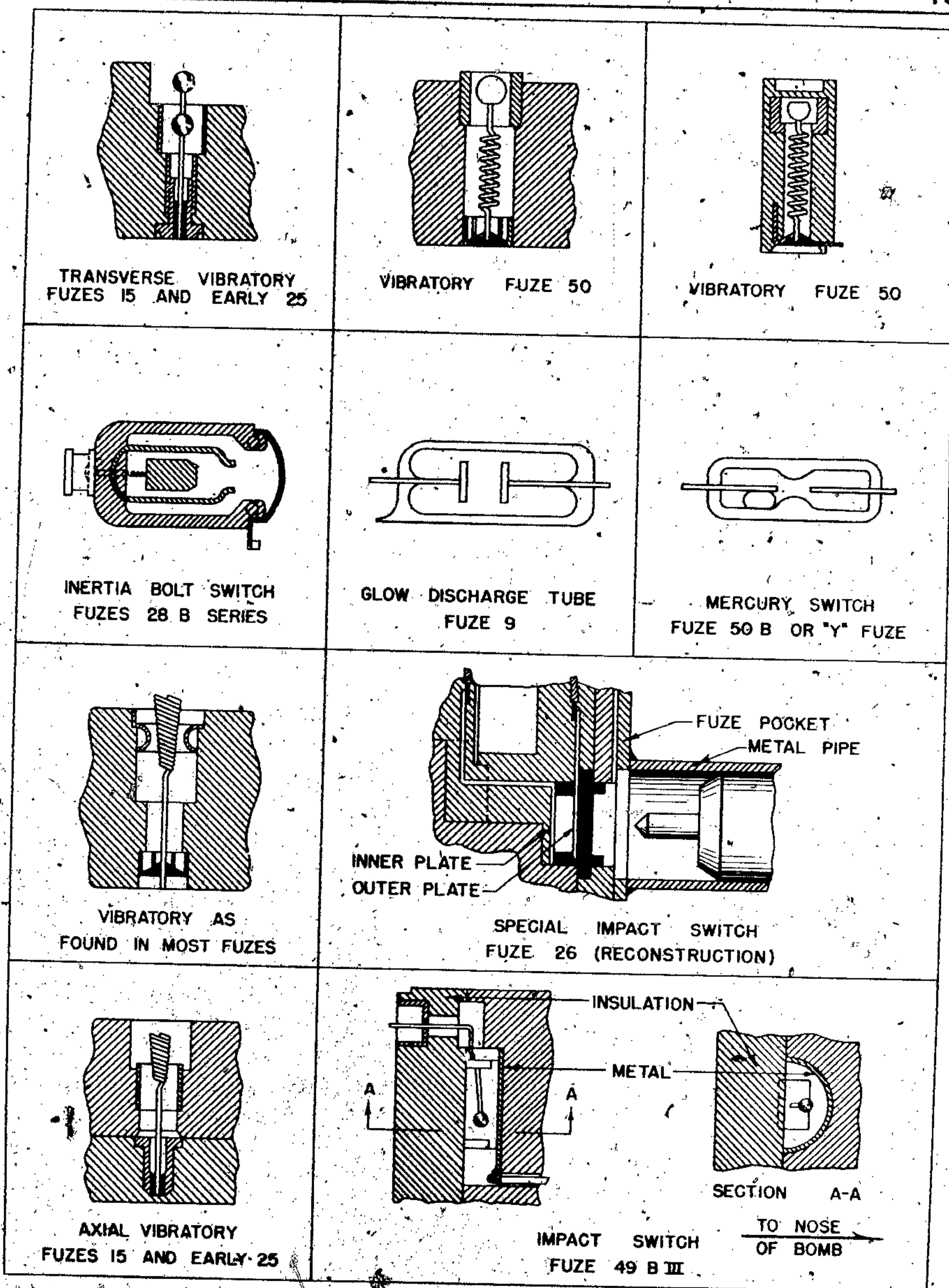
Figure 122—Types of Trembler Switches
