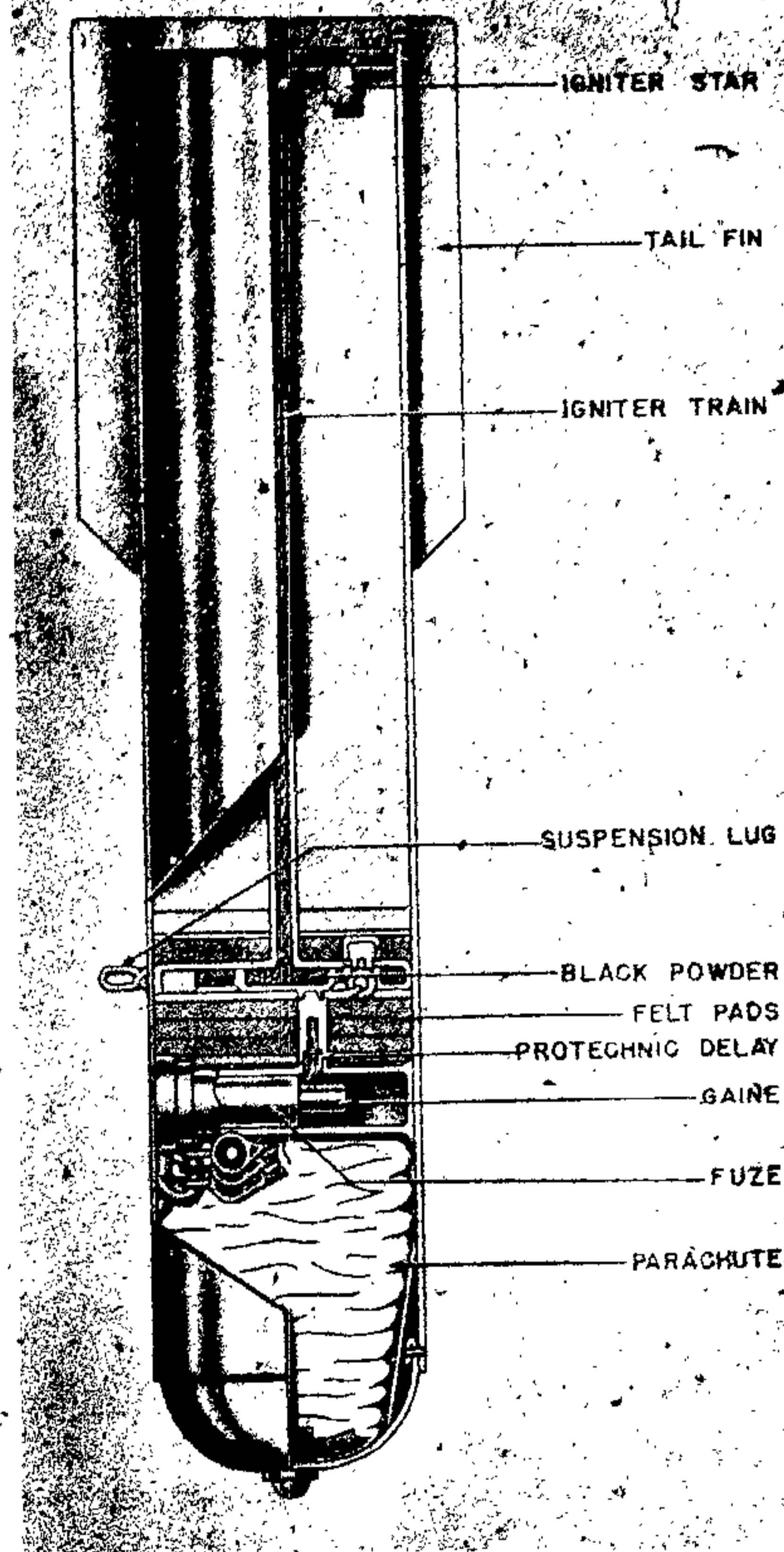
Figure 74—LC 50 F Ausf. G Parachute Flare
