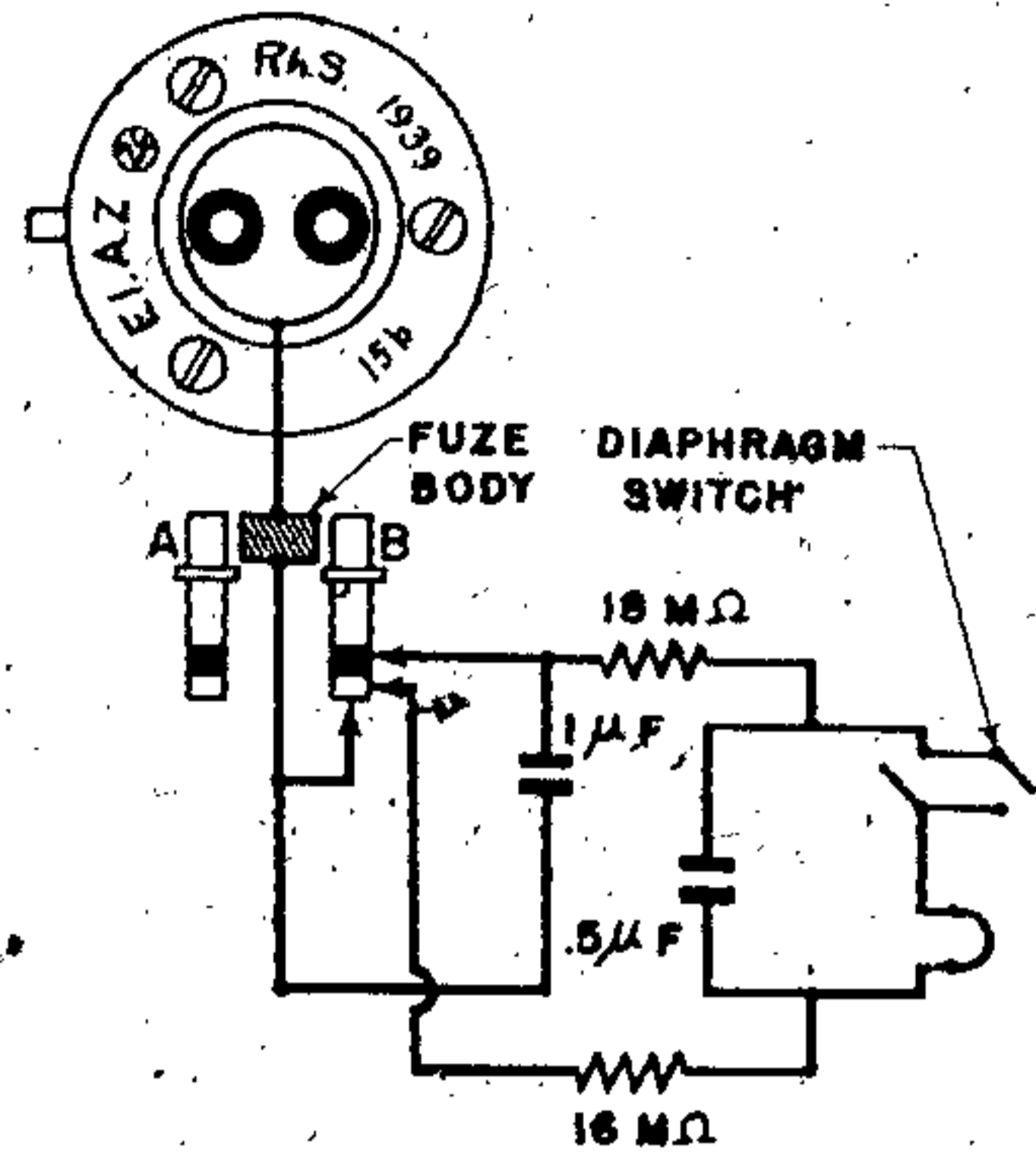
Figure 147B—(26) Electrical Impact (Special) Wiring Diagram
