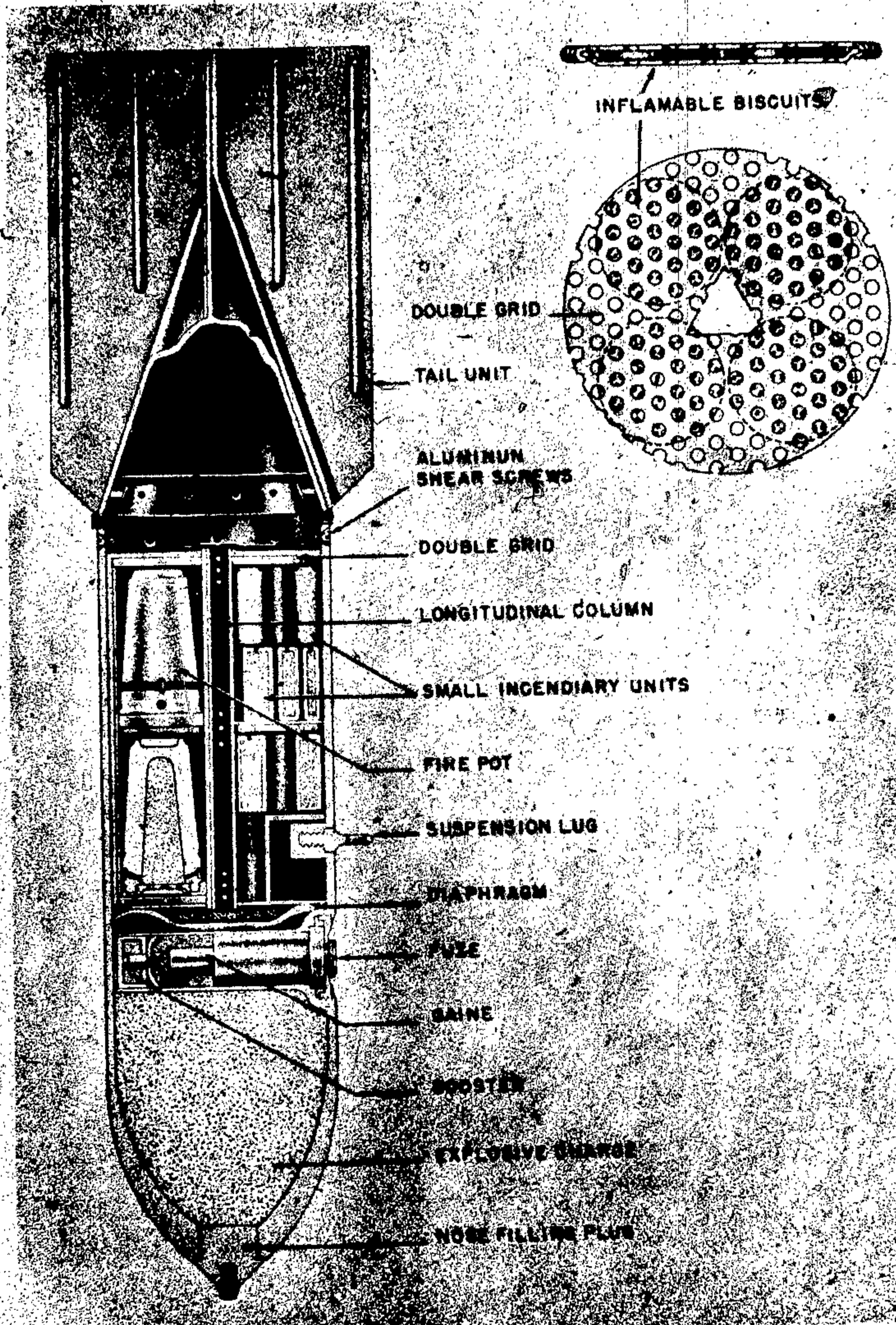
Figure 54—Sprengbrand C-50 Bomb
