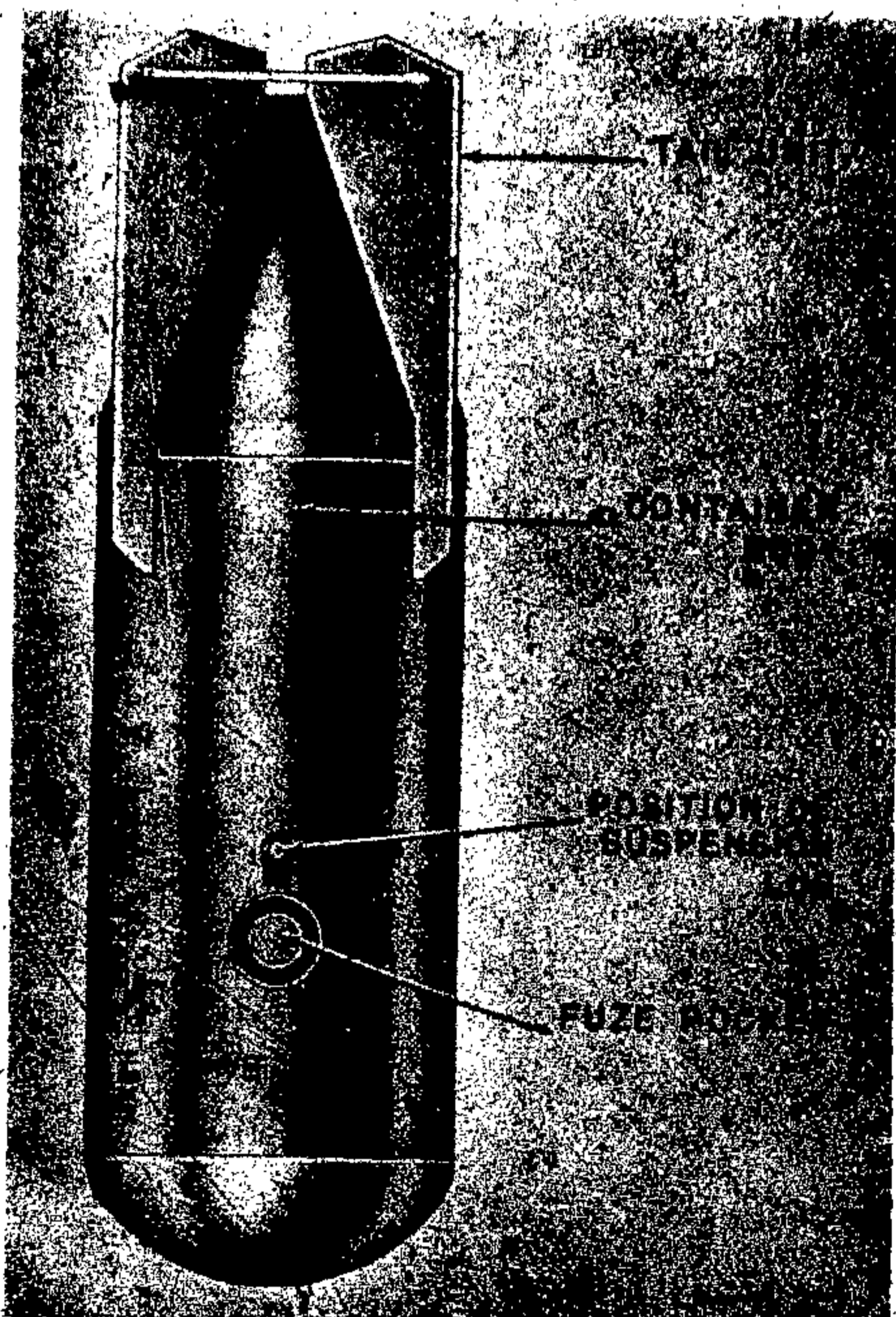
Figure 108—AB 250 KZ Boden Container
