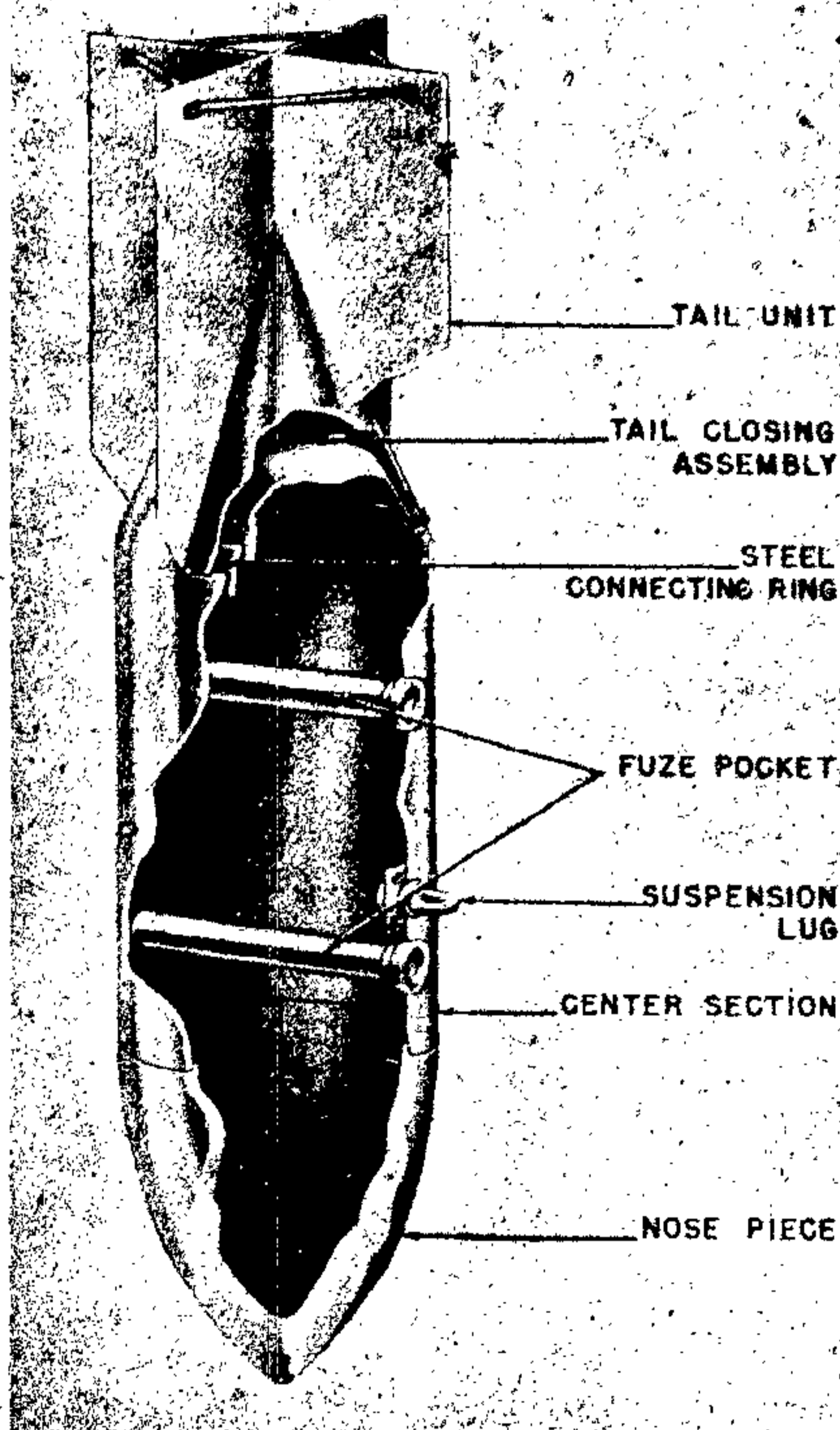
Figure 13—SC 500-Kg Bomb
