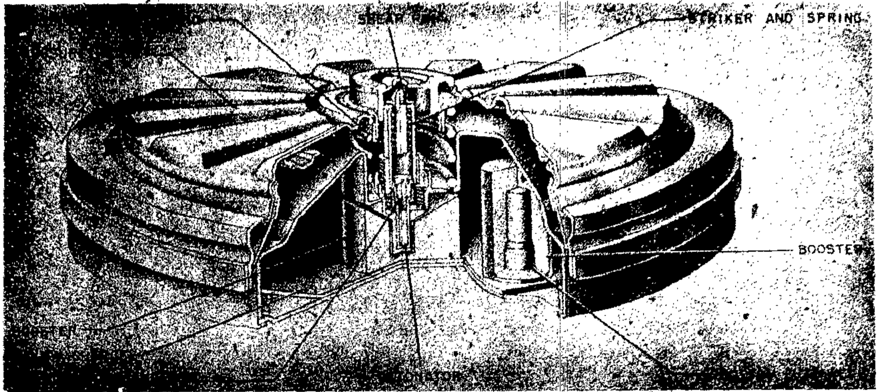
Figure 231—Tellermine 35 (Steel Antitank)
