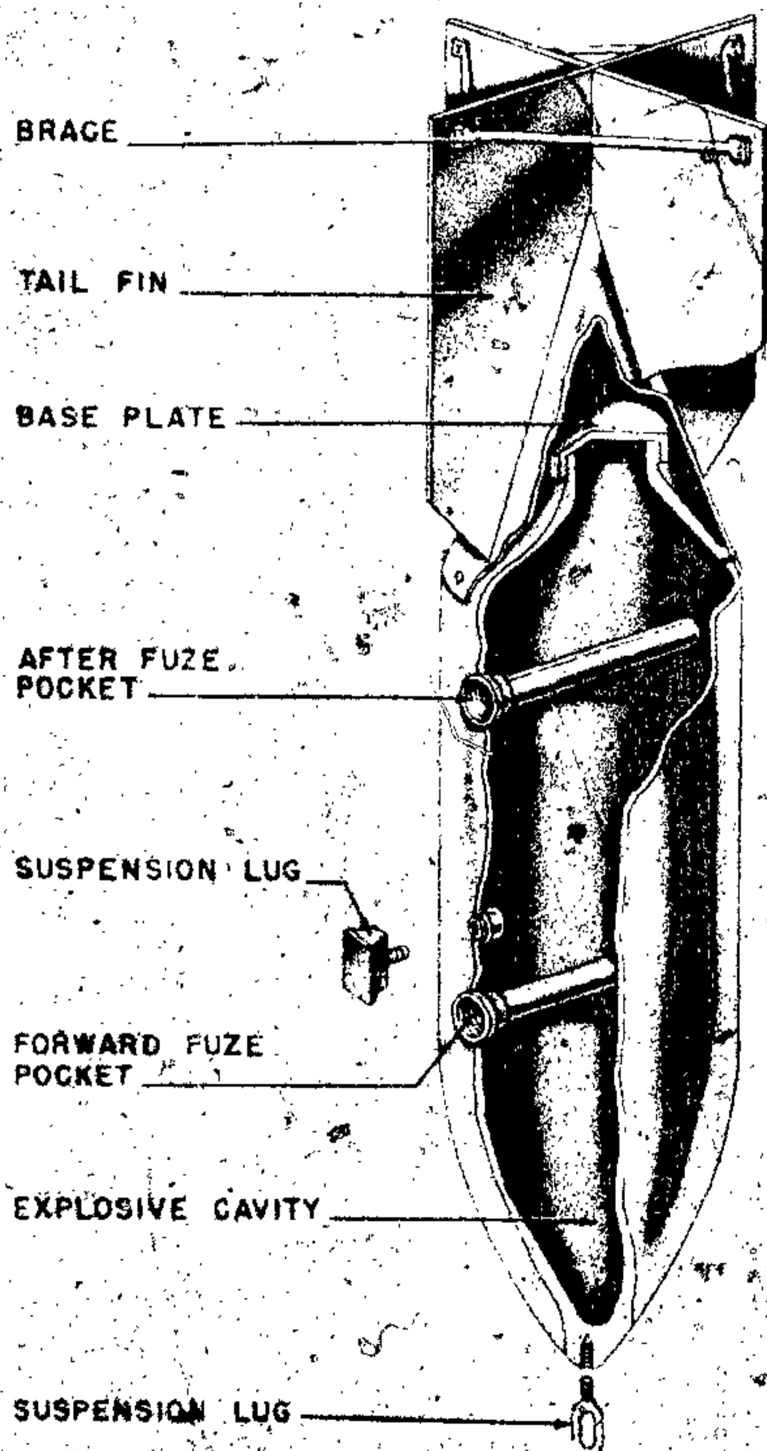
Figure 12—SC 250 Bomb; types 1, 2, and 3
