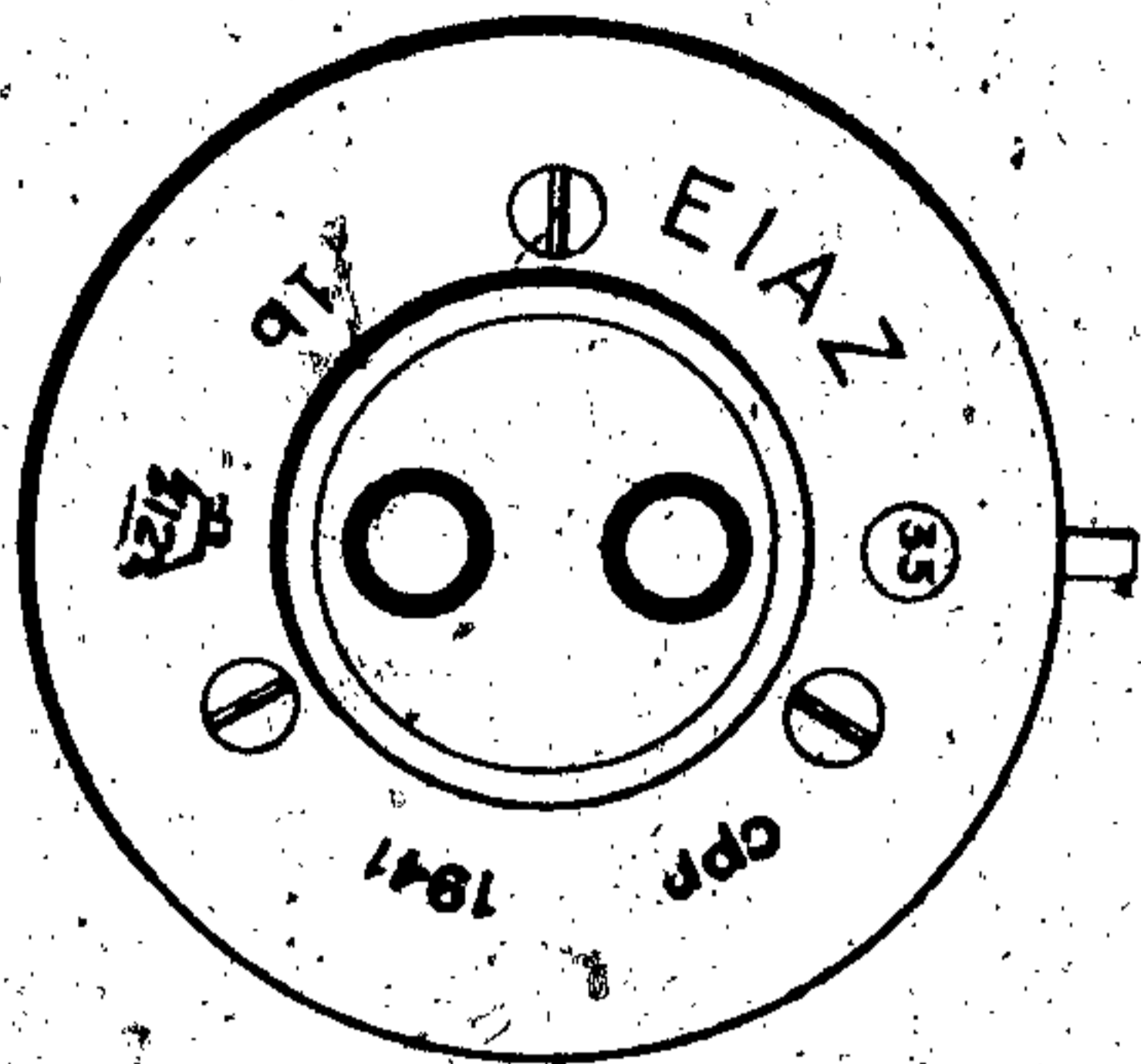
Figure 125—Fuze Markings
