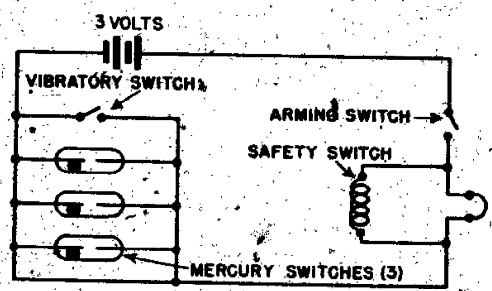
FIRING CIRCUIT DIAGRAM
