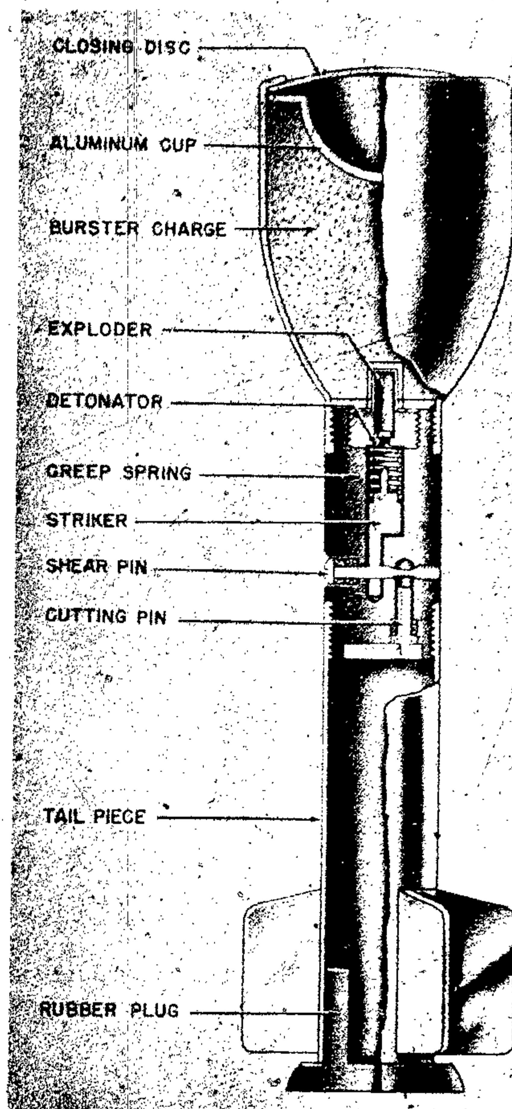
Figure 305—Schuss Gg. P-40 Hollow Charge Rifle Grenade
