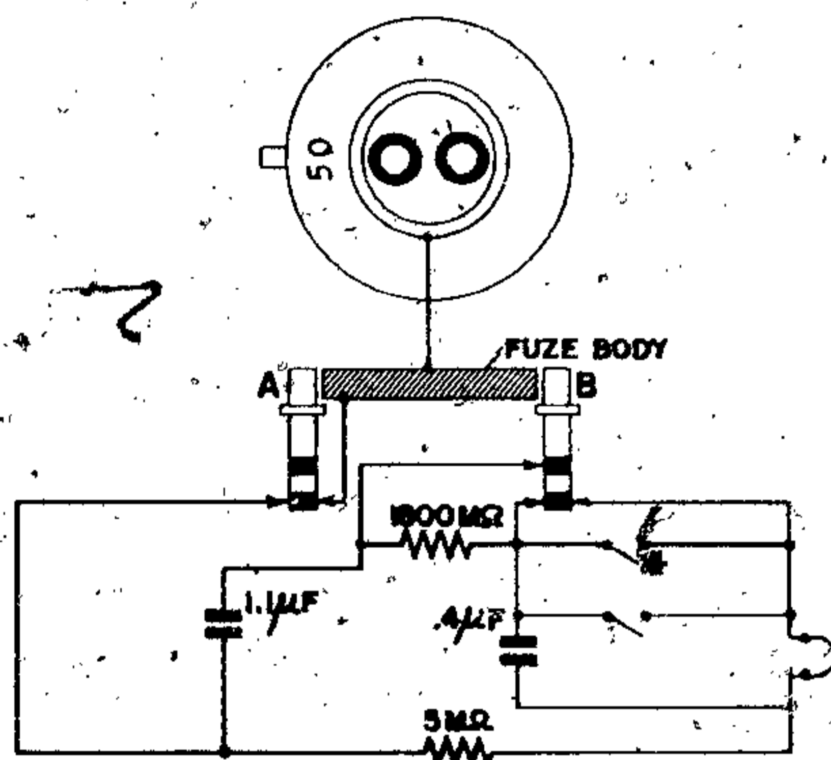
Figure 183—50 Electrical Antidisturbance Fuze
