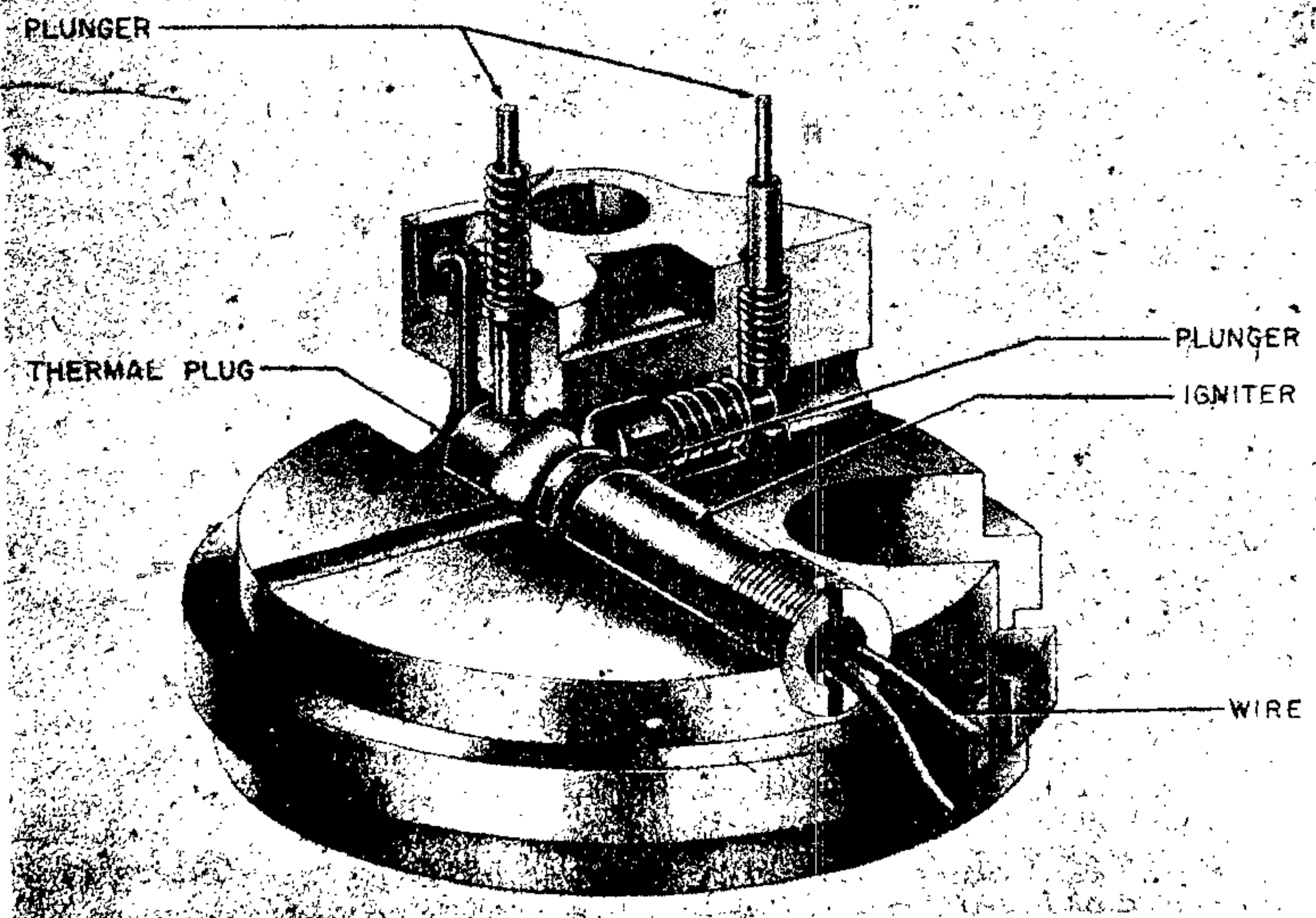
Figure 179—(89)B Clockwork Aerial Burst Fuze
