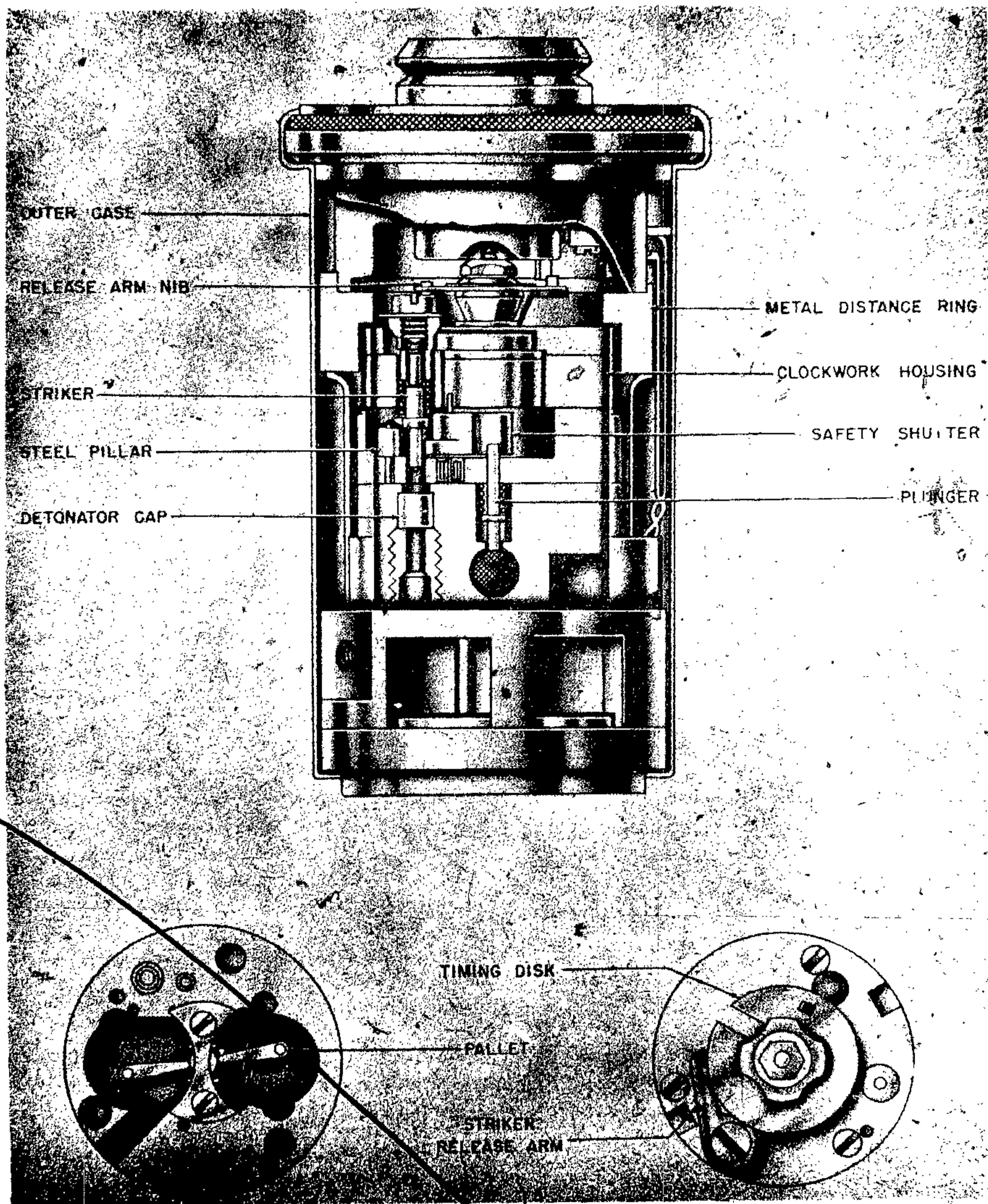
Figure 180—(89)D Clockwork Aerial Burst Fuze
