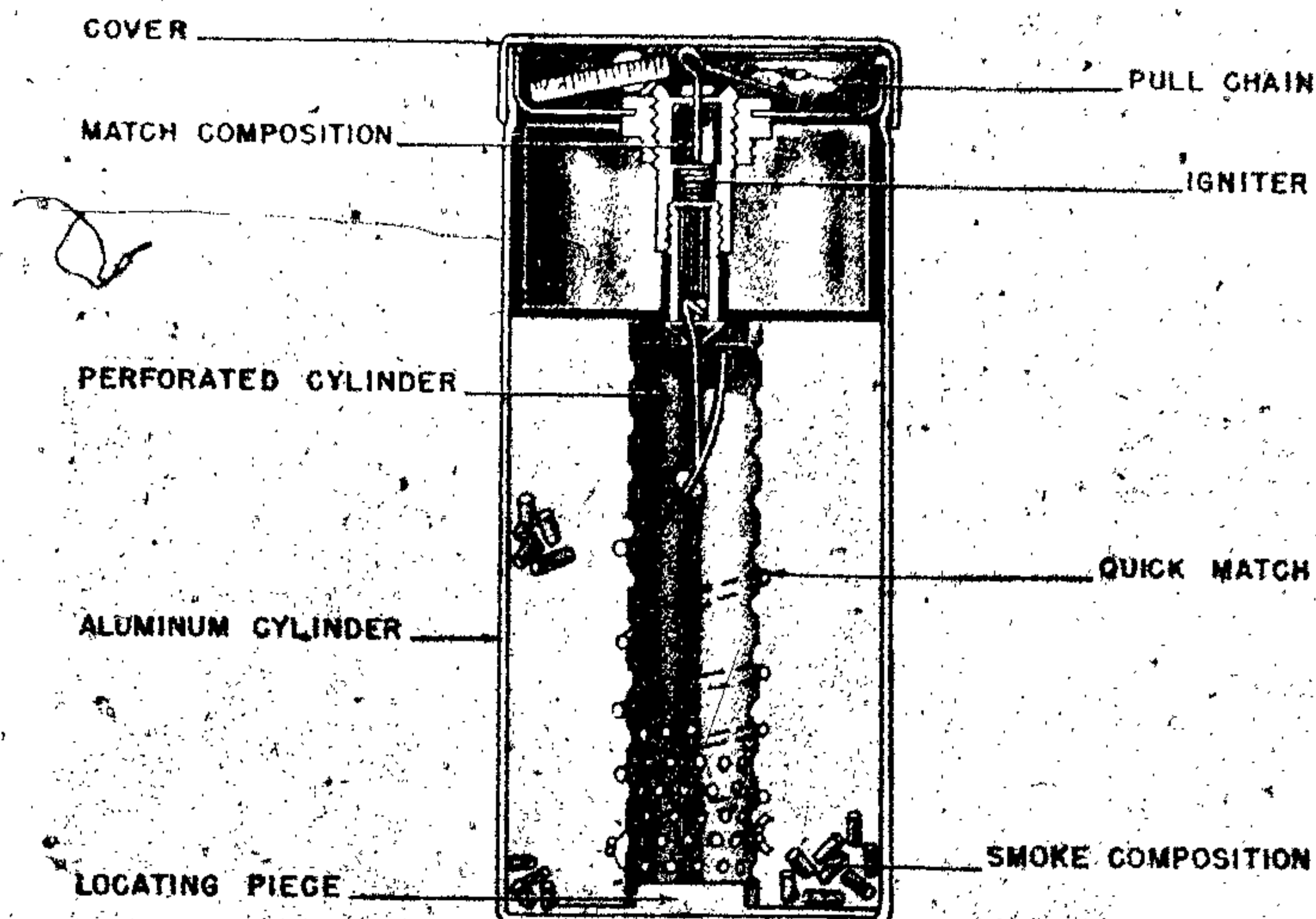
Figure 81—Smoke Flare, Orange, 160
