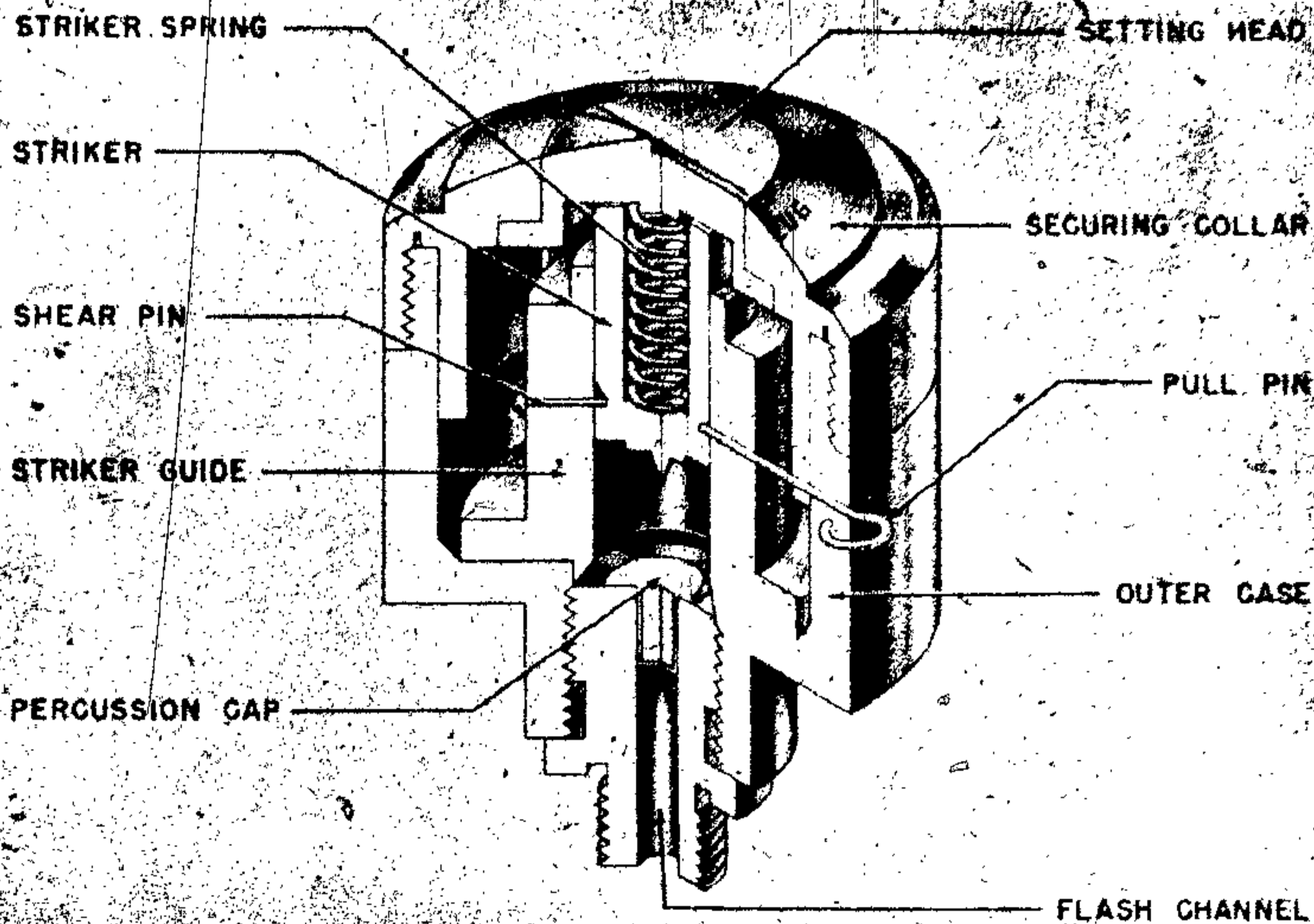
Figure 259—Z. D. Z. 29 Igniter—Pressure and Pull
