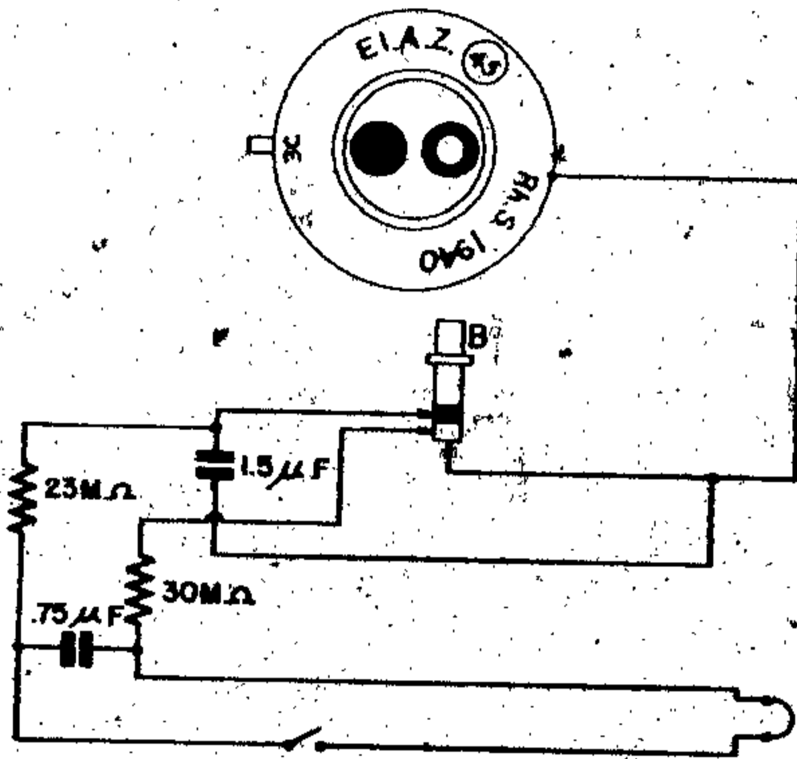
Figure 144—(45) Electrical Impact Fuze
