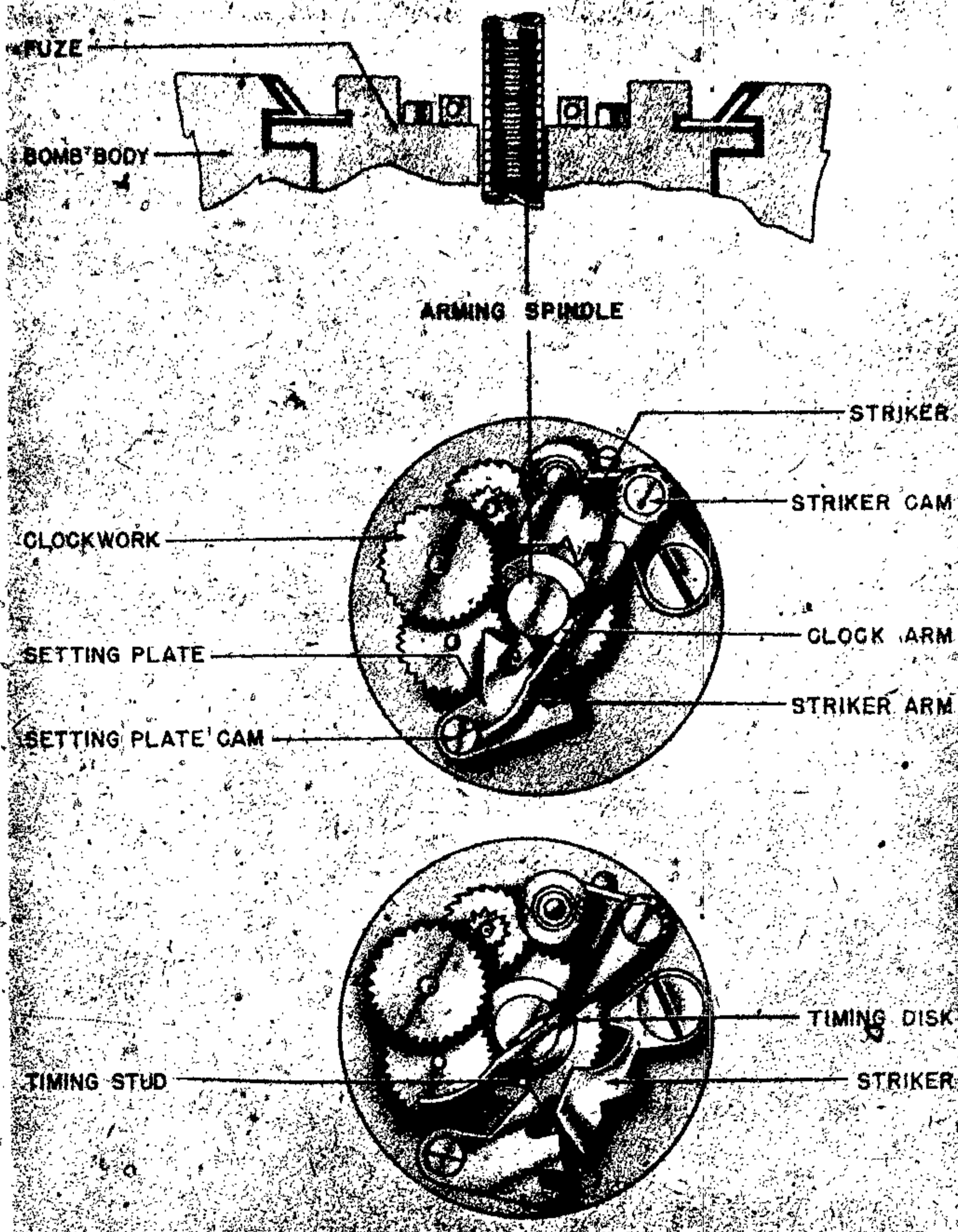
Figure 157—(67) Mechanical Clockwork Time Fuze
