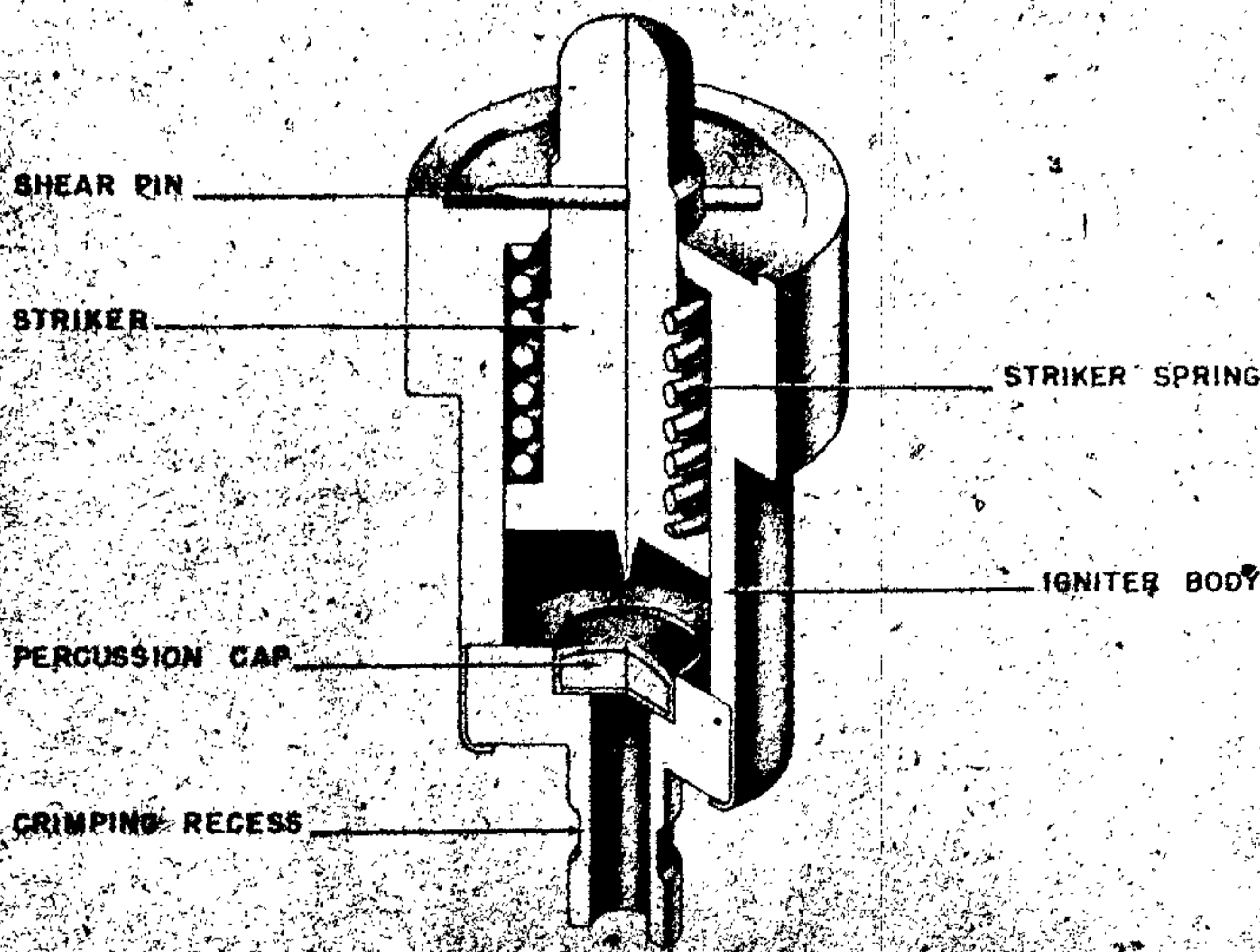
Figure 272—Mi. Z. 530 (e) Pressure Igniter
