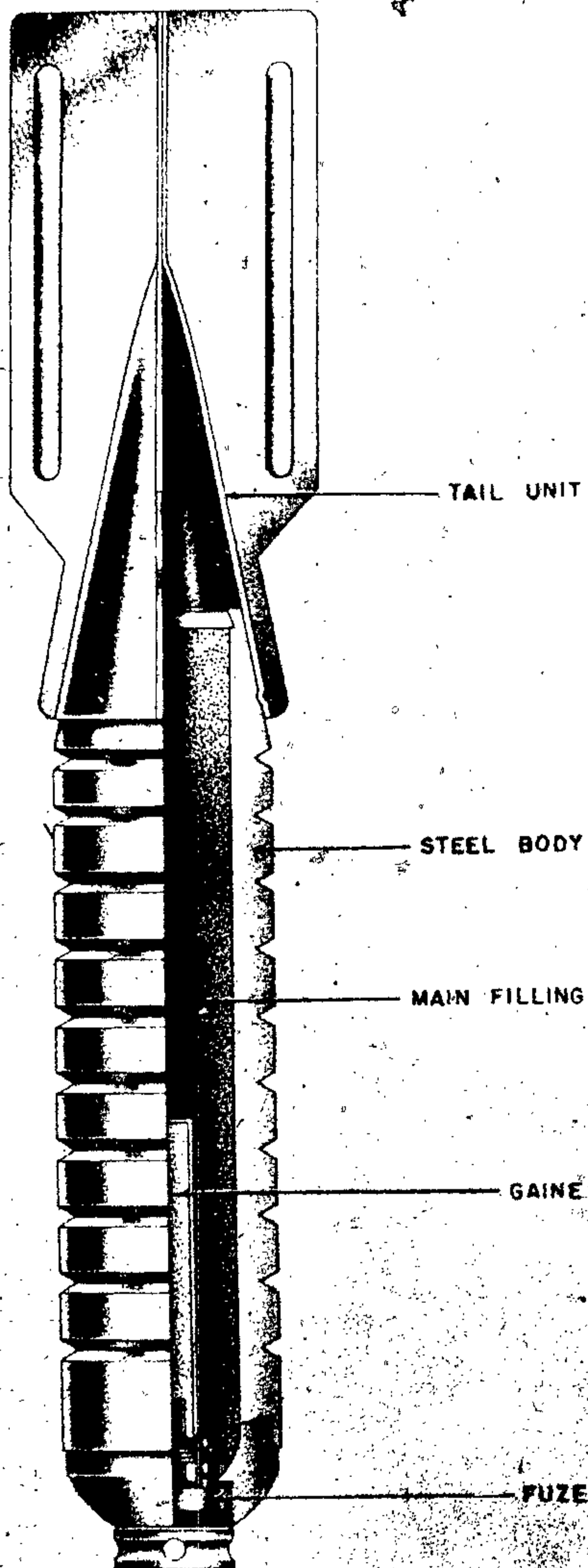
Figure 43—SD 10C Antipersonnel Bomb
