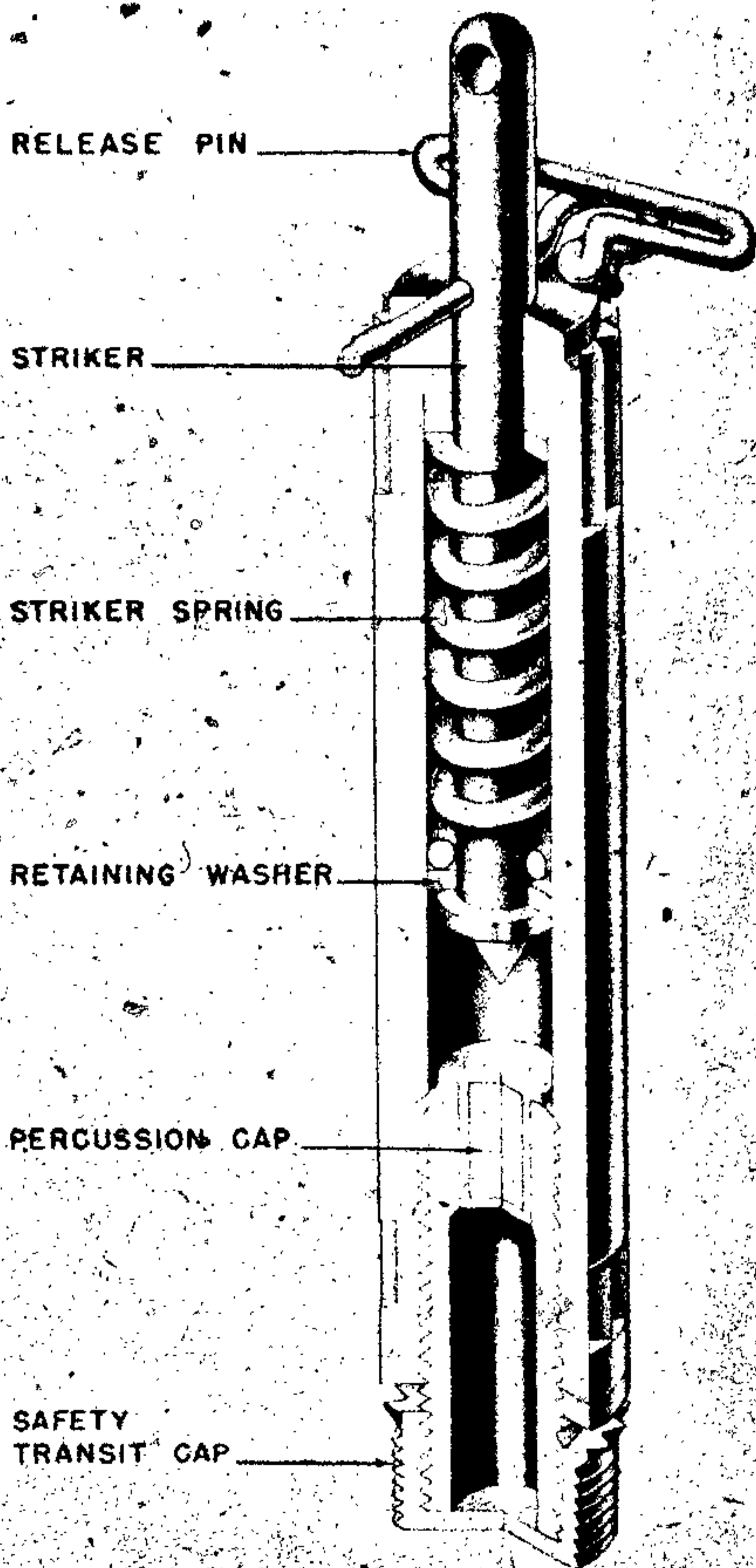
Figure 260—Z. Z. 42 Igniter—Pressure and Pull
