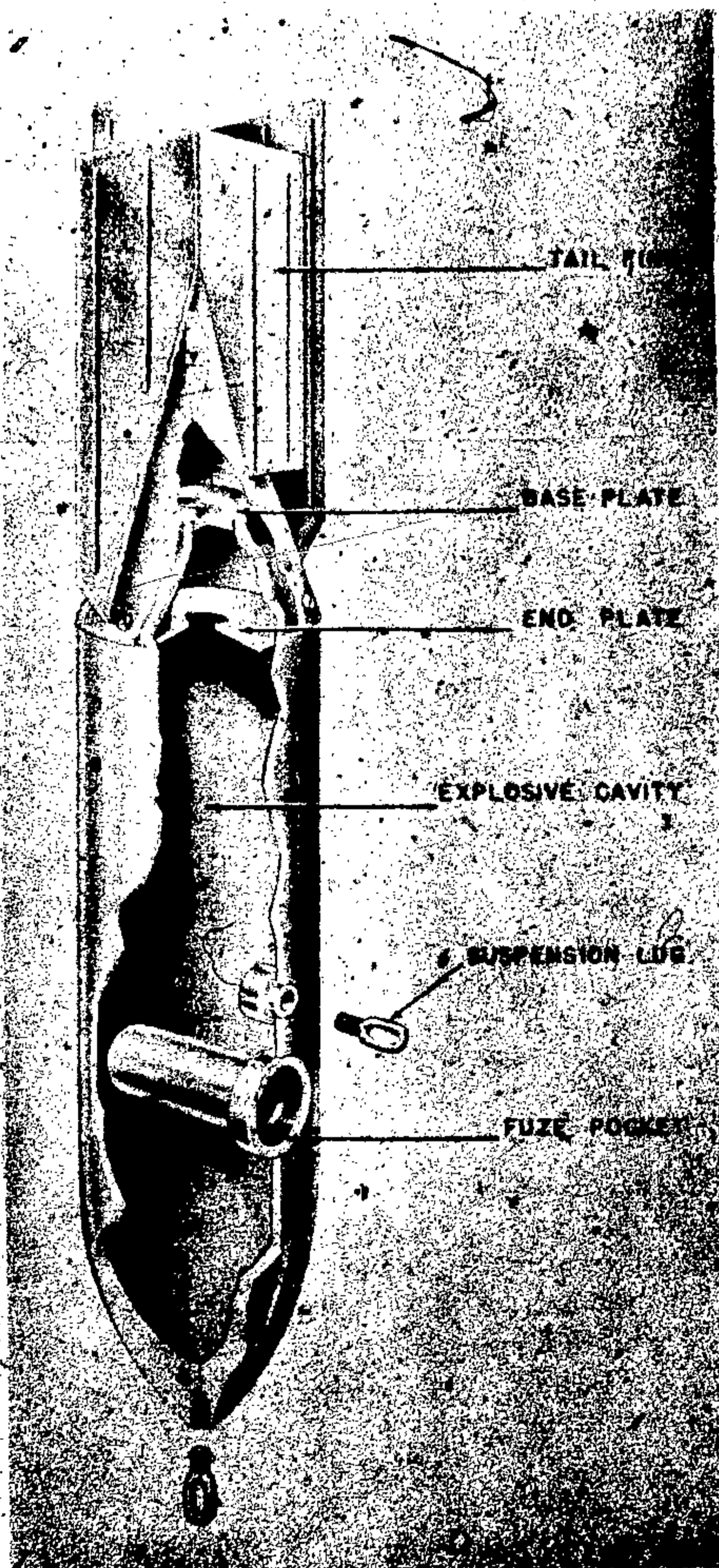
Figure 9—SC 50 Bi Bomb
