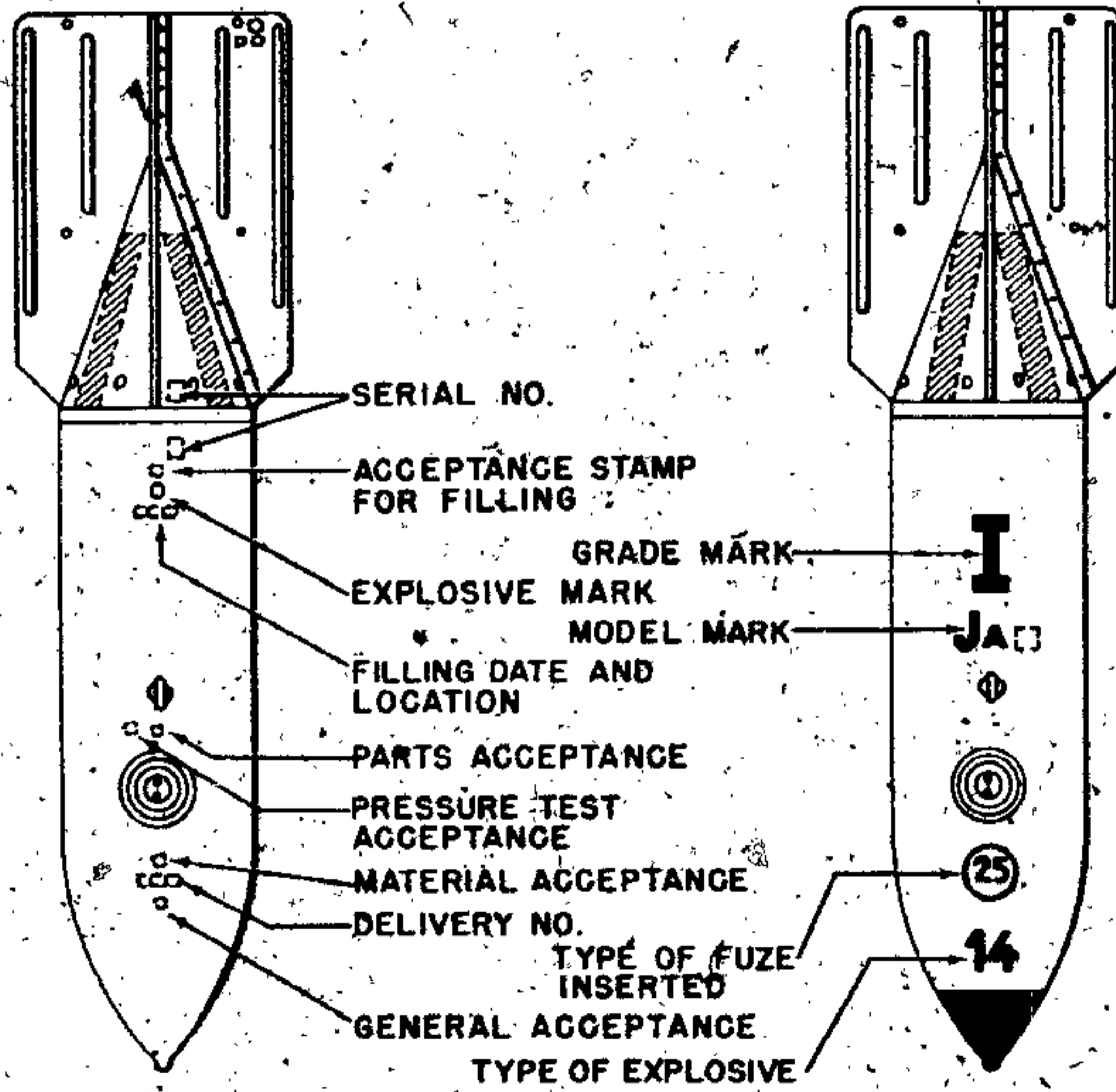
Figure 2—Paint Markings and Stampings
