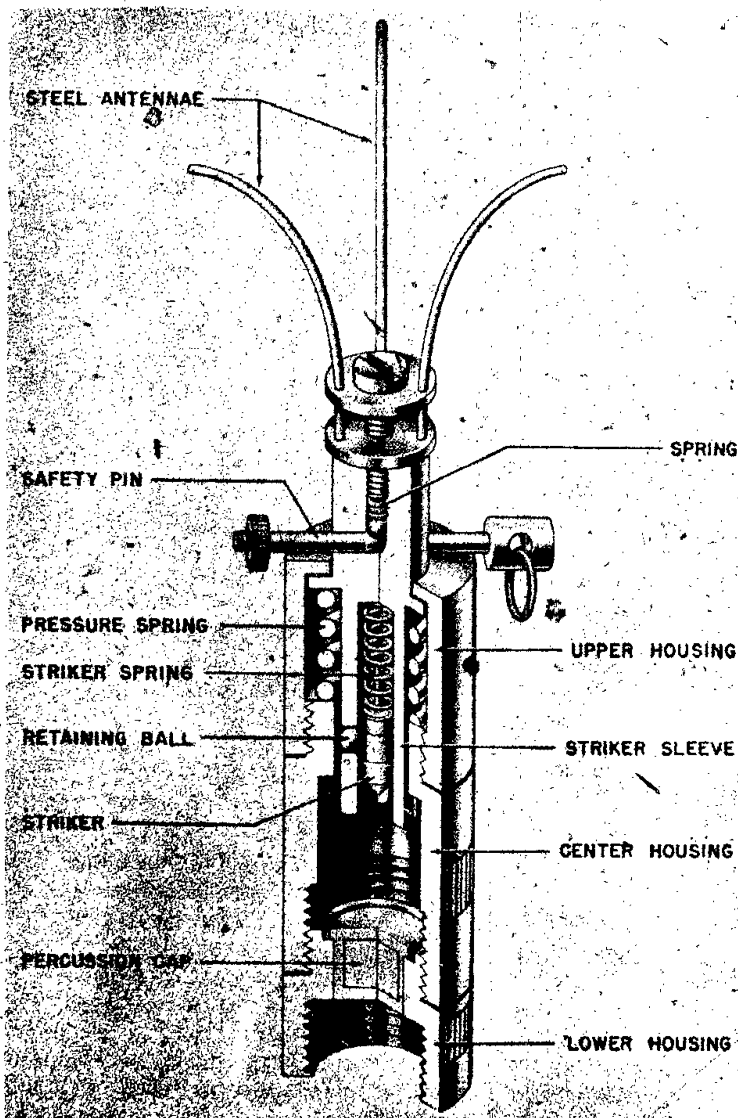
Figure 267—S. Mi. Z. 35 Pressure Igniter
