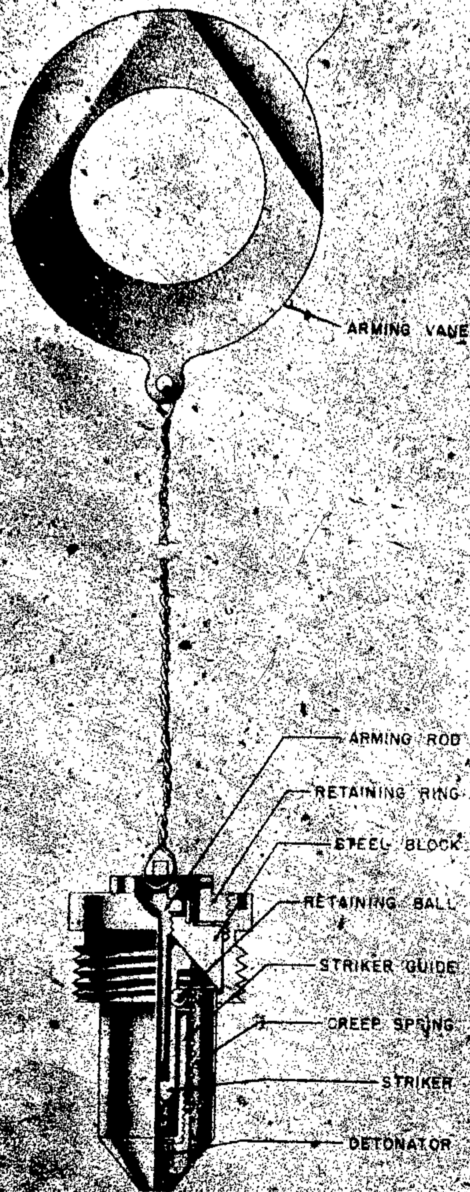
Figure 134—(23)A Mechanical Tail Impact Fuze
