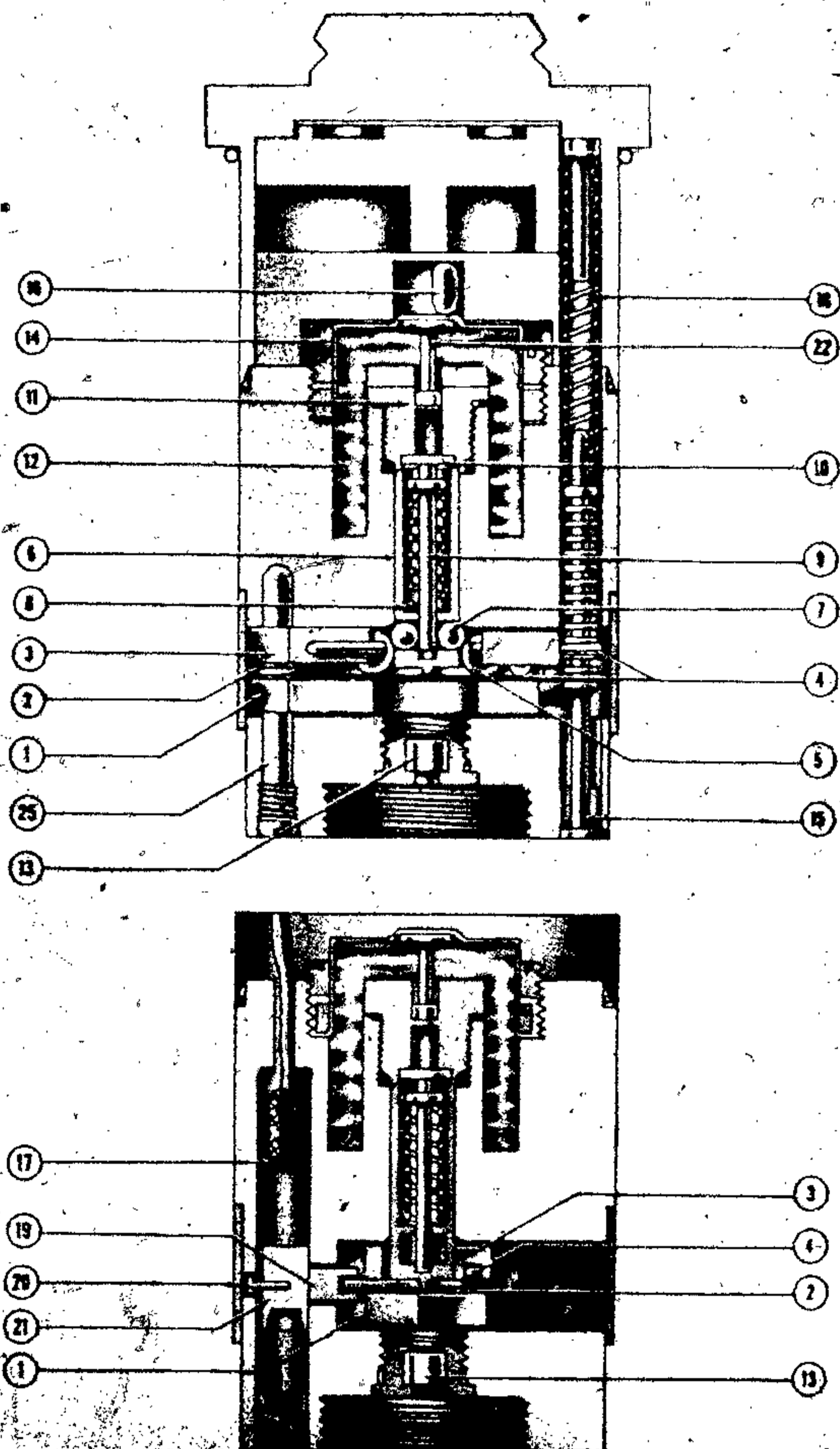
Figure 156A—(57) Electrical Chemical Time Fuze
