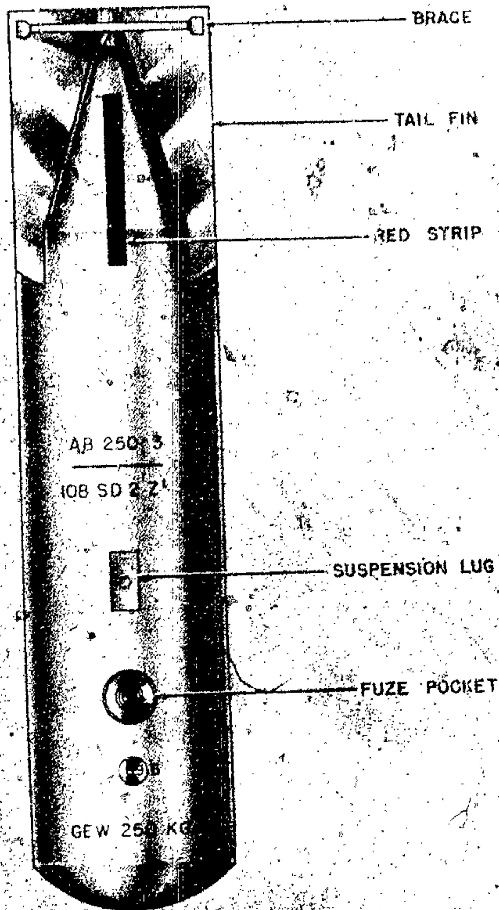
Figure 107—AB 250-3 Container, Types I and II
