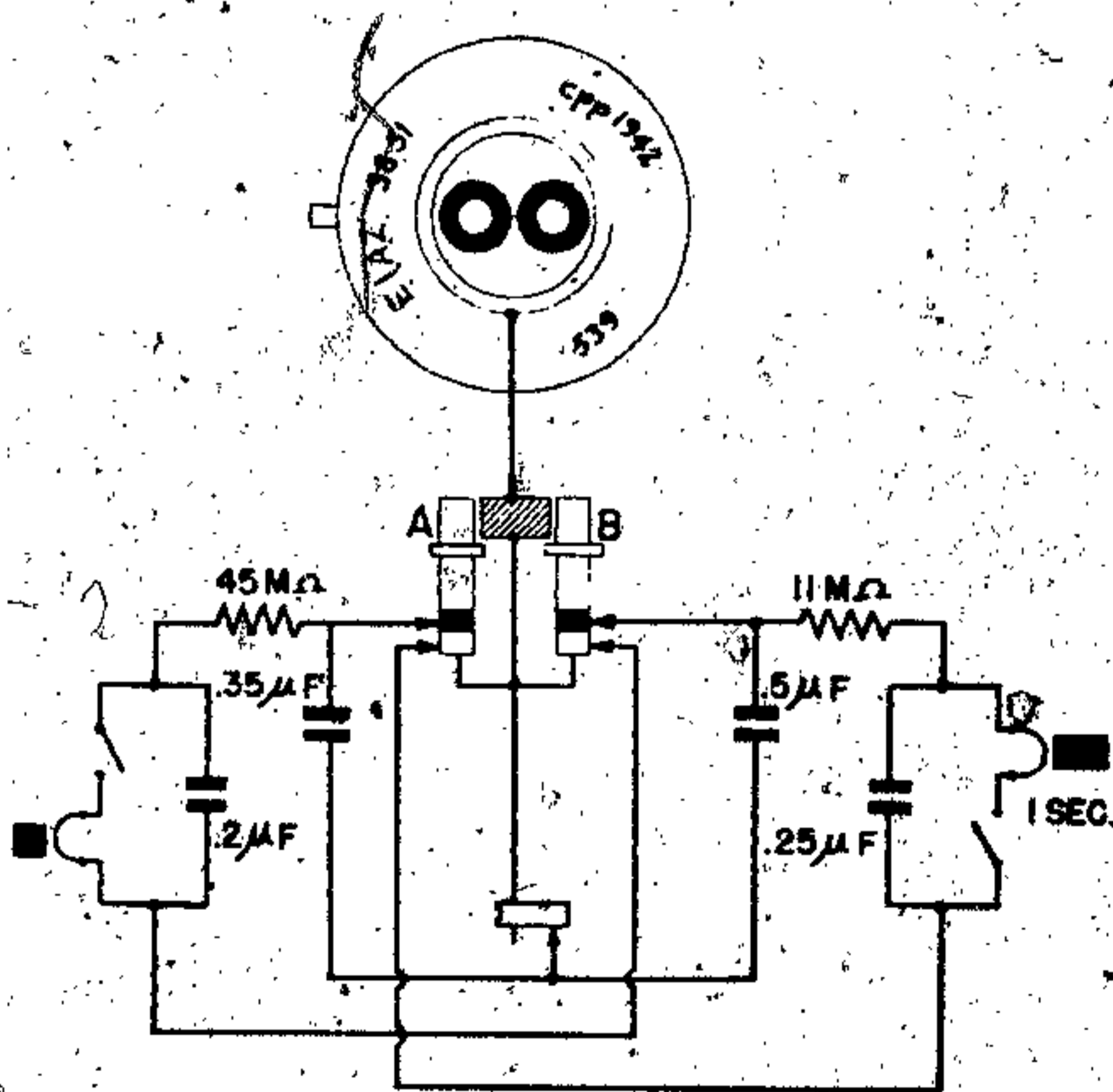
Figure 166—(38 sl) Electrical Impact Fuze
