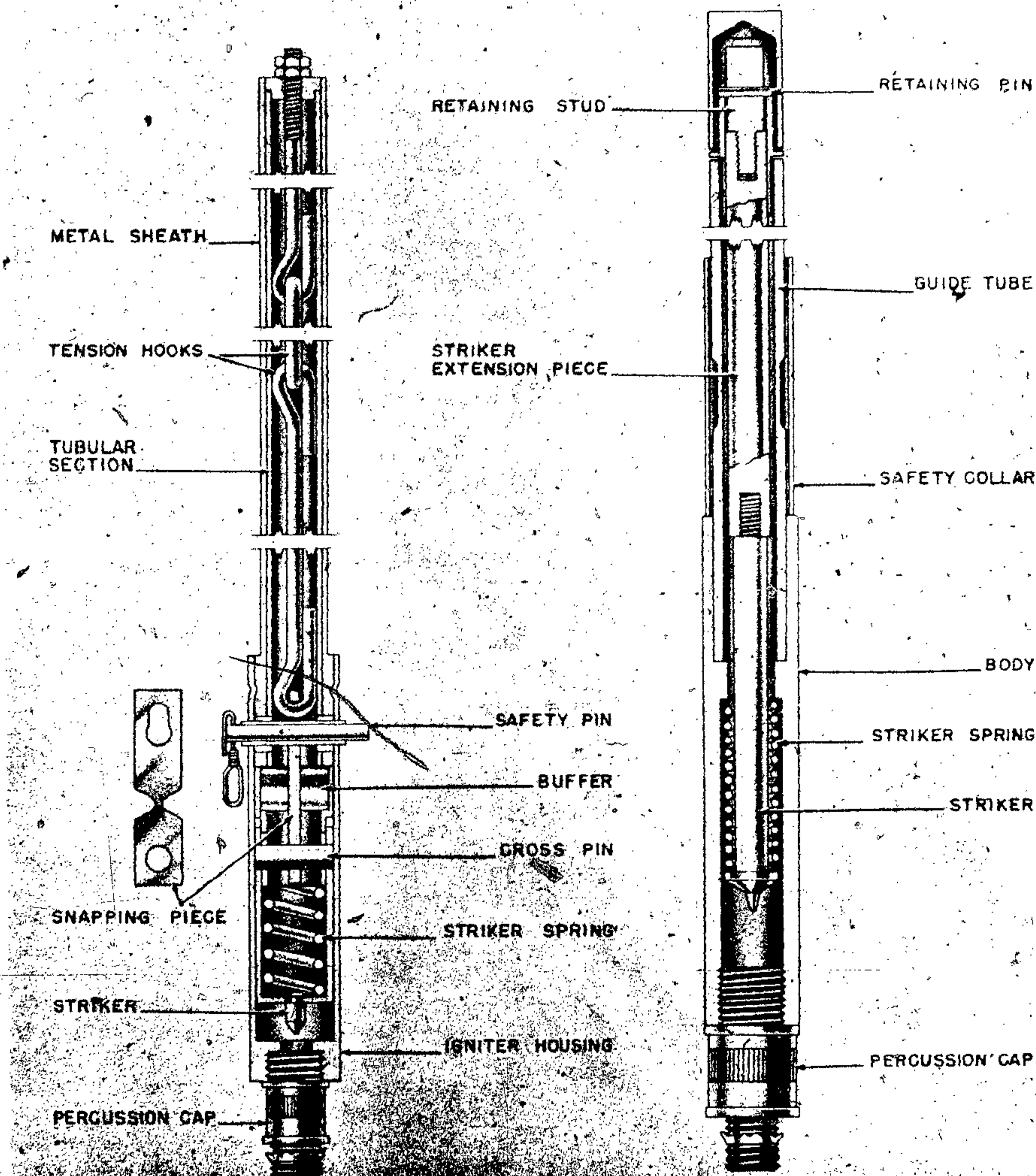
Figure 282—Knickzunder 43, Types I and II, Snap Type
