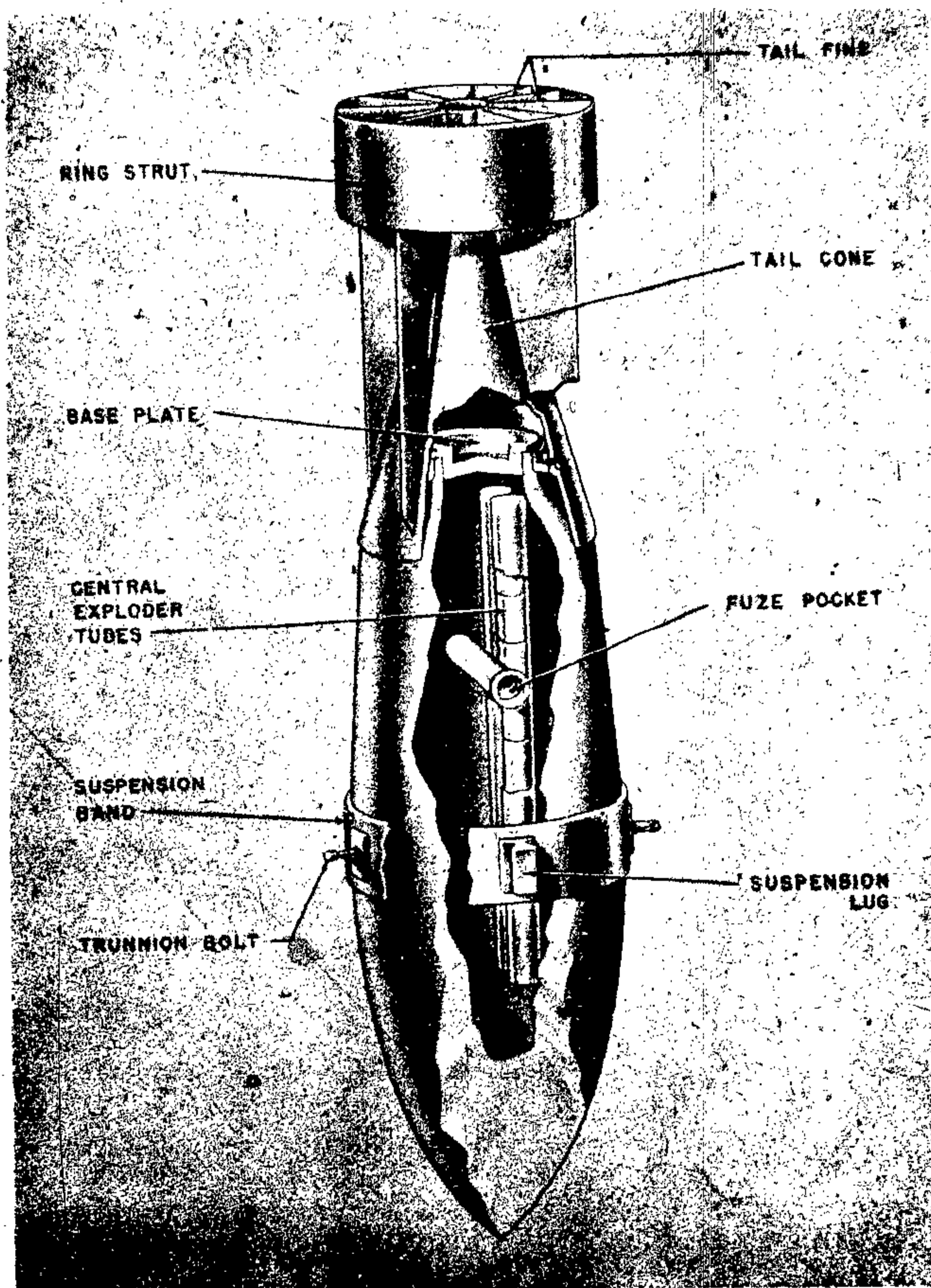
Figure 30—PC 1000-Kg Bomb
