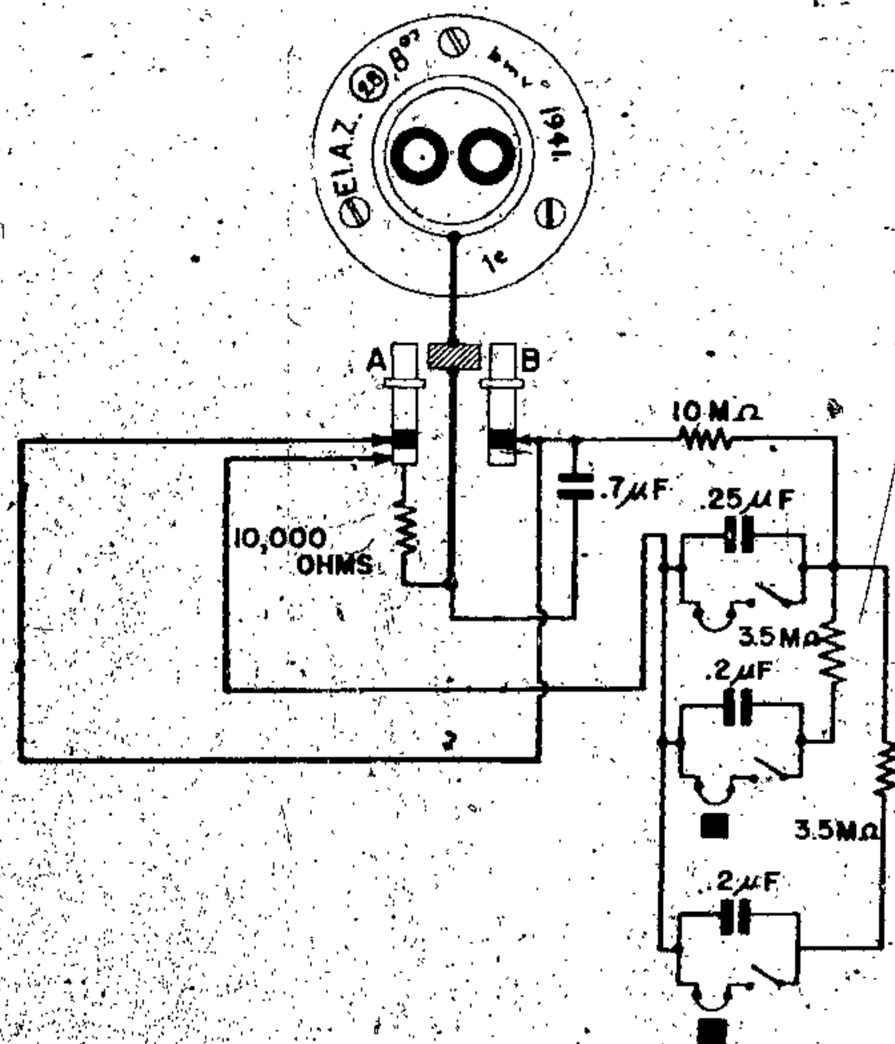
Figure 163—(28)B 07 Electrical Impact Fuze
