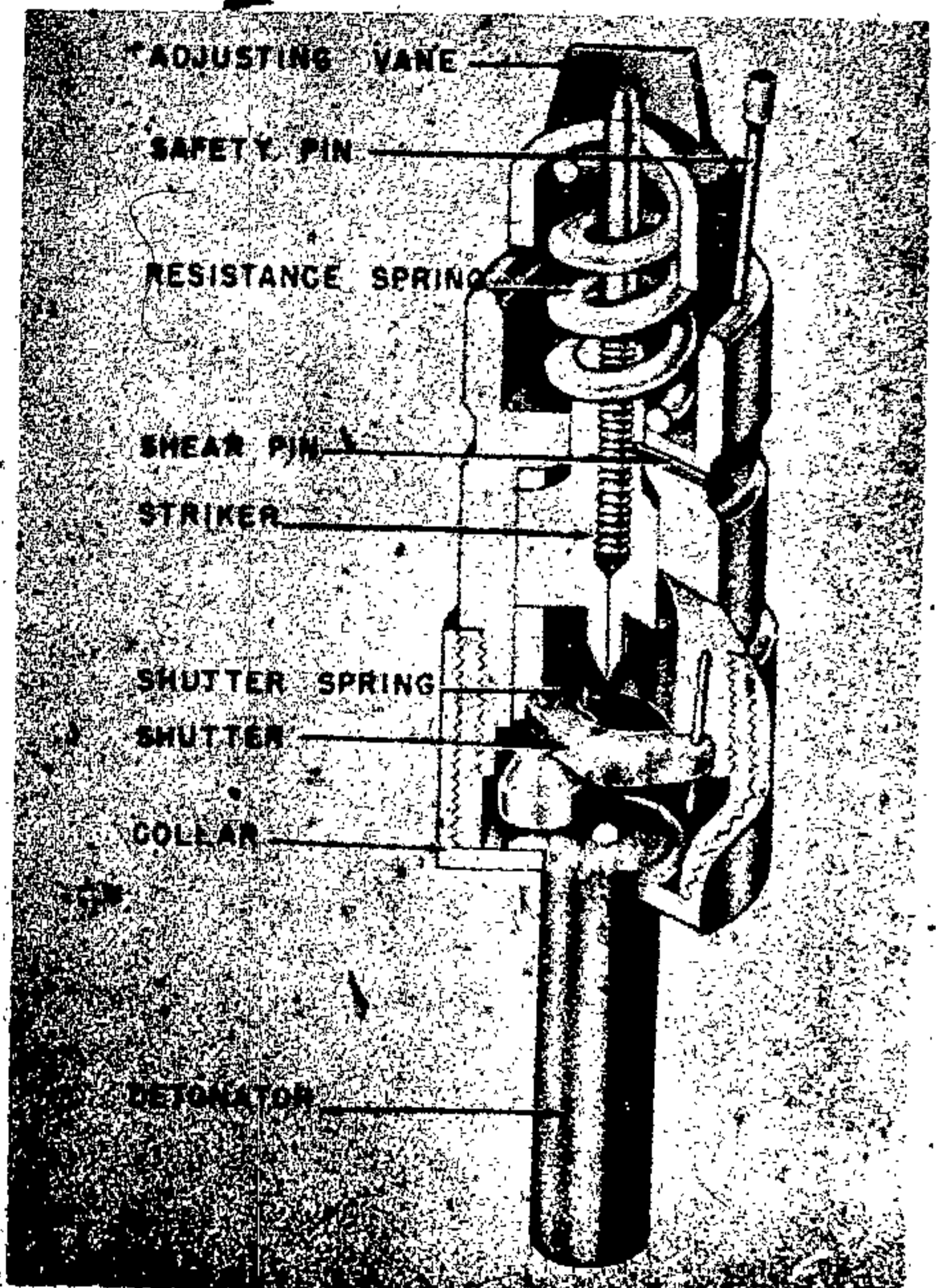
Figure 265—PX 32 Pressure Igniter
