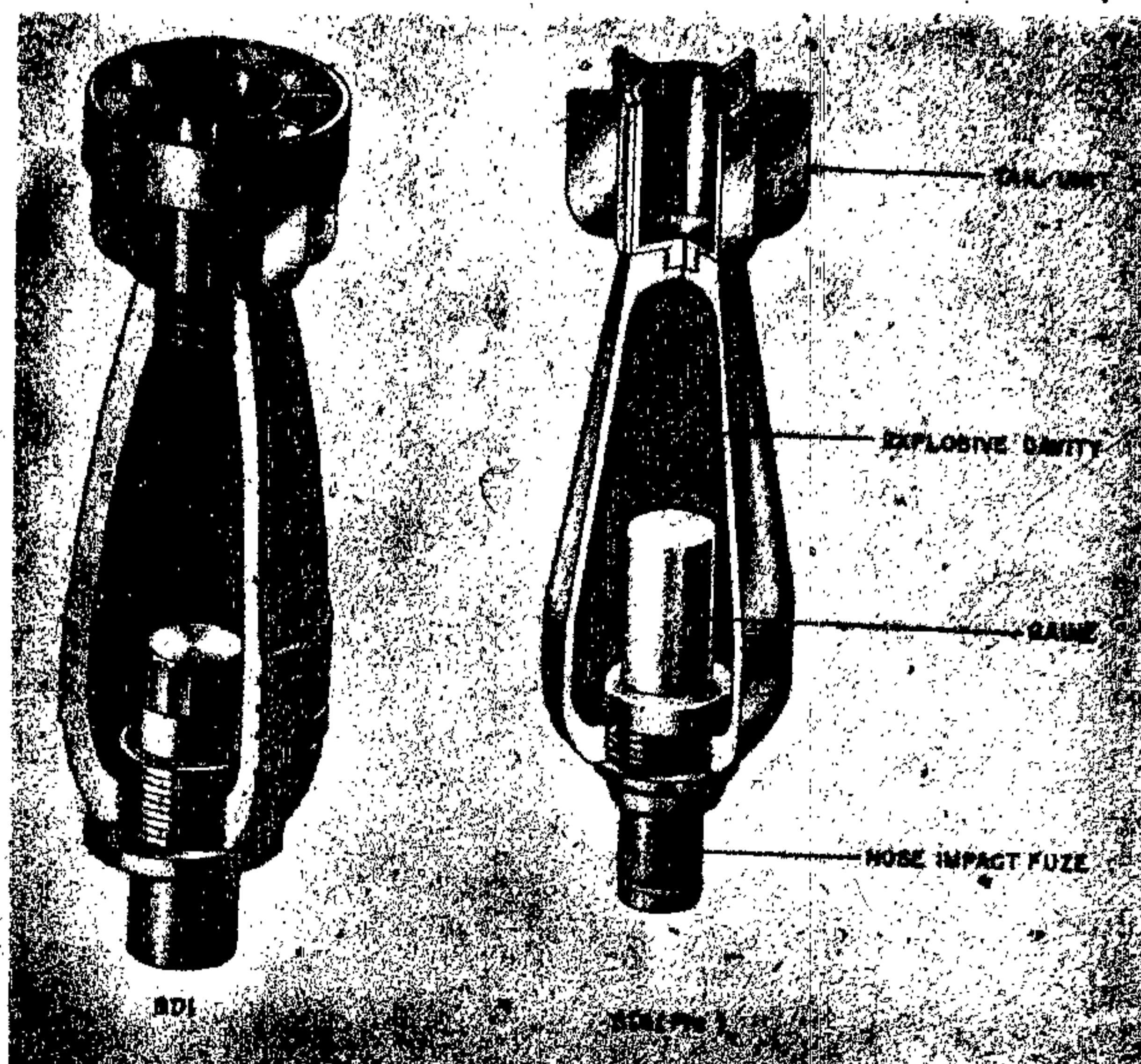
Figure 38—SD 1-Kg Mortar Bomb
