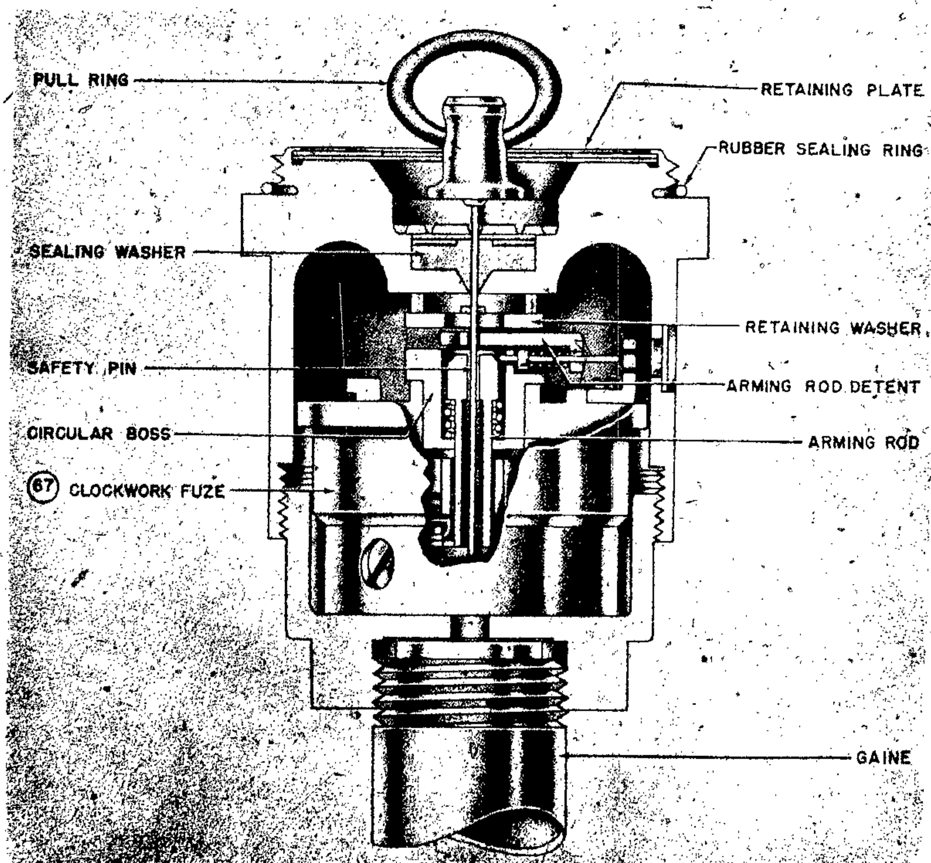
Figure 158—67/V Mechanical Clockwork Time Fuze
