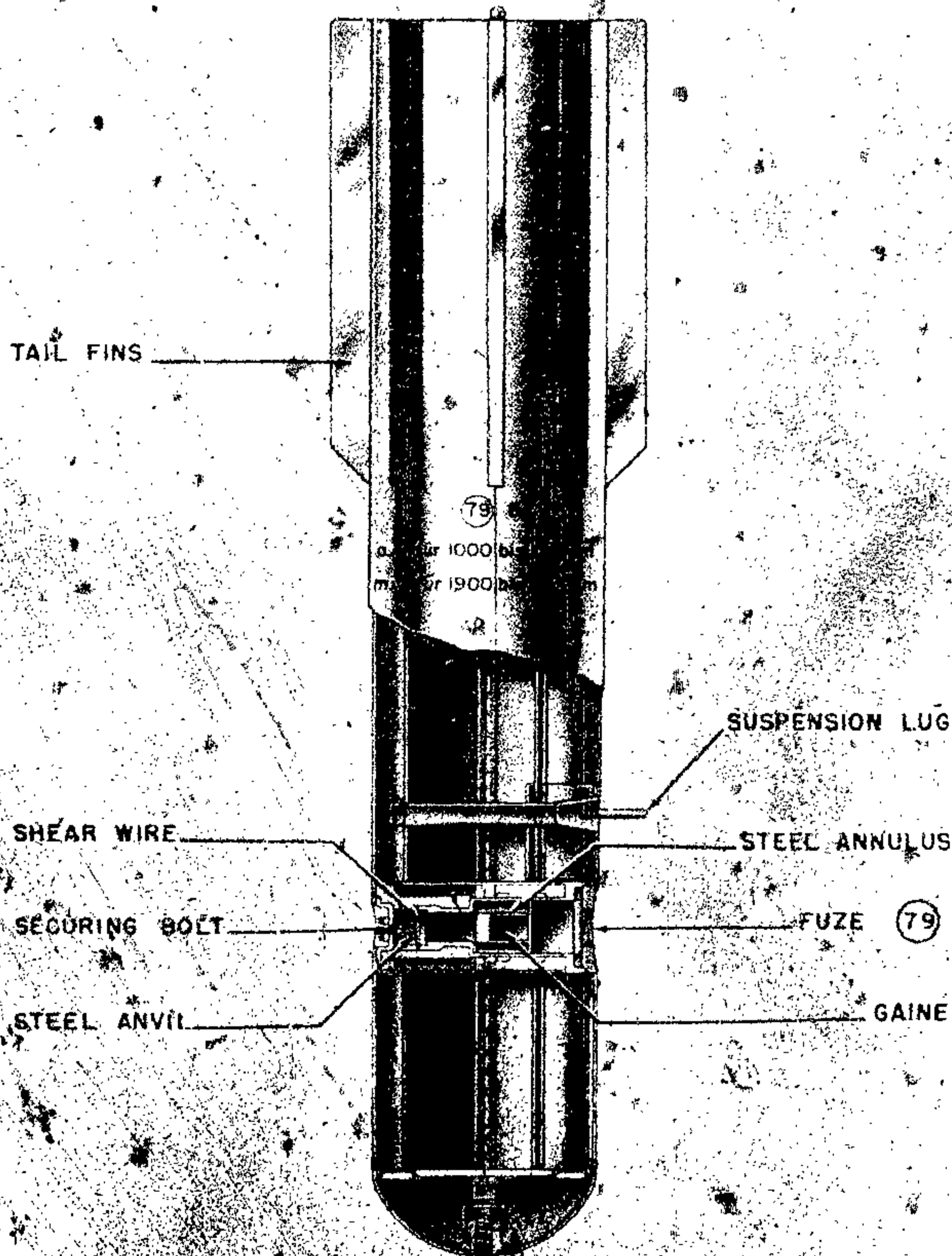
Figure 96—AB 23 SD 2 Container
