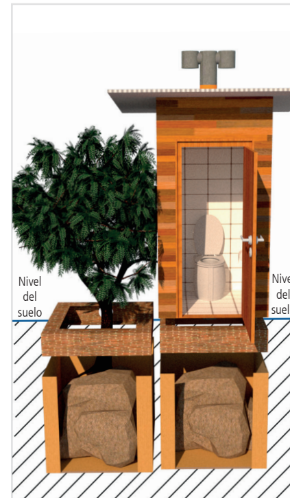
Fig.13: Vista frontal
