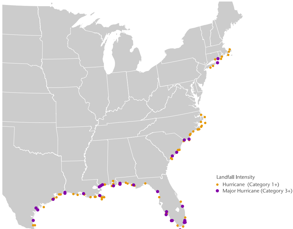
Exhibit 87: United States Hurricane & Major Hurricane Landfall Map
