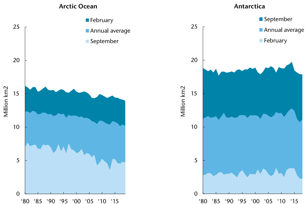
Exhibit 37: Global Sea Ice Extent 1980-2018
