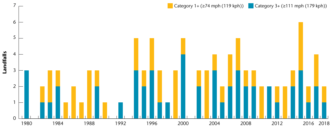
Exhibit 95: Southern Hemisphere Tropical Cyclone Landfalls
