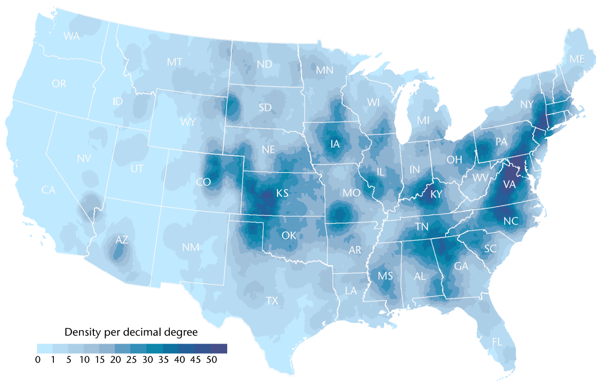
Exhibit 28: Density of 2018's Severe Weather Reports
