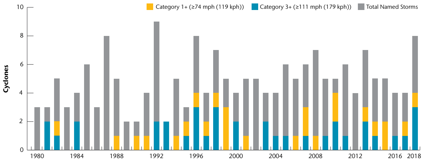
Exhibit 92: North Indian Basin Tropical Cyclone Activity
