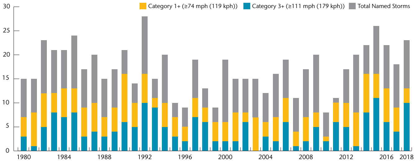
Exhibit 88: Eastern & Central Pacific Basin Tropical Cyclone Activity
