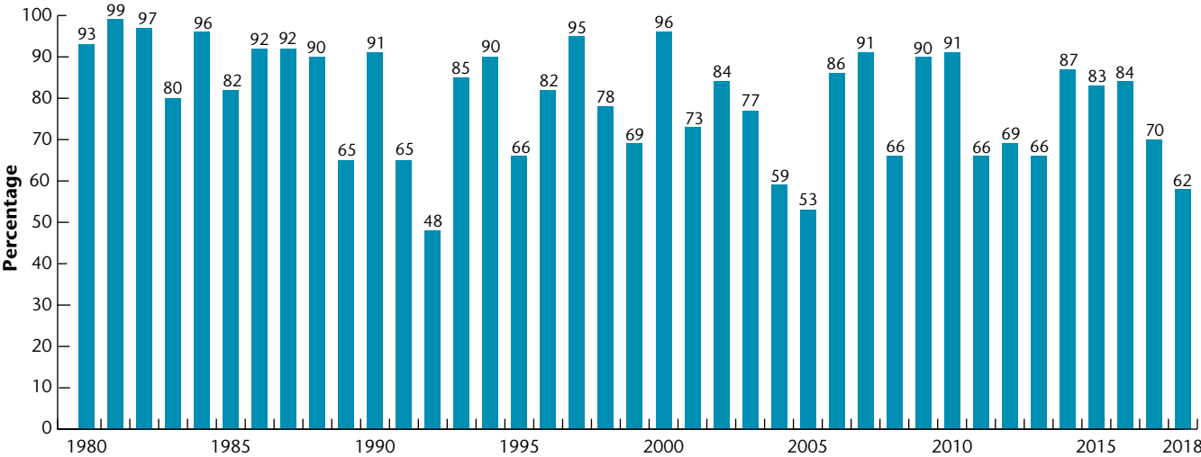
Exhibit 19: Global Protection Gap for Tropical Cyclones
