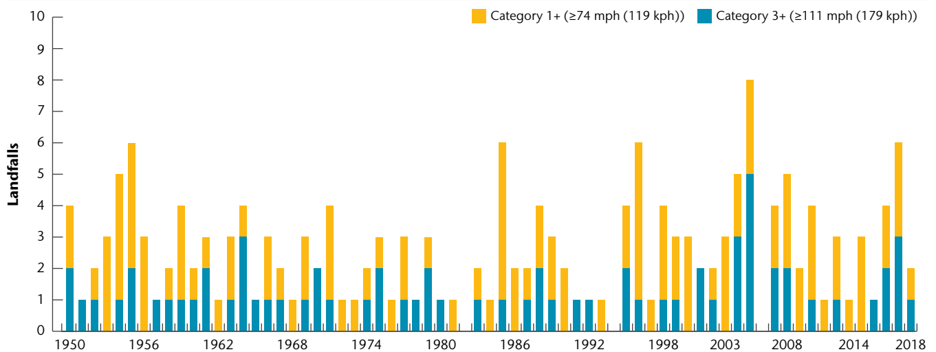
Exhibit 85: Atlantic Basin Hurricane & Major Hurricane Landfalls
