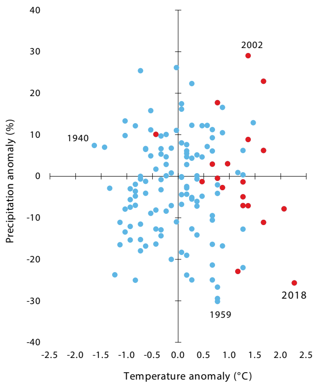
Exhibit 30: Annual Temperature and Precipitation Anomalies in Germany
