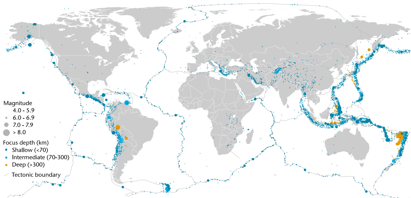
Exhibit 32: Global Earthquake Activity in 2018
