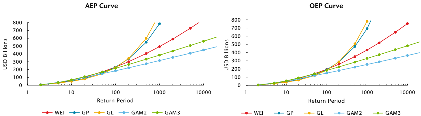
Exhibit 18: Example Exceedance Probability Curves
