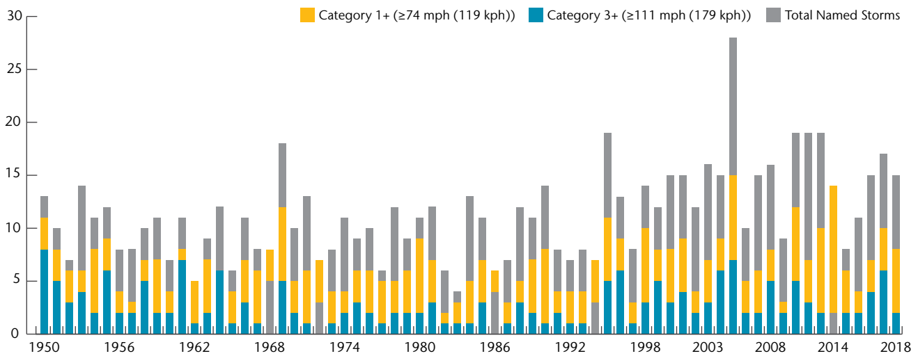
Exhibit 84: Atlantic Basin Tropical Cyclone Activity
