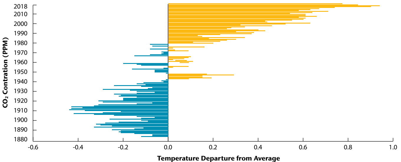
Exhibit 33: Global Land and Ocean Temperature Anomalies: 1880-2018
