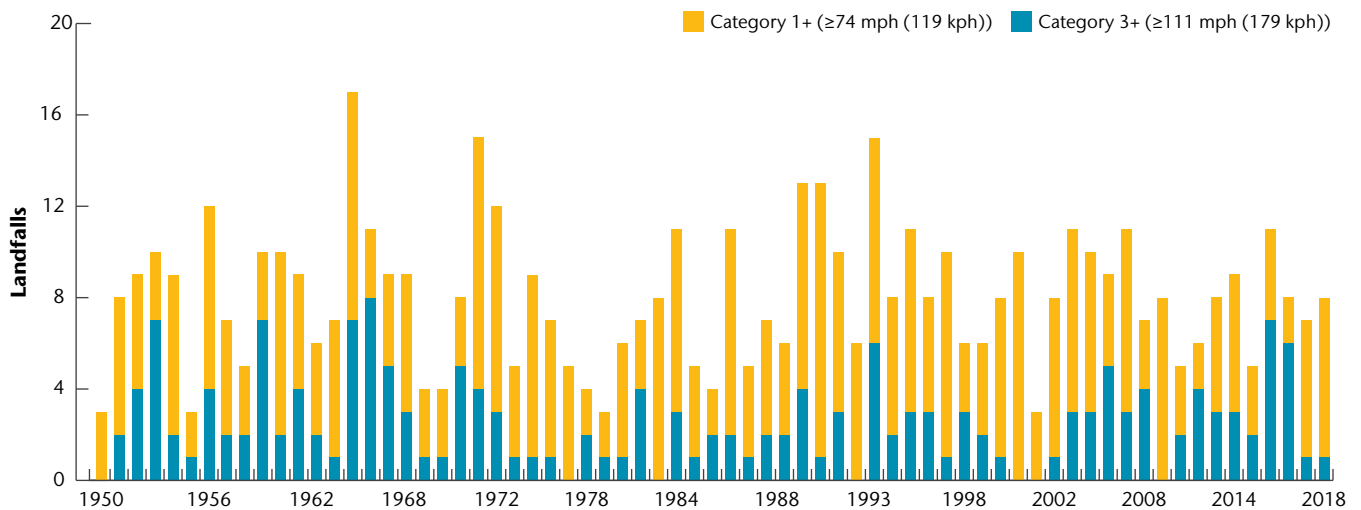
Exhibit 91: Western Pacific Basin Typhoon Landfalls
