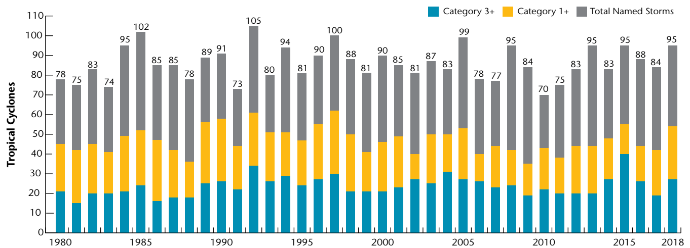
Exhibit 20: Global Tropical Cyclone Activity
