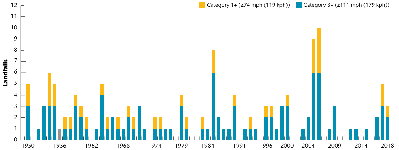
Exhibit 86: United States Hurricane & Major Hurricane Landfalls
