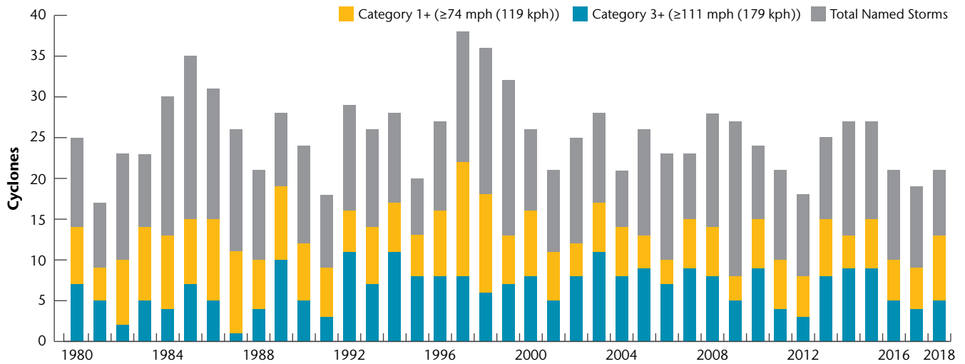
Exhibit 94: Southern Hemisphere Tropical Cyclone Activity
