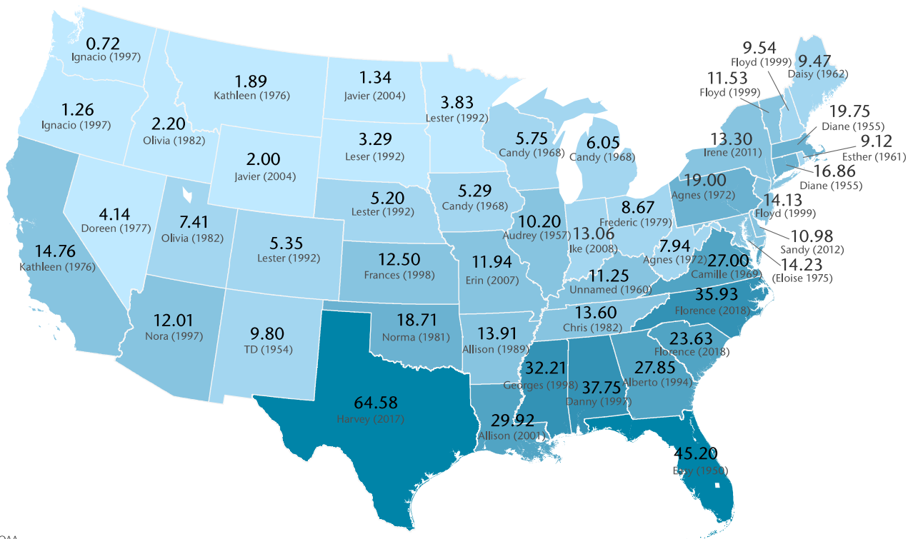
Exhibit 23: Maximum Tropical Cyclone Rainfall by State
