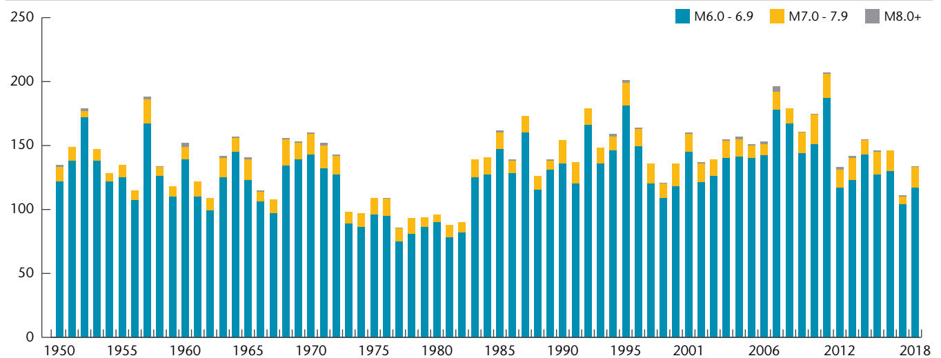
Exhibit 100: Global Earthquakes (M6.0+)
