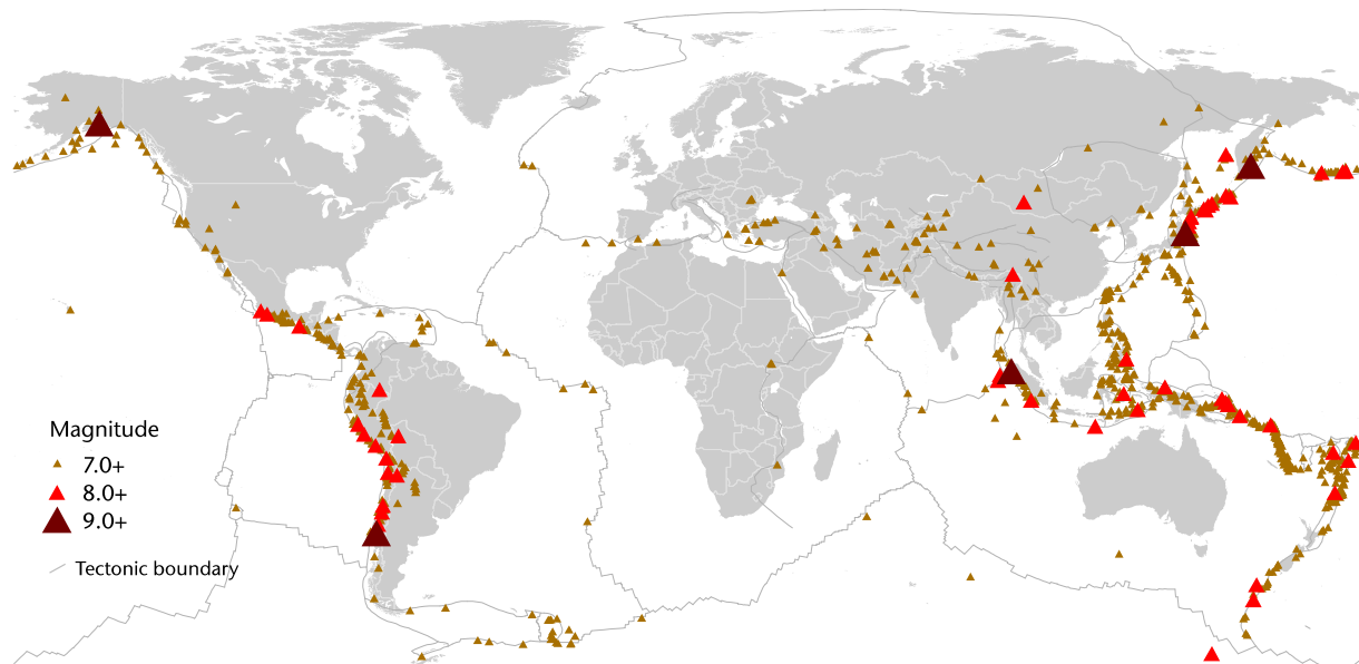
Exhibit 101: Global Earthquake Map; M6.0+ (1950-2018)
