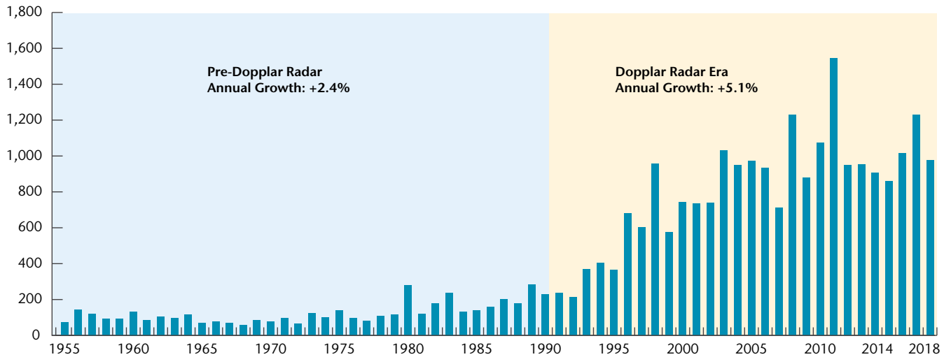
Exhibit 99: U.S. Damaging Wind Reports (75 mph or Greater)
