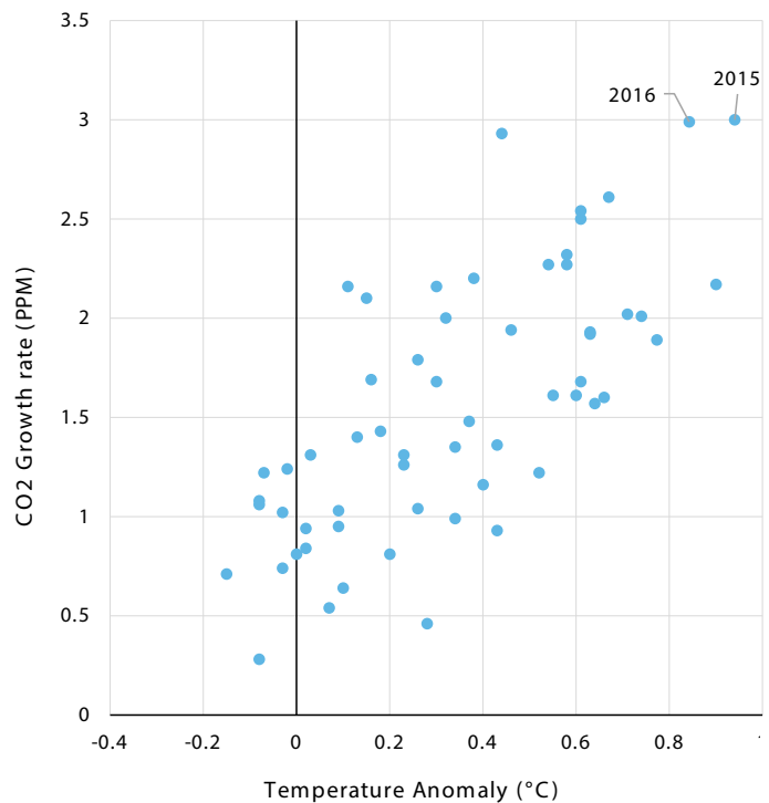
Exhibit 36: Average Atmospheric CO 2 Concentrations & CO 2 Growth Rate + Temperature Anomaly Plot (1960-2018)
