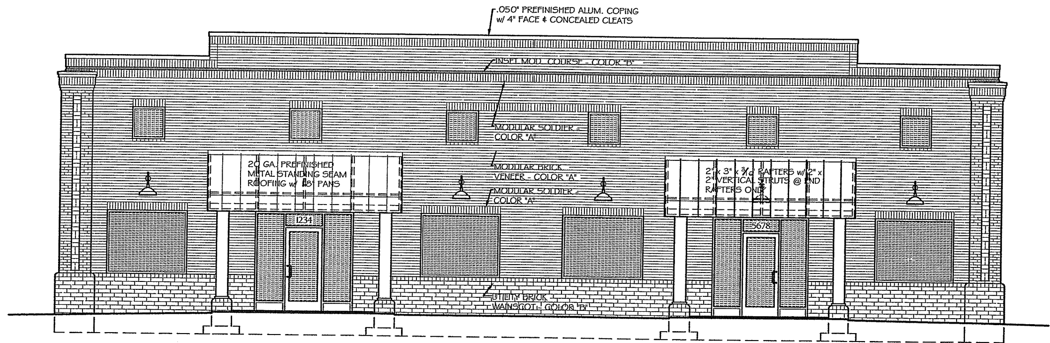
FRONT ELEVATION
