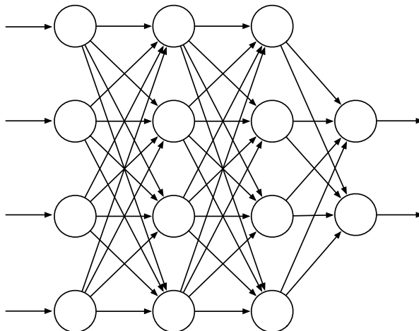
Figure 9.14: A generic feedforward neural network with four input units, two output units, and two hidden layers.
