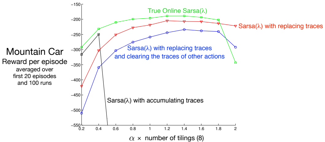
Figure 12.11: Summary comparison of Sarsa( \lambda ) algorithms on the Mountain Car task. True Online Sarsa( \lambda ) performed better than regular Sarsa( \lambda ) with both accumulating and replacing traces. Also included is a version of Sarsa( \lambda ) with replacing traces in which, on each time step, the traces for the state and the actions not selected were set to zero.
