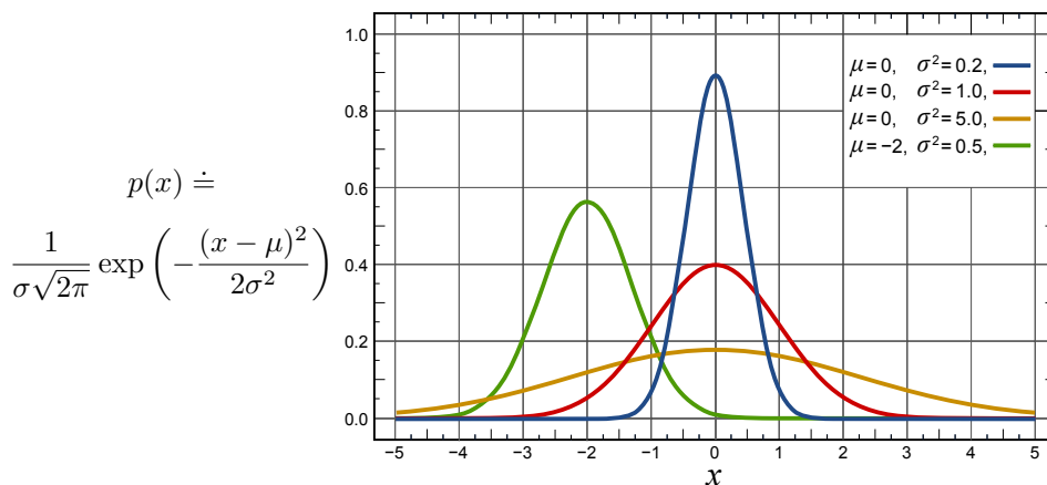
Figure 13.3: The probability density function of the normal distribution for different means and variances.
