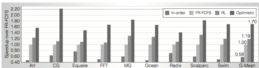
Figure 16.4: Performances of four controllers over a suite of 9 simulated benchmark applications. The controllers are: the simplest ‘in-order’ controller, FR-FCFS, the learning controller RL, and the unrealizable Optimistic controller which ignores all timing and resource constraints to provide a performance upper bound. Performance, normalized to that of FR-FCFS, is the inverse of execution time. At far right is the geometric mean of performances over the 9 benchmark applications for each controller. Controller RL comes closest to the ideal performance. ©2009 IEEE. Reprinted, with permission, from J. F. Martínez and E. İpek, Dynamic multicore resource management: A machine learning approach, Micro , IEEE, 29(5), p. 13.
