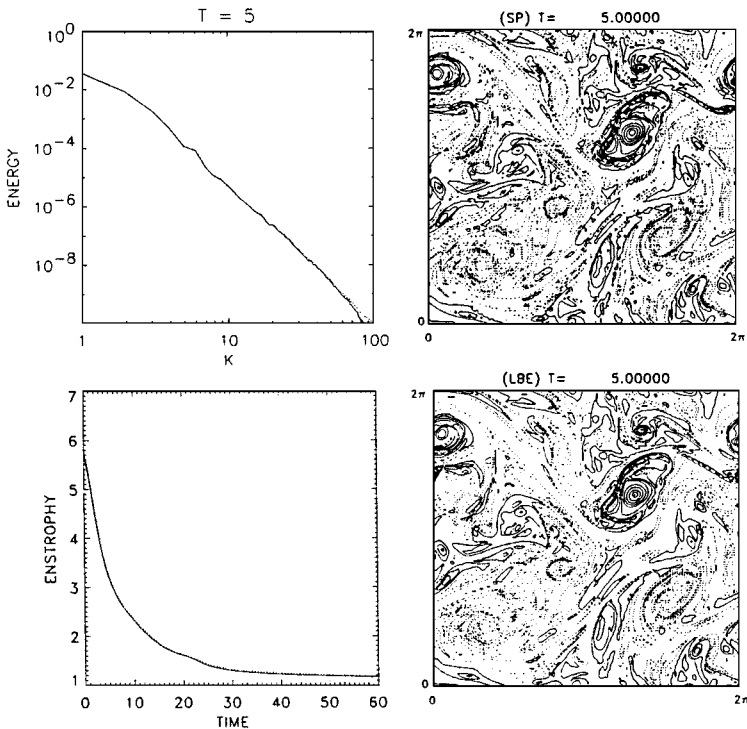
Figure 2 Velocity energy spectra versus wavenumber, k (top left). The entrophy of the system, \langle \omega^2 \rangle (bottom left), as a function of time. Right, a comparison of the vorticity distributions from a pseudospectral method and the LBM (Martinez et al 1994).
