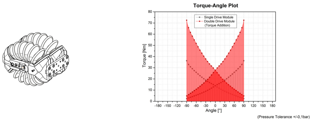
Figure 33. Double Module - Parallel Configuration
