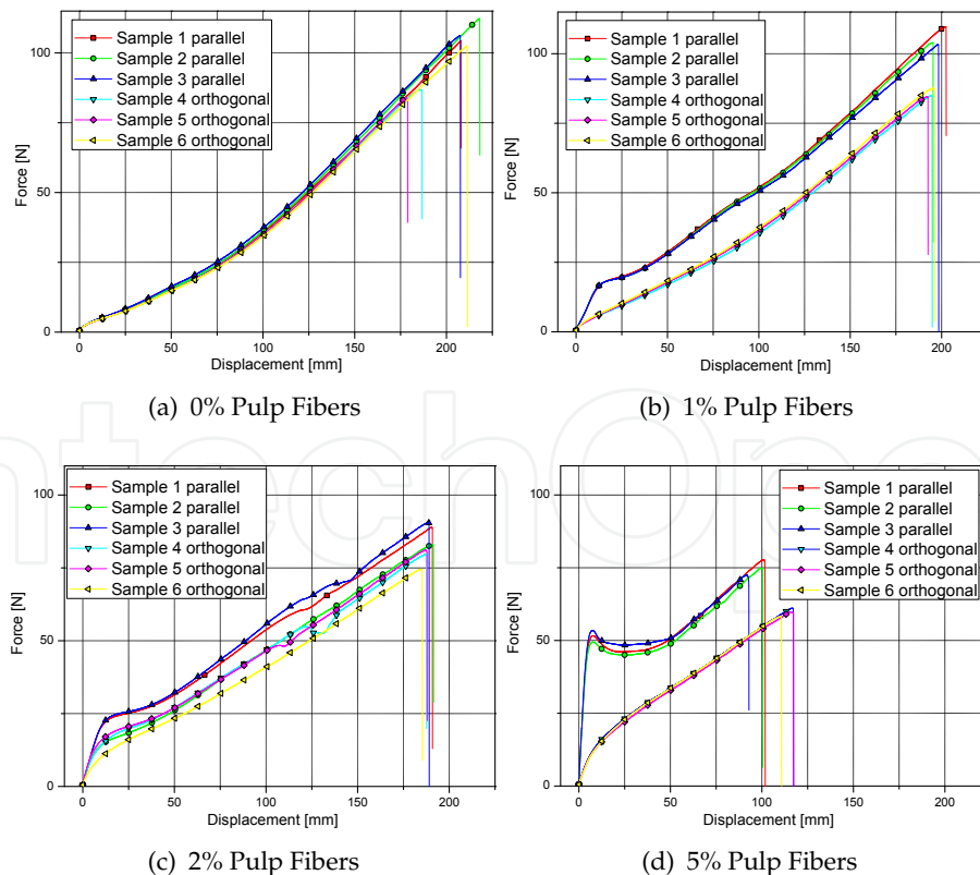
Figure 14. Force-Displacement Plots for different Pulp Fiber Concentrations
