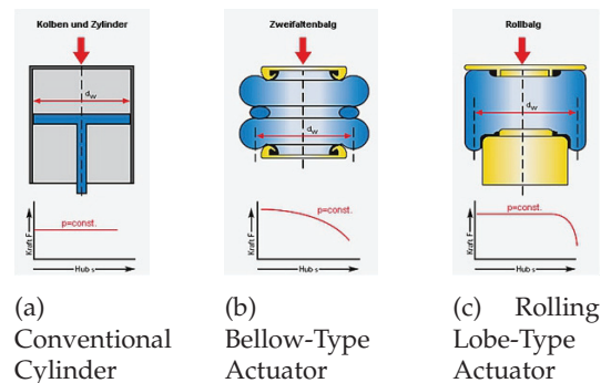
Figure 1. Comparison of Different Kinds of Expansion Actuators [17]
