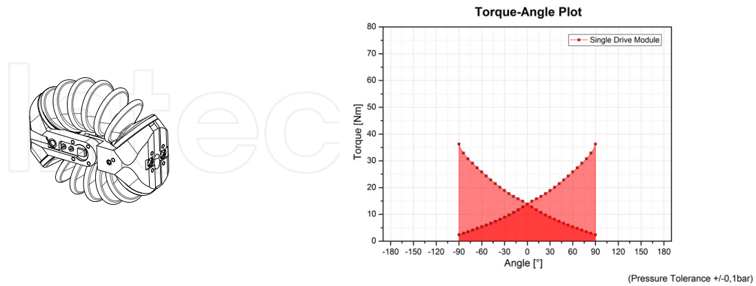
Figure 32. Single Drive Module
