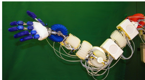
(b) 6-DOF GPA-Arm
