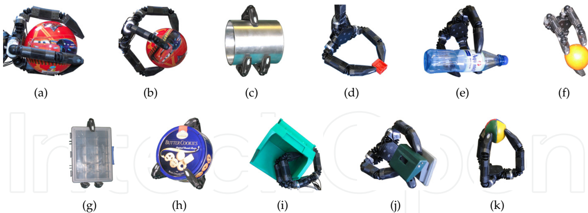
Figure 36. Grasp Taxonomy of the Composite Gripper
