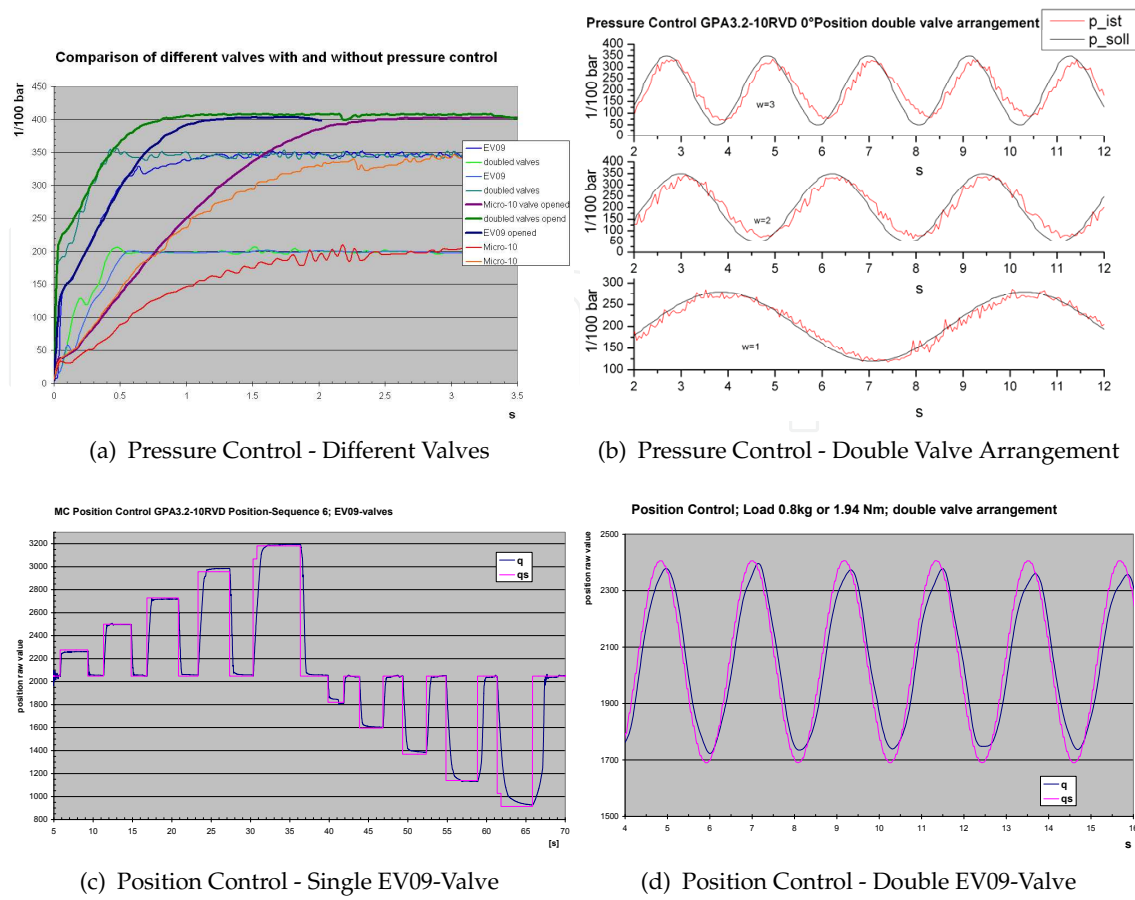
Figure 26. Results of Embedded Control using Switching Valves
