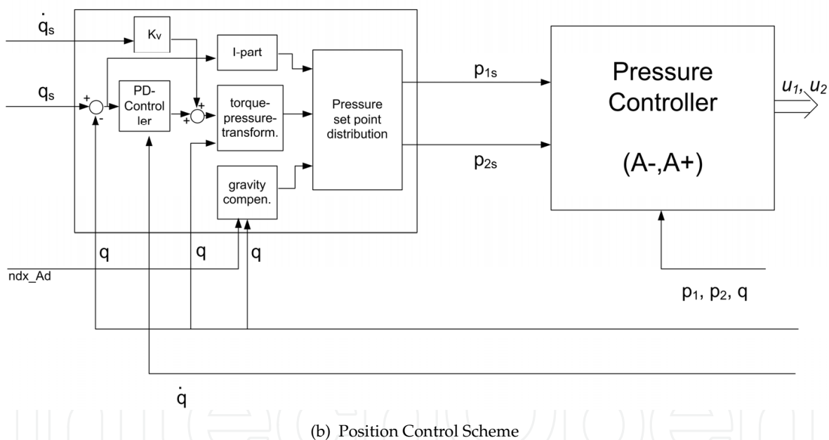
Figure 27. Different Control Schemes
