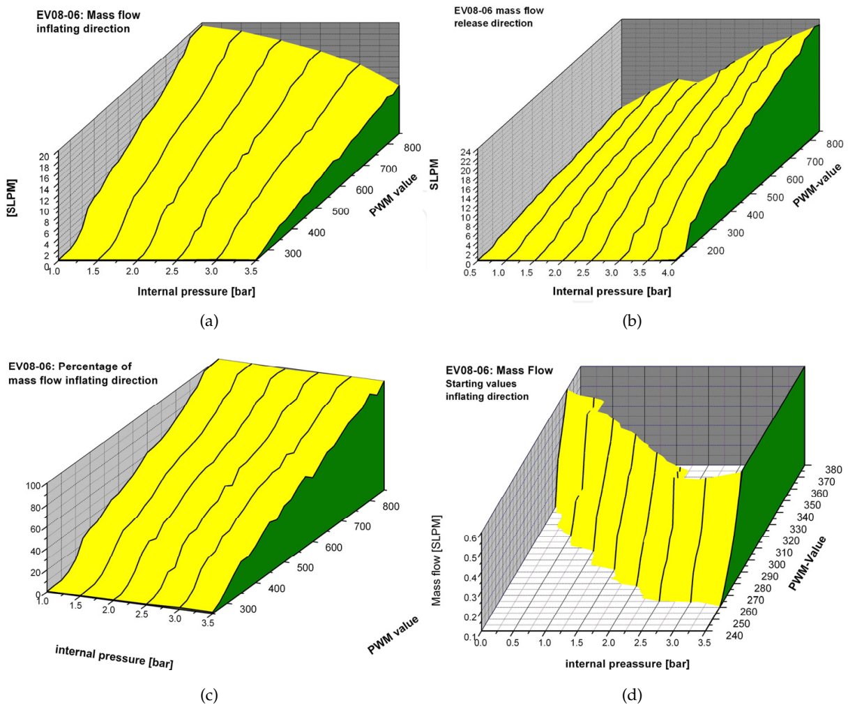
Figure 25. Flow Characteristics of an EV08-Switching Valve
