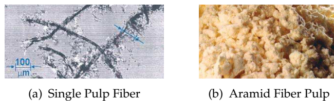
Figure 12. Morphology of Fiber Pulps
