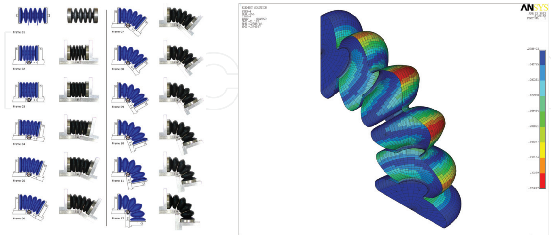
(a) Strain Analysis of a Flexible Fluidic Actuator ( \varnothing 18\text{mm} ), FEM-Model vs. Real Actuator
