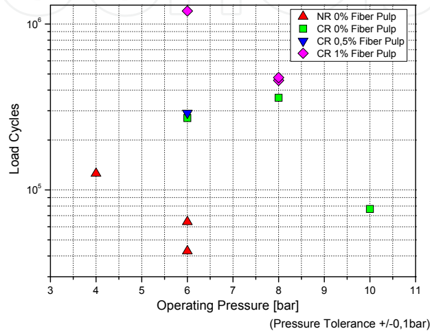
Figure 16. Fatigue Resistance of 18 mm -Actuators
