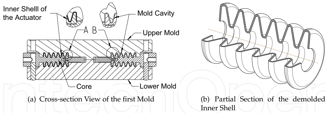
Figure 10. First Fabrication Step
