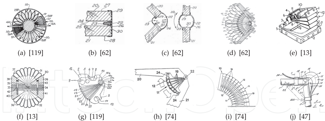
Figure 2. Radial Cross-Section View of Different Fluidic “Expansion” Drives
