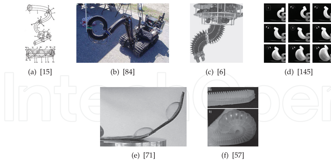
Figure 6. Trunk-Like Bending Actuators and Monolithic Bending Actuators
