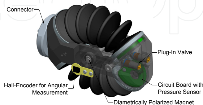
Figure 31. Highly Integrated Flexible Fluidic Drive Module
