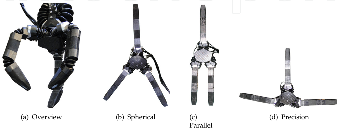
Figure 35. Main Base Positions of the Composite Gripper
