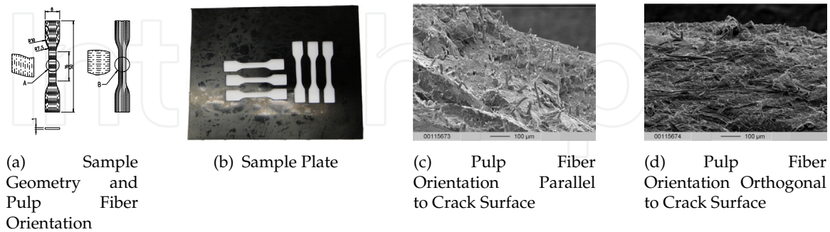
Figure 13. Material Characterization
