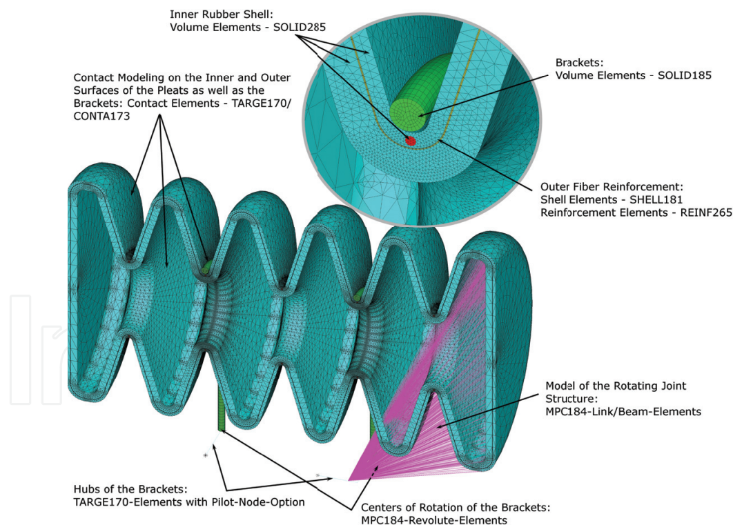
Figure 20. Set-up of the FEM-Model for a Flexible Fluidic Actuator
