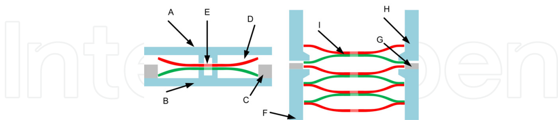
Figure 15. (A) upper welding electrode, (B) lower welding electrode, (C) centering coil, (D) two foil pieces, (E) hole for air passage, (F) lower welding electrode with undercut, (G) centering coil, (H) upper welding electrode with undercut, (I) foil segments from first step
