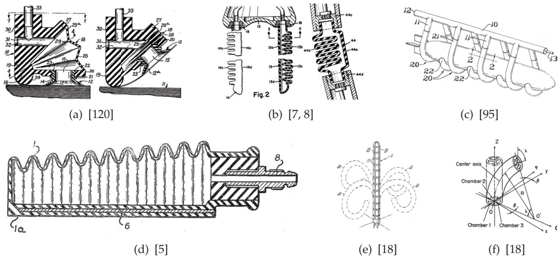
Figure 5. Bending Actuators
