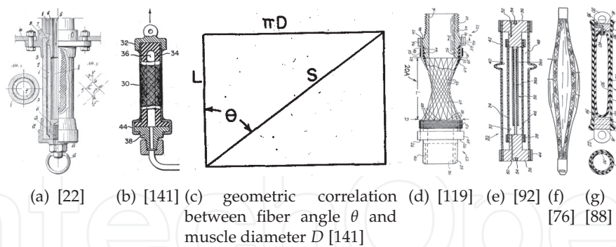
Figure 3. Different Fluidic Muscles
