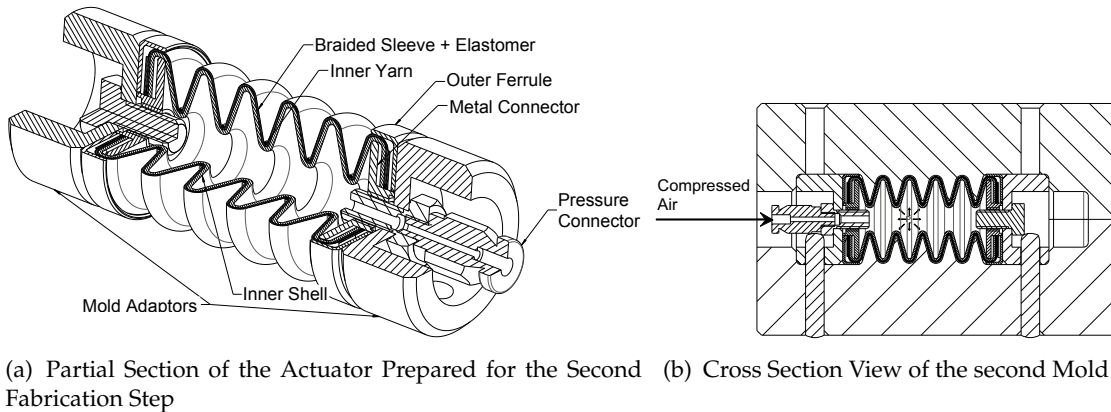
Figure 11. Second Fabrication Step
