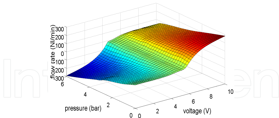
Figure 23. Experimentally determined flow map for the servo-valve Festo MPYE-5-1/8LF-010-B.
