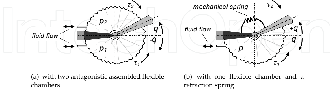
Figure 22. Working principle of a fluidic actuated rotary robotic joint
