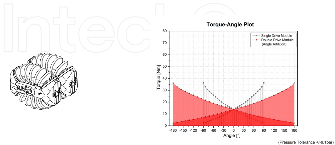
Figure 34. Double Module - Serial Configuration
