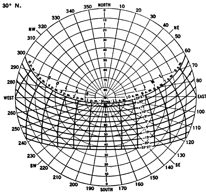
Figure 54.—Solar altitude and azimuth for selected days of the year at 30 degrees north latitude.
