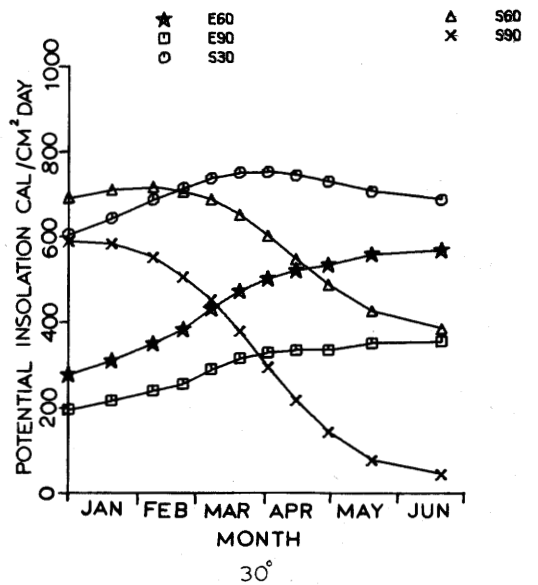
Figure 44.—Isograms of daily values of direct solar radiation on east 60-, east 90-, south 30-, south 60-, and south 90-degree slopes at 30 degrees north latitude.
