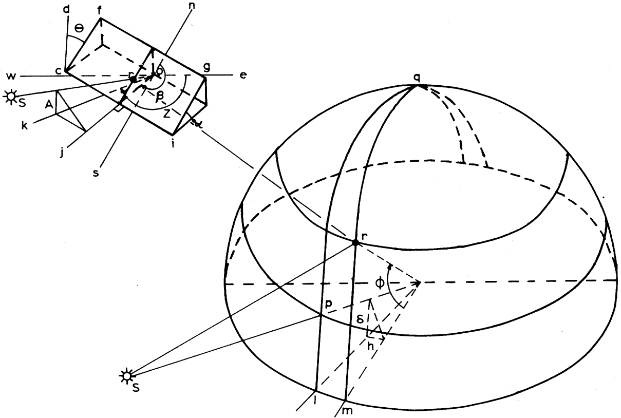
Figure 1.—Illustration of the angles necessary for the theoretical calculations of solar radiation on a particular surface in the Northern Hemisphere.
