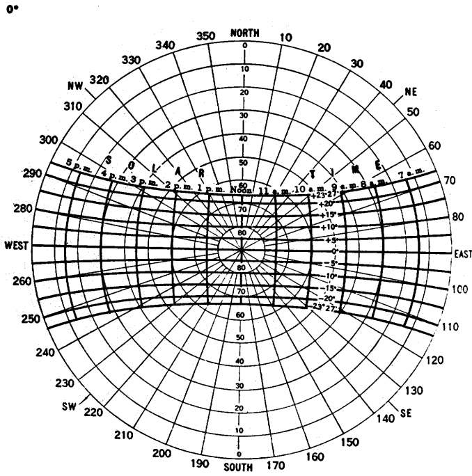
Figure 51.—Solar altitude and azimuth for selected days of the year at 0 degrees north latitude.
