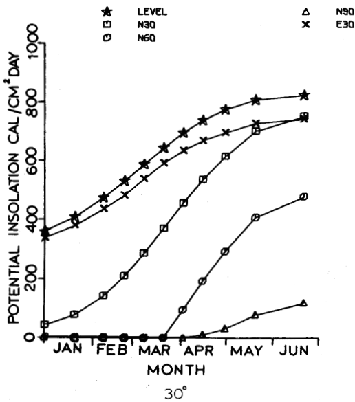
Figure 43.—Isograms of daily values of direct solar radiation on level, north 30-, north 60-, north 90-, and east 30-degree slopes at 30 degrees north latitude.
