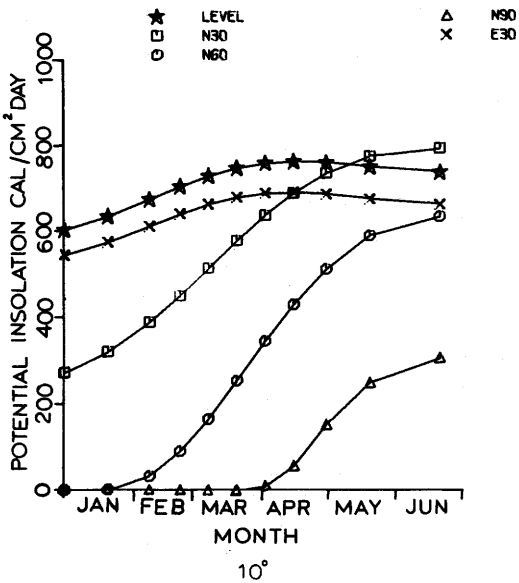
Figure 39.—Isograms of daily values of direct solar radiation on level, north 30-, north 60-, north 90-, and east 30-degree slopes at 10 degrees north latitude.
