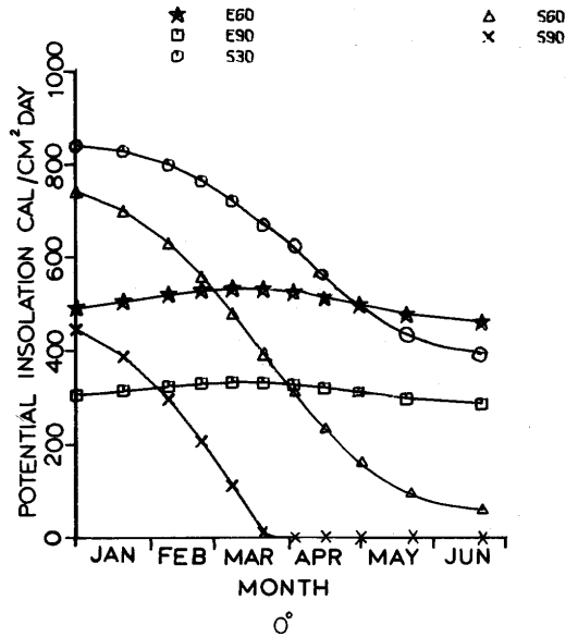
Figure 38.—Isograms of daily values of direct solar radiation on east 60-, east 90-, south 30-, south 60-, and south 90-degree slopes at 0 degrees north latitude.
