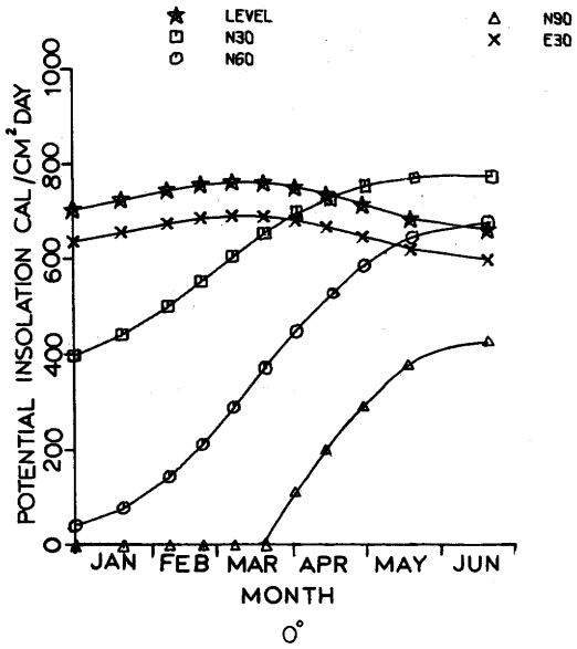
Figure 37.—Isograms of daily values of direct solar radiation on level, north 30-, north 60-, north 90-, and east 30-degree slopes at 0 degrees north latitude.
