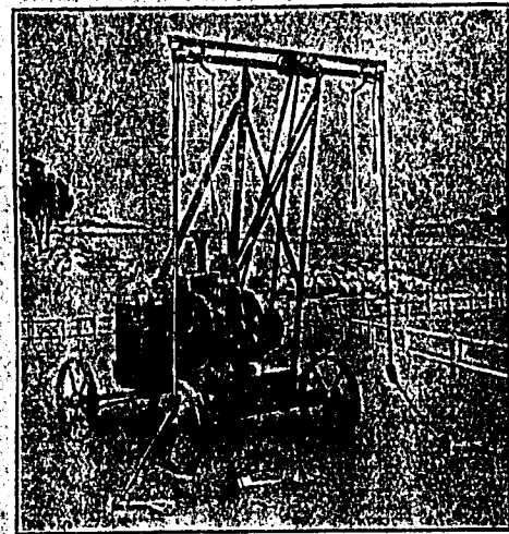
Illustration of the latest 2 Stand Improved "WOLSELEY" Crutching and Shearing Plant driven by 2 h.p. Triumph Engine
