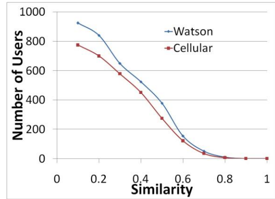
Fig 12 Similarity of user profiles (based on data accesses)
