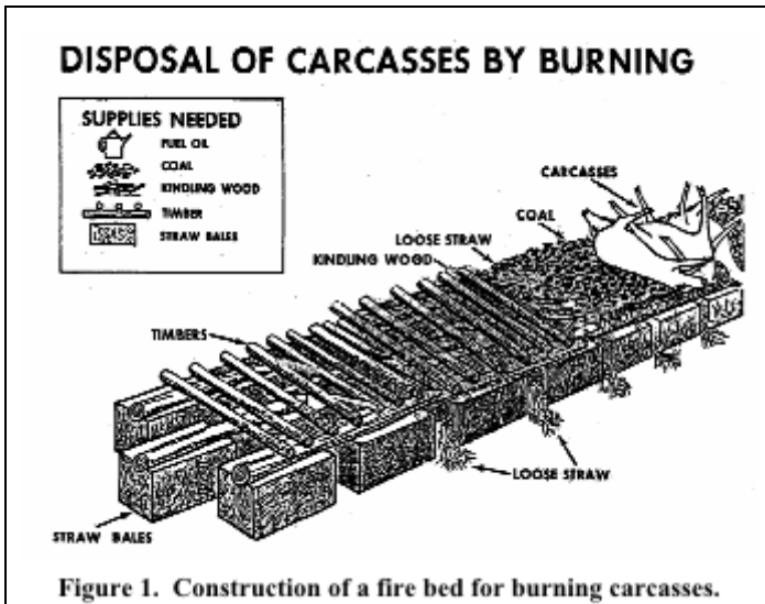
Figure 1. Construction of a fire bed for burning carcasses.
