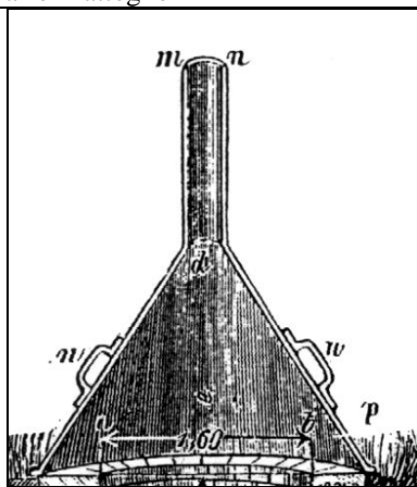
Illustration 12.10: Funnel and “chimney” of the Feist oven.
