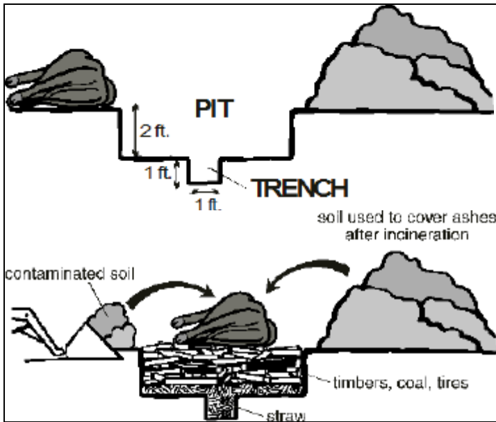
Illustrations 12.25 and 12.26: Cremation pit for animal carcass.
