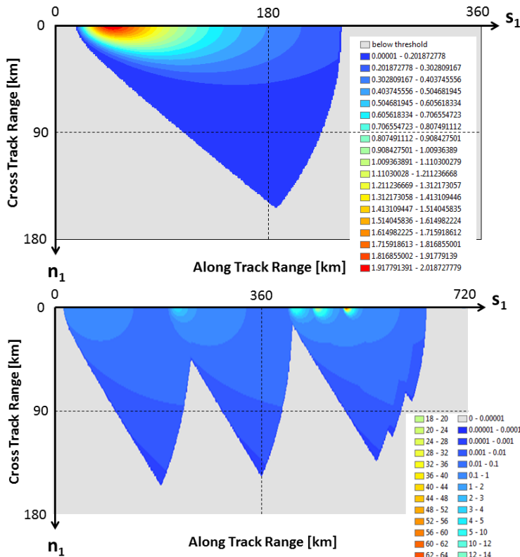
Figure 14. Apollo 17 LM descent engine deposition rate [ \text{g km}^{-2} \text{sec}^{-1} ] for 1 sec at start of braking at t=0 sec (LM at upper left). The distance cross track is shown from 0 (top) to 180 km (bottom).
