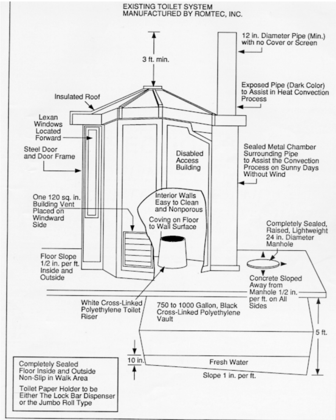
Figure 3. Vault Toilet
