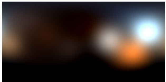
(d) Progressive least-squares encoding using 12 spherical Gaussian lobes (RMSE: 0.455971).
