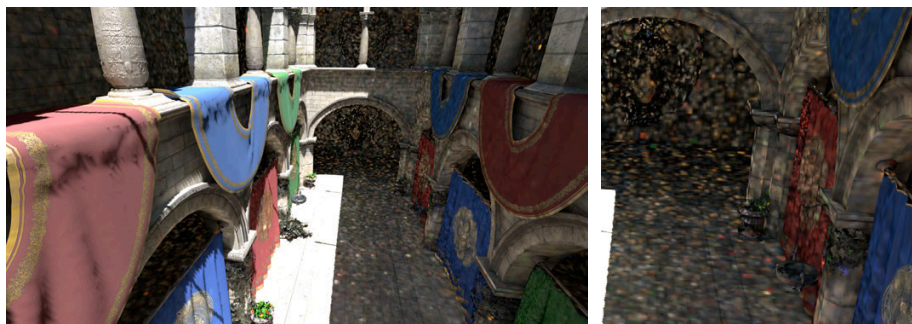
(b) Correlated Multi-Jittered sample sequence [70]
