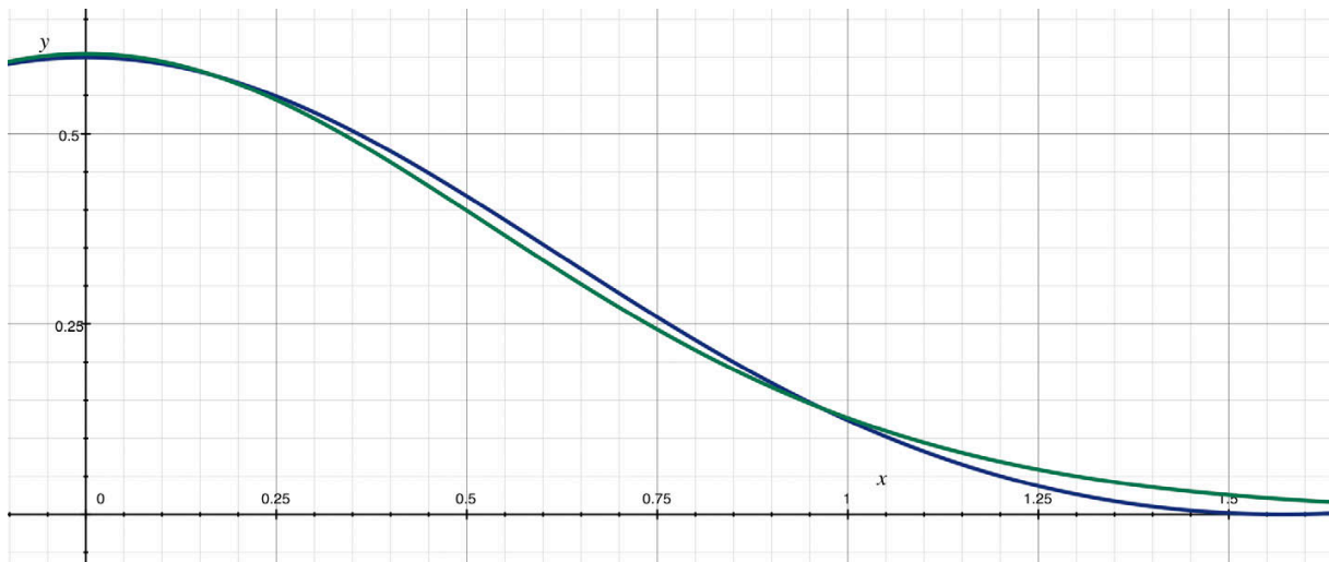
Figure 8.1: A spherical Gaussian lobe with \lambda = 3.4 (green) against the cosine-lobe variant of Ambient Dice (blue).
