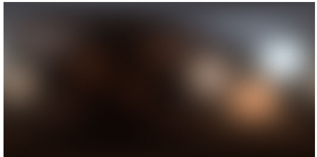
(b) Naïve projection onto 12 spherical Gaussian lobes (RMSE: 0.470525).
