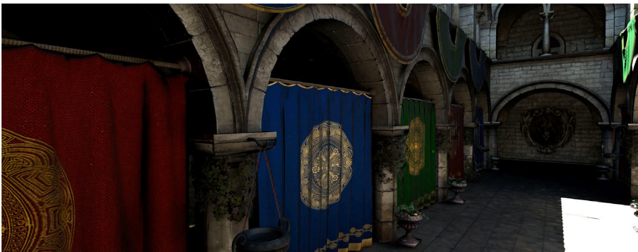
(b) Non-negative spherical Gaussians (12 lobes, \lambda = 8 )
