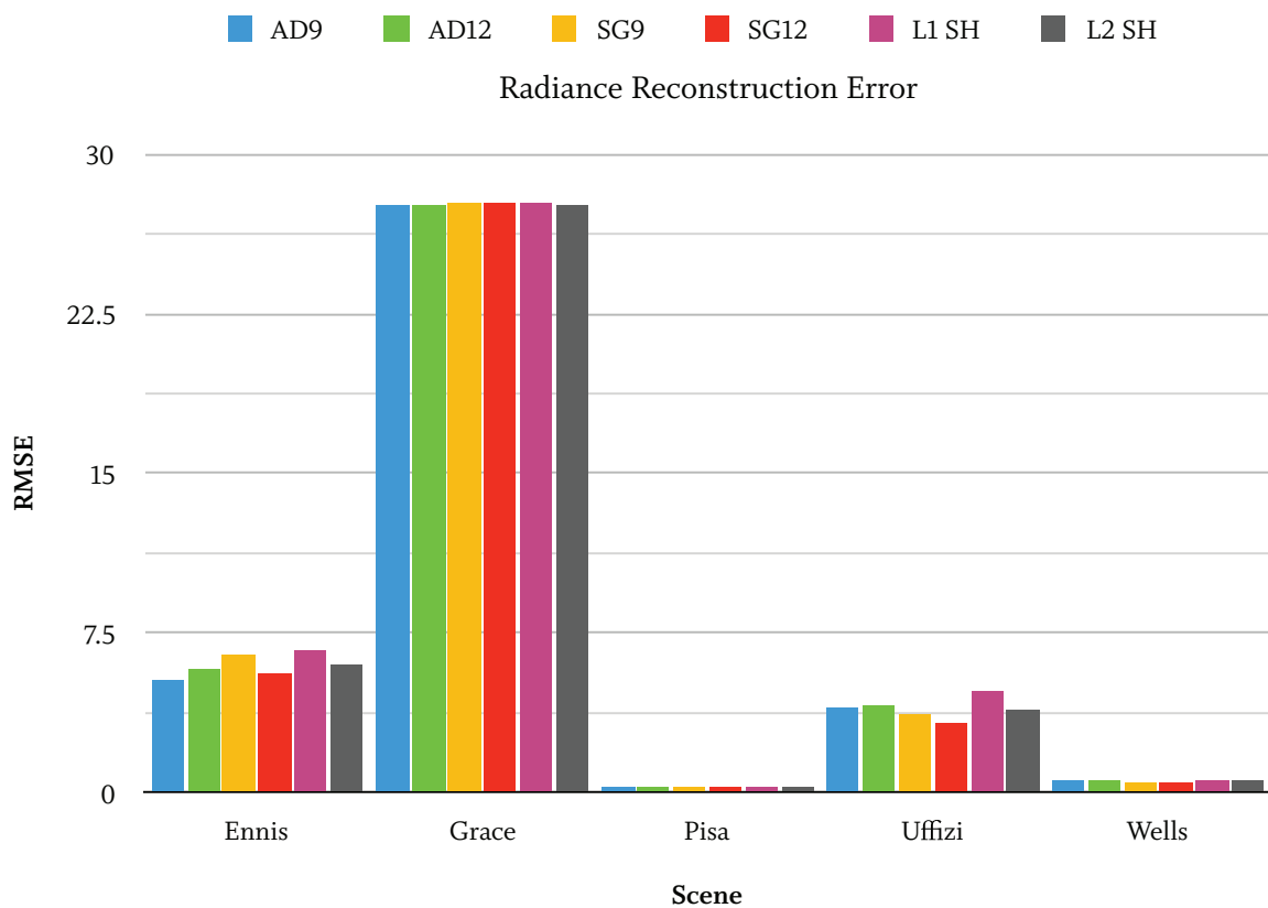
Figure C.6: Comparison graphs of reconstruction error for spherical harmonics, spherical Gaussians, and cosine-lobe Ambient Dice
