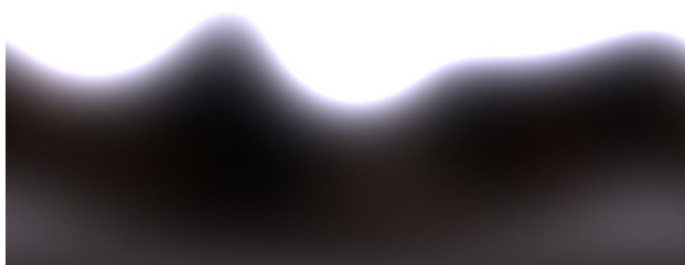
(c) A non-negative least-squares fit using 12 spherical Gaussian lobes (RMSE: 3.13181).
