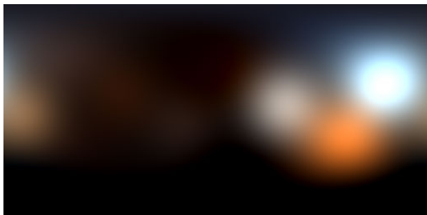
(c) A least-squares fit with 12 spherical Gaussian lobes (RMSE: 0.455862).
