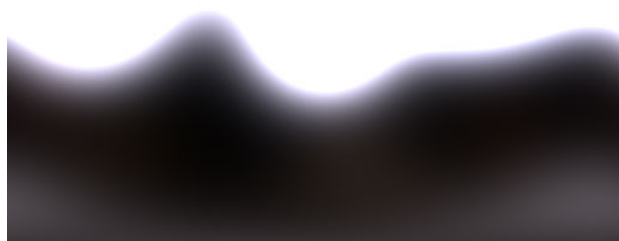
(d) Progressive non-negative least-squares encoding using 12 spherical Gaussian lobes (RMSE: 3.13928).
