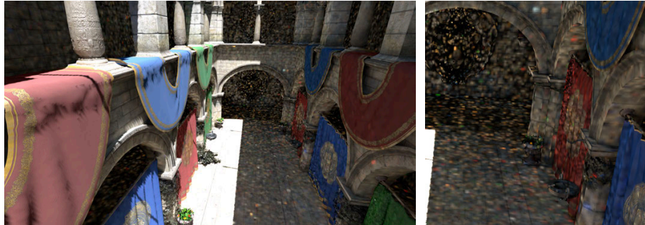
(c) Sobol sample sequence [71]
