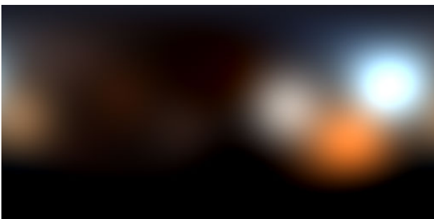
(a) Progressive least-squares encoding with samples from the Halton 2-3 sequence.
