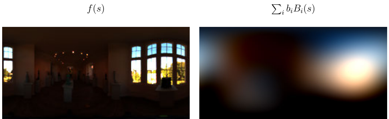
Figure 7.1: Approximation of the Wells HDR environment map [85] with the Ambient Dice SRBF basis functions.
