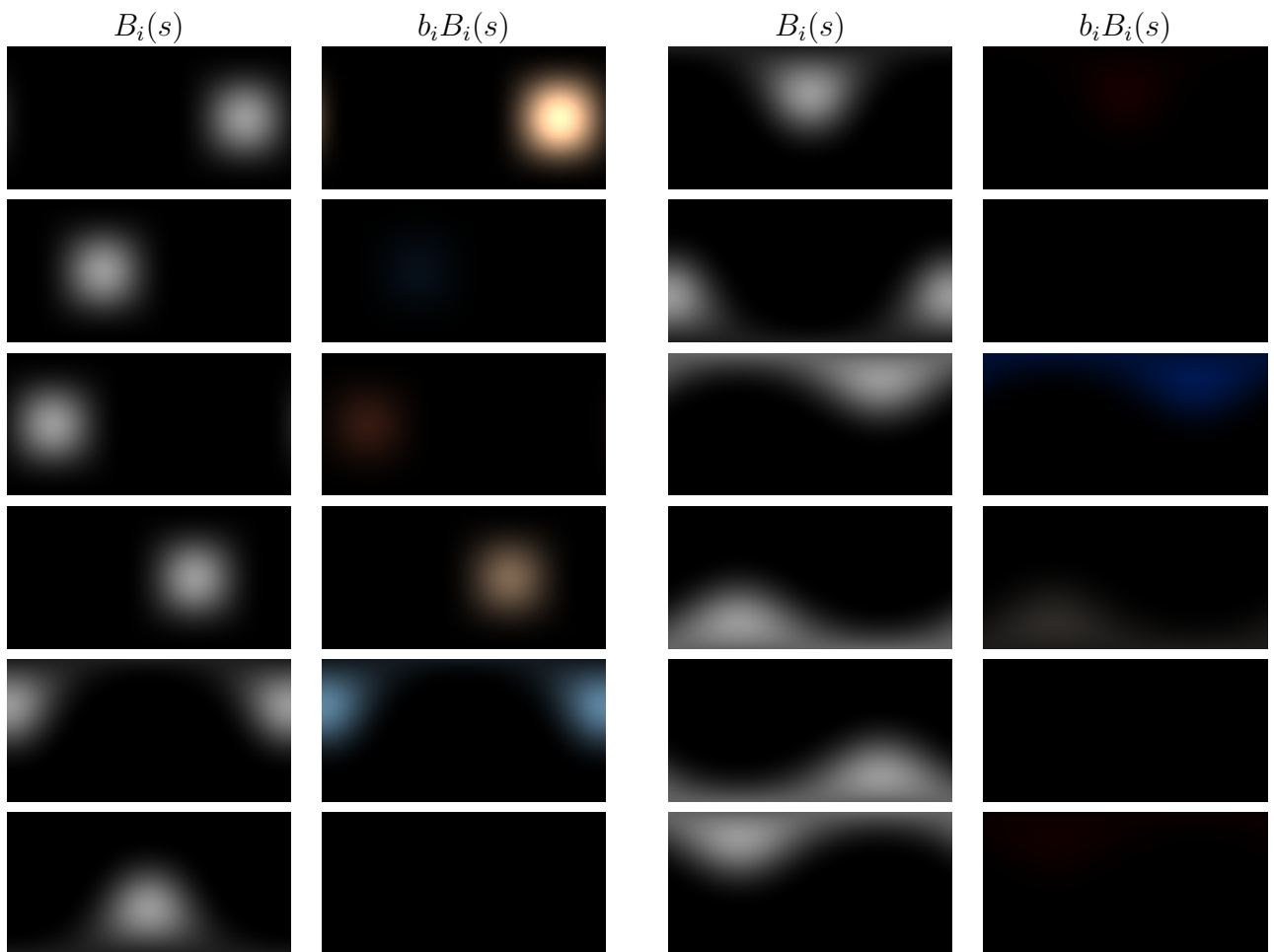
Figure 7.2: The individual Ambient Dice SRBF basis functions comprising the approximated Wells HDR environment map.
