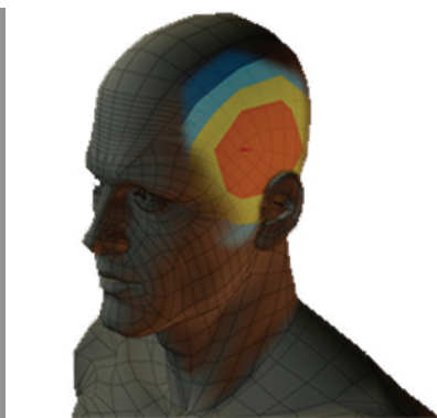
SAR Levels With R2L™
