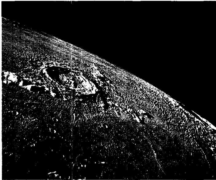
FIGURE 4-56.—This high-oblique view from the LM after lift-off from the lunar surface includes the craters Eratosthenes, 60 km in diameter, at left center, and Copernicus on the horizon at the right. The view is to the southwest from southern Mare Imbrium. To the left of Eratosthenes is the southern end of Montes Apenninus. Patterns of secondary craters are emphasized in this low-Sun-angle photograph (AS17-145-22285).
