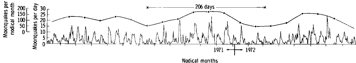
FIGURE 11-3.—Moonquake activity recorded at the Apollo 14 station between February 7, 1971, and July 27, 1972, showing the number of moonquakes detected per day. Peaks in activity occur at 2-week intervals corresponding to the apogee/perigee cycle. A longer term variation in moonquake activity, with a period of 206 days, is also seen in the smoothed activity plot shown above the daily count. This 206-day period corresponds to the period of the tidal variation introduced by solar perturbation of the lunar orbit.
