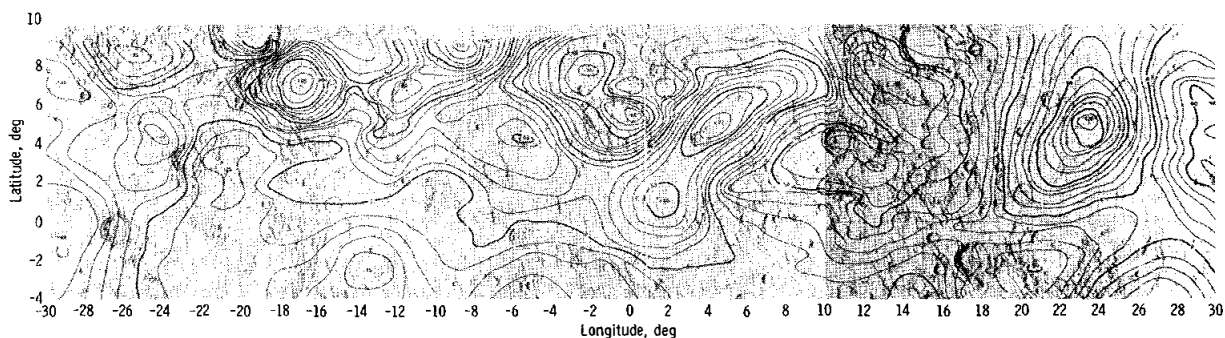
FIGURE 14-5.—Contour map of gravity from longitude 30° to -30° based on line-of-sight acceleration data from the Apollo 16 subsatellite. (Contour units are in milligals.)
