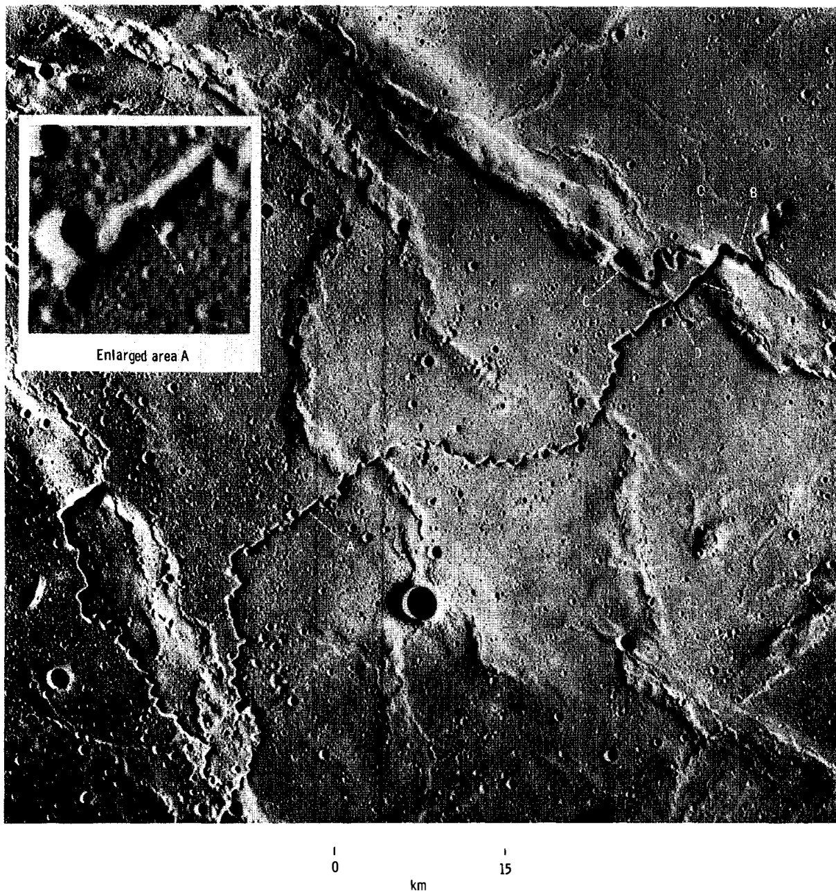
FIGURE 31-1.—Herigonius rille complex: (A) collapsed roof(?) remnant; (B) secondary(?) vent; (C) blocked primary(?) vent; (D) and (E) intrusive or extrusive(?) postrille features (Apollo 16 metric camera frame AS16-2837).
