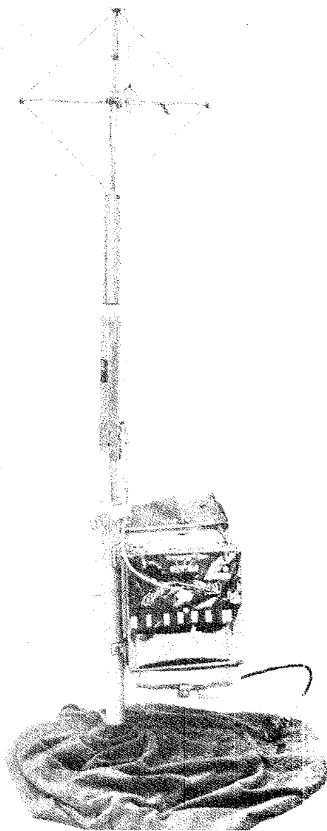
FIGURE 15-8.—The SEP experiment receiver and antennas. The receiver electronics, including tape recorder and battery, are contained in the box ( 23 \text{ cm}^3 ), which usually is completely enclosed in a thermal blanket. The thermal blanket has been opened to show optical surface reflectors. The three-loop antenna assembly, folded during the journey to the Moon, is shown unfolded as it was used on the Moon.
