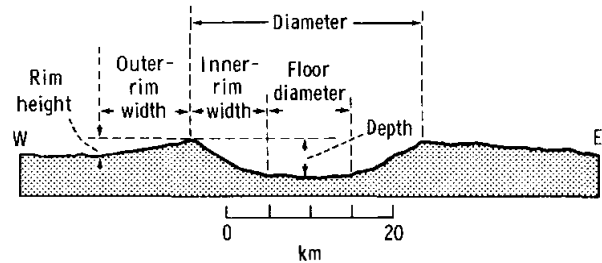
FIGURE 32-1.—Six crater dimensions. Topographic profile across the near-side crater Proclus from photogrammetry of Apollo 17 metric camera photographs. Corrected for planetary curvature. No vertical exaggeration. Directions are approximate only.
