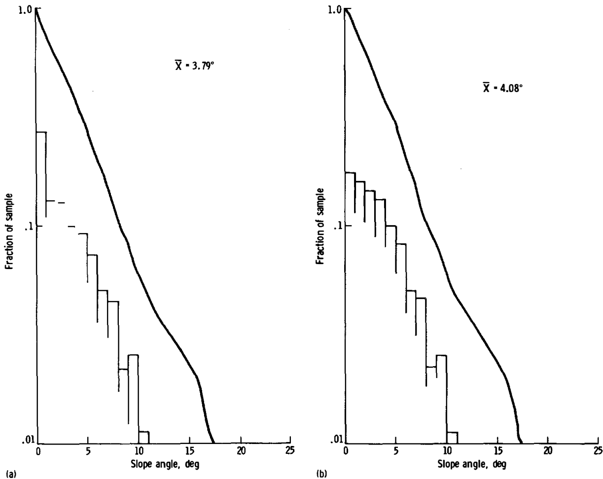
FIGURE 33-18.—Slope-frequency distribution of Apollo 17 landing site. (a) Corrected for reading error. (b) Uncorrected for reading error.
