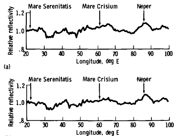
FIGURE 23-9.—Lunar transit data divided by far ultraviolet Hapke function. (a) Revolution 28. (b) Revolution 29.
