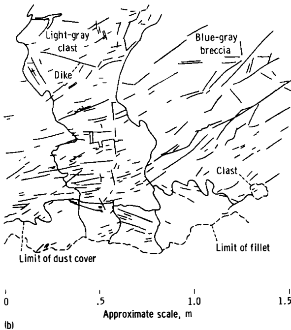
FIGURE 6-31.—Fractures in blue-gray breccia and light-gray inclusion in station 7 boulder. Note differences in spacing of fractures. (a) Photograph AS17-146-22310. (b) Sketch map.
