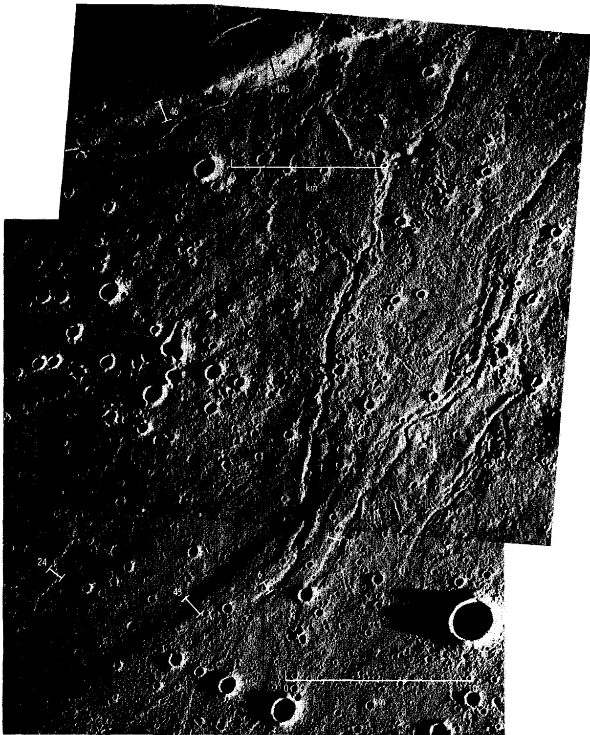
FIGURE 30-22.—Apollo 17 Hasselblad photographs AS17-155-23717 and 23718 showing the braided lava channels near the source vents of the phase III eruptives. Numbers (e.g., 24) are heights in meters measured at indicated points. The Sun elevation angle is approximately 1^\circ .
