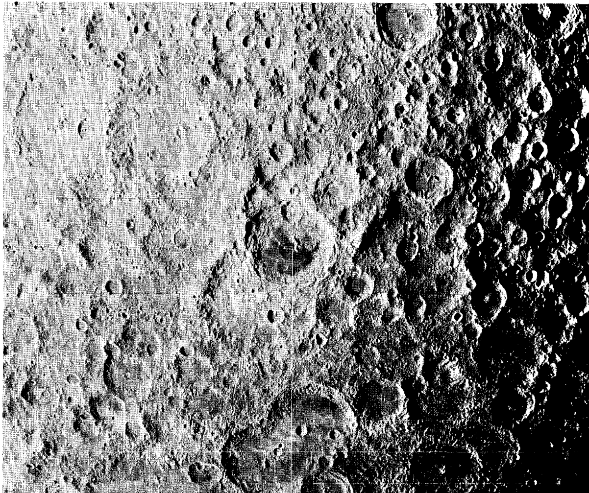
FIGURE 32-6.--Part of Lunar Orbiter II frame 33-M centered on the crater Aitken (lat. 17^{\circ} S, long. 173^{\circ} E). Relative high albedo rim deposits of Aitken extend outward to one crater diameter. Icarus Crater with its large central peak is in the upper right corner; west of it is Daedalus Crater. Northwest of Aitken is the pair of old subdued craters, Heaviside (right) and Keeler (left). Due south of Aitken Crater is the crater Van de Graaff, on the northeastern rim of Mare Ingenii.
