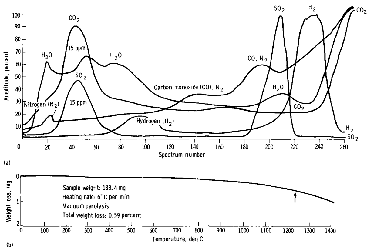
FIGURE 7-26.—Gas-release profile of soil sample 74220,5 (orange soil). Note the low-temperature release of \text{CO}_2 and \text{SO}_2 . The gas-release patterns as compared to temperature have been plotted so that each of the gases have been normalized to 100-percent amplitude in their region of greatest abundance. The arrow on the weight-loss curve represents the initial melting of the sample. (a) Gas-release profile. (b) Weight-loss curve.
