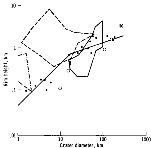
FIGURE 32-4.—Logarithmic rim height/diameter plot for 25 lunar far-side craters (dots and circles). Circles are markedly older appearing craters. Bracketed data point (crater Gagarin) is from inadequate data. Solid polygon contains Zond 3 data for 29 far-side craters. Inflected curve is best fit to 325 lunar near-side craters; terrestrial meteorite craters (not shown) also follow this trend. Dashed polygon contains data for 44 terrestrial calderas. Dashed-dotted polygon contains data for seven craters atop lunar mare domes.
