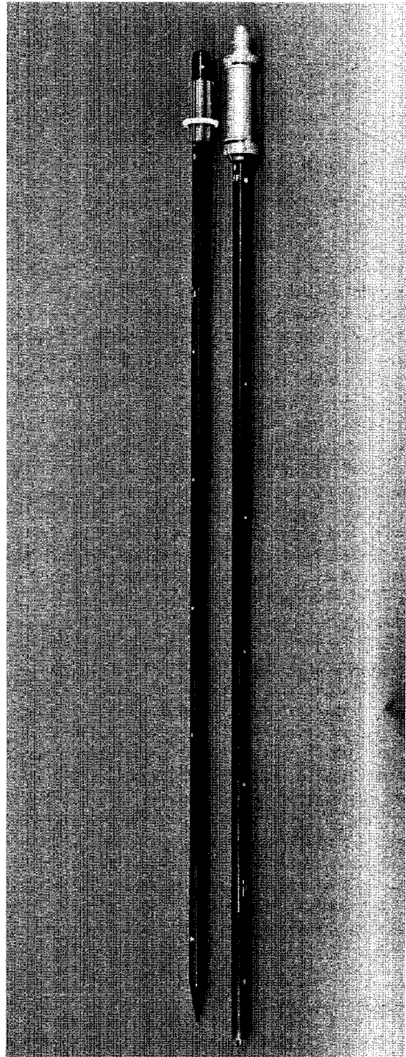
FIGURE 18-7.—The assembled flight unit of the lunar neutron probe. The upper section, with the probe handle at the top, is on the right. The lower section with its removable dust cap is on the left. Coupling of the two sections is accomplished by screwing the lower and upper units together after removing the dust cap. Each section is approximately 1 m long.
