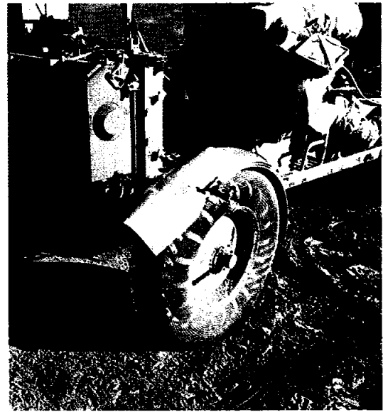
FIGURE 4-21.—The partial loss of the right rear fender during EVA-1 threatened to limit the use of the LRV. Without complete fenders, the wire mesh wheels threw a plume of lunar dust across the crew and the LRV. At the beginning of EVA-2, the crew replaced the missing section using maps, tape, and two clamps from the LM. The repairs proved to be satisfactory, and no further problems were experienced. The MPM sits in the LRV (AS17-137-20979).
