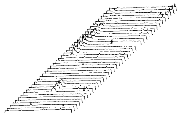
FIGURE 24-6.—This sequence of nighttime scans runs westward approximately between 35^{\circ} and 38^{\circ} W longitude at latitude 7^{\circ} N. The crater in the foreground is Kepler A, and the extended feature in the background is the crater Kepler. North is to the left; west is at the top.
