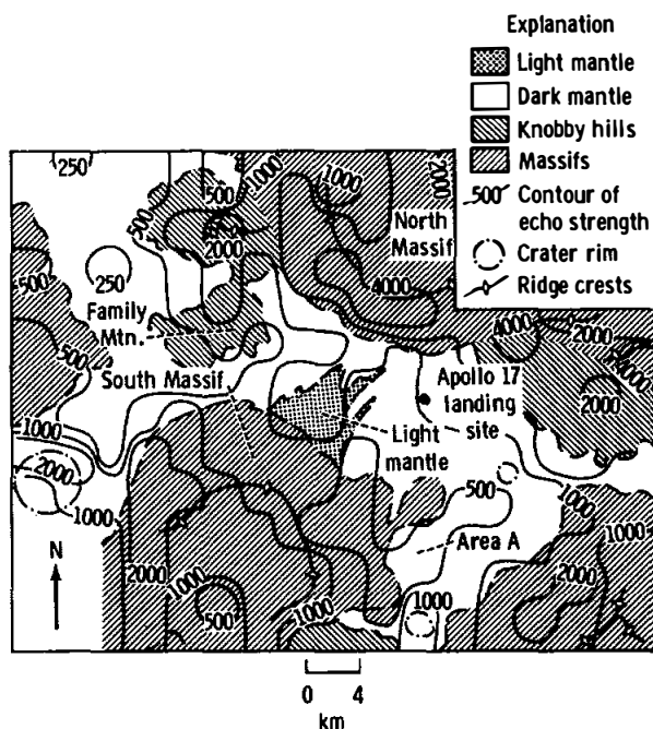
FIGURE 33-6.—Correlation of echoes to topography of the Apollo 17 landing site. (a) Contour map of depolarized radar echoes at the Apollo 17 landing site. (b) Photographic mosaic of Apollo 17 landing site (Apollo 17 panoramic camera frames AS17-2309, 2311, 2312, and 2314).
