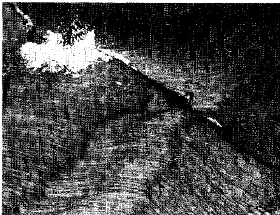
FIGURE 31-17.—Mauna Ulu lava lake, Hawaii. Squeeze-outs (splash) and overthrusting at junction of crustal plates in circulating lava lake. Plates on each side of junction are flat; appearance of curvature is optical illusion caused by striated texture of crust. Squeeze-out ridge at upper left is about 1 m wide (photograph by W. A. Duffield).
