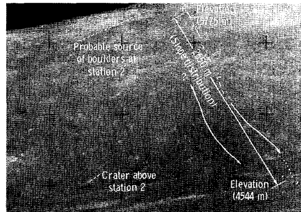
FIGURE 6-6.—Boulder tracks on the South Massif in the vicinity of station 2.
