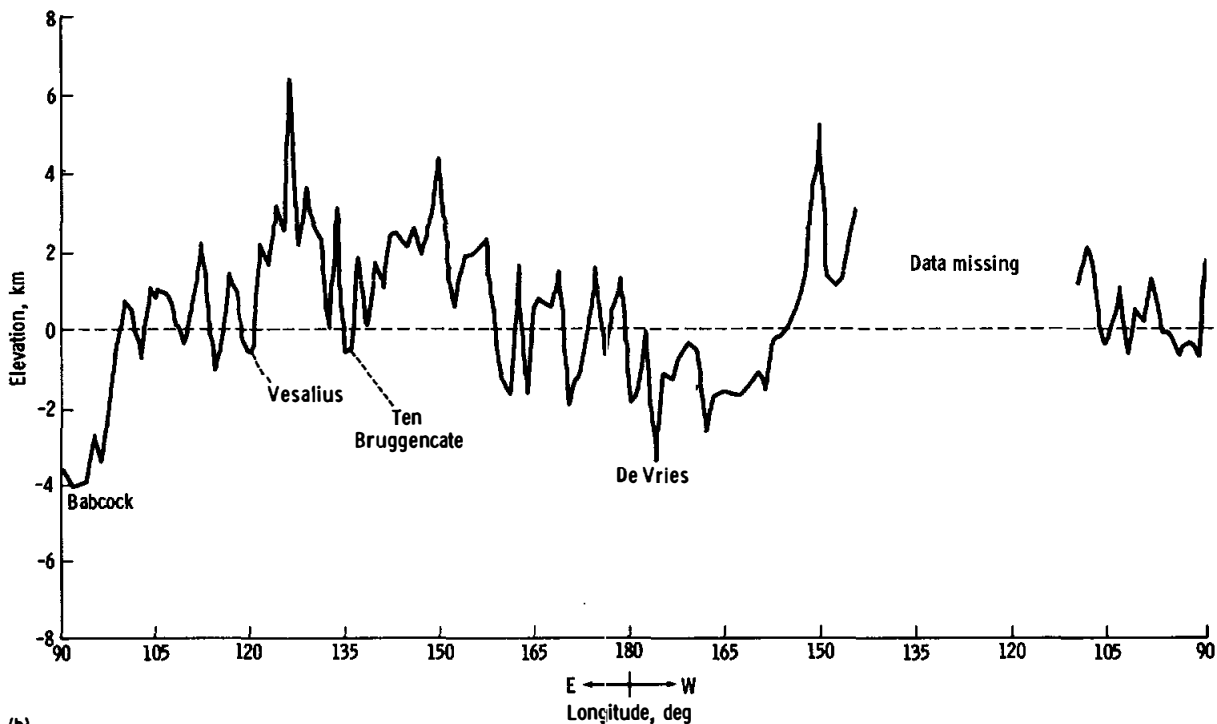
FIGURE 33-24.—Profile of Apollo 17 elevations with respect to a 1738-km sphere about the center of mass. (a) Lunar near side. (b) Lunar far side.
