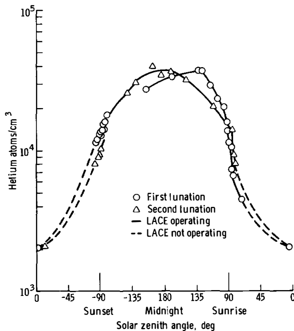
FIGURE 17-5.—Diurnal variation of 4 He. Concentration is plotted as a function of solar zenith angle with nighttime in the center of the figure. The distribution is typical for a noncondensable gas.
