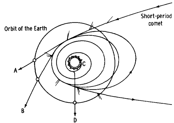
FIGURE 16-3.—Cometary debris.
