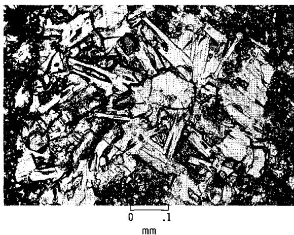
FIGURE 7-10.—Thin sections of blue-gray breccias. (a) Clasts and very-fine-grained dark matrix of blue-gray breccia (sample 76315,11). Note the alinement of elongate clasts and foliation of light and dark streaks in matrix. Several pink spinels (medium gray) occur in the light band along the edge of the photograph (plane light view) (AS17-73-19998). (b) Clast in blue-gray breccia (sample 76315,11). Several equant, pink spinels (medium gray) occur in this plagioclase and olivine clast, suggesting a source for the crushed material in the spinel-bearing light band of figure 7-10(a) (plane light view) (AS17-73-20000).
