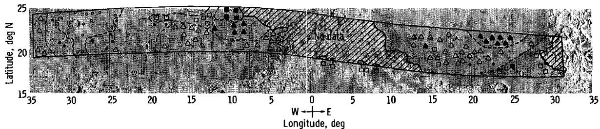
FIGURE 29-24.—Areal distribution of mare units as defined by relative ages. The symbols are the same as those shown in figure 29-23. No data are presented for the uplands (hatched areas). The dashed lines are intended to accentuate units of approximately uniform age.
