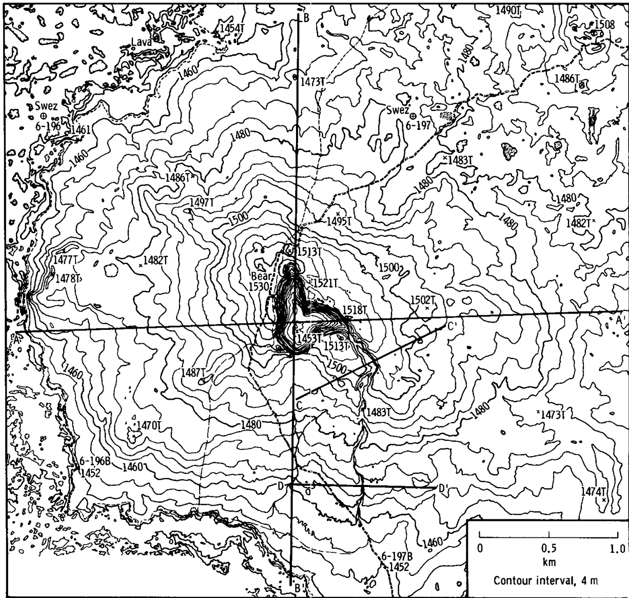
FIGURE 30-5.—Preliminary topographic map and profiles of Bear Crater and vicinity. Topography by U.S. Geological Survey. (a) Topographic map.
