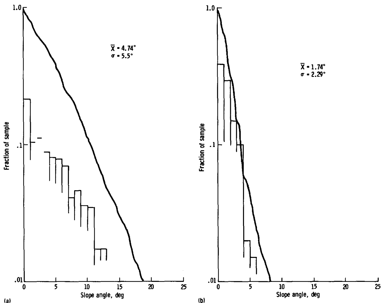
FIGURE 33-7.—Frequency distribution of absolute slope values for surface in Mare Serenitatis. Bars represent fraction of sample contained in 1^\circ increments of slope angle. Solid lines indicate cumulative fraction of sample with absolute slopes larger than angle indicated. The quantity \bar{X} is mean absolute slope and \sigma is algebraic standard deviation of distribution. (a) Slope length \Delta L 25 m. (b) Slope length \Delta L 200m.
