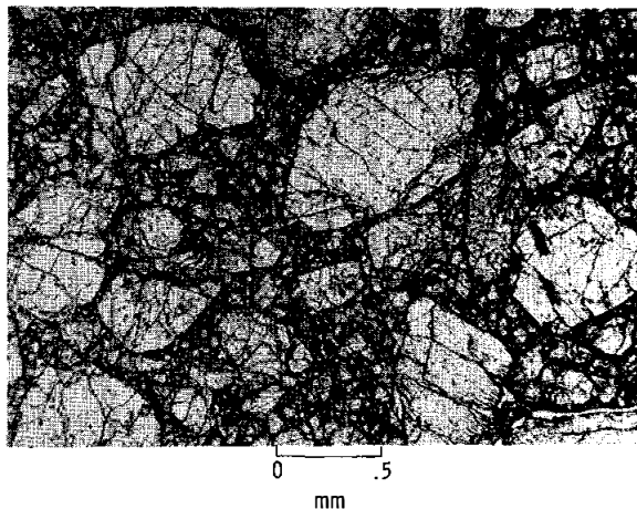
FIGURE 7-18.—Thin section of dunite with large olivine crystals set in a crushed matrix of the same material comprise this entire clast (sample 72415,12, plane light view) (AS17-73-19947).
