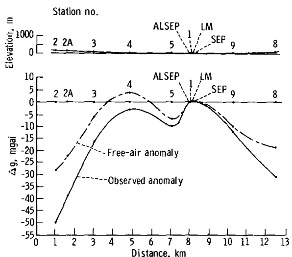
FIGURE 13-6.—Observed anomaly and free-air anomaly profiles across the Taurus-Littrow valley.
