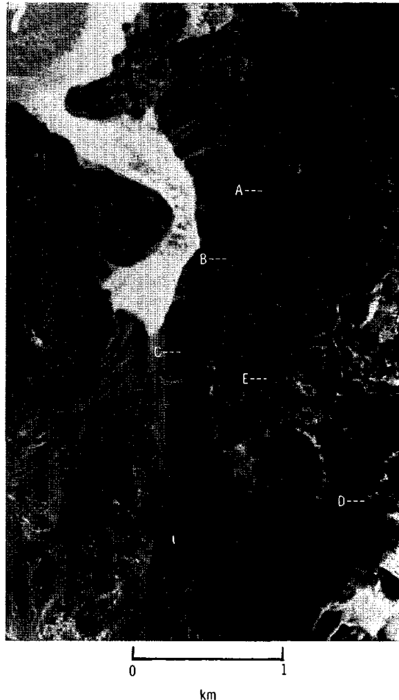
FIGURE 30-8.—Terrestrial cinder cones in Nevada. Breached cones along a fracture (A, B, and C) and small cinder mounds (D and E) (U.S. Geol. Survey photograph).
