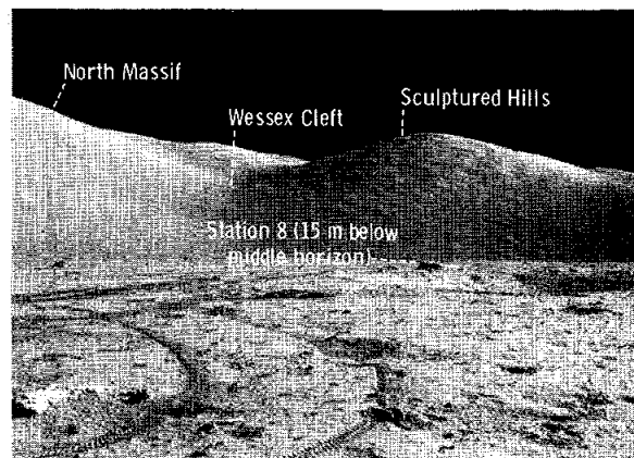
FIGURE 6-35.—Station 8 area at Sculptured Hills as viewed from the LM, 4 km away. Note the contrast between the hills on the right and the massif material directly above Wessex Cleft, although both slopes have similar orientations (AS17-137-20876).
