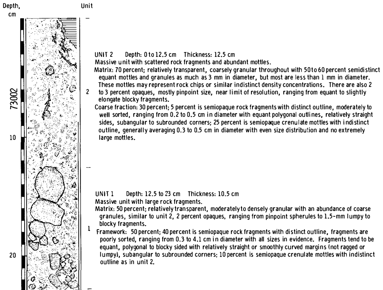
FIGURE 7-30.—Interpretation of X-radiograph of 73002 drive tube. The X-radiograph symbols are the same as in figure 7-27.
