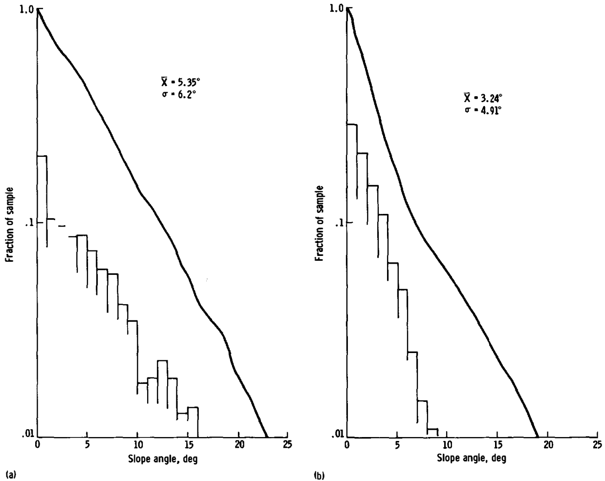
FIGURE 33-8.—Frequency distributions of absolute slope values for Cayley Plain at the Apollo 16 landing site. Bars represent fraction of sample for 1^\circ increments of slope angle. Solid lines indicate cumulative fraction of sample with absolute slopes larger than angle indicated. The quantity \bar{X} is mean absolute slope and \sigma is algebraic standard deviation. (a) Slope length \Delta L 25.1 m. (b) Slope length \Delta L 201 m.
