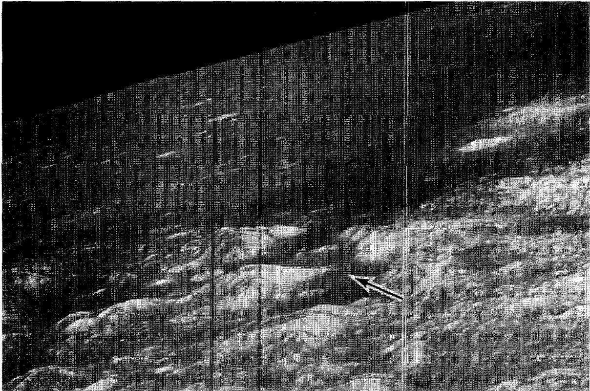
FIGURE 28-21.—Oblique view looking westward from the Taurus-Littrow landing site. Arrow, showing the direction of flight, indicates the landing point (ASI 7-148-22770).
