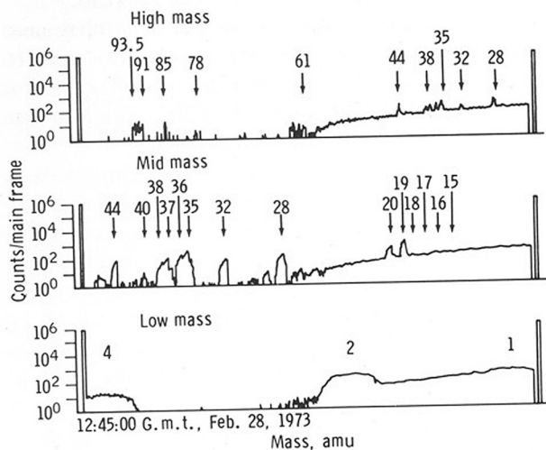
FIGURE 17-3.—Quick-look data recorded on a strip chart recorder. These mass spectral data were taken near the antisolar point during the third lunar night. Three output channels are identified as high-, mid-, and low-mass ranges. The ordinate is a logarithmic scale of ion counts from 10^0 to 10^6 counts per telemetry main frame (0.6 sec). Mass scale is plotted on the abscissa. Principal peaks are identified by mass number. The large pulses at the beginning and end of each spectrum are internal calibration frequencies to check operation of detector circuit. The solar zenith angle is 160^\circ .
