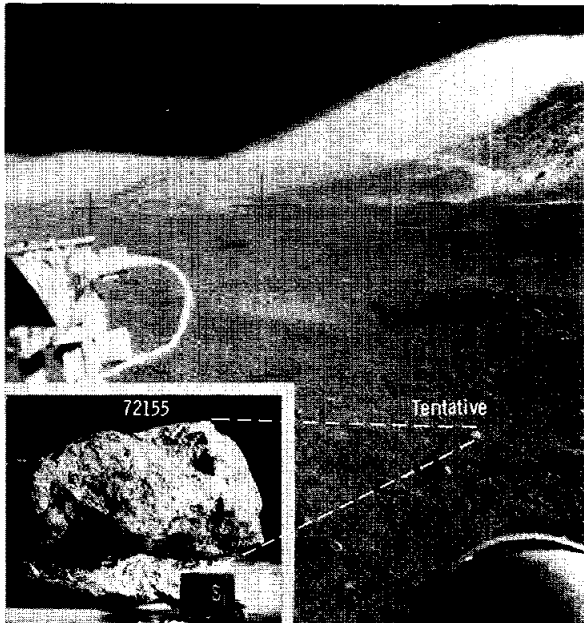
FIGURE 6-72.—Sample 72155 showing approximate lunar orientation reconstructed in the LRL tentatively compared to a portion of LRV driving photograph AS17-135-20649, looking north. No photograph was taken after collecting the sample (inset photograph, S-73-18406).
