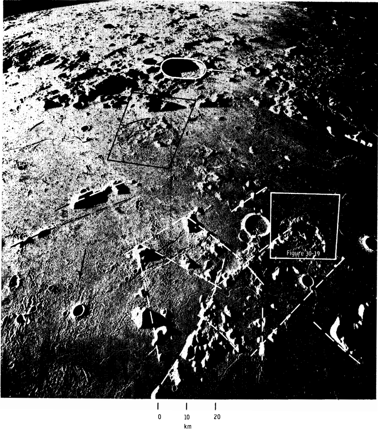
FIGURE 30-17.--South-looking oblique photograph showing the suggested regional volcanic source area for all Eratosthenian-age mare lavas in the Imbrium basin. Structural control of mare islands is indicated by dashed lines; areas of figures 30-18 and 30-19 are indicated (Apollo 17 metric camera frame AS17-2450).
