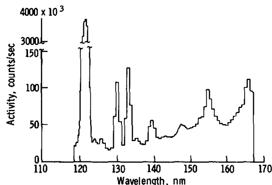
FIGURE 23-6.—Spectrum obtained from UVS observation of the lunar surface near the subsolar point.
