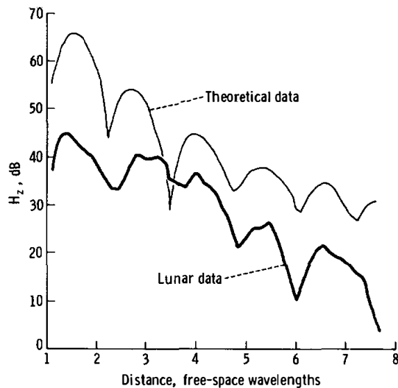
FIGURE 15-15.—Comparison of lunar data for H_z , 16-MHz, N-S transmitting antenna with the theoretical curve calculated from mode theory. Parameters are given in table 15-I.
