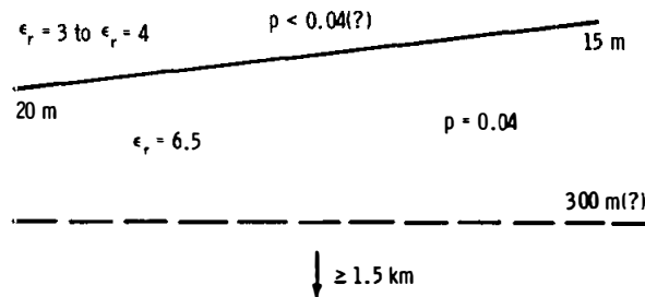
FIGURE 15-19.—The alternate model of the electrical structure at the Apollo 17 site. A layer of thickness between 0.2\lambda and 0.3\lambda is present at the SEP experiment site (left) and thins toward station 2 (right). The broken line at 300 m indicates a possible discontinuity in \epsilon_r at that depth.
