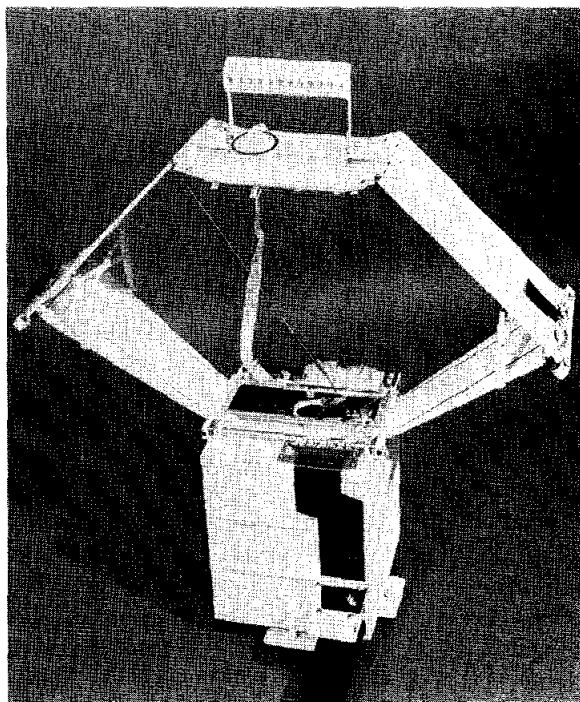
FIGURE 12-1.—Lunar surface gravimeter.
