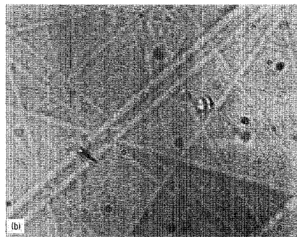
FIGURE 19-12.—Etched tracks in phosphate glass (GE-1457). (a) A typical view in the Apollo 16 detector, which was exposed during a solar flare known to have ejected particles into the interplanetary medium. (b) An atypical view in the Apollo 17 detector. The view is unusual in that it contains a track. Each detector was etched in 48 percent hydrofluoric acid to remove 0.5 \times 10^{-4} cm of glass.
