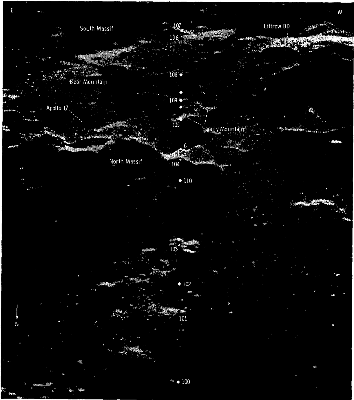
FIGURE 22-25.—ALSE 2-m-wavelength image of the area round the Apollo 17 landing site obtained during revolution 25. See figure 22-24 for the appearance of the scene in a stereoscopic view. The numbered points correspond to those in figure 22-26. The crater Littrow BD is 4 km in diameter.
