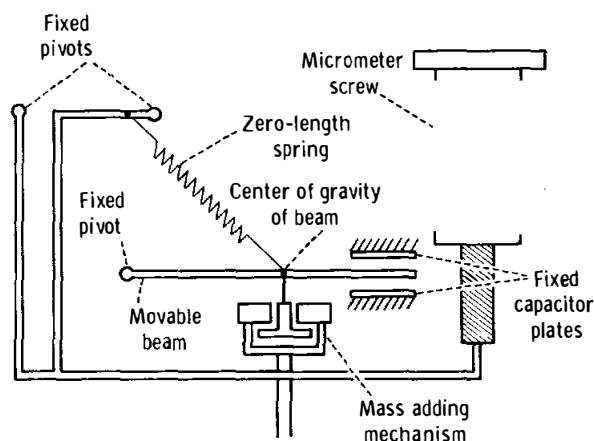
FIGURE 12-2.—Schematic diagram of the lunar gravity sensor.
