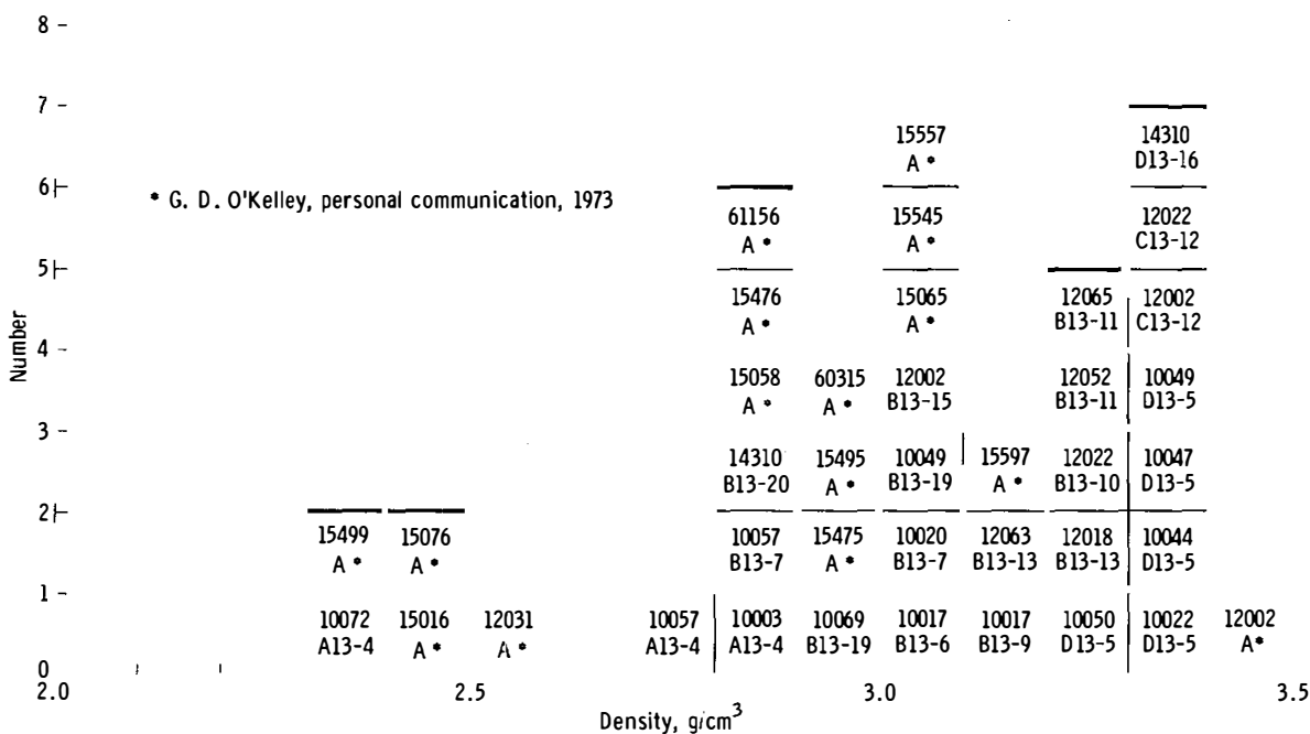
FIGURE 13-8.—Measured density values for lunar samples. (a) Breccia. (b) Basalt.
