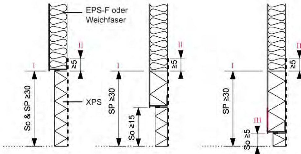
Figure 45: Fundamental rules for heat insulation composite systems
