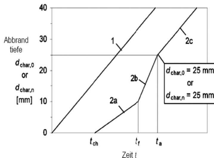
Figure 5: Representation of charring depth as a function of time for t_f > t_{ch} for gypsum boards type F and DF or GKF planked woods, source: [ÖNORM EN 1995-1-2]
