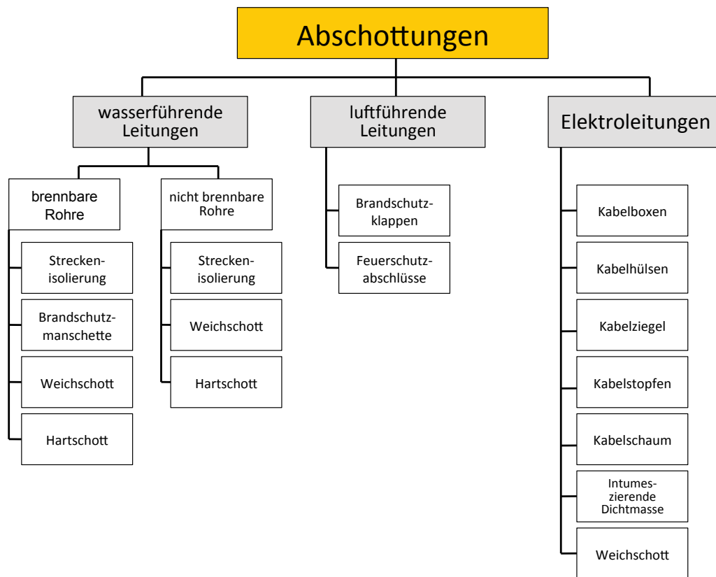
Figure 79: Survey of partitioning systems for water and air-bearing lines and electric cables
