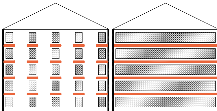
Figure 104: Example of the arrangements of fire protection partitions with perforated façades or strips of ribbon windows
