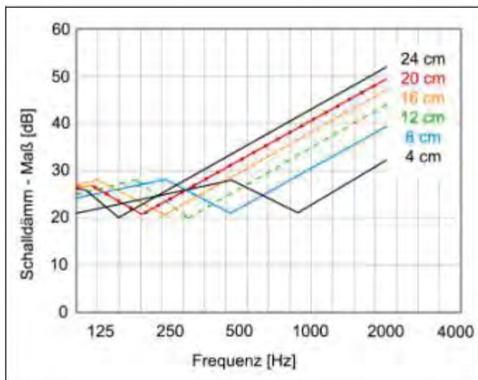
Figure 17: Calculated sound insulation index of jointless solid timber slabs depending on their thicknesses, source: [Bednar et al. 2000]
