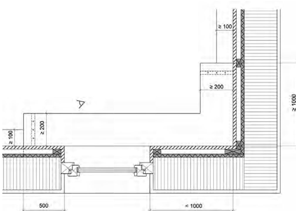
Figure 102: Example of minimum distances of fire barriers for internal corners or windows from internal corners, source: [ÖNORM B 2332]
