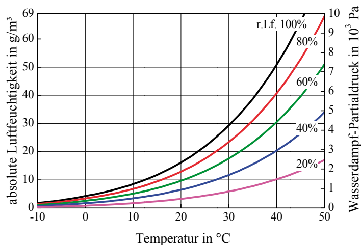
Figure 24: Dependence of absolute humidity and water vapor partial pressure on temperature and relative humidity
