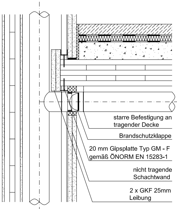
Figure 91: Installation of a fire protection flap in a shaft wall
