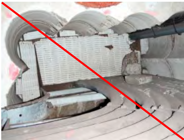
Figure 84: Improper installation of a soft partition in a wall penetration, source: bip company
