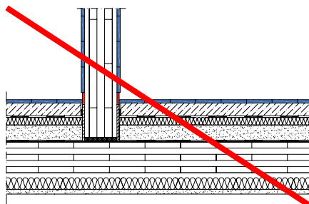
Figure 65: Joint filler between wall and floor tiles
