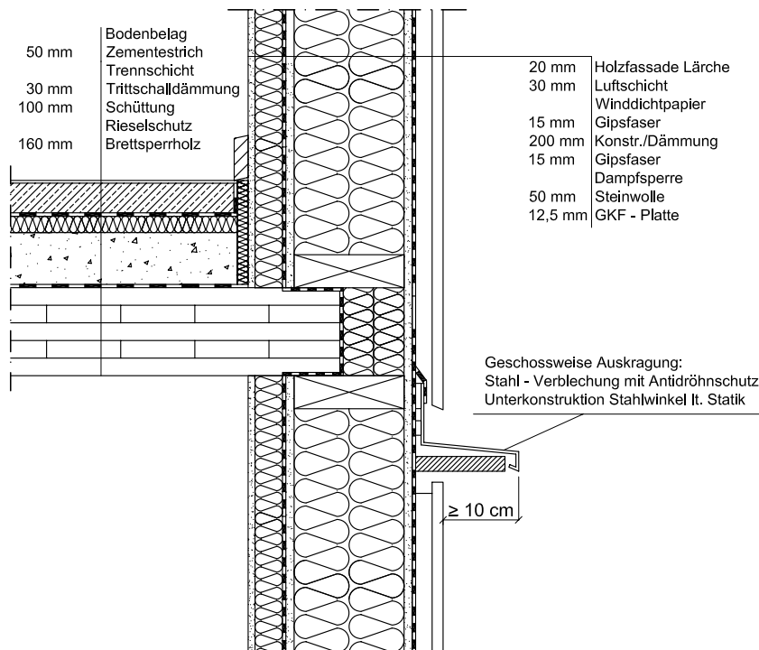
Figure 103: Exemplary façade design with four-storied timber façades
