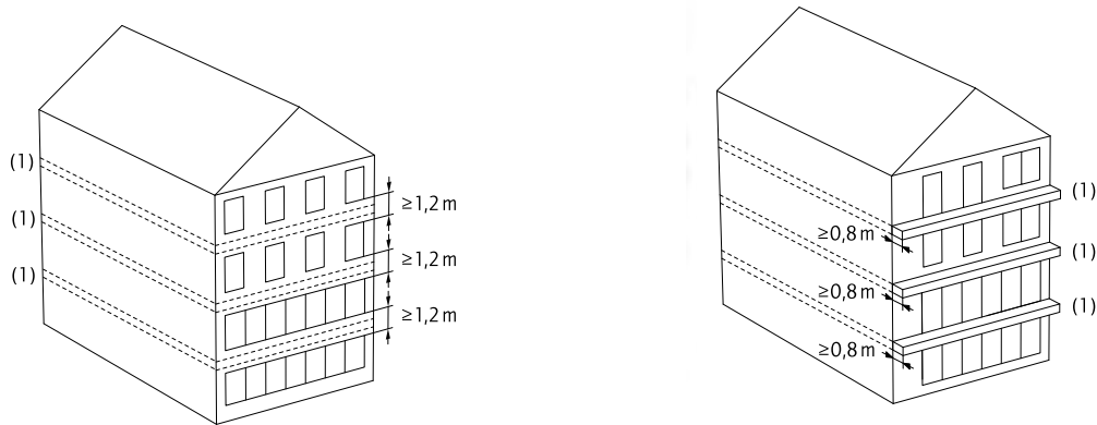
Figure 10: Measures for restricting vertical fire propagation on fire-compartment forming floors
