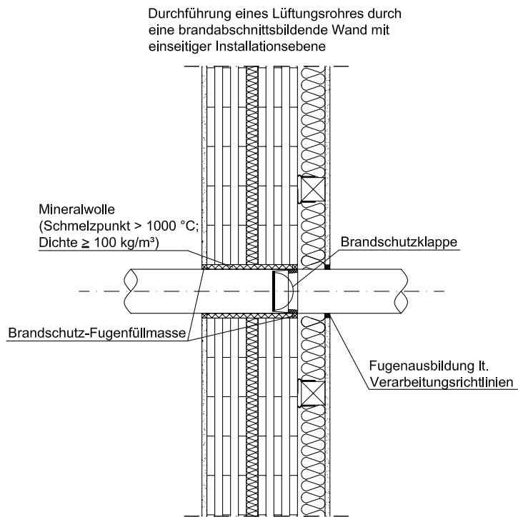
Figure 90: Installation of a fire protection flap in a fire compartment forming partition wall
