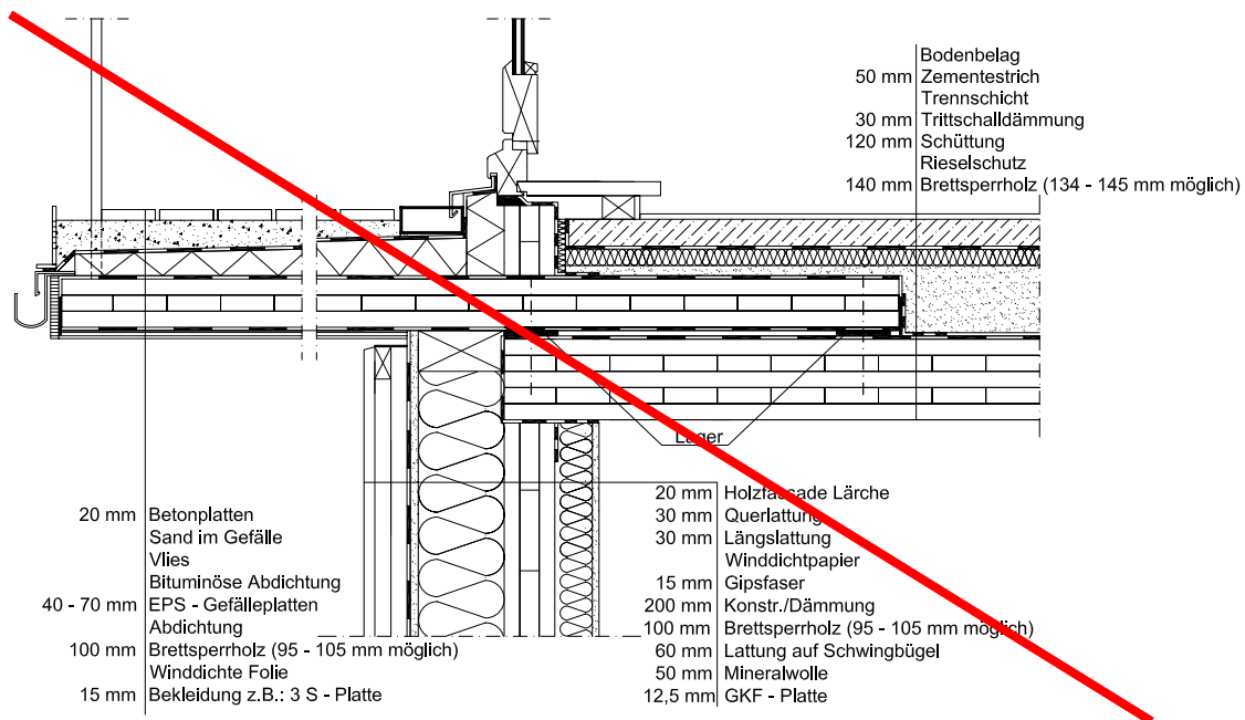
Figure 106: Insufficient execution of an overhanging balcony slab
