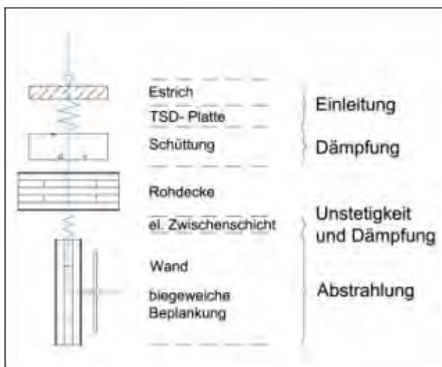
Figure 18: Reduction of impact sound
