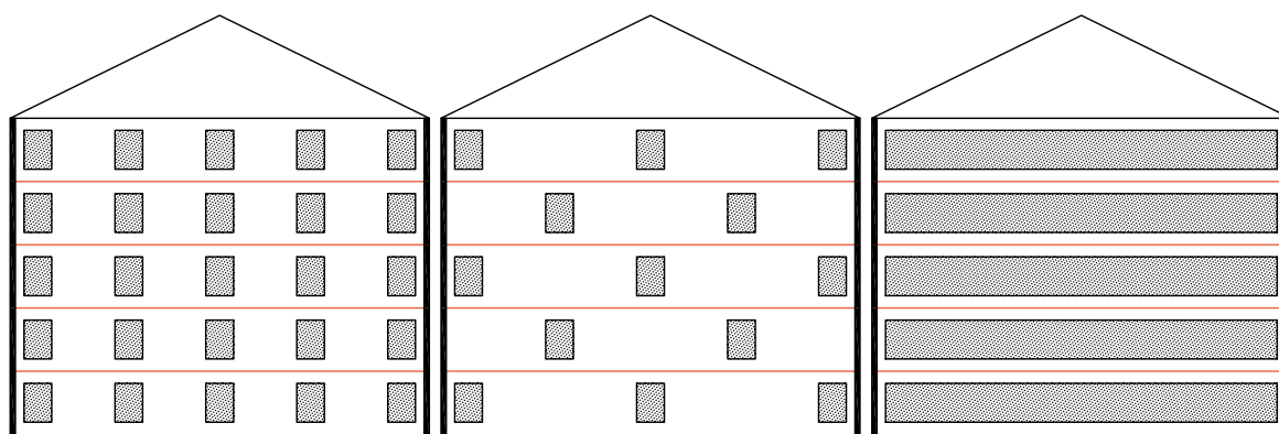
Figure 100: Examples of the arrangement of fire protection partitions with perforated façades or strips of ribbon windows
