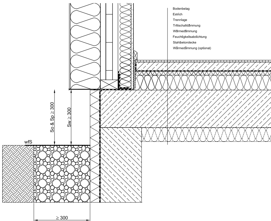
Figure 42: Standard base detail
