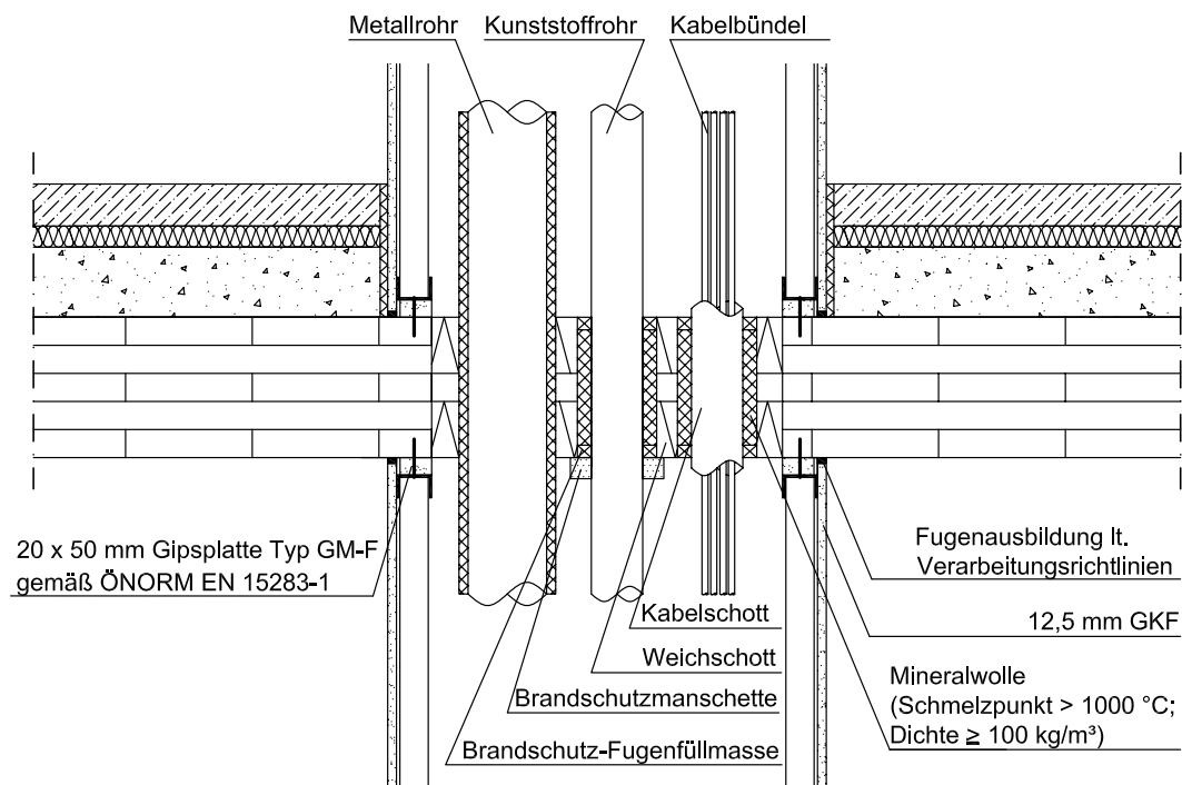
Figure 75: Exemplary design of horizontal partitioning in the area of a solid timber floor (shaft type B)
