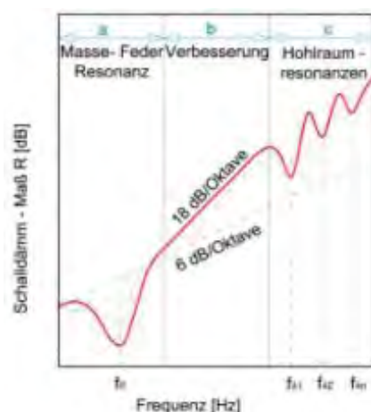
Figure 16: Sound reduction index of double-leaf components
