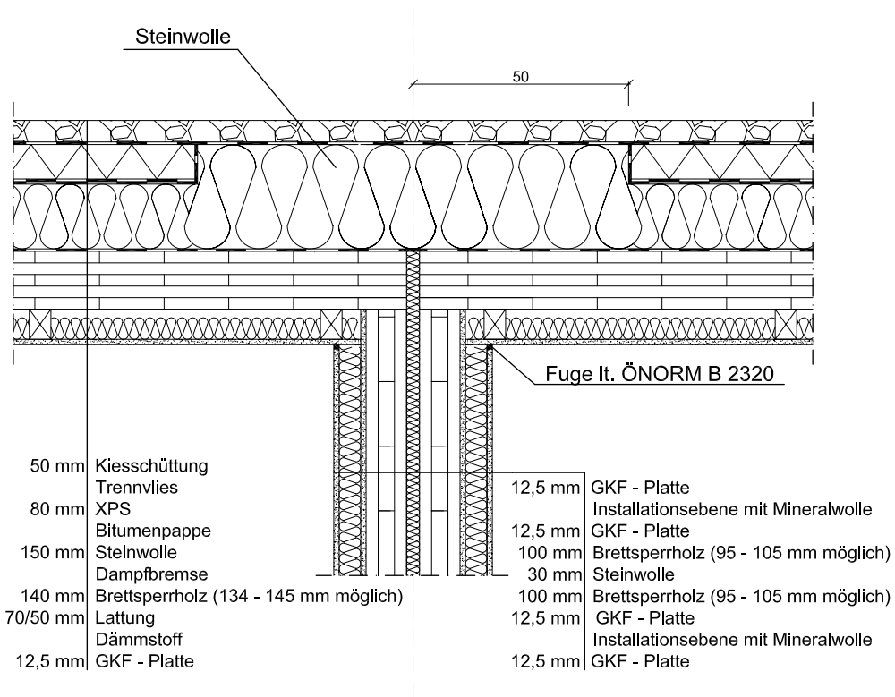
Figure 71: Exemplary connection of a fire compartment forming wall to a flat sloping roof with on-roof insulation
