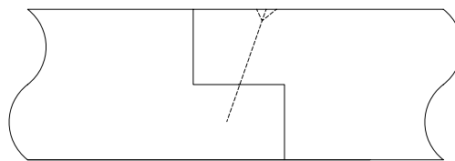
Figure 56: Remaining wood cross section in the joint area of rebated connections
