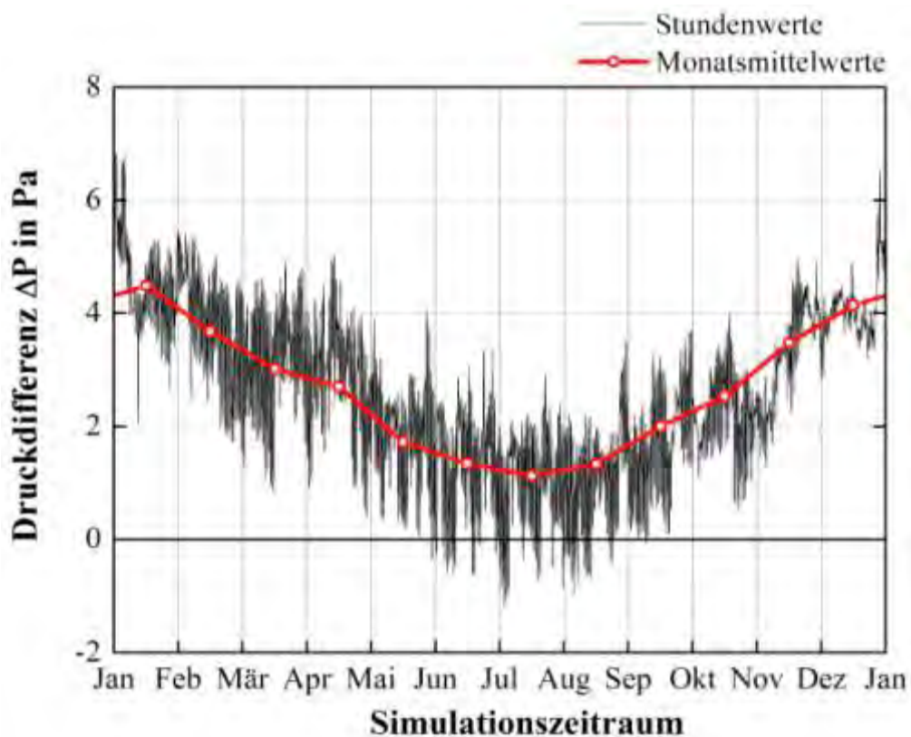
Figure 25: Pressure difference due to thermal in an 8 m high room at the Klagenfurt site with an inside temperature of 24 \pm 2 \text{ }^\circ\text{C}
