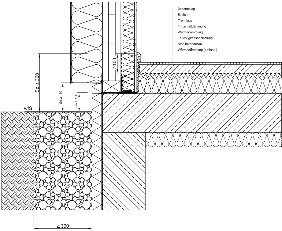
Figure 43: Base detail with minimum heights
