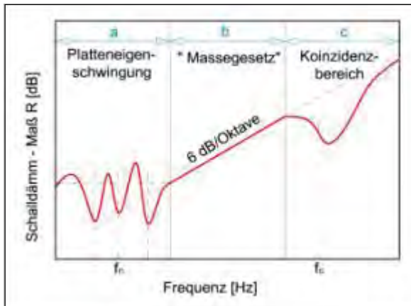
Figure 14: Characteristic portions of airborne sound insulation of single-leaf components
