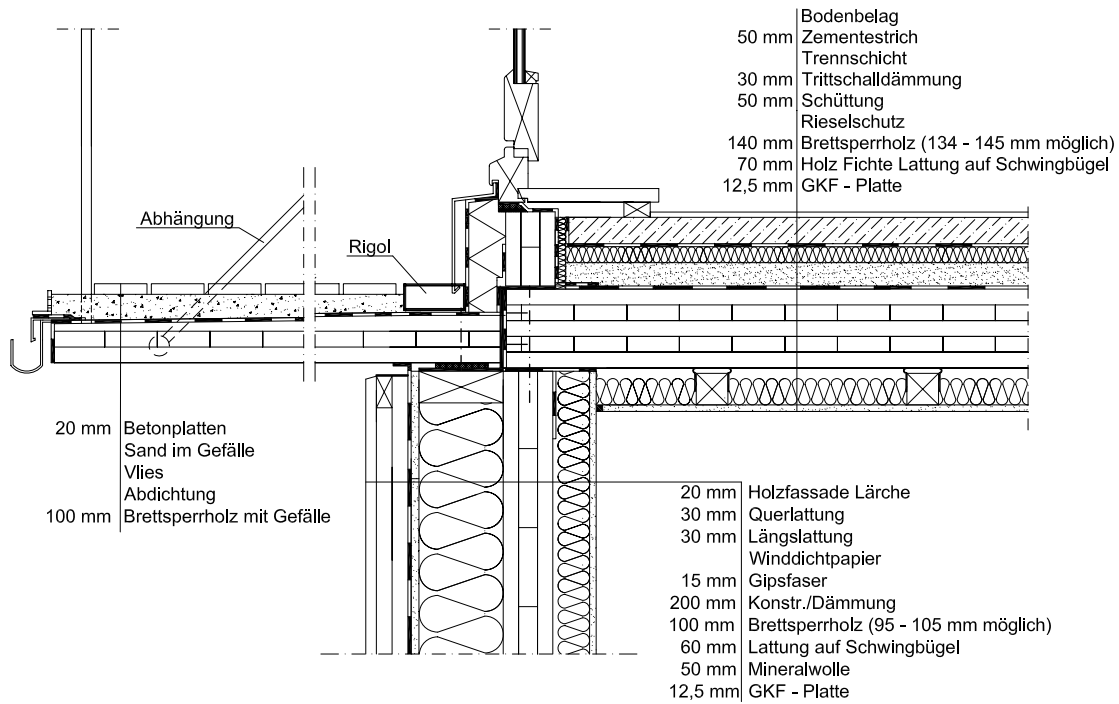
Figure 107: Recommended execution of an curtained and decoupled balcony slab
