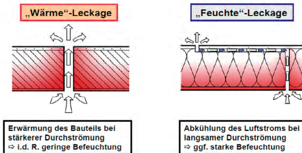
Figure 27: Heat and moisture leakages, source: [Künzel 2011]
