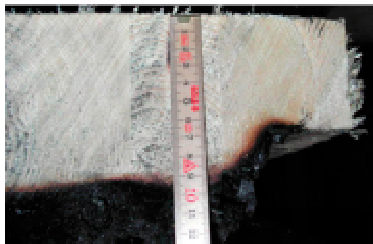
Figure 56: Remaining wood cross section in the joint area of rebated connections
