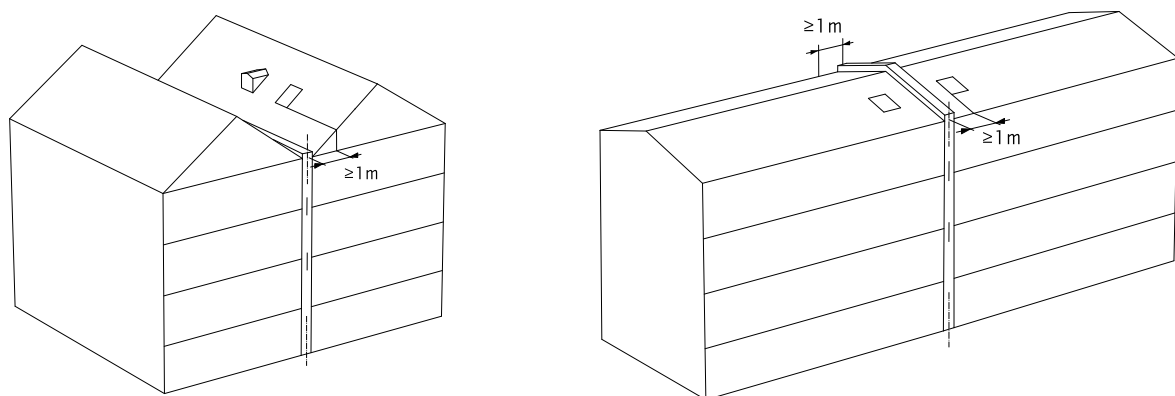
Figure 9: Distance between roof openings and fire-compartment forming walls
