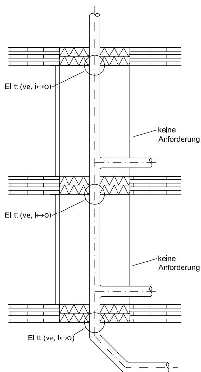
Figure 74: Schematic diagram of shaft type B, source: [Installationen-Richtlinie MA 37]
