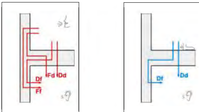
Figure 19: Airborne sound and impact sound transmission routes between neighboring rooms
