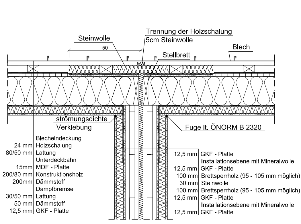
Figure 70: Exemplary connection of a fire compartment forming partition wall to a tin roof
