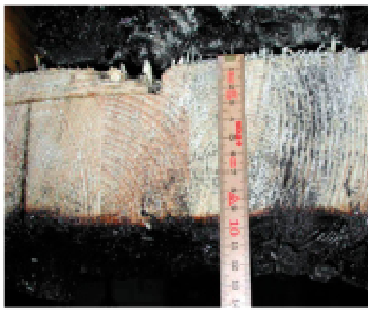
Figure 55: Remaining wood cross section in the joint area of welted boards
