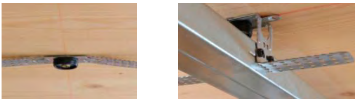
Figure 34: Mounting with decoupled suspension of whip arm, source: Knauf company
