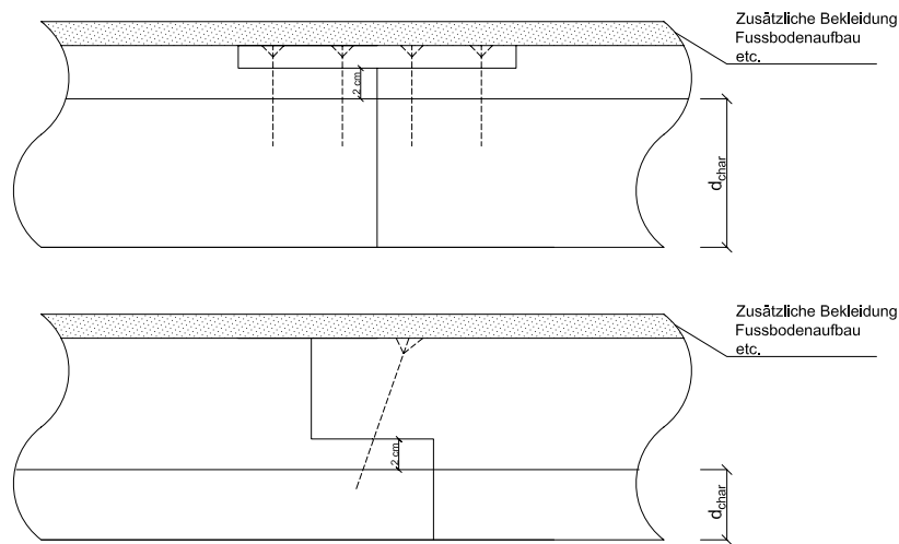
Figure 57: Element butt joint design of cross-laminated timber elements for verifying the integrity and heat insulation function, source: [ÖNORM B 1995-1-2]
