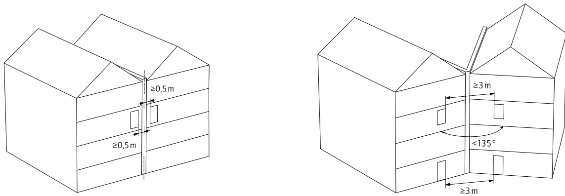
Figure 8: Distances between openings in external walls and fire-compartment forming walls
