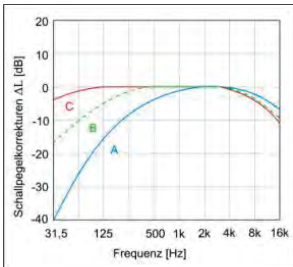
Figure 12: Frequency weighting curves
