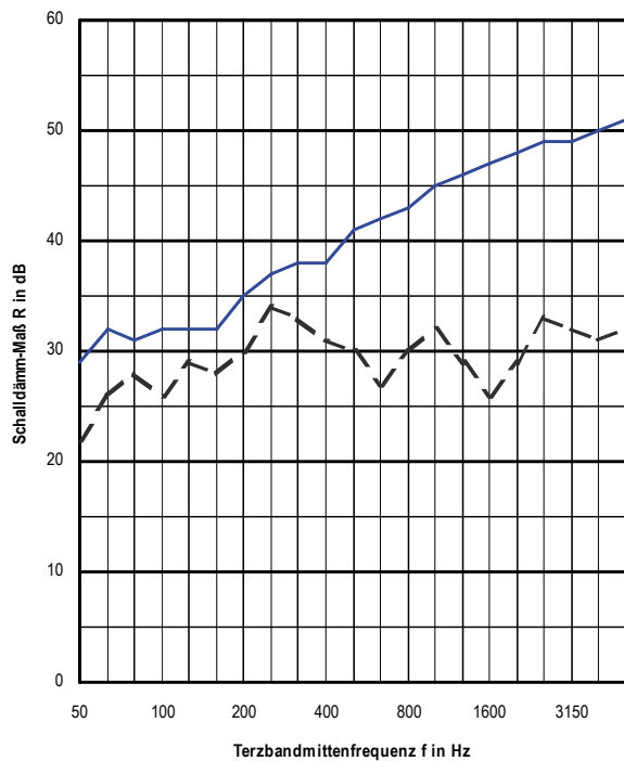
Figure 28: Impact of joint design on airborne sound insulation for a 160 mm thick cross-laminated timber floor, butt joint open R_w = 30 dB; butt joint sealed R_w = 45 dB, source: [Holtz et al. 2002]
