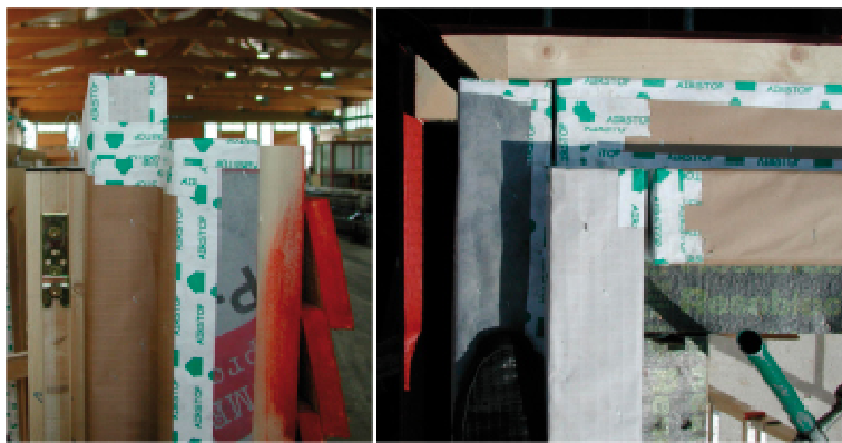
Figure 52: External wall corner: on the left, prefabrication (view); on the right, assembly (top view)
