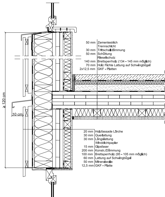
Figure 67: Exemplary connection of a fire compartment forming separation floor to the external wall (120 cm external wall strip)
