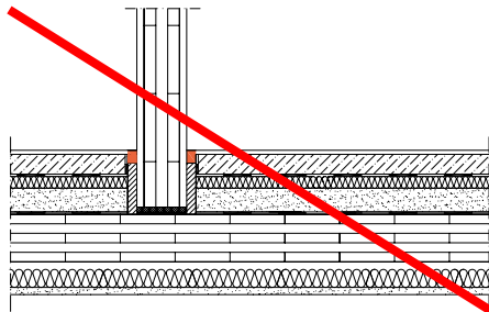
Figure 64: Coupling by filler due to screed insulating strips cut too short
