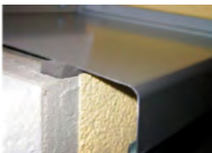
Figure 50: Horizontal joint under window sill towards façade surface with permeable sealing tape. Can also be executed in open form Source: [Österreichische Arbeitsgemeinschaft Fensterbank]
