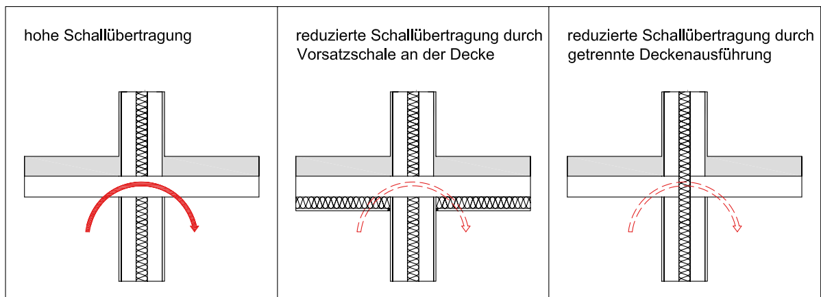
Figure 37: Sound transmission with continuous floors
