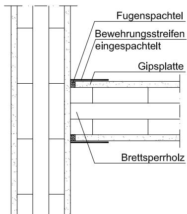
Figure 58: Connection details of a clad cross-laminated timber wall following [ÖNORM B 2320]
