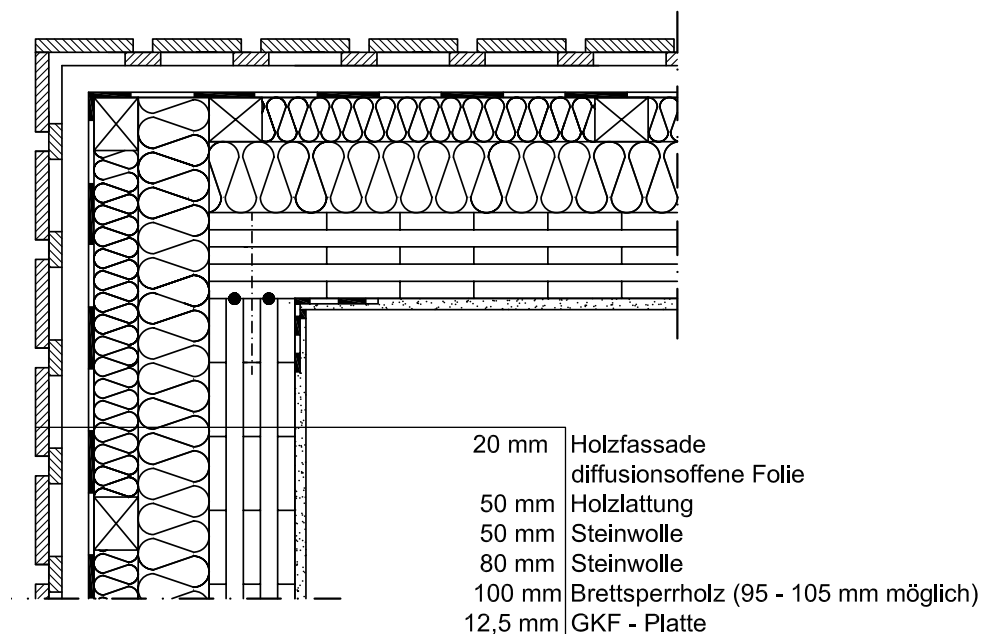
Figure 53: Exemplary execution of external wall corner
