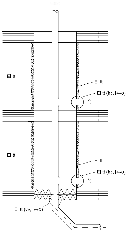
Figure 72: Schematic diagram of shaft type A, source: [Installationen-Richtlinie MA 37]
