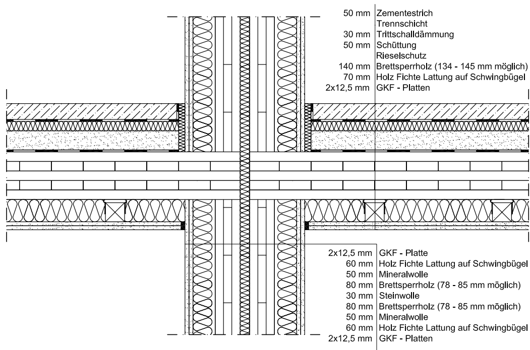
Figure 69: Exemplary connection of a fire compartment forming partition wall to a separating floor
