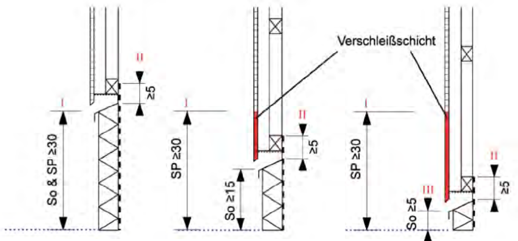
Figure 46: Fundamental rules for timber façades
