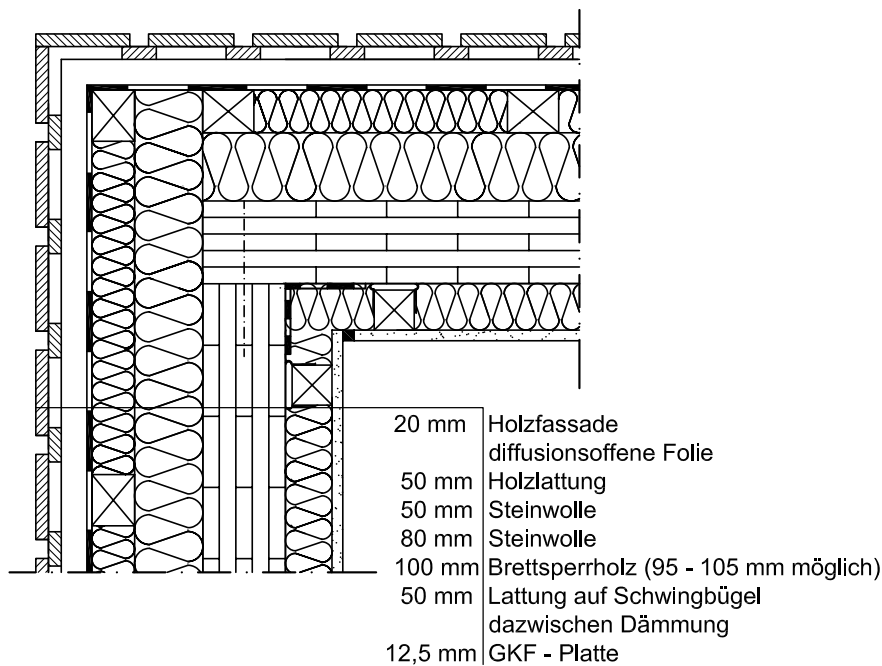
Figure 54: Exemplary execution of outer wall corner with installation level
