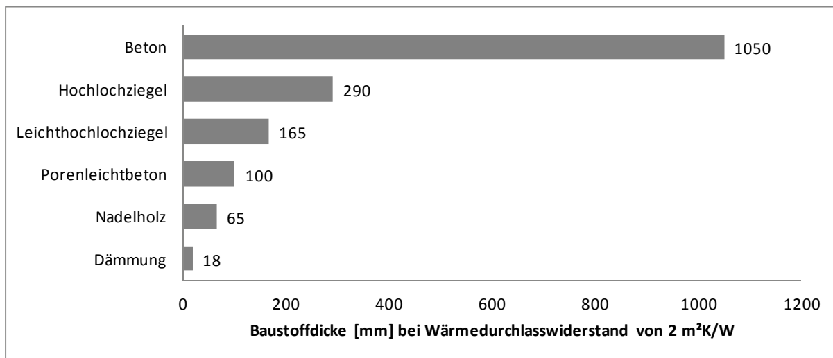
Figure 20: Comparison of required thicknesses of various construction materials for achieving an area thermal resistance of 2 \text{ m}^2\text{K/W}
