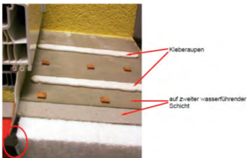
Figure 49: Windows sill installation on second sealing plane, bonded with adhesive beading. The resulting void spaces are admissible. The insulation material wedges / façade bead is connected with the window sill connection profile by means of a sealing tape (red circle Source: [Österreichische Arbeitsgemeinschaft Fensterbank])
