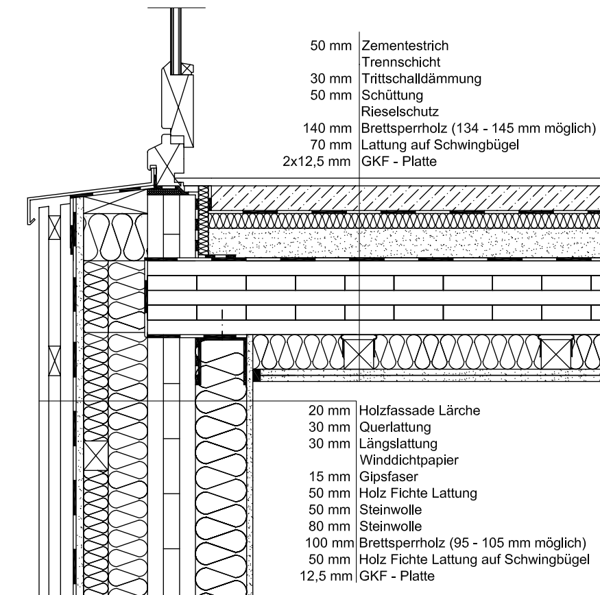
Figure 51: Example of a door connection for a French balcony
