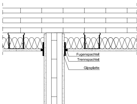
Figure 60: Connection detail of a clad cross-laminated timber wall to a suspended floor construction following [ÖNORM B 2320]
