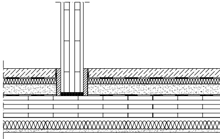
Figure 63: Lead edge insulating strip to the raw floor
