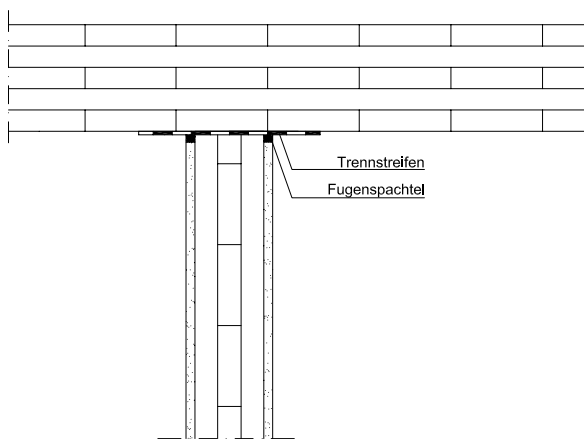
Figure 59: Connection detail of a clad cross-laminated timber wall to a floor construction following [ÖNORM B 2320]
