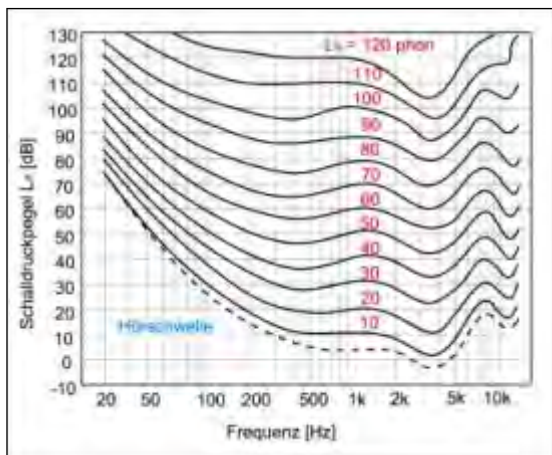
Figure 11: Curves of equal volume
