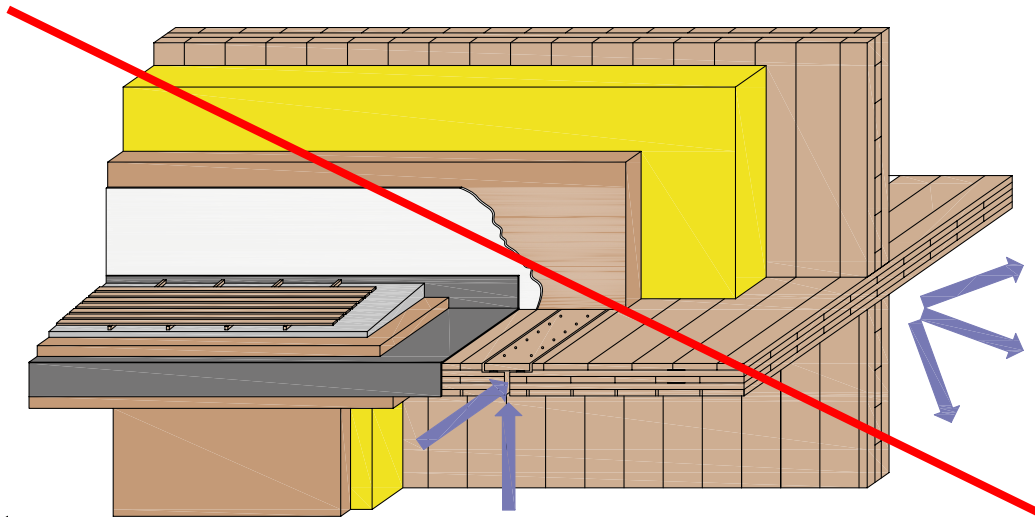
Figure 105: Schematic representation of continuous balcony slabs
