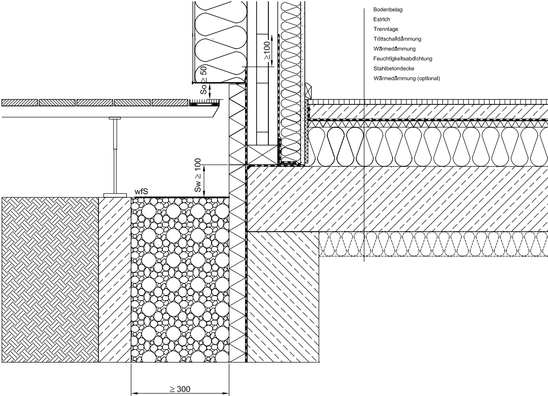
Figure 44: Detail of terrace connection
