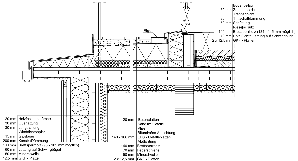
Figure 109: Terrace with recessed building shell
