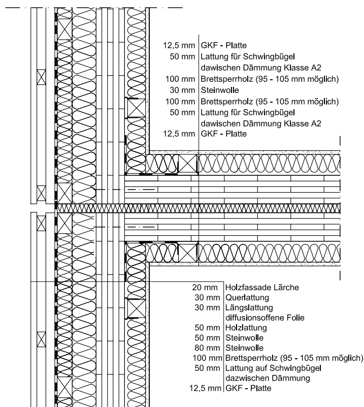
Figure 66: Connection of a fire compartment forming partition wall to an external wall. The external wall should have a fire resistance of 90 minutes at a point of 0.5 m away from the axis of the fire compartment forming wall
