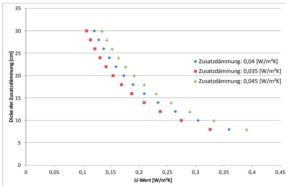
Figure 23: U values of a 8 cm thick cross-laminated timber wall ( \lambda : 0.13 W/m 2 K) as a function of thickness and heat conductivity of additional insulation
