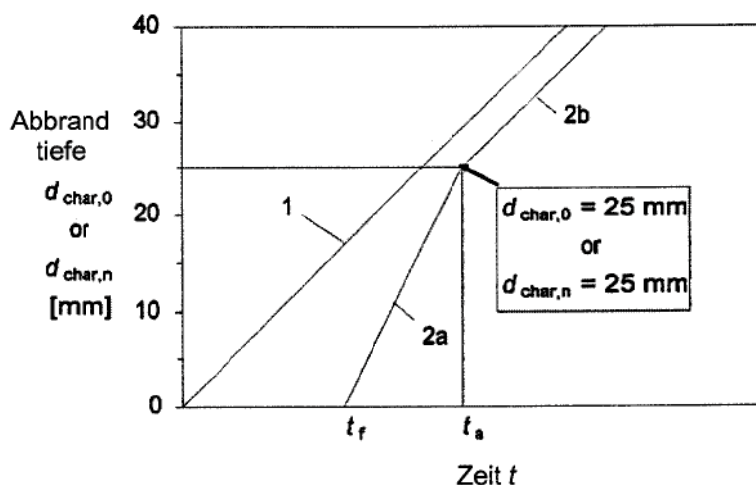
Figure 4: Representation of increased charring depth of another layer if the carbon layer of the top (2a) falls off, reduced combustion if a carbon layer of 25 mm is formed (2b) and of constant burn-off without flaking off of the carbon layer (1), source: [ÖNORM EN 1995-1-2]
