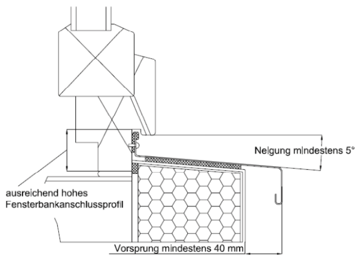
Figure 48: Window sill connection with sufficiently high window sill connection profile with at least 5° window sill inclination and a minimum façade overhang of 40 mm, source: [Österreichische Arbeitsgemeinschaft Fensterbank]
