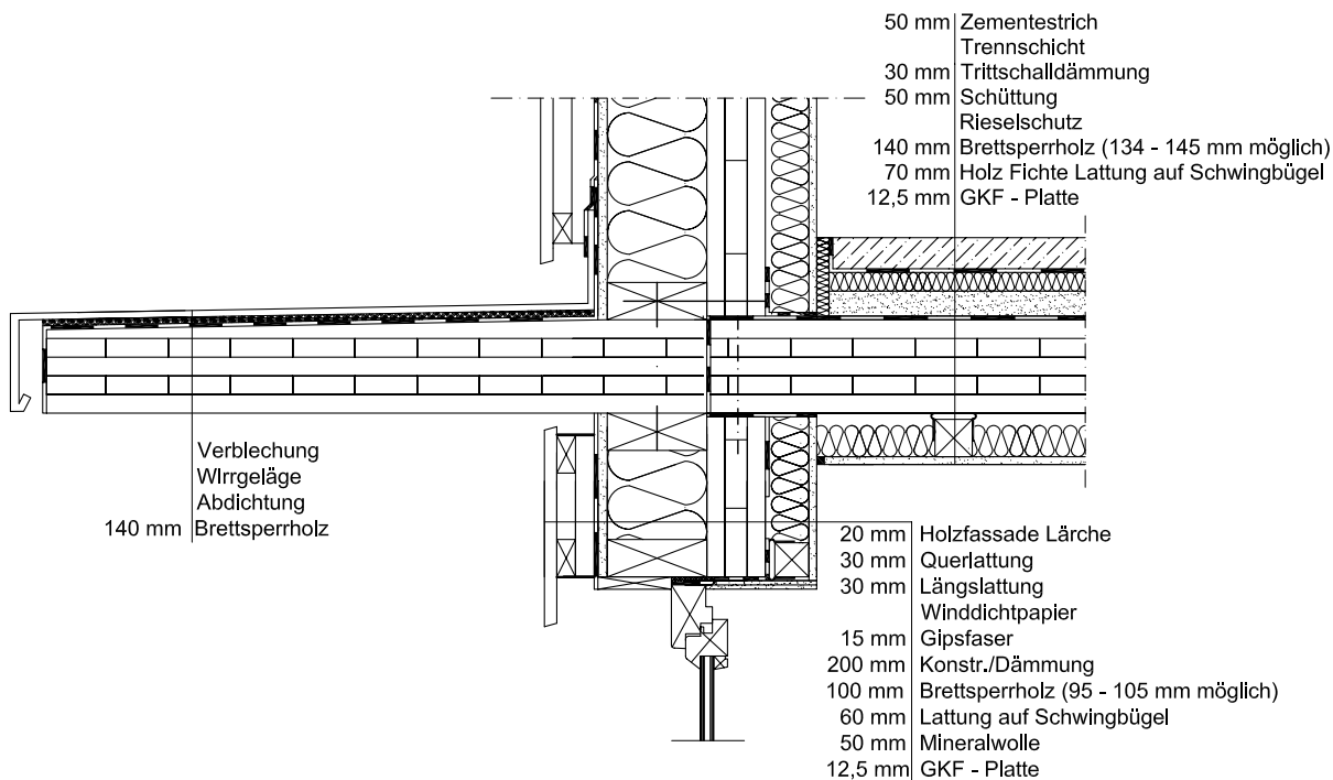
Figure 68: Exemplary connection of a fire compartment forming separation floor to the external wall (80 cm overhang)
