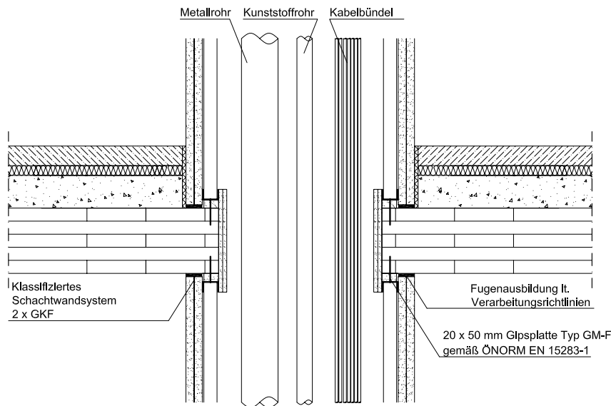
Figure 73: Exemplary design of a penetration of shaft type A for a solid timber floor
