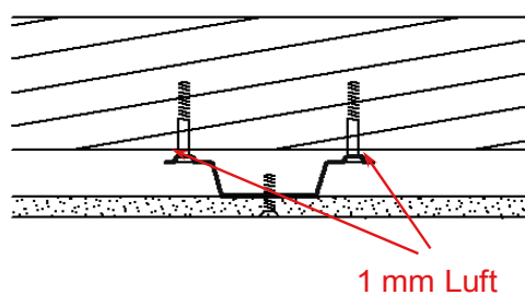
Figure 33: Schematic represented of the mounting of a decoupled suspension, source: [Holtz et al. 1999b]
