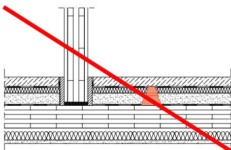
Figure 39: Faulty installation of screed film created a direct connection between screed and raw floor
