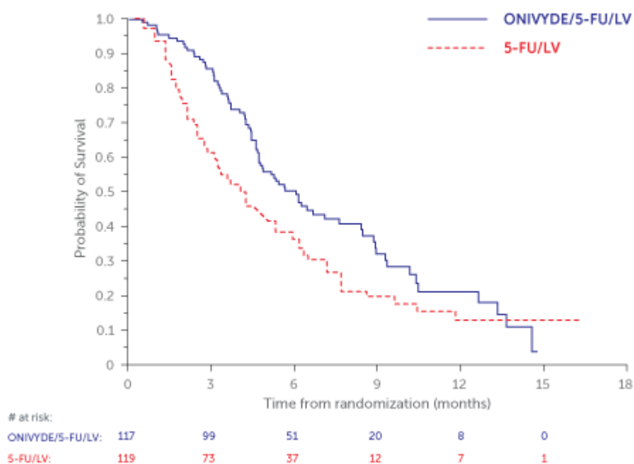
Figure 1: Overall Survival
