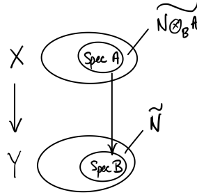
FIGURE 16.1. The pullback of a quasicoherent sheaf (module-theoretically)
