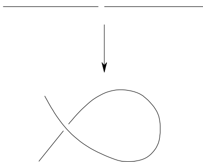
FIGURE 19.1. The projectivity hypothesis in Theorem 19.1.1 cannot be dropped
