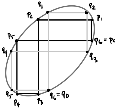
FIGURE 19.9. Exercise 19.10.I (with 17 replaced by 3)
