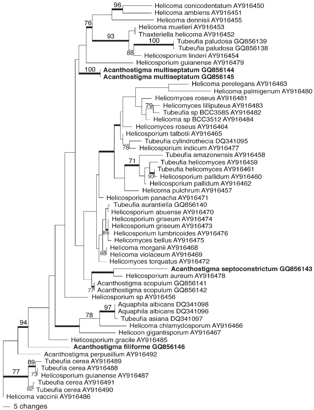
FIG. 25. Tubeufiaceae phylogeny of one of 111 most parsimonious trees generated from a MP analysis of ITS sequence data for 56 taxa showing the phylogenetic placement of five Acanthostigma species within the family ( L = 705.76 steps, CI = 0.456 , RI = 0.738 , RCI = 0.337 ). The three newly described species are in boldface. Thickened branches indicate Bayesian posterior probabilities \geq 95\% , while numbers above or below branches refer to MP bootstrap values \geq 70\% . Helicoma vaccinii is used as outgroup.
