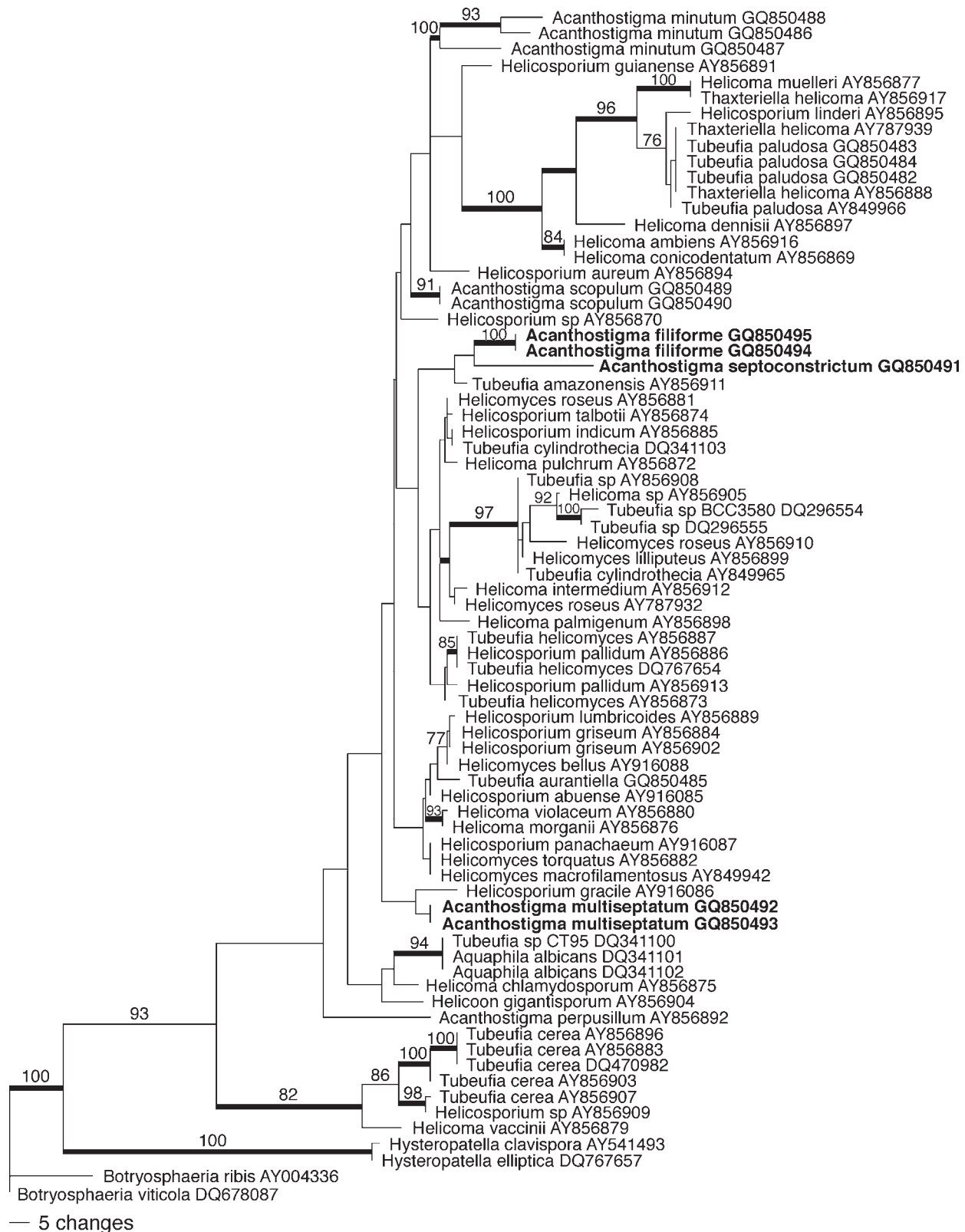
FIG. 24. Tubefiaceae phylogeny of one of 33 most parsimonious trees generated from a MP analysis of LSU sequence data for 75 taxa showing the phylogenetic placement of six Acanthostigma species within the family ( L = 590.91 steps, CI = 0.550 , RI = 0.840 , RCI = 0.462 ). The three newly described species are in boldface. Thickened branches indicate Bayesian posterior probabilities \geq 95\% , while numbers above or below branches refer to MP bootstrap values \geq 70\% . Two species of Hysteropatella and two species of Botryosphaeria are outgroups.
