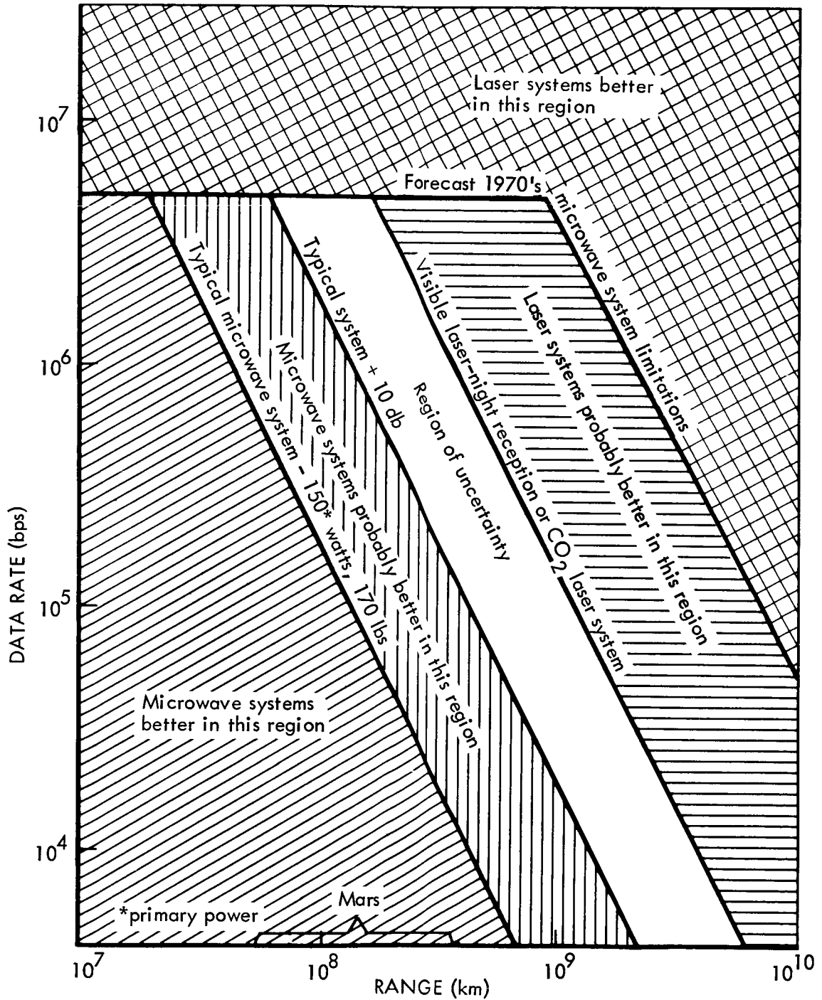
Figure 7.3-3: COMPARATIVE PERFORMANCE OF RF AND LASER DEEP SPACE COMMUNICATIONS SYSTEMS FOR THE MID-1970'S
