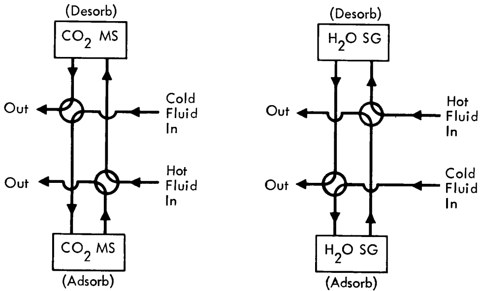
Figure B-1: CO 2 REMOVAL — MOLECULAR SIEVES
