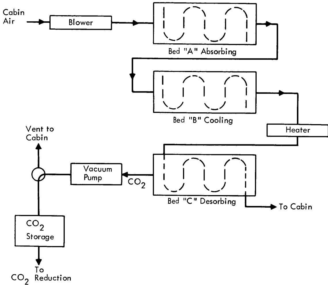
Figure B-3: CO 2 REMOVAL — SOLID AMINES
