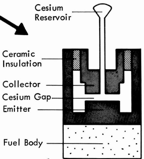
Thermionic Converter
