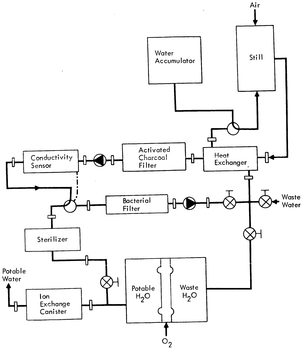
Figure D-3: VACUUM COMPRESSION DISTILLATION SYSTEM SCHEMATIC
