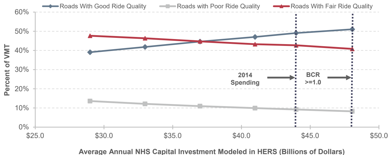
Exhibit 10-11: Projected Impact of Alternative Investment Levels on 2034 Pavement Ride Quality Indicators for the National Highway System
