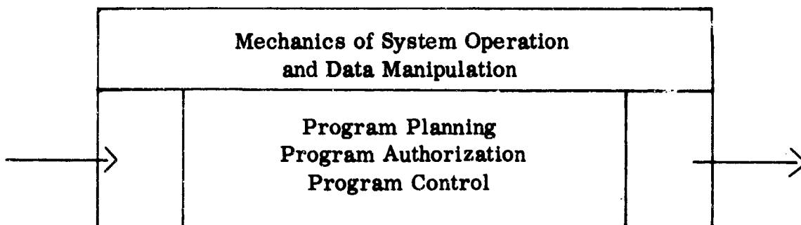
Fig. 1. Program Model
