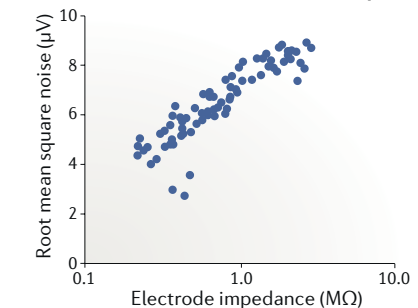
c Electrode noise vs electrode impedance
