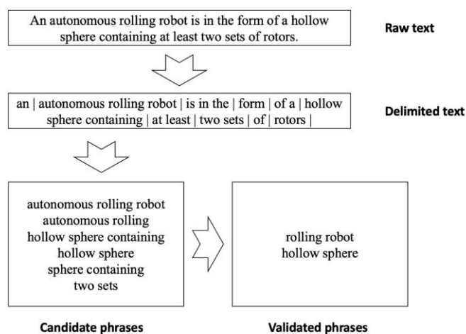
Figure 2. An example run of phrase extraction process
