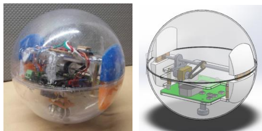
Figure 4. An example SRR (courtesy of Weng Ho Lok, Jin Sen Tan, Paiputra Fleming, Huishan Tan and Cheng Yuen Ong in the SUTD engineering design innovation class in 2015)
