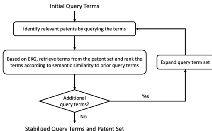
Figure 1. Overall framework for data-driven keyword based patent search
