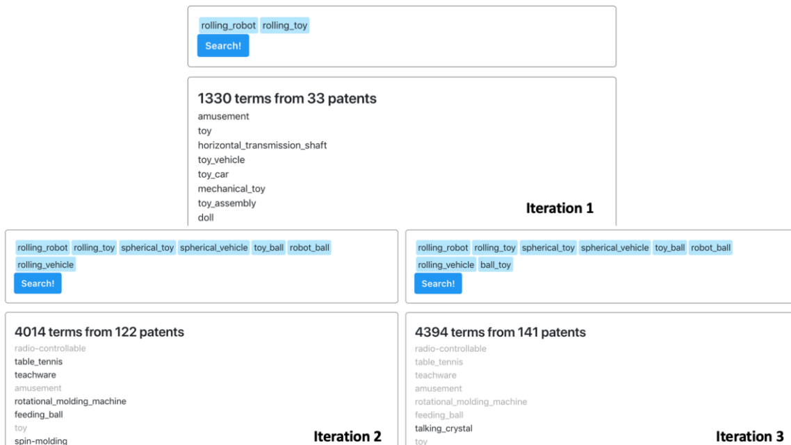
Figure 3. Screenshots from the keyword discovery and patent retrieval tool. Candidate keywords found in prior iterations are in grey, whereas new keywords are in black
