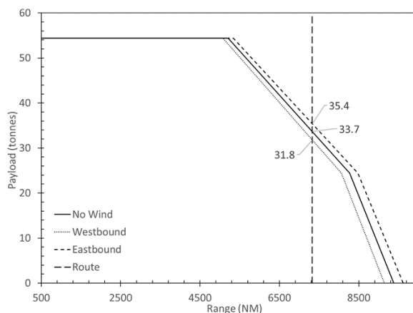
Figure 4. Payload range diagram of the Boeing 787-9, with 3 curves for the no wind condition, westbound, and eastbound. The mission range between Singapore (SIN) and San Francisco (SFO), and the corresponding mission payloads are marked
