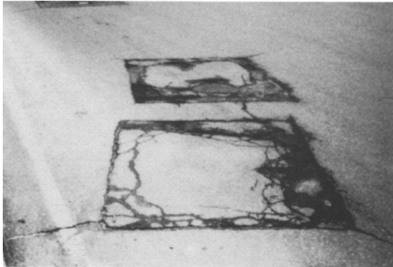
Failure by water intrusion
