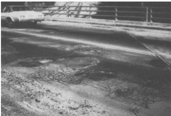
Bridge deck failure
